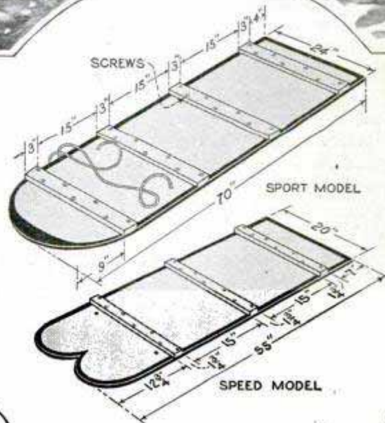
Right. Constructional Details of the "Water Sprites" or Aquaplanes; Above, Aquaplanes in Action.
