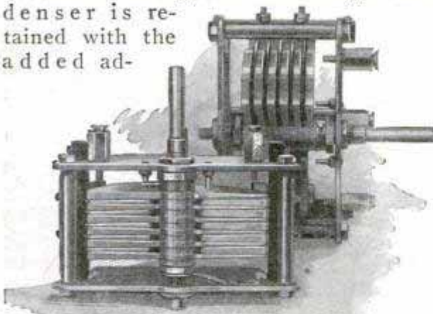
Side View Showing Wedge-Shaped Rotor and Stationary Plates
