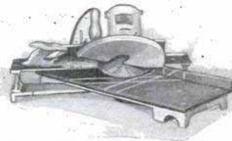
Illustrating Four Uses of the Outfit; Driving a Bit, Cutting a Groove, Operating Straight-Blade Saw, and in Miter Box
