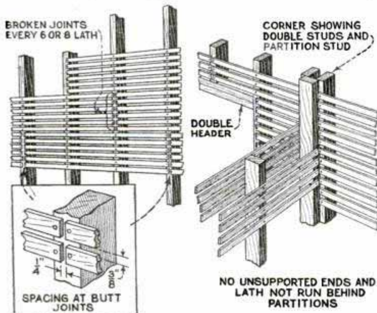
Proper Method of Applying Lath and Supporting It at Corners
