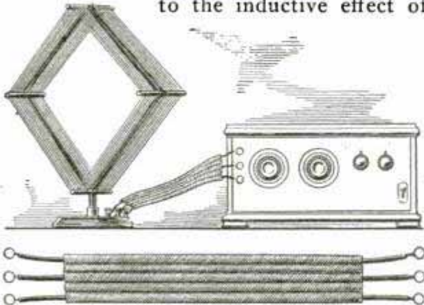
Loop Leads Are Threaded through Webbing to Prevent Induction and Improve Appearance
