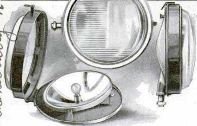
Upper Photo Shows Both Side and Front Illumination Afforded by the Headlight; Details of the Lamp Below
