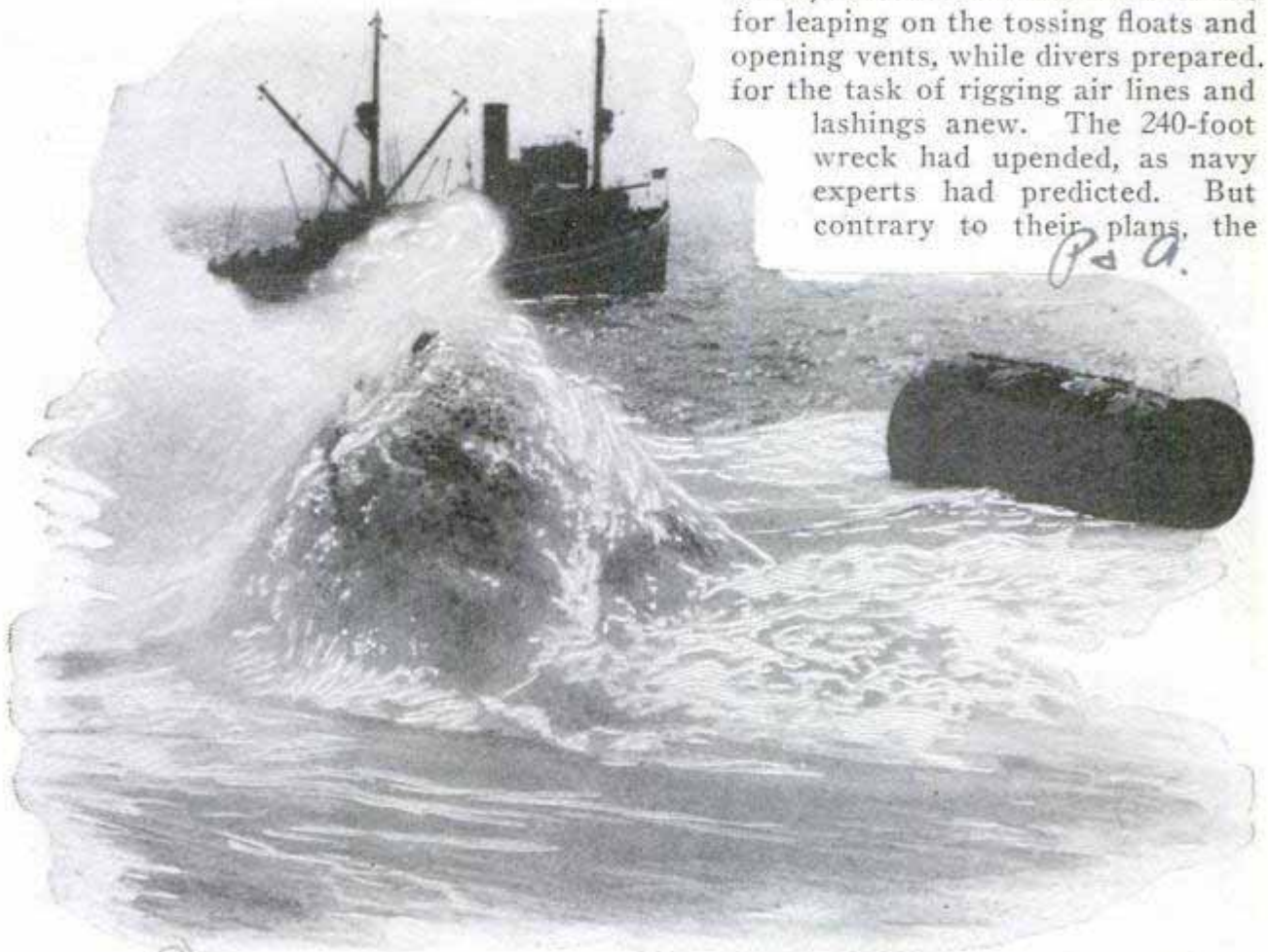
Why the "S-51" Slipped Back after the First Raising; Pontoons Lashed to the Stern Broke Loose and Leaped to the Surface; Photo Shows One Coming Up
