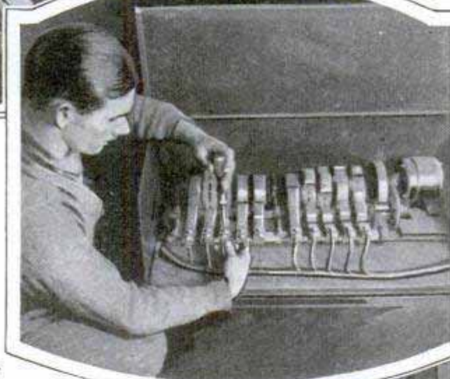
The Making of Electric Signs Is a Highly Skilled Profession; Center Shows a "Flasher" Assembly for an Animated Advertisement
