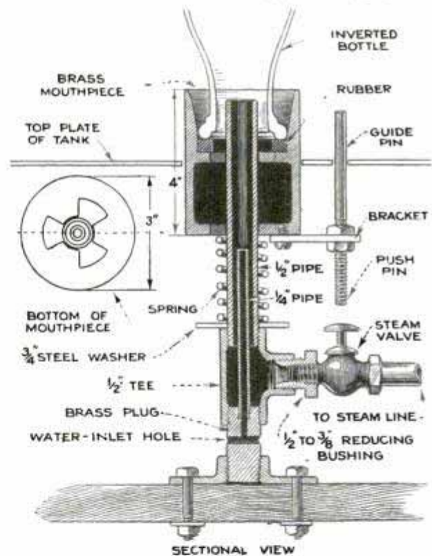
SECTIONAL VIEW Inexpensive Milk-Bottle Washer Lightens Labor on Small Dairy Farm
