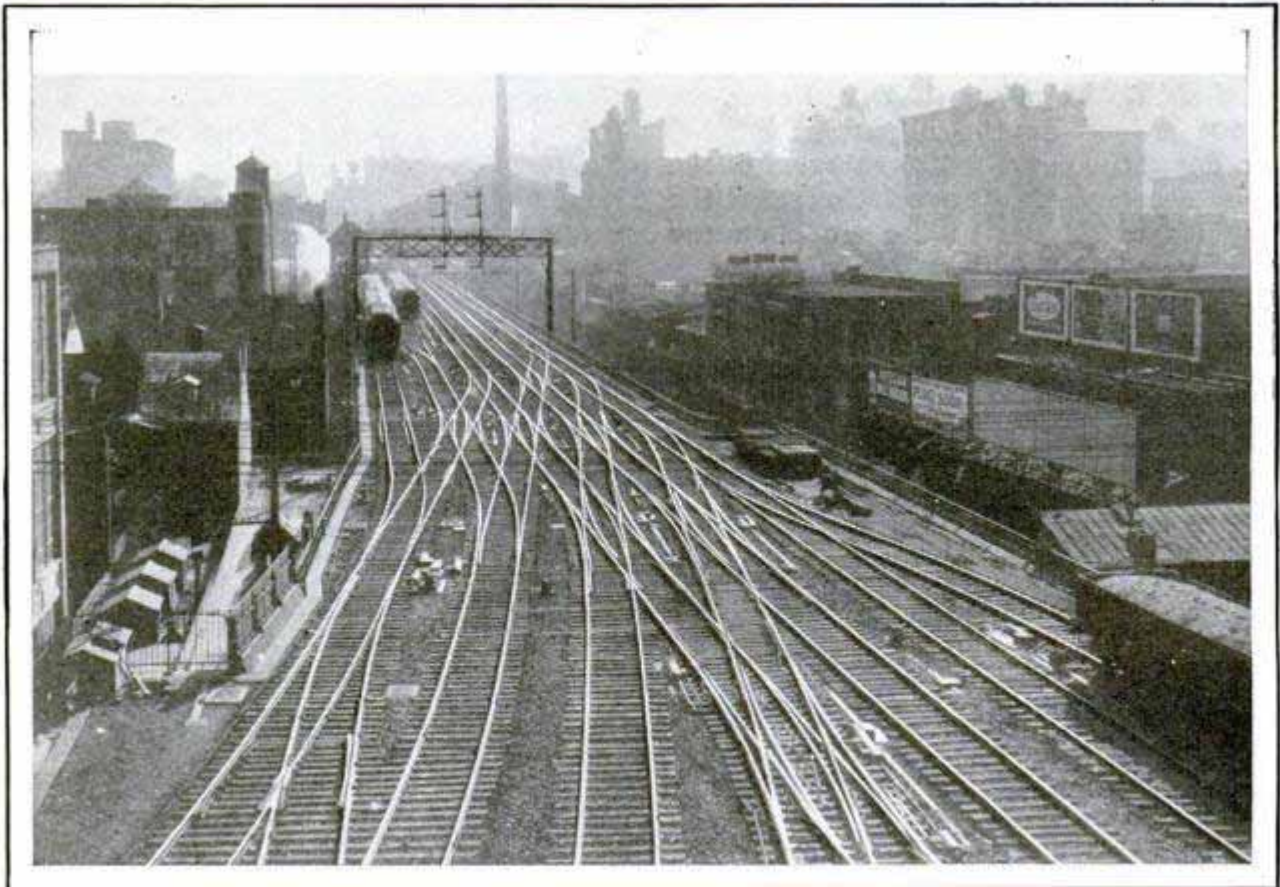
Electric Interlocking Signals Control the Network of Tracks Leading Out of the Terminal and Guide the Trains over the Route Designated by the Dispatcher's Office
