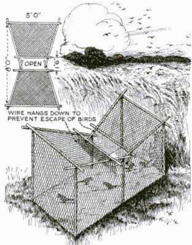
An Effective Crow Trap Which Can Be Made of Old Poles and Poultry Mesh
