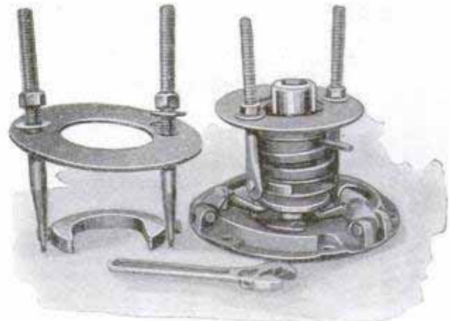
Spring Compressor for Ford Clutch Simplifies Task of Removing Spring
