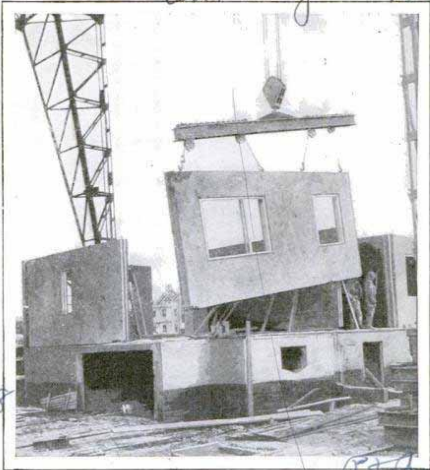
Where Derricks Serve as Masons: Lowering Side of Concrete House as Unit to Foundation during Rapid Construction
