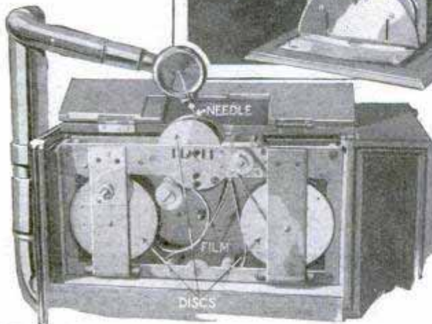
Views of the Film-Record Phonograph Showing the Winding Reels and Position of Needle
