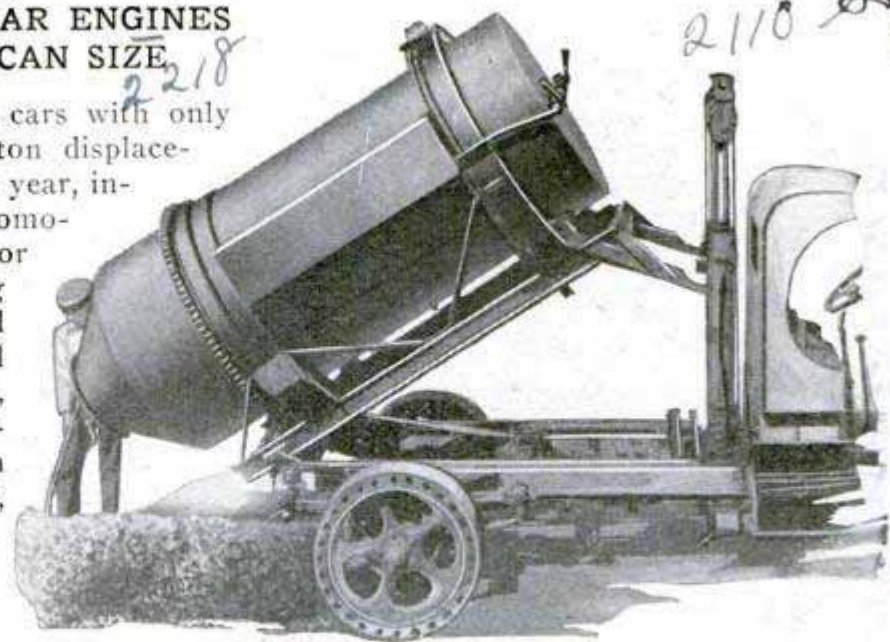
Truck Body Raised to Dump Contents of Mixer, Which Is Turned by Power from the Motor
