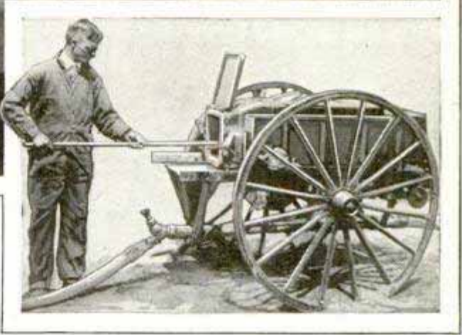
Conquering the Blazing Pool of Oil with Stream of Foam, and Close View of the "Gun"
