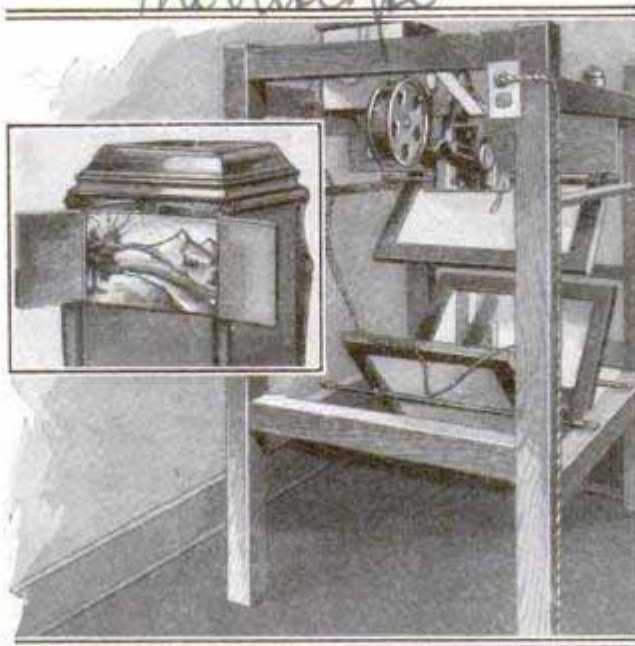
Interior of Motion-Picture Cabinet, with Inset Showing How Film Appears during Operation
