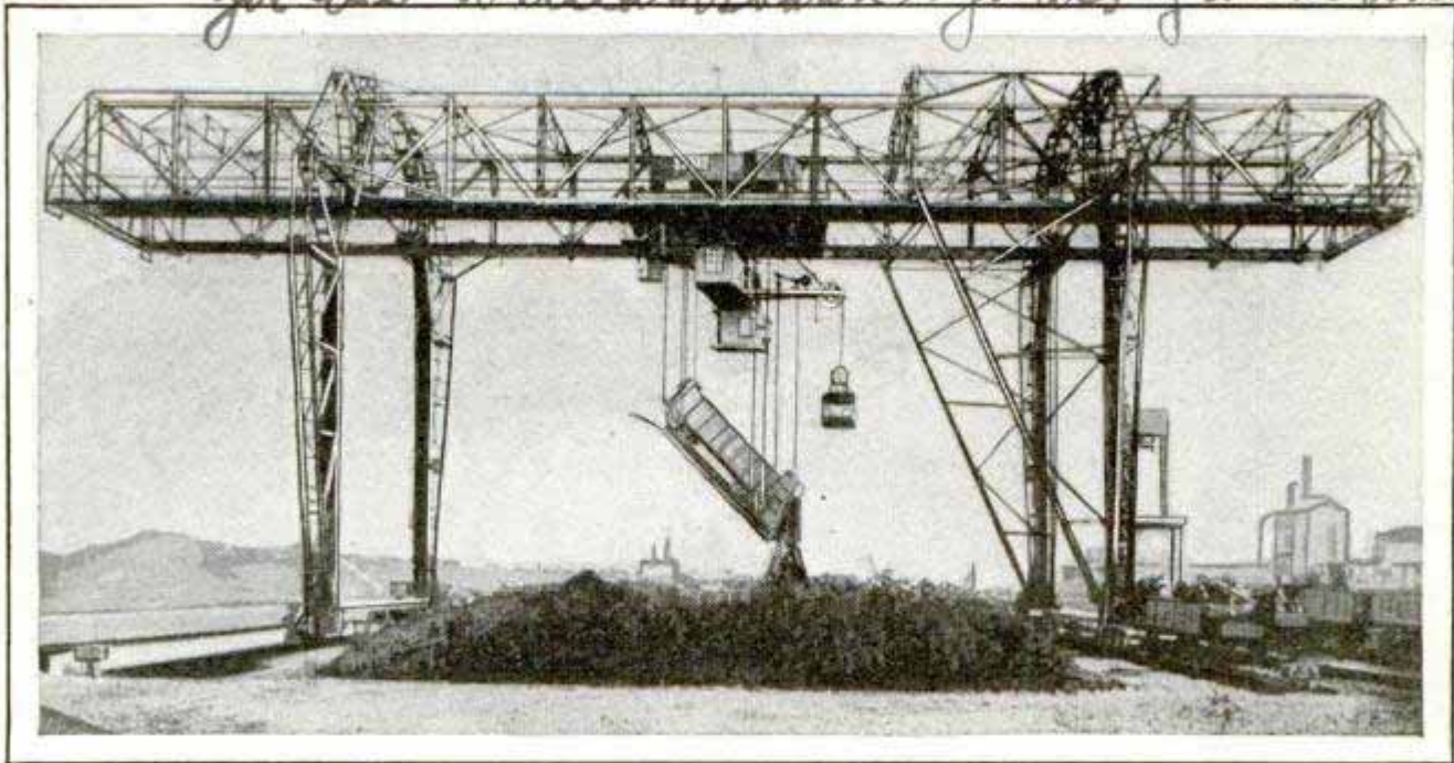
Powerful Coal Unloader in Operation; Cars Are Lifted from the Tracks, Moved to the Dumping Heap and Then Tipped, Permitting the End Gate to Open and the Contents to Run Out
