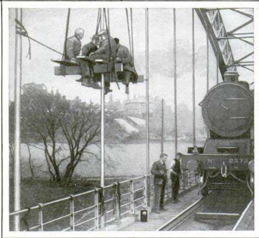
Testing Strain on Bridge While Engine Is Run over It; Observers on Platform Study Stresses with Aid of Special Instruments
