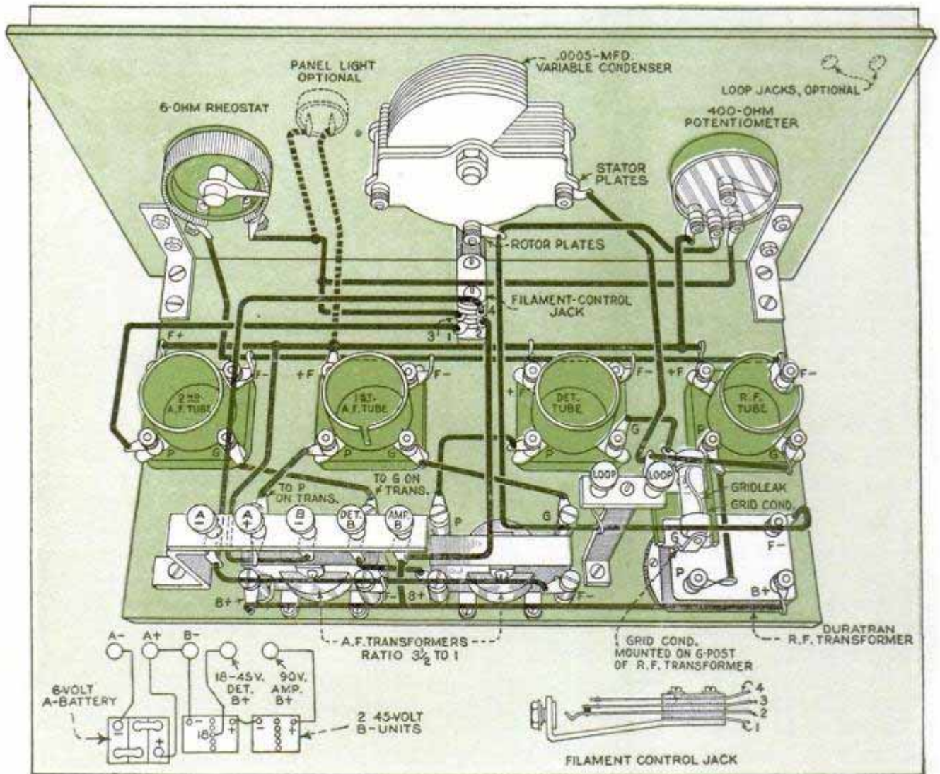
Wiring Diagram Showing Lugs under All Terminals to Be Soldered; Below, Battery Connections and Details of Filament-Control Jack
