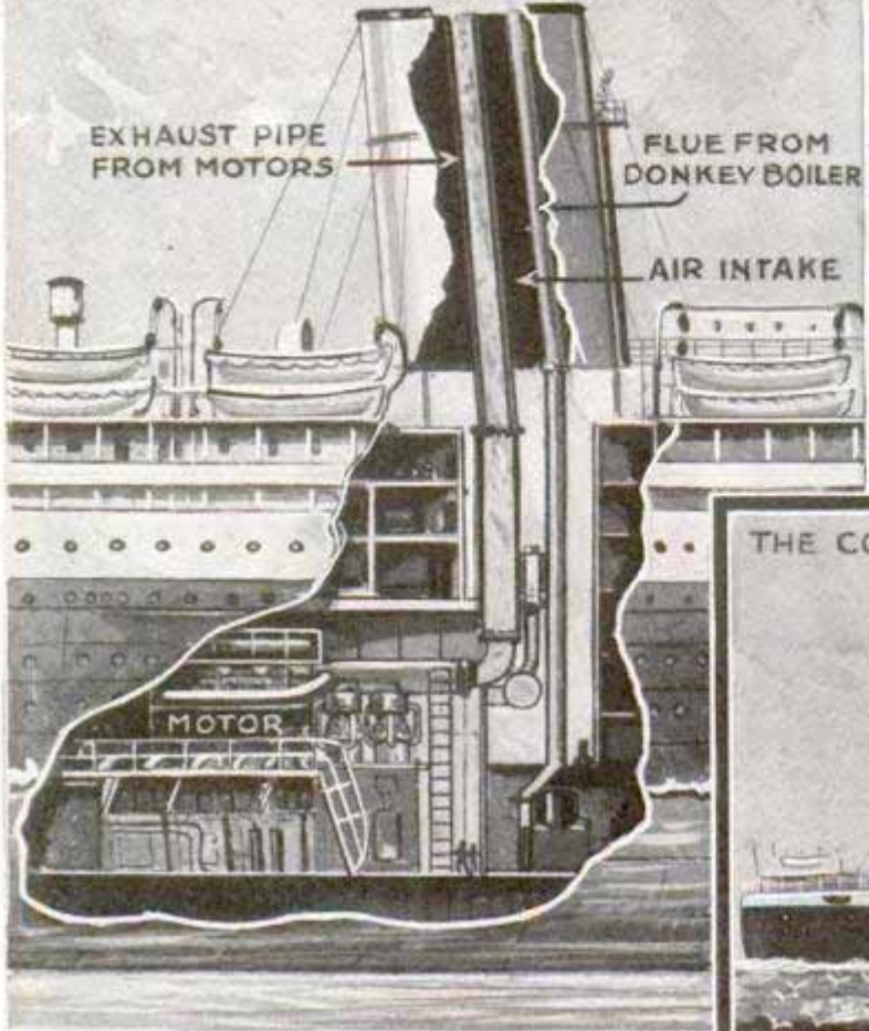
SPACE OCCUPIED BY MACHINERY IN A FUNNEL-LESS SHIP
