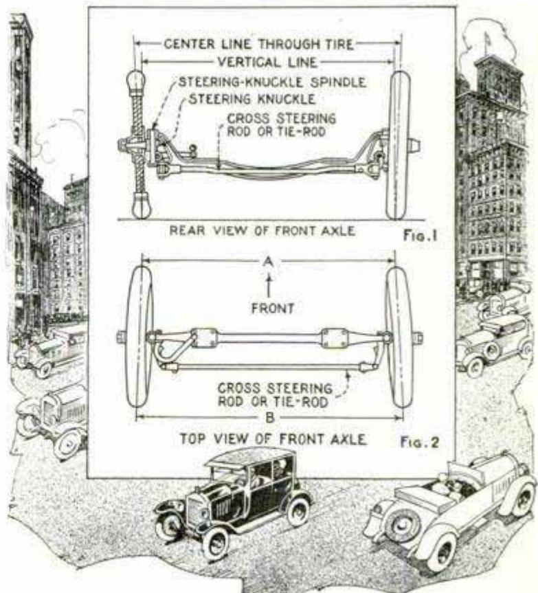
Rear View and Plan of Front Axle, Illustrating What Is Meant by "Camber" and "Toe-In" on the Front Wheels of the Car
