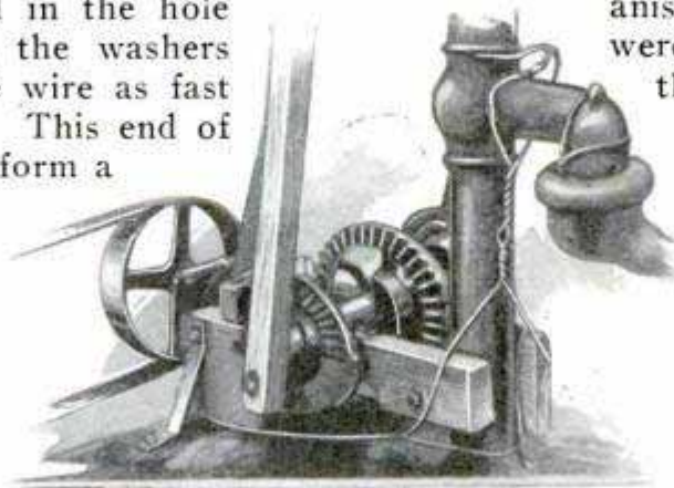
Efficient Pump Jack Made from Old Binder Parts Gives a 6-Inch Stroke
