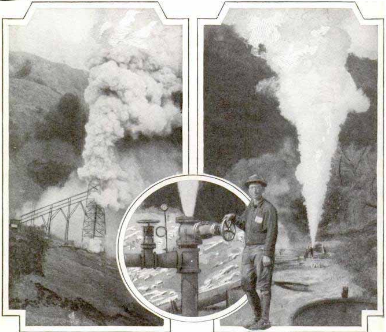
Scenes at California's Natural Power Plant Where Man Has Tapped and Harnessed a Subterranean Steam Supply; Pressure of 276 Pounds Was Developed at One of the Wells
