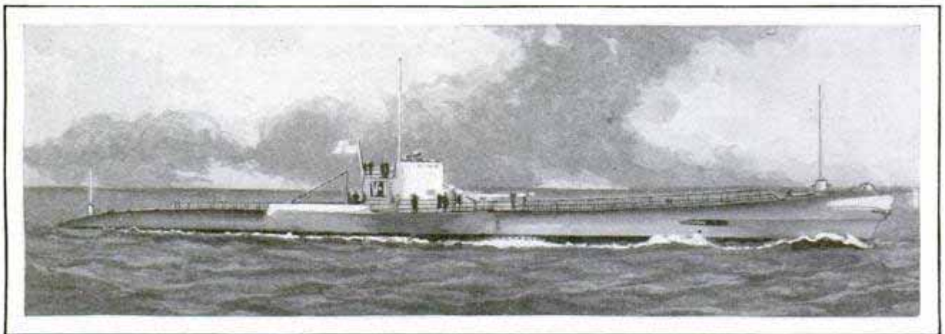
One of America's Biggest Fleet Submarines, the "V-1," Which Recently Established a World's Record by Submerging to a Depth of 220 Feet; on the Surface, It Is as Fast as a Battleship
