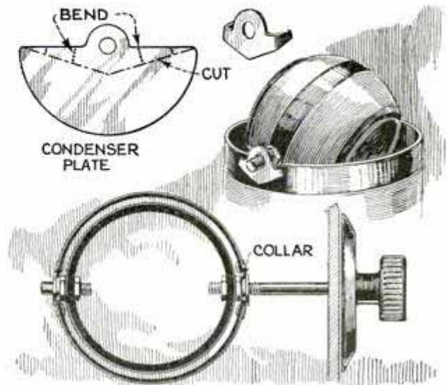
Mounting Collar for Rotor Unit Is Cut from Old Variable-Condenser Plate
