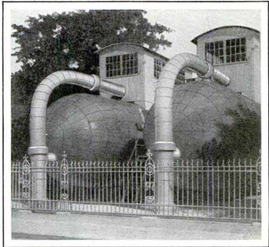
Where Reserve Steam Power Is Held for Swedish City When Hydroelectric Plant Fails; the Two Accumulators
