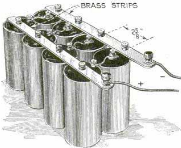
Dry Cells Connected in Parallel Series, Showing Brass Strips Used for the Parallel Connections
