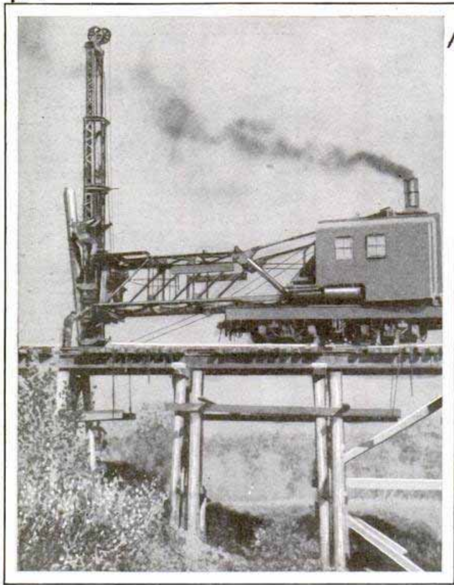
Combination Outfit in Use as a Pile Driver; It Can Easily Be Converted into a Crane for Heavy Lifting
