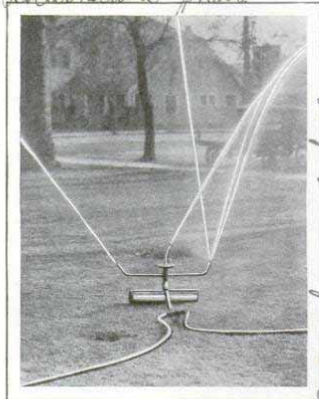
Sprinkler Nozzles on Cylinder Are Easily Moved by Pulling Hose without Danger of Upsetting Them
