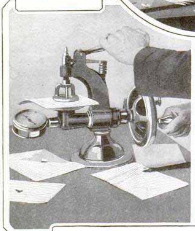
Applying the Bursting Test; Pressure of Glycerin Expands the Rubber Diaphragm Pressed against the Sample, Finally Causing the Paper to Break
