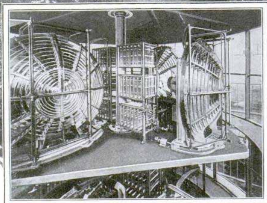
View of the Lighthouse on Mt. Afrique, Where It Is Visible to Aviators over a Wide Area, and Interior of the Lamp Room, Showing the Reflectors
