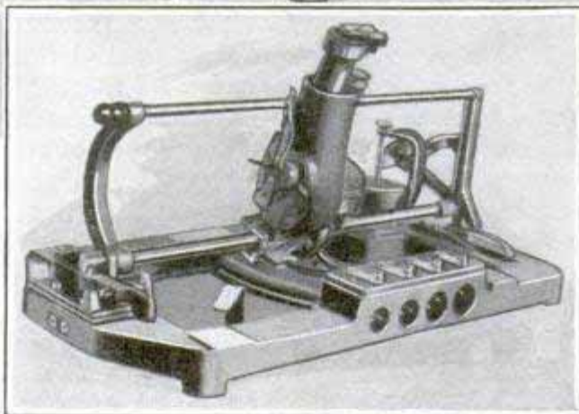
Blind Man Reading as Type Is Translated into Sound; the Perforated Disk and Instrument Uncovered
