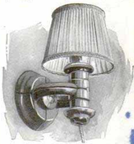
Various Lighting Effects Are Possible with This Perpendicular Lamp Bracket, and Socket at Bottom Affords Extra Connection for Cord or for Another Bulb
