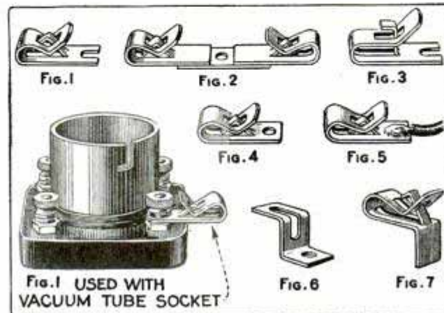
Clips from Discarded B-Batteries Make Handy Connectors for the Experimental Hookups
