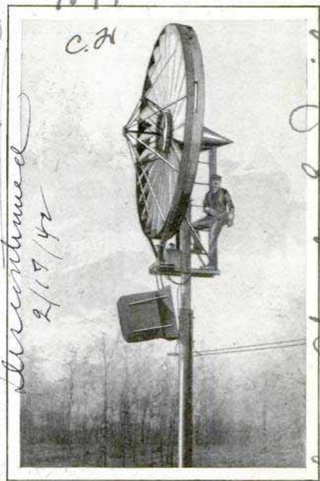
Indiana Farmer's Homemade Windmill Plant Which Generates Current for Lighting and Power
