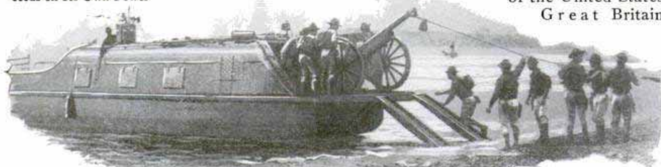
Submarine Dashing Shoreward with Amphibian Tank on Back; When the Sub Goes Down the Tank Proceeds on Its Own Power
