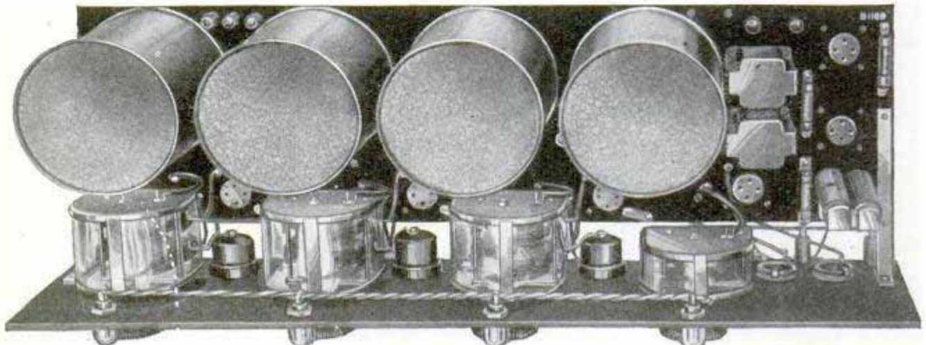
Interior View of the Set, Showing "Canned" Coils and General Layout of the Receiver; Notice the Panel Lights over Each Dial to Make Tuning Easier in Dim Light
