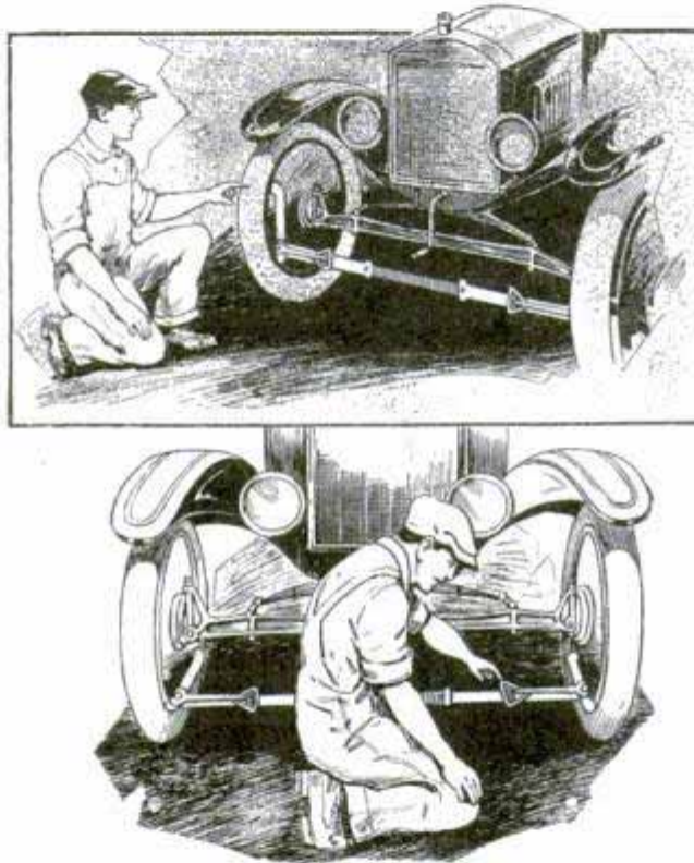
Above, Checking the Camber of the Wheels with Special Gauge; Below, Checking Toe-In
