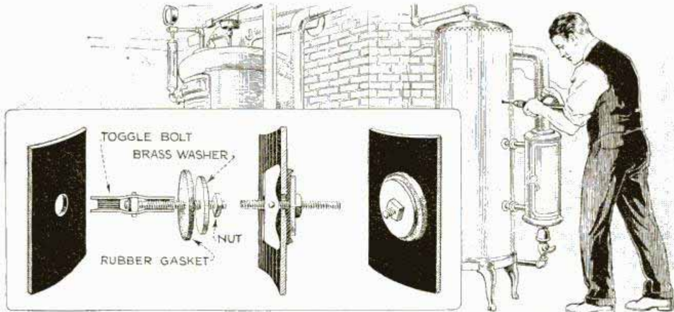
Simple Repair for the Leaky Range Boiler or Tank, Employing Only a 5-Cent Toggle Bolt, a Brass Washer and a Rubber Gasket
