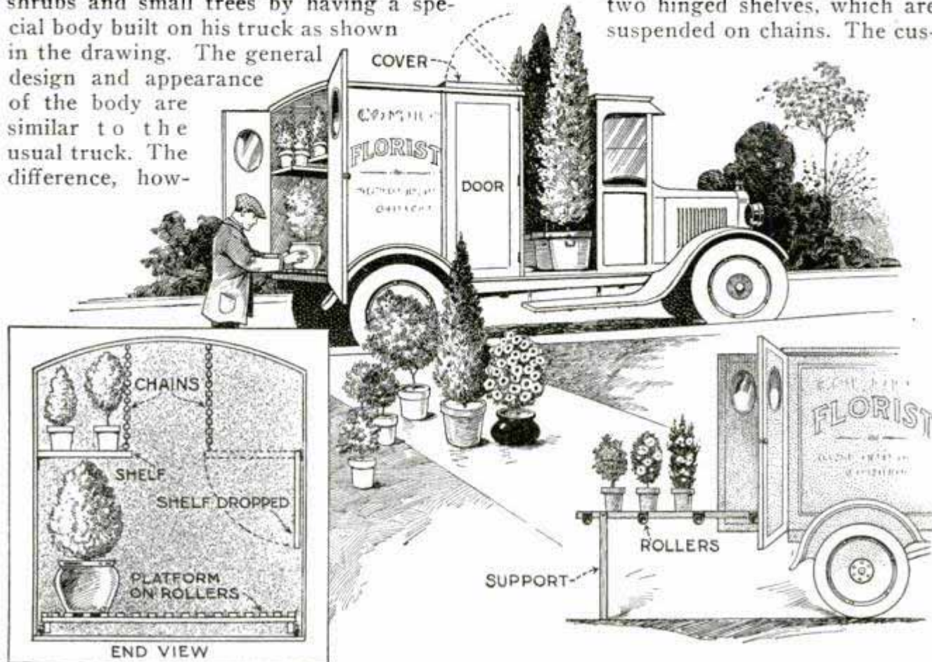
Specially Built Body on Florist's Truck Accommodates All Kinds and Sizes of Plants and Shrubbery Conveniently and a Rolling False Bottom Facilitates Loading
