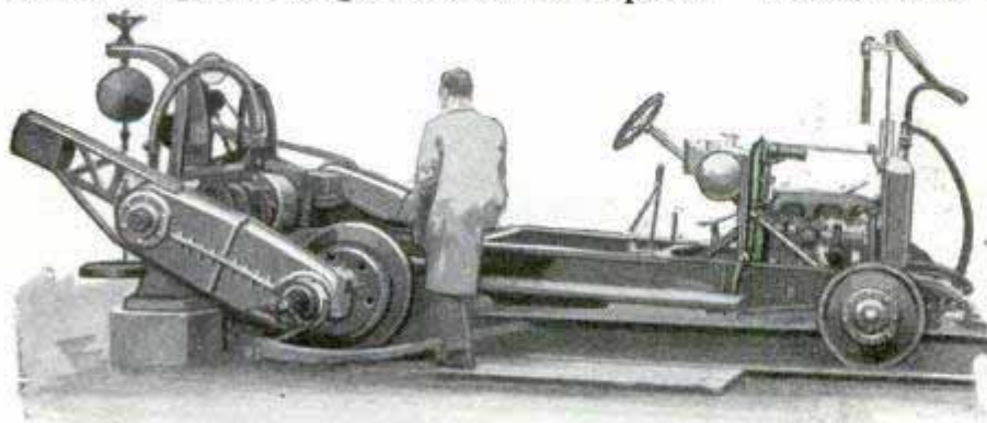
Giving Auto Chassis Road Test, While It Remains Stationary; Performance on Grades Is Easily Checked
