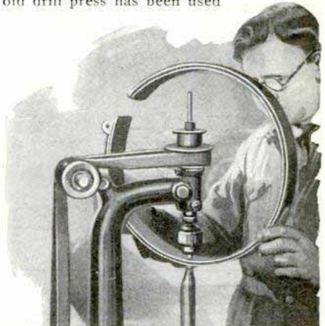
Homemade Machine for Drilling and Countersinking Rivet Holes in Auto Brake Bands
