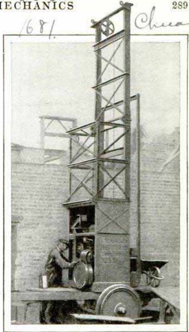
Contractor's Portable Hoist in Operation; It Can Be Moved Quickly to Any Part of the Job
