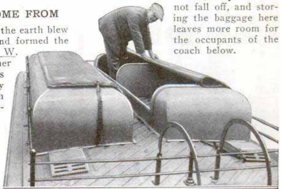
Baggage Compartments on Top of Motor Coach Have Tight-Fitting Covers to Keep Off Dust and Rain
