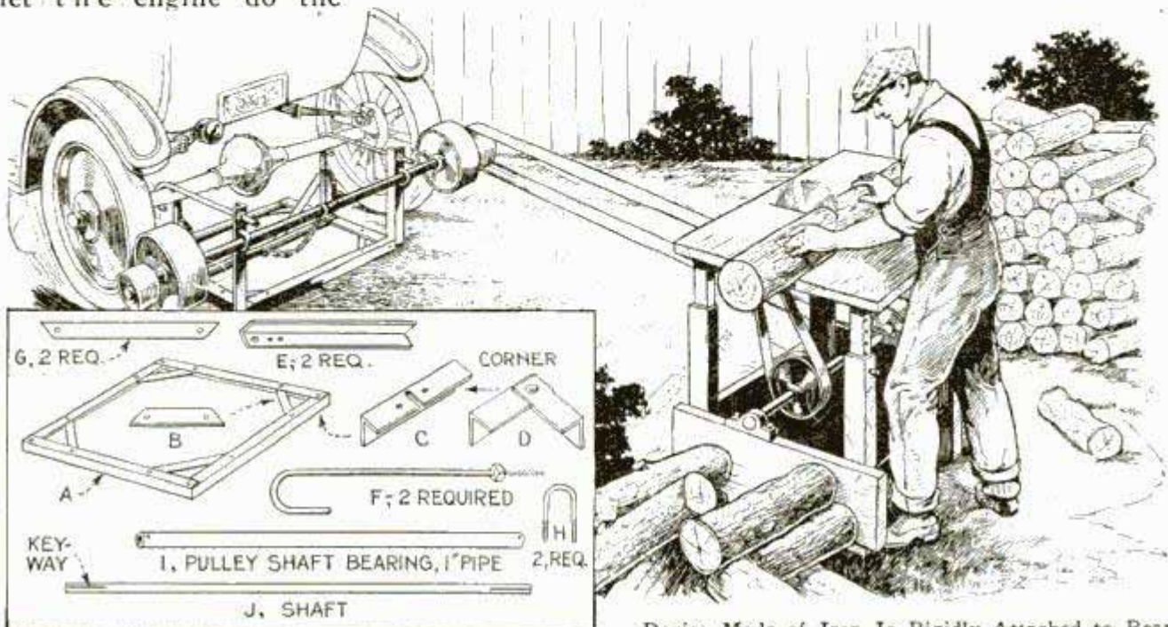
Device Made of Iron Is Rigidly Attached to Rear of Auto for Running Circular Saw
