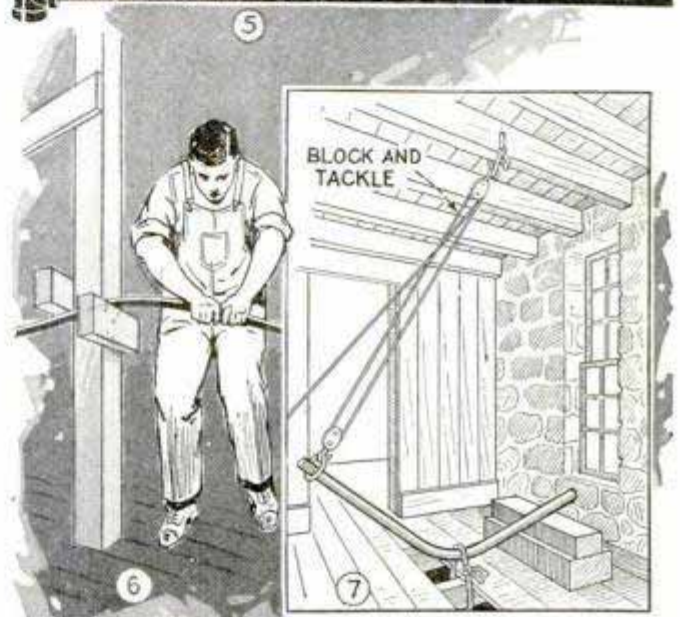
METHODS OF BENDING CONDUIT
