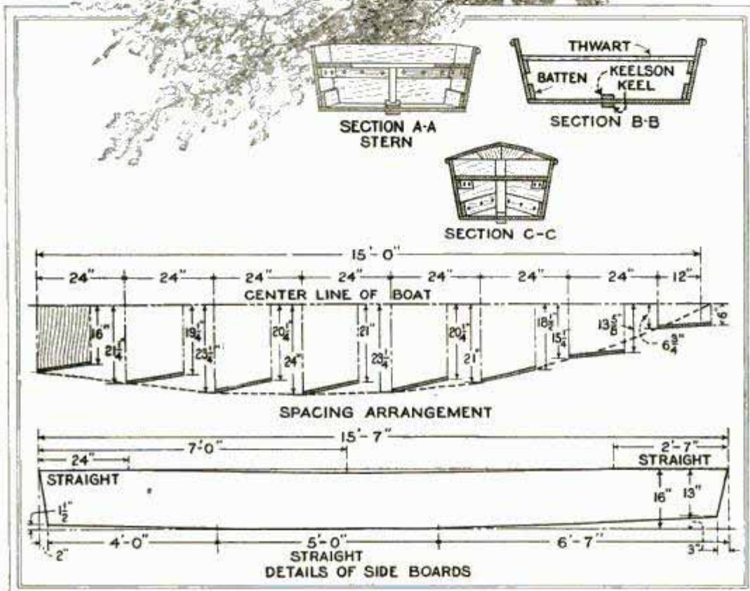
Details of Construction of the Outboard-Motor Boat. This Craft Is Simple Enough for Any Handy Man to Build, with Ordinary Tools
