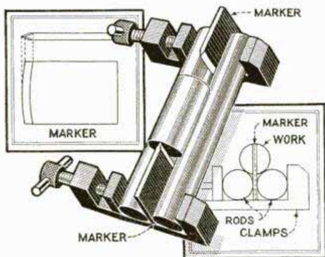
Handy Tool for Center Marking Short Round Stock Quickly and Conveniently
