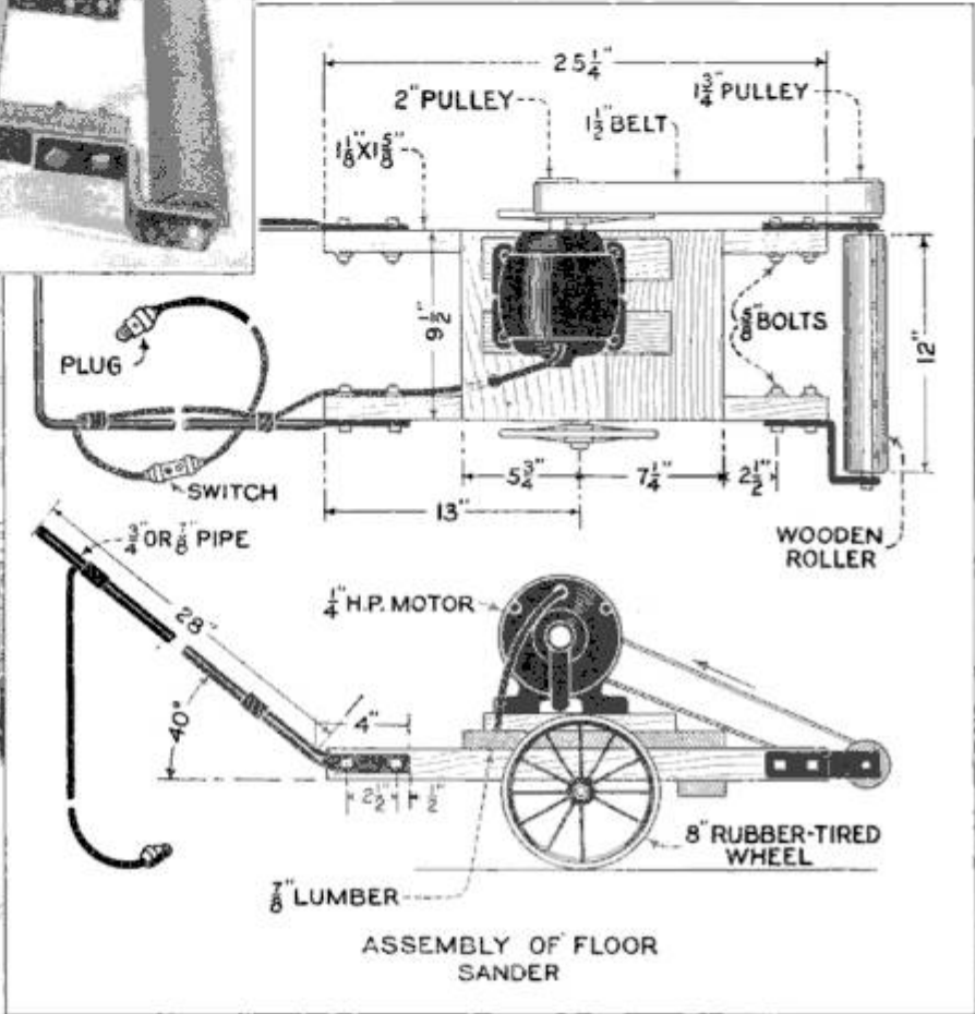
Upper Left, Photo of the Original Machine; Below, Drawings for Assembling the Sander
