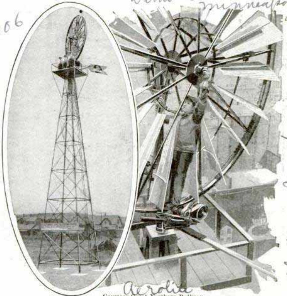
Tower and Close View of Wind Wheel Railroad Uses to Generate Current for Operating Light Signals
