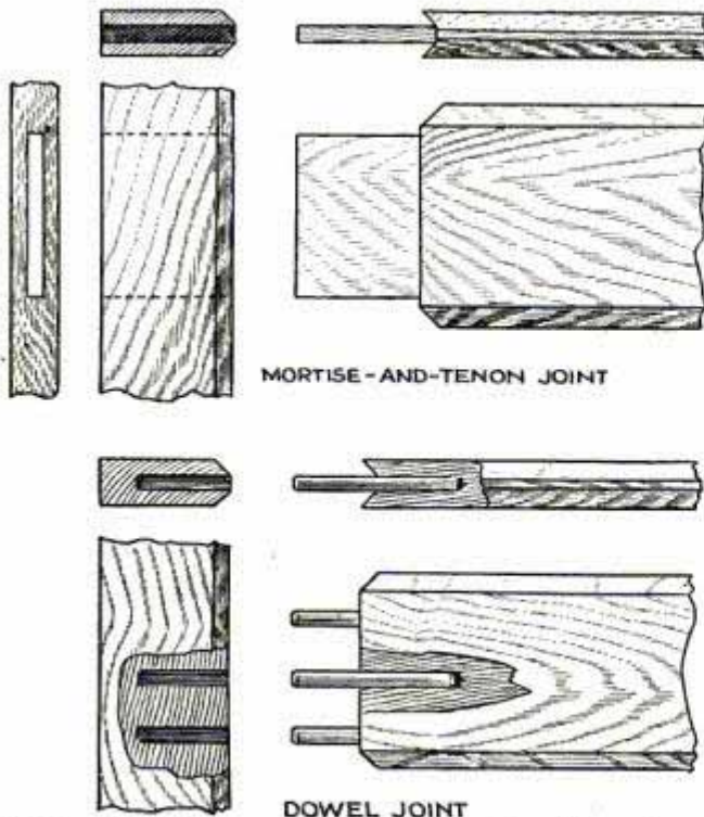
Doors with Mortise-and-Tenon Joints Are Stiffer But Swell More Than Those with Dowel Joints
