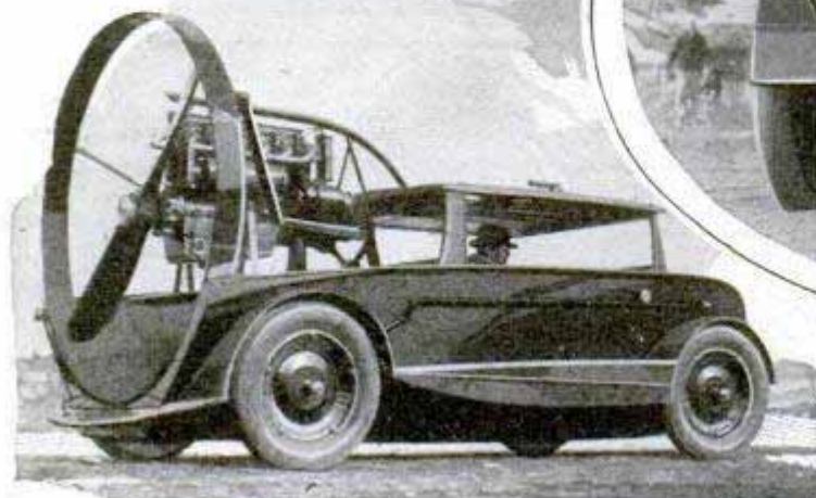
Views of Versatile Air-Driven Auto; Band over Propeller Blades Insures Greater Safety
