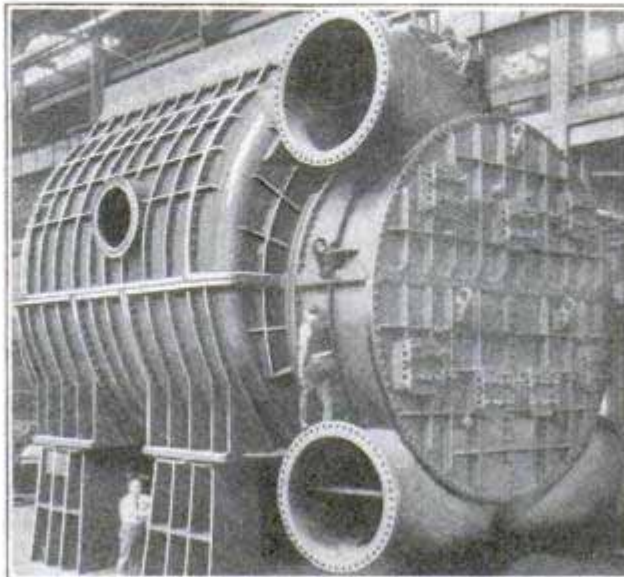
Huge Steam Condenser Weighs Nearly Million Pounds and Has Over Fifty-One Miles of Tubes
