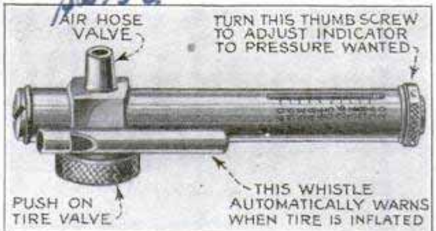
Safety Tire-Gauge Which Prevents Overinflation by Automatically Shutting Off Excess Air
