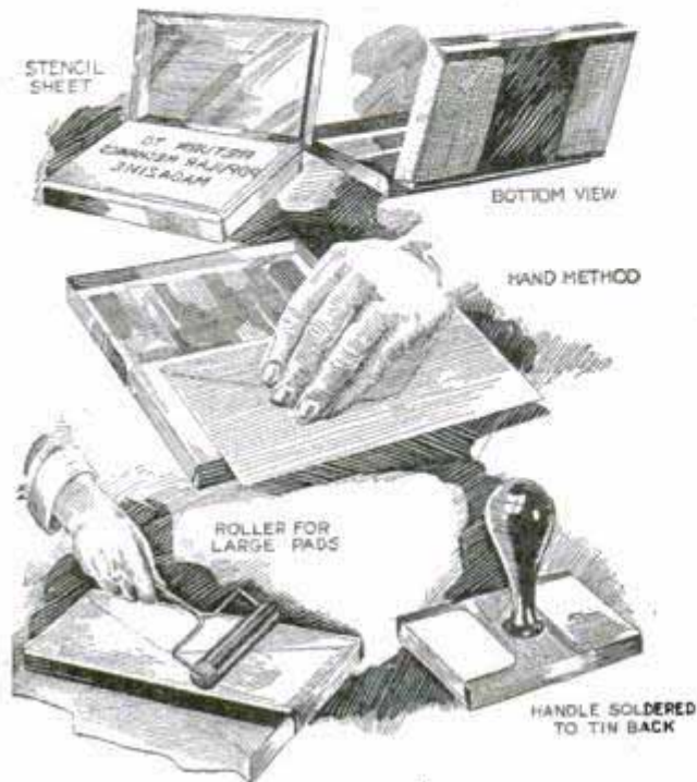
Self-Inking Stamp Made from a Mimeograph-Paper Stencil and an Ordinary Pad
