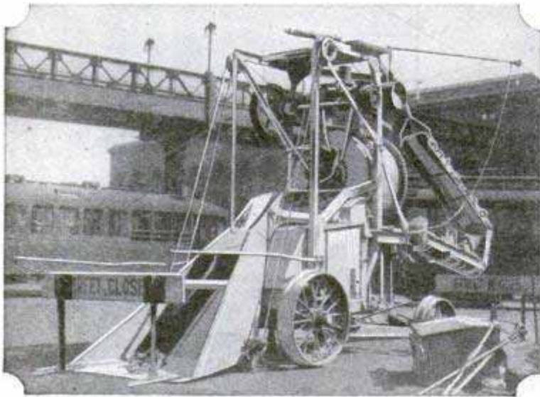
Novel Concrete Mixer That Runs on Street-Car Tracks and Uses Trolley Current
