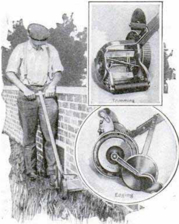
Trimmer in Side and Rear Views and in Use Flush against a Wall
