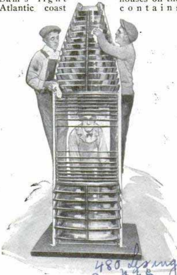
Polishing the Huge Glass Lighthouse Lens; Pieces Are Set to Intensify and Focus the Rays
