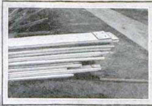
Shingles Nailed to Planks Prevent End-Splitting
