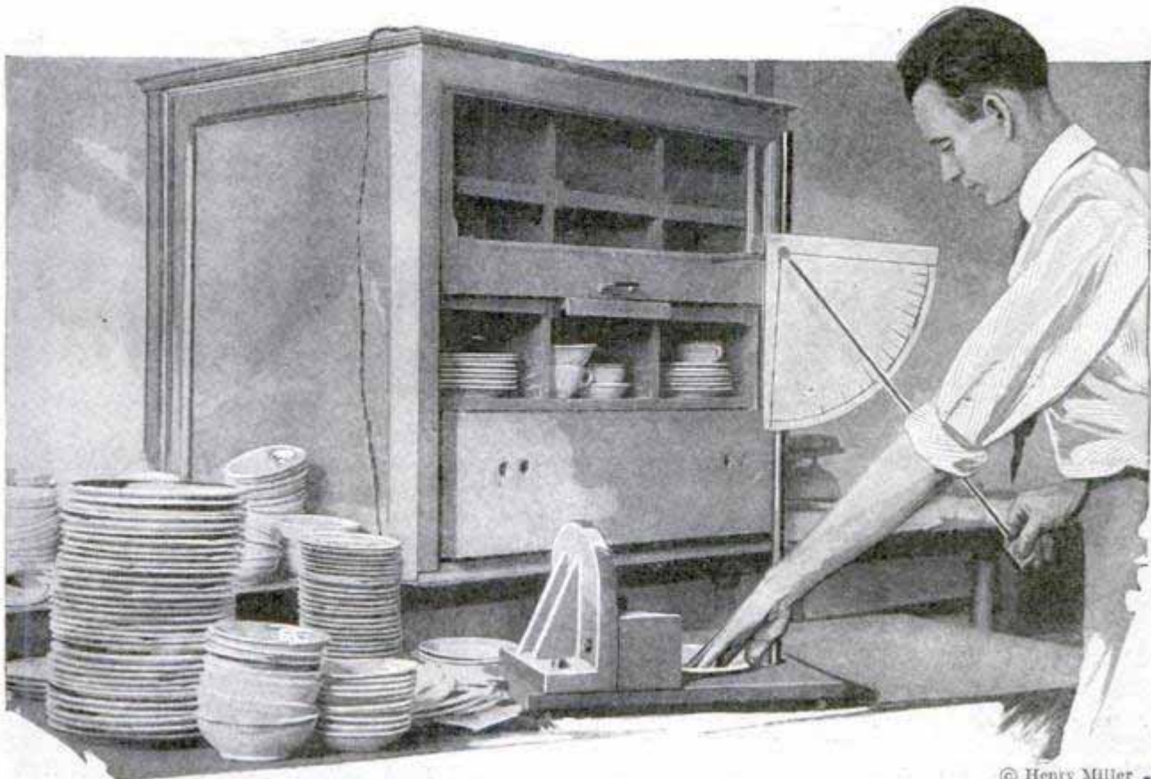
This Man Is Paid to Nick Dishes. The Weight Is Drawn Back, Then Allowed to Strike against Plate; the Force of the Blow Is Indicated on Dial
