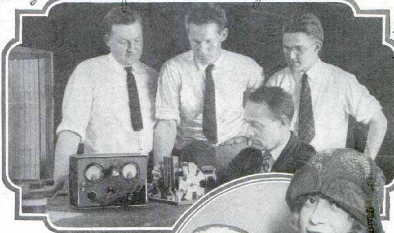
Multiple System of Radio Transmission Promises New Usefulness for Wireless; Eight Telegraphic Code Messages Were Broadcast Simultaneously on This One Transmitter and All Were Registered on a Single Receiving Set; the Process Involves a Short Carrier Wave at 30,000,000 Vibrations per Second on Which Are Impressed Several "Modulatory Waves"
