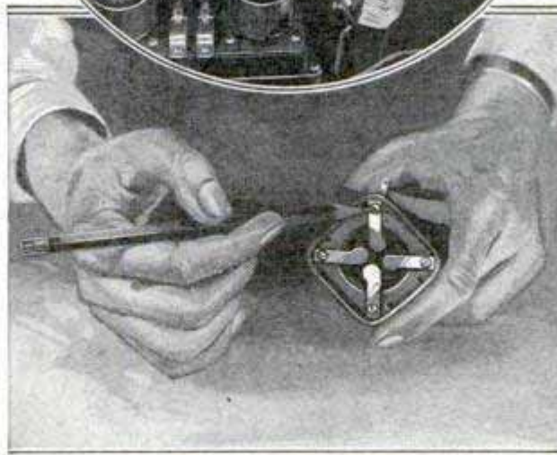
Above, Inspect Tubes for Loose Prongs; Below, See That the Socket Contacts Are Tight
