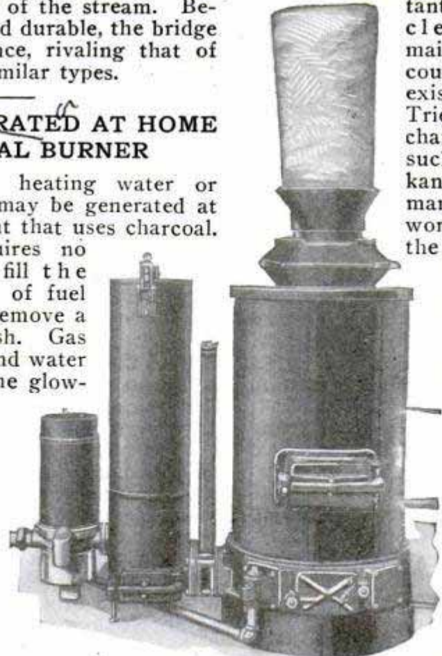
Home Gas Generator Complete; Inverted Bag of Charcoal Fuel on Hopper of Main Unit
