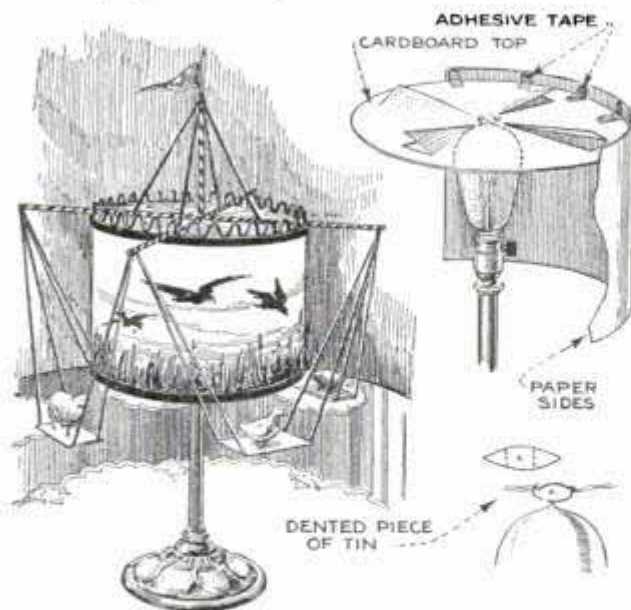
Novel Parchment Lampshade Which Is Rotated by Rising Heat from the Lamp
