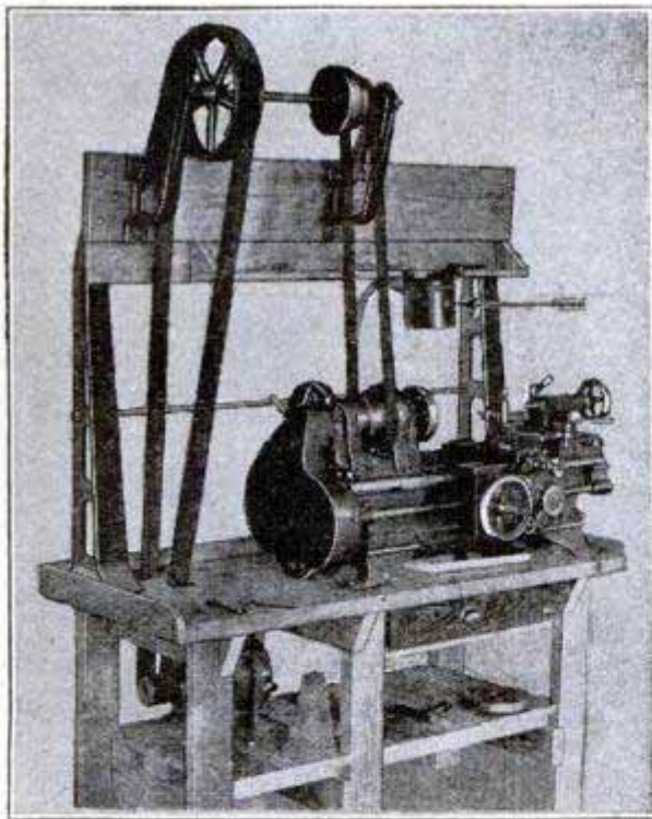
11" x 3½' Bench Lathe Unit Complete with D. C. Motor, $323.50 WRITE FOR OUR EASY PAYMENT PLAN
