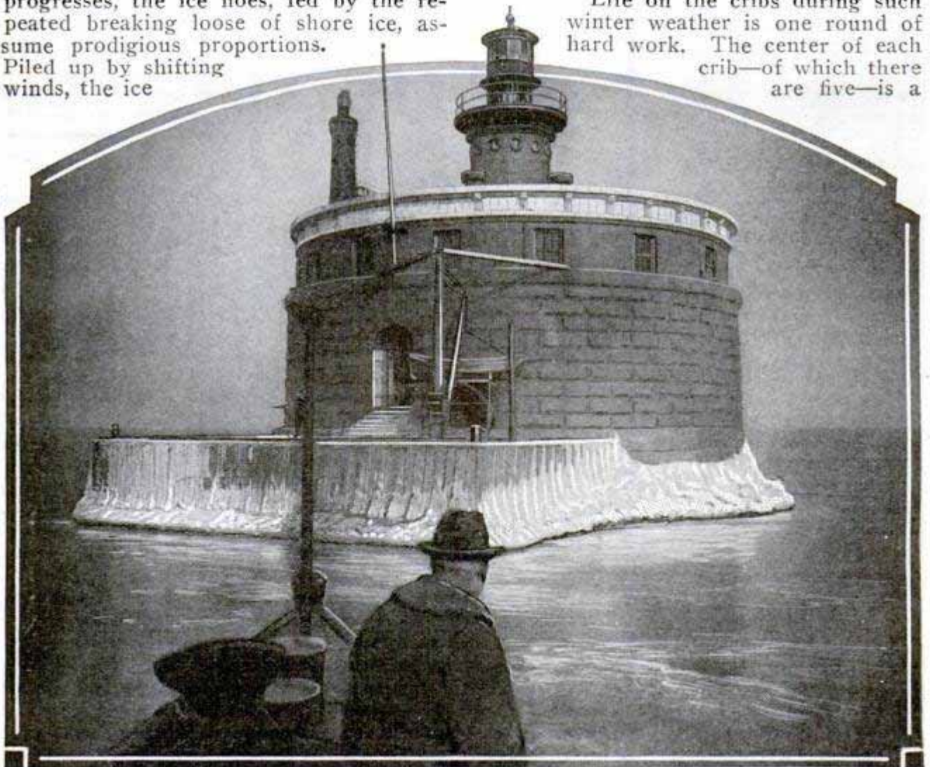
One of the Stone-Walled Cribs in Winter; Often the Northwest Gales Will Send Tons of Green Water High over the Roof, Frequently Breaking the Windows Forty Feet above the Lake
