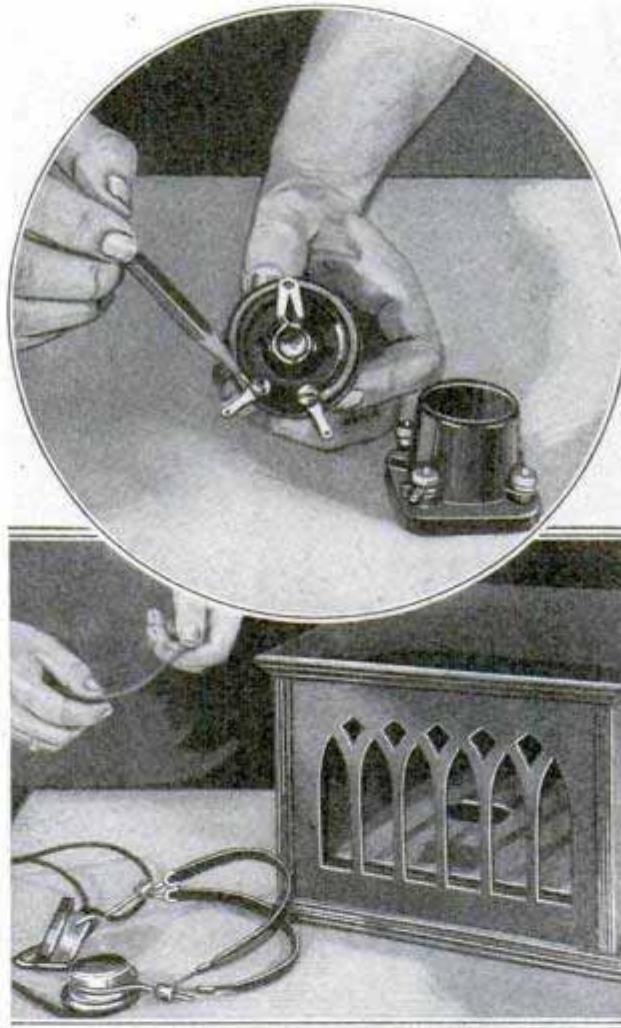
Lugs on Rheostats and Sockets Must Be Tight and Clean; Below, Inspecting Phone and Speaker Cords
