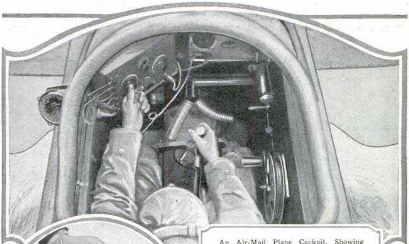
An Air-Mail Plane Cockpit, Showing the Corner Receiving Set, Where It Does Not Obstruct the Instrument Board, and, Right, the Aerial Reel, Both Out of the Way of the "Joystick" in the Pilot's Hand
