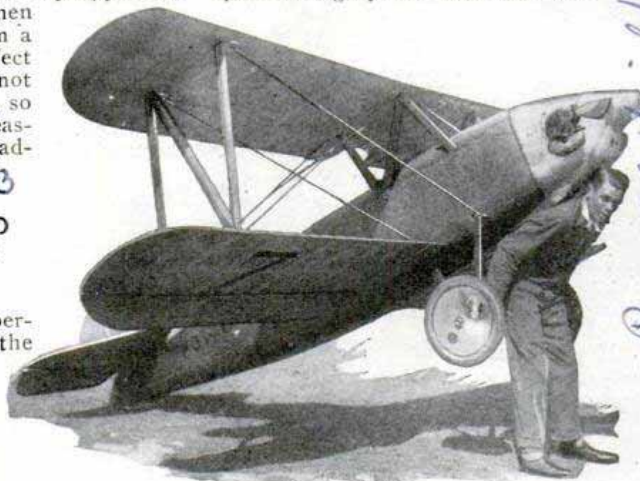
One Man Can Lift Tiny Airplane, as It Weighs Only 320 Pounds, But It Can Fly Eighty-Five Miles an Hour
