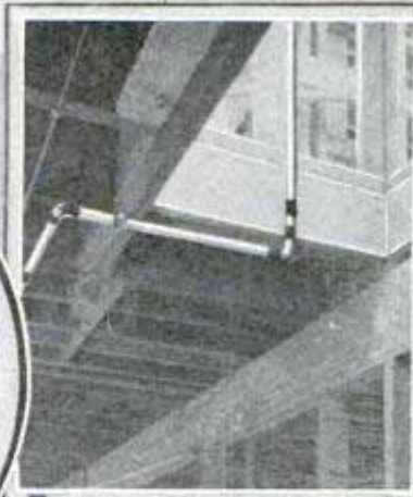
Taping Speaking-Tube Joints Prevents Leakage
