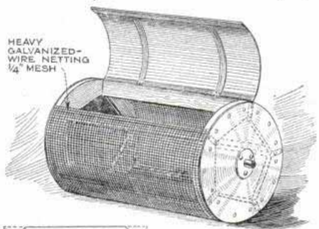
CUT FROM 1"X3" CYPRESS Galvanized Wire Mesh Used to Repair a Washing-Machine Cylinder
