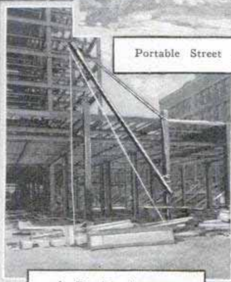
A Derrick Swung from the Steel Column of a Building under Construction Is Handy for Many Jobs
