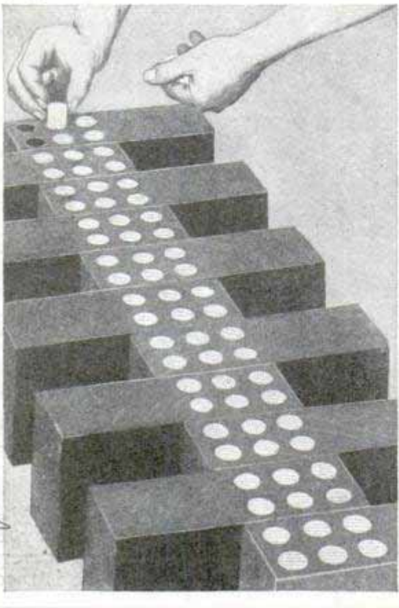
White Tile Markers for Traffic Lines and How They Are Inserted in Wooden Blocks
