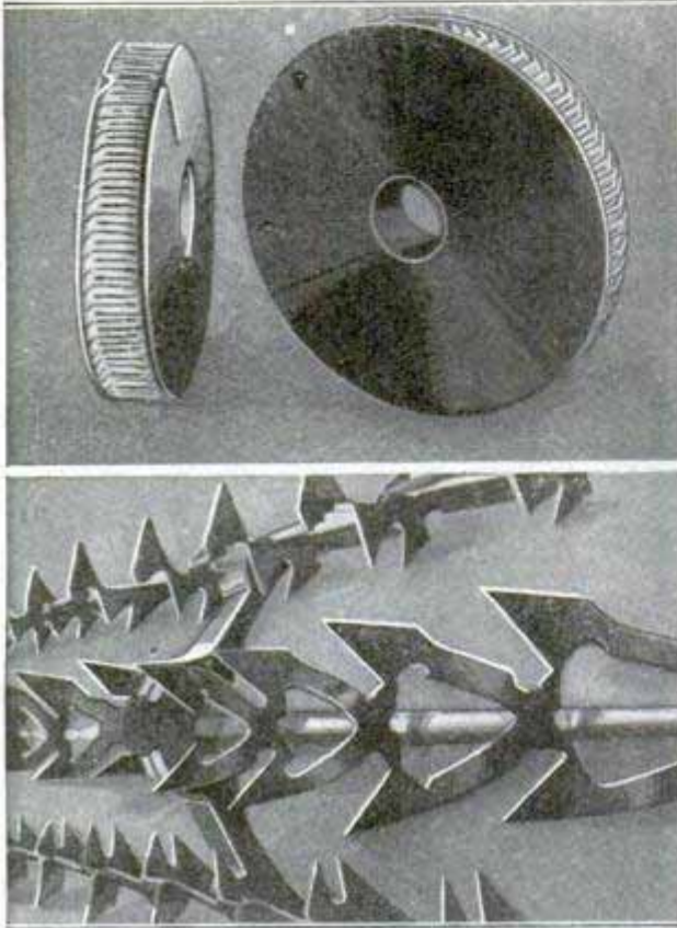
Bands Flat on Spools and Unwound, Showing How Barbs Extend When Strand Is Stretched
