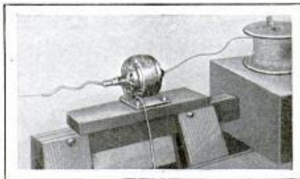
Taking the Coil Out of Spring Wire with a Small Motor and a Bent Tube
