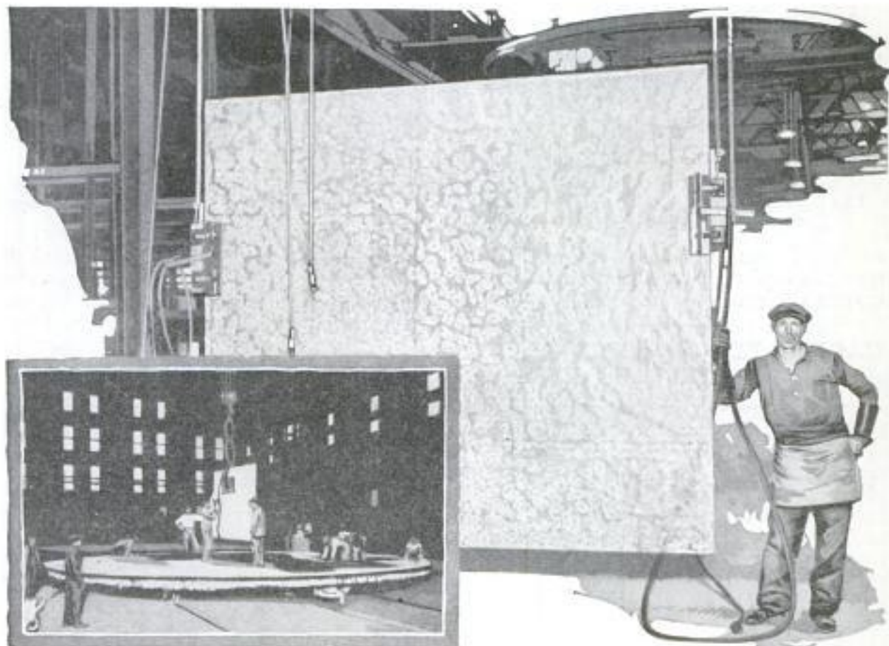
Overhead Cranes Carry These Big Sheets of Rough Glass from the Pouring Tables to the Polishing Beds; Right, a Polished Sheet Ready to Have the Plaster Washed Off
