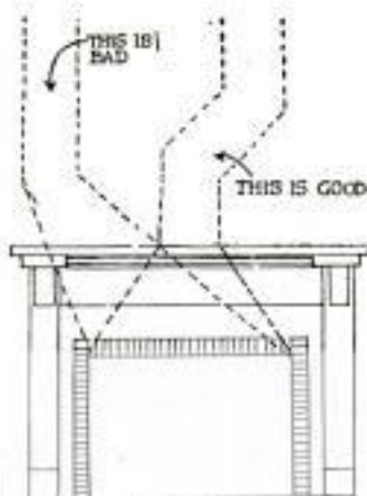
If the Flue Must Angle Be Sure the Angle Is Right
