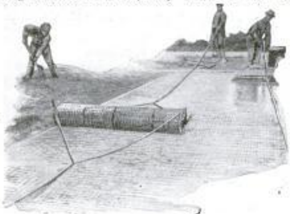
Smoothing Concrete with Roller That Presses Down Small Stones and Has Rope Handle
