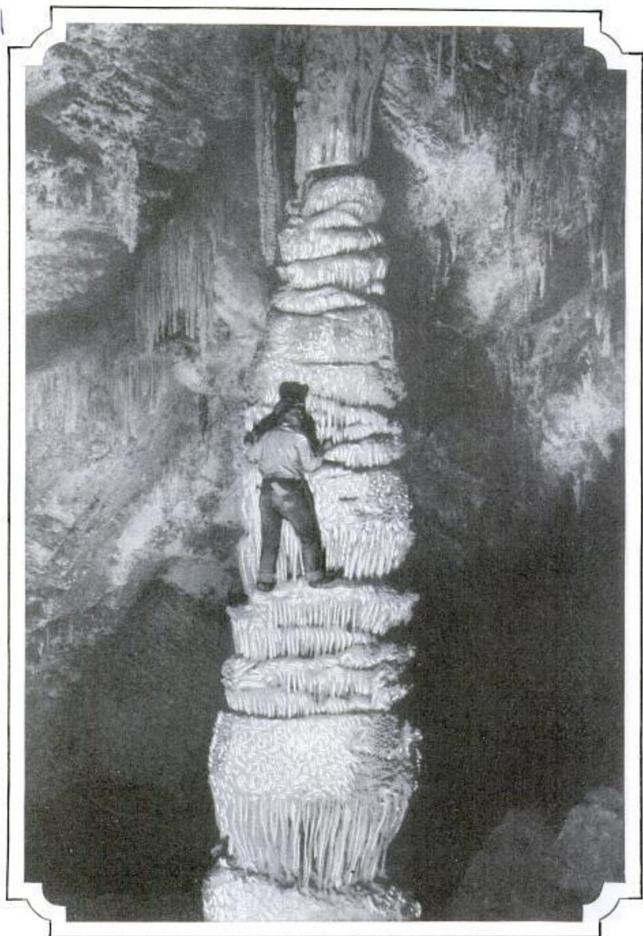
© J. W. Walker One of Nature's Cavern Wonders, Stalactite and Stalagmite Linked as a Fantastic Pillar with Smaller "Icicles" of Stone Adorning the Sections That Form a Ladder
