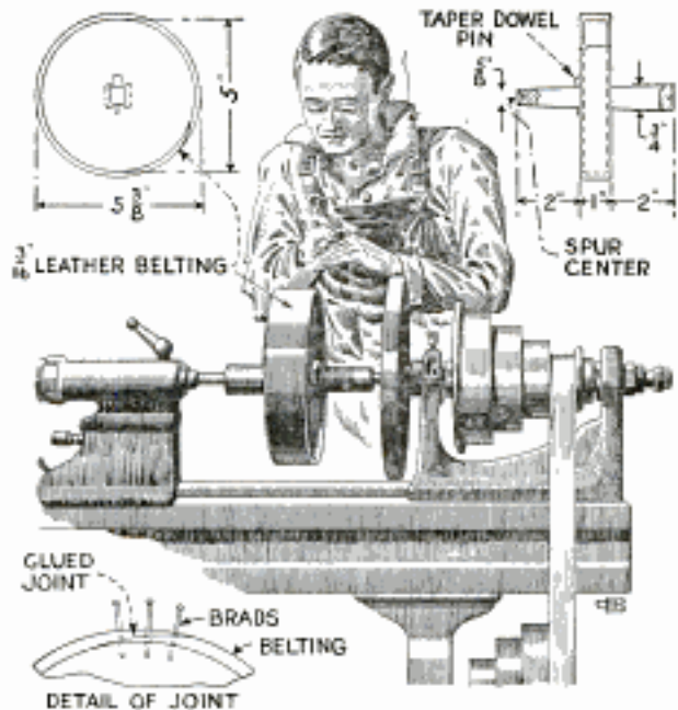
Stropping Wheel Faced with Leather Belting Found Convenient
