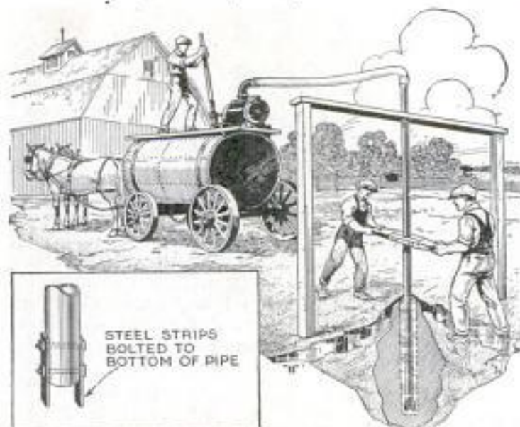
A 25-Foot Well Can Be Sunk in One Hour by Using This Method of Drilling
