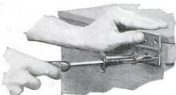
Driver with Spring Grip, Holding Screw in Place Until It Can Be Started
