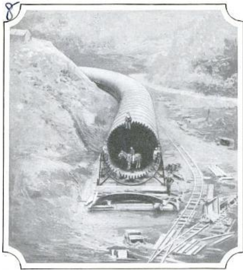
Record-Breaking Wooden-Stave Flume; Notice the Horse and Man Standing Inside and the Workman Perched on Top
