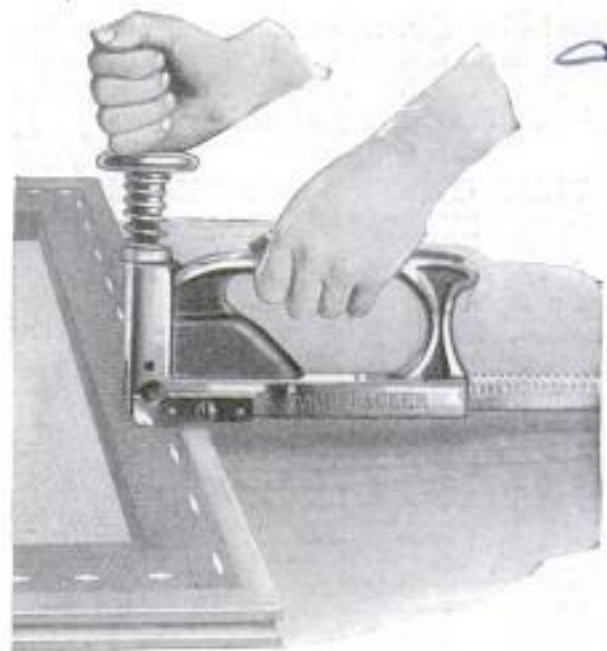
Screen Stapler and Stretcher in Operation; the Teeth That Grip and Mesh Are under the Plunger
