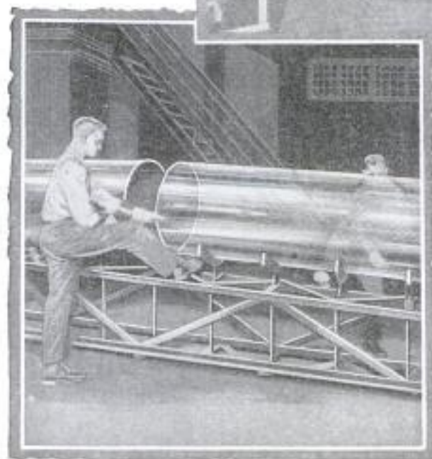
Plain Window-Glass Cylinders Are Split Open and Flattened after Being Cut in Short Lengths
