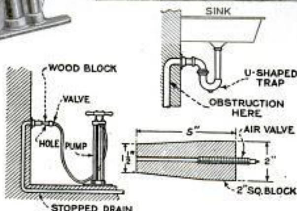
A Force Pump Made from an Automobile Tire Pump Which Will Remove Obsolete Obstructions from the Drain Pipe
