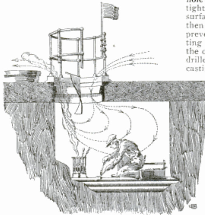
Simple Method of Ridding Manholes of Gas with Rubber Blanket Which Causes Draft
