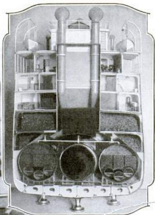
Cross-Sectional Model of Big Liner, Showing Midship Details from Keel to Boat Deck and Bridge
