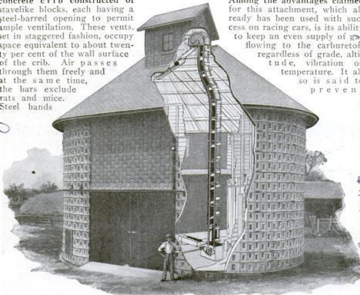
This Concrete Corn Crib Has Openings in the Blocks to Allow Ventilation; Steel Bars in Openings Prevent Entrance of Rodents, and a Chainless Lift for the Grain Simplifies Filling
