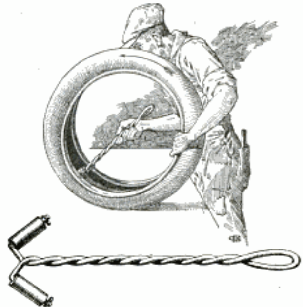
Twisted Iron-Rod Tool with Wooden Rollers Enables Tire Man to Make Thorough Examination of Fabric
