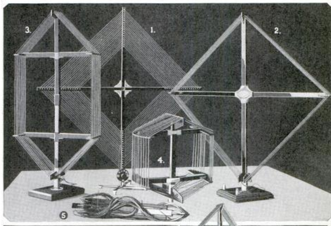
A Few of the Most Popular Loops; 1, Pancake Type; 2, Diamond-Shaped Box Type; 3, Console Type, Exposed; 4, Console Type, Inclosed; 5, Small Loop Folded, and 6, Proper Method of Rotating a Loop
