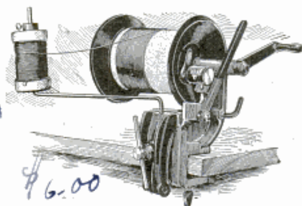
Made to Clamp to the Work Table. This Handy Coil Winder Is Five Tools in One
