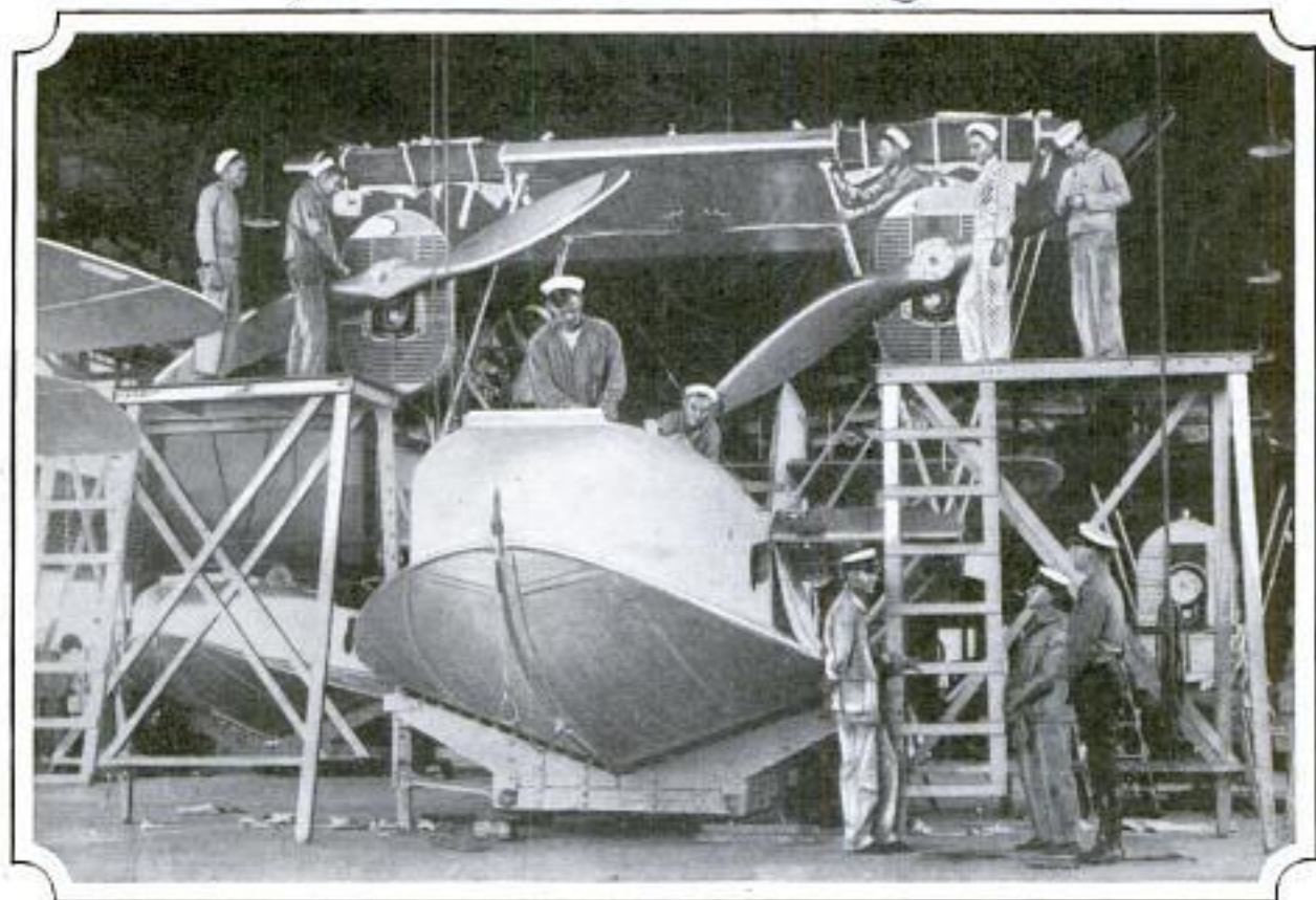
Latest Navy Plane, Especially Designed for Long Ocean Voyages, Has Wings Seventy-Two Feet Across, and Is Said to Be Seaworthy Even When Alighting on the Roughest Waves
