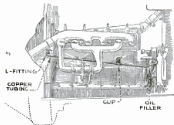
An Improved Outside Oil Line Installed on a Ford Motor
