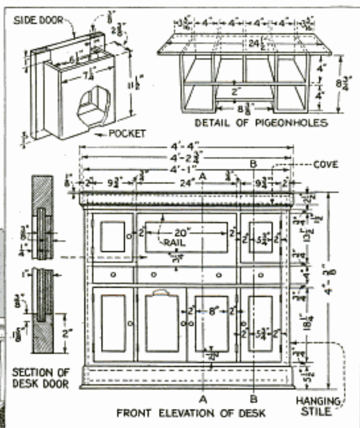
Front Elevation of Writing Desk, Detail of Pigeonholes and Pockets on Side Doors, and Method of Building Up Door for Desk Section
