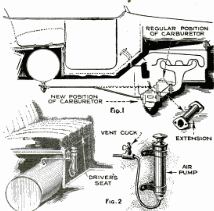
Two Simple Methods of Getting Gasoline into the Carburetor of Gravity-Feed Car When Ascending Steep Grades
