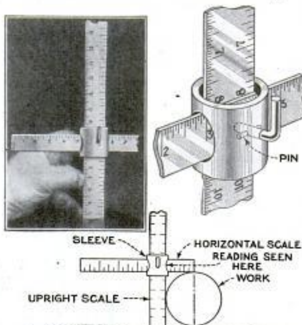
Double-Scale Holder Facilitates Scribing Shafts
