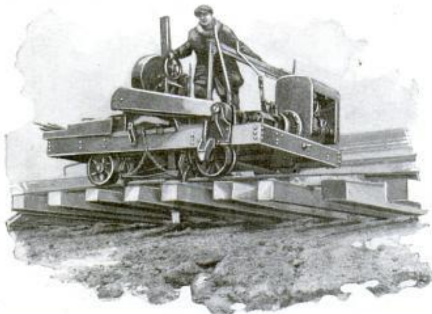
Track Lifter in Operation: Spud Is Set between Rails, and Truck, Clamped to Them, Is Elevated upon It
