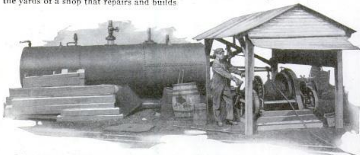
Old Steam Boiler Used as Compressed-Air Tank to Operate a Winch, Trip Hammer and Other Air Tools.
