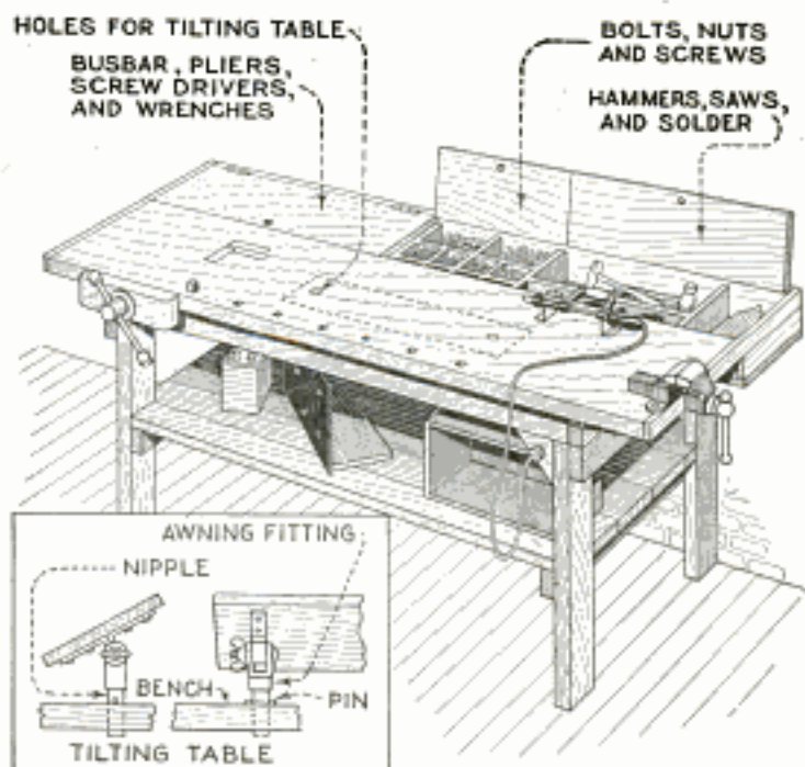
Handy Radio Workbench Saves Many Steps; Insert, Method of Mounting the Tilting Table
