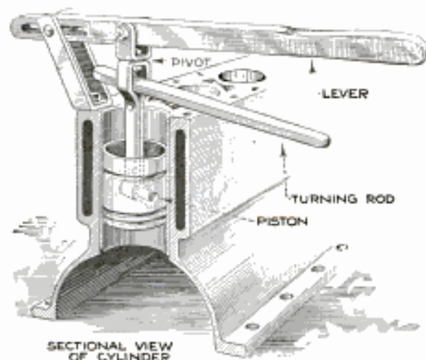
Handy Lever Arrangement Reduces Work of Lapping Pistons
