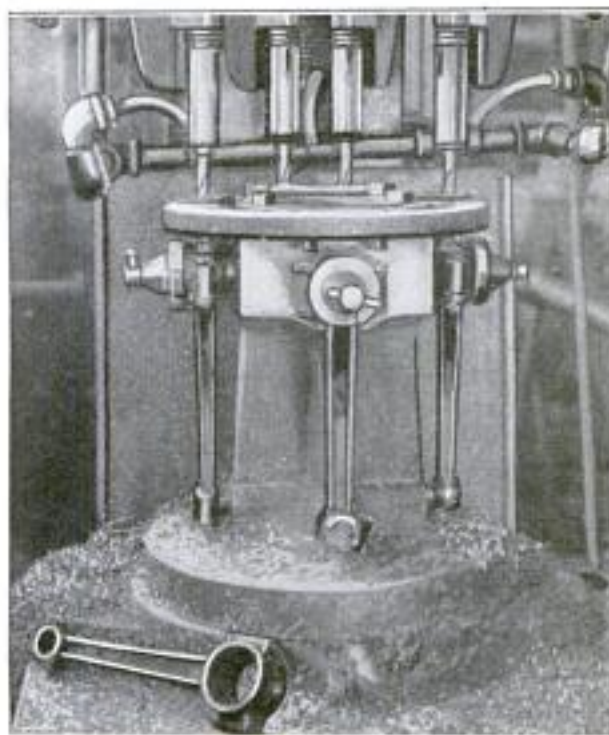
Four Spindles Each Drill a Hole, While the Completed Work Is Removed and a New Part Loaded
