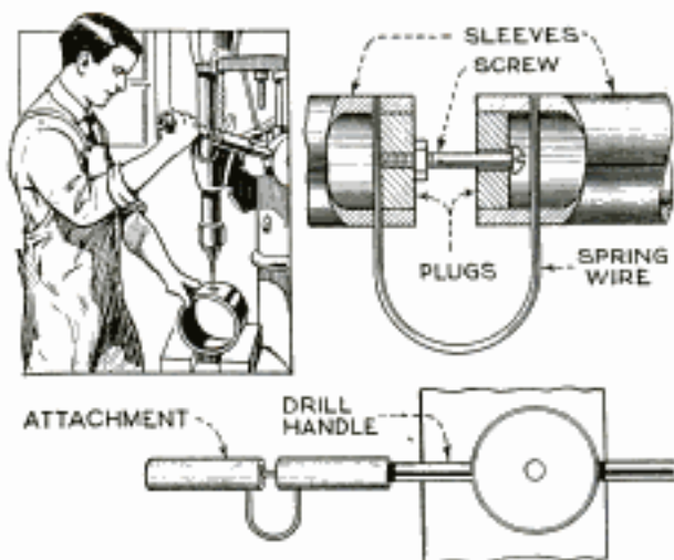
Spring Attachment on Handle Makes Ordinary Drill Press Sensitive
