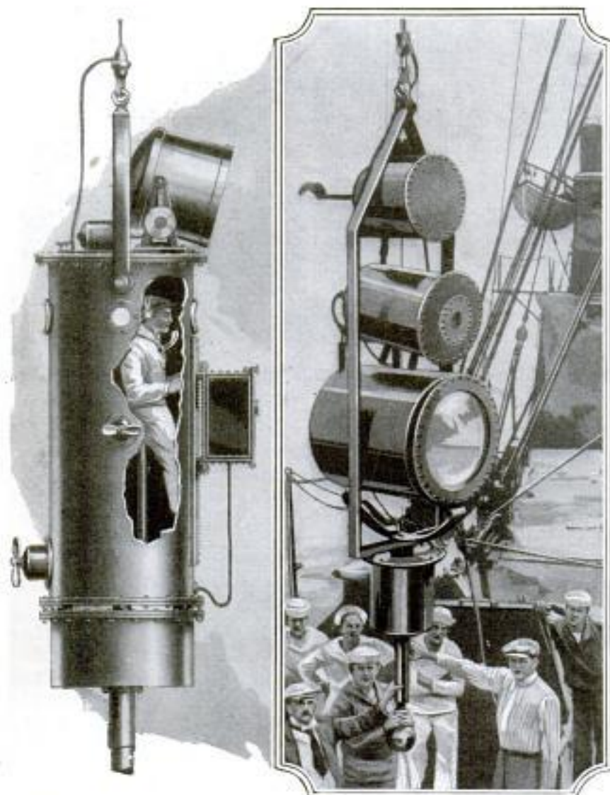
Swinging the Battery Tanks and Lights of the Deep-Sea Camera into Position for an Under-Water Descent; Left, Operator in Projector Chamber
