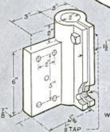
ARM BEARING, CAST IRON
