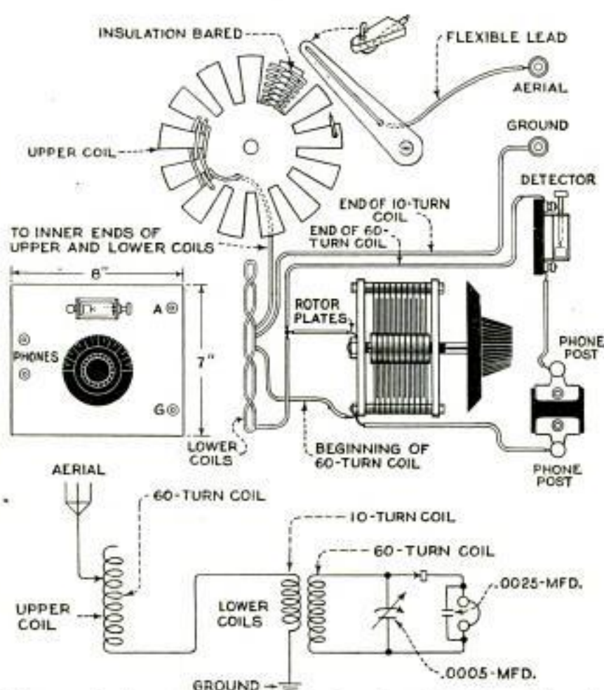
Diagram of Connections of the Selective Crystal Receiver; Schematic Diagram and Panel Template
