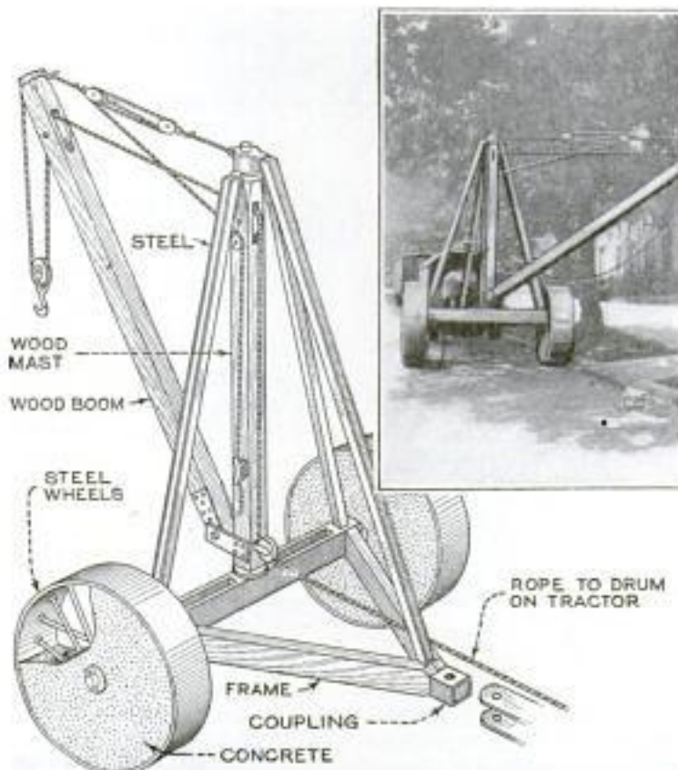
Above, Photo of the Trailer Hoist on the Job; Below, Perspective View of the Hoist, Showing the Lifting and Boom Tackles
