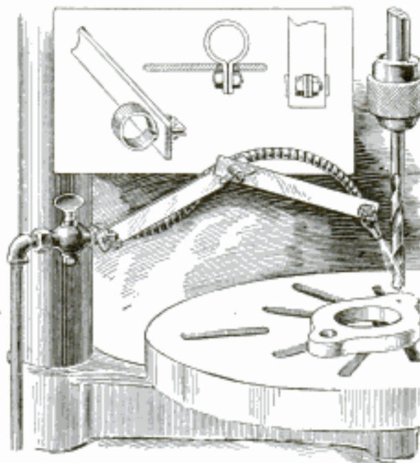
Convenient Clamp Holds Flexible Tubing in Any Position
