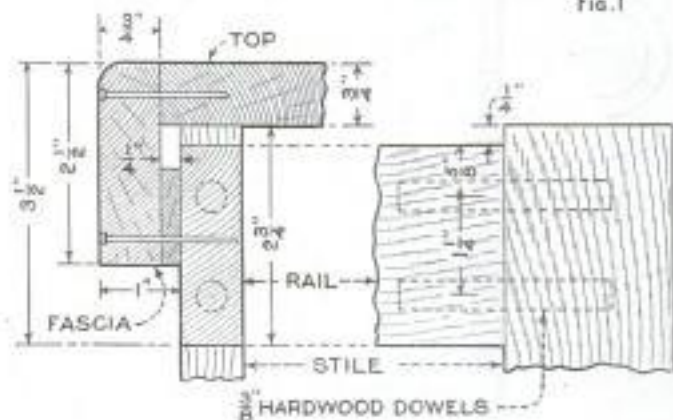
JOINT BETWEEN RAIL AND STILE
