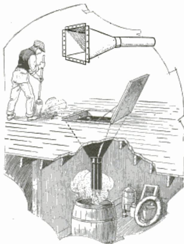
Galvanized-Iron Chimney Cowl Makes Handy Dirt Chute in Store
