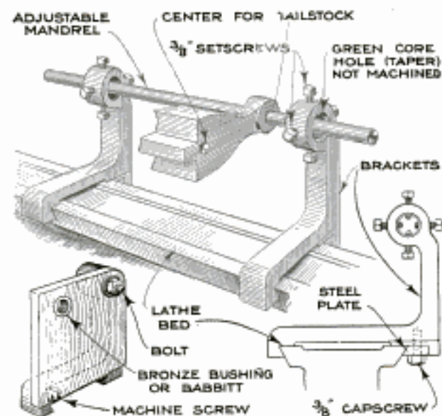
Brackets for the Lathe Bed Make It Possible to Use Milling and Grinding Attachments with a Minimum of Difficulty
