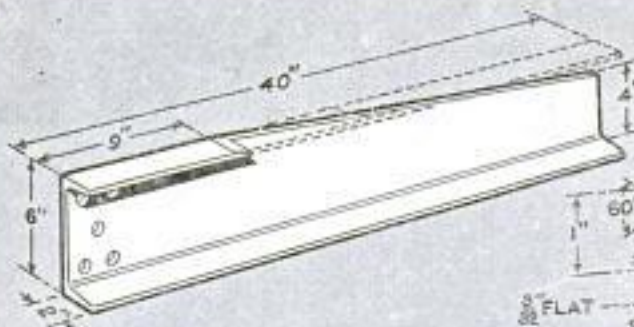
DETAIL OF ARM
