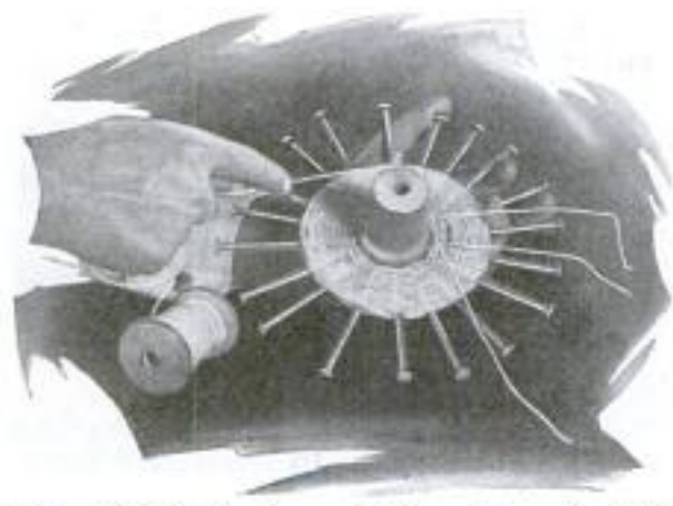
Method of Winding Lower Coils on Form; the Nails Are Removable
