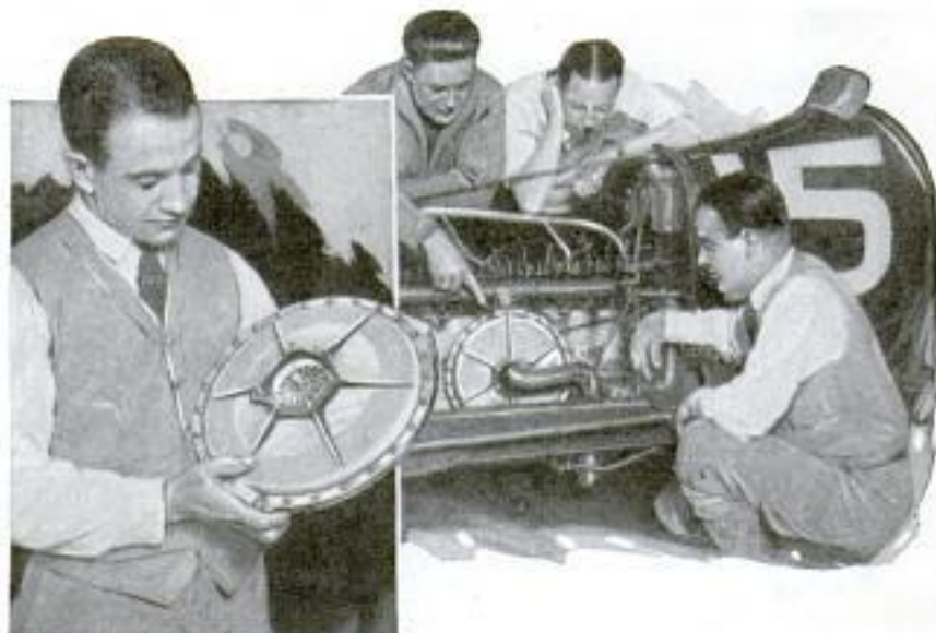
Close View of Supercharger Showing Its Blowerlike Construction, and Position It Occupies When Installed in Racer
