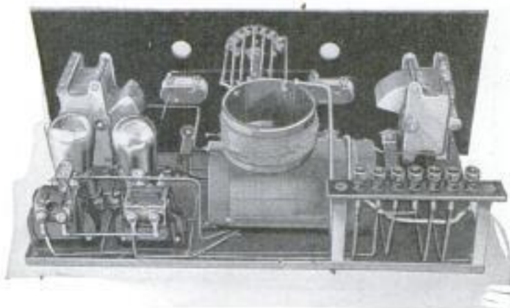
Rear of Cockaday Receiver; Note How the Coil Is Arranged So That the Leads to the Switch Are Straight and Direct
