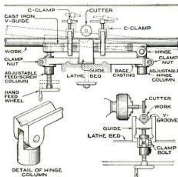
Attachment for Cutting Woodruff Keyways in the Lathe, Which May Be Built from Stock Parts
