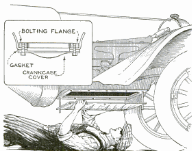
Guide Studs Provide Easy Method of Replacing Crankcase Cover
