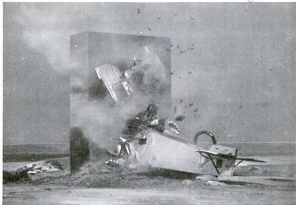
Wrecking an Old Plane against a Concrete Wall at the Army Testing Field to Study Its Weak Points and Determine Dangers of Gasoline Explosion
