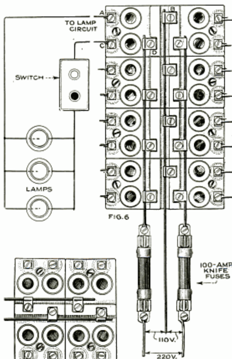
FIG. 6 Three and Two-Wire Porcelain Fuse Blocks Used in Most Apartment Buildings Having Numerous Branch Circuits
