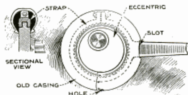
Old Auto Casing Prevents Cement from Getting under Strap on Eccentric of Concrete Mixer
