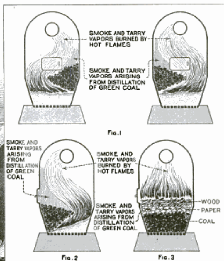
Fig. 1, Firing the Furnace on Either Side Alternately; Fig. 2, Effect of Firing at the Front; Fig. 3, Proper Method of Starting the Furnace Fire
