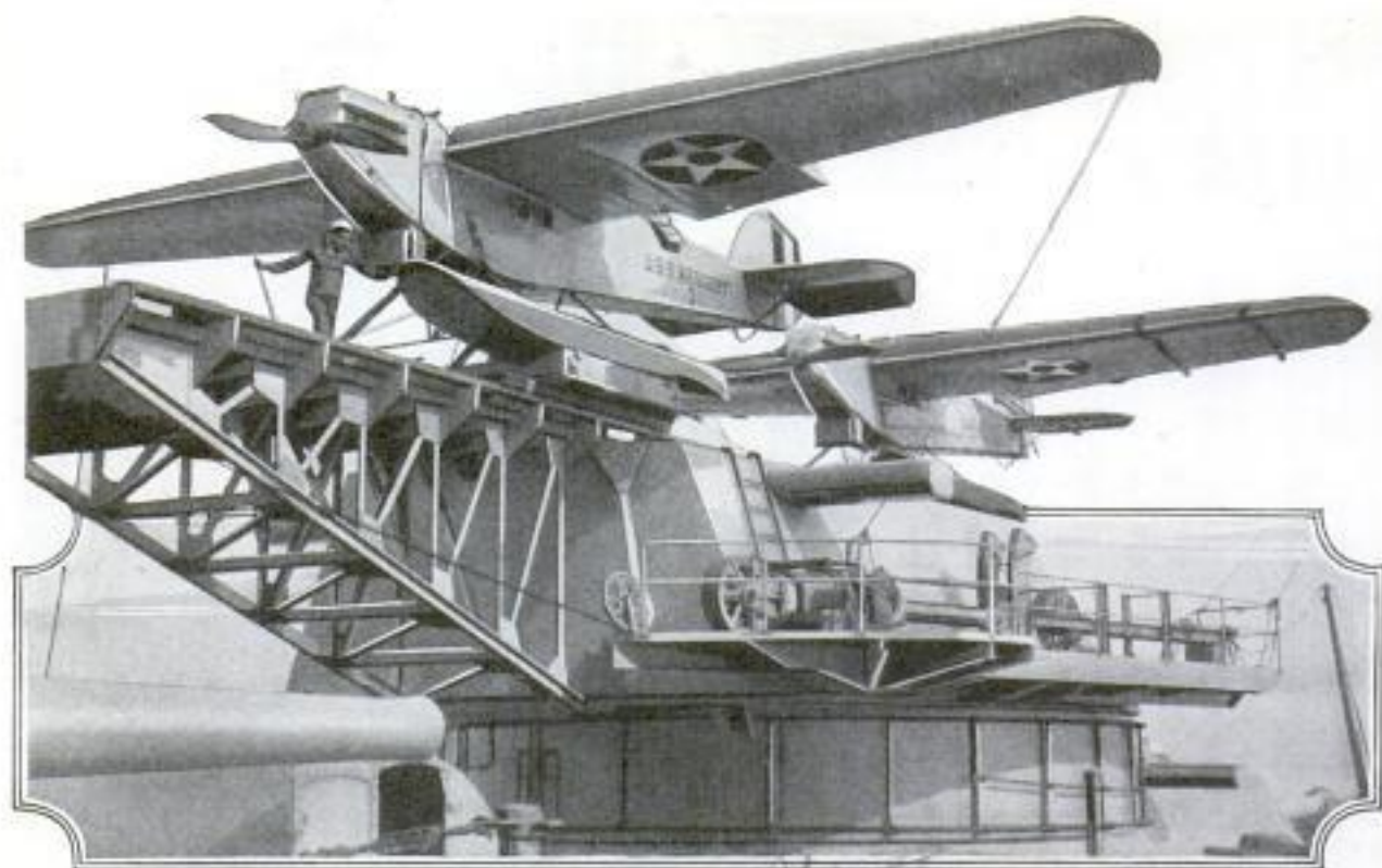
From This Launching Turret on the U. S. S. "Mississippi," Planes Are Sent Skimming Seaward by Firing a Charge of Smokeless Powder, Releasing Apparatus That Acts as a Catapult
