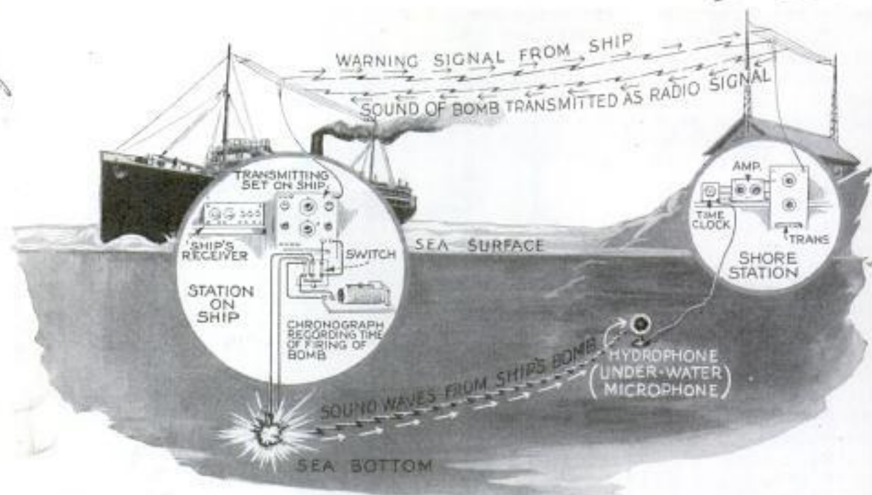
Photodiagram of the Combination Wireless and Under-Water Sound-Wave Device Developed for Use as a Direction Finder for Ships Navigating near Shore
