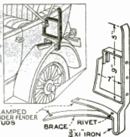
DETAIL OF REAR BRACKET
