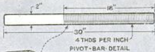
PIVOT-BAR-DETAIL
