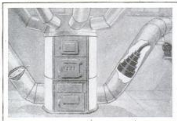
Circulator Installed in Pipe of Warm-Air Furnace to Induce Draft and Distribute Heat Evenly
