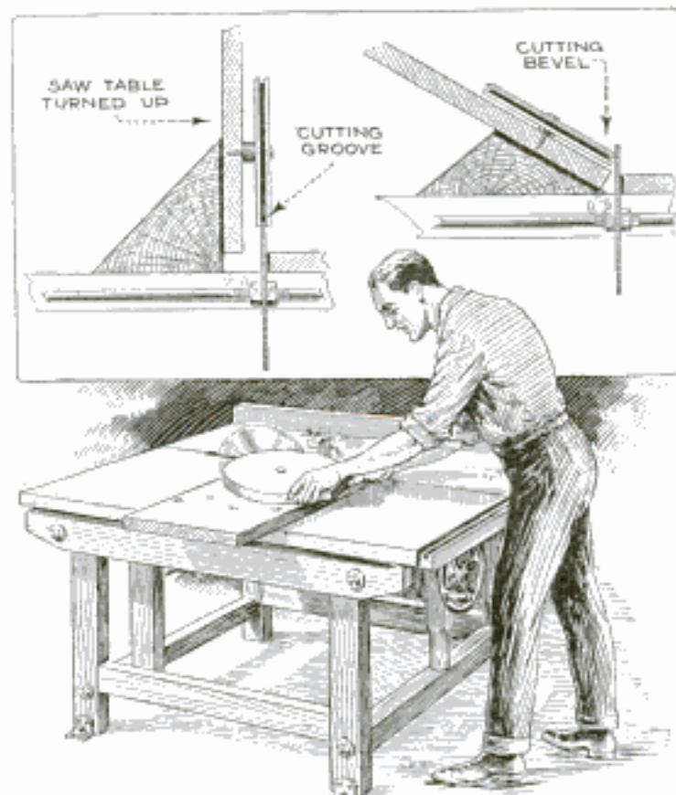
Simple Fixtures That Enable the Amateur Woodworker to Turn and Groove Disks on the Saw
