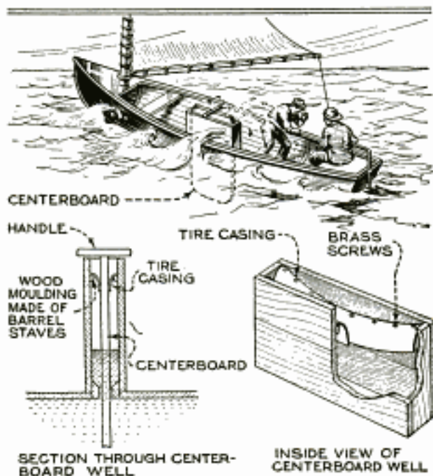
Splash Guards Made from Auto Tire Make Centerboard Well Splash-Proof
