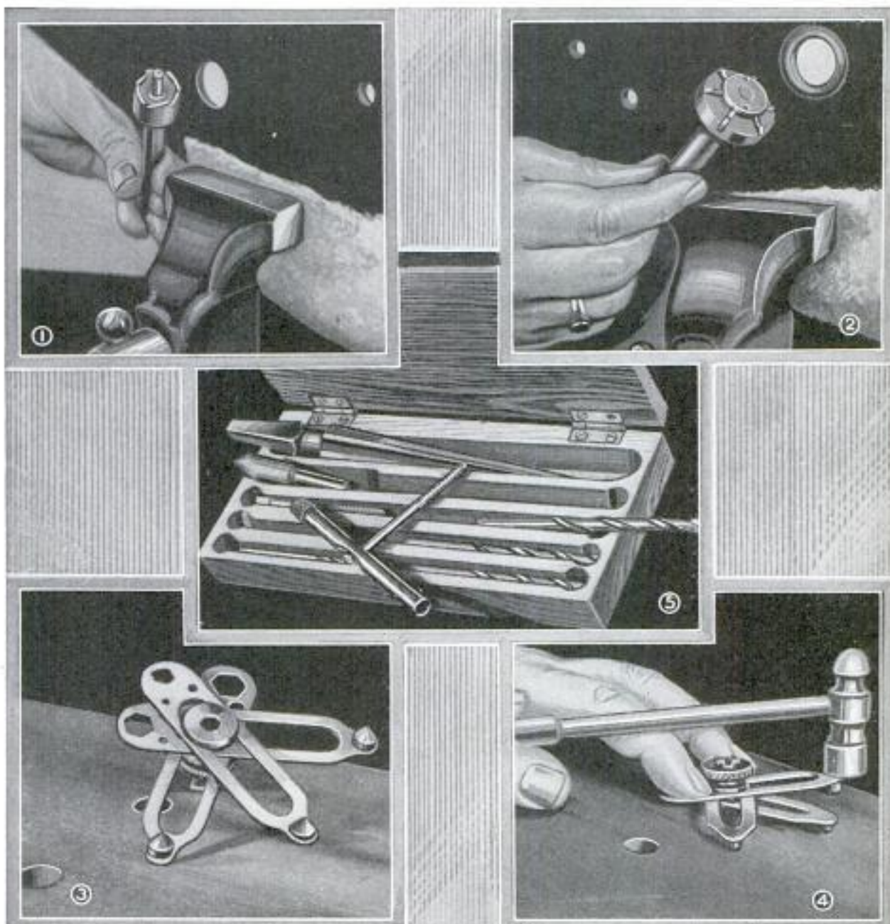
Clever Tools for the Radio Builder That Aid in Drilling and Finishing Peepholes and Socket Holes; Drilling and Tapping Panels, and Marking Off for Various Instruments
