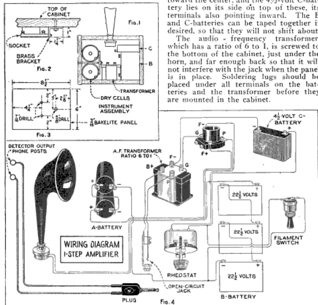
Above, Panel Layout for One-Step Instrument, Mounting of Tube Socket and Arrangement of Components; Below, Wiring Diagram for One-Step Amplifier
