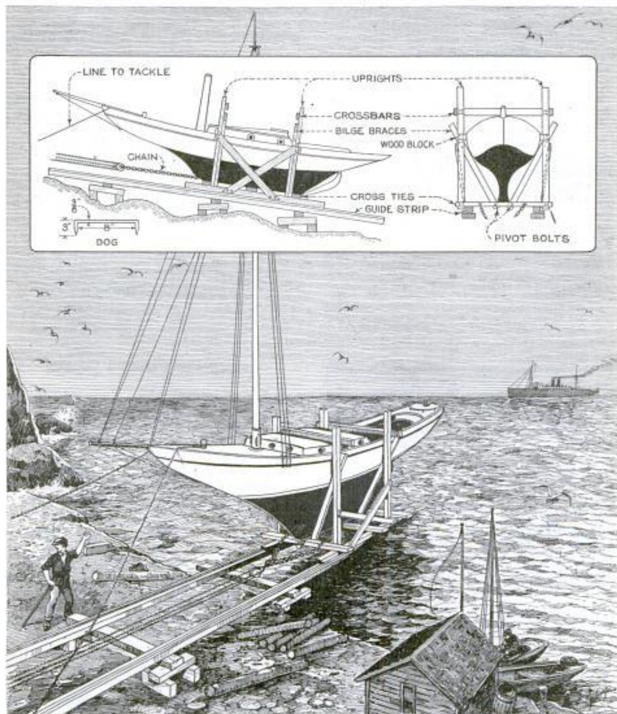
To the Small Repair Yard as Well as the Individual Yacht or Small-Boat Owner, This Homemade Marine Railway Will Prove of Value; the Underwater Shape of the Boat Need Not Be Known
