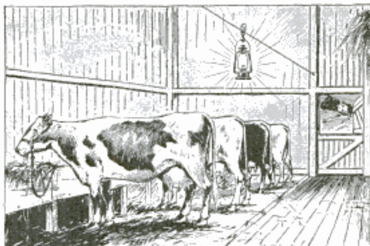
Danger of Fire Is Lessened and Light Is Distributed More Evenly by Hanging a Lantern on Wire Trolley
