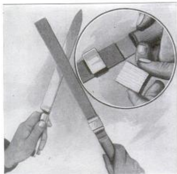
Whetting Knife and Inserting Wedge under Sleeve to Hold Abrasive Strip to Bar
