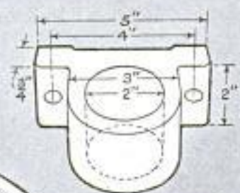
PIVOT BEARING, CAST IRON, 2 REQUIRED
