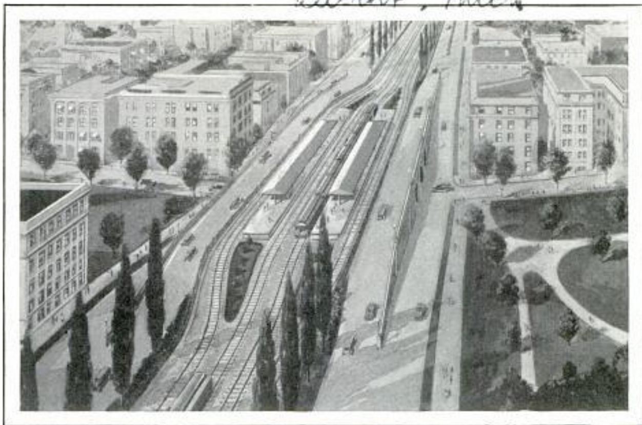
Type of Super-Highway Planned for Detroit, Showing Method of Carrying Express and Through Traffic Overhead at Street Intersections, Where Only Local Vehicle Lanes Connect with Cross Thoroughfares
