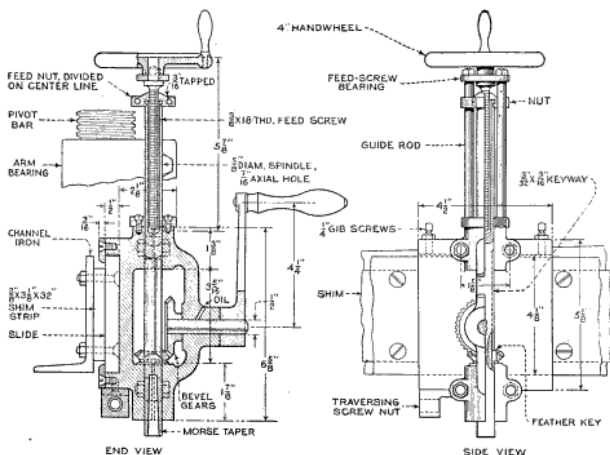
DRILL-HEAD AND SADDLE DETAILS
