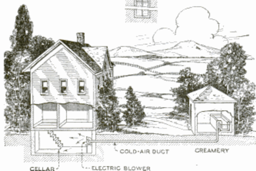
Novel Method of Cooling and Ventilating Farm Cellar with Air Cooled by Contact with Water and Drawn through an Underground Duct
