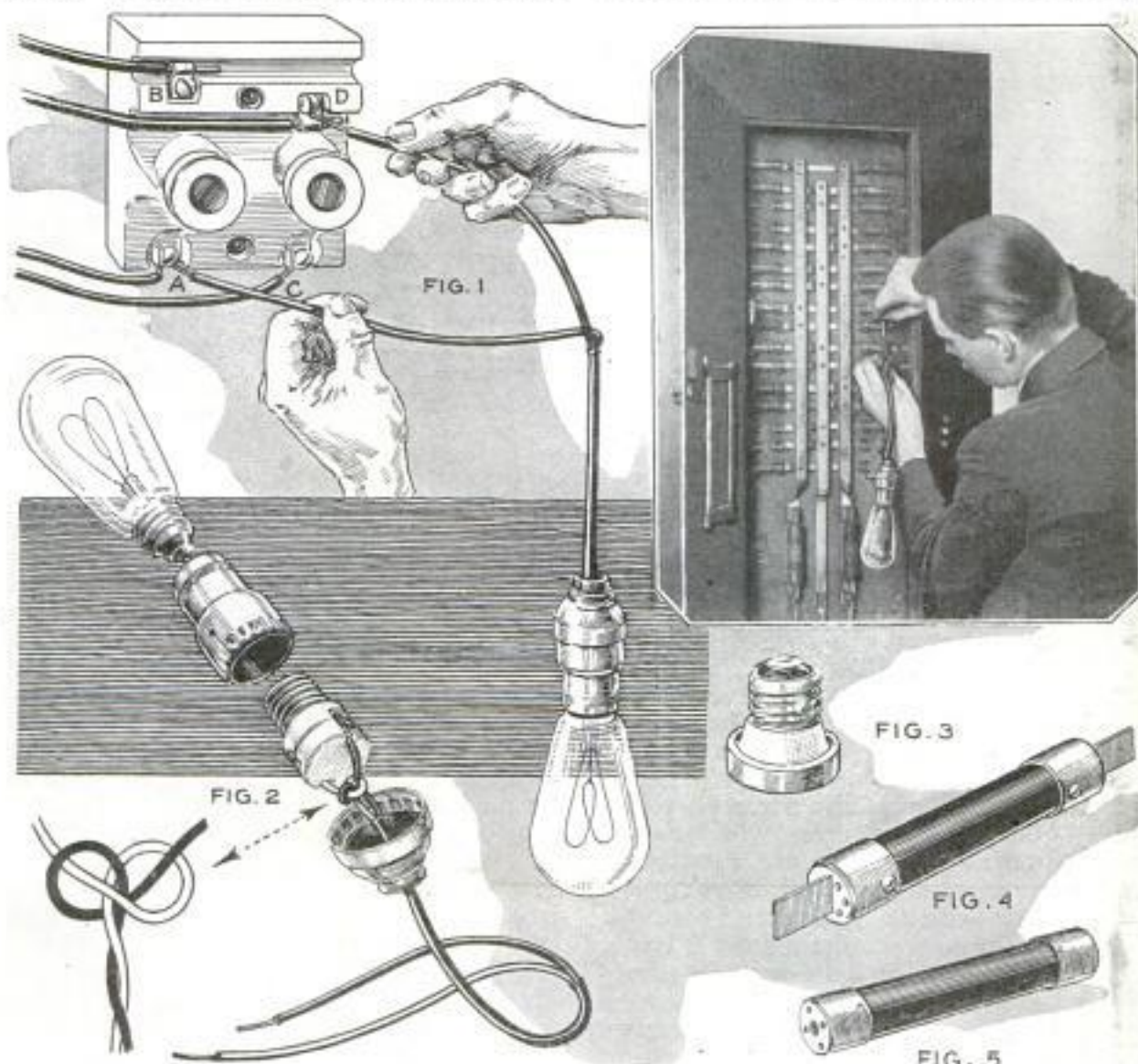
With This Homemade Test Lamp Anyone Can Find Blown Fuses No Matter How Complicated the Fuse Panel May Seem, Eliminating the Expense of Calling an Electrician for Such Simple Jobs
