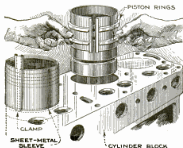
Sheet-Metal Sleeve Proves Useful in Assembling Piston Rings
