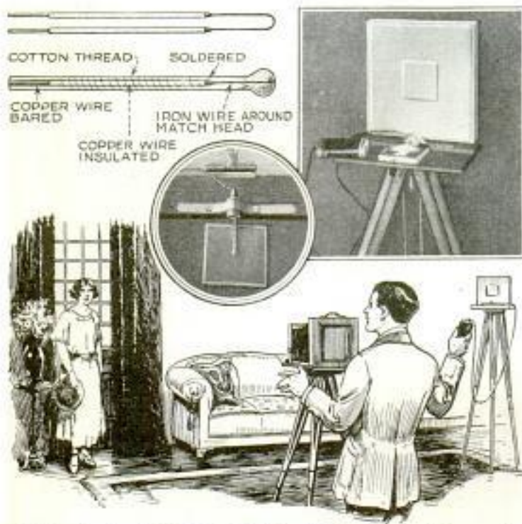
Safe Igniter for Flash Powder When Taking Interior Photographs
