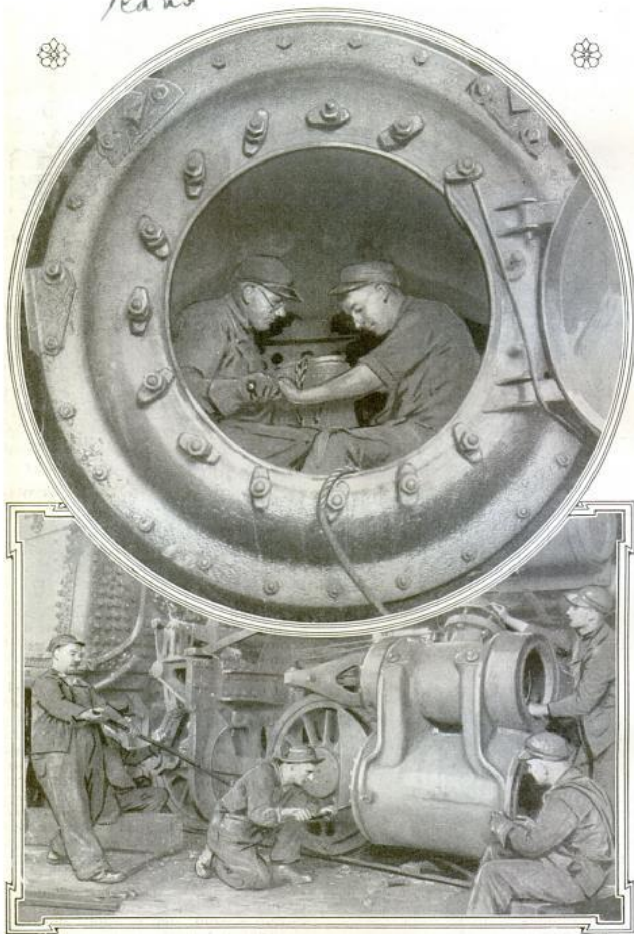
When Iron Horses Go to the Hospital—Men Grinding Exhaust Joint in a Locomotive Smokebox; Below, Overhauling the Huge Cylinder of a Twenty-Four-Drive Wheel Engine
