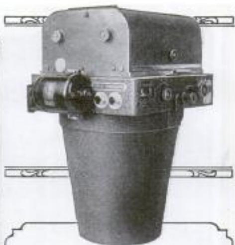
View of Camera with Film Holder in Place; the Battery Wire and Switch Control Are Attached to the Two Plugs beside Motor
