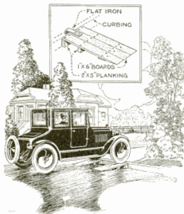
Inclined Wooden Runways Permit Autos to Run over High Curb
