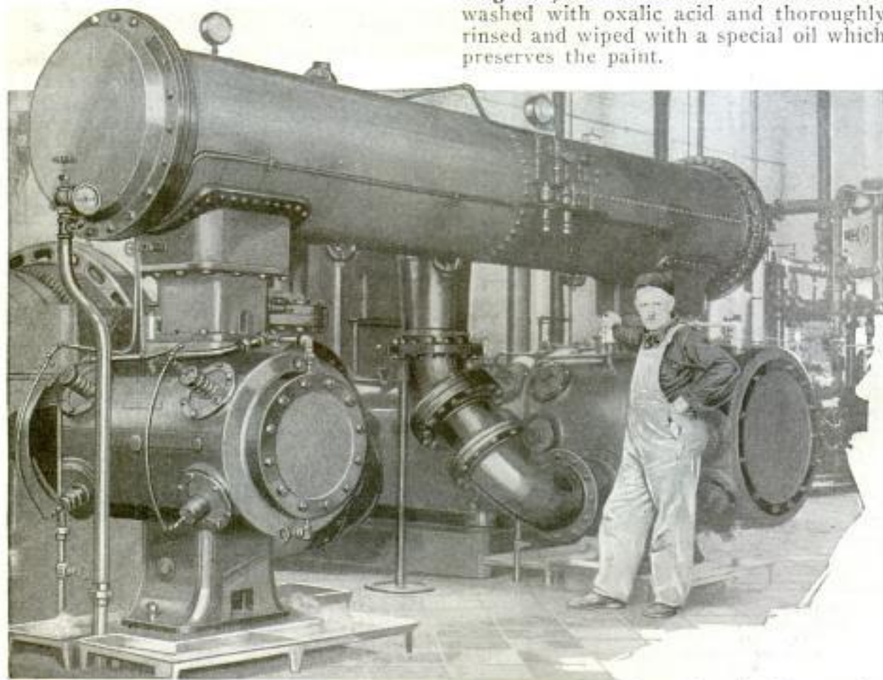
Big Compressor and Storage Tank, the Source of the Air for Making Brake Tests, Operating Cleaners and Various Repair Tools in Coach Yards and Shops
