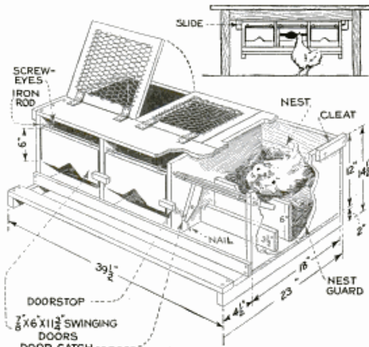
Method of Constructing the Trap Nest; the Door of the Right Compartment Is Open to Show the Latch; It Normally Closes When the Hen Enters
