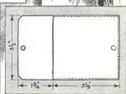
Pocket Shoe Shiner That Aids in Preserving Neat and Tidy Appearance during the Day
