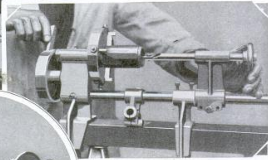
Views of Hand Lathe, Showing Block Adjusted, Boring Operation and Turning a Candlestick
