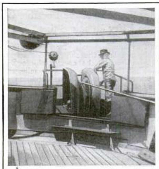
Lifting the Cable, with the Wire Passing through the Bow Sheaves on the Foredeck
