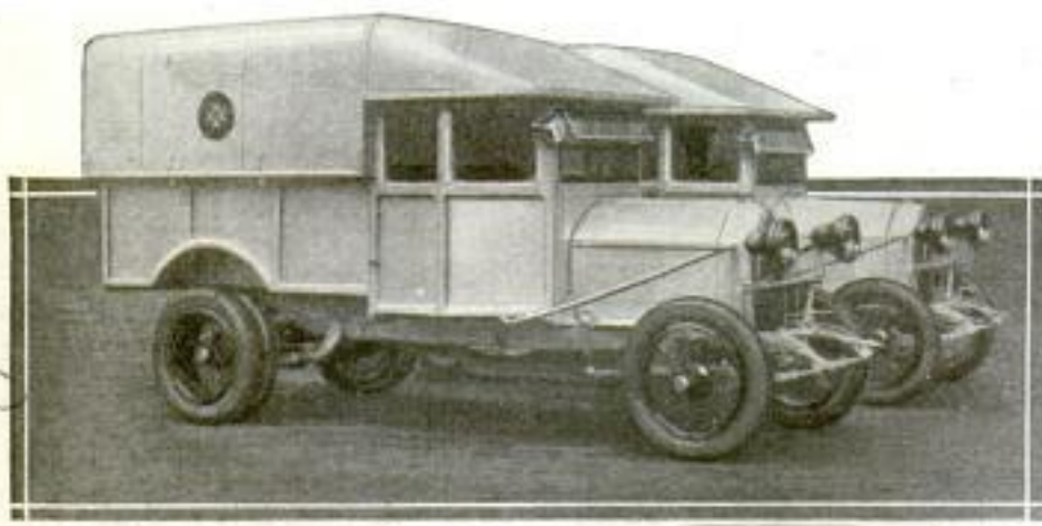
Motor Transports for the African Expedition with Metal Tops in Normal Traveling Position; Putting the Boat Together, and Ferrying a Car over a Stream in It; Double-Tired Rear Wheels, Wire Spokes Throughout and Capacious Drinking-Water Tanks Are Included in Equipment to Aid in Blazing 7,000-Mile Motor Trail through Wilderness
