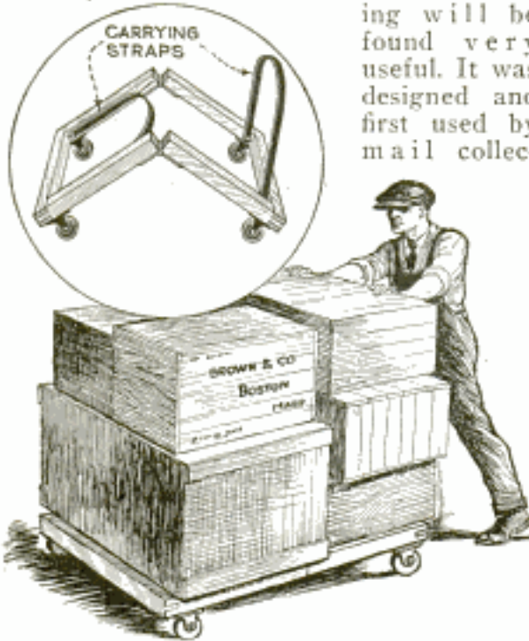
Collapsible Dolly Is Light in Weight and Can Easily Be Carried
