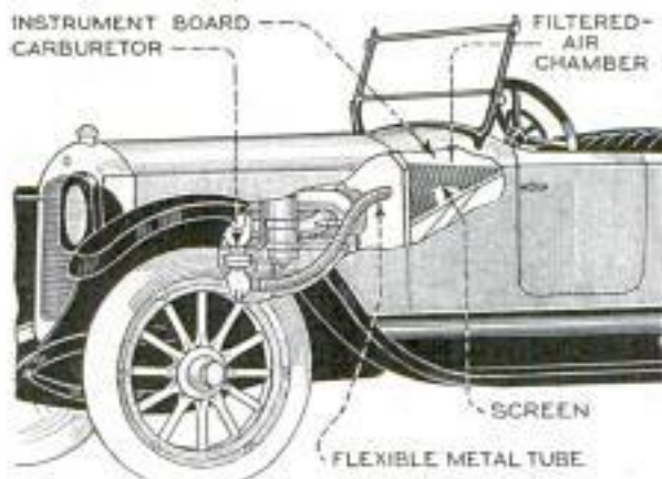
Air Filter on Carburetor Keeps Grit Out of Motor
