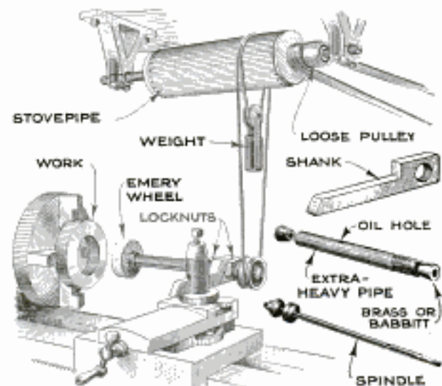
An Easily Constructed Toolpost Grinding Fixture for the Lathe That Is Adaptable to Internal, External and Surface Grinding Operations
