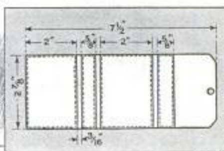
Holder for Preserving Original Shape of Packet of Cigarets and Keeping Them in Good Order. Made from Strip of Leather with Four Small Panels Sewn On; Dimensions at Right
