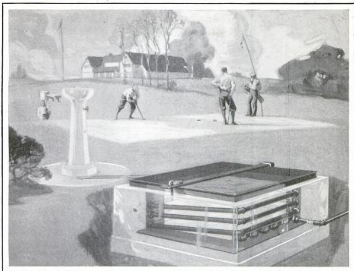
Water Cooler Installed Close to Drinking Fountain on Golf Links; Pipes Fitted in Hollow Square Form Convenient Ice Space, and Thick Concrete Wall Provides Insulation
