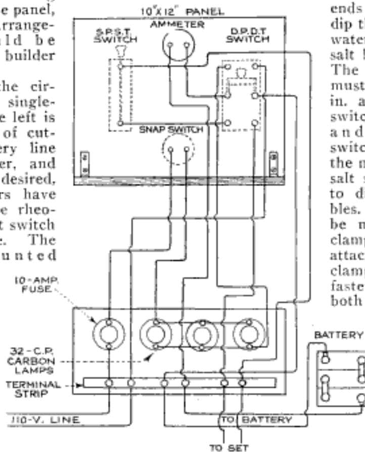
WIRING DIAGRAM FOR PANEL AND LAMP BANK
