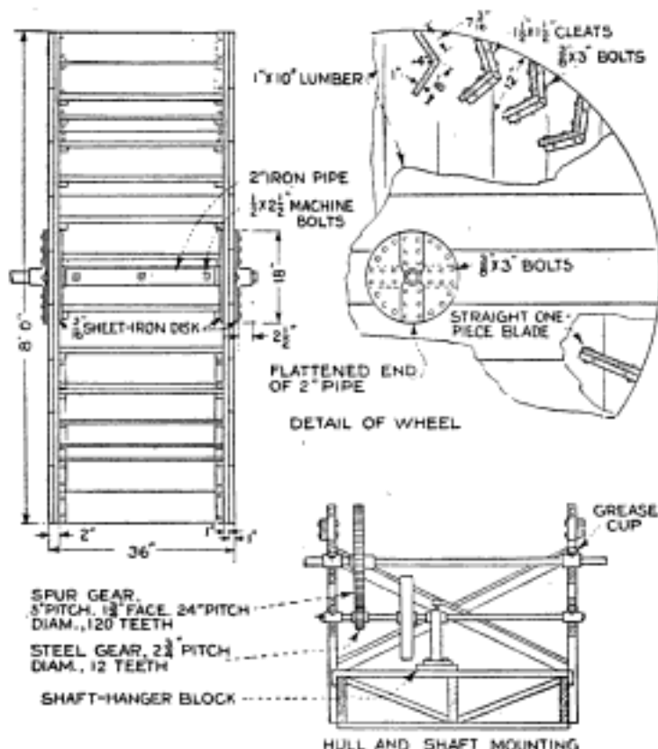
Details of Water Wheels, Showing Method of Attaching Blades and Hubs; Lower Detail Shows Arrangement of Shaft, Gears, Pulley and Cross Section of Hull
