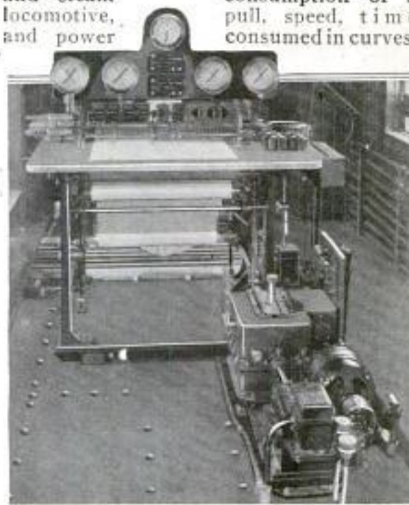
Car Equipped with Automatic Instruments Which Measure Impacts and Record Locomotive Performance
