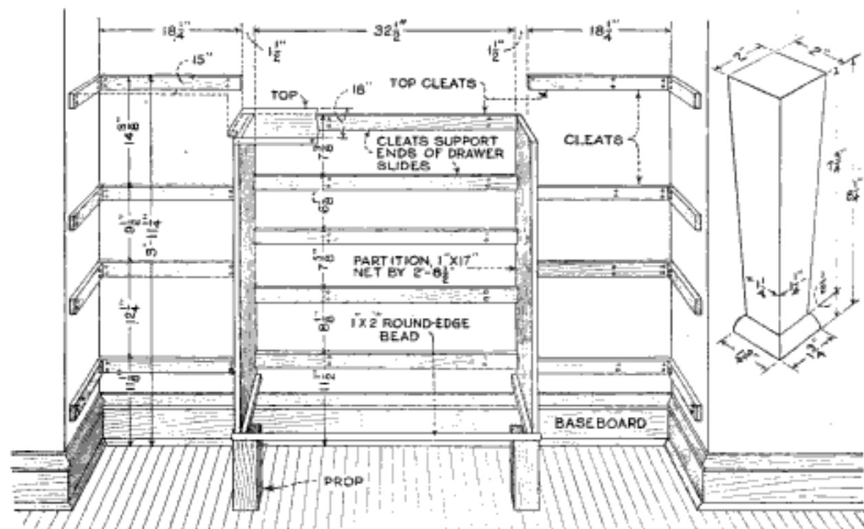
Details of the Shelf and Drawer-Slide Cleats, Nailed to the Wall Studs; Partitions in Place Ready for the Frames, and Detail of Legs
