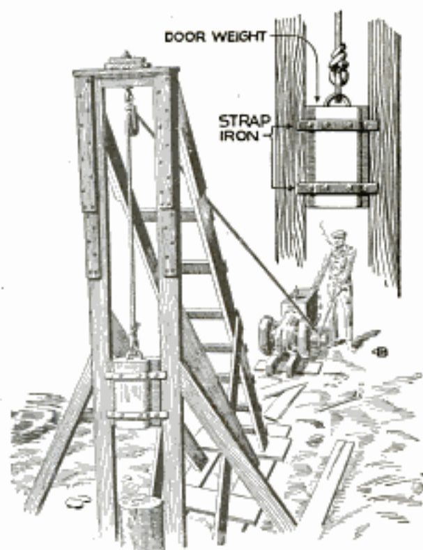
Small Homemade Pile Driver Used by Bridge Contractor Saves Considerable Expense
