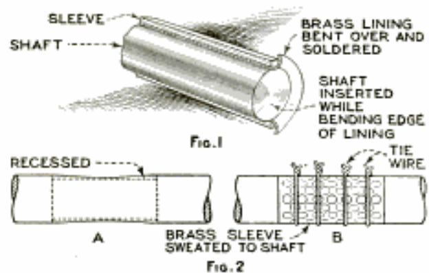
Making Temporary Bushings for Bearings and Building Up Wearing Surfaces of Journals
