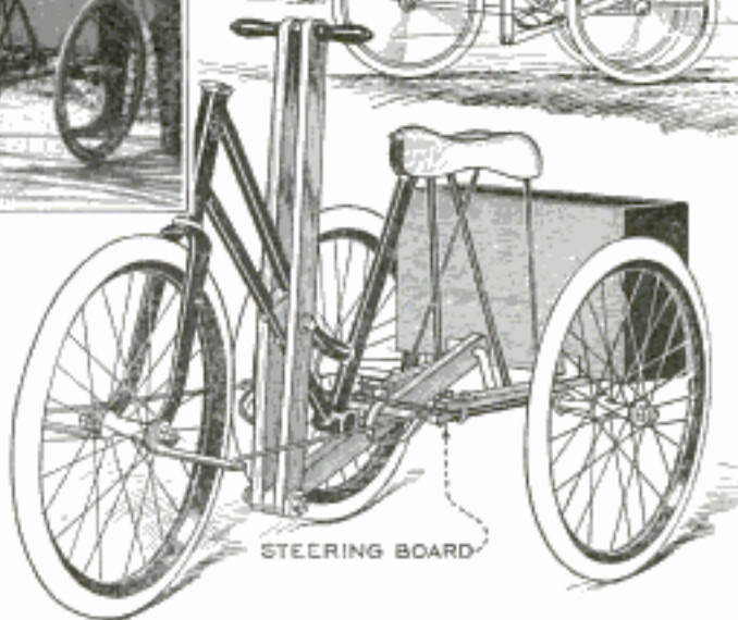
Newsboy's Unusual Three-Wheeled Vehicle Made from Old Bicycle; It Is Driven by Hand and Steered by Foot
