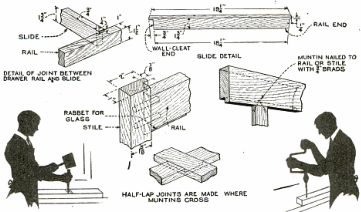
Various Constructional Details; Joints of Drawer Rails and Slides, Door Stile and Rail Joints, Muntin Joints, and Cutting of Drawer Slides
