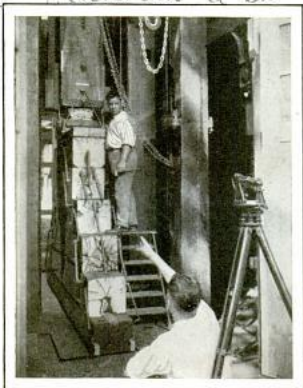
As Big Blocks Were Squeezed in Powerful Press, Cracks Were Measured with Surveyor's Instrument
