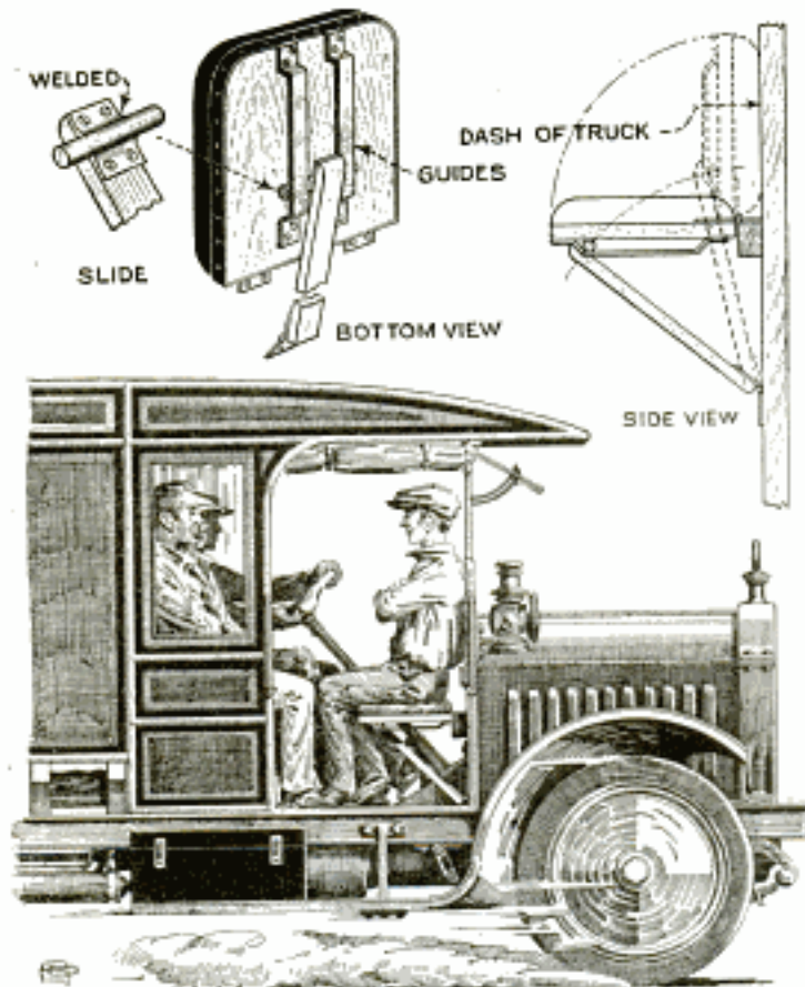
The Extra Helper Is Accommodated on a Long Haul by a Simple Folding Seat in the Cab
