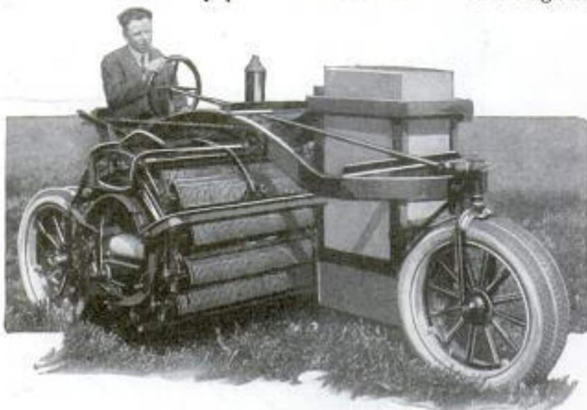
Tractor Cranberry Picker in Operation, Steered by a Single Large Front Wheel, While Revolving Rows of Teeth Remove the Fruit
