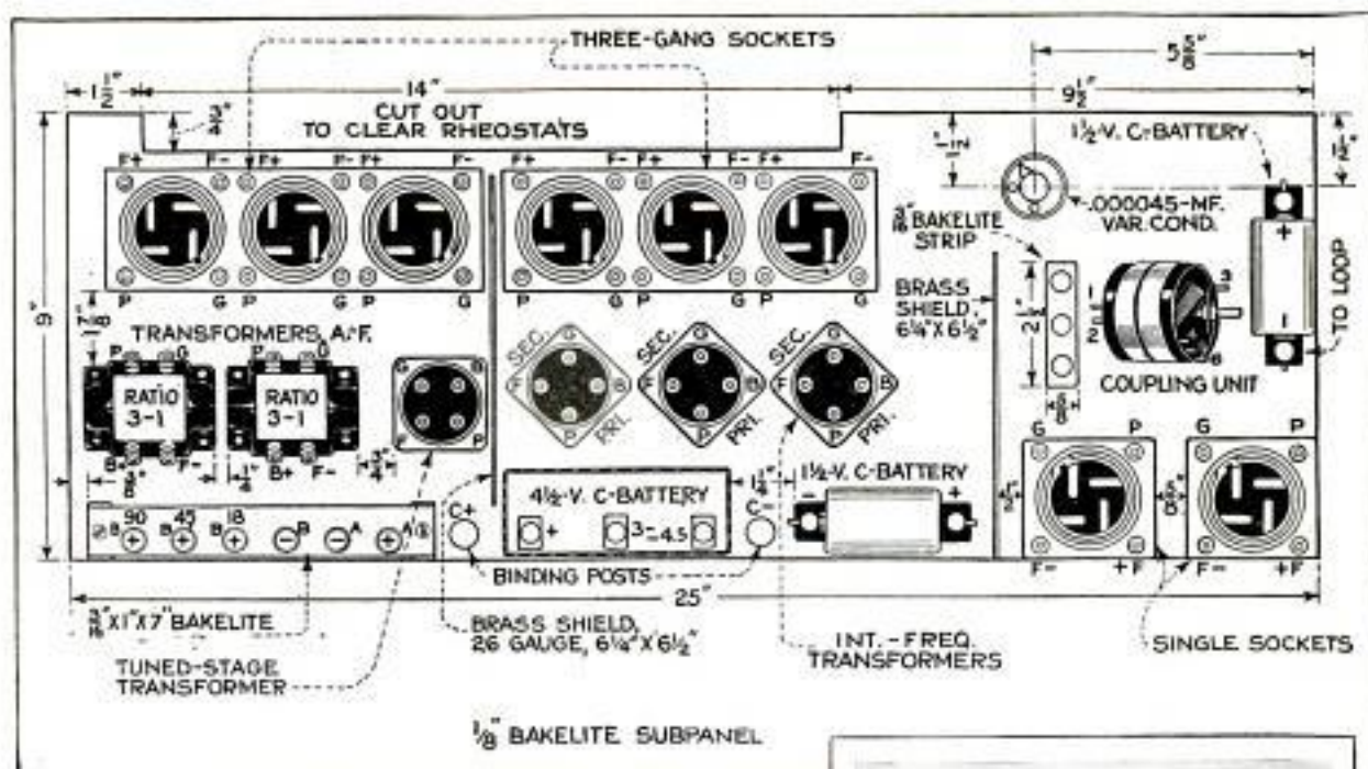
Above, Layout of Subpanel, Showing Location of the Various Instruments; Below, View of Rear of Completed Instrument
