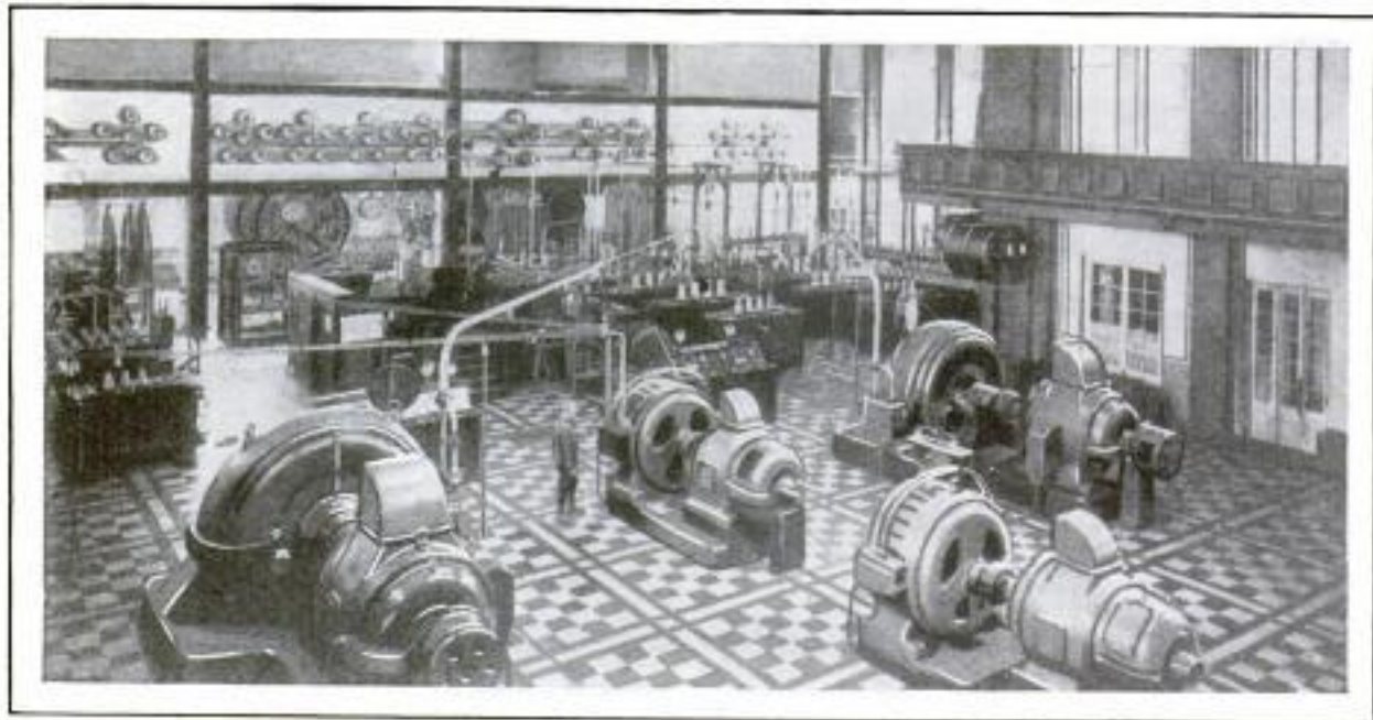
Generating Plant of the Huge Wireless Station at Nauen, Where 1,060 Kilowatts Are Generated as Compared to America's One-Kilowatt, or Less, Broadcasting Stations
