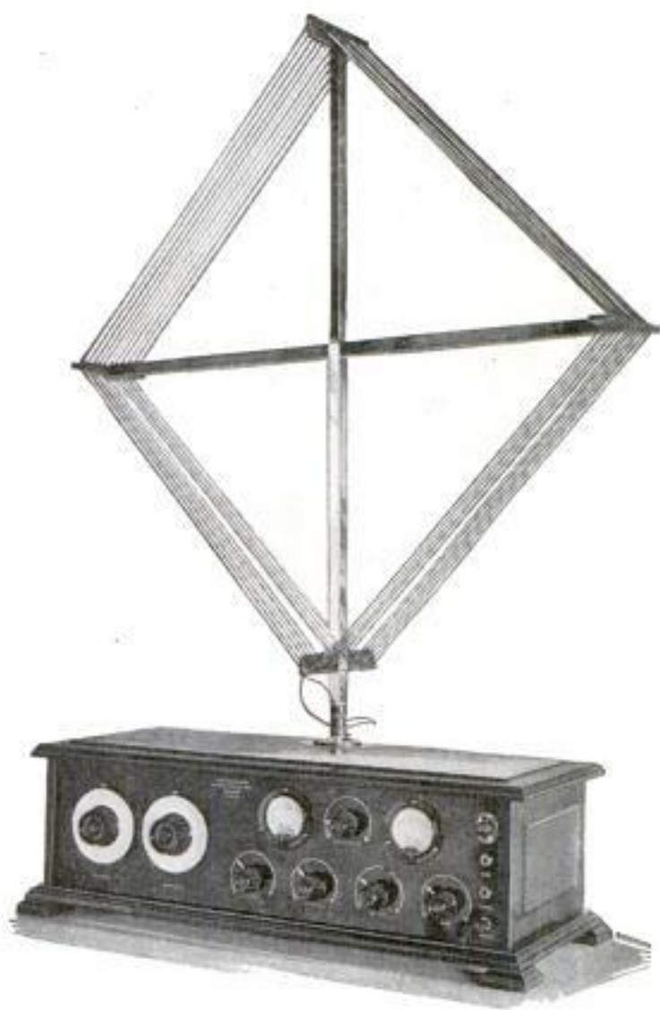
View of the Completed Superheterodyne Receiver, with Collapsible Loop Extended and Plugged into the Jack in the Cabinet Lid
