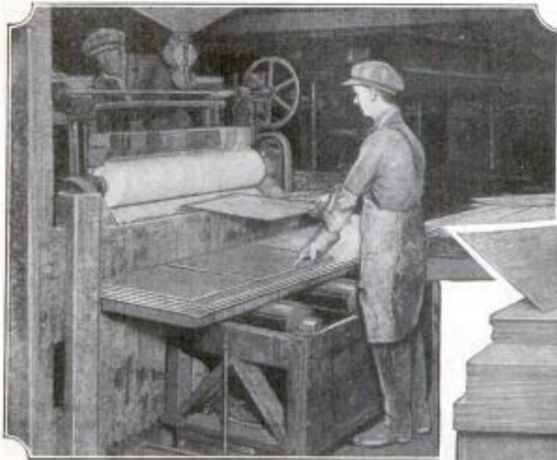
Glue Spreader into Which Center Cores Are Fed for Coating Before Outer Pieces Are Applied
