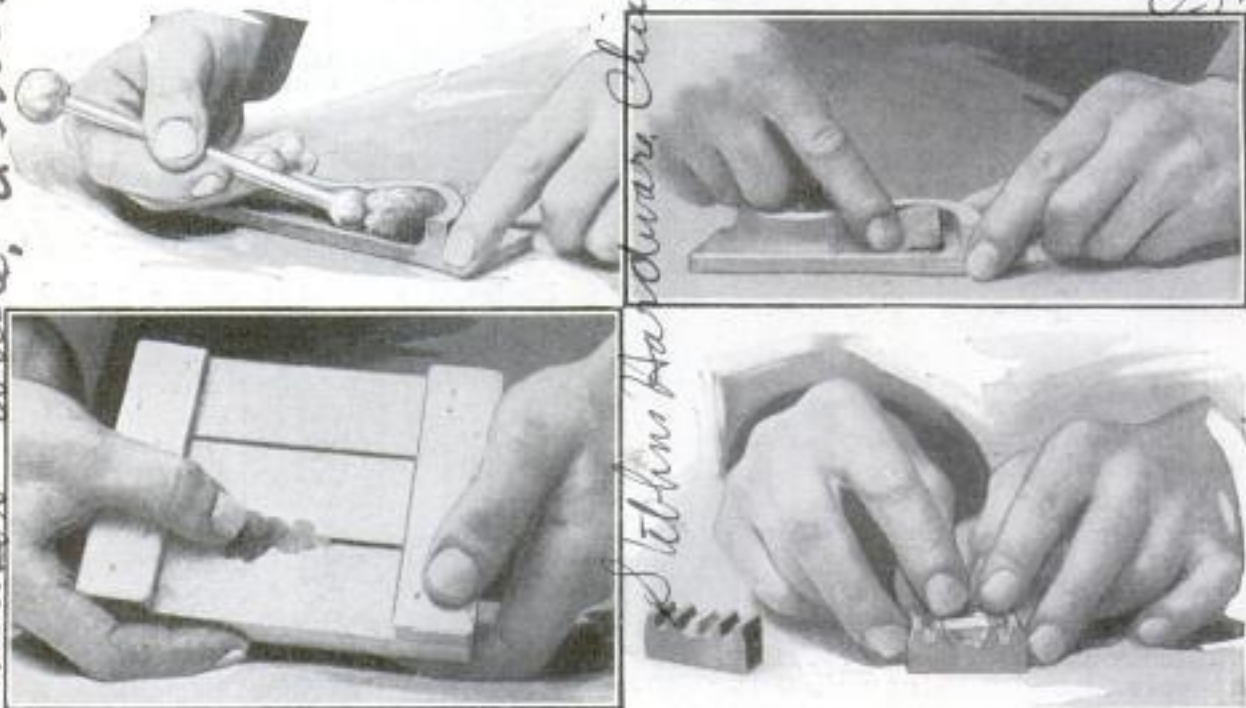
How Plastic Wood May Be Used as Filler for Seams and to Replace the Broken Parts of a Pattern; Above, the Material Being Molded into Ornamental Shapes
