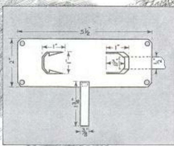
Handy Matchbox Holder for the Autoist; It Is Attached to the Steering Column at a Convenient Height
