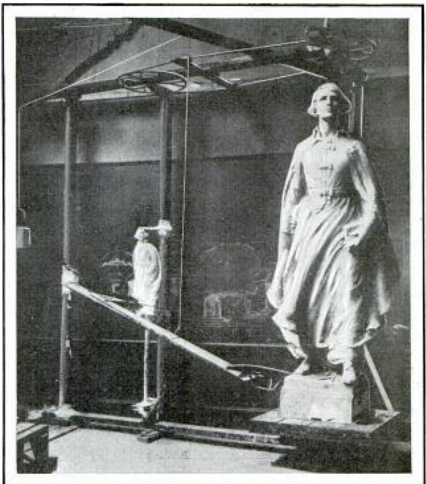
Sculptor's Enlarging Apparatus, Showing Big Piece That Has Been Reproduced with Help of Mechanical Finger Pointing from Tiny Model
