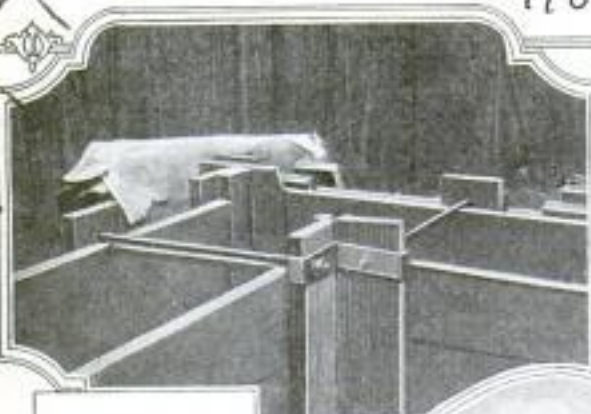
The Forms Are Stronger and More Rigidly Fastened and Braced than for Concrete Walls
