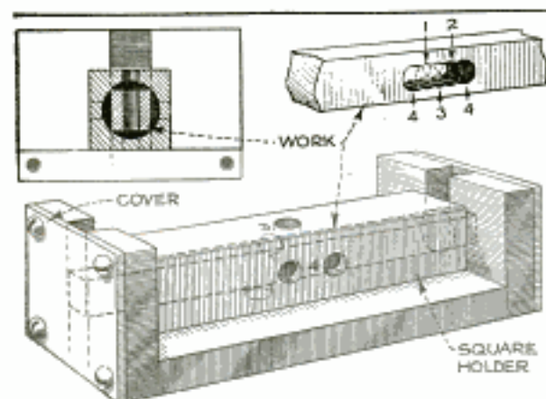
Quick-Action Slot-Drilling Jig for Cutting Slots in Square Shafts
