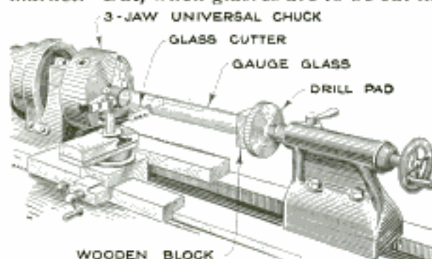
Lathe Set Up for Cutting Quantities of Gauge Glasses into Any Desired Length
