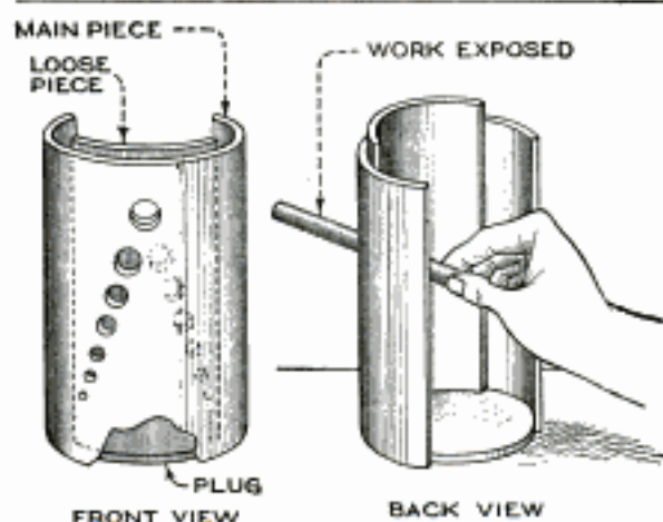
Hardening Small Tools with Acetylene Torch Is Aided by Flame Shield
