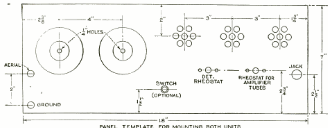
PANEL TEMPLATE FOR MOUNTING BOTH UNITS
