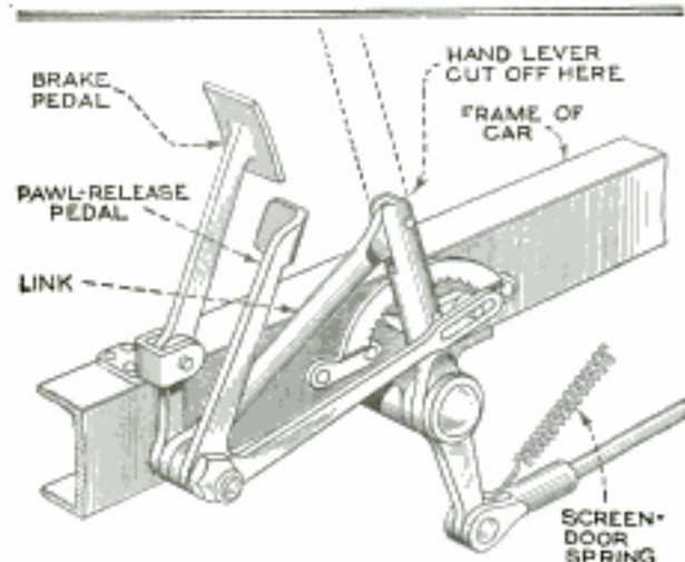
This Simple Attachment Replaces the Hand Lever on the Ford Car
