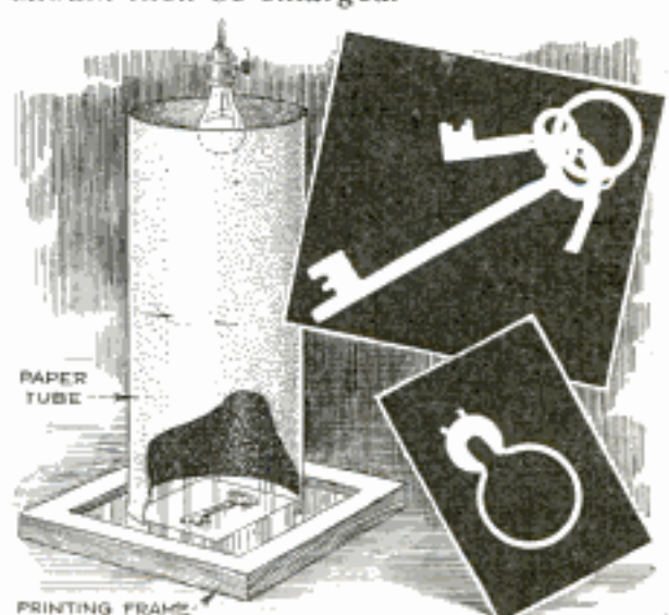
Printing Outline of Irregular Objects on Sensitized Paper to Aid in Measuring Them
