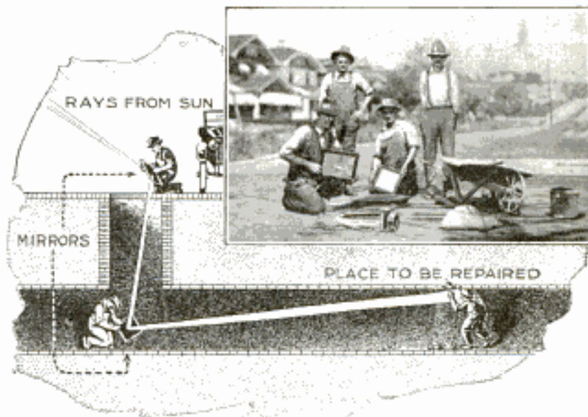
Sun's Rays Reflected Inside of Sewer with Aid of Mirrors Give Workers Plenty of Light
