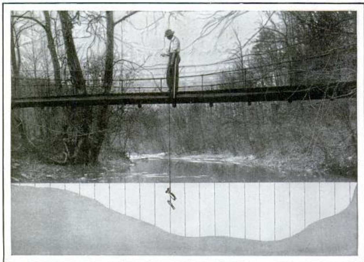
Taking Readings of Water Current and Depths from a Footbridge, Showing a Cross Section of the Stream and the Meter Which Registers the Speed and Volume Passing through the Channel
