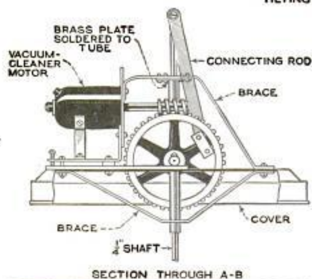
SECTION THROUGH A-B
