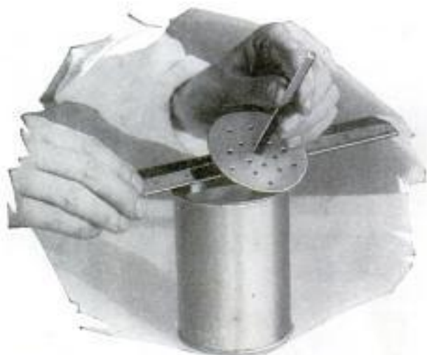
Measuring Proportion of Liquid Content of Can with Graduated Bar Gauge and Ruler
