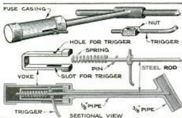
A Welding-Rod Holder Made from Scrap Parts That Will Be of Value in Any Shop
