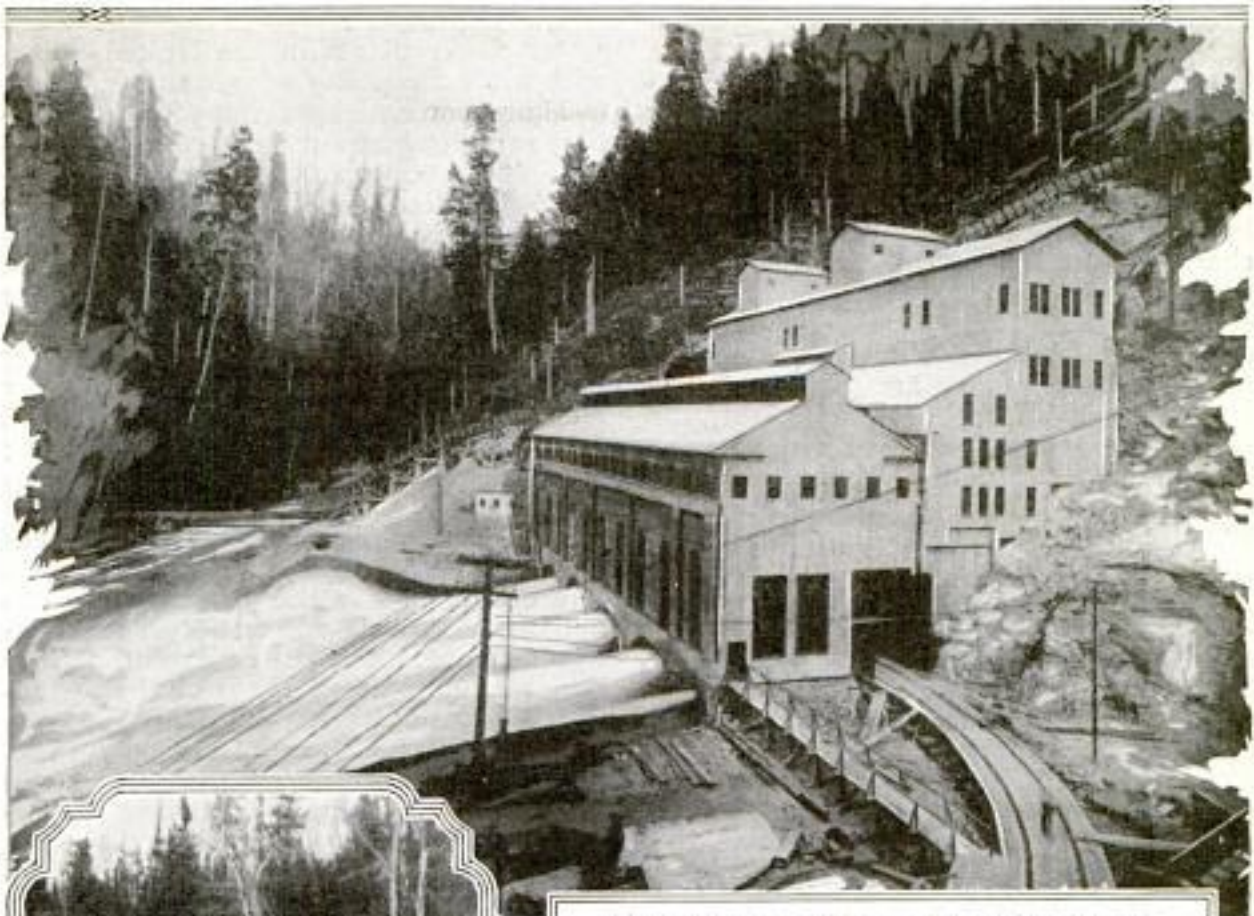
Hydro-Power Plant Where Energy from Remote Mountain Streams Is Harnessed to Produce 20,000 Horsepower of Electric Force; the Current Is Developed under a High Head of Water, as Is Shown by the Rush of the Tailrace
