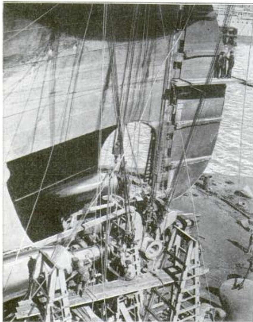
Slipping a New Propeller into Place on the Steamship "Olympic" after It Was Raised from the Water by the Giant Drydock
