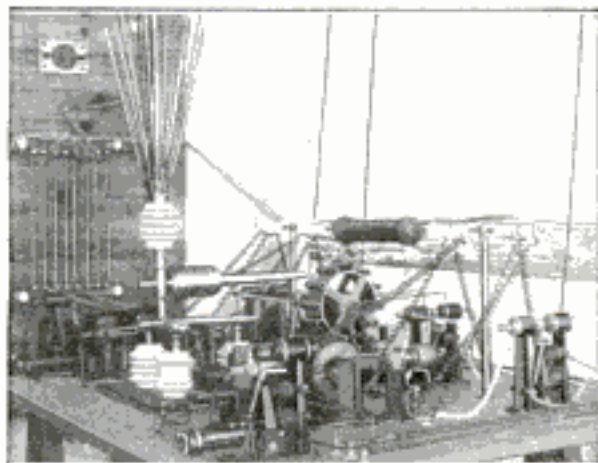
Insulated Aerials, Transformers and Batteries of Apparatus to Gather Electricity from the Air
