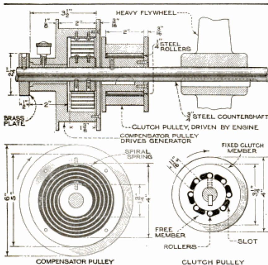
A Spring-Controlled Compensating Clutch on Countershaft with Separate Flywheel Prevents Fluctuation of Lights Connected Directly to Generator
