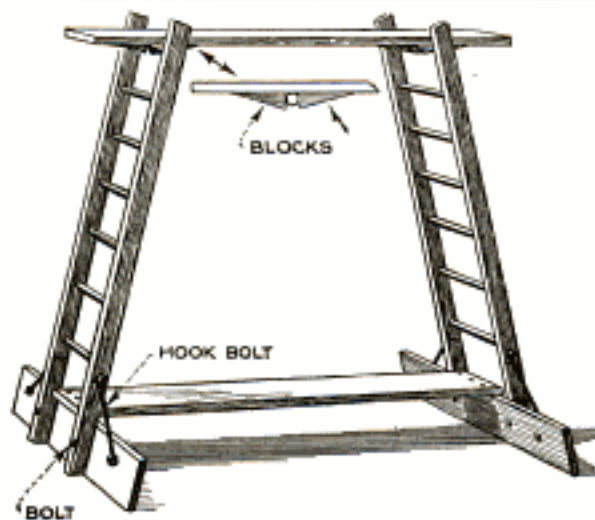
Portable Ladder Scaffold that Has Been Found Very Convenient for Reaching High Ceilings
