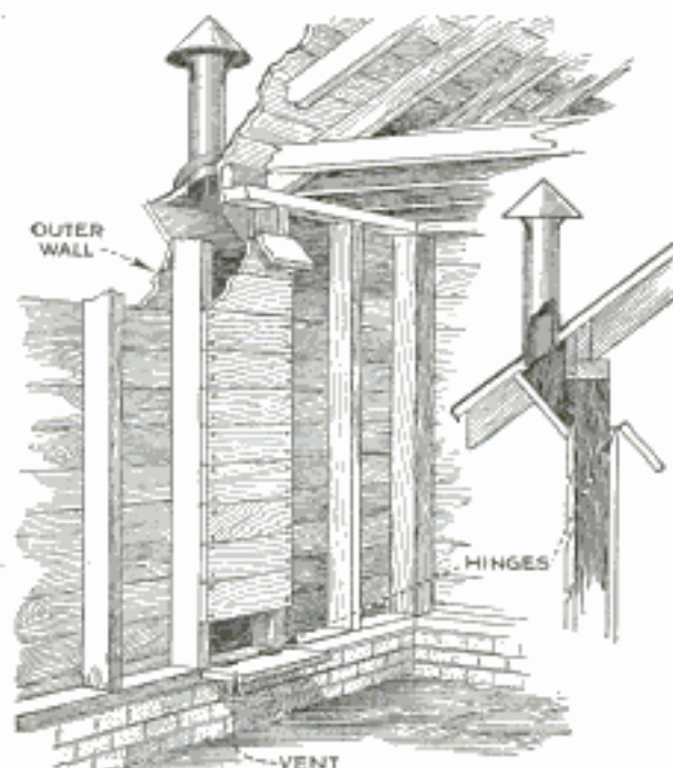
Proper Ventilation in Barns Provided by Means of a Simple Installation
