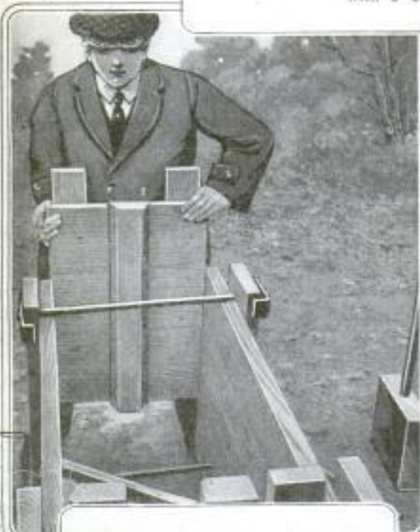
Setting the End Board into the Form; Note Solid Construction
