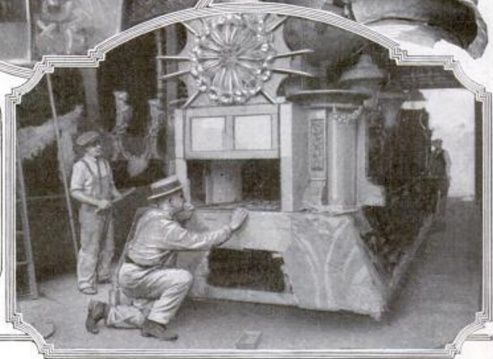
Laying Outer Paper Covering on Wire Framework at Base of Float before Applying Finishing Paints and Decorations; Batteries and Switches for Illuminating Piece Are Put in Opening above Worker's Hand
