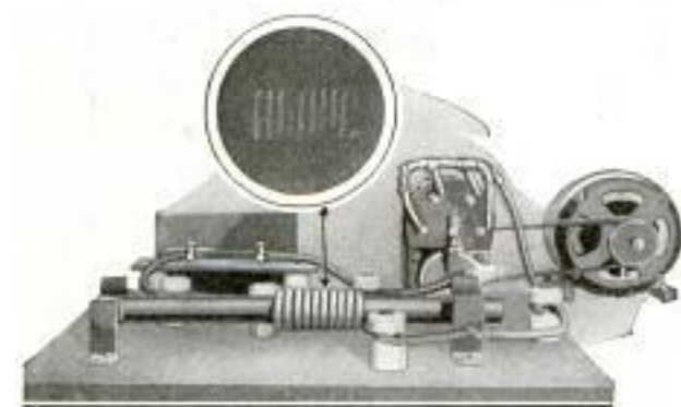
Electric Testing Apparatus Trying Out Insulation on Wire Wrapped around a Charged Steel Bar
