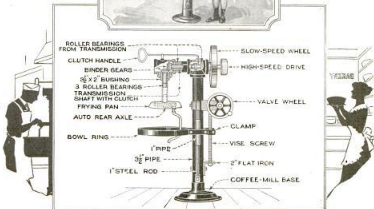
A Mixing Machine for the Small Bakery That Cost Less than $10, and Mixes Dough, Mashes Potatoes and the Like, Much Quicker than the Operations Can Be Done by Hand
