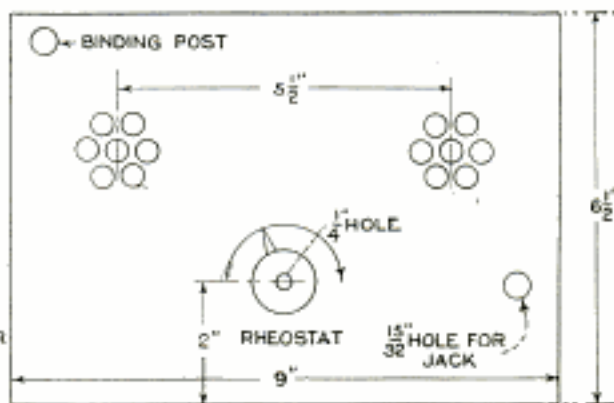
SIMPLE PANEL TEMPLATE FOR TWO-STEP AMPLIFIER UNIT
