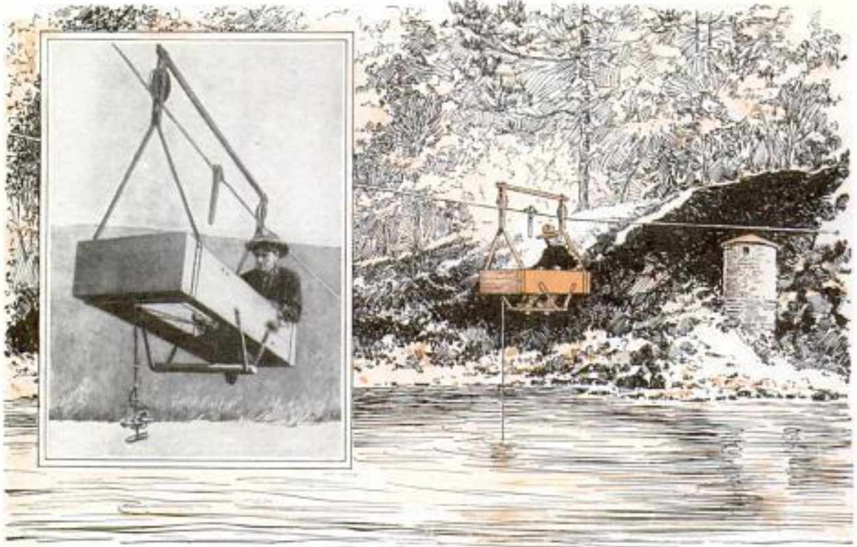
Where Bridges Are Absent, the Water-Power "Scout" Spans the Stream with a Cable and Basket Car, Dropping and Raising the Gauge as He Propels the Carrier along the Aerial Track
