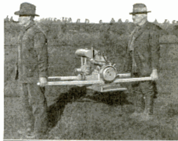
Transporting Portable Fire Pump to Aid in Fighting Blaze in Isolated Stretch of Woods
