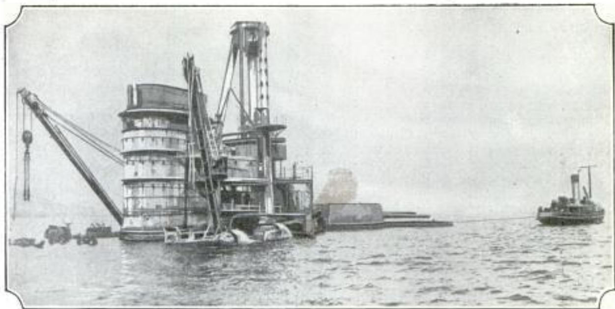
Salvaging the Former German Battleship "Hindenburg" from the Muddy Bottom of Scapa Flow, Where It Was Sunk with More Than a Half Hundred Similar Craft Over Five Years Ago
