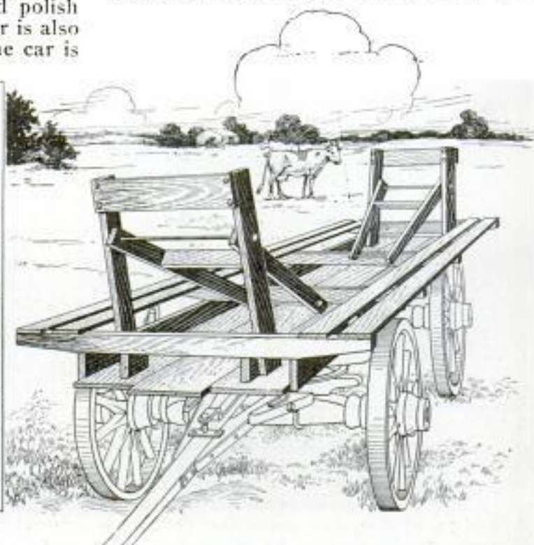
Folding End Ladders on the Hayrack Are of Considerable Convenience When Using a Hay Loader or When Passing through Orchards
