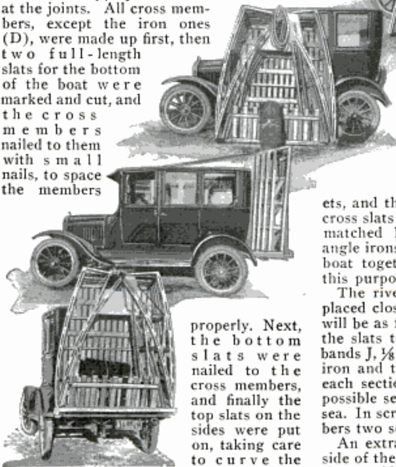
Four Views Showing How the Portable Canvas Boat Is Knocked Down and Mounted on a Small Car for Transportation
