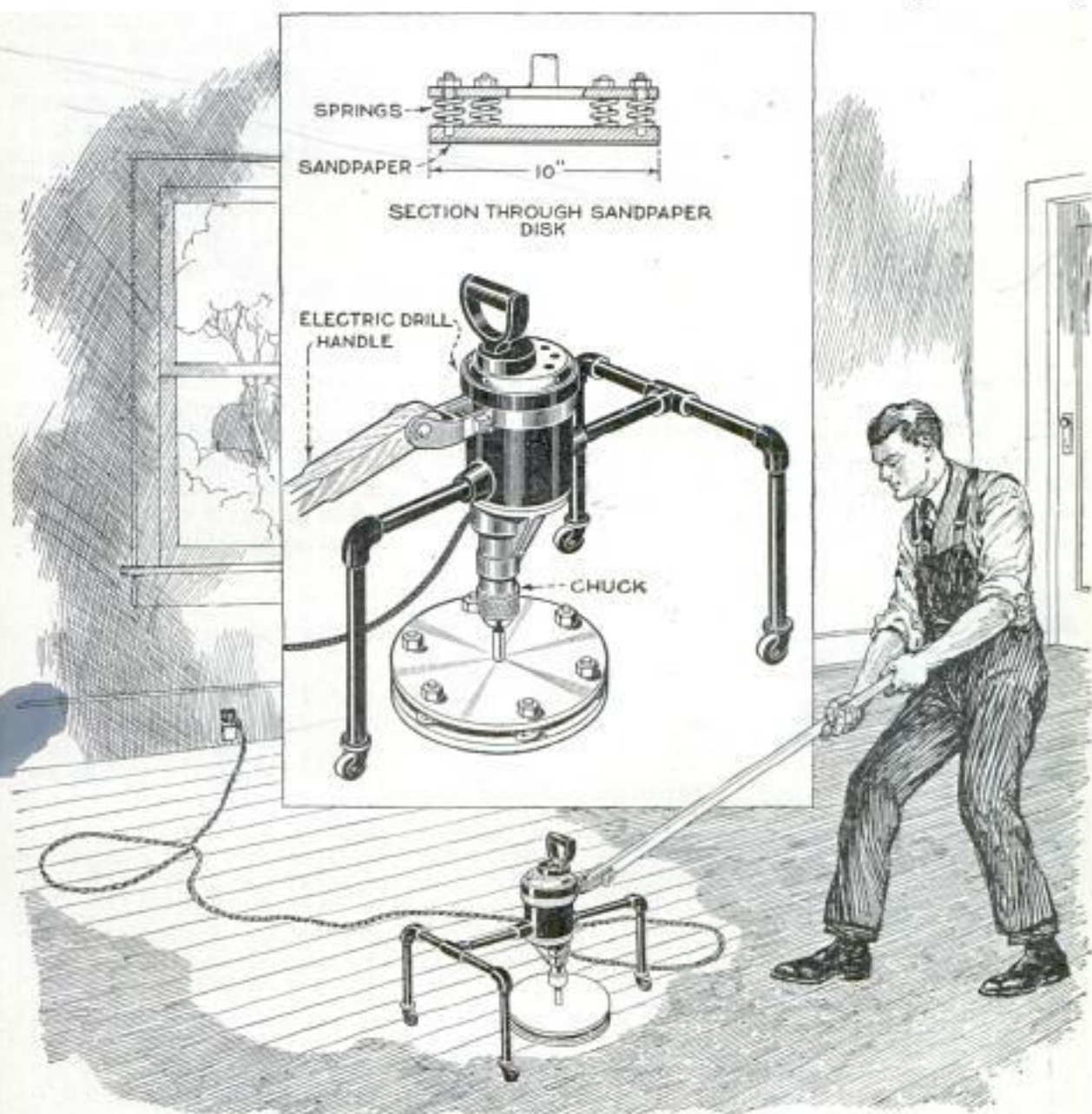
Portable Floor-Sanding Machine, Consisting of a Small Electric Drill and a Pipe Framework Mounted on Casters, Enables Carpenters and Painters to Sand Floors Quickly and Satisfactorily
