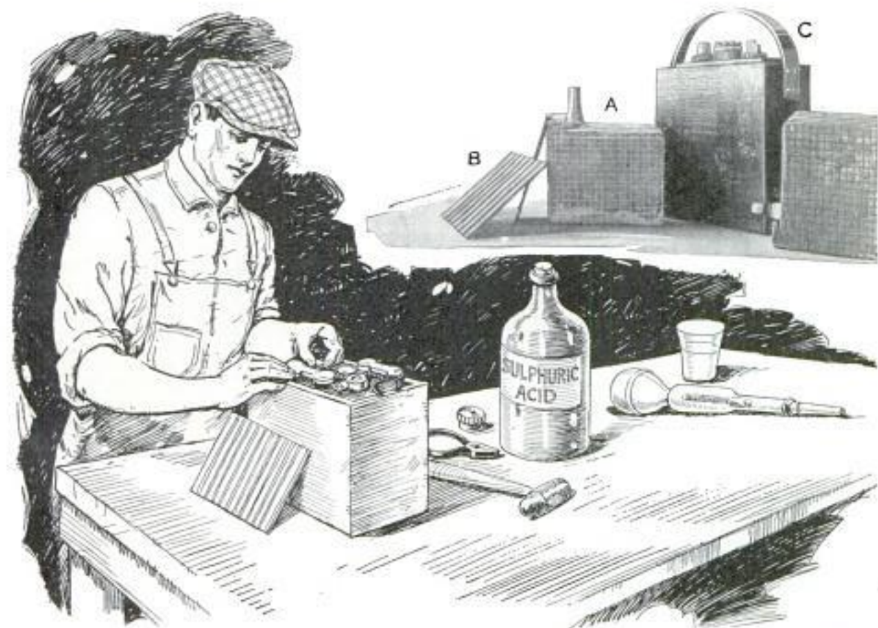
Set of Negative Plates as Taken from the Battery Shown at A; B Is the Separator and C the Finished Battery; This Cell Has the Original Filler Plug, but if This Is Spoiled, a Cork Can Be Used as Suggested
