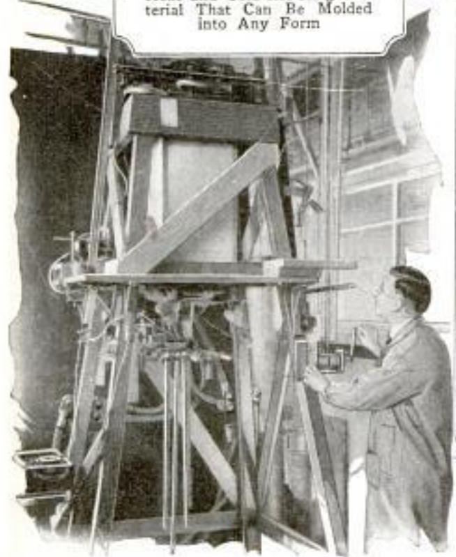
Making Rods of Fused Quartz Which Is Forced by a Heavy Weight through Shapers as It Flows Hot from Furnace, and Tubes of the Crystal Used for Experimenting with Light
