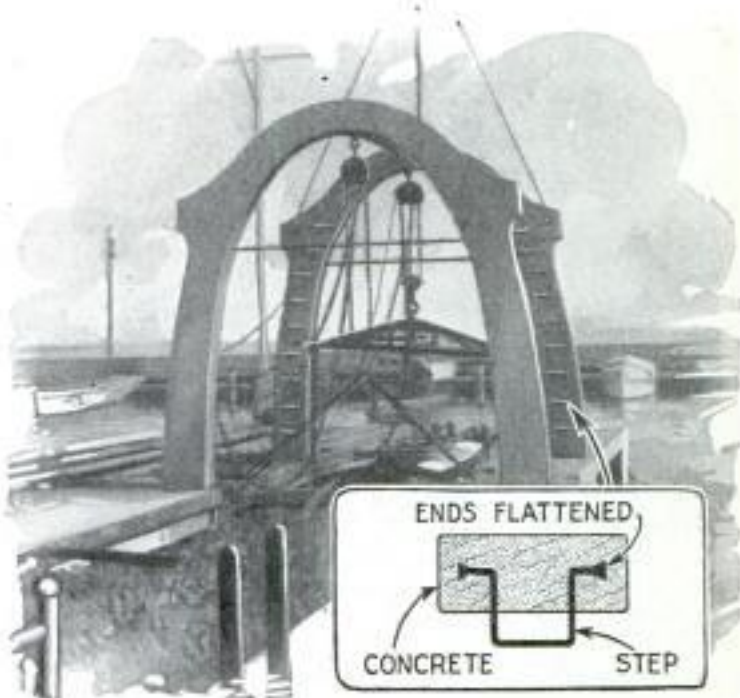
Useful Concrete Hoist, of Novel Design and Permanent Construction, for Lifting Small Boats Out of the Water
