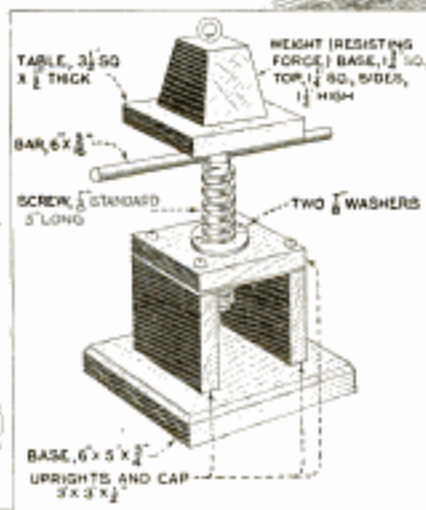
Detail Drawing for Constructing the Model of the Simple Screw with Illustrations Showing How It Is Used
