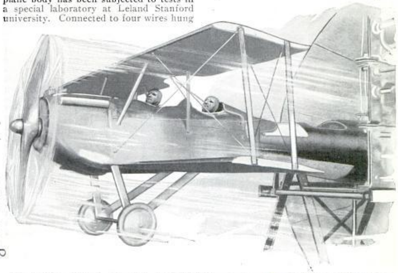
Model Airplane Flying in Motor-Made Gale While Undergoing Experiments for Design of Propeller and Wing Curves in Special Laboratory of Leland Stanford University
