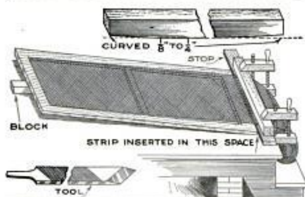
Covering Screen Frames with New Wire Cloth Is Greatly Simplified by the Method Illustrated
