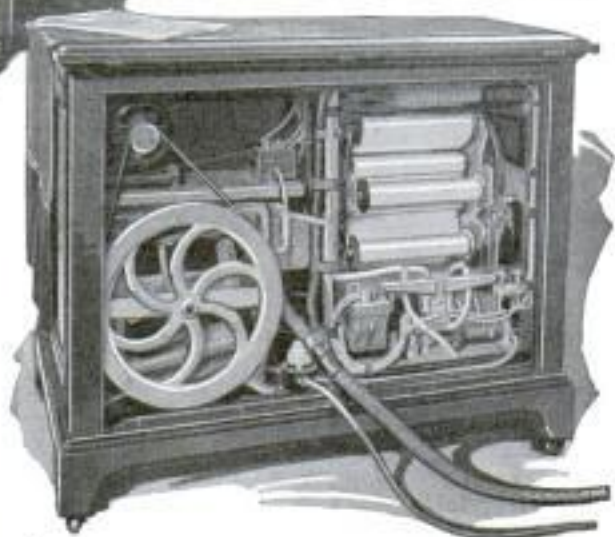
Push-Button Record Selector in Use and Interior View of Playing Side of Cabinet, Showing Cable Connections and Rolls on Battery of Reels
