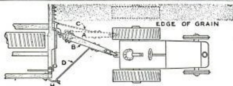
Arranging a Binder Hitch So That It Can Be Used with a Small Tractor, Enables the Farmer to Harvest More Effectively
