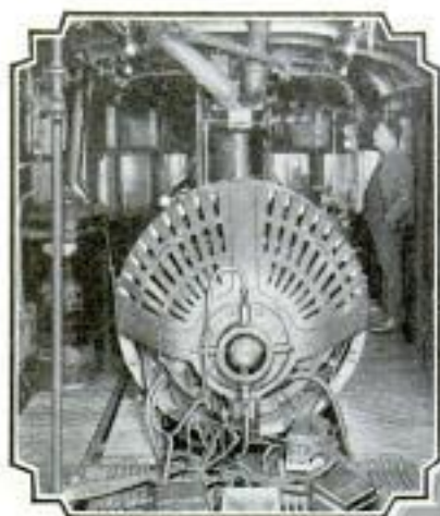
Electric Switch Engine Which Can Be Operated at One-Third Fuel Costs of Coal-Burning Locomotives; Left, View of Interior Showing One of Fifty-Horsepower Motors
