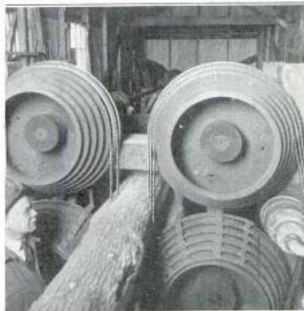
Multiple Band-Saw Ribbons That Cut Several Boards from a Single Log at Once
