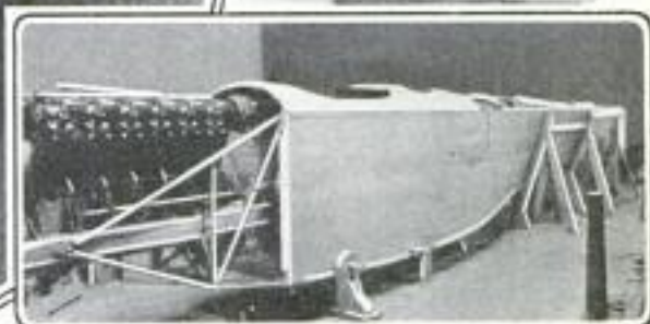
Flying Boat with Fuselage and Hull Built of Aluminum Alloy; Left, Working on One of the Light Metal Girders, and Right, Airplane Body in Course of Construction
