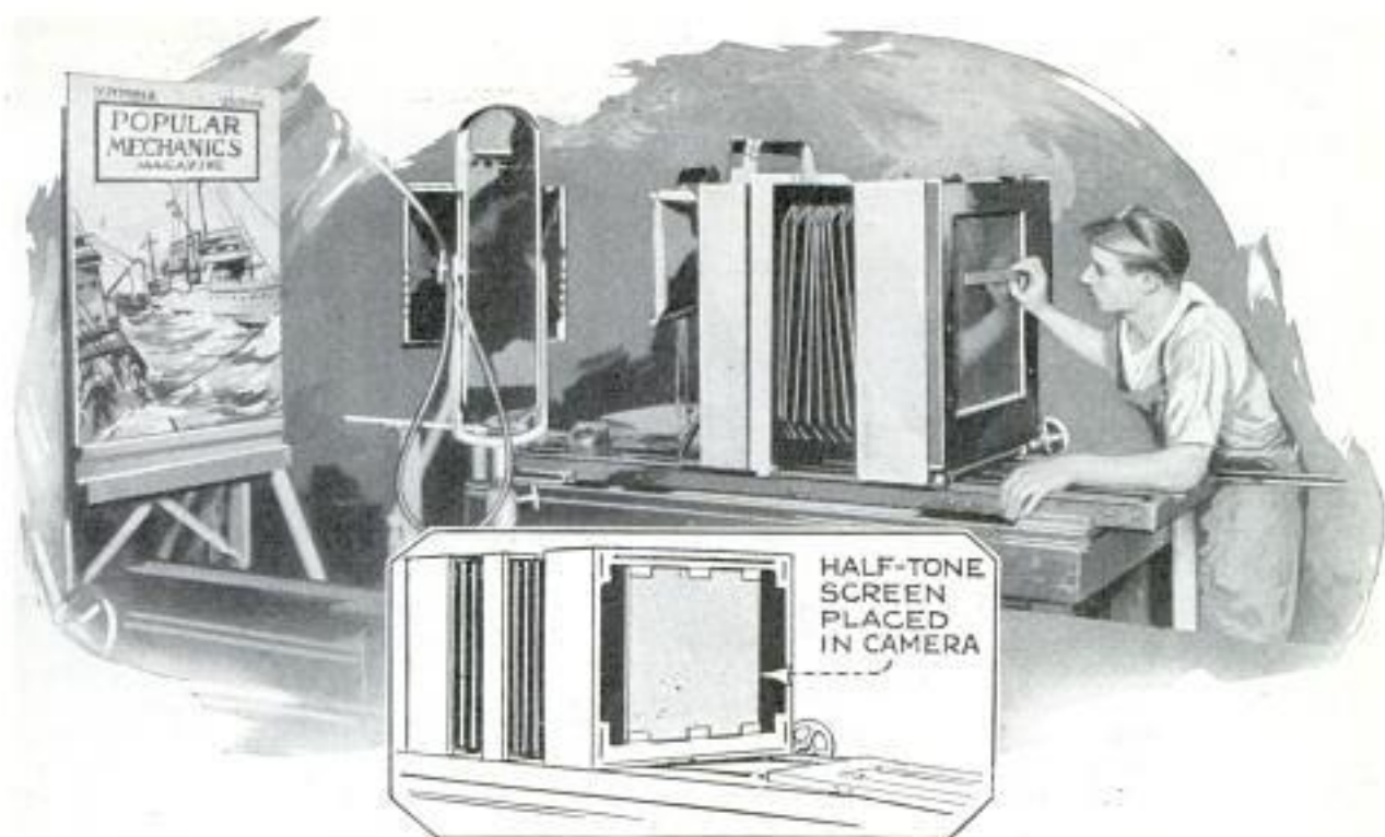
Carefully Focusing the Camera to Get a Sharp Picture of the Object in the Right Size for the Half-Tone Negative Is the First Step in the Process
