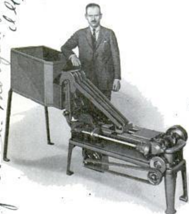
Machine with Capacity of Cracking 1,200 Pounds of American Walnuts in Eight Hours
