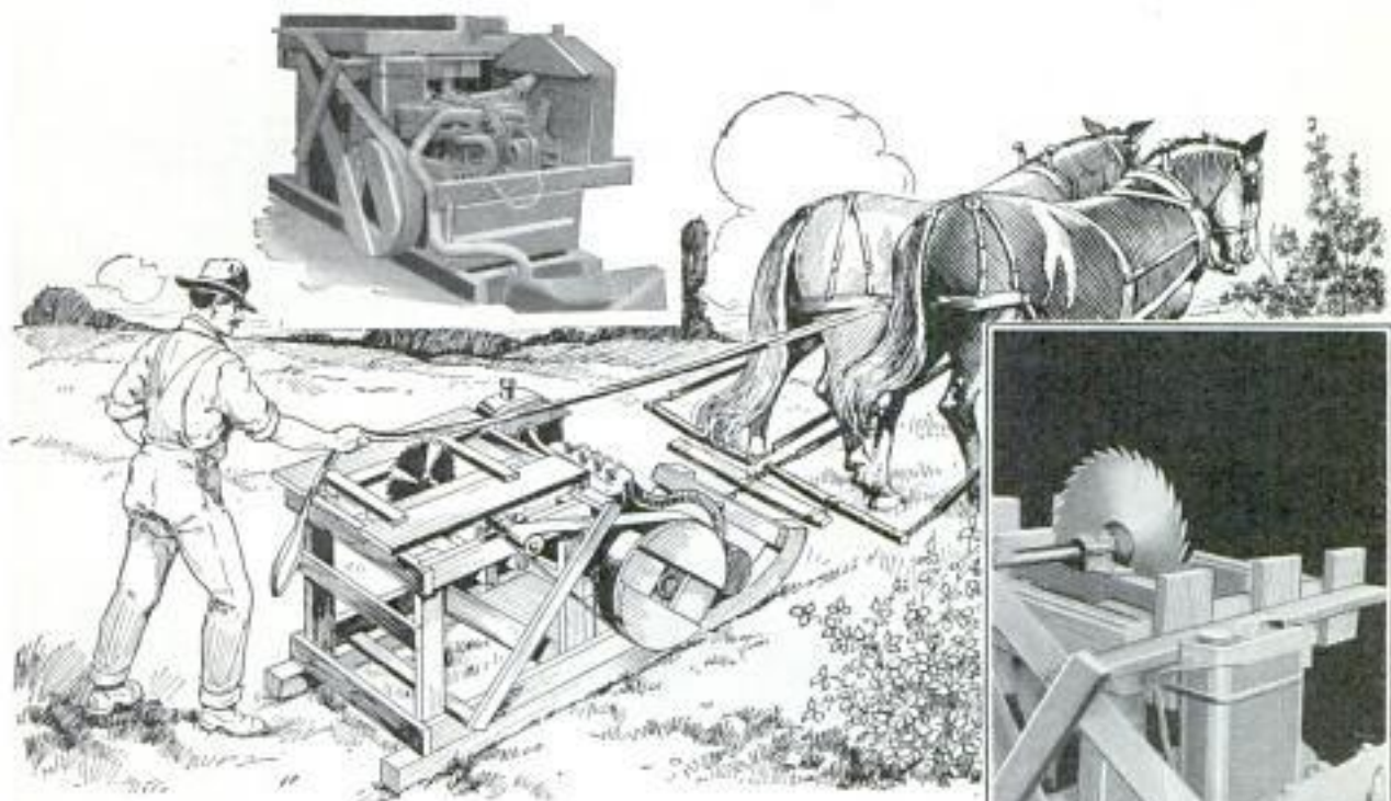
Above, Engine End of Saw Frame; Center, Saw Mounted on Skids for Farm Use; Right, Closeup of Table Guides and Gasoline Tank on Frame
