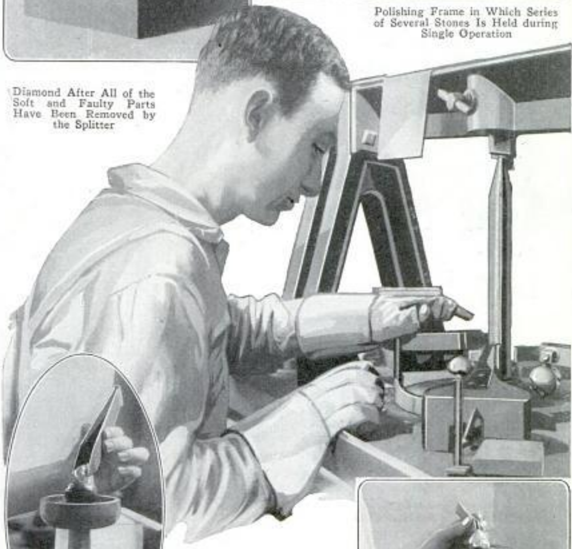
Setting the Mounts Containing Raw Gems in Holding Frame of Polishing Machine; Left and Right, Shaping the Soft Mold for the Diamond, and Placing the Stone in the Tip of the Cone
