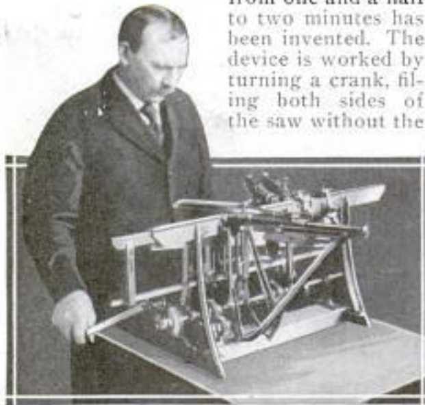
Inventor with Machine That Files and Sets Teeth of Saw at Same Time
