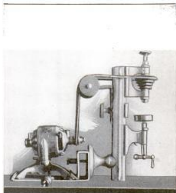
Discarded Watchmaker's Lathe and Sewing-Machine Motor Make Precision Drill Press
