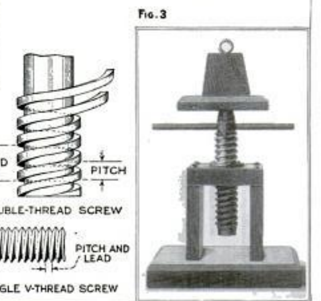
Diagrams Showing the Principle of the Screw, and Illustrating the Difference between Pitch and Lead in Single and Multiple-Thread Screws; Right, Model of Screw
