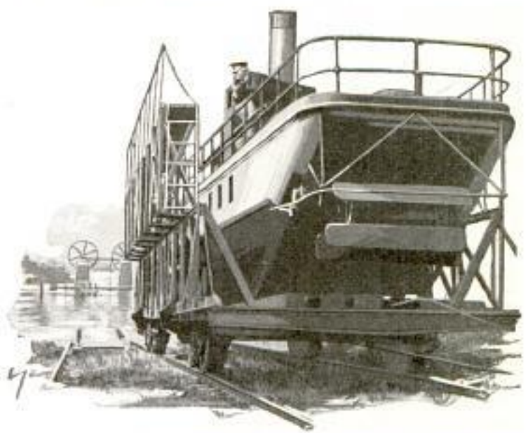
Flat Car Carrying Ship down Incline to Launch It in Deep Water after Transporting the Craft over Land
