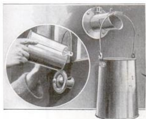
When Knob Is Drawn Out, Milk Is Poured into Pail through Door Spout
