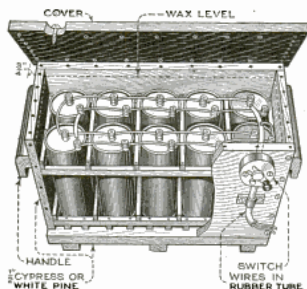
A Battery Box That Will Appeal to Motorboat Owners, as It Is Completely Waterproof
