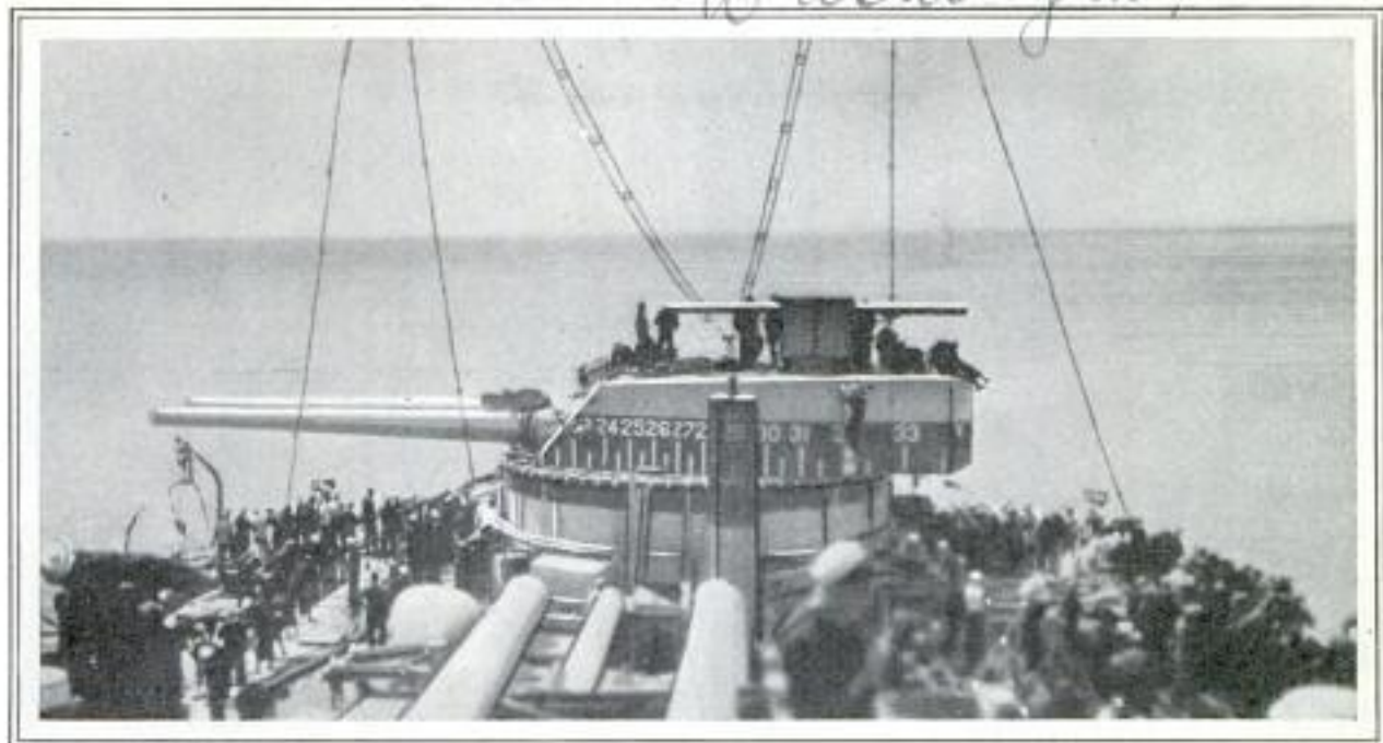
Gun Turret of Big War Vessel with Indicating Dial Set to Inform Gunners of Following Ship of Location and Identity of Target on Which Its Rifles Are Trained
