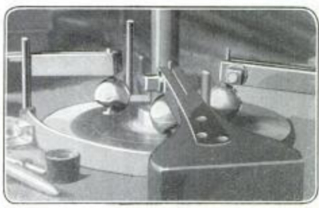
Polishing Frame in Which Series of Several Stones Is Held during Single Operation
