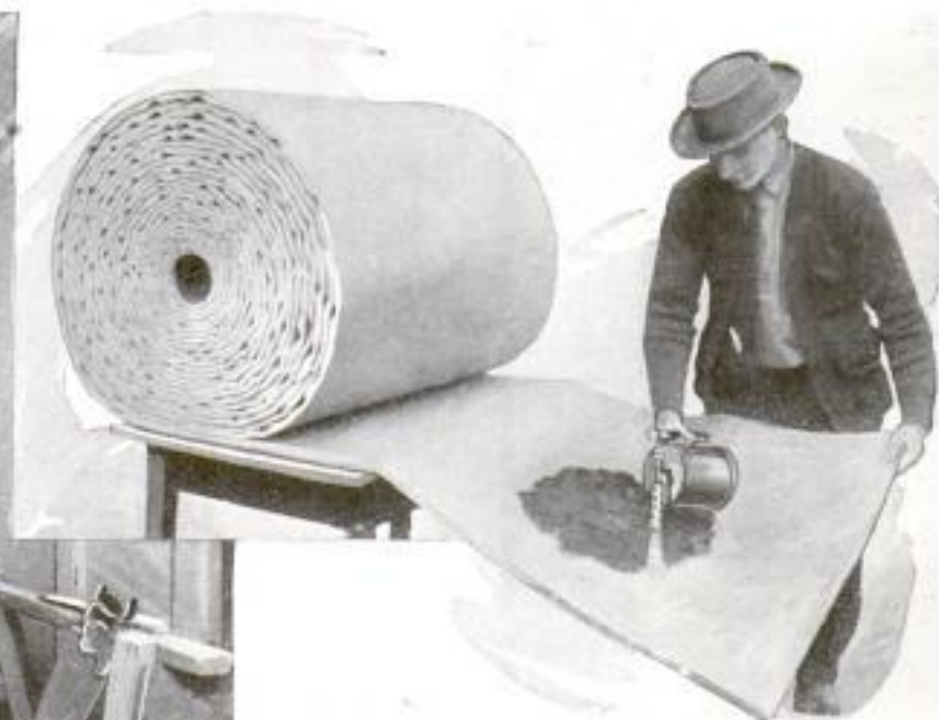
Trying Fireproof Qualities of Wood Wool for Building Walls with Flame of Blowtorch, and Left, Attaching the Sheets Inside of Frame for House to Prevent Entrance of Cold
