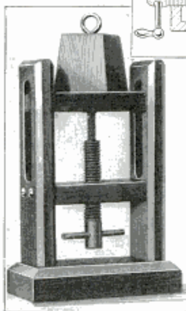
Model of the Differential Screw: Above, One Application of This Mechanism
