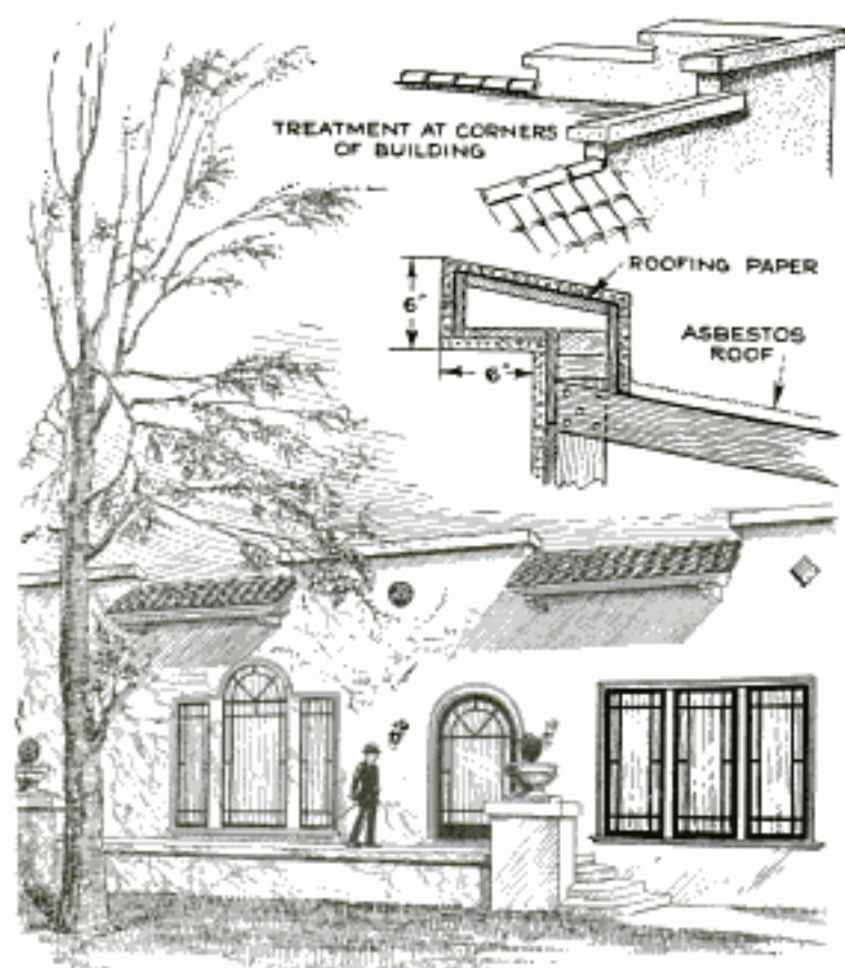
Wide Coping Slanting toward the Inside Prevents Rain and Dirt from Running Down the Outside Wall
