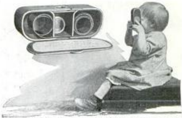
Method of Viewing Scenes in Pocket Movie Machine, and Case Open Showing Film
