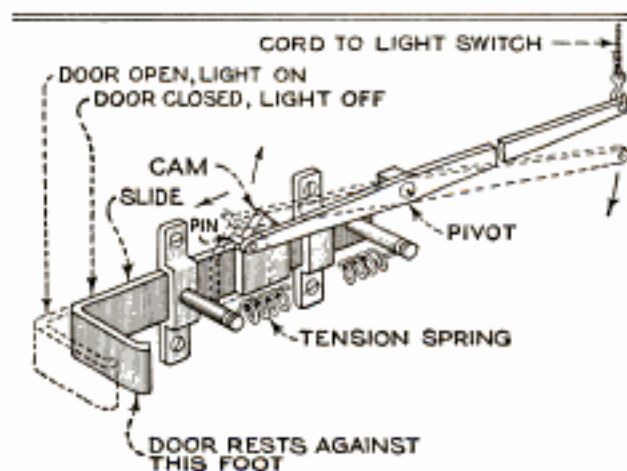
Attachment for Operating Electric Garage Light Automatically by Opening and Closing Door
