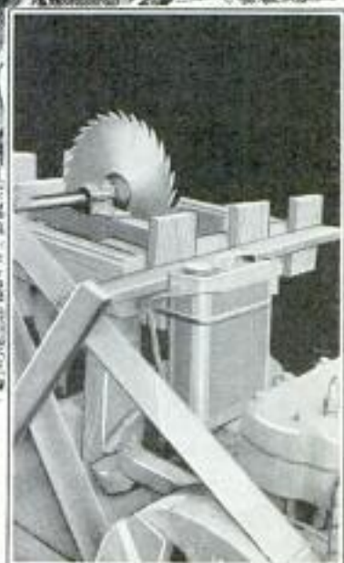
Above, Engine End of Saw Frame; Center, Saw Mounted on Skids for Farm Use; Right, Closeup of Table Guides and Gasoline Tank on Frame
