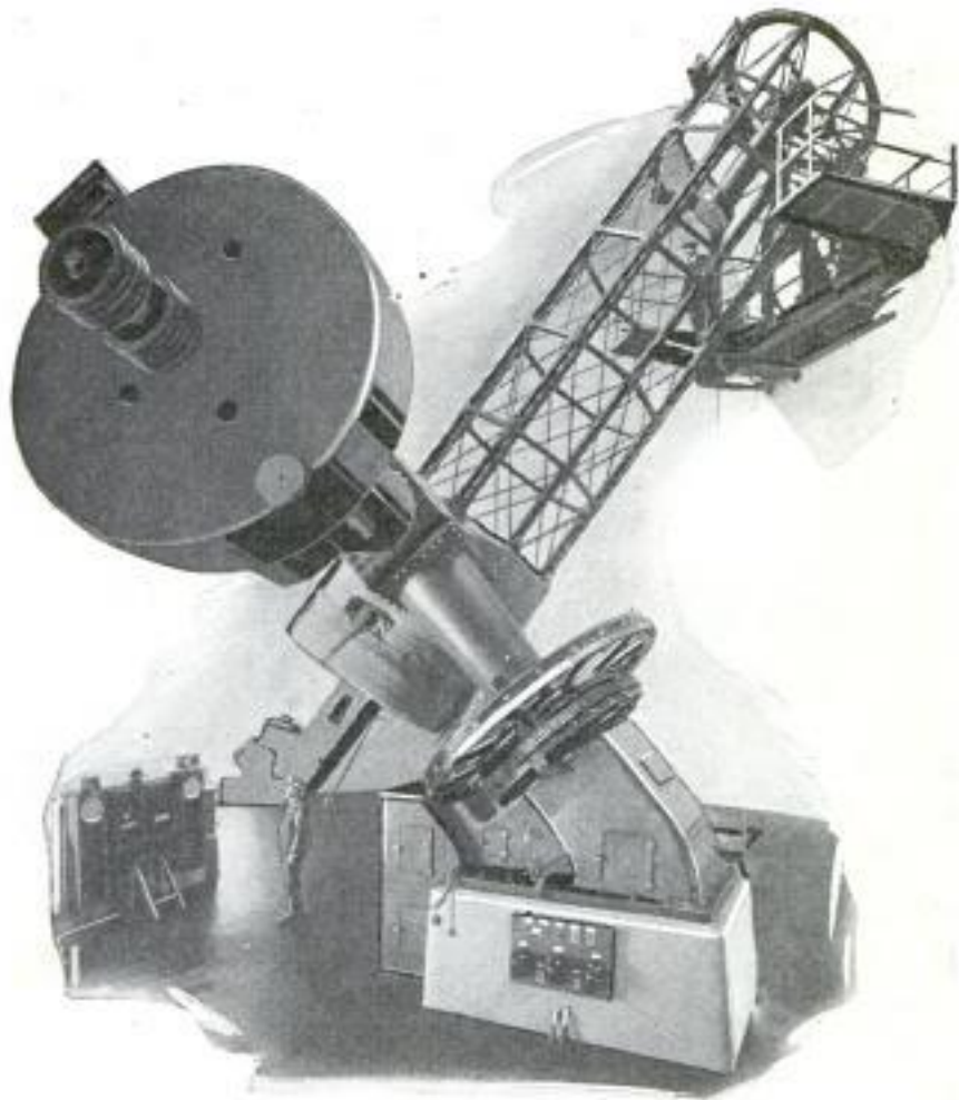
Forty-Ton Telescope by Which Efforts Will Be Made to Get Close-Up Photograph of Planet Mars and Any Possible Evidence of Life
