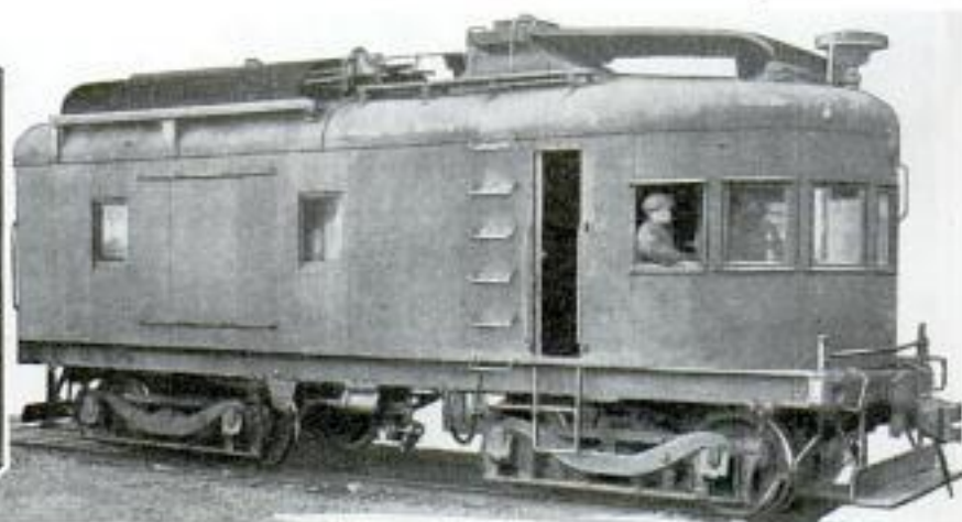
Electric Switch Engine Which Can Be Operated at One-Third Fuel Costs of Coal-Burning Locomotives; Left, View of Interior Showing One of Fifty-Horsepower Motors
