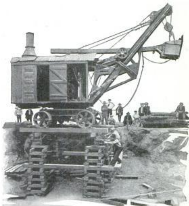
A Novelty in Small Cellar Excavation: the Shovel Was Jacked Up and Removed from the Hole on Rollers
