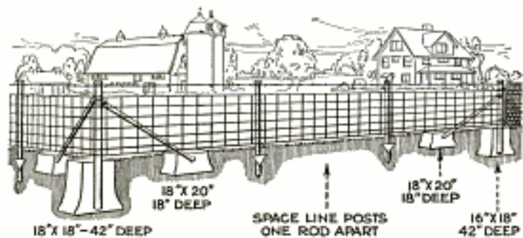
Proper Method of Setting Steel End and Corner Posts in Concrete Foundations
