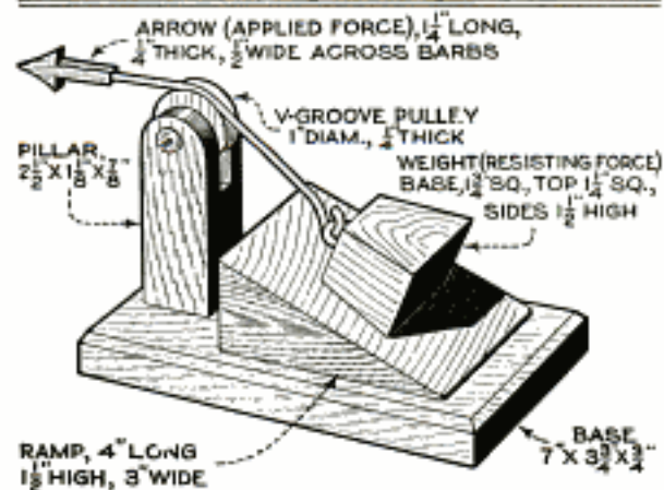
Details of Model of Inclined Plane; Above, a Modern Use of the Ramp
