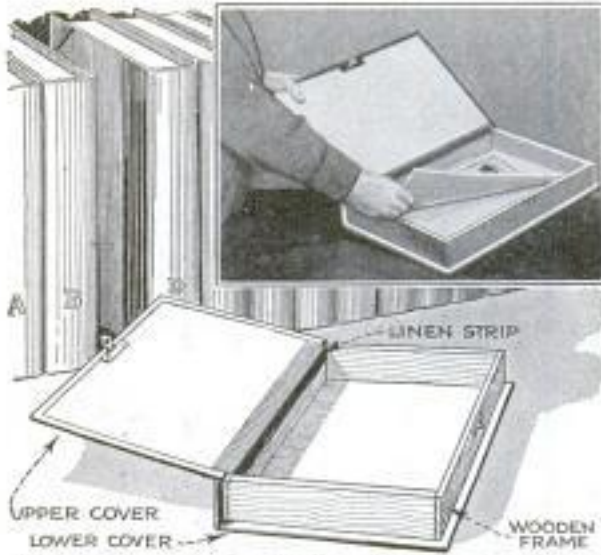
Letter-Filing Boxes Made from Covers of Discarded Books; the Frame Is of Thin Wood
