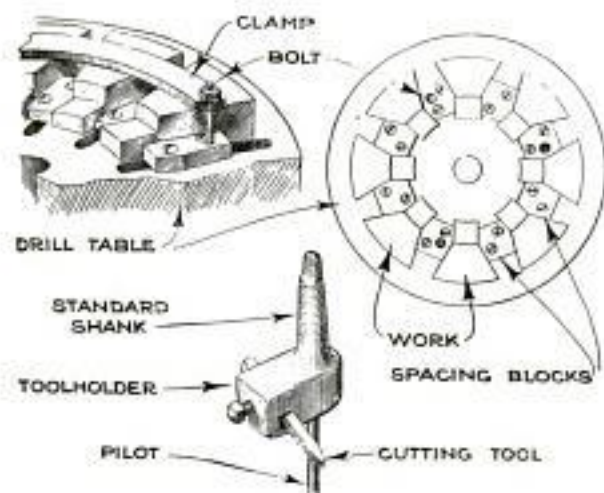
A Method for Turning Radii on a Drill Press, Adapting the Machine to Production Work
