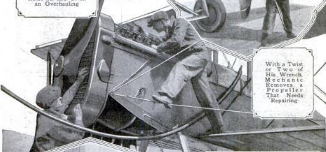
At End of Run, Mechanics Remove Engine Cowl to Inspect Motor, Radiator and Running Parts; Hose in Foreground Is Replenishing Tank
