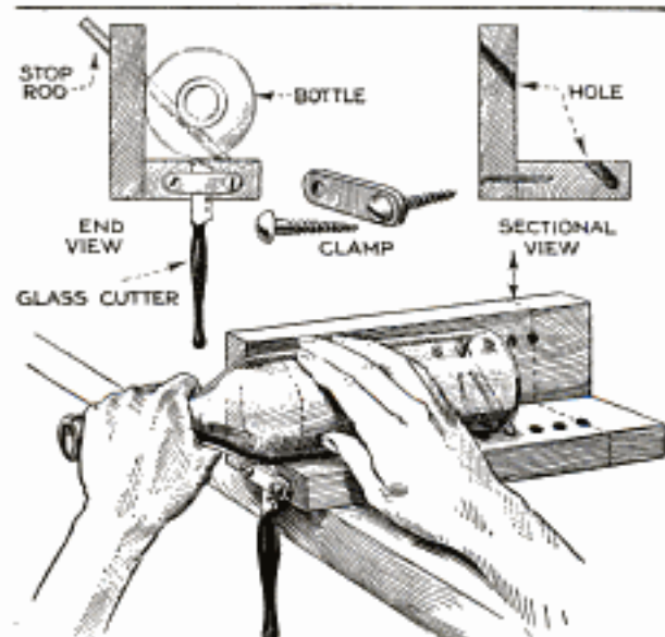
Simple Homemade Circular-Glass Cutter Cuts Bottles Quickly and Accurately
