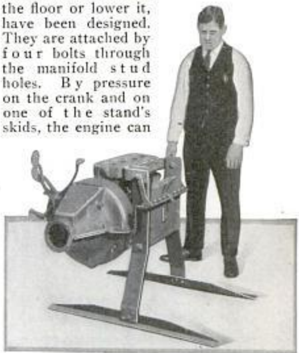
Engine Bolted to Stand and Raised from Floor by One Man; Note Broad Supports
