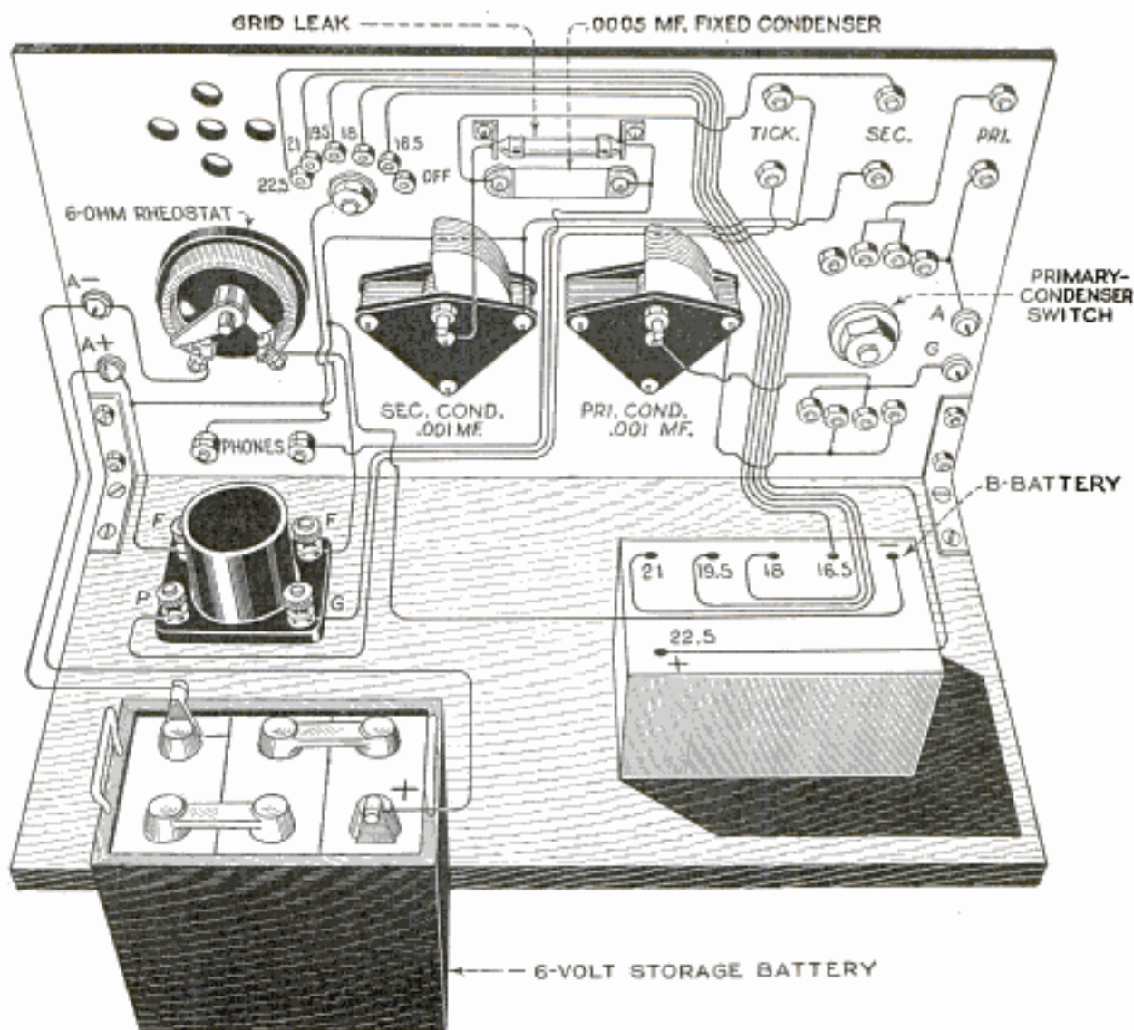
Back View of Panel and Baseboard, Showing All Connections and Position of the Instruments; Note Particularly the Wiring of the Primary-Condenser Switch
