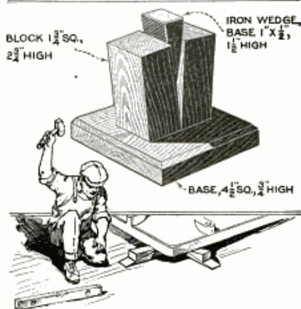
Wedge-Model Dimensions and Illustration Showing Use of Wedge in Leveling Machinery
