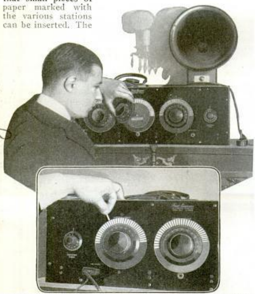
New York Radio Fan Invents Novel Calibrating Device Which Enables Stations to Be Logged on Tuning Dials
