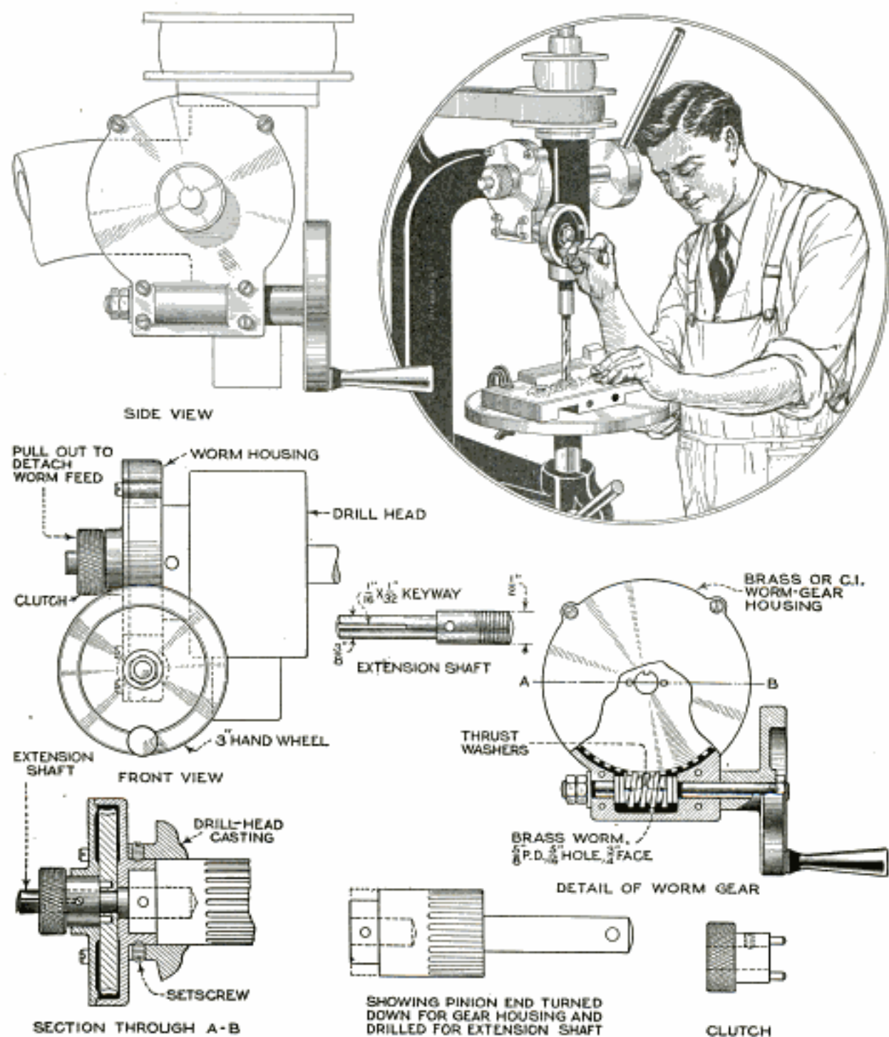
Fitting a Handwheel Feed to a Sensitive Bench Drill Press; an Attachment of This Kind Permits Heavy Work to Be Done over a Long Period without Fatigue
