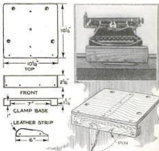
Wooden Holder for Light Portable Typewriter Is Clamped to Table Top
