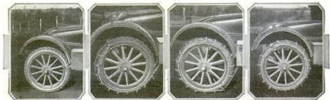
Views of Rear Wheel While Chain Is Being Put On as Car Proceeds. Clamped to Tire (left) It Unwinds from Box and Automatically Locks in Place
