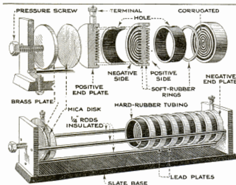
Construction and Details of Homemade B-Battery Which Does Away with External Connections between the Individual Cells
