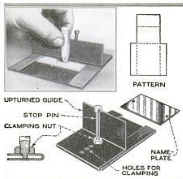
Sheet-Metal Fixture for Holding Brass Nameplates While Lettering Them
