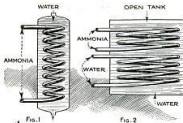
Fig. 1. Customary Method of Coil in Tank; Fig. 2. Better Method Which Prevents Freezing
