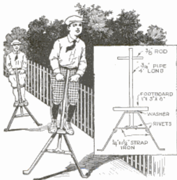
The "Walking Stick"—a Combination of Stilts and the "Pogo" Stick
