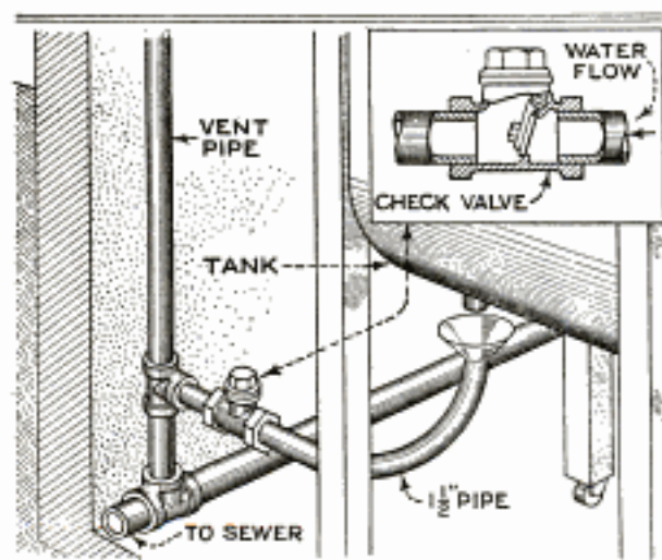
Connecting the Washing Machine to the Drain Pipe through a Check Valve
