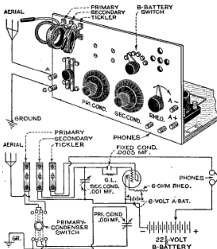
Above, Front View of Panel, Showing Mounting of Honeycomb Coils; Below, Wiring Diagram for Checking Purposes
