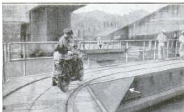
Steel Plate Used at Angle of Guard Gates at Panama Canal to Permit Vehicles to Turn Corner Safely
