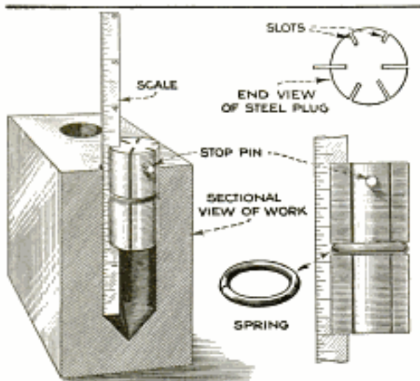
Accurate Plug Depth Gauge for Measuring Drilled Holes
