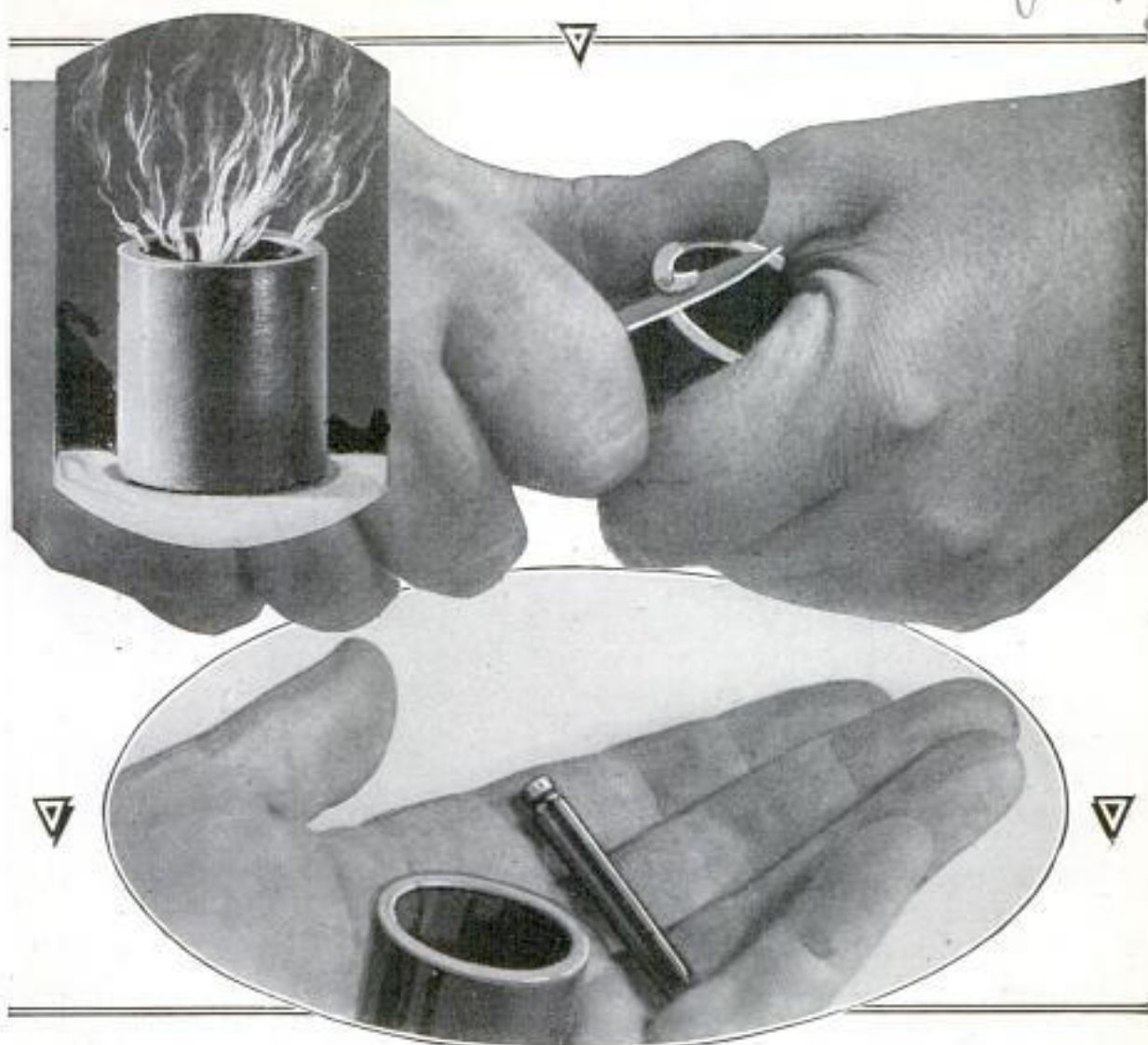
Oil-Absorbing Bushing Doing Service as a Wick; Chipping Piece of the Unannealed Metal with Ordinary Penknife, and Volume of Lubricant the Porous Tube Will Hold
