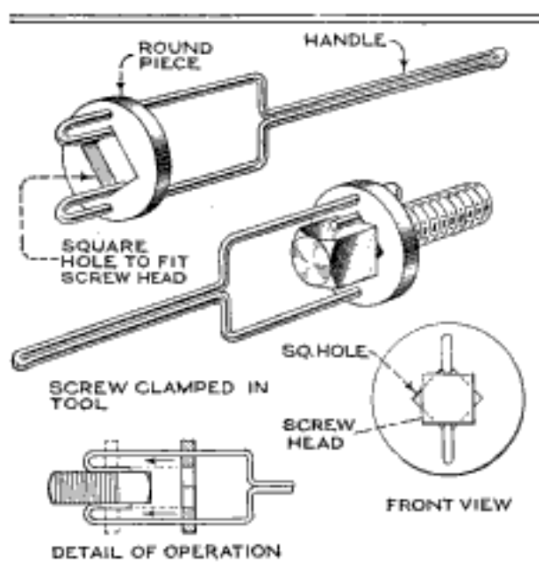
Nonslipping Holder for Square-Head Screws
