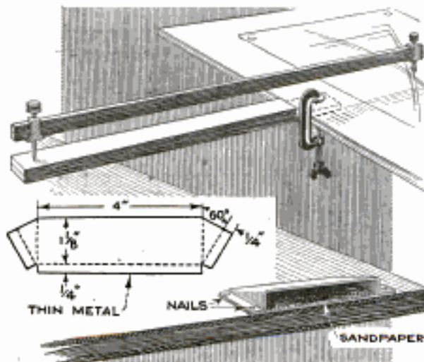
Above, Extension on Drawing Board Aids in Scribing Large Arcs; Below, Pencil-Dust Guard
