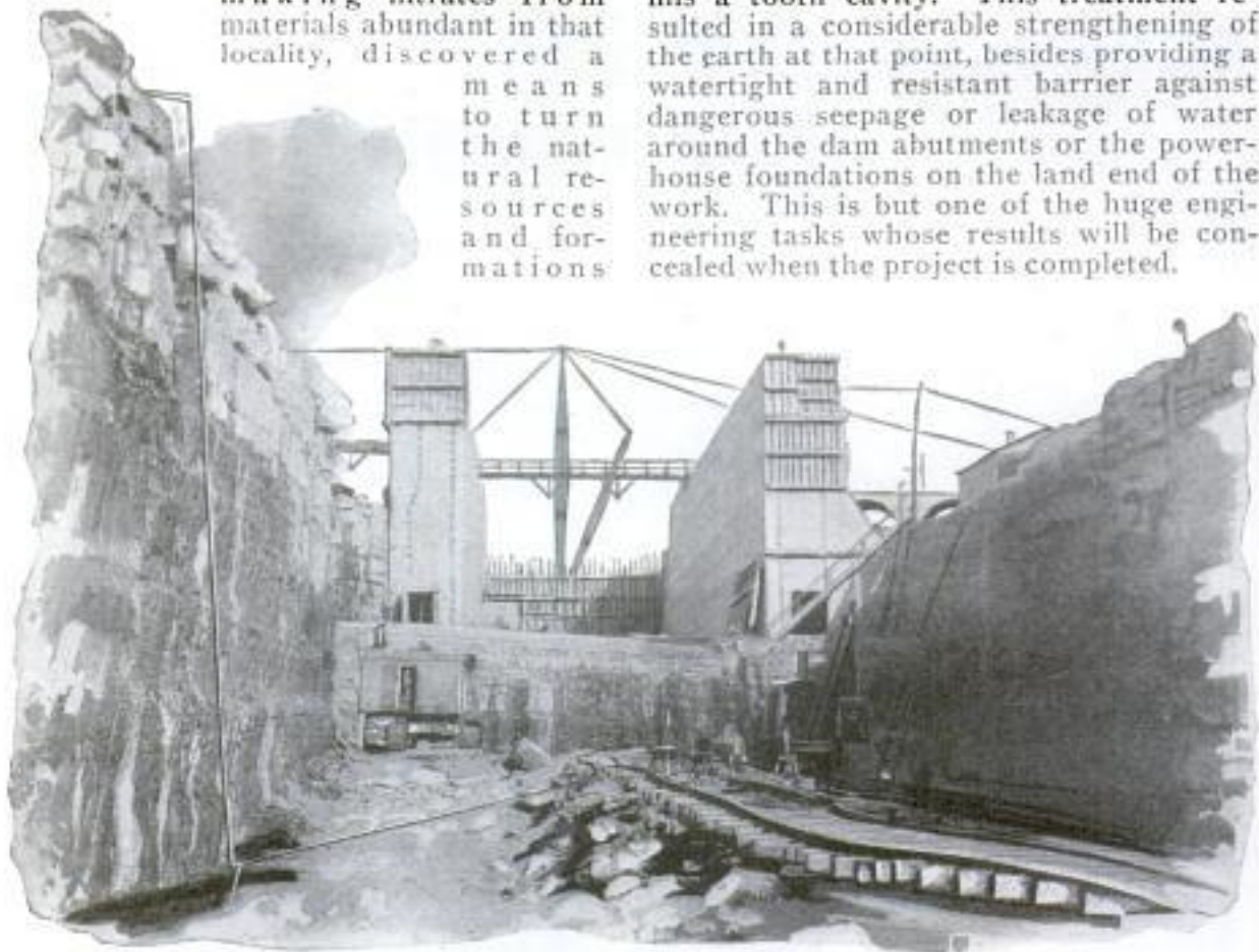
One of the Locks of Wilson Dam That Will Be the Means of Putting the Upper Reaches of the Tennessee River into a Great System of Water Traffic
