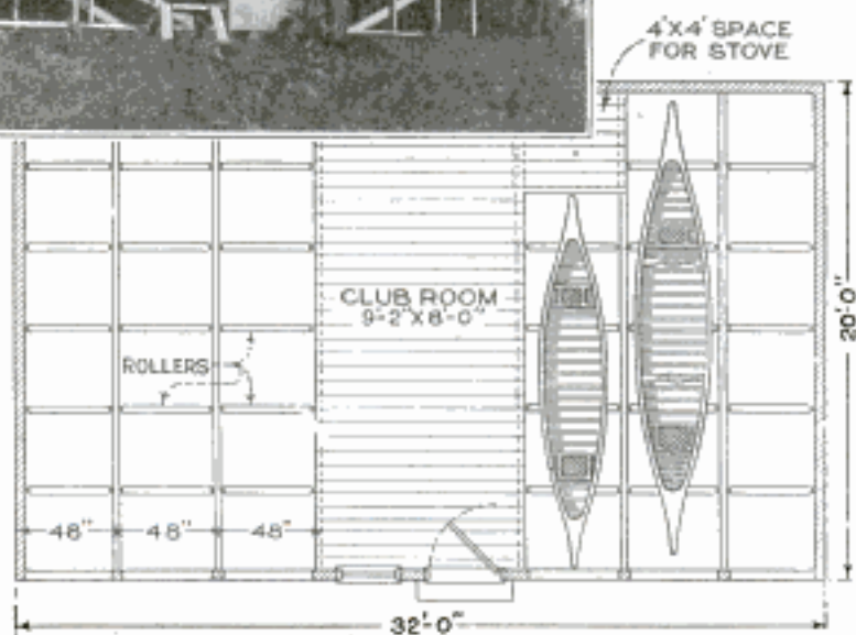
Floor Plan of Boathouse. Showing How the Canoes Are Stored; Insert, Building under Construction; Note the Compartment Framing
