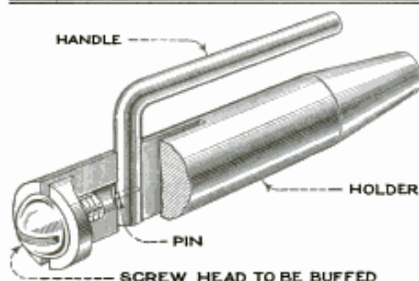
Holder for Buffing Short Screw Heads that Is Quick-Acting and Holds the Screws Securely
