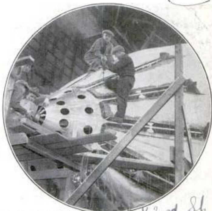
Copyright, Kadel & Herbert Putting Finishing Touches on "Shenandoah's" Tip and Mooring Coupling That Holds It to Mast
