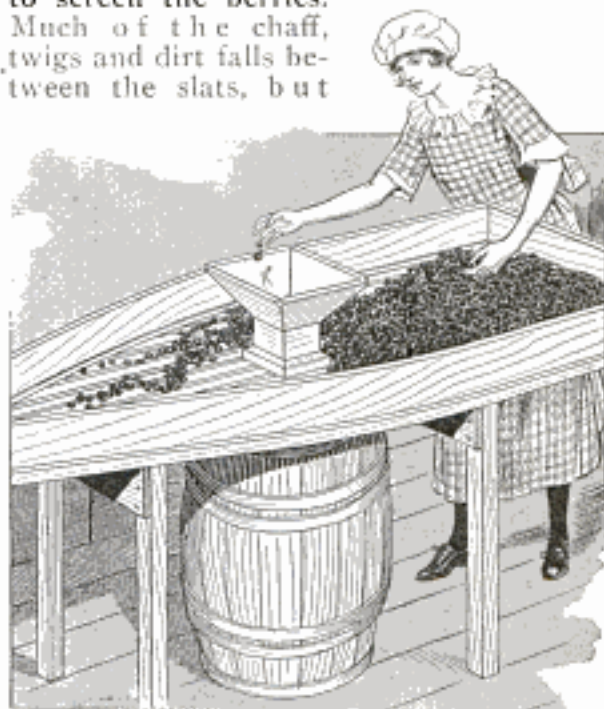
Hopper Built over Hole in Screen Bed Conveys Unsound Berries into Large Barrel
