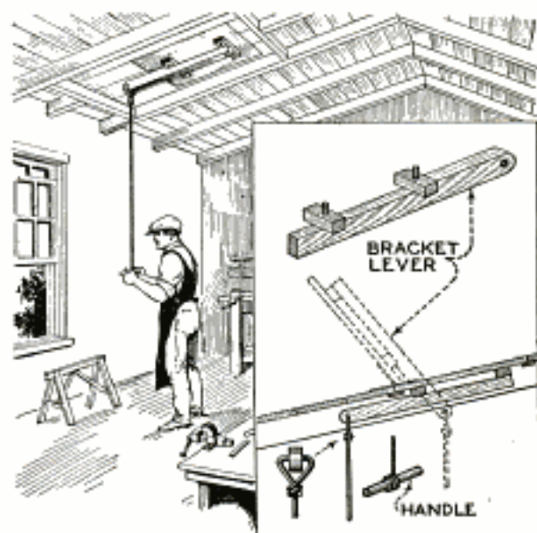
Bracket Lever and Iron Rod Used to Control Roof Trapdoor from Below
