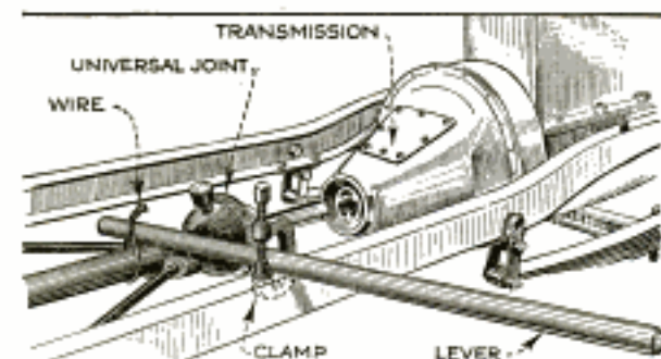
Lever Aids in Connecting Universal Joint to Engine When Rear End Is Replaced
