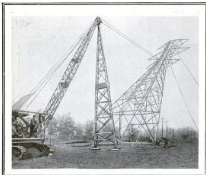
Tower-Raising Machine Lifting Steel Transmission-Line Support into Position after Assembly on Ground
