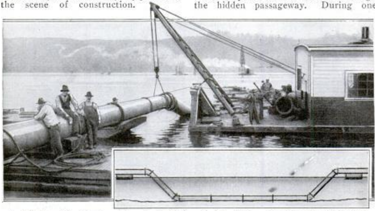
How Sand for a Dike Was Forced through a Pipe Laid on the Bed of a River, Out of the Way of Ships, from a Pit Almost a Mile from Scene of Construction
