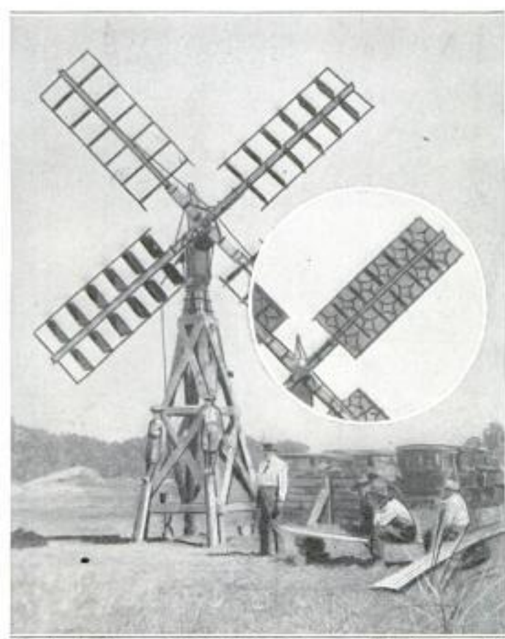
Handmade Kansas Windmill for Power and Irrigating with Swinging Wing Blades. Inset Shows Them Folded Flat
