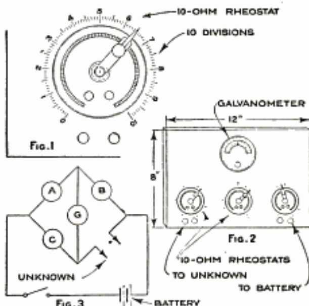
A Wheatstone Bridge for Finding the Unknown Resistance of the Windings of Electrical Instruments
