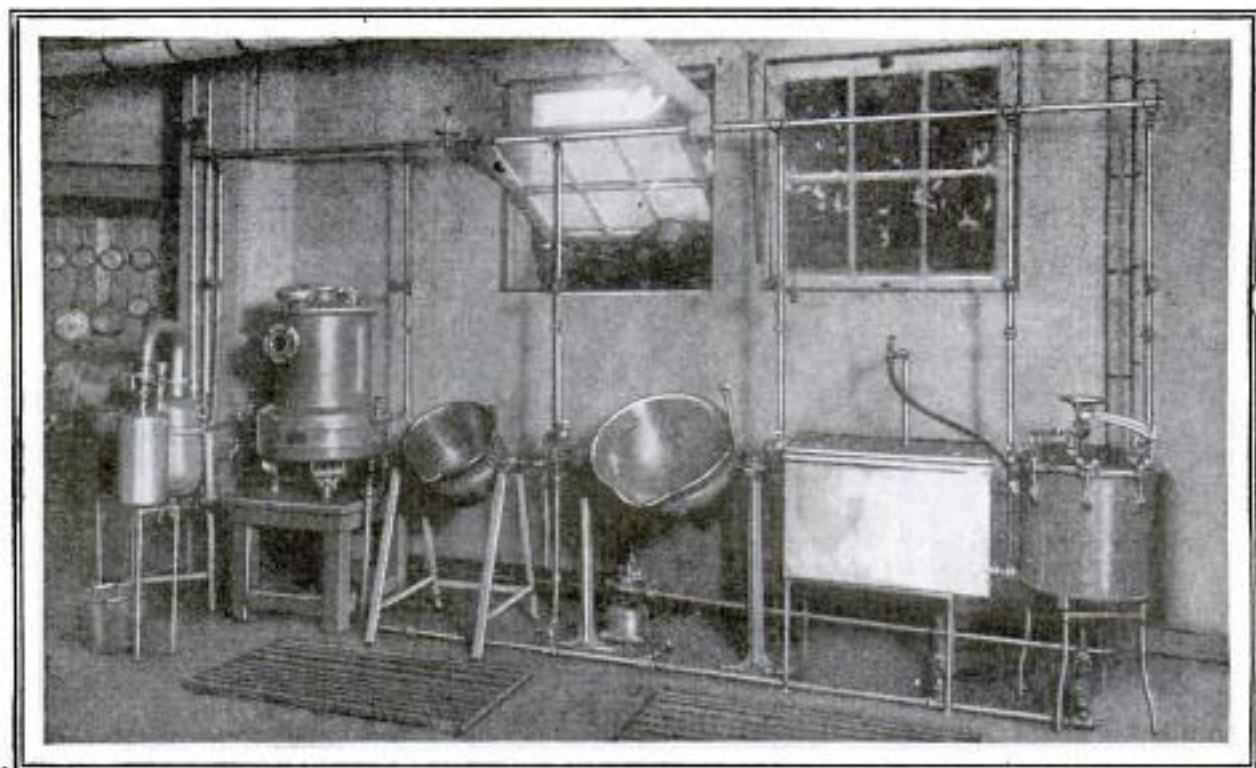
Apparatus Devised by the Faculty and Students of the College of Agriculture of the University of California in Their Discovery of Method of Preserving Fresh-Fruit Juices
