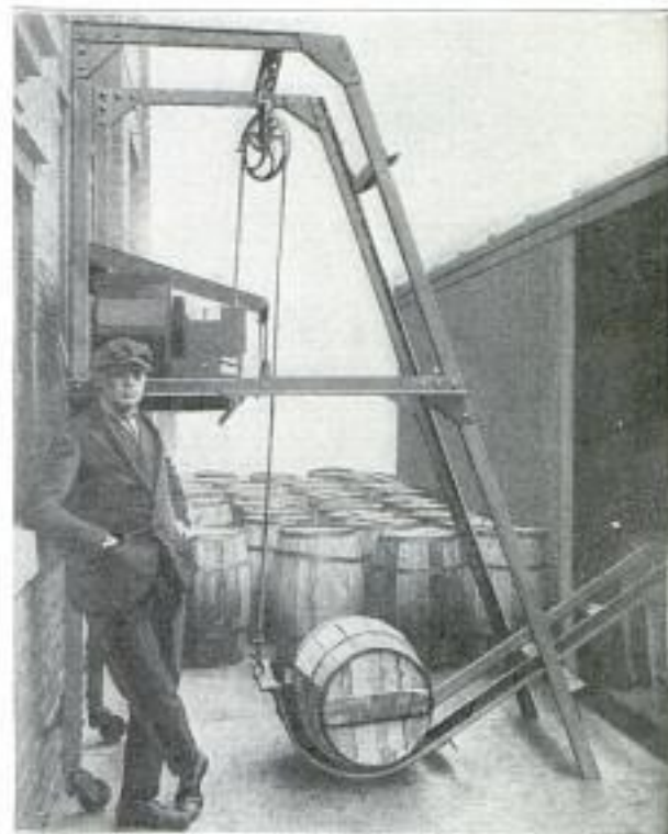
Electrically Operated Barrel Loader for More Easily Filling Upper Tiers of Freight Cars
