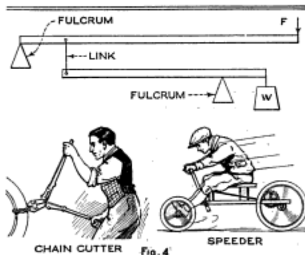
Fig. 4 Compound Lever of First and Second Orders, with Examples of Everyday Compound Levers
