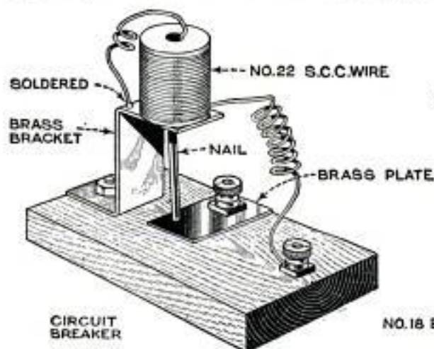
An Electric Insect Killer, Which Uses House-Lighting Current, and Has Been Found Very Effective. A Small Circuit Breaker Protects the Fuses in Case Too Much Current Flows
