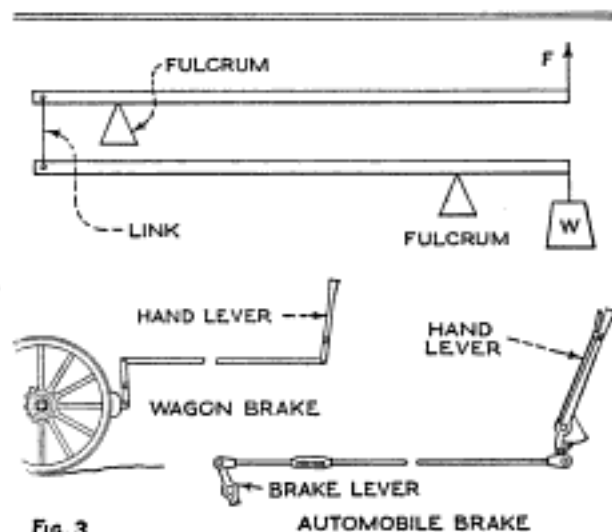
Fig. 3 Simplified Drawing of Compound Lever of First Order, with Examples of Its Use
