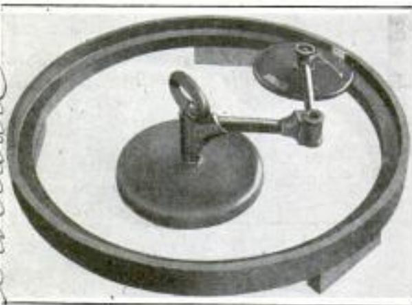
Dial Wheel on Arm that Measures the Inside Circumference of Tires and Rims
