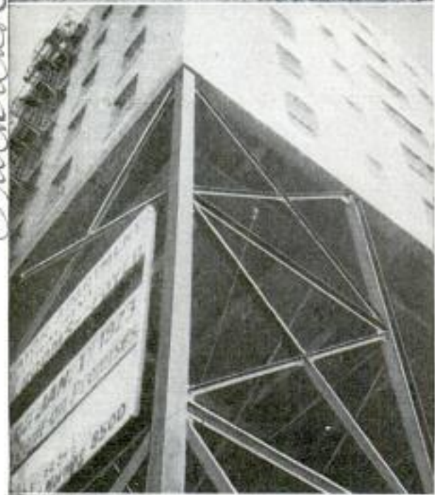
Apartment Building on Its Foundation of Braced and Riveted Strong Steel "Stilts"
