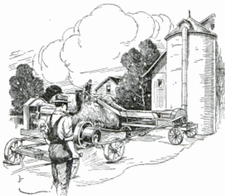
Driving the Silage Cutter and Elevator with the Portable Auto-Engine Power Plant
