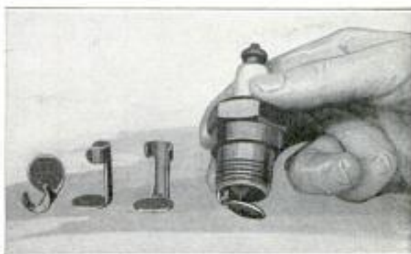
Spark Plug and Shield Designed to Prevent the Collection of Oil and Carbon
