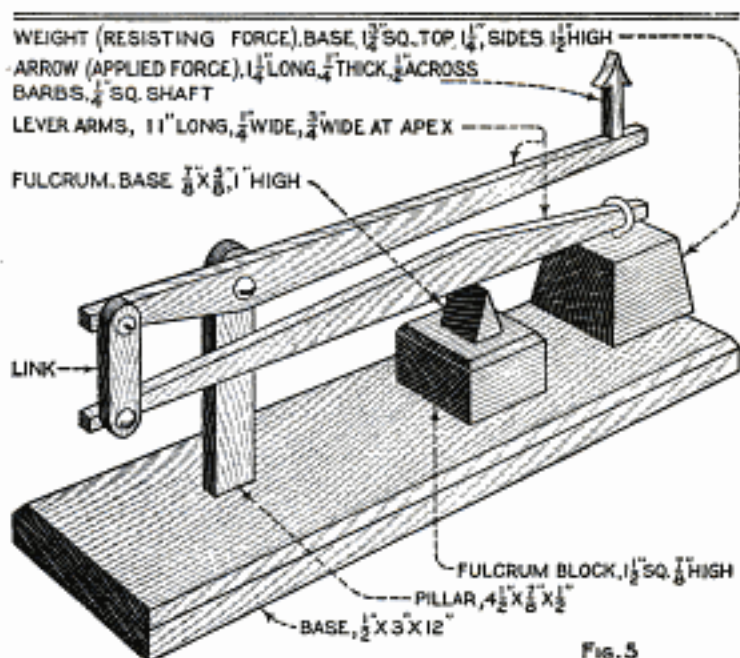
Dimensioned Drawing for Constructing Reproduction of Model of First-Order Compound Lever
