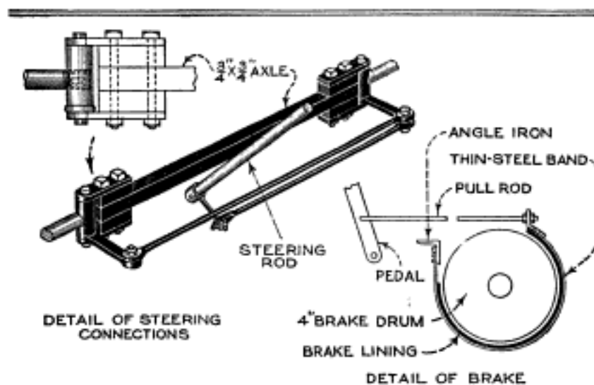
Details of Front Axle, and Steering Mechanism; Also Method of Mounting Brake and Its Connections to Brake Pedal
