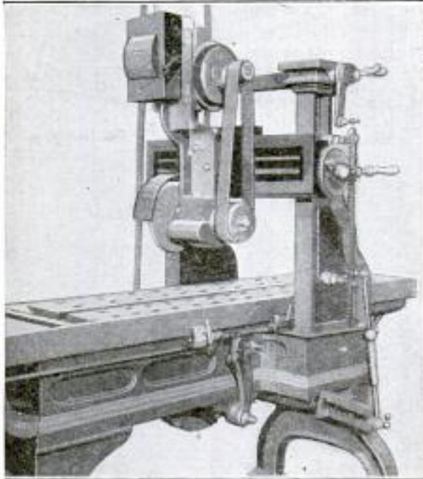
Attachment that Converts the Planer into an Efficient Surface Grinder
