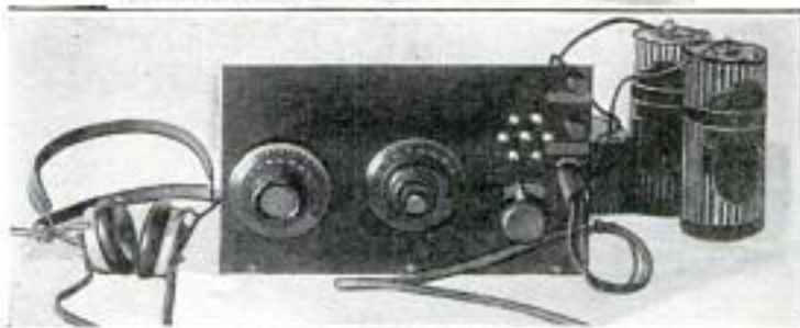
Photos of Front and Rear of Simple Receiver Incorporating the Ultra-Audion Circuit
