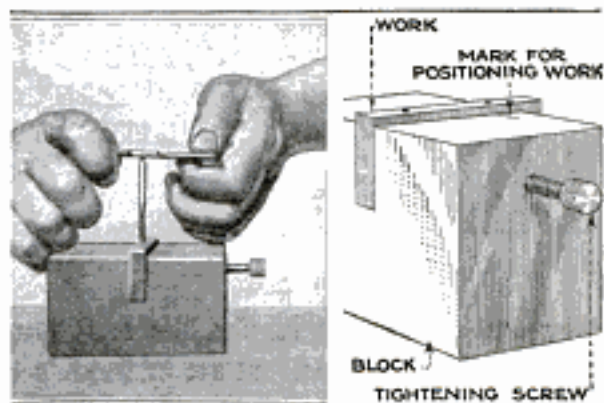
Left, Using Loose Block to Tap Small Work; Right, Details of Block
