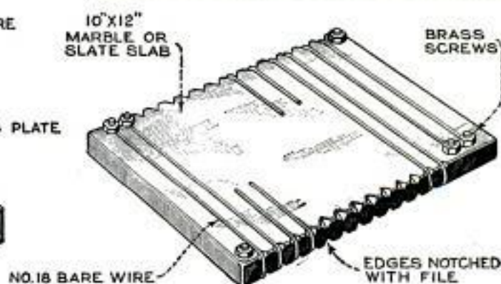
An Electric Insect Killer, Which Uses House-Lighting Current, and Has Been Found Very Effective. A Small Circuit Breaker Protects the Fuses in Case Too Much Current Flows
