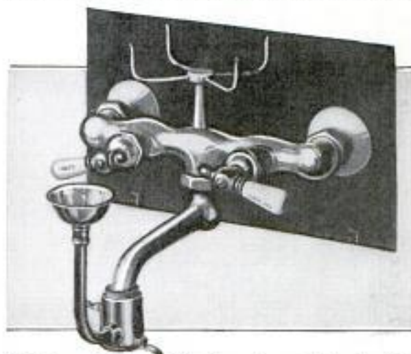
"Drinking Bubbler" Fitted on Faucet Nozzle: The Trap Release Is Seen at Bottom
