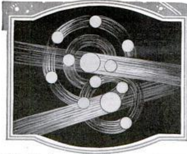
Minute Solar System Formed by Electrons Constantly Whirling About a Center Like the Planets
