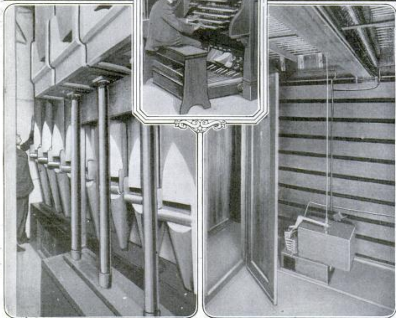
Electrical Control (Top); Organ Keyboard (Center); Mouth of Several of the Pipes (Left), and Wind Chest that May Be Entered During Concert (Right)
