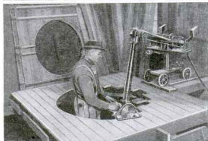
Above, Cutting Off Stock, with Machine on Special Runway; Below, Cutting Circular Holes in Concrete Forms
