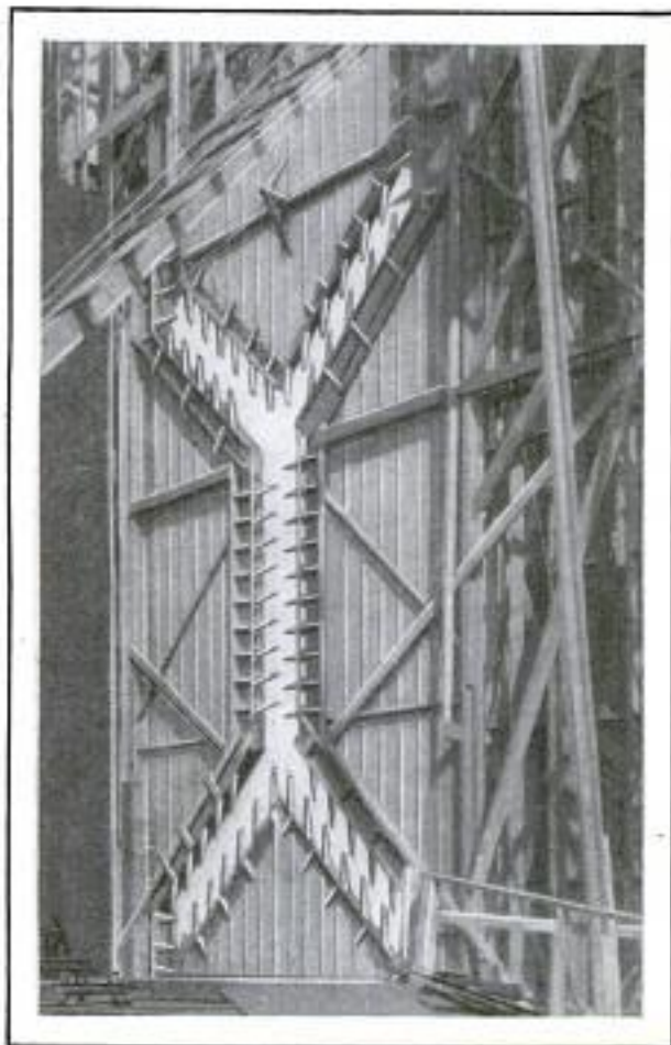
Back of Gate Weighing Seven Tons Yet Operated by One Man, So Accurately Was It Poised
