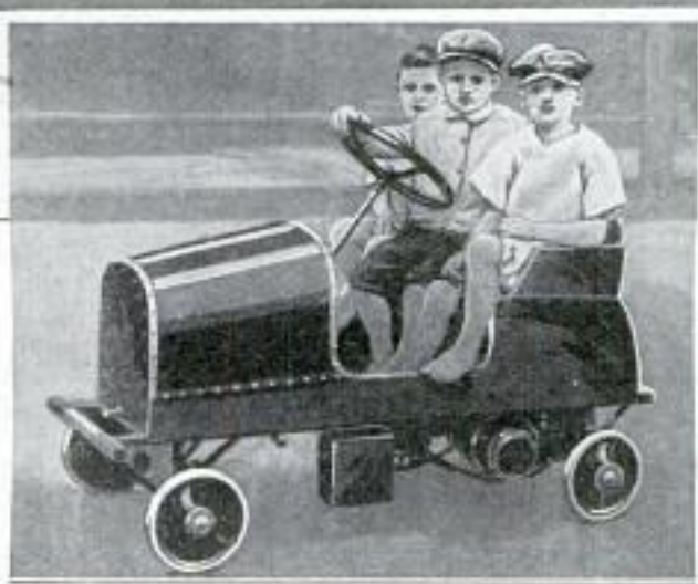
Above, Front View of Car; Center, View of Underside, Showing Transmission, Brake, Etc.; Below, Side of Car, Showing Location of Switch and Motor
