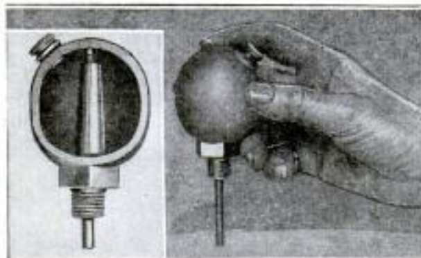
Interior and Exterior of Pulley Oiler, Illustrating Brass Feed Pipe and Spring Control
