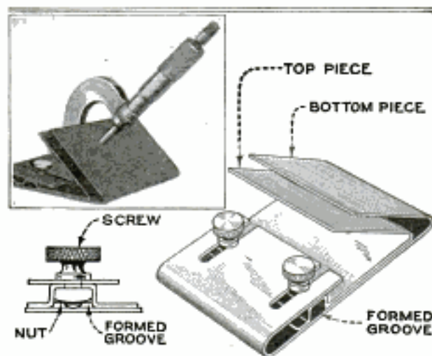
Simple Holder for Micrometer Used to Gauge Oily Work
