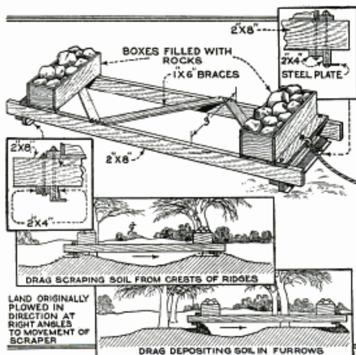
A Homemade Drag that Has Been Found Very Efficient for Leveling Orchard Lands
