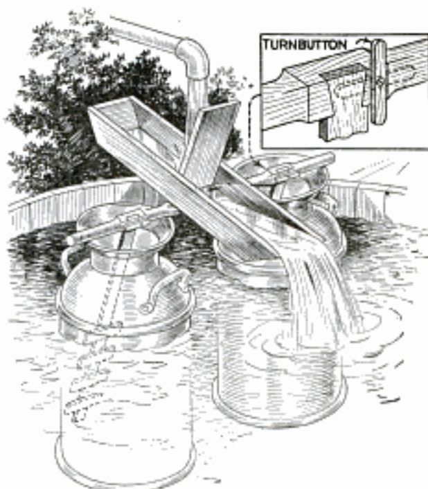
A Simple Rocking-Box for Stirring Fresh Milk Automatically by Water Flow
