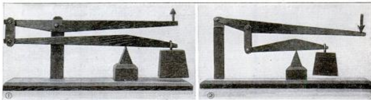
Photo No. 1, Completed Model of Compound Lever of the First Order; Photo No. 2, Model of Compound Lever Combining First and Second Orders
