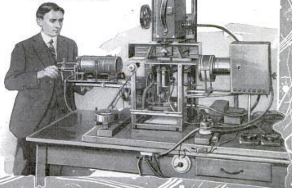
Producing Charged Particles in Cylinder to Reveal Paths
