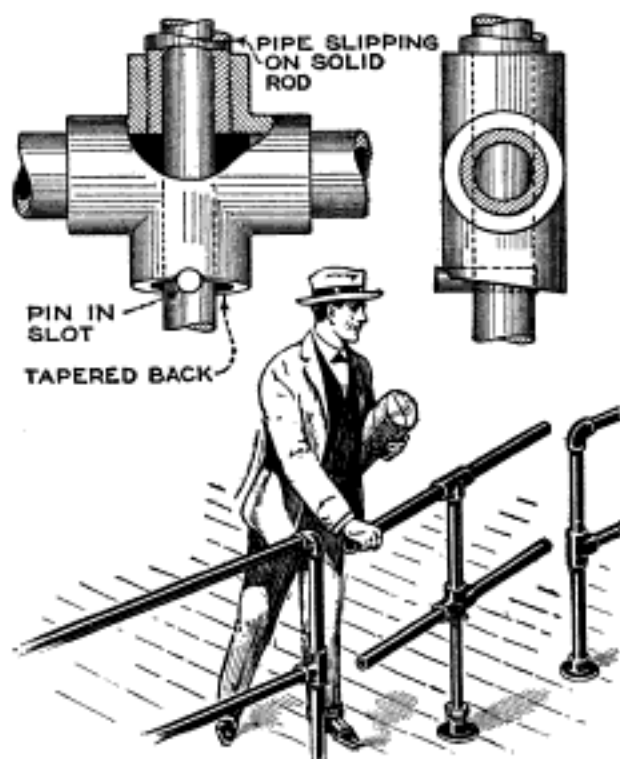
A Self-Closing Gate that Can Be Made from Lengths of Pipe and Fittings
