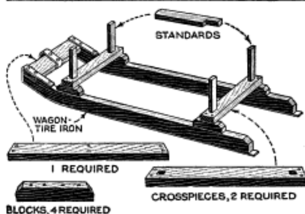
Easily Built and Sturdy Skid for Hauling Heavy Loads over Mud and Snow
