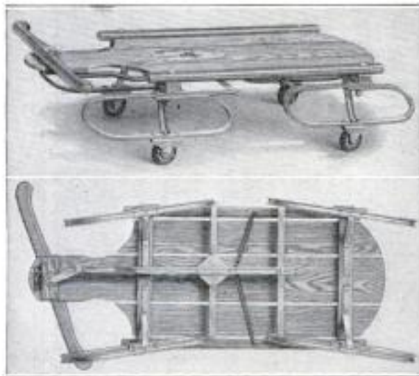
Side and Bottom Views of All-Year Coaster, Showing Rollers Attached and Steering Gear
