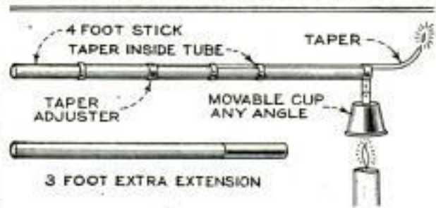
Candle Extinguisher with Taper Concealed Inside Tube to Prevent Dripping on Altar Linen
