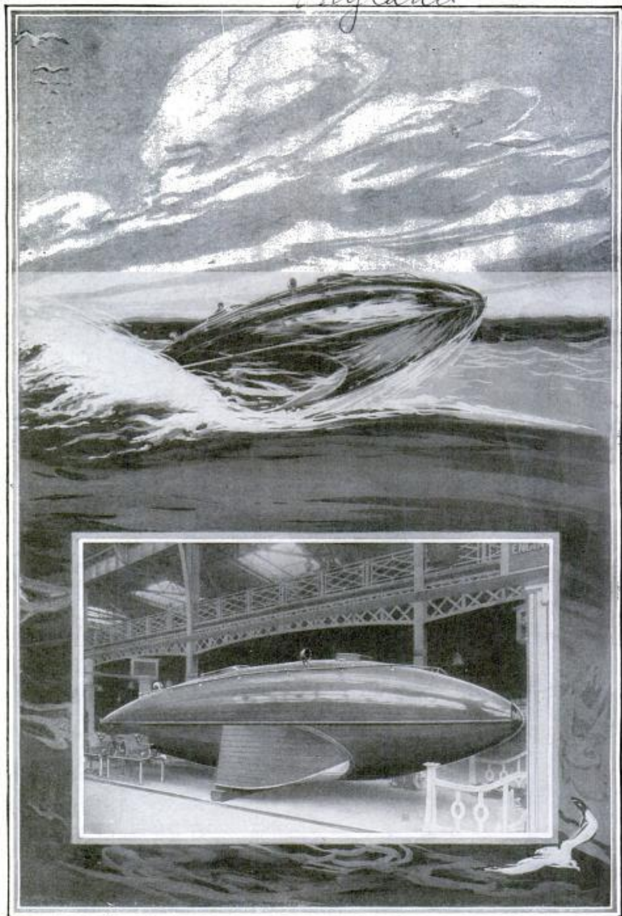
Mile-a-Minute Speed Boat that Is Built Like an Airship, the Hull Being Driven over the Waves by an Eighteen-Cylinder Gas Engine Developing over Four Hundred Horsepower
