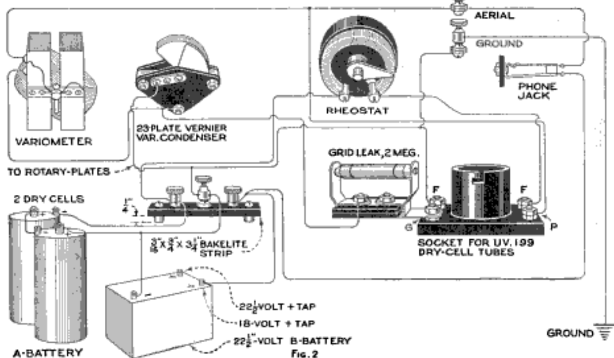
Fig. 1, Layout of Panel; Fig. 2, Simplified Wiring Diagram of Ultra-Audion Receiver Suitable for 3-Volt Dry-Cell Tubes. Variometer and Variable Vernier Condenser Are Used for Tuning
