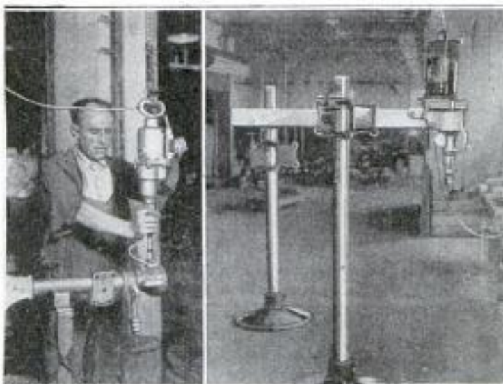
Left, Portable Tool in Operation; Right, Tool Mounted on Stand that Converts It into a Stationary Machine
