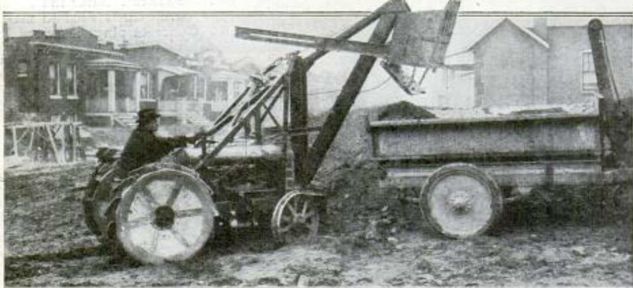
Combination Shovel, Crane and Hoist Attached to Tractor; It Is Operated by One Man and, by Covering the Wheels with Rubber, May Be Used on Factory Floors
