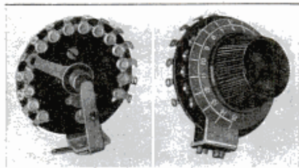
Left, Back of Inductance Switch, Showing Contact Points; Right, Graduated Dial and Knob
