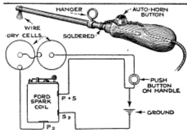
Simple Electric Gas-Stove Lighter Using an Induction Coil Can Be Made by Any Boy
