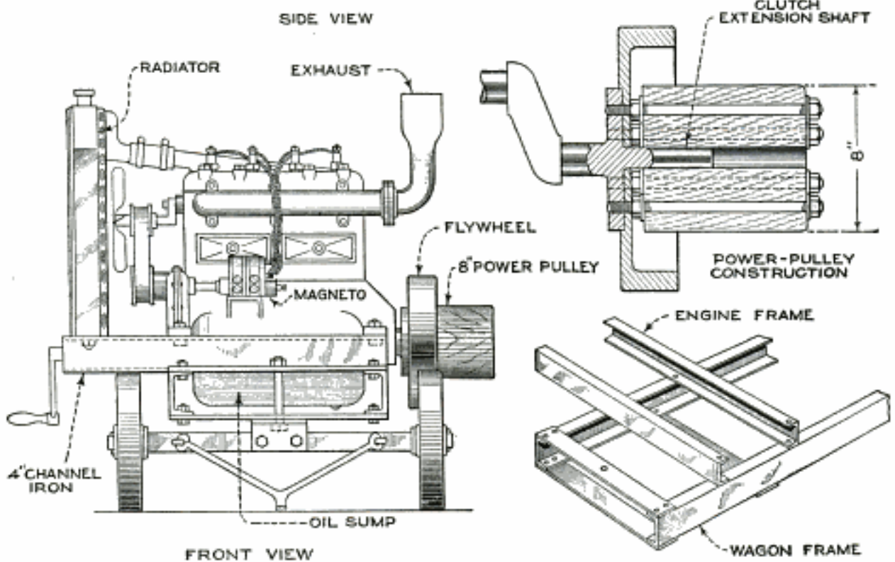
General Arrangement of Portable Gasoline-Engine Plant for the Farm, Showing Details of Frame, Sub-Frame, Drive Pulley, and Method of Mounting Engine
