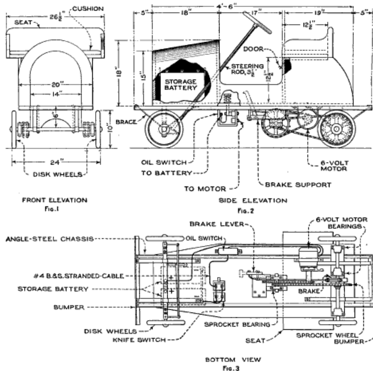
Detailed Drawings, Showing Dimensions and Location of Every Part of the Mechanism of the Small Electric Automobile; Also Wiring of Batteries, Switch, and Motor
