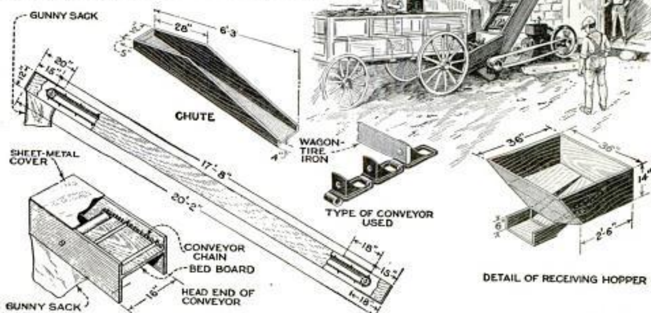
A Homemade Grain Conveyor that Can Be Made from Materials Available on Every Farm, and Costs Approximately $18: It Is Run by a Two or Three-Horsepower Gasoline Engine
