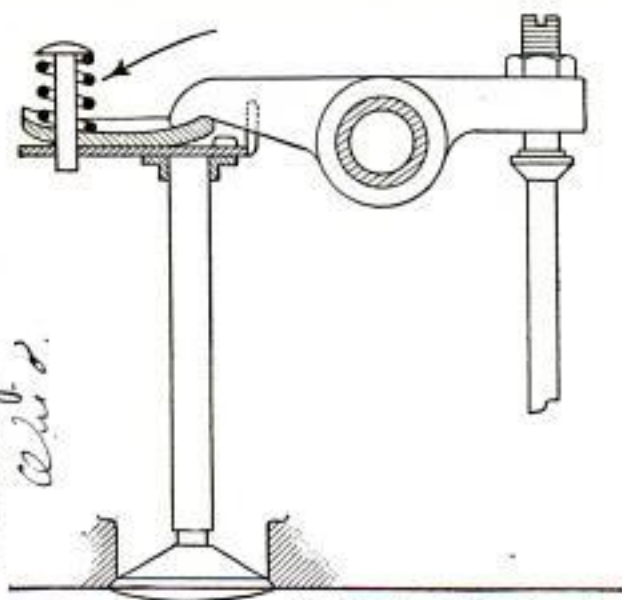
Rocking-Chair Silencer, Held in Place by Spring, that Silences Noisy Overhead Valves
