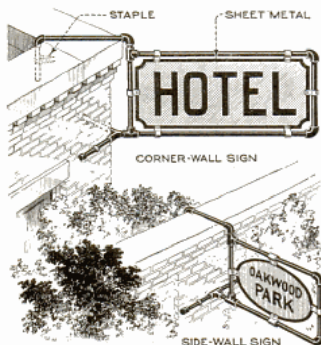
Substantial Signs Made from Pipe and Fittings and Heavy Sheet Metal
