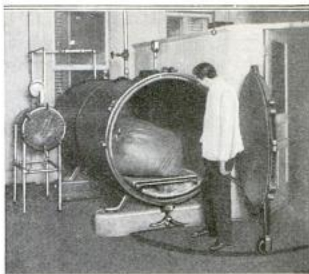
Vacuum Cylinder for Fumigating Cereal, Plant, and Cotton Shipments Received from Europe
