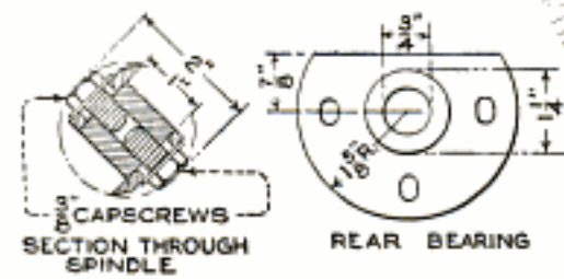
Full Details of Construction of the Homemade Bench Jointer. No Castings are Necessary, and All Material is Standard, and Easily Obtainable
