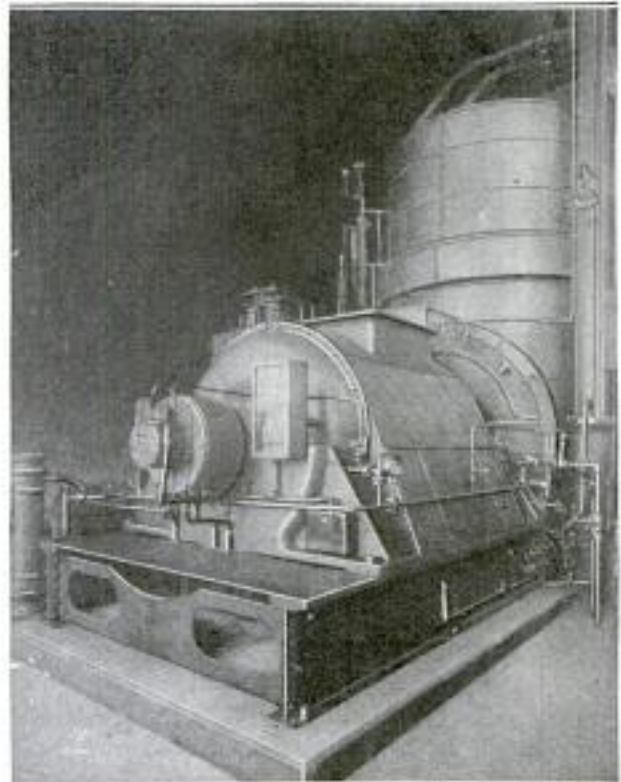
Mercury-Vapor Engine that Showed Great Increase in Efficiency in Recent Tests
