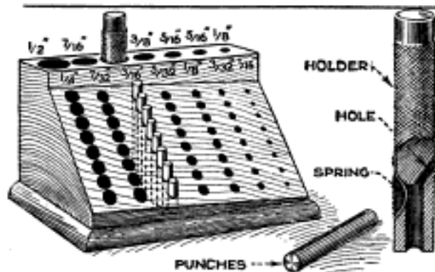
Drift-Pin Punches That Replace the Common Type, Which Are Easily Broken
