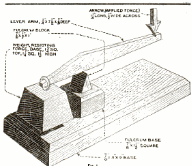
Showing How the Model of the First-Order Lever Is Constructed, with Full Dimensions
