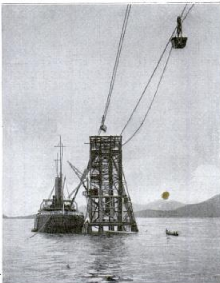
Sturdy Structure that Helps to Defy Rocky Coasts
