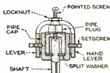
THRUST-BEARING DETAIL
