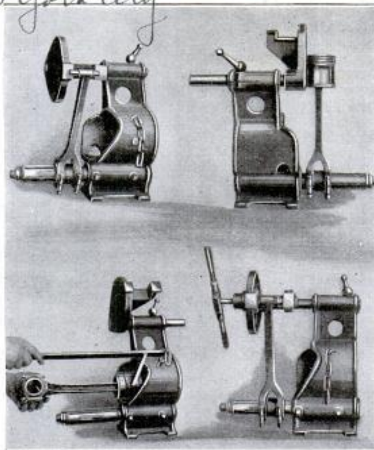
Upper Left, Testing Alignment of Wristpin; Upper Right, Testing Piston; Lower Left, Forcing Out Wristpin; Lower Right, Reaming Wristpin Bushing
