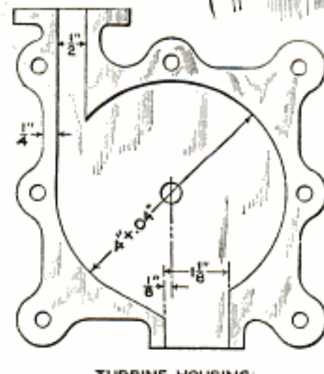
Details of Construction of Simple Turbine for Operation on Steam, Water, or Compressed Air, Which Can Be Built in the Small Workshop and Used for a Variety of Purposes
