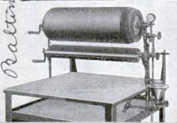
Sponger that Forces Steam through Fabrics to Shrink Them for Tailoring into Suits
