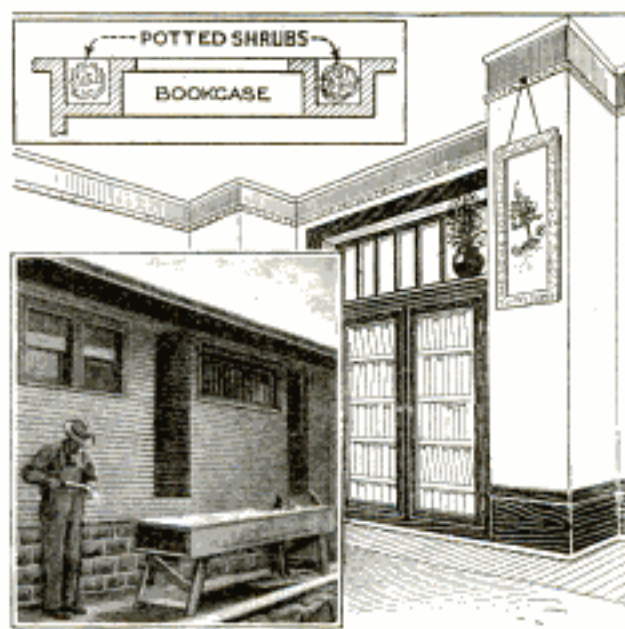
Jogging a Wall Makes the Bookcase Flush with Interior Surface. Left, View of Outside of Wall
