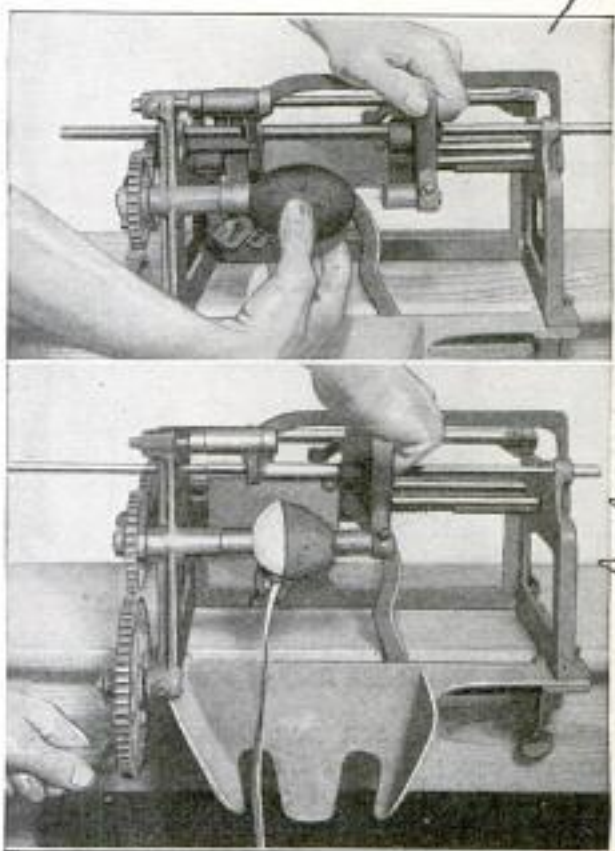
Automatic Peeler with Self-Sharpening Knife that Pares Vegetables Evenly as Spindles Revolve
