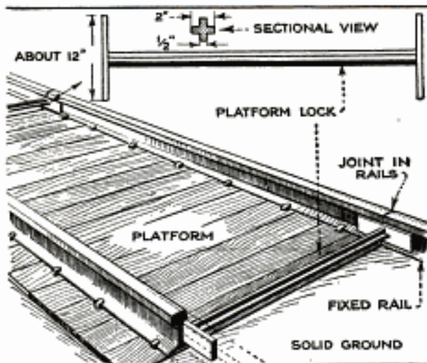
Protecting Platform Scale from Loads Beyond Its Rated Capacity
