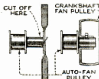
CONE PULLEYS
