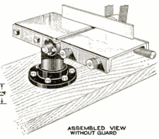
Full Details of Construction of the Homemade Bench Jointer. No Castings are Necessary, and All Material is Standard, and Easily Obtainable
