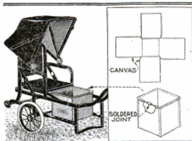
A Canvas Basket on a Sulky Has Been Found Useful for Keeping the Blanket in Place
