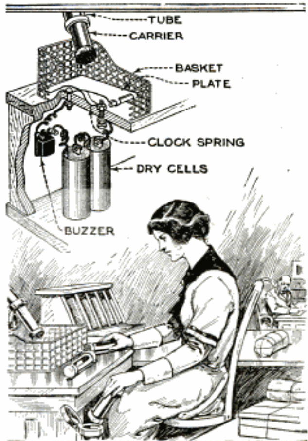
A Buzzer Connection to the Receiving Basket of a Pneumatic Tube Announces Arrival of Carrier
