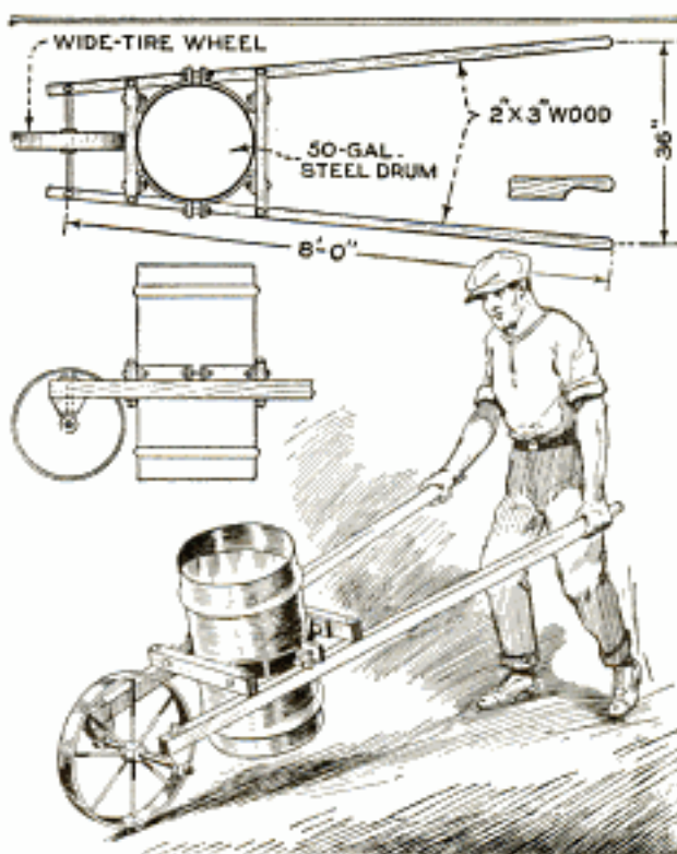
Handy Homemade Wheelbarrow for Carrying Concrete, Water, Sand, and Similar Materials
