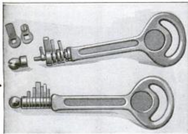
Adjustable Key Teeth that Can Be Changed to Fit Any Position of Lock's Levers
