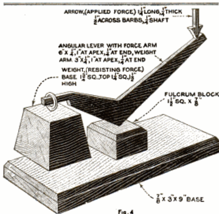
Model of Angular Lever of the First Order, with Dimensions of All Details
