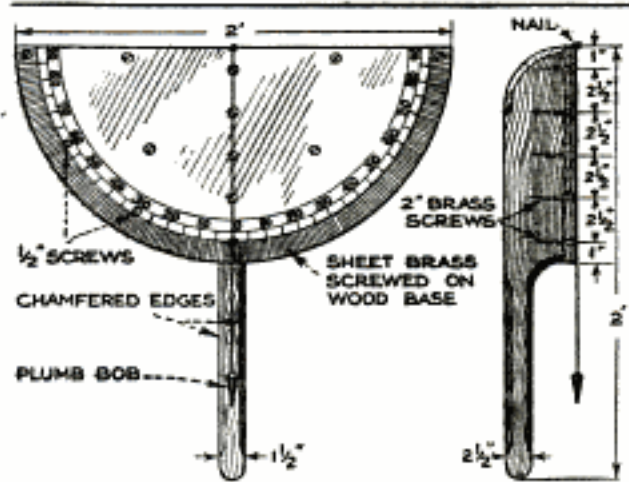
A Simple Homemade Hand Level Which Will Prove of Assistance to the Amateur Surveyor
