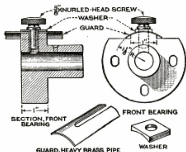
Detail of Adjustable Brass Guard, Attached to Left-Hand Bearing
