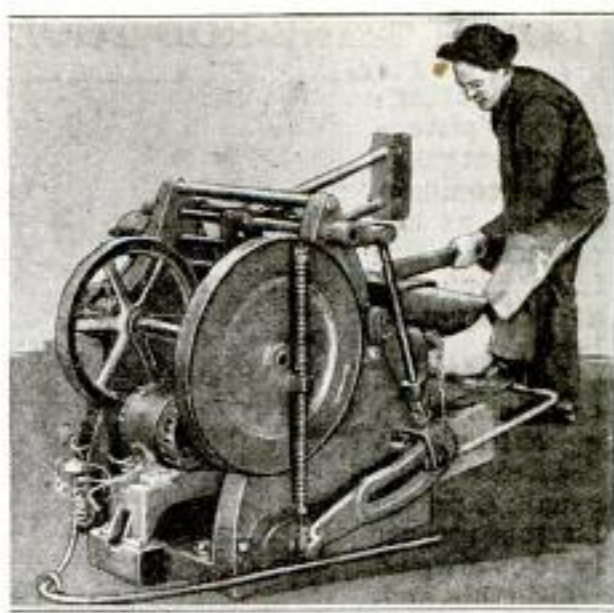
Forging Light Work with a New Power Hammer, Which Is under the Complete Control of the Smith
