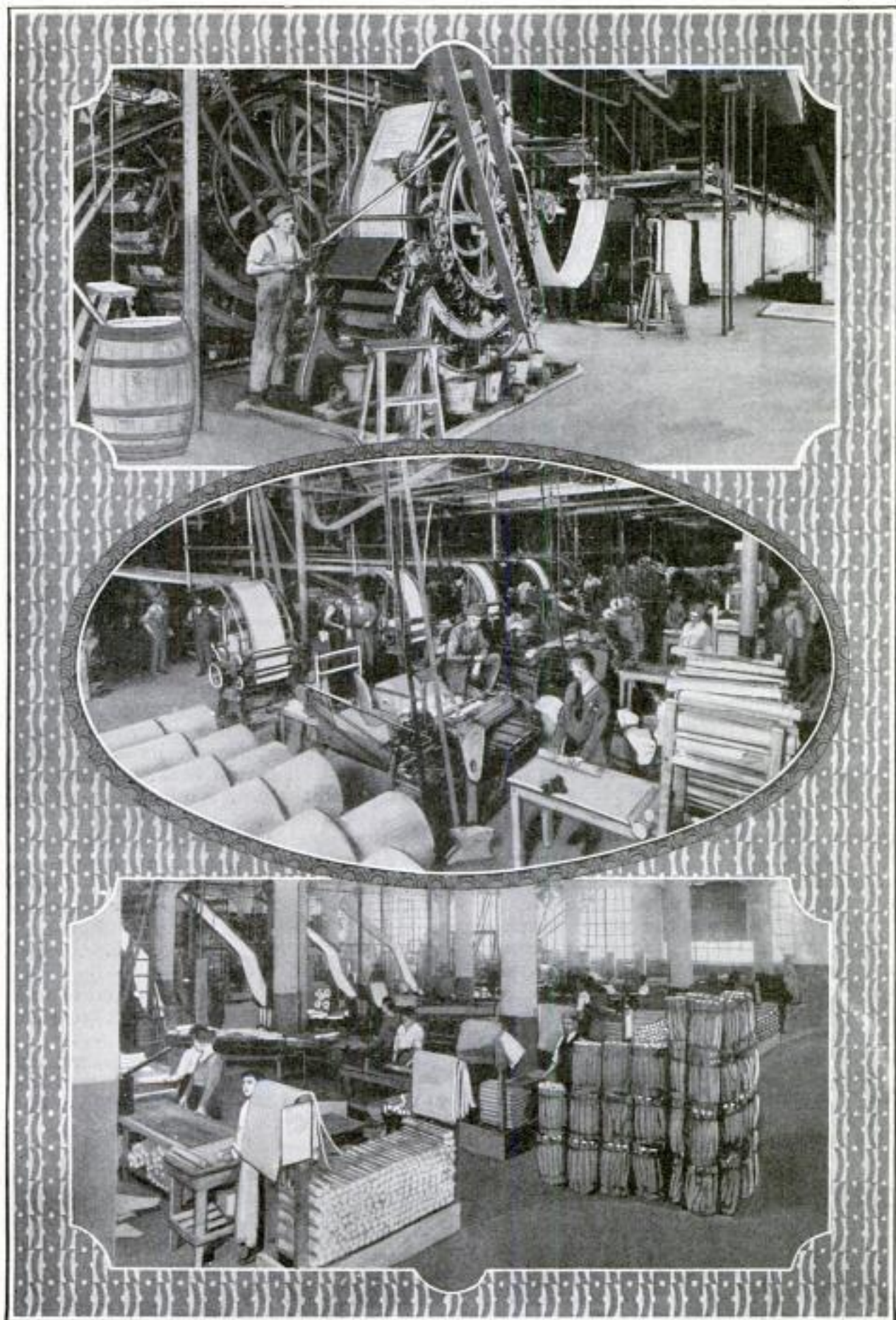
After Passing through the Great Printing Machines where Every Roll Adds Its Separate Color, the Wallpaper Is Dried, Sorted and Wrapped in Preparation for Shipment
