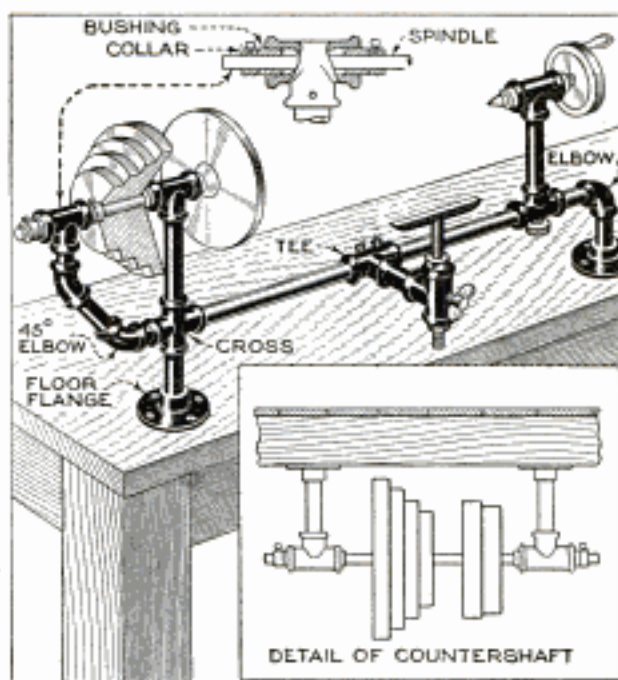
Simple Lathe for the Amateur, Made Almost Entirely of Pipe and Fittings
