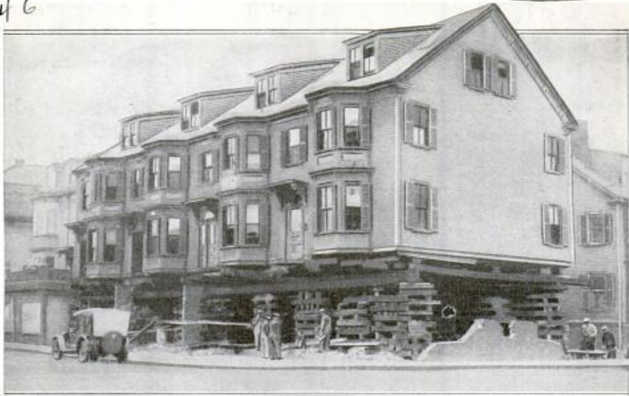
Block of Houses Raised Fourteen Feet; Although Only an Inch of Space Separated the Structure from an Adjacent Building, the Movement Was Made without Affecting It
