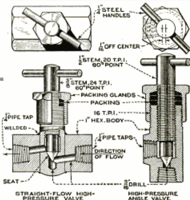
Stronger Valves, Made for High Pressure, from Similar Materials
