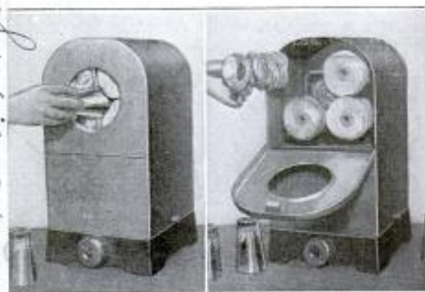
Cabinet with Rotating Cloth Buffers Run by Electricity to Shine and Dry Glasses
