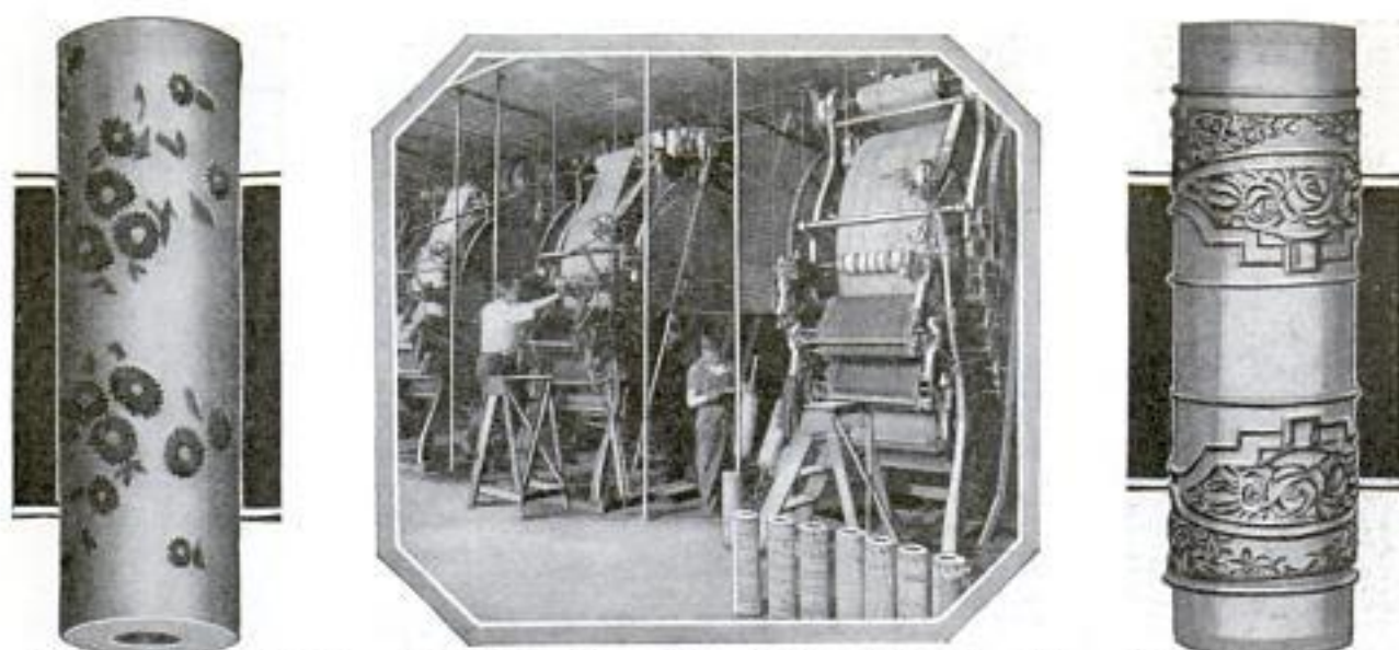
Printing Rolls with Patterns Outlined by Strips of Brass Packed with Felt and Three of the Great Presses which Resemble Those Used in Textile Mills
