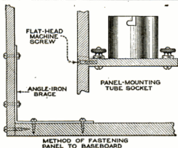
Method of Fastening Socket Bases to Panel and of Fastening Panel to Baseboard
