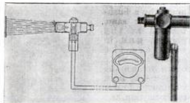
Left, Sectional View of Pyrometer, Showing Lens System and Wiring; Right, Complete Pyrometer
