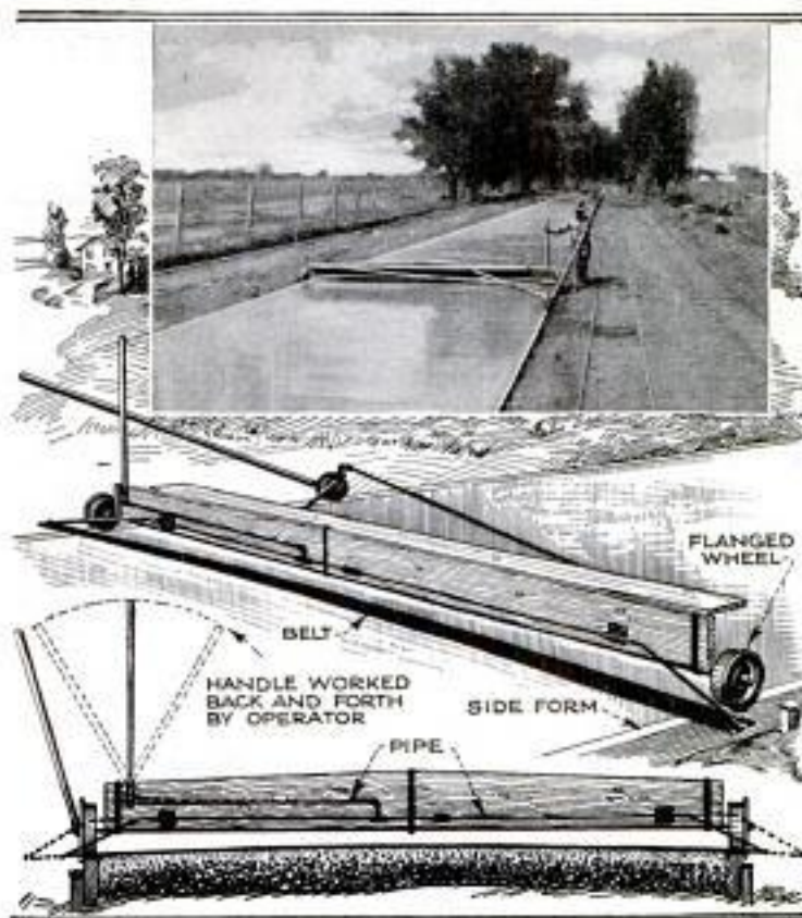
Homemade "Belter" for Concrete Roads, Moved and Operated by One Man
