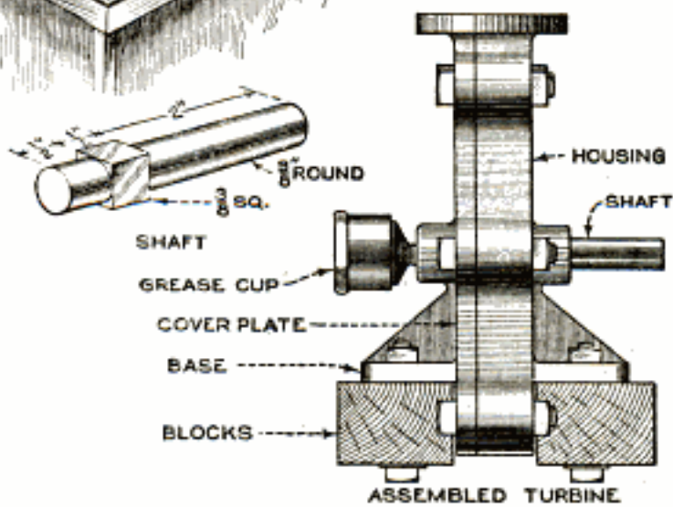
Details of Construction of Simple Turbine for Operation on Steam, Water, or Compressed Air, Which Can Be Built in the Small Workshop and Used for a Variety of Purposes
