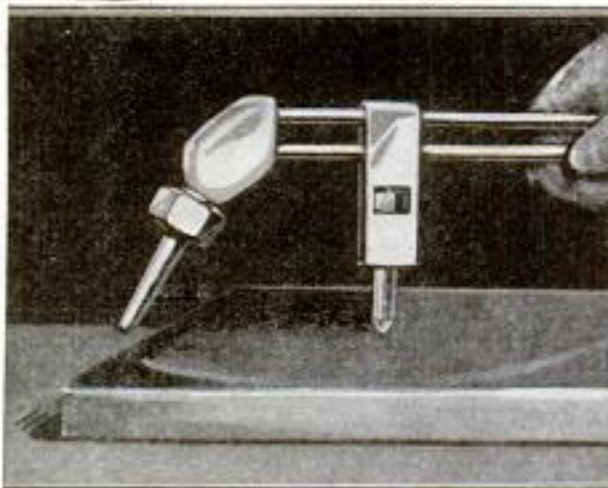
Simple Attachment for a Cutting Torch, Which Is of Great Assistance in Making Circular Cuts
