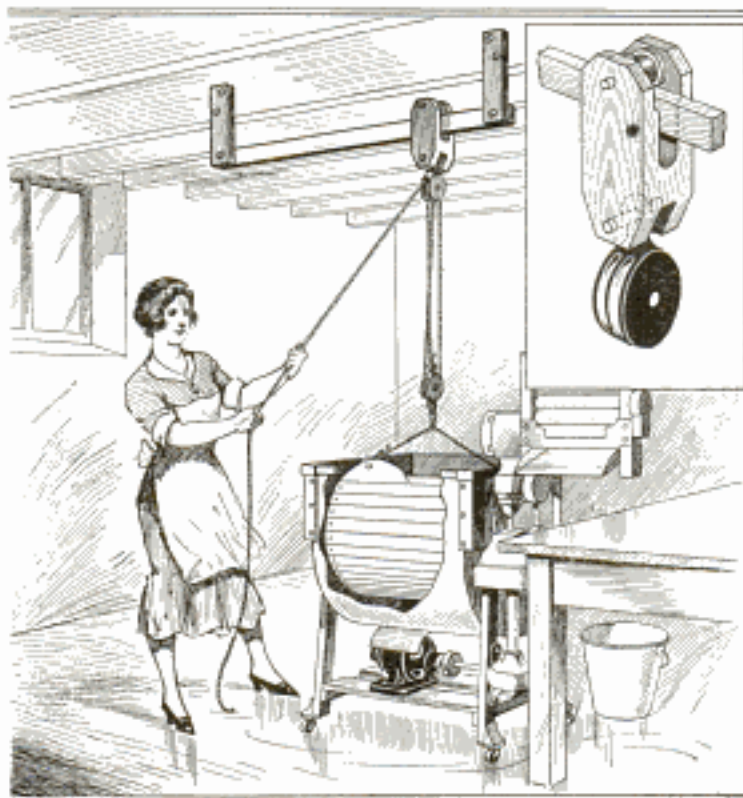
A Convenient Block-and-Tackle Arrangement Used for Hoisting the Cylinder Out of the Washing Machine
