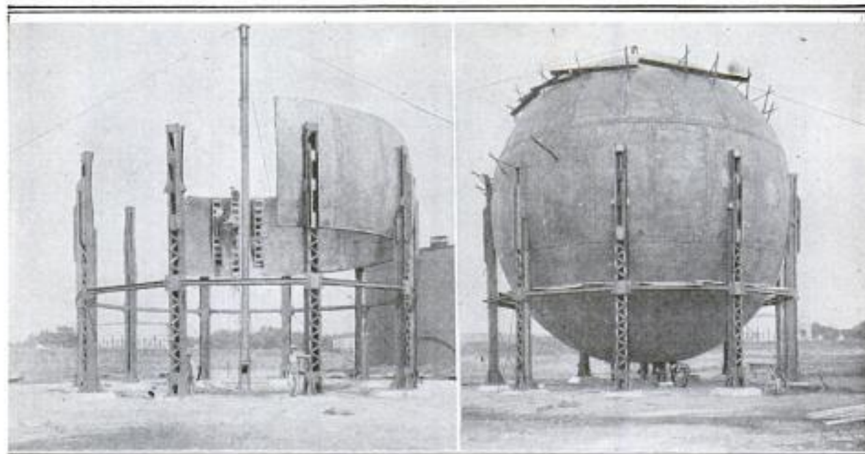
Gasoline Tank Built in the Form of a Globe so that Pressure May Be Equalized, Thus Preventing Distortion and the Consequent Loss through Evaporation
