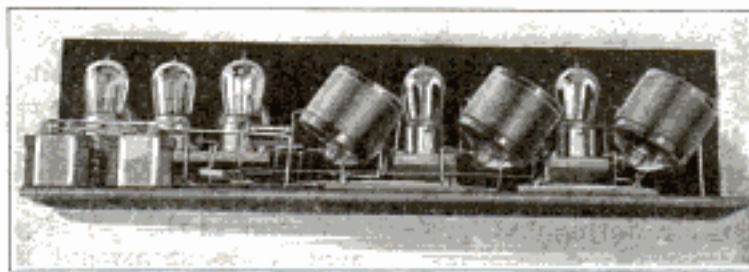
Above, Buzzer Circuit for Adjusting Neutrodyne Receiver. Upper Detail Shows Construction of Neutrodon; Below, Another View of Rear of Set
