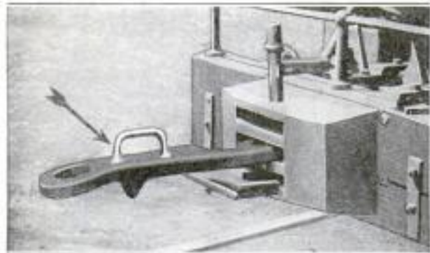
Handle on Coupler Arm of Railroad Freight Car to Aid Switchmen in Avoiding Injury
