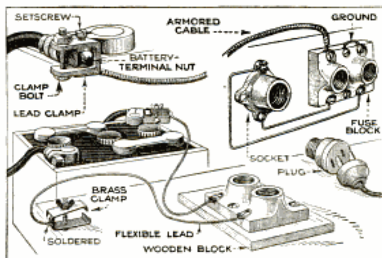
An Arrangement for Drawing Current from the Storage Battery of an Automobile for Lighting the Camp or Summer Cottage
