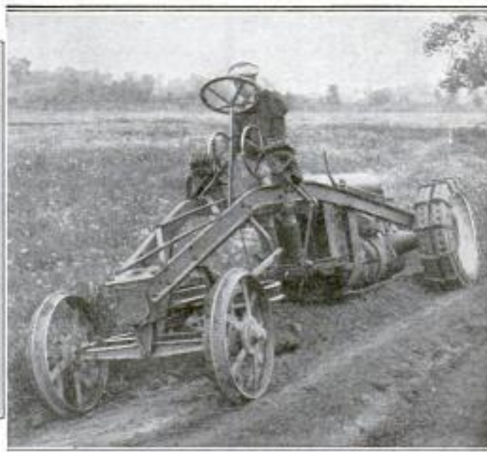
Road Grader Operated by Kerosene Engine that Requires Services of Only One Man
