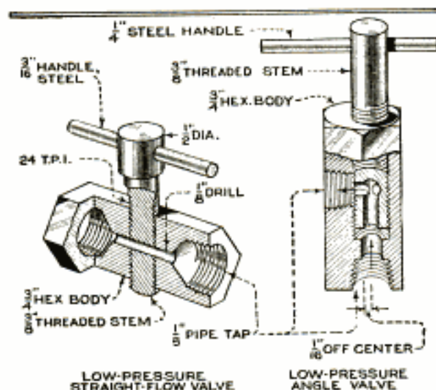
Low-Pressure Straight-Flow and Angle Valves Made from Stock Material
