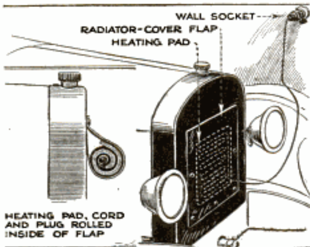
An Electric Heating Pad Used for Keeping the Radiator Warm during Cold Weather
