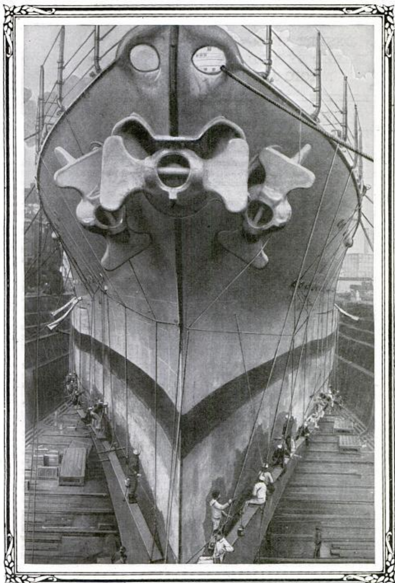
Fighting Face and Mammoth Anchors of the Electrically Propelled Warship "Colorado"; a Swarm of Workers Are Applying the First Coats of Paint to the Ironclad Hull
