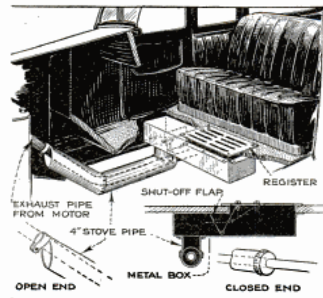
A Homemade Heater Adds Considerable Comfort to Auto Driving During the Cold Winter Months
