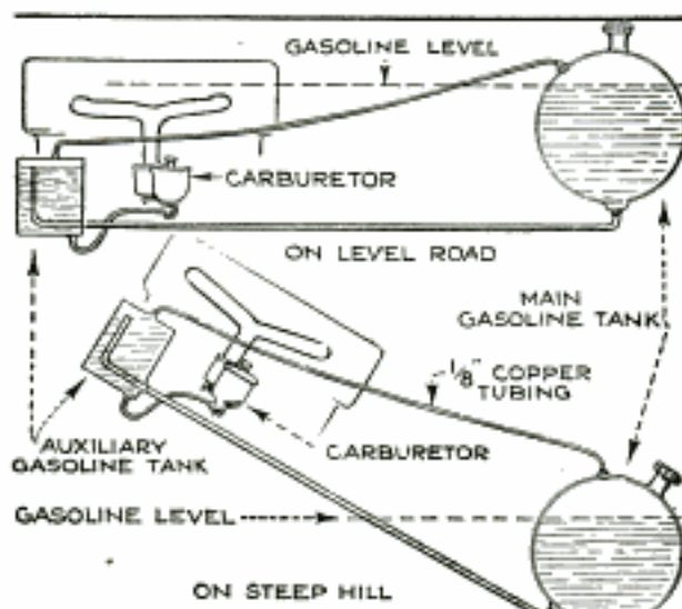
Auxiliary Gasoline Tank Supplies Carburetor with Gasoline When Climbing Steep Grades
