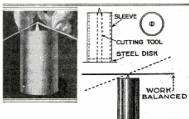
Tool for Dividing Brass Strips Equally: Insert, Bending Balanced Strip Before Cutting
