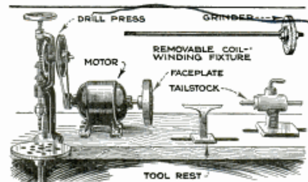
Doubling the Usefulness of the Bench Motor by Driving from Both Ends of the Shaft
