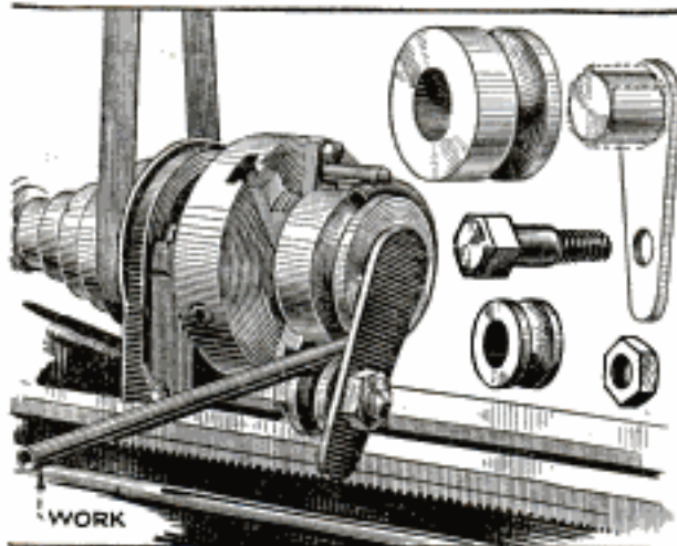
A Homemade Pipe Bender that Is Attached on the Lathe, Has Been Found Very Efficient
