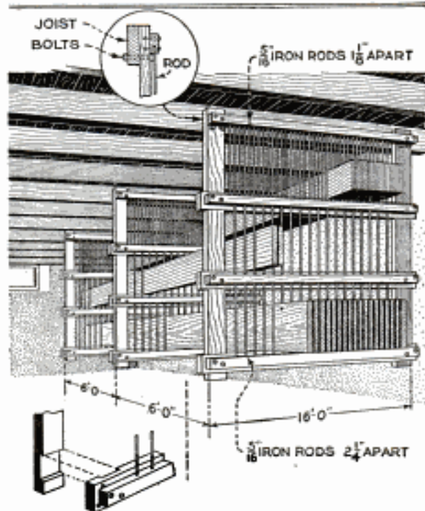
A Novel and Substantial Lumber-Drying Rack for the Woodworking Shop
