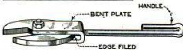
Insert, Loosening Torch-Tip Nut; Below, Details of Wrench Construction
