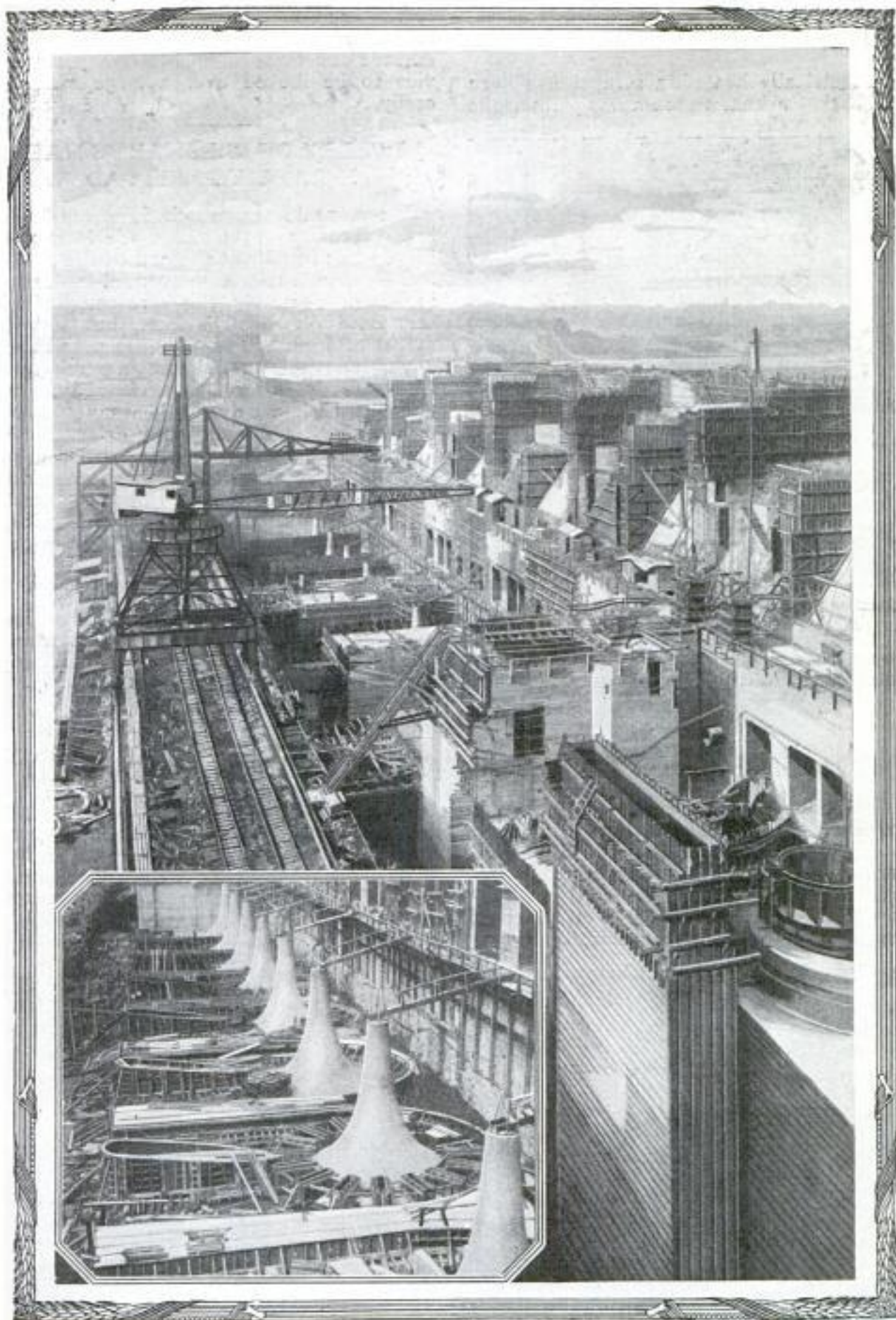
Harnessing Nearly 1,000,000 Horsepower with Monster Wilson Dam, a Part of the Muscle Shoals Project: Concrete Foundations for the Turbines Are Shown in the Lower Picture
