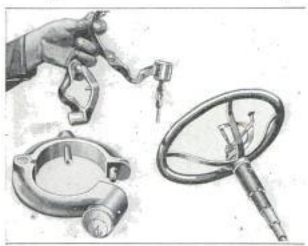
Auto Lock and Screws that Hold It Like a Handcuff to Steering Column
