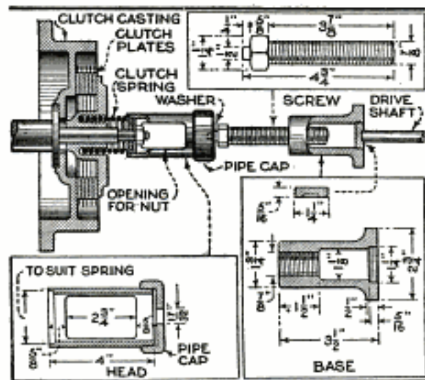
A Jack for Compressing an Automobile Multiple-Disk Clutch Spring that Has Been Found to Save Time
