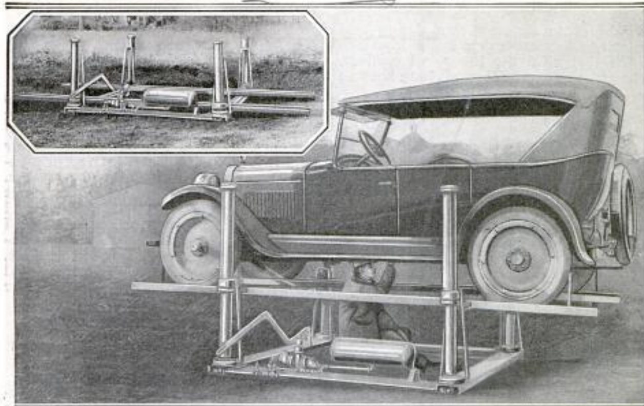
Hydraulic Hoist that Eliminates Pit in Repairing Automobiles and Lightens Mechanics' Labors. Below: Car Clamped to Runway and Raised
