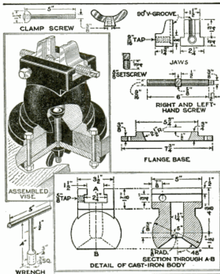
Bench Vise that Will Be Found Very Useful by Toolmakers and Machinists, as the Base Can Be Adjusted to Many Positions
