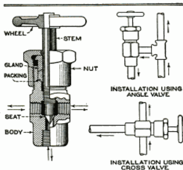
Left: An All-Steel Angle Valve for Use as a Cross Valve. Right: Comparative Installations
