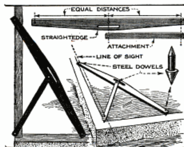
Accurate Method of Laying Off Right Angles by Means of a Simple Attachment for the Straightedge.
