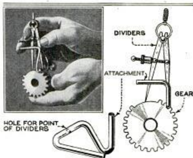
Simple Attachment that Enables the Repairman to Space Pegs Correctly When Repairing Gears
