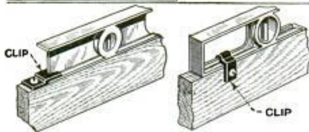
Above, Plumbing a Door Jamb; Below, Clips for Solid or Open-Frame Levels
