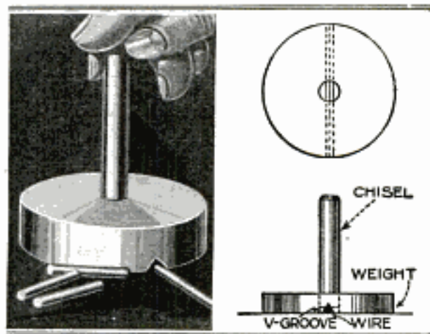
Left, Cutting Heavy Wire; Right, Details of Cutting Fixture
