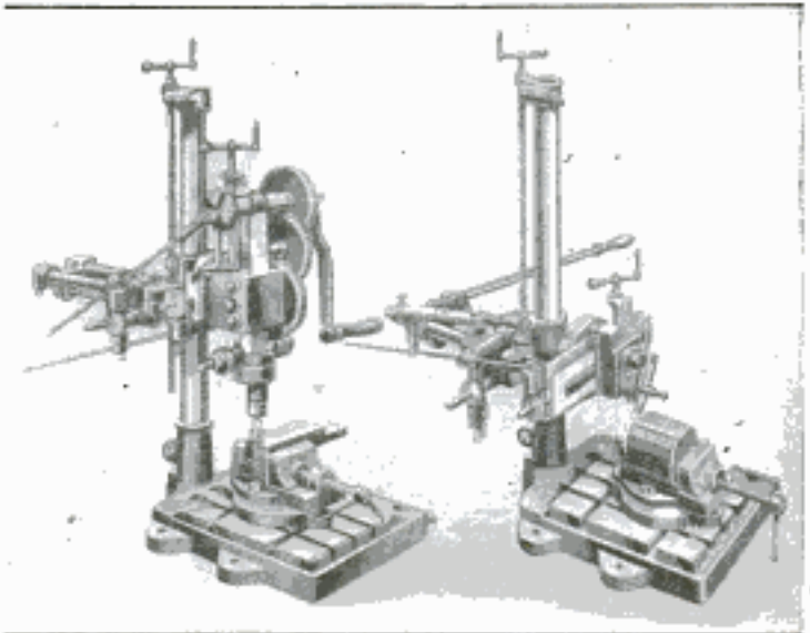
Left, "The Complete Workshop" Set Up for Milling; Right, in Use as a Shaper
