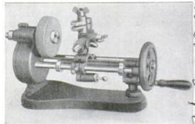
Scissor Sharpener with Vise and Handwheel that Moves Tool across Revolving Grindstone
