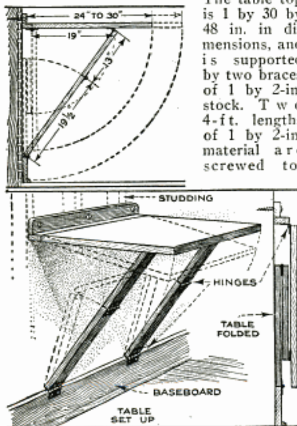
Folding Table for Small Kitchens that Can Be Set Up or Folded with One Hand
