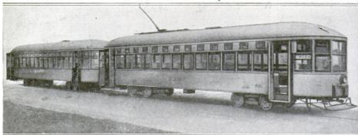
Trolley Cars in which the Usual Roar and Grind Has Been Eliminated by the Use of Automobile Brakes Instead of the Ordinary Iron Ones, and Roller Bearings
