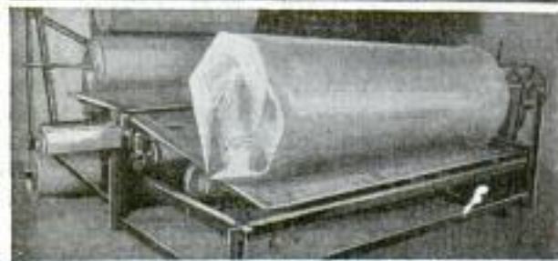
Machine that Replaces Hand Labor in the Packing and Wrapping of Mattresses
