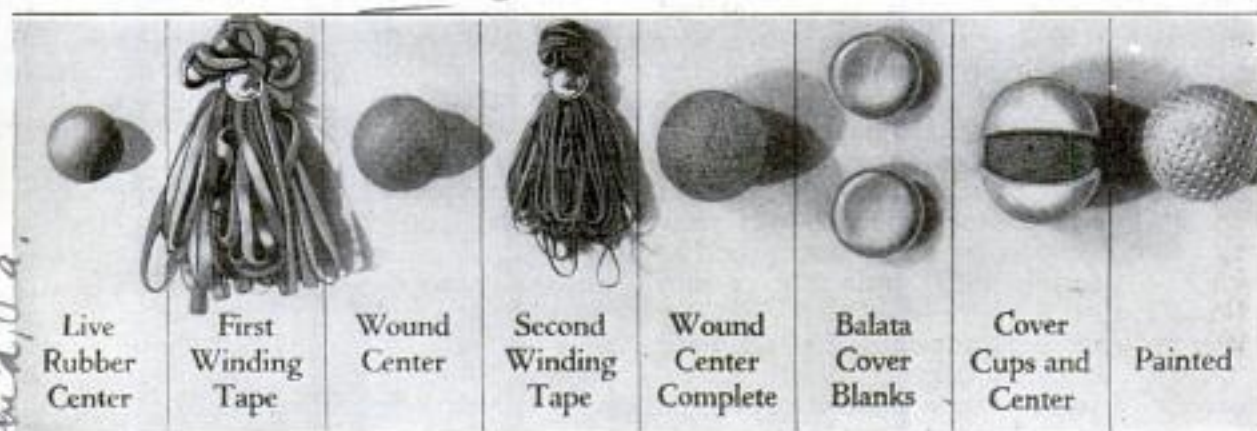
From a Center of Soft, Live Rubber, the Golf Ball Passes Through Various Stages, Acquires a Hard Rubber Shell, and Is Finally Ready for the Tee
