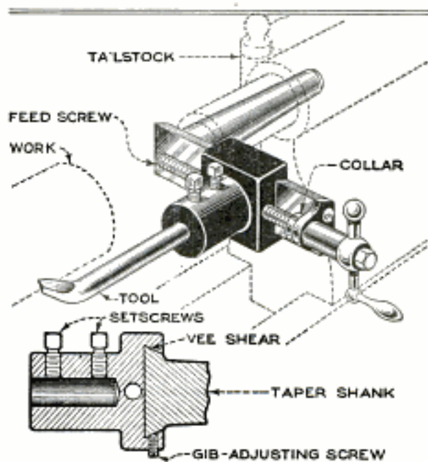
A Useful Attachment on Small Lathes for Boring and Turning Short Lengths Accurately
