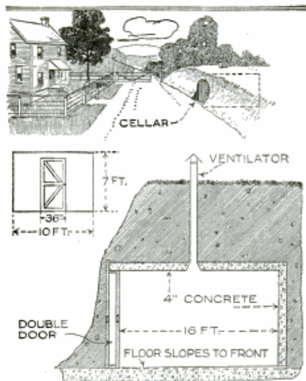
A Concrete Cold Cellar, Built in a Bank, that Has Many Advantages Over an Underground Cellar
