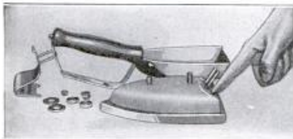
Electric Iron that Maintains a Working Heat Forty-Five Minutes After Current Is Shut Off
