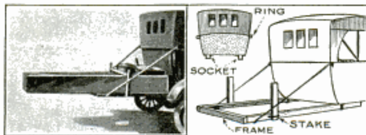
Attachment for Light Touring Car Permits Bulky Objects to Be Carried Easily
