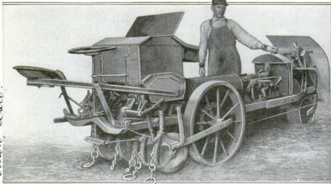
Tractor, Sower, and Cornstalk Turner Complete in One and Geared to an Automobile Motor for Planting Between Rows: Grain Is Carried in a Hopper
