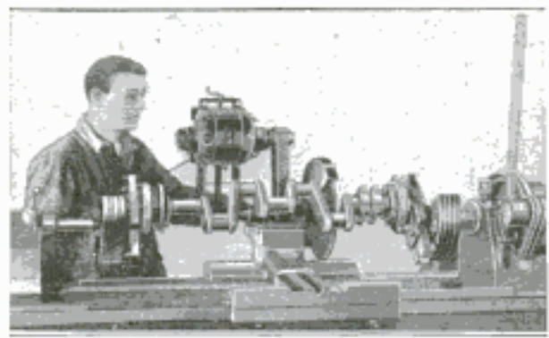
Grinding Crankshaft on Lathe, Using Ball-Bearing Throw Blocks
