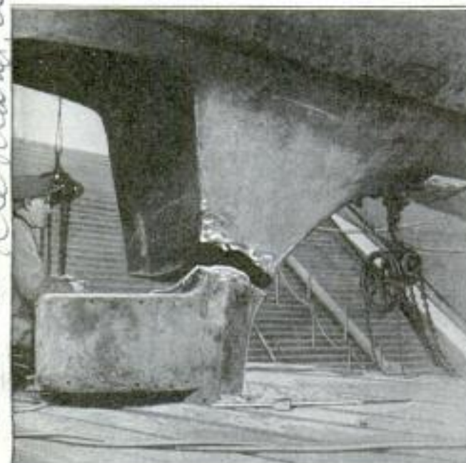
Broken Sternpost, Forced into Correct Position, Is Ready to Be Welded
