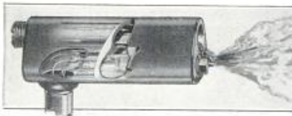
The Illustration Shows How Oil Is Mixed and Sprayed at the Combustion Point
