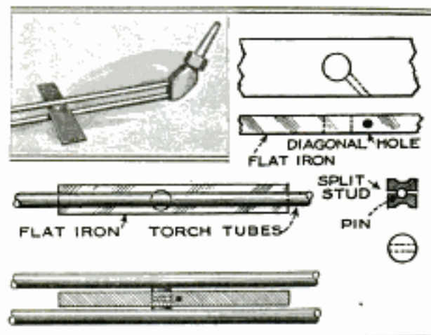
A Rest for the Acetylene Torch, of Utility when Laying Aside the Tool to Change Work
