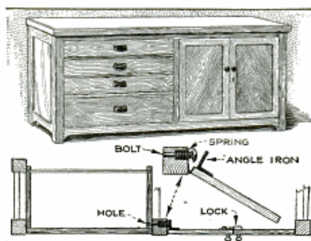
A Simple and Practical Arrangement for Making One Lock Do the Work of Five
