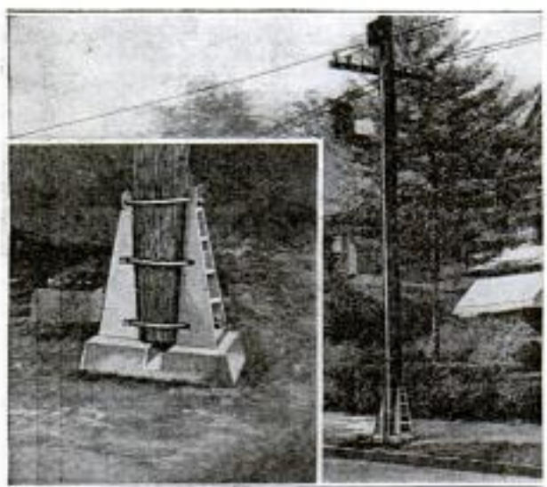
Pole Base of Concrete with Metal Grips that Are Tightened with Strap Bolts
