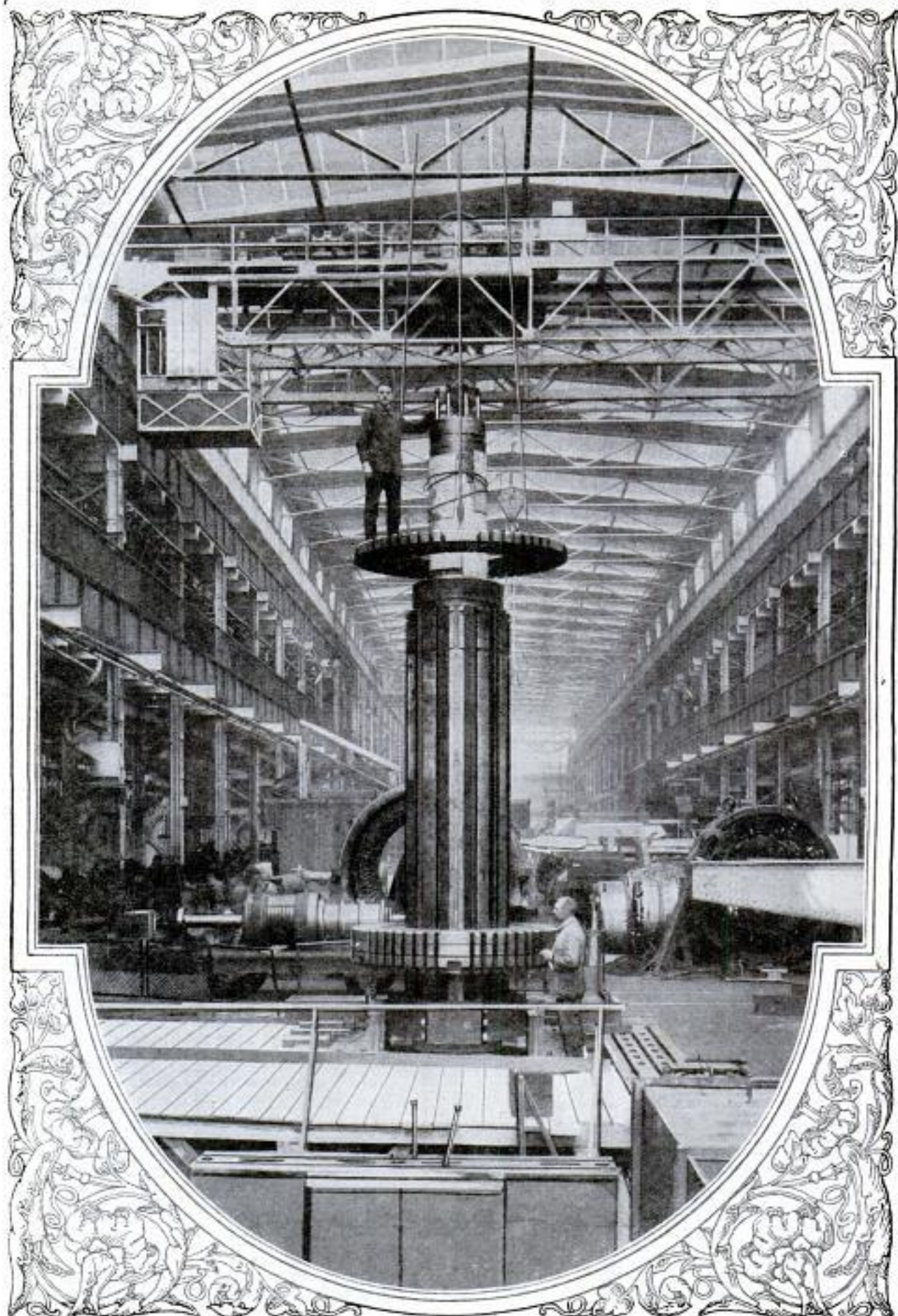
Putting the Finishing Touches on a Great Turbine Shaft in a German Erecting Shop—a Real, Man-Sized Task, Calling for the Highest Degree of Skilled Craftsmanship
