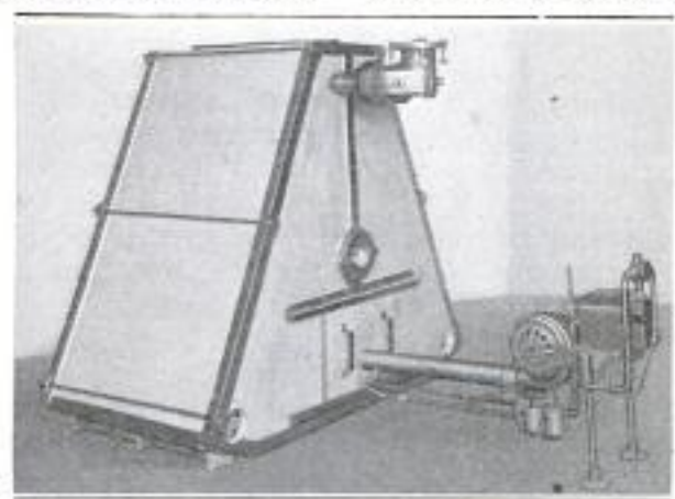
Striking the Sloping Side of this Triangular-Shaped Boiler at the Apex, Flames from the Burner Quickly Generate Steam. The Old and New Principles Are Illustrated by the Drawings
