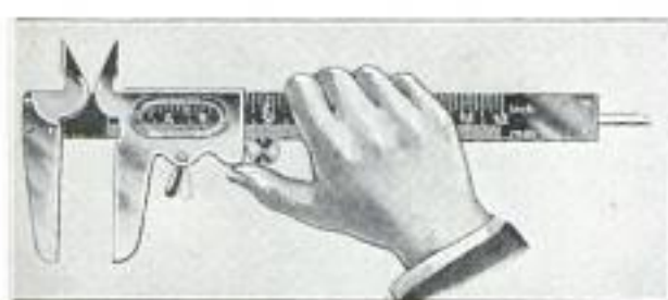
Method of Setting Movable Jaw of Caliper, Using Only the Thumb
