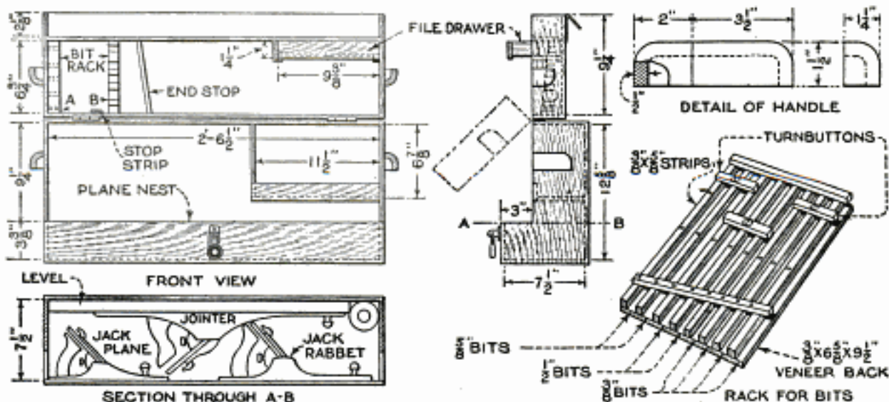
Above, Tool Box Open Ready for Work, with Saws on Shelf; Below, Full Details of Construction, and Method of Nesting Planes
