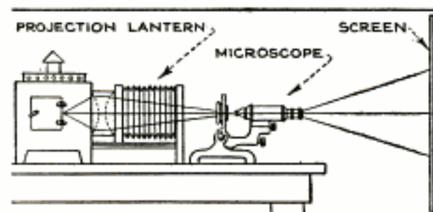
Simple Arrangement of Lantern and Microscope to Project Microscopic Slides in a Class Room
