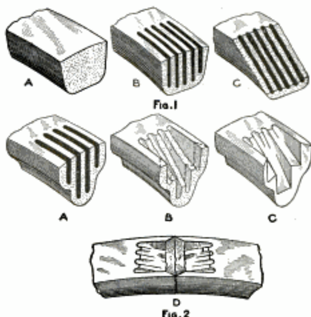
Improved Method of Doing a Good Job of Welding on Small, Irregularly Shaped Pieces
