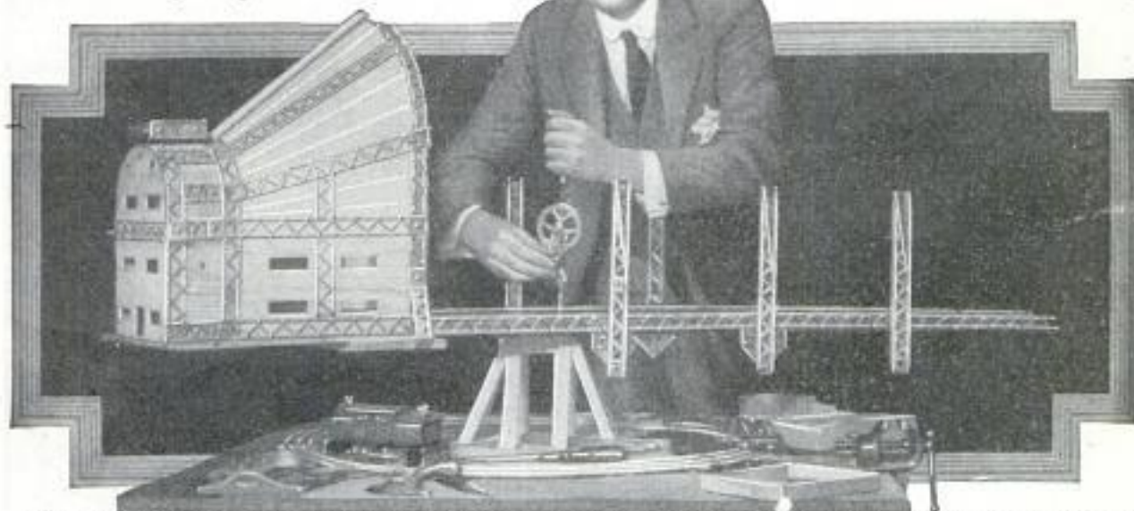
Model of Hangar Showing Construction of Hood and Floor which Will Support Sliding Platforms for Handling Dirigible Airships: One Section of the Roof Is Shown Completed
