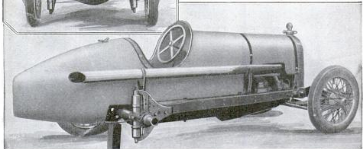
How the Telescoping Spring Cylinders on the Rear Axle Are Attached to the Racing-Car Chassis on a Yoke Bracket to Reduce Shocks While Speeding
