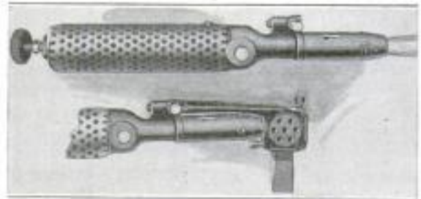
Blowtorch that Becomes a Soldering Iron with the Addition of a Detachable Tool
