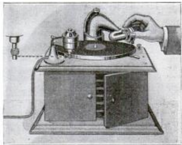
Electric Fan Motor Adjusted to Run Phonograph by Friction on Edge of Turntable
