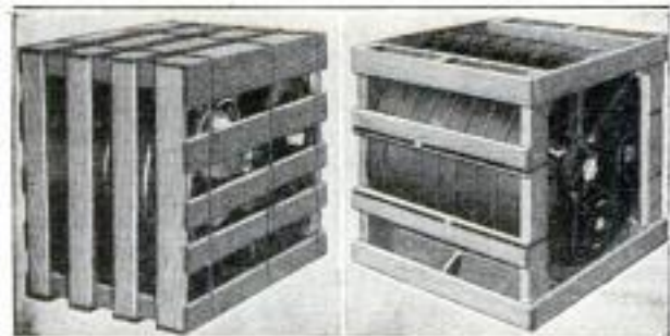
Shipping Crate Made by Experts to Save Lumber and Give Greater Strength
