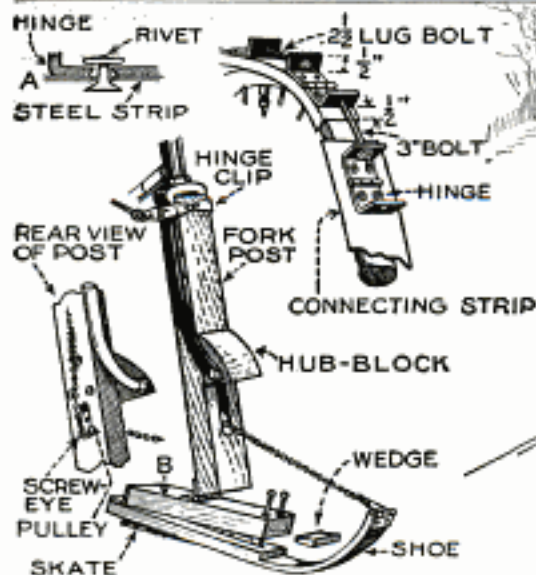
A Simple Tread and Steering Runner for the Bicycle that Will Enable It to Be Used in Winter as Safely as in Summer, and that Lessens the Hard Work of Pedaling in the Snow
