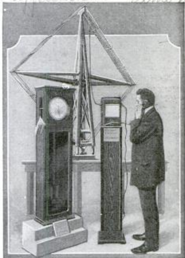
Aerial, Receiver, and Regulator that Compose Part of Wireless System for Setting Nation's Clocks
