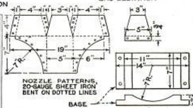
A Sturdy and Simple Blower for the Garage or Machine-Shop Forge Made from Scrap Material
