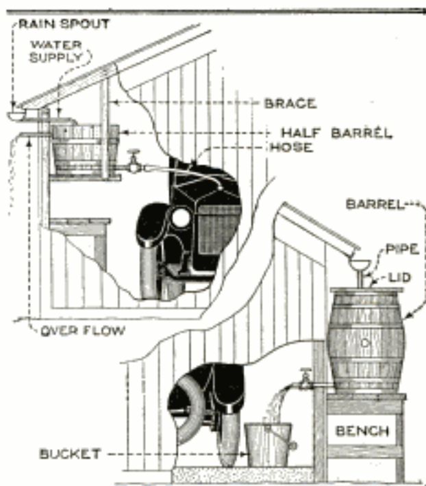
Easily Installed and Convenient Reservoirs for the Garage to Store Rain Water for the Radiator
