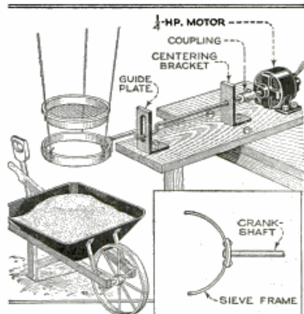
A Motor-Driven Sieve that Has Been Found a Time and Labor Saver
