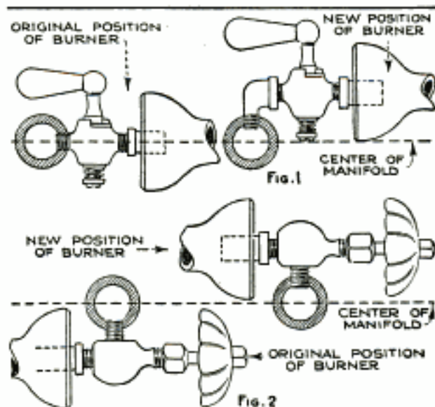
Changing Position of Natural-Gas Range Burners to Suit Lower Pressures
