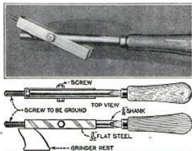
Simple but Effective Tool for Grinding Small Screws Rapidly
