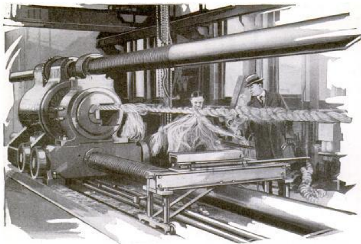
Photos Copyright, Underwood & Underwood Inspecting Manila Hemp Hawser as It Is Being Broken by Machine Capable of 2,000,000-Pound "Pull"
