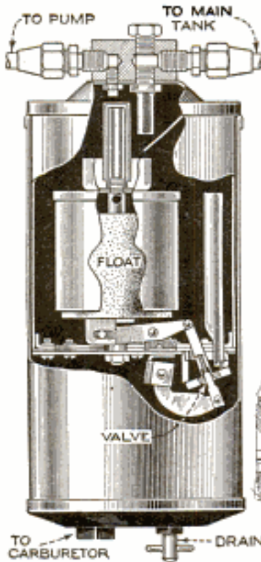
SECTION OF TANK AND VALVE MECHANISM
