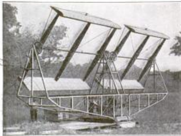
Helicopter with Revolving Wings that is Designed to Rise Directly from Narrowly Limited Spaces
