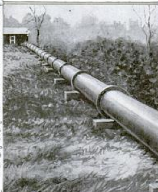
For Testing the Einstein Theory of Relativity this Vacuum Chamber Was Built of Sewer Pipe. Above: Instrument to Aid Scientists in Study of Action of Light in Tube
