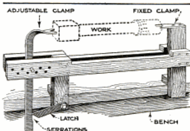
A Simple Clamp for the Woodworker's Bench Holds Work for Scraping, Shaving, or Sanding
