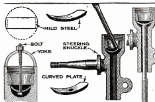
Method of Extracting Roller-Bearing Race without Distorting the Shell
