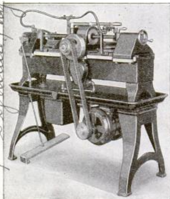
Both Ends of Automobile Axle Shafts and Similar Parts Are Turned at Once on This Lathe
