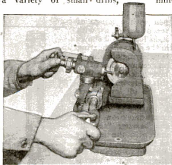
Drills, Milling Cutters, and Engravers' Tools Can Be Accurately Ground on This Bench Machine
