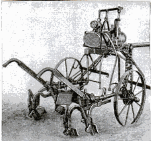
Light and Compact Spraying Outfit Mounted on Cultivator
