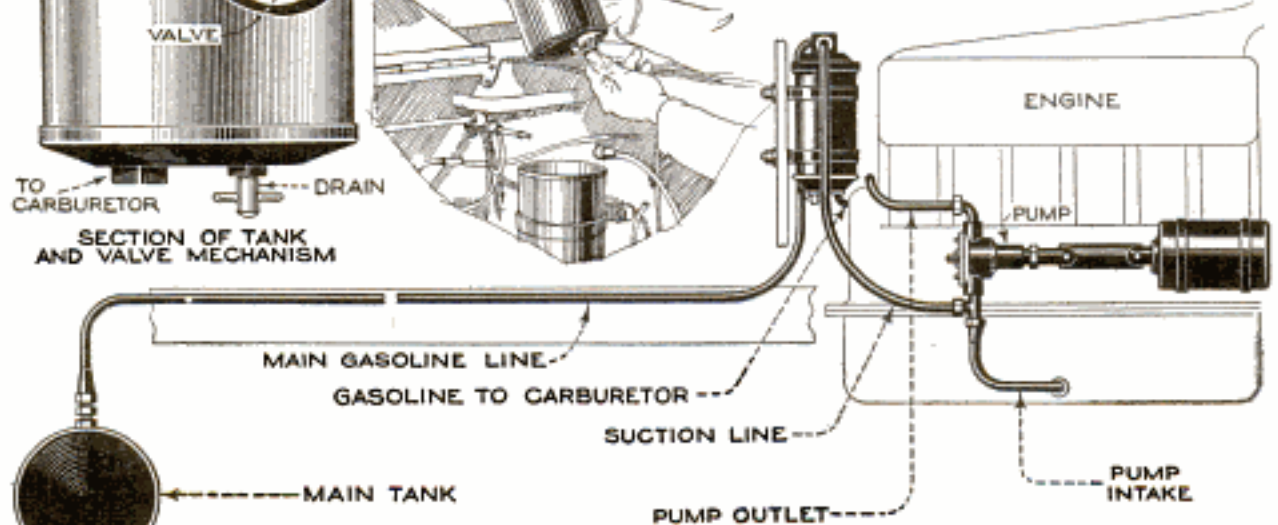
New Form of Vacuum-Tank System in Which the Suction Is Derived from a Specially Designed Oil Pump: When the Oil Runs Low, the Engine Stops
