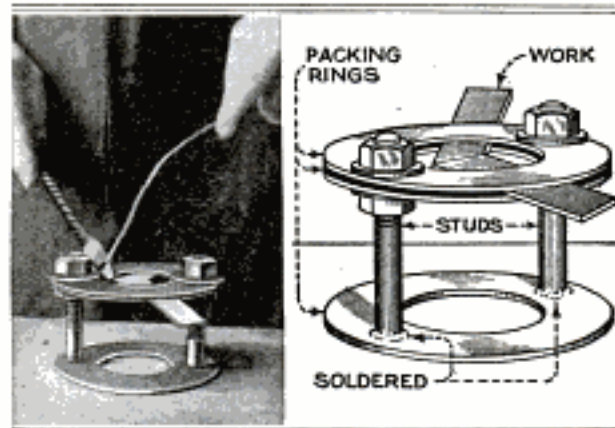
A Useful Clamp Made from Rings and Studs, Used for Holding Thin Pieces While Soldering
