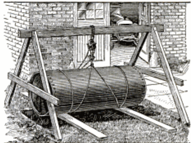
A Simple and Convenient Method of Lowering Large Metal Storage Tanks into Pits Dug for Them
