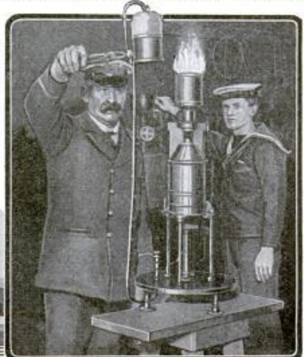
Attaching Powerful Oil-Vapor Lamp to Sea Buoy. One of Many that Guide Ships along English Coast at Night: Right, Regulating Light before Installing It
