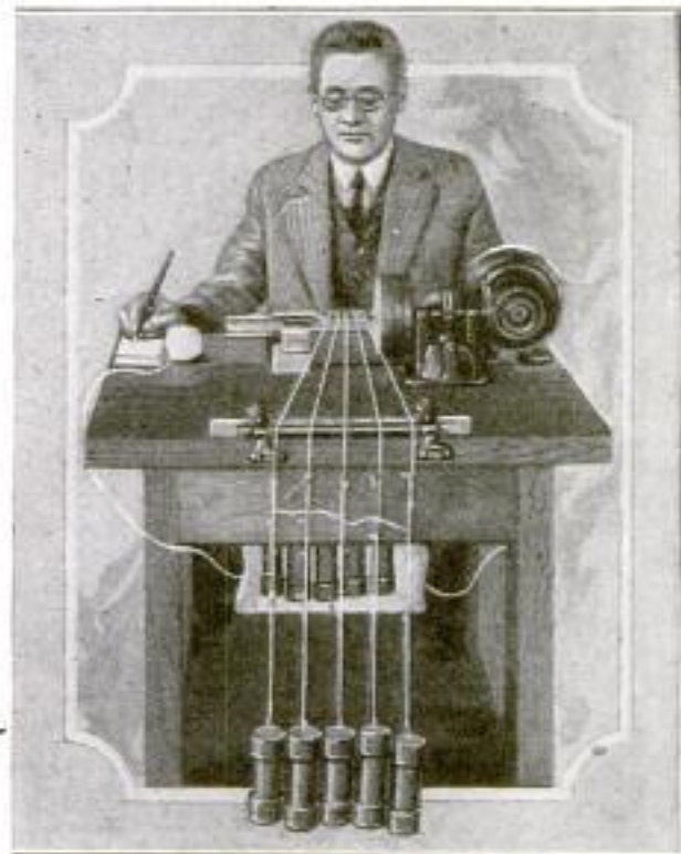
Testing Cords that Are to Be Used in Fish Nets to Determine Strength
