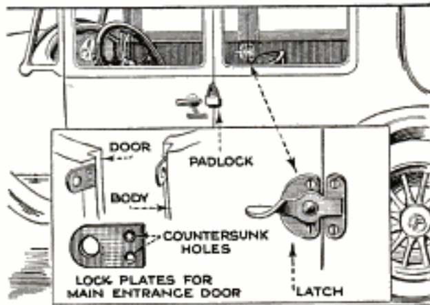
Simple Method of Locking the Doors of a Small Closed Car Using Only One Lock
