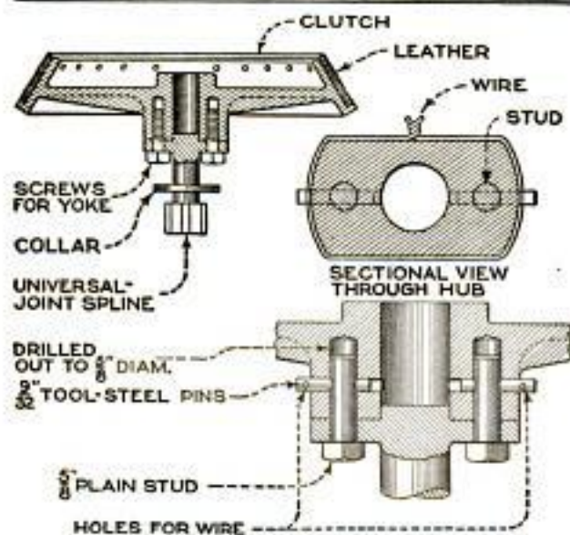
Quick Repair on an Auto Clutch: The Screws Are Removed and Plain Studs Substituted for Them
