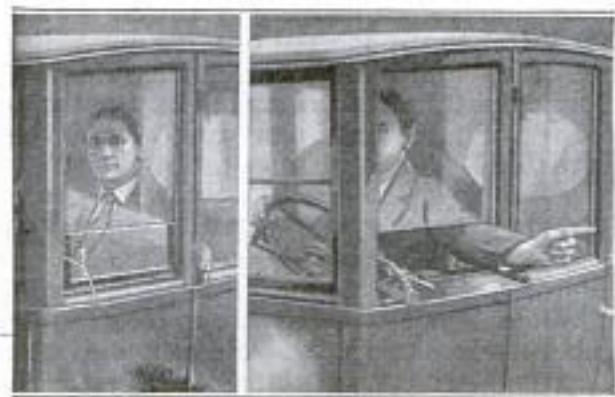
Hinged Window Section for Automobiles that Permits Hand Signaling on Outside of Closed Car
