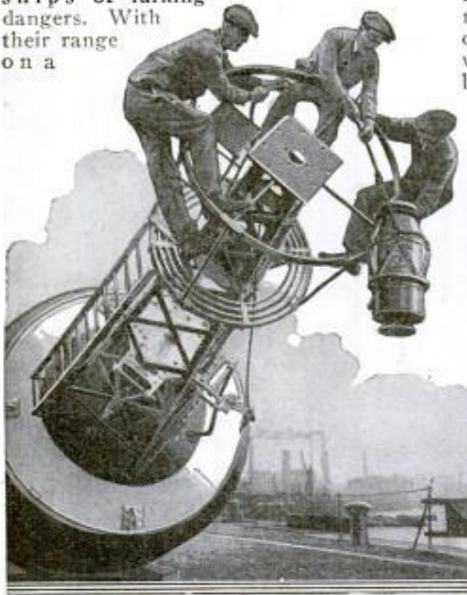
Attaching Powerful Oil-Vapor Lamp to Sea Buoy. One of Many that Guide Ships along English Coast at Night: Right, Regulating Light before Installing It
