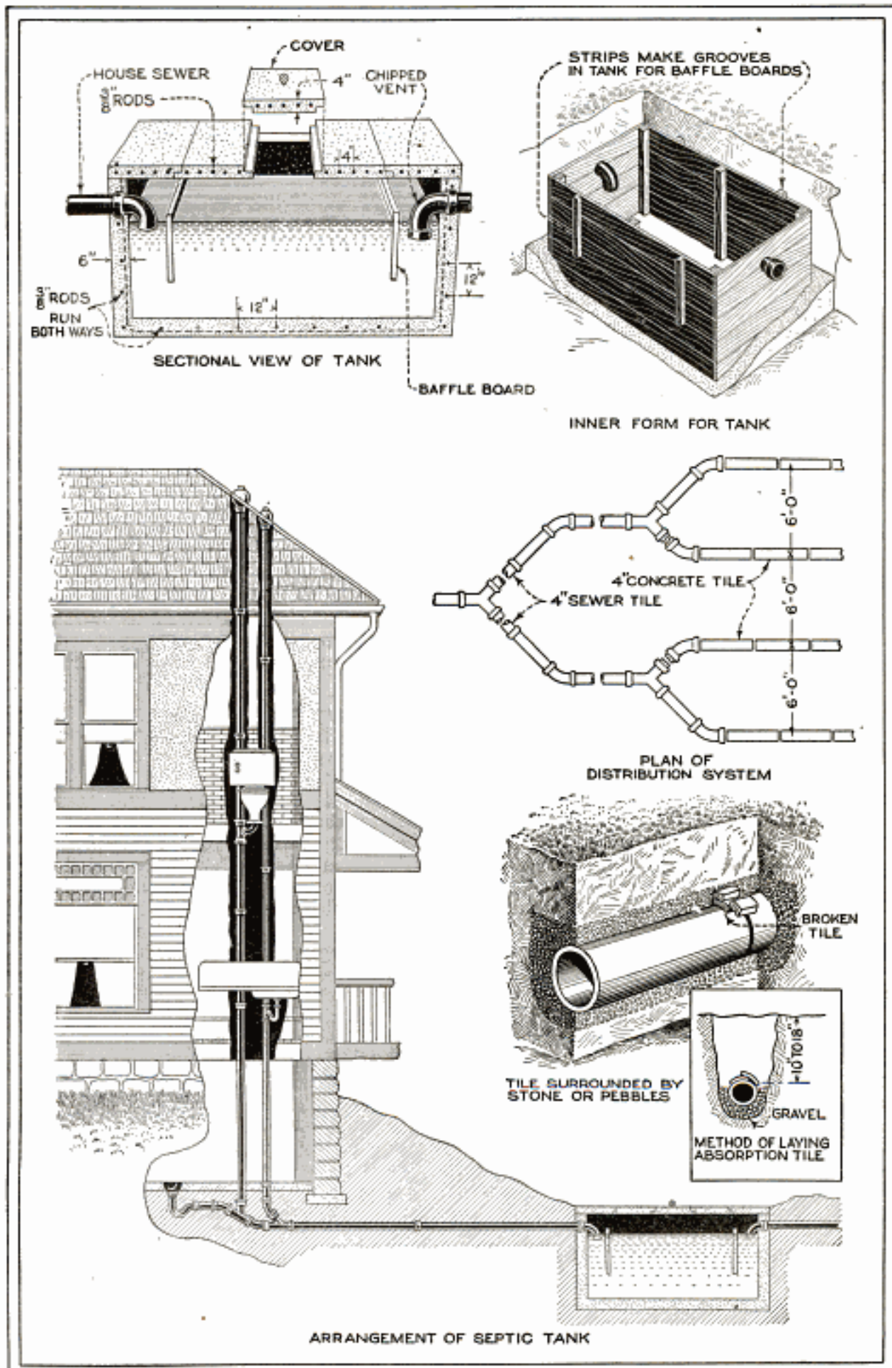
Details of the Making and Installation of a Simple Concrete Septic Tank: This Allows the Farmer to Install a Modern Plumbing System Where Sewers Are Not Available
