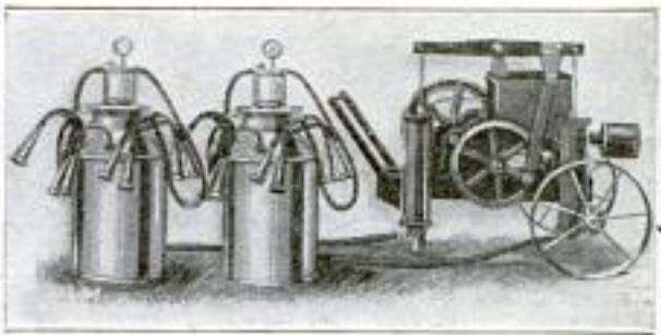
Self-Cleaning Milking Machine that Performs Work as Gently as when Done by Hand
