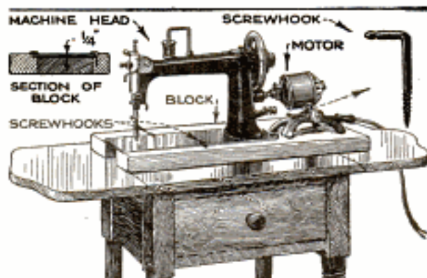
An Old Sewing Machine Made Portable and Run with an Electric Motor
