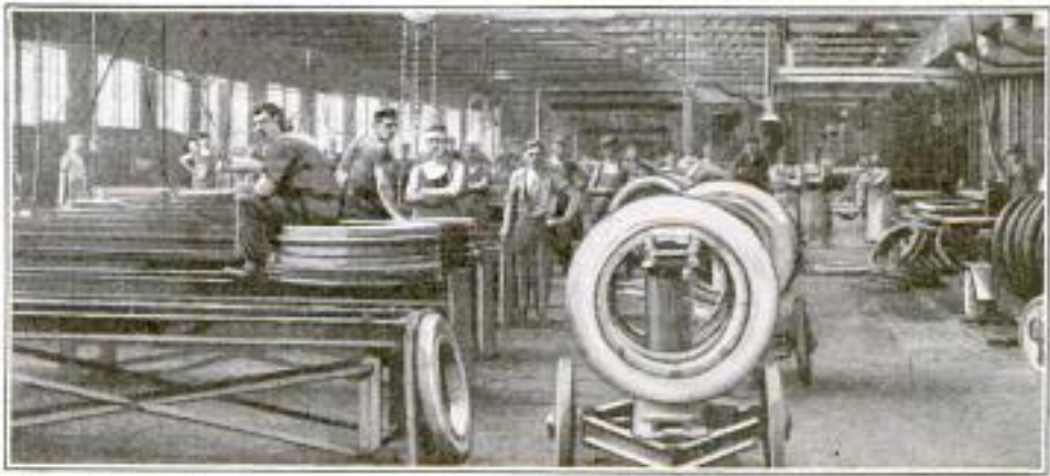
Vulcanizing Room of an Automobile Tire Factory where Casings Are Cured After Being Built Up of Raw Rubber
