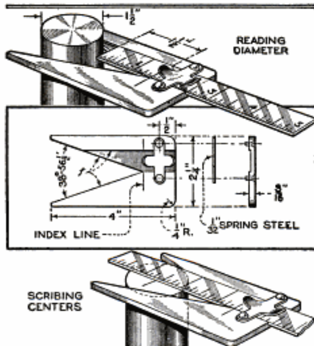
A Serviceable and Convenient Tool for Centering and Measuring Shafts
