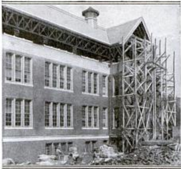
Inserting Extra Story at Top of School Building after Roof Was Raised
