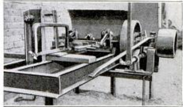
An Efficient Power Hacksaw, Made from an Old Automobile Engine Mounted on a Steel Frame
