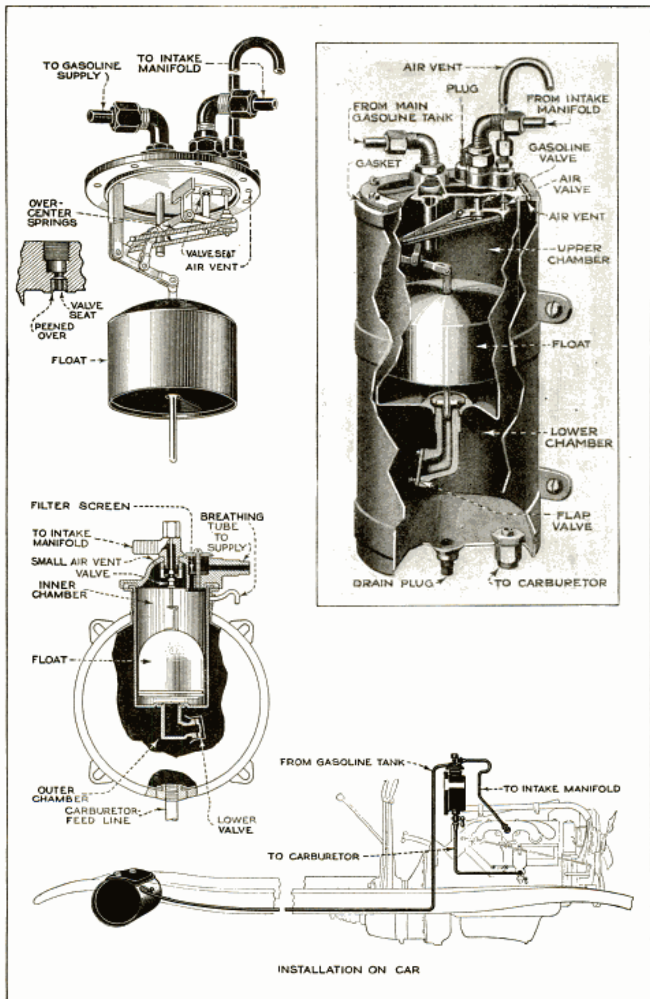
Above, Most Widely Used Type of Vacuum Tank, Showing Operating Mechanism; Below, a Simple, Compact Tank, and Its Mounting and Connections on the Automobile
