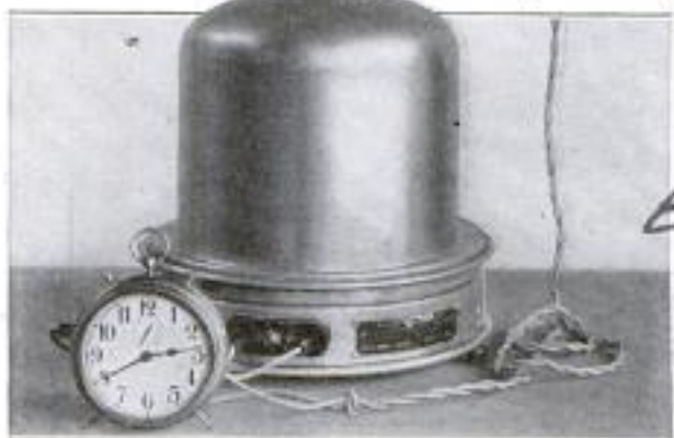
Electric Stove Controlled by Alarm Clock that Keeps Heat Below Burning Point after Food Is Cooked
