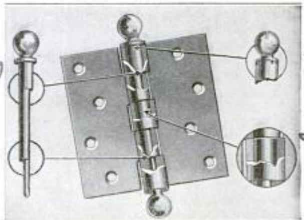
Adjustable Hinge that Is Said to End Door Rattling or Jamming with Turn of Center Pin
