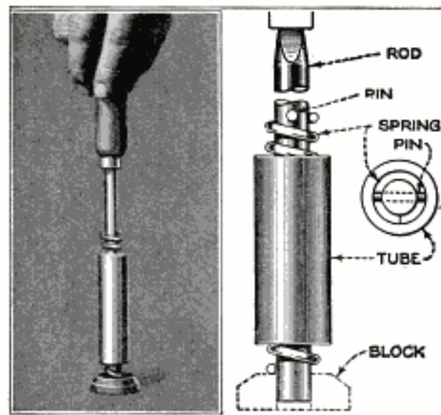
An Effective Tool for Flattening the Ends of Coil Springs Can Be Made from Scrap Stock
