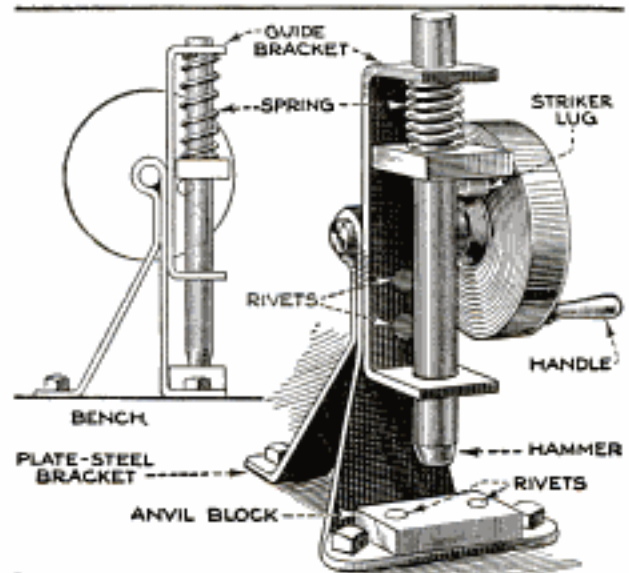
A Simple Hand-Operated Machine which Facilitates Riveting Operations Considerably
