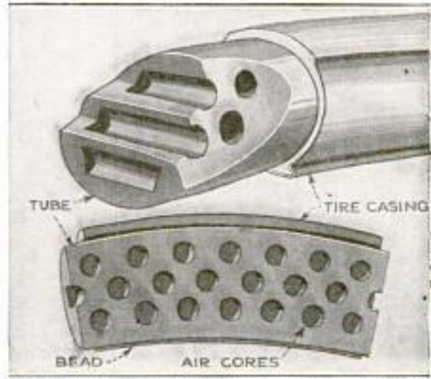
Puncture-Proof Tire Filled with Small Air Chambers that Needs no Other Inflation
