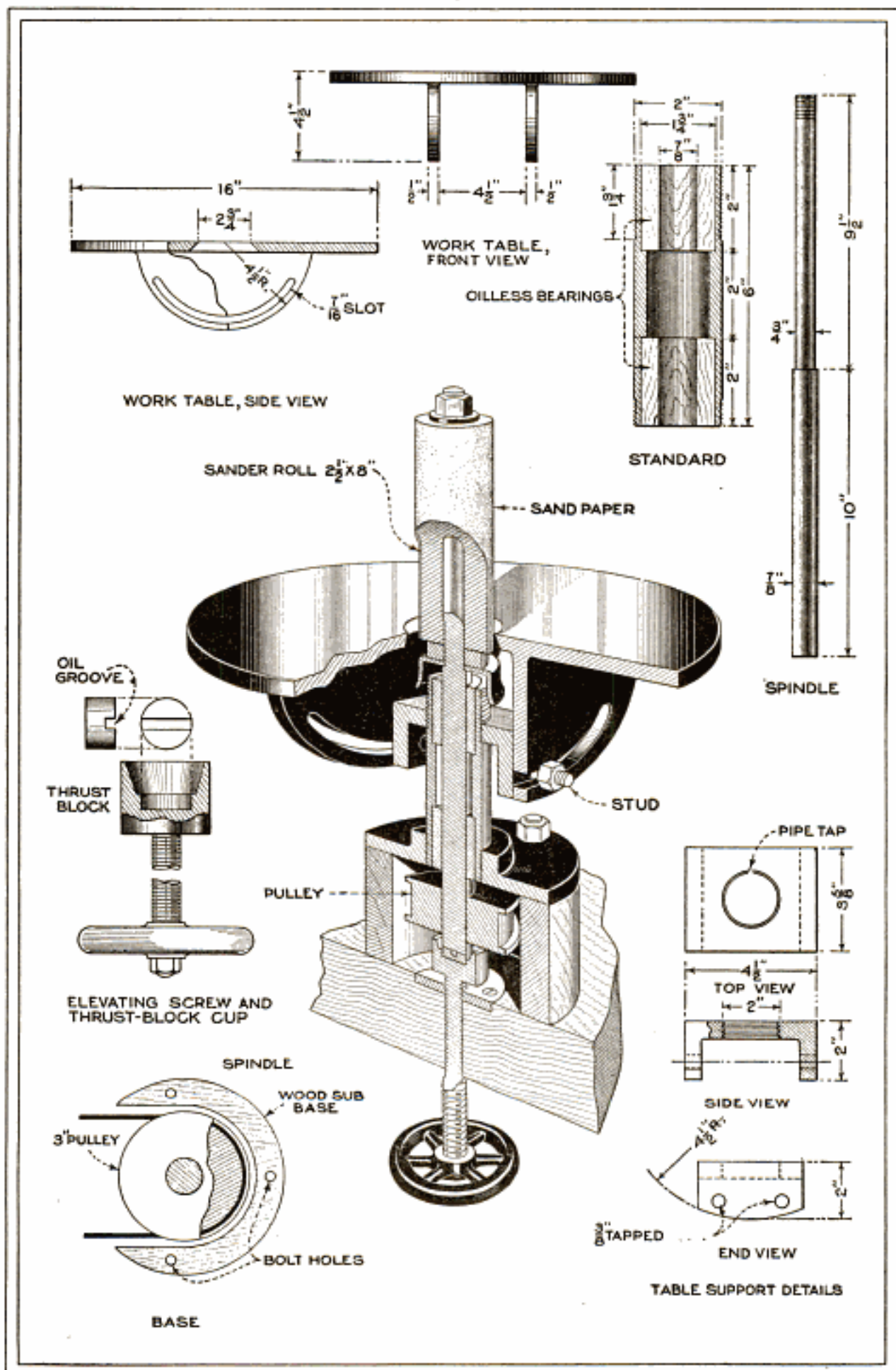
A Vertical-Spindle Sander that May Be Built in Any Small Shop, and that Will Prove of Great Value to Woodworkers and Patternmakers
