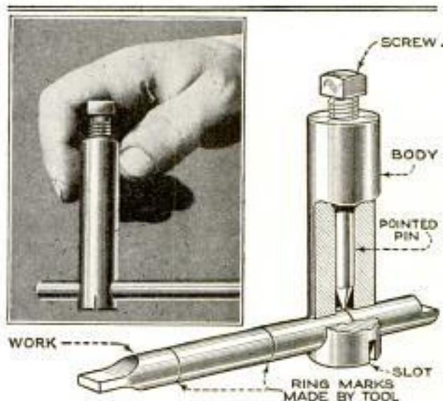
An Easily Made Tool for Scribing Circles on Light Rods Accurately and Quickly
