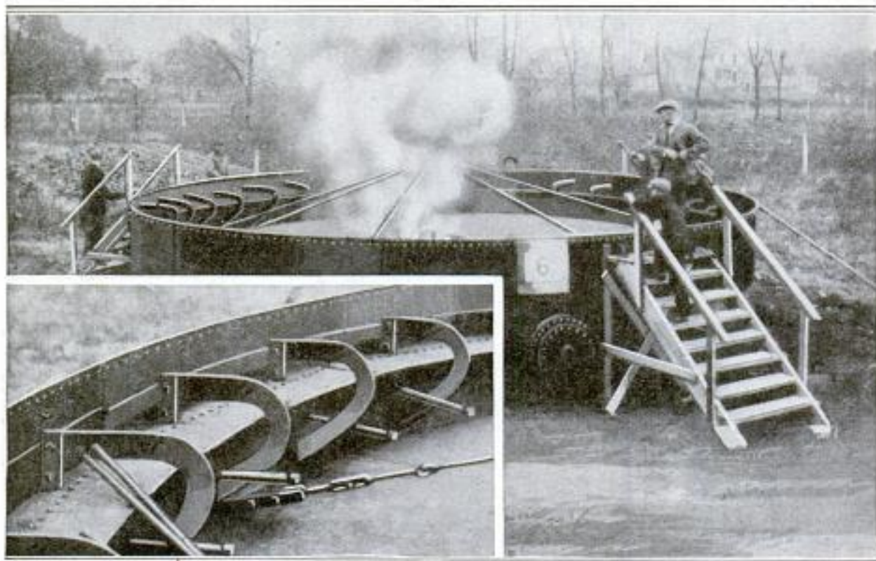
Floating Steel Roof for Oil Tanks to Reduce Evaporation and Fire Losses by Preventing Air Circulation at the Top: Left, Sealing Braces that Make Edges Tight
