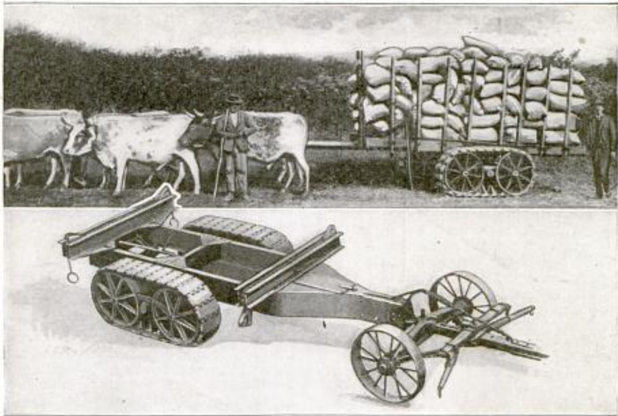
Above: Oxcart Fitted with Tank Tread that Makes Hauling over Rough Roads Light on the Animals. Below: Steel Frame of Horse-Drawn Truck with Banded Wheels
