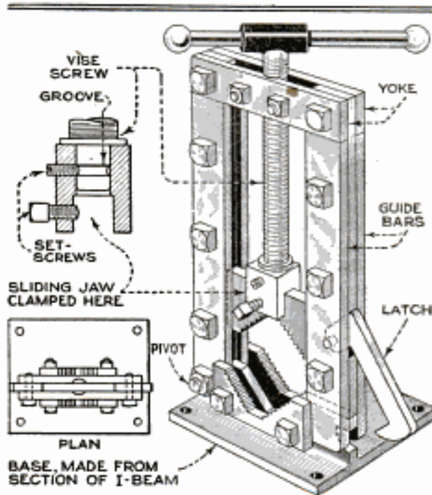
A Homemade Pipe Vise, Made from a Section of I-Beam and a Number of Short Steel Bars
