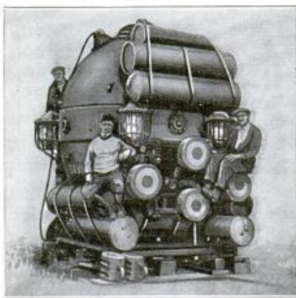
Diving Bell that Magnets Hold to Ship while Several Men Work Many Hours under Sea
