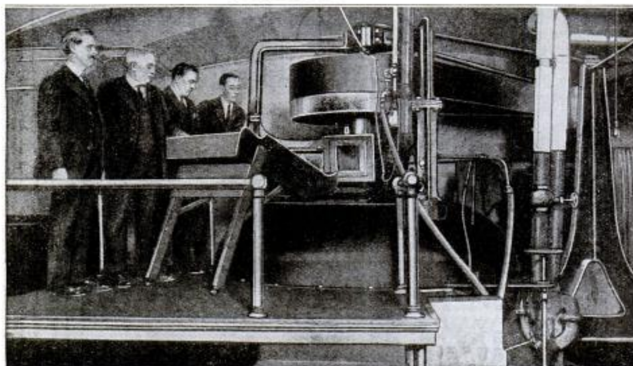
Giant Machine in United States Treasury Department, One of Ten, that "Eats" Millions of Dollars in Paper Money Which Are no Longer Fit for Circulation
