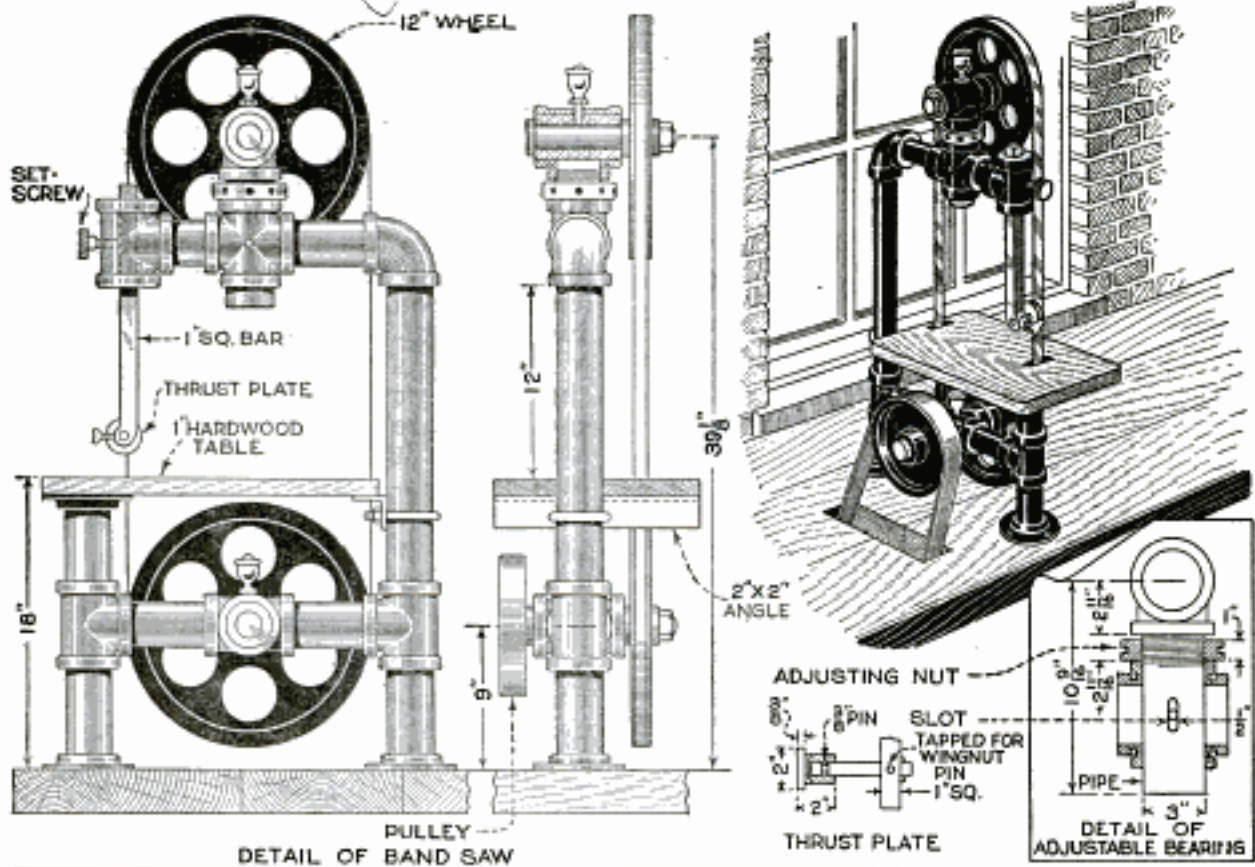
Pipe and Fittings, About the Most Easily Obtained of Materials, are Used Exclusively for the Frame of This Sturdy Bench Band Saw for the Small Shop
