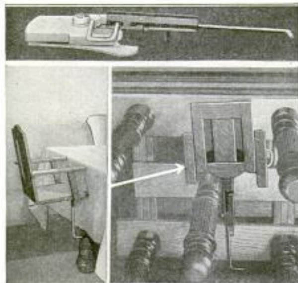
Folding Chair for Small Children That Disappears beneath Table Top When Not Needed
