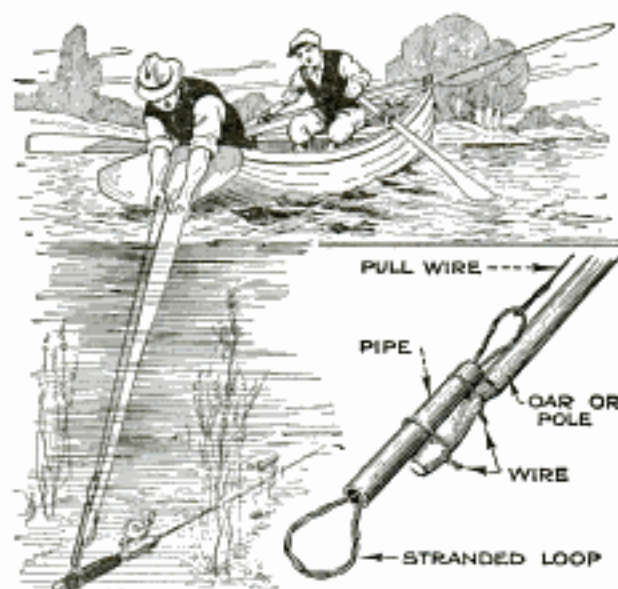
A Handy Device for Salvaging Objects Submerged in Shallow Water
