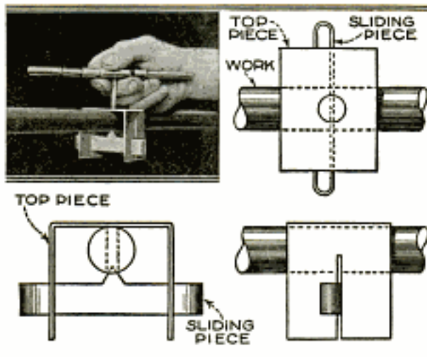
A Simple Guide Used for Tapping Round Work Square and Straight
