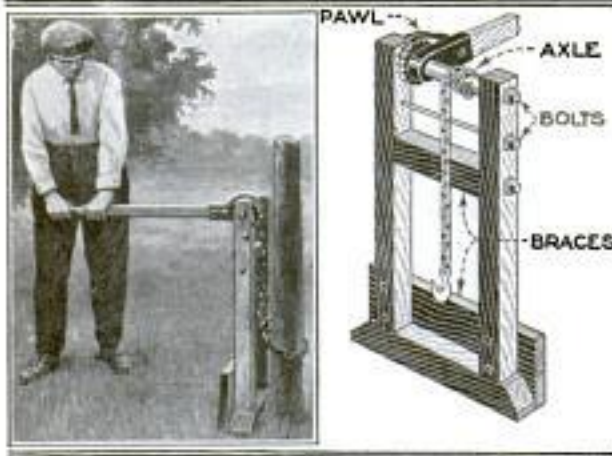
A Ratchet Post Puller will Pull Almost Any Post, Due to the Leverage Obtained
