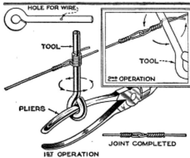
Lower Illustration Shows Method of Tightening Wire, and Insert, Method of Fastening Free End
