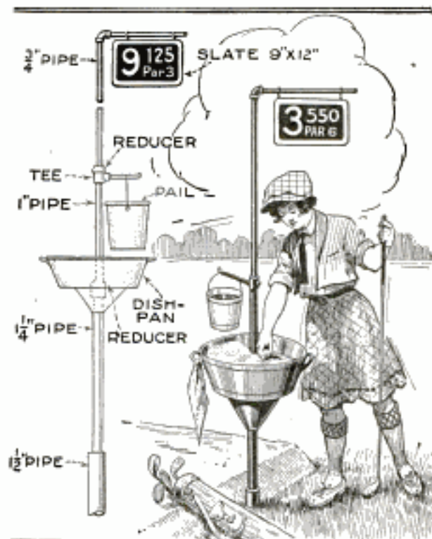
Homemade Sand Stand for the Golf Course That Is Just as Satisfactory as a Manufactured One
