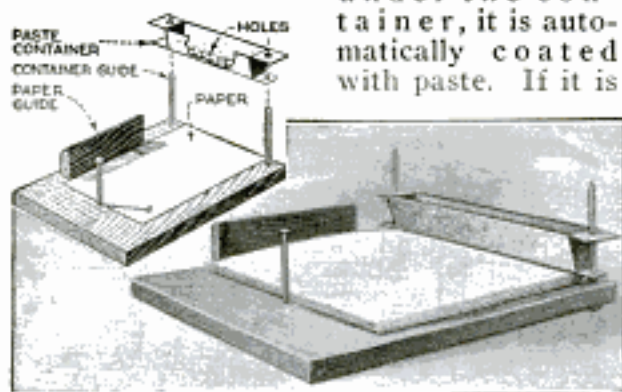
Device for Applying Paste to the Ends of Wrappers, That Speeds Up the Wrapping Process Considerably
