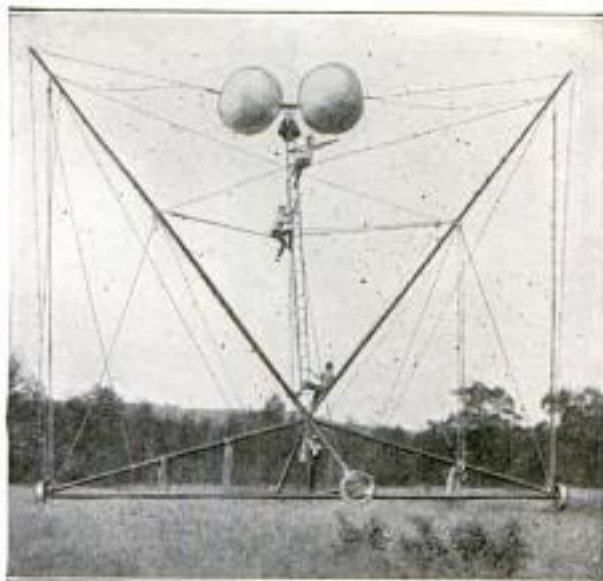
Army Balloons are Suspended from Mooring Frame for Spraying Crops to Kill Destructive Pests
