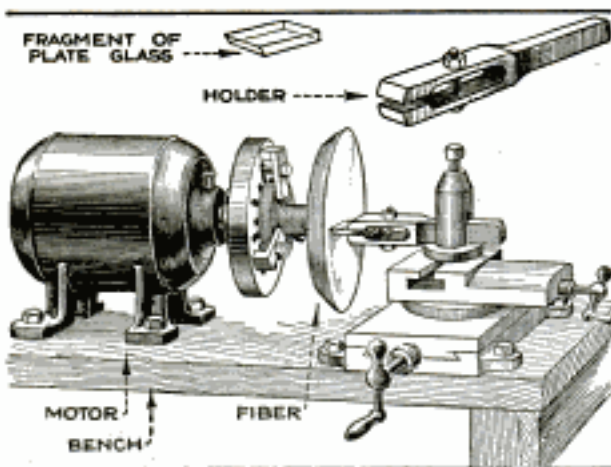
Method of Cutting and Facing Hard Rubber with Pieces of Plate Glass
