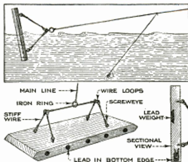
Fishing Block or Trolling Guide for Fishing in the Middle of a Swift Channel
