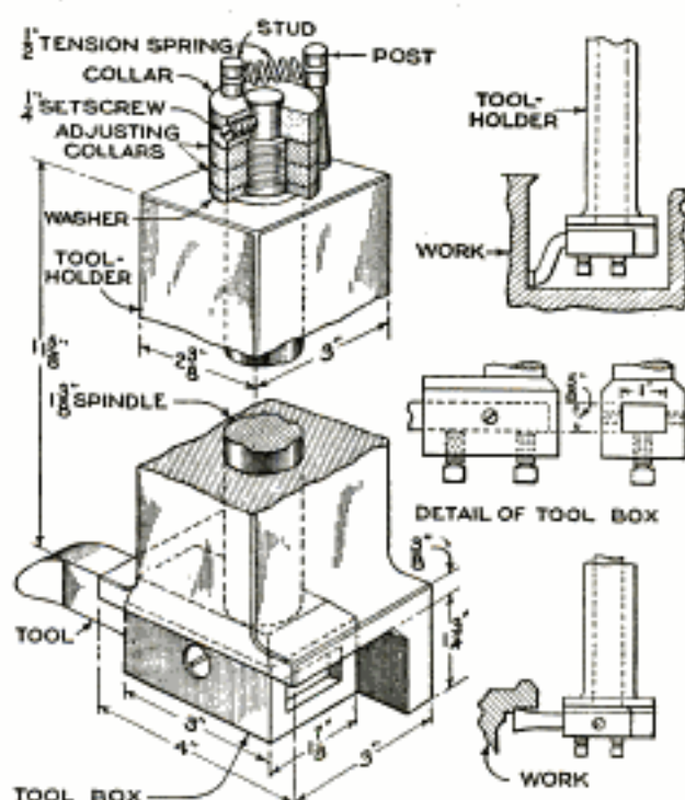
An Improved Holder for Side Planing That can be Used on Right or Left-Hand Work
