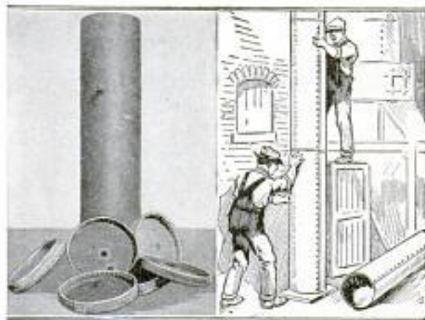
Left, Boiler with Ends Cut Off; Right, Erecting the Smokestack
