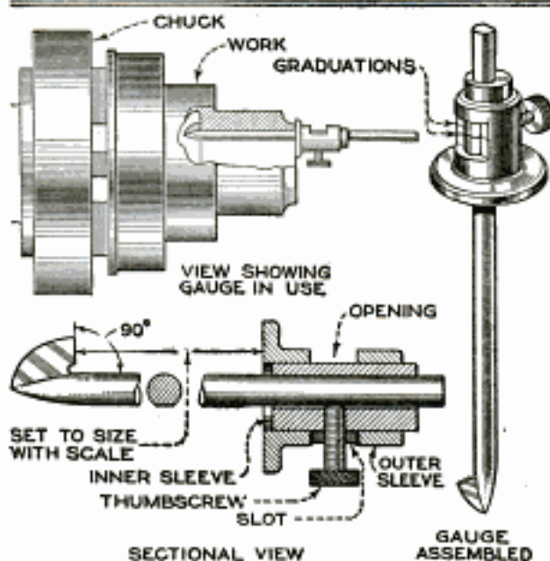
A Handy Hook Gauge for Measuring the Thickness of Hubs of Wheels, Gears, and Pulleys
