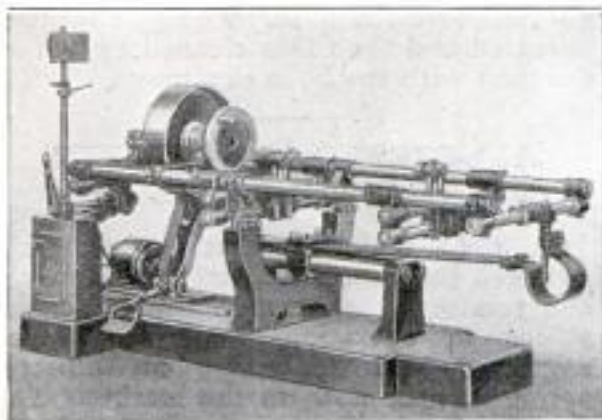
Machine That Determines Accurately How Much and Where Parts of High-Speed Machinery are Unbalanced
