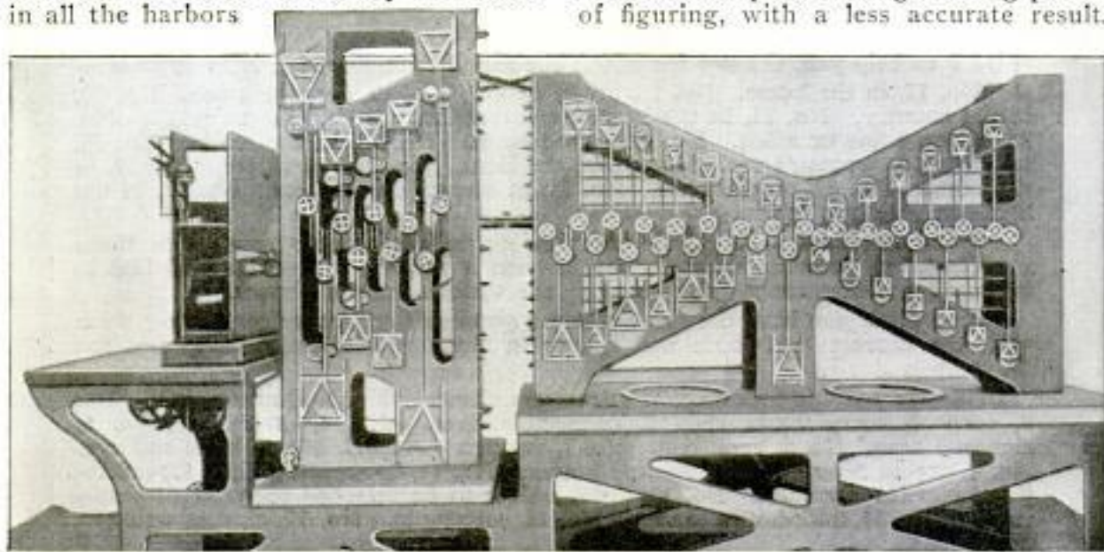
Predicting Time and Heights of Tides in the World's Principal Ports Far in Advance of Their Occurrence, Is the Work of This Remarkable Piece of Machinery
