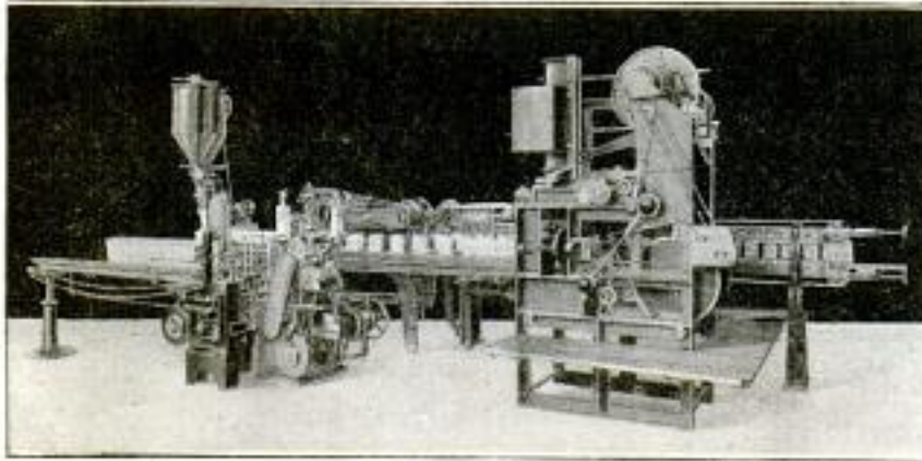
An Automatic Machine That Fills, Weighs, and Seals Cereal and Other Packages at the Rate of 18,000 per Day
