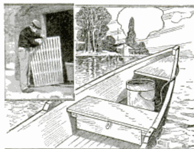
Left, Making a Slat Floor for the Fishing Boat; Right, Tackle Box Built under Seat
