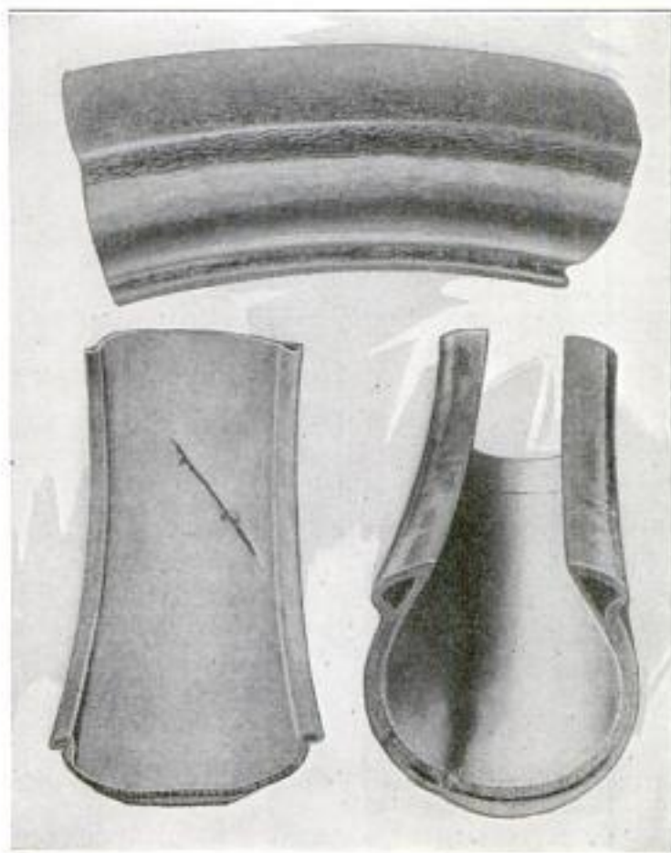
Above, Car-Track Wear; Left, Fabric Break from Stone Bruise; Right, Fabric Break Due to Running in Car Tracks
