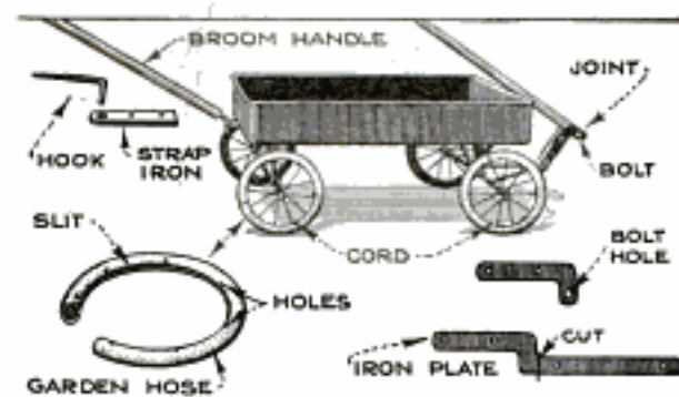
In Reconstructing a Small Cart, the Wheels were Rubber-Tired with Lengths of Ordinary Garden Hose
