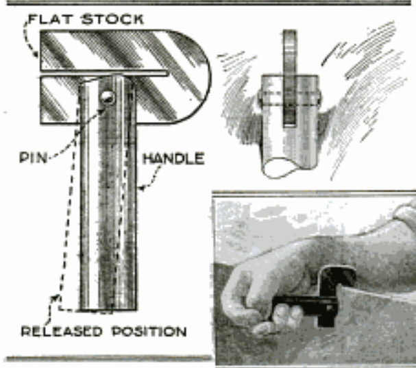
A Simple Holder That Enables Sheet Metal to be Carried with Ease
