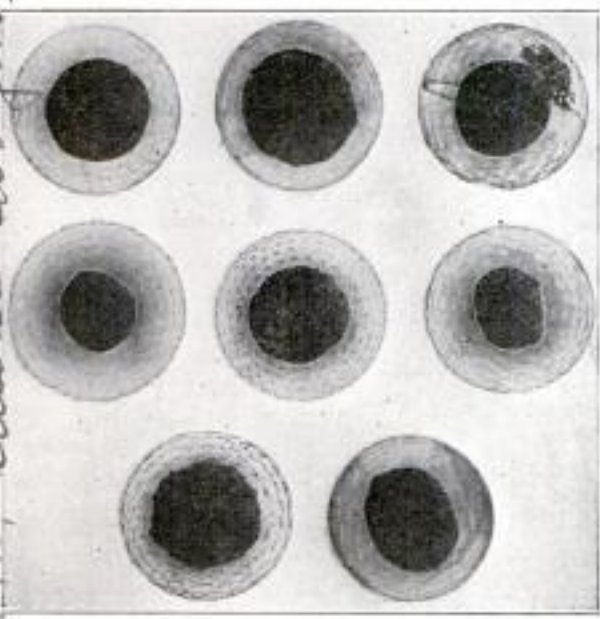
X-Ray Views of Golf Balls That Show Imperfect Cores, Which Pull or Slice the Drives
