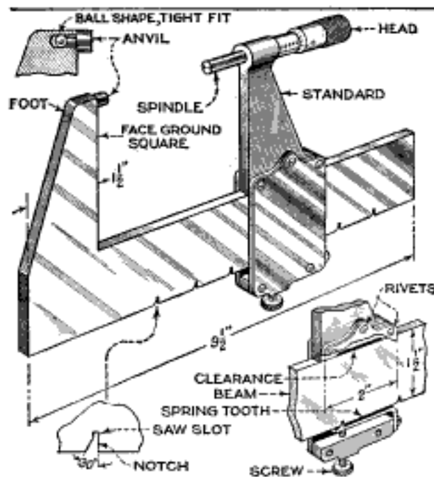
Beam Micrometer, Measuring from 0 to 6 Inches, That may be Made by Any Skilled Workman
