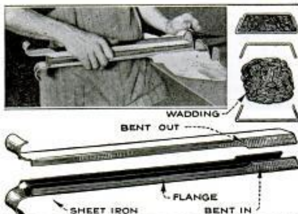
Auto Upholsterer's Stuffing Tool Permits Pleats to be Sewed First and Stuffed Afterward
