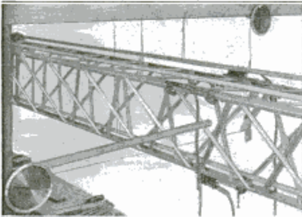
Strain Gauge for Detecting Weak Braces, Clamped in Position on Girder for Airship
