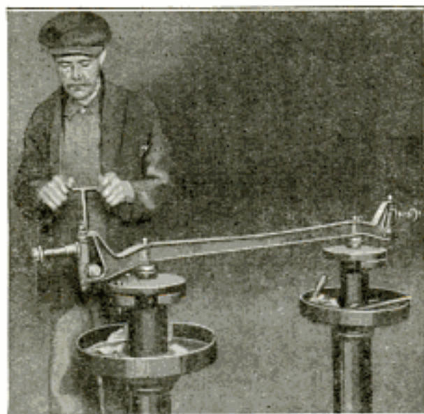
Stand Used for Assembling Front Axles of Automobiles That Facilitates the Work Considerably
