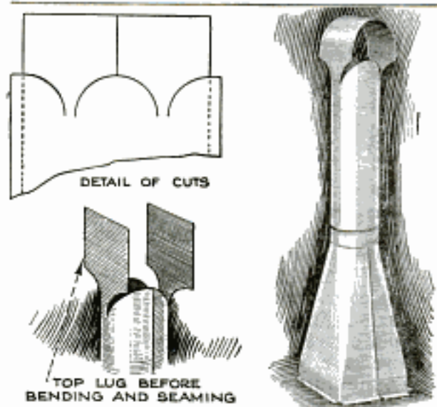
A One-Piece Chimney Extension Cap That may be Cut without Any Waste
