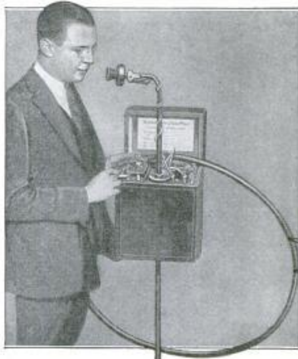
Radiotelephone That Carries Voice through Earth, Water, or Stone without Use of Aerial
