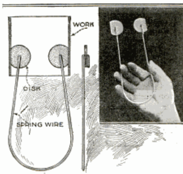
A Simple Holder for Handling Light Tubular Work for Such Operations as Dipping and Tinning
