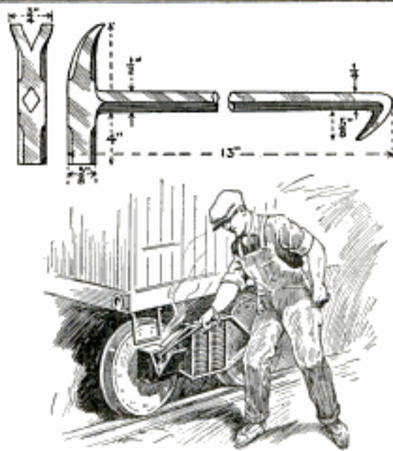
A Combined Tack Hammer and Journal Hook That Greatly Facilitates Railroad-Car Inspection
