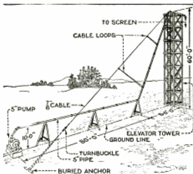
Efficient Method of Supporting a Long Discharge Pipe at a Gravel-Washing Plant
