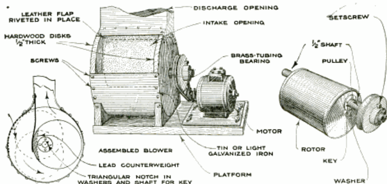
Where a Fairly Large Volume of Air at Low Pressure is Required in the Small Shop, a Blower Made from a Tin Can and Some Scrap Materials will do Satisfactory Work
