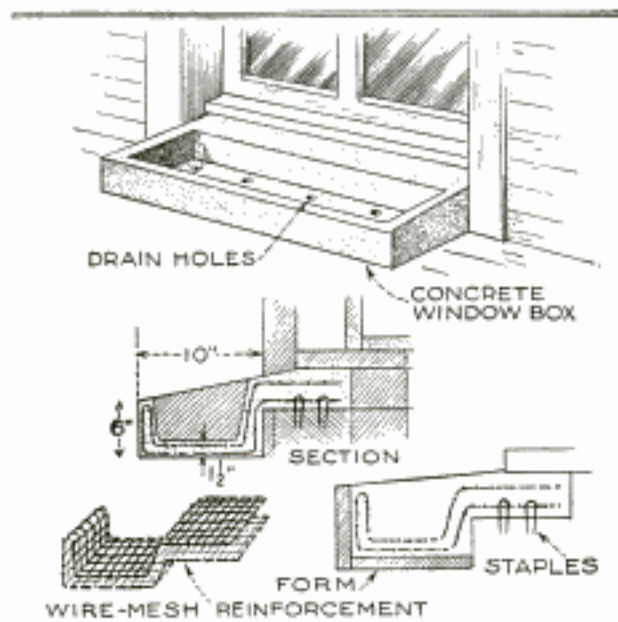
Combination Window Boxes and Sill in Concrete That Is More Durable than the Wooden Sill
