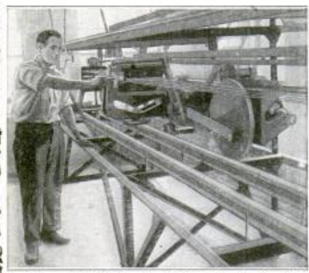
Twisting and Polishing Gut Strings for Tennis Rackets in One Operation
