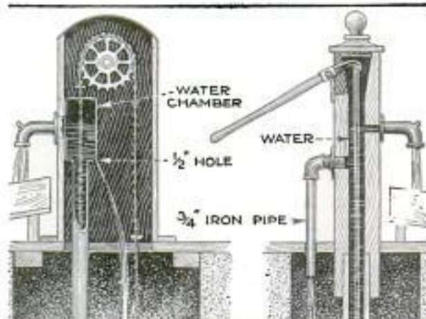
Simple, but Effective Method of Aerating Well and Cistern Water That Tends to Become Stagnant
