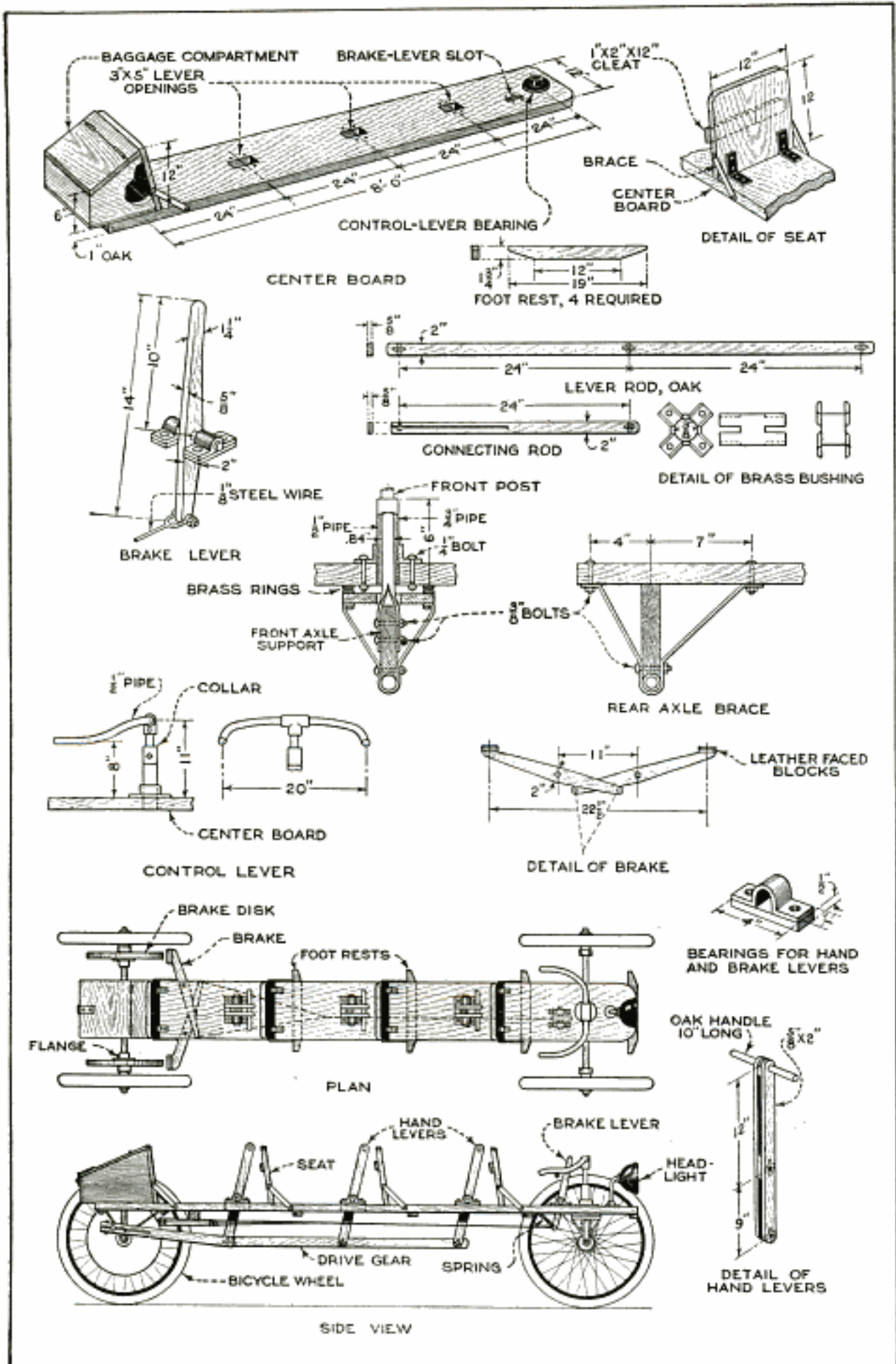
Top, Details of Main Board, Showing Baggage Compartment, Method of Bracing Seats, Sizes and Details of Lever and Connecting Rods and Their Bushings; Center, Cross Sections of Front and Rear Axles, and Details of Steering Post, Brake, and Lever Bearings; Below, Plan and Elevation of Car and Detail of Hand Levers
