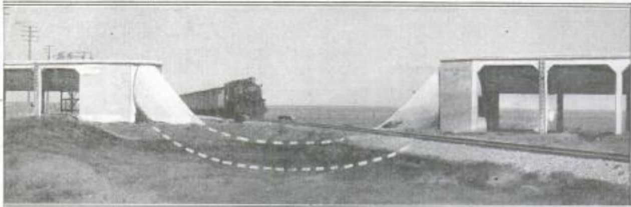
Inverted Siphon, Connecting Opposite Ends of Flume, Carries Water beneath Railroad Tracks, as Height of Curved Shell did Not Provide Sufficient Clearance for Crossing above Ground
