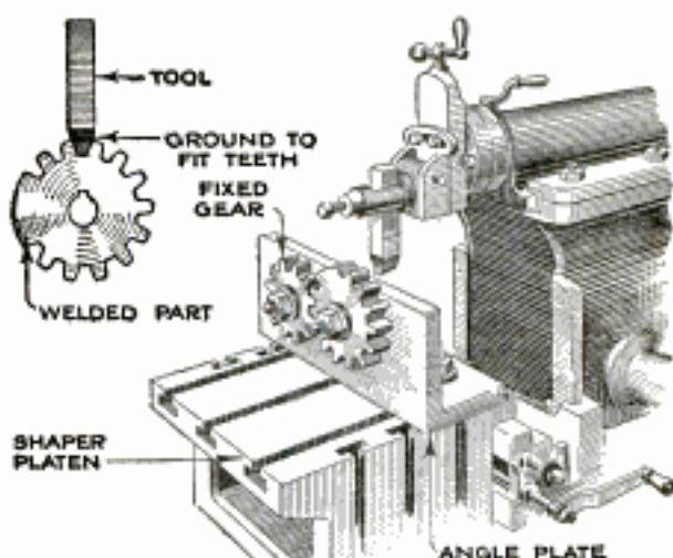
Machining New Teeth in a Damaged Gear Repaired by Welding
