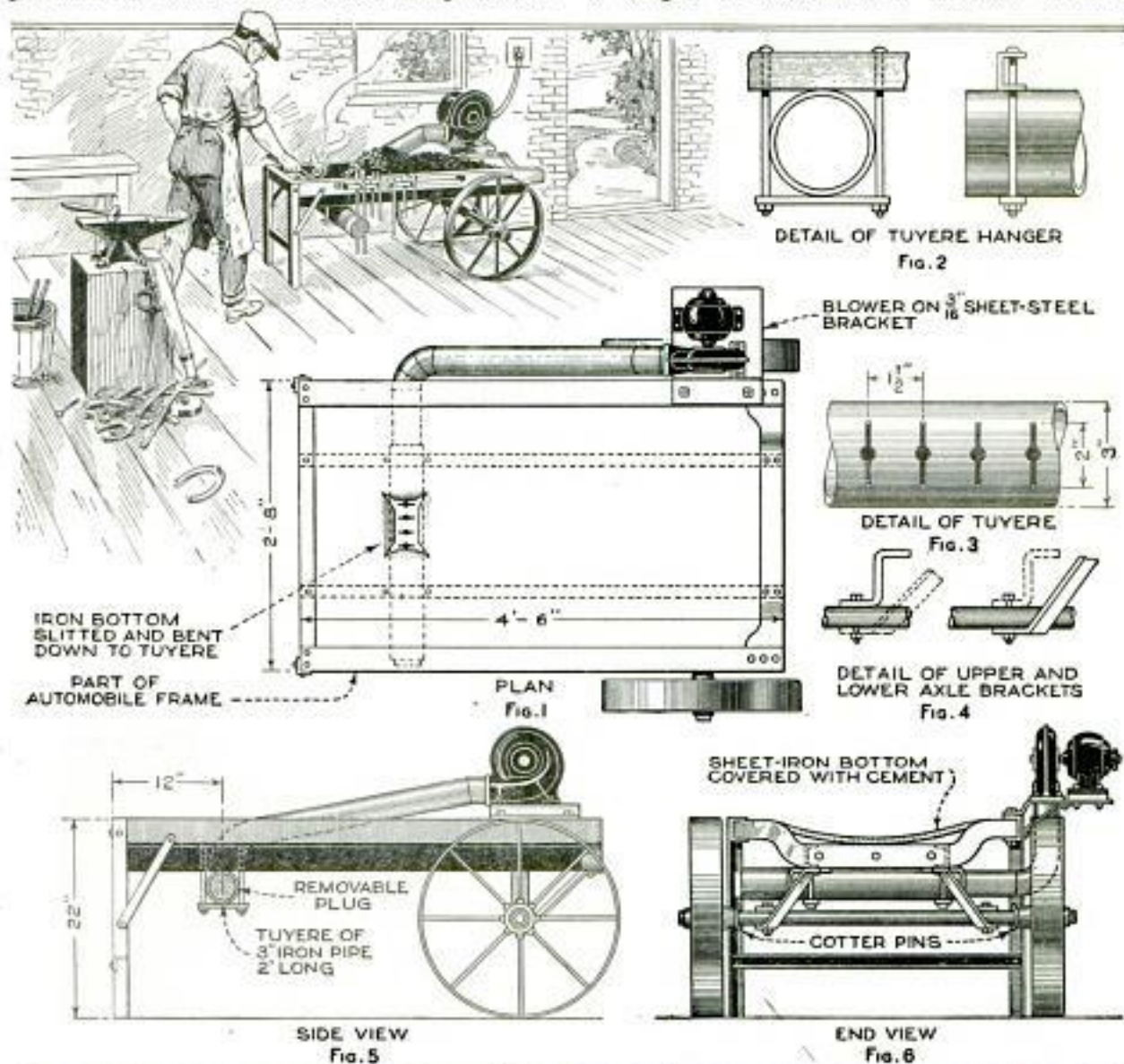
Figures 1, 5, and 6 Show the Plan, Side View, and End View of the Forge. Figures 2, 3, and 4 Give Details of the Tuyere Hangers, the Tuyere Draft Outlets, and the Axle Brackets
