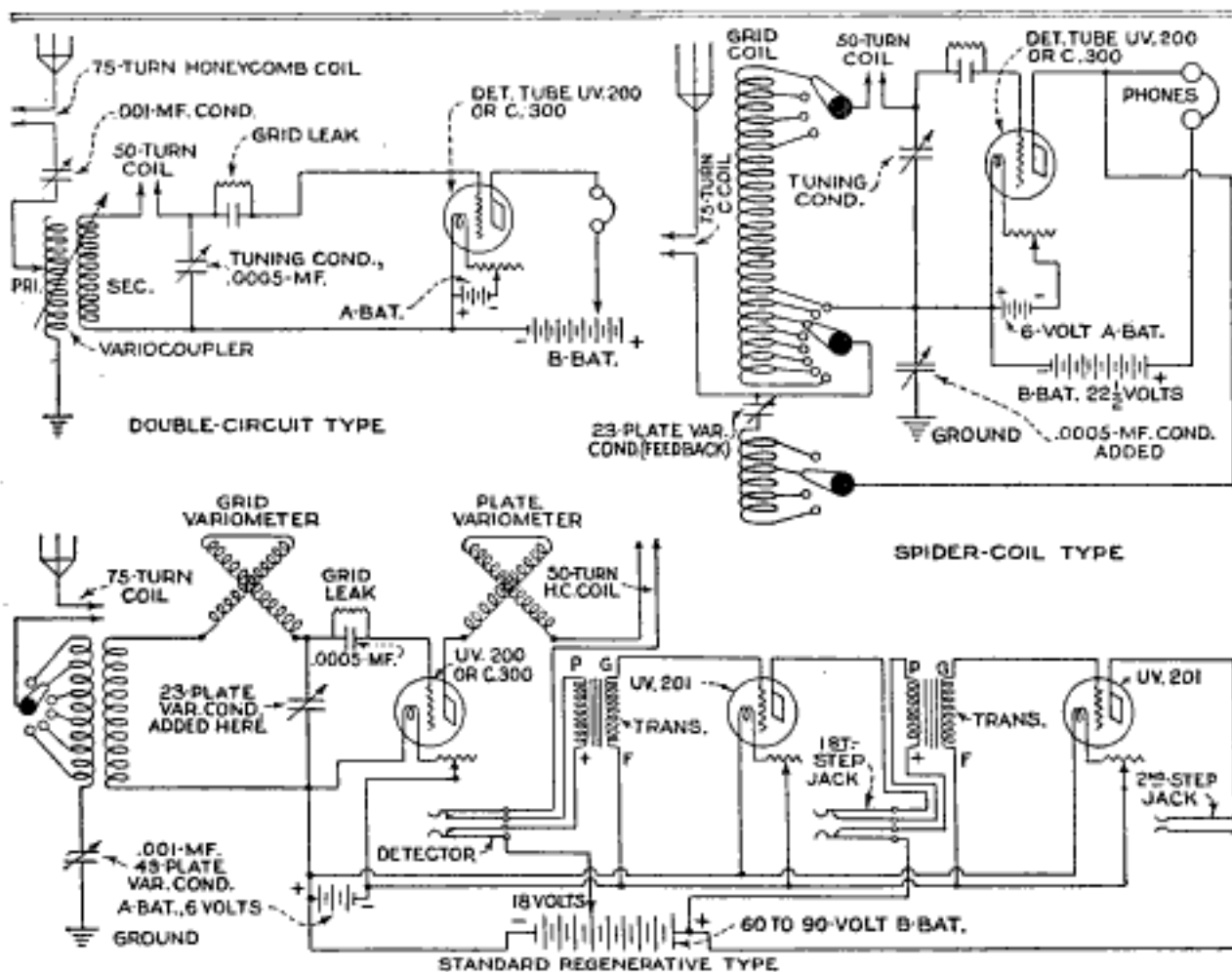
The Addition of Honeycomb Coils and Variable Condensers to the Common Types of Radio-Receiving Instruments Allows Them to be Tuned to the Longer Wave Lengths That are Now Used
