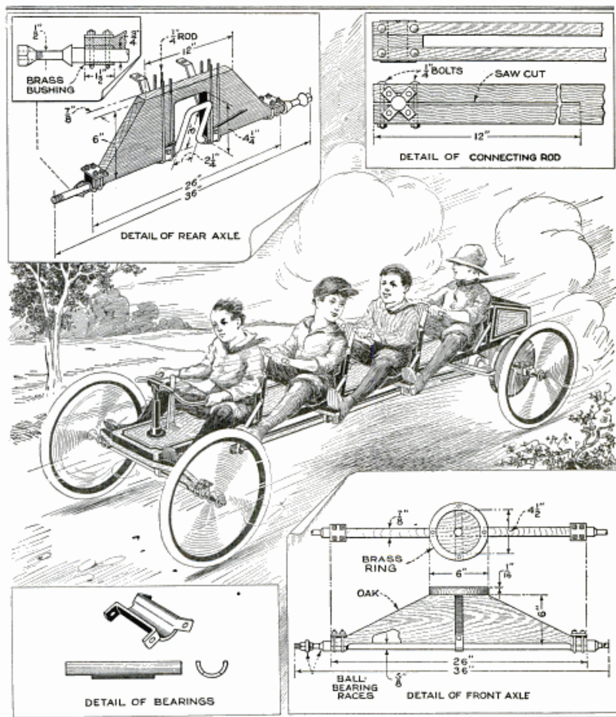
Full Details of Front and Rear Axles of Hand Car, Construction of Connecting Rod, Method of Making Bearings, and Perspective View of Car in Action
