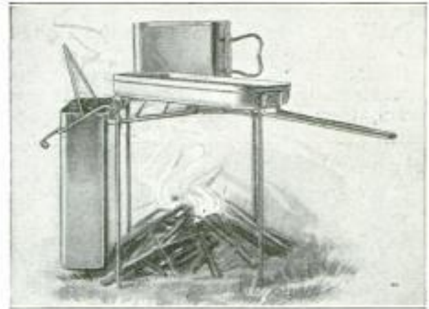
Mess Kit That Fits in Pocket, Containing Frying Pan, Kettle, Cup, Pail, Grid, and Broiler
