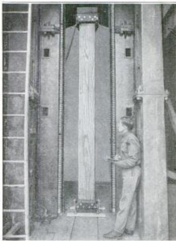
Giant Testing Machine, That Exerts Great Pressure, Determines Strength of Heavy Structural Beams
