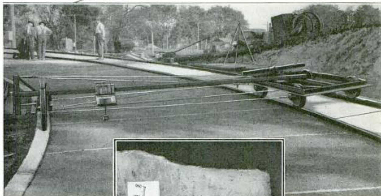
Apparatus for Testing Road Pavements of Various Materials
