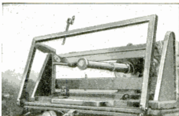
An Additional Clamp on a Cylinder-Grinding Machine to Prevent Vibration
