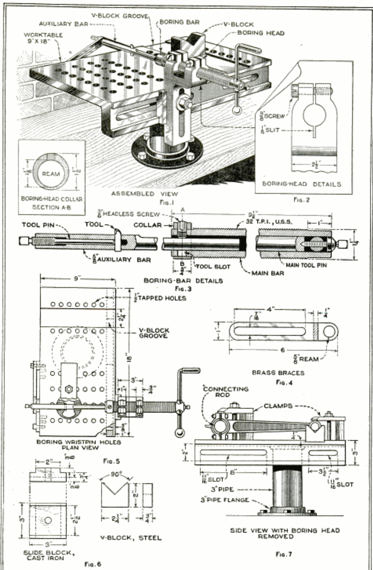
Figure 1 Shows the Fixture Completely Assembled; Figure 2, Details of the Boring Head; Figure 3, Main and Auxiliary Boring Bars; Figure 4, Braces for Auxiliary Bar; Figure 5, Set-Up for Boring Wristpin Holes; Figure 6, Dimensions of Blocks, and Fig. 7, Method of Reboring Connecting Rods
