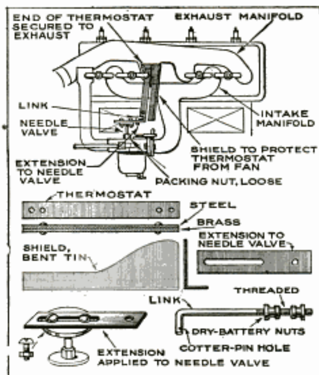
An Automatically Controlled Carburetor Needle Valve That Opens and Closes as the Engine Heats or Cools
