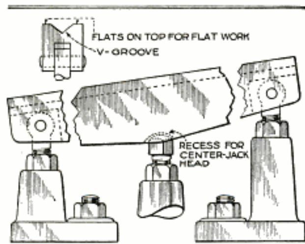
A Steady Rest on a Milling Machine That has been Found to Be of Considerable Usefulness for Tapered Work
