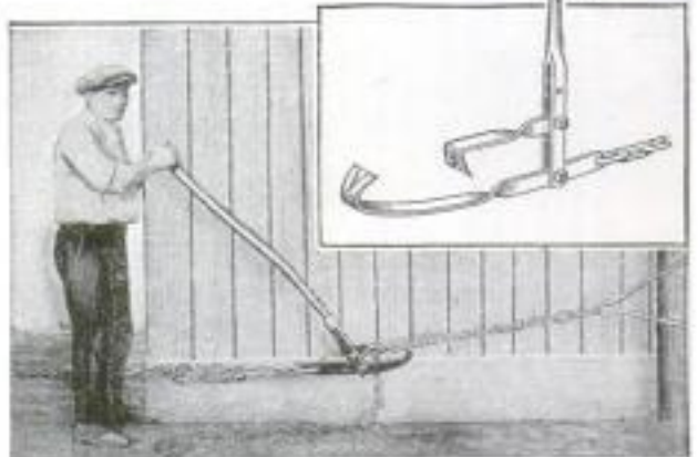
Wire Stretcher Operating with a Chain: Insert, Close-Up of the Claw Arms
