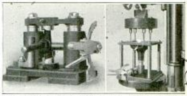
Left, Bushing Type of Jig, with Work in Place; Right, Plate Type on Drill-Press Table
