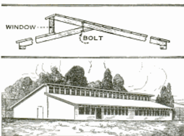
A Semimonitor Laying House with a Simple Rafter Construction Having No Cross Braces
