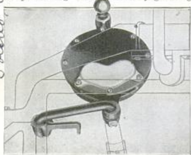
Steering Device for Small Cars That Eliminates Shocks and Operates in a Bath of Oil
