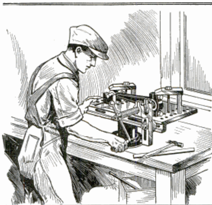
Reboring a Connecting-Rod Big End with a Portable Hand Fixture: Note How the Rod is Clamped
