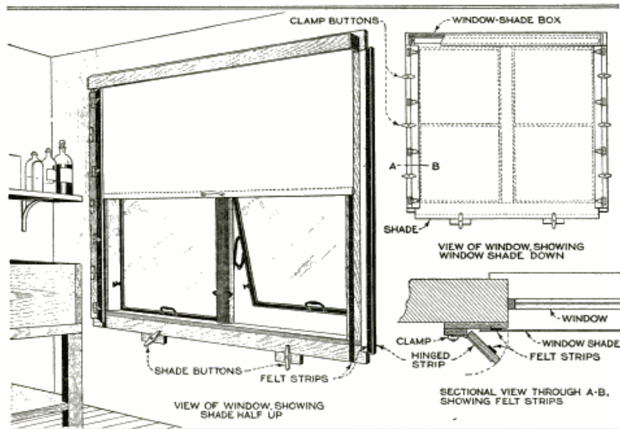
Method of Making the Dark-Room Window Light-Proof of Interest Not Only to the Professional, but Also, Because of Its Simplicity, to the Amateur Photographer
