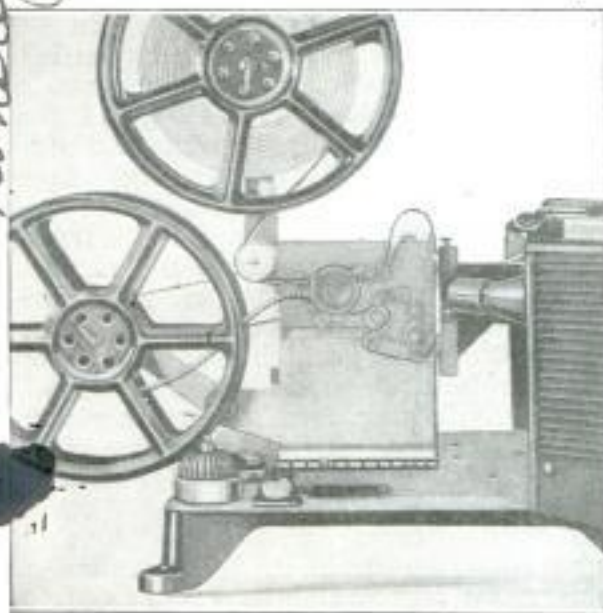
Portable Motion-Picture Machine That Uses Paper Instead of the Usual Celluloid Films
