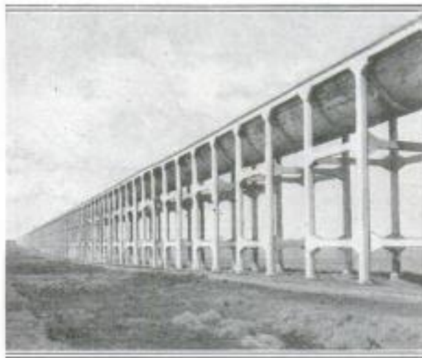
Huge Aqueduct of Irrigation Project, Supported by Concrete Trestle across Surface of Two-Mile Wide Valley
