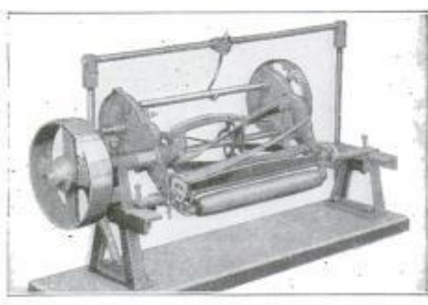
Machine for Sharpening the Blades of a Lawn Mower without Removing Them from Wheels
