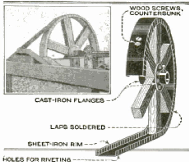
Large Pulleys That Are Light but Rigid can Readily be Made in the Out-of-the-Way Workshop
