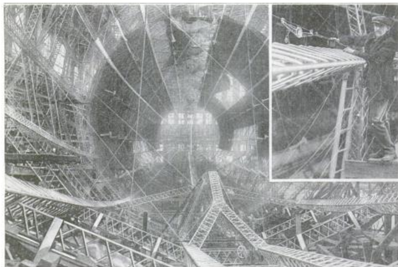
Naval Dirigible being Given Finishing Touches in Preparation for Its First Flight, While Guide Wires are Tensioned to Safeguard Lives of Crew
