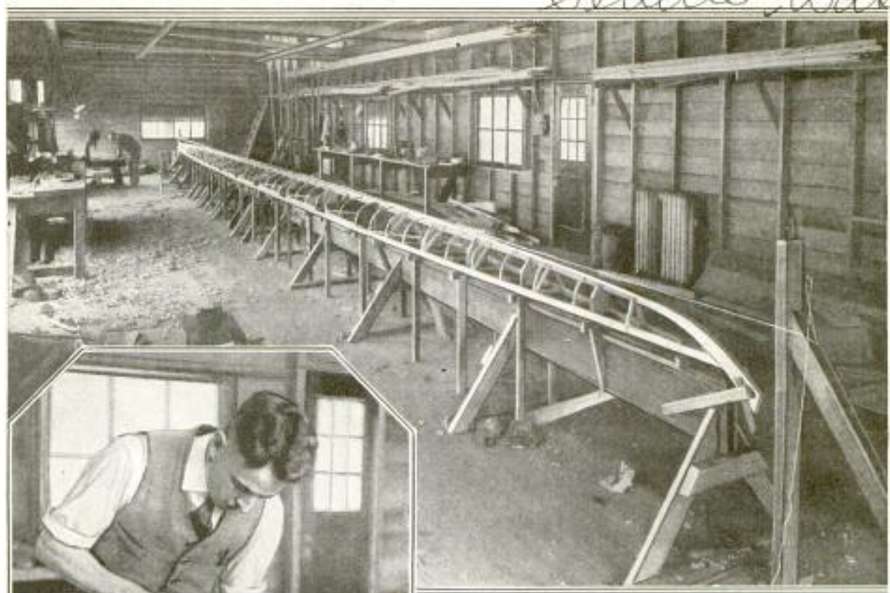
Above: One of the New Racing Shells of the University of Washington in the Course of Construction. The Framing is Made of Spruce and the Planking of Port Orford Cedar. In Order to Meet the Requirements of the Western Oarsmen, the Shell is Designed with a Decided Bow Lift. Left: Close-Up, Showing the Joining of the Keel and Ribs
