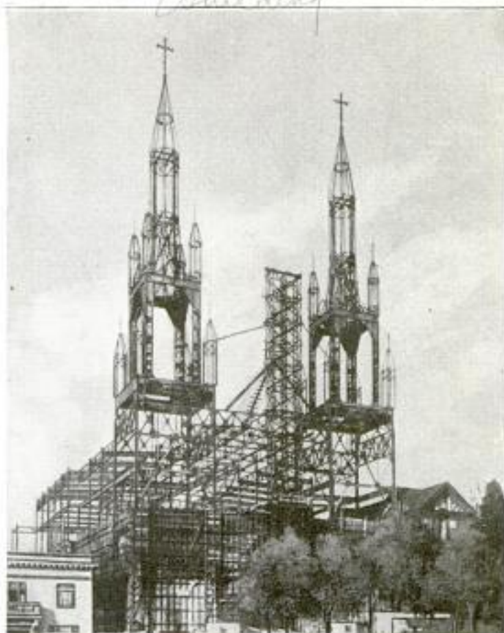
Frame of Church in Construction, Showing Steel Skeleton Far in Advance of Concrete Walls: The Beauty of the Completed Structure is Suggested Even in This Unfinished State
