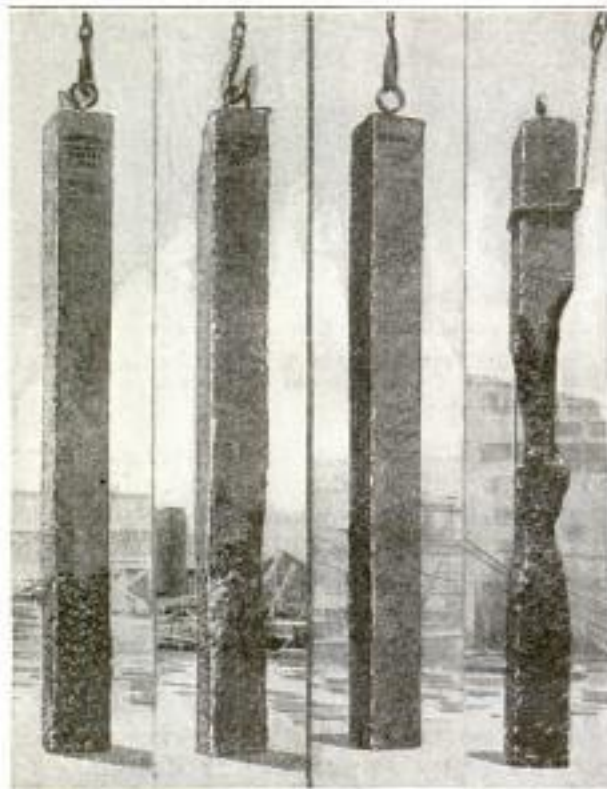
Left: Concrete Piles of a Rich and Lean Mix after Four Years in Sea Water. Right: Same Two Piles after 12 Years' Immersion
