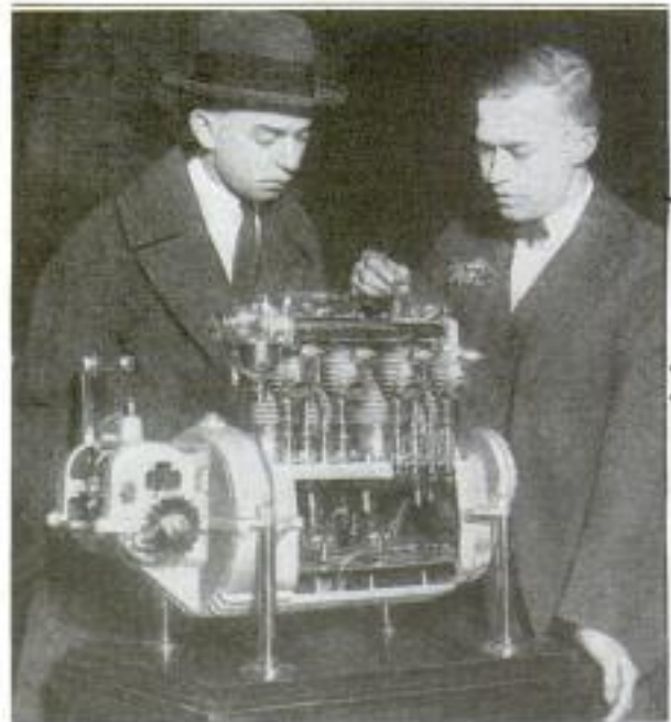
This Four-Cylinder Aluminum Motorcycle Engine Was One of the Chief Attractions at a Recent New York Exhibit Because of Its Light Weight
