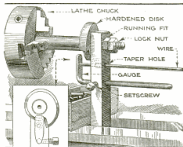
An Easily Made Wire-Cutting Fixture Arranged on a Lathe: It will Cut Various Sizes of Pins Accurately to Any Length
