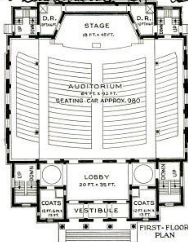
Plan of the Main Auditorium and Stage of the New Radio Church, to be Finished in June: The Seating Capacity will Be 980. There will Be No Pulpit
