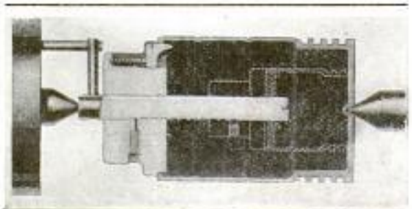
Arbor That Permits Pistons of Various Lengths and Diameters to be Finished without Changing the Set-Up: It Is the Notches along One Side That Makes This Possible
