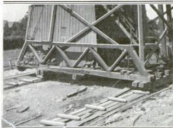
Base of the Derrick, and Roller Track on Which It Traveled in Excavating and Filling for the Bowl of the Stadium: As the Middle was Excavated and the Sides Filled, the Derrick was Moved
