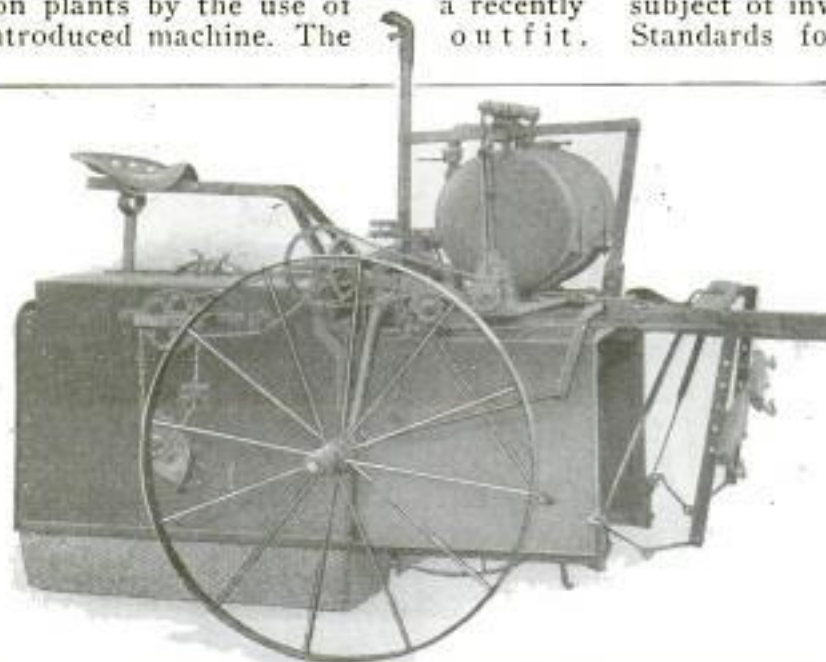
Machine for Spraying Cotton Plants with Poison, Which may Be in Either Liquid or Powder Form: The Liquid is Forced by Compressed Air through Nozzles, and the Powder Blown onto the Damp Plants
