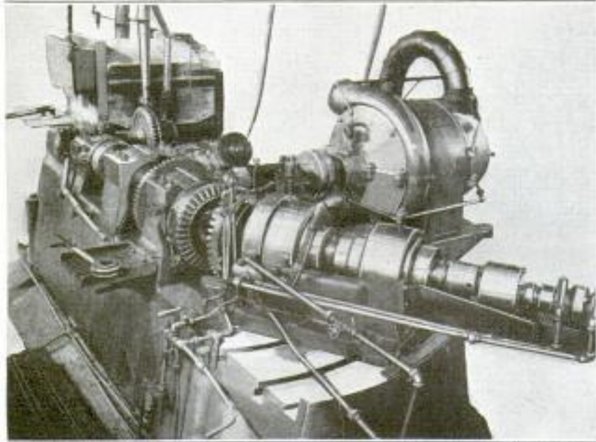
A Machine for Producing Accurately Formed Gears by Hot Rolling: Power is Transmitted through the Two Bevel Gears at the Ends of the Spindle Shafts. The Plastic Gear Blank and the Forming Gear are Rigidly Mounted between Them, in Forced Contact with Each Other, and the Former is Kneaded into Shape
