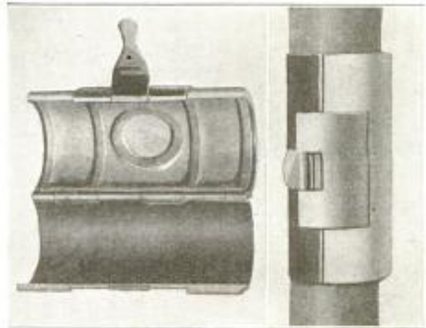
Left: Showing How One-Half of the Clamp is Lined with Sheet Rubber Having Raised Edges. Right: Locked in Position, around a Defective Portion of Hose
