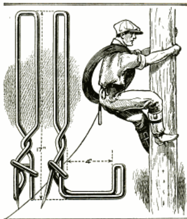
Climbing Irons Made of Four-Foot Lengths of \frac{1}{4} -Inch Steel Rod, That will be Found Very Serviceable by Linemen
