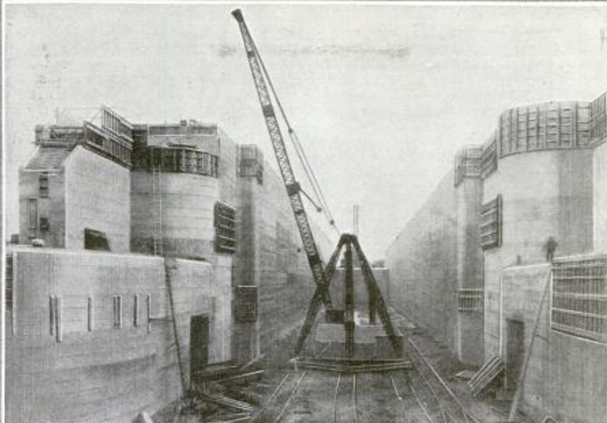
Above: A View during Construction of One of the Locks of the New Welland Ship Canal That the Canadian Government is Building between Lake Ontario and Lake Erie. The Foundations are Carried Down to Bedrock and the Present Excavation Provides for Boats of a Draft of 25 Feet, Which will Later be Deepened to 30 Feet. Below: One of the Large Steel Forms Used in Building the Concrete Work for the Locks
