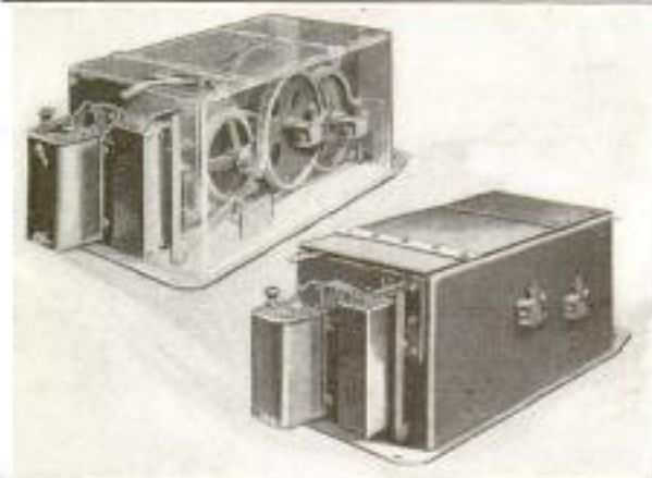
Above, Phantom View of the Portable Hoisting Unit, Shown Complete Below: Both Driving Gears and Pinions are Machine-Cut from Electric Steel
