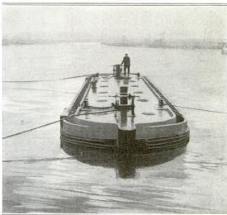
Head-On View of the Concrete Floating Caisson Which, When Swung into Place at the Entrance to the Dock, will Serve to Stop the Spread by Water of an Oil Fire
