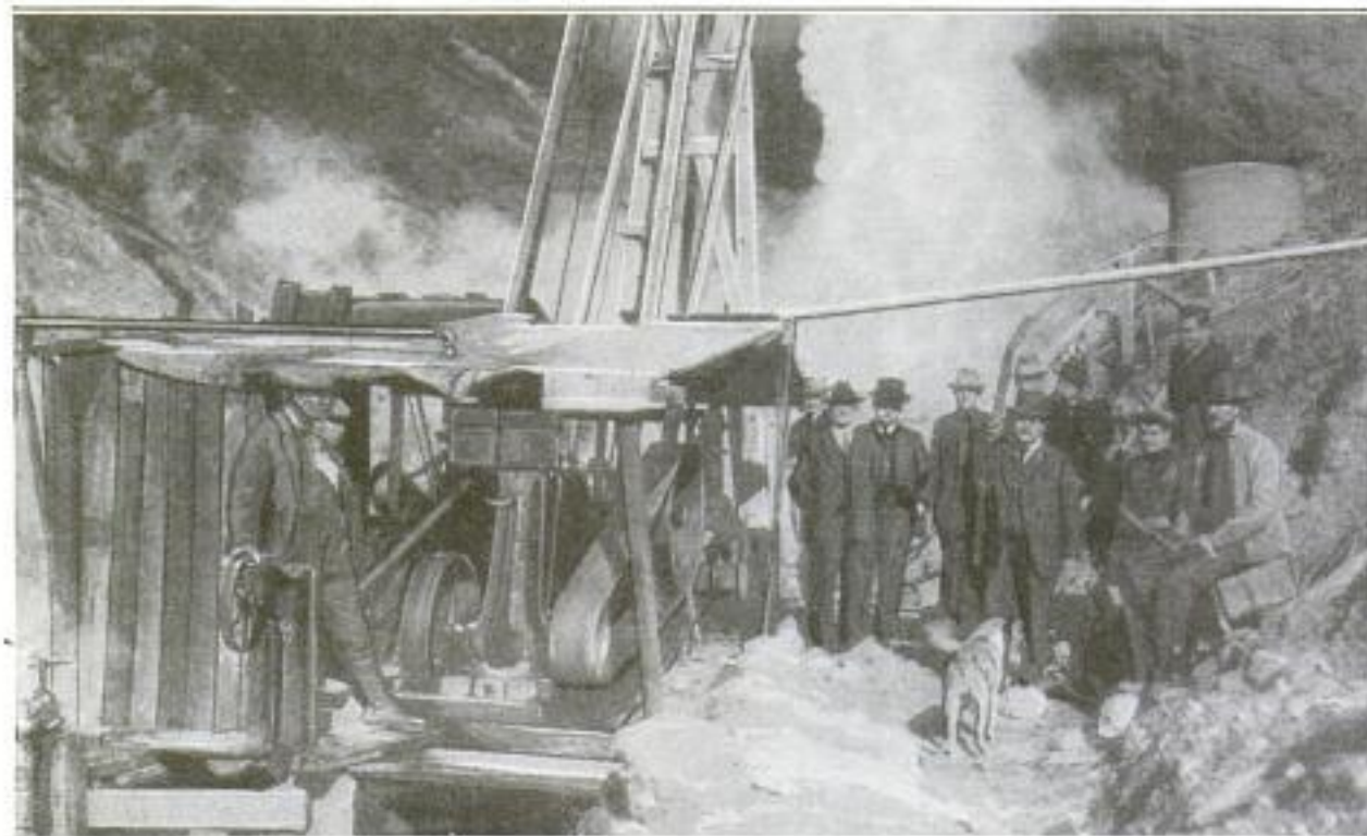
The First Engine to be Operated by Steam Direct from a Geyser in the United States: It is Installed at The Geysers, Sonoma County, California, and Takes Steam from One Geyser There, Developing 150 Horsepower
