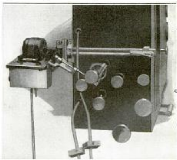
A Continuous Arc-Feed Attachment for Projecting Machines Which Relieves the Operator Entirely of Hand Feeding
