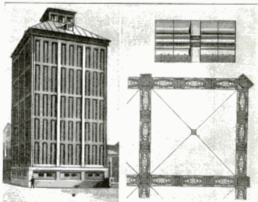
A Concrete Silo of Hollow-Sidewall Construction: Standardized Arch Blocks were Used, Avoiding Extensive Shuttering, and Cutting Down Costs
