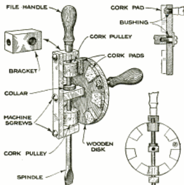
A Valve-Grinding Tool for Internal-Combustion Engines That Imparts the Proper Back-and-Forth Rotation to the Valves While Turning the Handwheel in But One Direction
