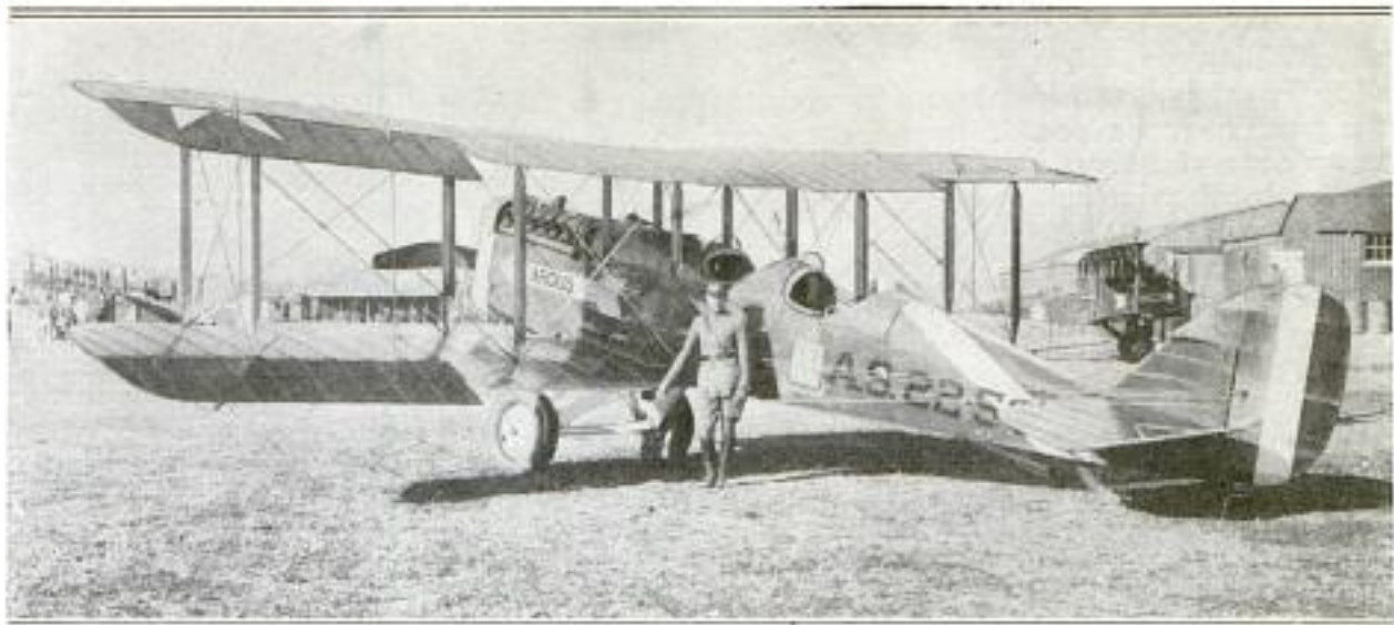
The DeHaviland Airplane Which Lieutenant Nowland Piloted in Making an Aerial Survey of the Salt Creek-Tea Pot Dome Oil Fields near Casper, Wyoming: A Film-Type Camera was Suspended Vertically in the Rear Cockpit of the Machine
