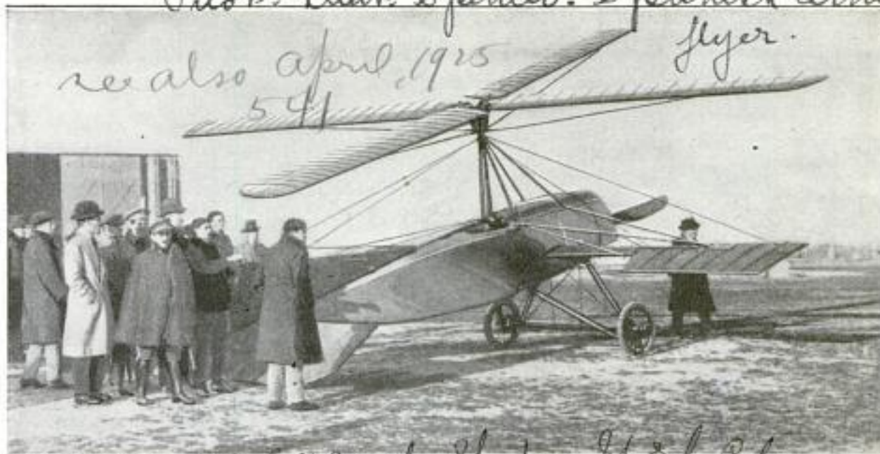
Spanish Helicopter Which is Reported to have Recently Ascended to a Height of 81 Feet and to have Successfully Carried Out Several Horizontal Flights: The Machine is Supported by a Four-Bladed Propeller and is Motored by an 80-Horsepower Engine
