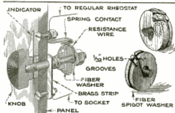
A Homemade "Vernier" Rheostat That can be Made by Any Amateur: Its Maximum Resistance Equals That of a Single Turn of Wire of the Regular Rheostat
