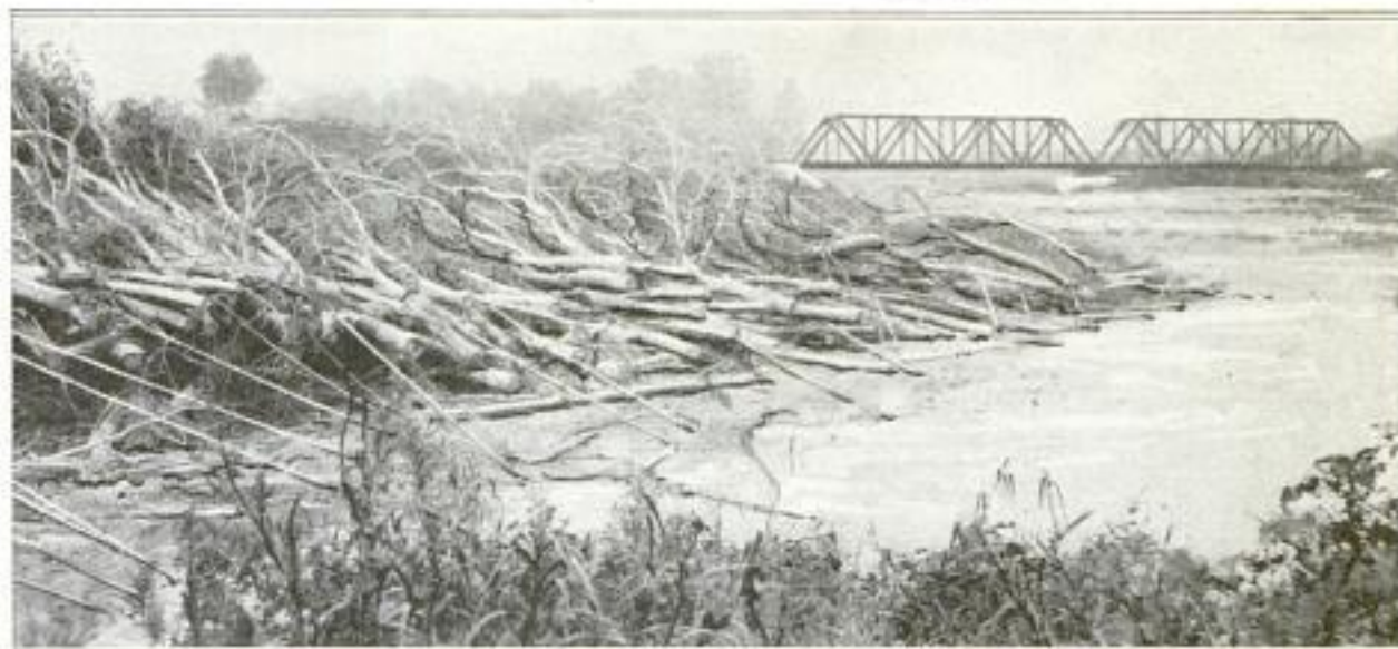
One of the "Retards" Used to Change the Course of the White River in Indiana: Note How the Brush is Held in Place by the Cables Leading to Submerged Piles. The Railroad Bridge can be Seen in the Background
