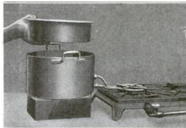
European Gas Saver Cooks with Double Boiler at Left, While Food is Cooking over the Burner
