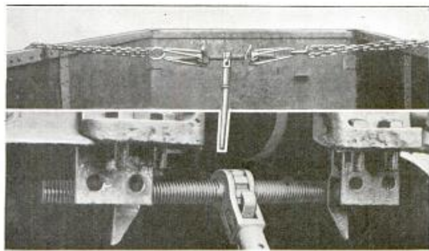
A 10-Ton-Capacity Push-and-Pull Jack, Combining Ruggedness and Simplicity of Construction, for Straightening Center Sills on the Draft-Gear End of Railroad Cars: Flat Lugs are Provided for Pushing, Hooks for Pulling, and Extra Hooks on the Sides for Pulling with Chains
