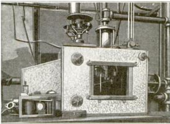
Close-Up of Carburetor-Testing Apparatus Which has been Worked Out to Give Results Quickly and under Conditions Actually Existing on an Engine
