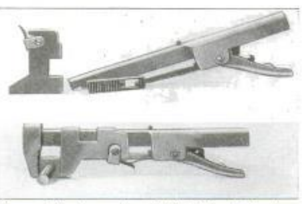
Above: The Lower Jaw of This Wrench has been Removed and Set Up on Its Face, for Use as a Jack. Below: The Assembled Wrench, Showing the Trigger Release and the Ratchet Handle
