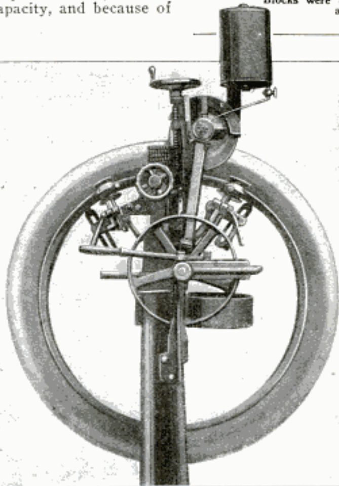
A Tire Skiver, or Slicer, Set Up for Operation: The Machine can be Adjusted to Skive All Sizes and Styles of Tires, Leaving a Feather-Edge Which Facilitates Insertion into Another Tire of the Same Diameter
