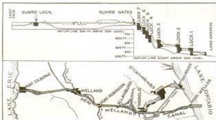
Above: At the Top of the Diagram is Given a Profile of the New Welland Canal, While below It Is a Map Showing the Course of the Canal When Completed. Below: View Showing Completed Section of Center Wall of Lock Number Six
