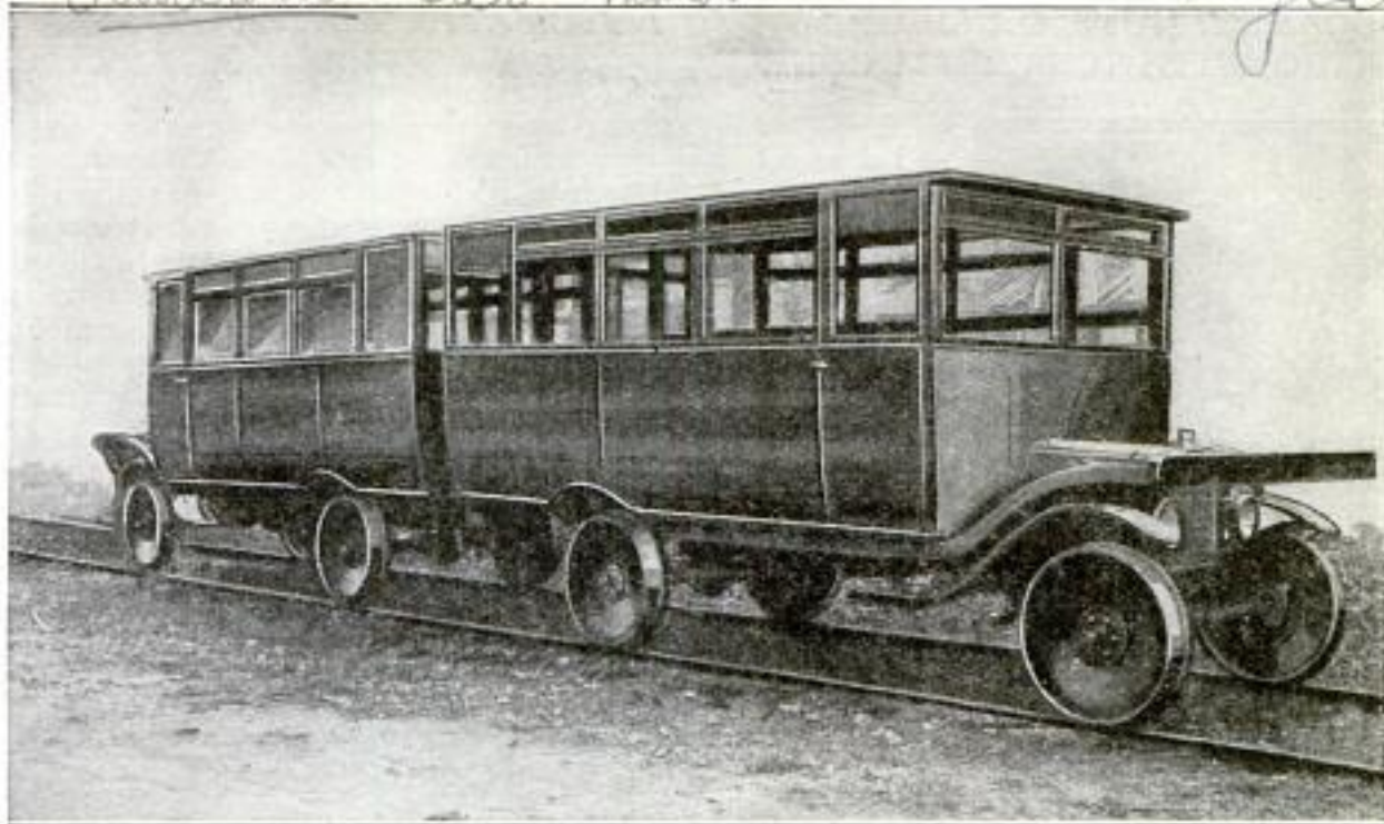
Gasoline Rail Cars Operated in Tandem by Placing Back to Back Two Automobile Chassis, on Which are Fitted Passenger-Carrying Bodies: A Center Buffer and Draw Pin Combined is Used, and a Sliding Door is Provided at the Rear of Each Body
