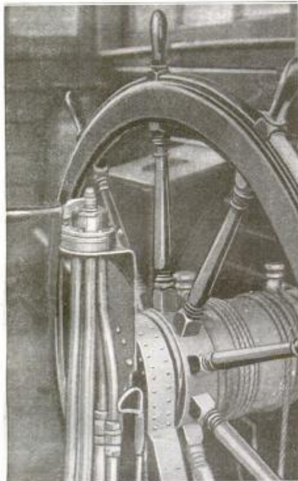
The Controller for Compressed-Air Device, Which Actuates the Steering Gear and Moves the Rudder, is Shown Here Immediately behind the Wheel
