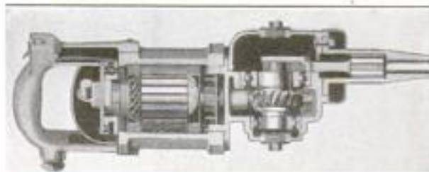
Sectional View of Riveting Hammer and Concrete Drill, Showing Interiors of Motor and Driving Mechanism, and Ball-Bearing Journals
