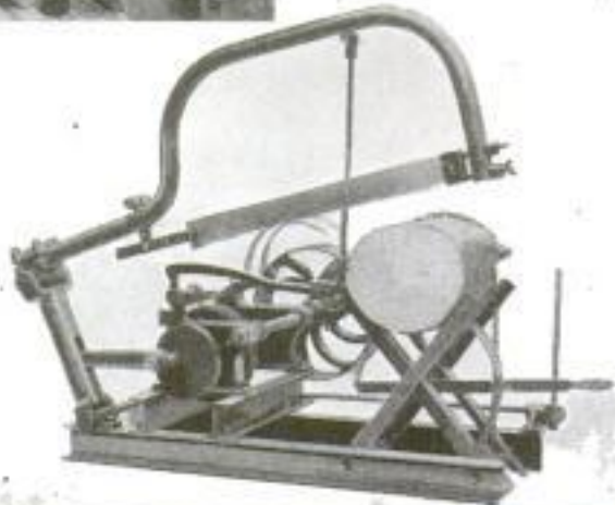
Above: The Bucksaw and Engine at Work Sawing a Log. Both Mounted on a Truck. Left: Engine Alone Dismounted. Right: Saw and Buck for Holding Timbers. Note the Locking Chain and Lever at the Right-Hand End.
