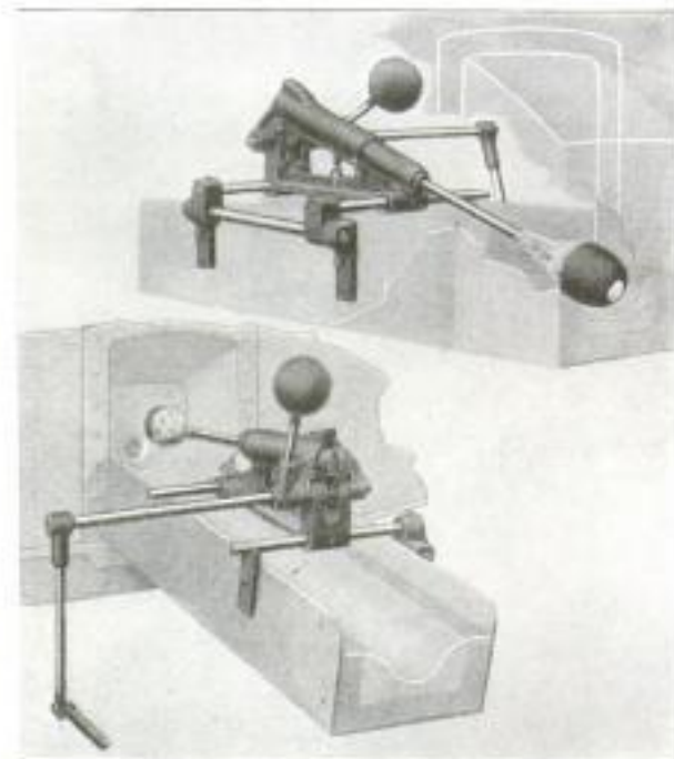
Above: Cupola Tapper and Stopper Device in the Position When the Flow is Stopped. Below: Position When the Flow is Tapped
