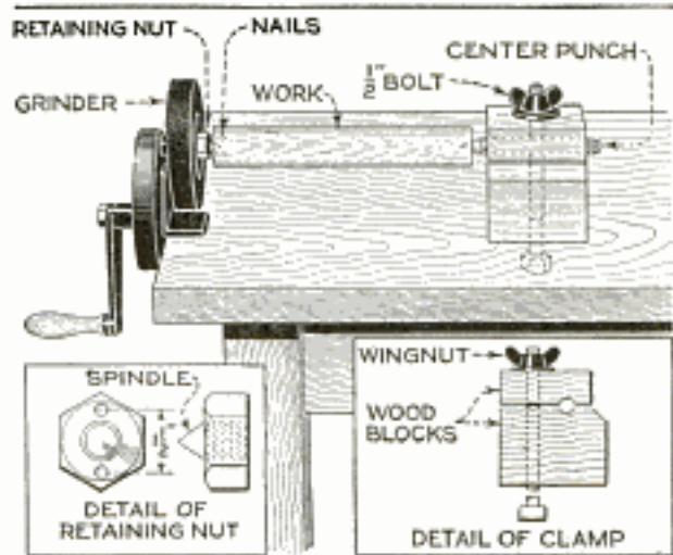
A Hastily Improvised Lathe That Accomplishes the Work of Turning Wood with Surprising Speed and Ease, Considering Its Crude Construction
