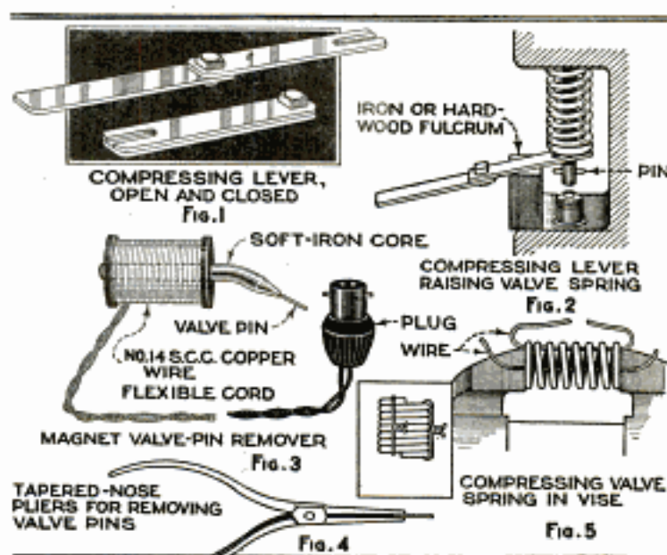
Figure 1: Tool for Compressing Valve Springs. Figure 2: Method of Using. Figure 3: Homemade Electromagnet Used to Extract Pins. Figure 4: Tapered-Nose Pliers for Extracting Pins. Figure 5: Method of Holding Springs Compressed
