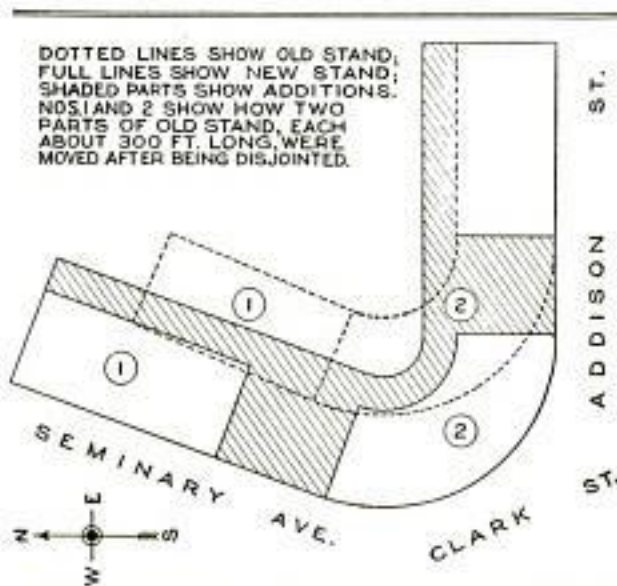
Diagram Showing the Relative Size, Shape, and Location of the Old and New Stands at the Chicago National League Ball Park
