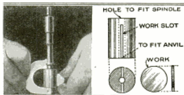
Simple Attachment for Measuring Disks with a Micrometer Caliper That Insures Each Disk being Held Square and Central between Spindle and Anvil
