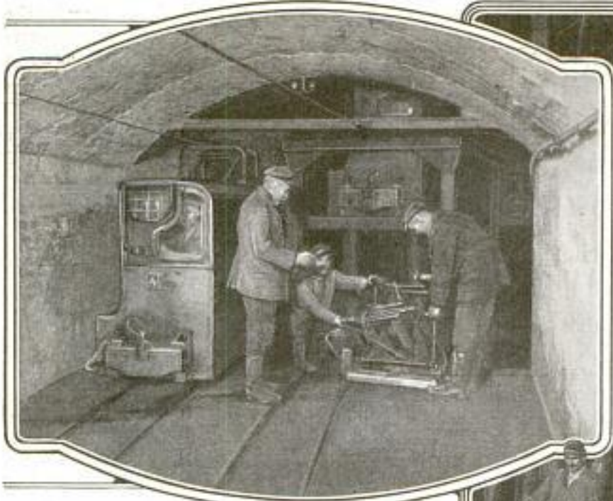
Above: A Workshop 400 Feet Underground Where Mechanics Repair Electric Locomotives Used for Hauling Trains of Small Cars in the German Coal Mines. Right: Miners at Work with Compressed-Air Machines Drilling Holes in the Coal
