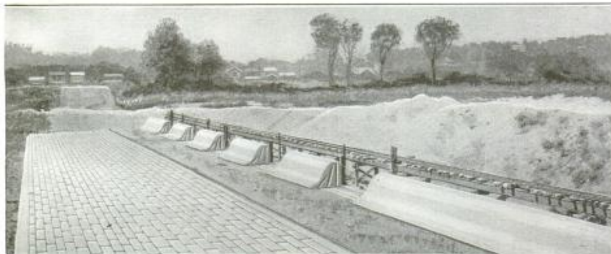
First Section of the Hamilton, Ohio, Dam during Construction: Note the Gaps Left in This Section to Carry the Flow of the River While the Remaining Portion was being Built; Also the Flexible Concrete Apron along the Downstream Apron
