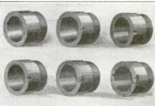
Showing the Successive Stages in Preparing a Bit for Setting with Diamonds, Beginning at the Upper Left of This View with a Blank Bit
