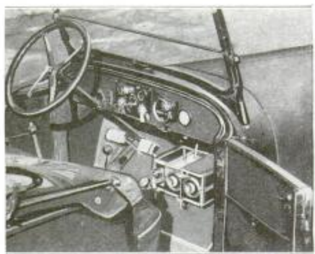
An Automatic Recorder of Road Conditions: A Clutch is Provided So That the Instrument can be Operated, or Disengaged at Will
