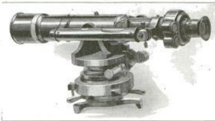
A New Surveyor's Level of Simplified Construction: Instead of Centering between Hair Lines on the Level Tube, One End of the Bubble is Brought Up to a Pointed Indicator. The Bubble is Visible from the Eyepiece
