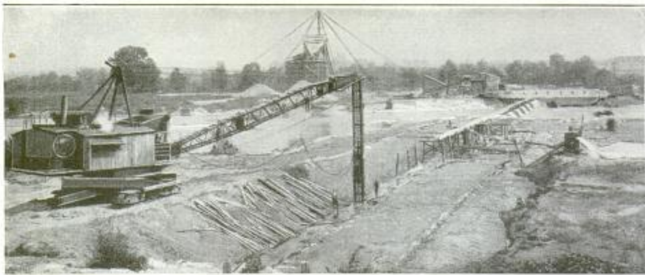
Dragline Excavator Operating a Pile Driver during Construction of a Dam across the Miami River at Hamilton, Ohio: In the Background Appears the Gravel Plant That was Built to Handle Gravel Accumulating in the Artificial Settling Basin Created by the Dam
