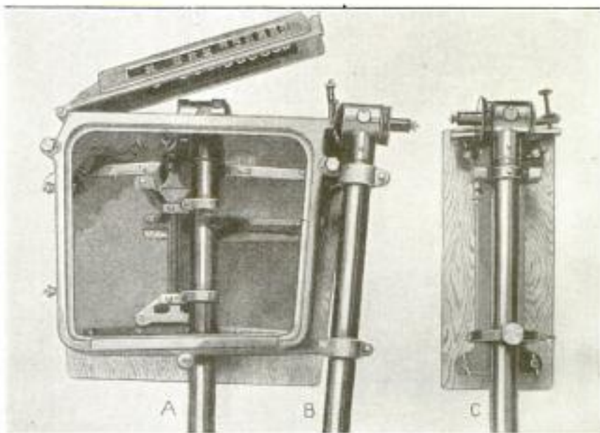
Apparatus for Night Indication of Airplane's Flying Height: Each of the Three Tubes Has a Small Incandescent Lamp at the Upper End, Which Throws an Illuminated Image upon the Ground. B and C Are Stationary, While A Is Movable and Projects a Number from the Scale Directly above It
