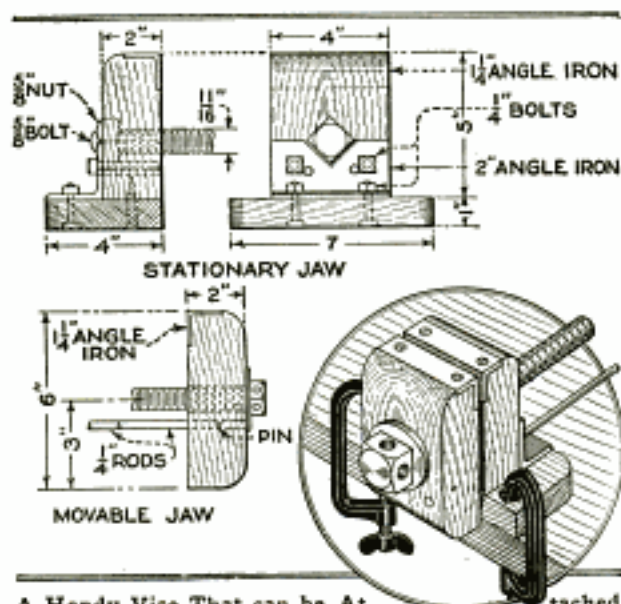
A Handy Vise That can be Attached to Any Table or Bench with Ordinary C-Clamps: It is Made of Hardwood and the Jaws are Protected with Angle Iron
