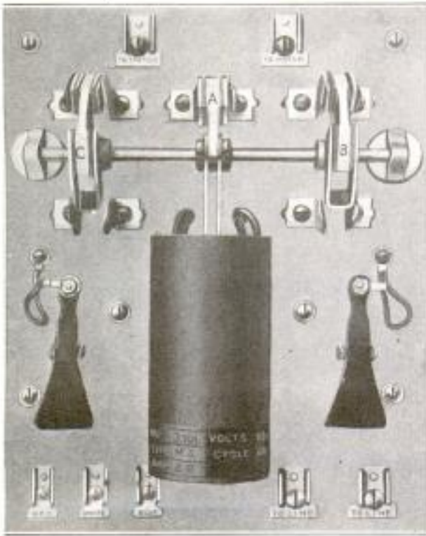
A Heat-Governed Electric Switch: A Is the Main-Line Switch to Apparatus to be Controlled; B Is the Selector Switch, and C Controls the Two Contactors on Either Side of the Containing Cylinder
