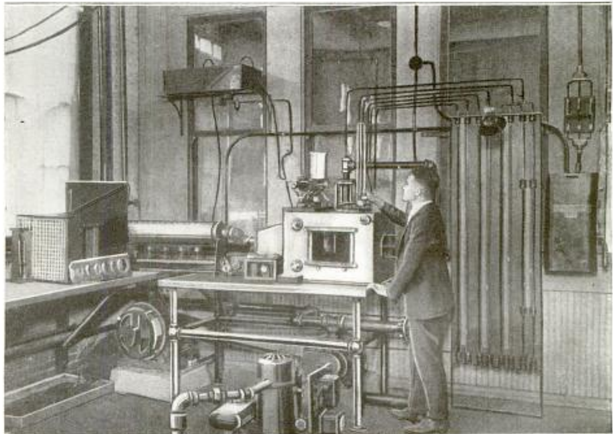
General View of Testing Apparatus Built with the Idea of Reducing the Gasoline Consumption of Automobiles, by Furnishing Carburetor Designers with Information as to the Fuel-Air Ratios of an Engine
