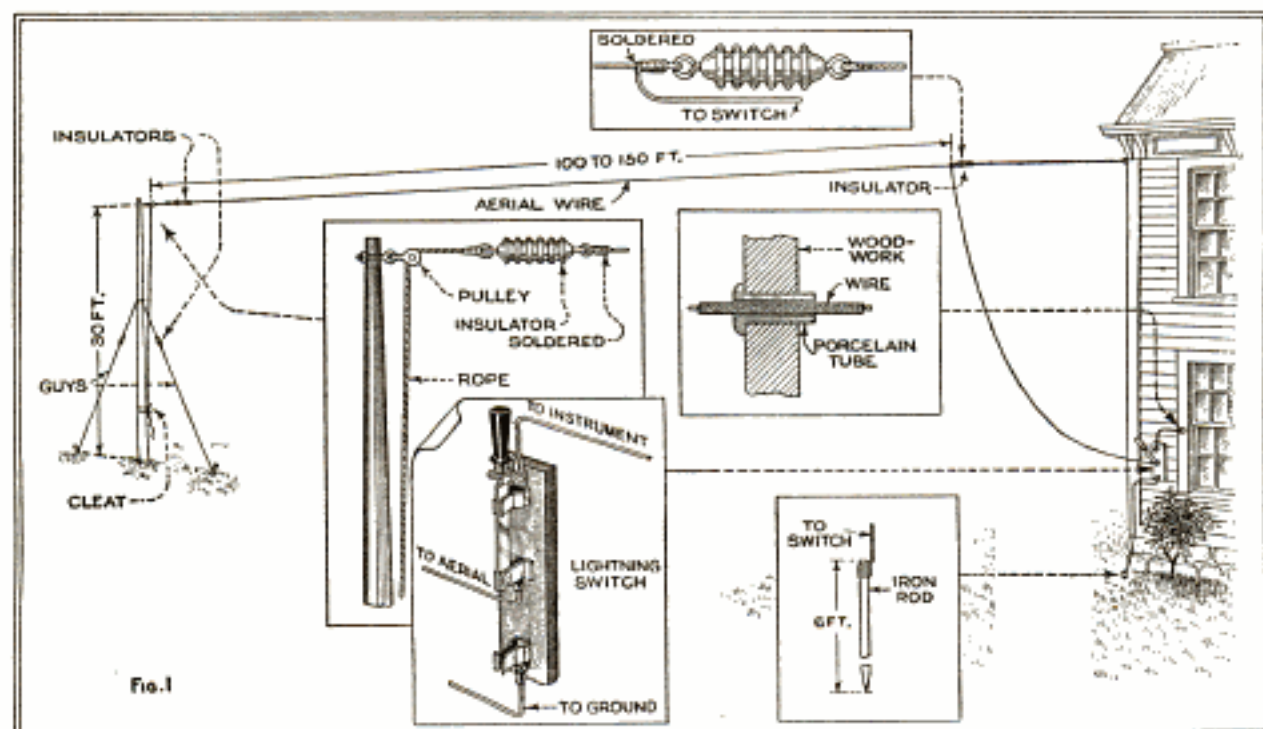
The Single-Wire Aerial Is the Most Commonly Used, and has been Found to Be Universally Successful. Its Length Is from 100 to 150 Feet, and It is Suspended at a Height of 30 to 60 Feet above the Ground. The Illustration Shows All the Details of Installation and the Necessary Connections
