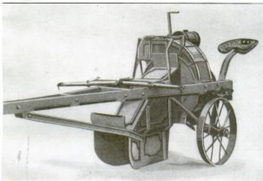
The Machine Which Uses the Vacuum Principle for Sucking Boll Weevils and Their Eggs from Cotton Plants: It Is Adjustable for Height, to Facilitate Operations on Rolling Ground
