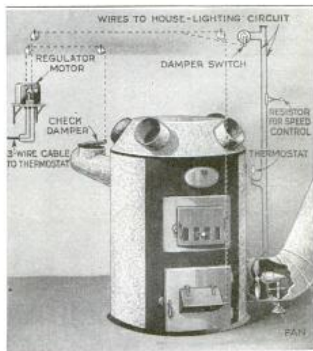
Furnace, Showing Installation of Devices to Promote Air Circulation and Fuel Economy: Upper Left, Motor Regulator and Check-Damper Control; Right, Fan in Air Inlet, and Thermostat.
