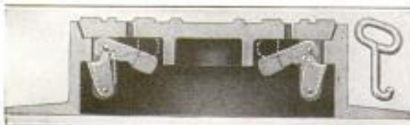
Manhole Cover Which Locks Automatically: At Right is One of the Keys Required to Unlock It
