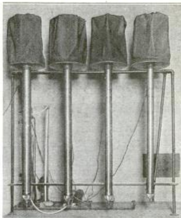
With This Apparatus for Analyzing the Fineness to Which Cement is Ground, Particles as Small as .00035 of an Inch can be Separated
