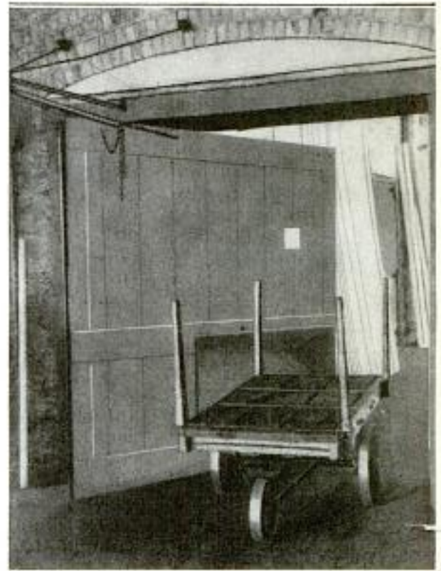
Double-Swing Door in a Factory, Opened by Simply Pushing the Trucks against It: A Spring Attachment Makes It Self-Closing
