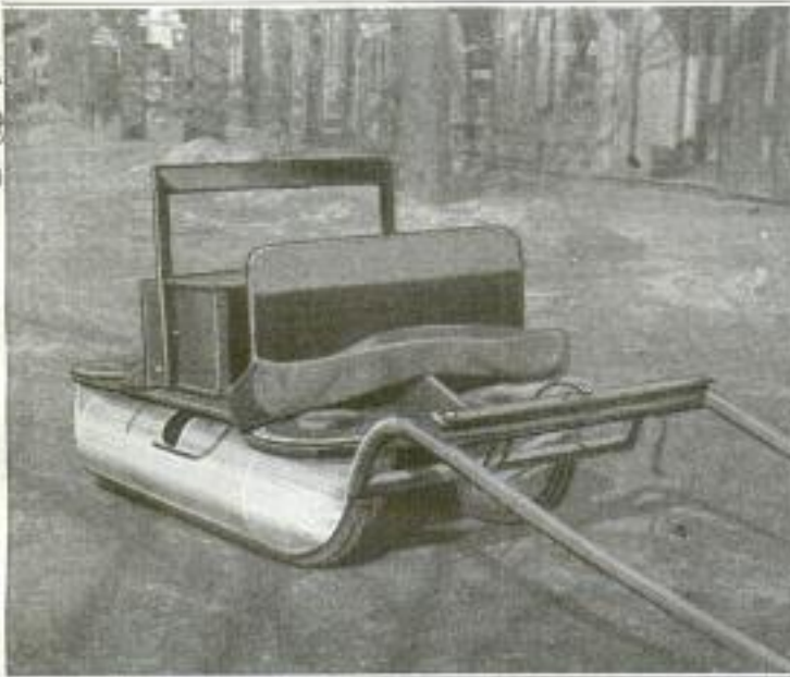
This Sled, Built with Cylindrical Runners, That will Hold Luggage, Glides over Ice, Snow, or Water
