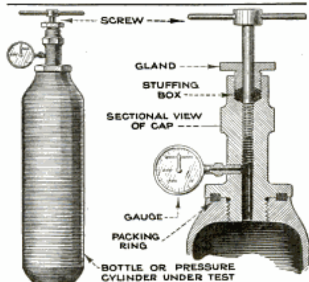
A Simple and Effective Method of Testing Pressure Vessels: Any Leakage That Takes Place While Testing can be Detected Immediately and Stopped
