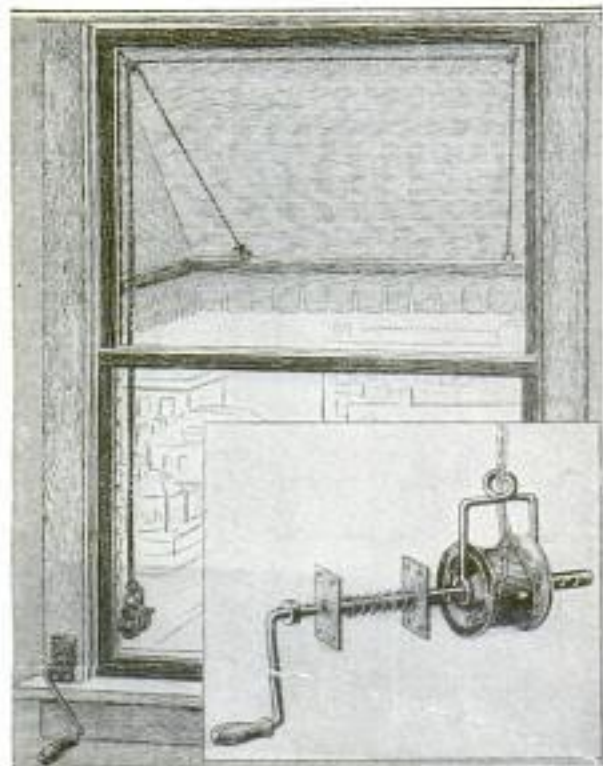
Device for Raising and Lowering Window Awnings from Inside in Place: The Inset Shows the Construction of the Device in Detail
