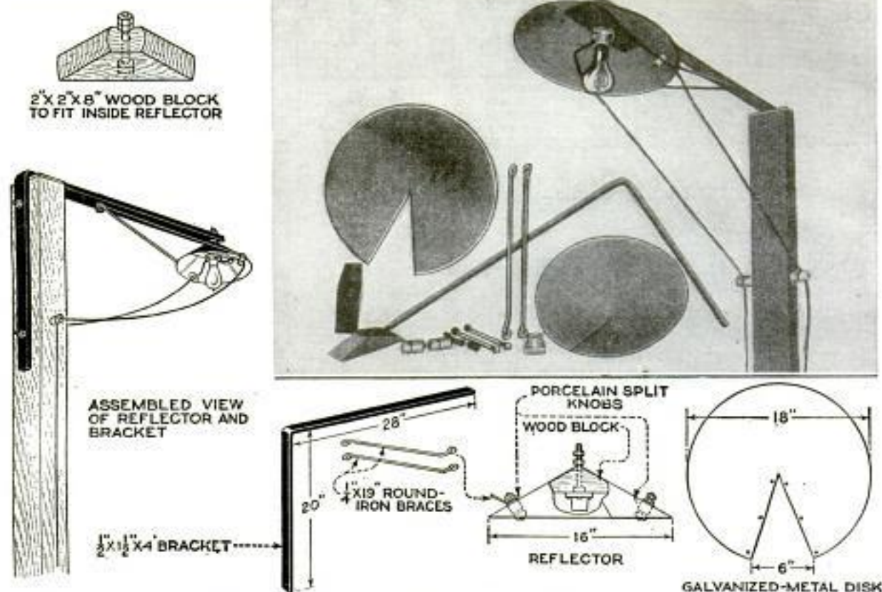
The Photos Show All the Material Necessary to Construct the Yard Light, Together with a Completed Fixture. The Drawings Show Details of the Various Parts Used, and the Method of Assembling Them. The Cost of the Purchased Material for the Fixture Shown Was Only $1.30
