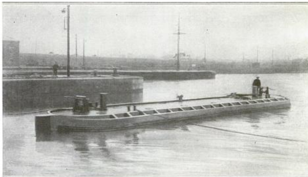
In This View, Note the Projection at the Stem. This, and a Similar One at the Stern, Fit into Two Vertical U-Grooves in the Entrance Piers. The Over-All Length of the Vessel Is Slightly More than 82 Feet, the Beam 12 Feet, and the Depth from Deck to Keel About 10 Feet
