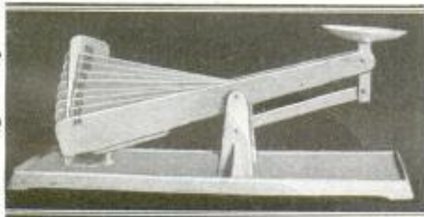
With This Grading Scale, the Lowest Number Visible on the Blades to the Left Indicates the Weight per Dozen of Any Egg Which is Placed in the Cup
