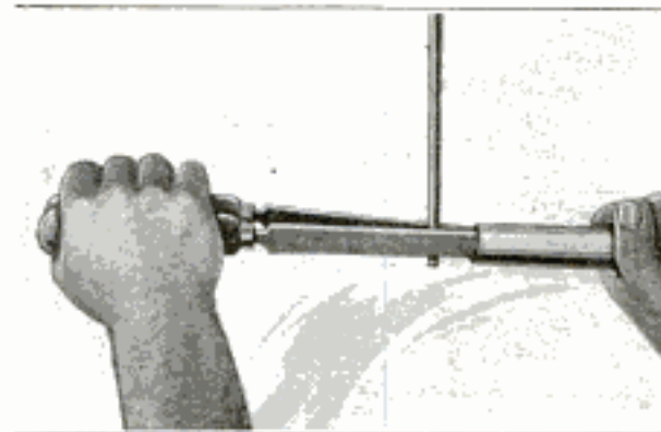
A Handy Gripping Tool, Improvised from Two Files and a Length of Pipe, Is an Excellent Substitute for a Pair of Pliers and in Some Cases Is More Suitable
