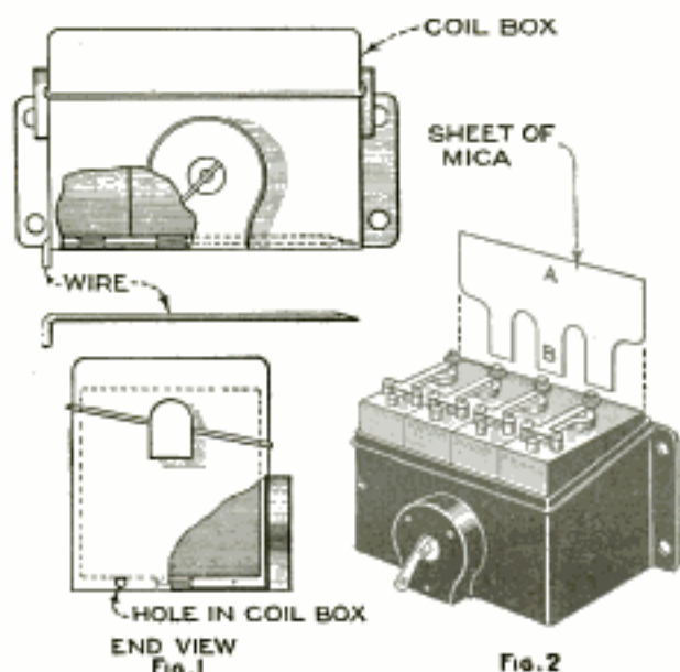
Two Methods for Foiling Automobile Thieves: Figure 1, Wire That Lifts the Coils to Separate the Bottom Contacts; Figure 2, Sheet of Mica That Separates Back Contacts
