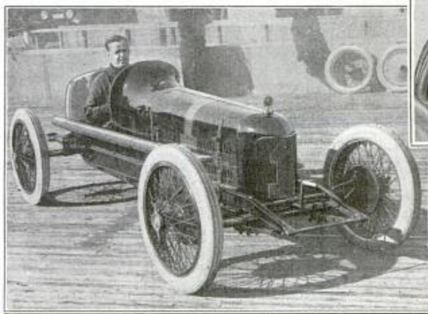
Upper Left: One-Man Racing Car with Hood Raised, Showing Eight-Cylinder Motor. Upper Right: Rear View, Showing the Narrow Streamline Body. Lower Left: Side View of Car Which Is About 400 Pounds Lighter than Other American Racers. Above: Steering Wheel and Instrument Board of New Car
