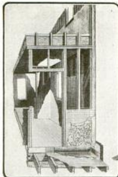
An Exterior View, Showing the Application of the Steel Fabric to Both Exterior and Interior Walls, as Well as to Porch Floors
