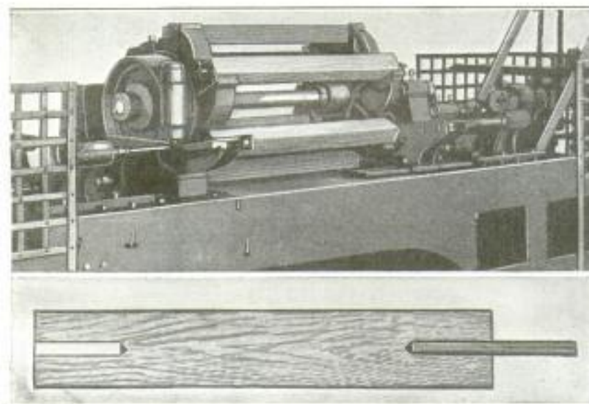
Above: Gudgeon-Drilling and Inserting Machine Which Is Automatic Except for the Placing and Removal of Pieces on the Carrier. Below: Wooden Roller with Holes Drilled and One Gudgeon Inserted
