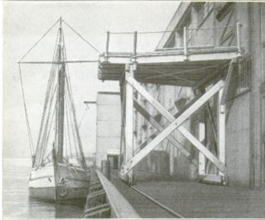
One of the Traveling High-Leg Platforms Adopted by the Port Authorities at Seattle, for Loading from the Second Story of Warehouses into Ships
