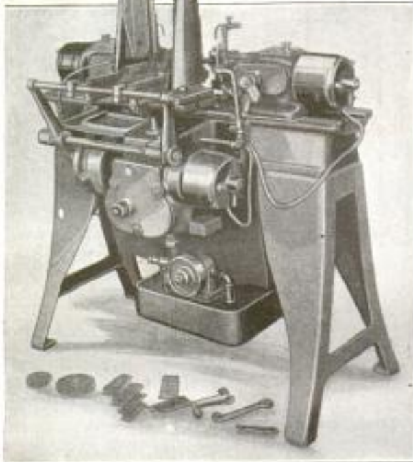
This Machine, Designed for Production Shops, Automatically Centers and Drills Work That is Taken to Other Machines for Various Finishing Operations
