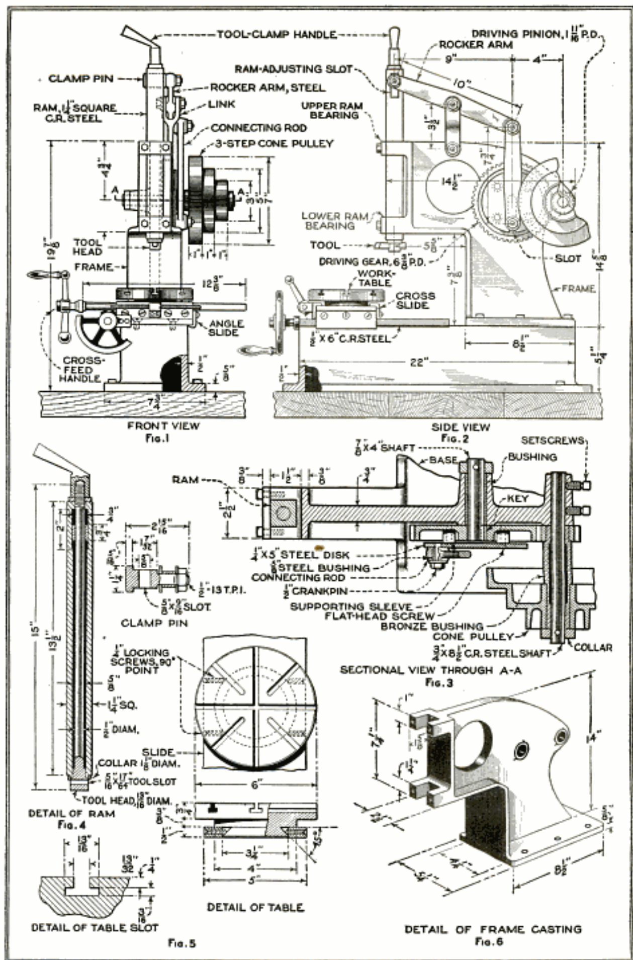
Figure 1, Front Elevation of Completed Machine; Figure 2, Side Elevation; Figure 3, Sectional View, Showing Details of Driving Mechanism; Figure 4, Section of Ram, Detail of Clamp Pin and Tool Head; Figure 5, Plan and Part Section of the Table and Dimensions of Slot; and Figure 6, Perspective View of Frame Casting
