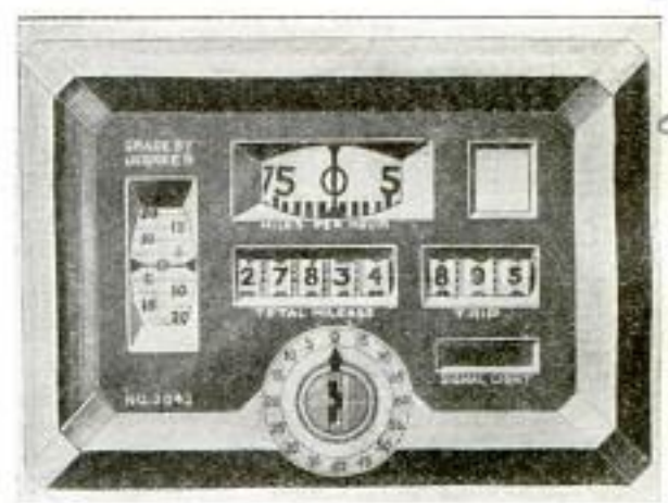
The Signal-Flashing Speed Recorder: Speed Limits may be Quickly Set with a Turn of a Key, Which is Also Used to Lock the Ignition
