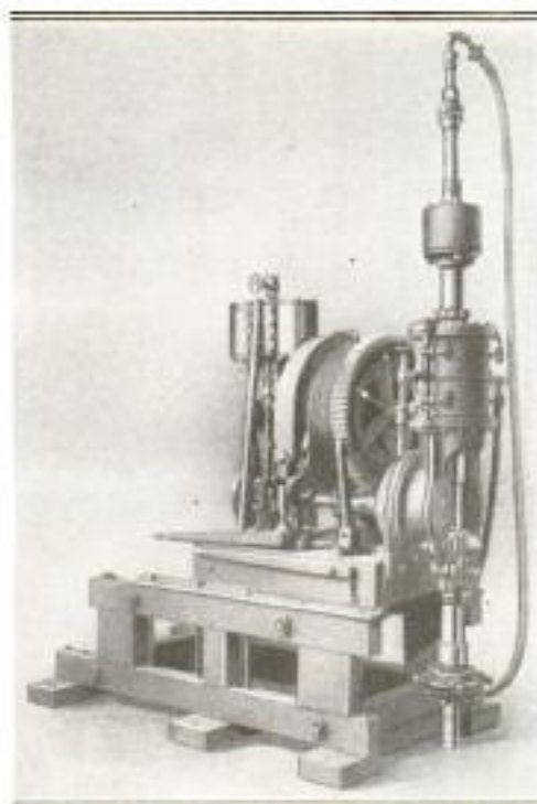
A Diamond Core Drill: Its Use Is the Only Known Method of Securing a Stratified Core of Tough Ore Which Reveals the Formation
