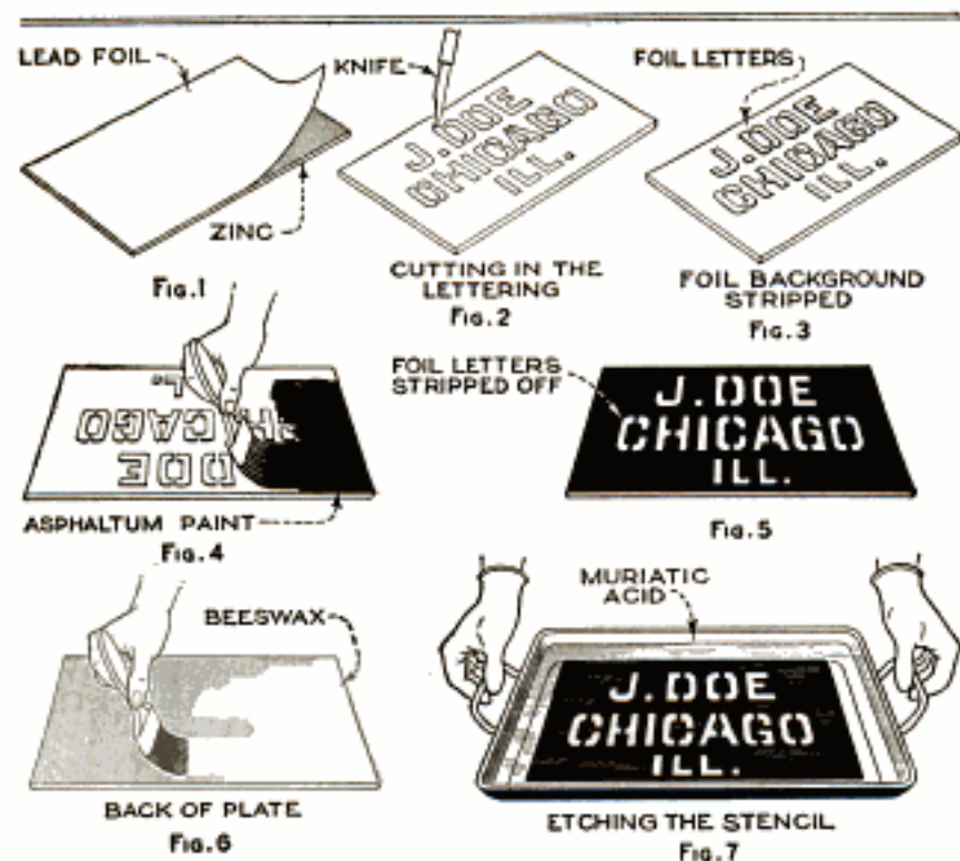
Figure 1, Applying the Lead Foil; Figure 2, Cutting In the Lettering; Figure 3, Plate Ready for Painting; Figure 4, Painting the Plate; Figure 5, Plate with Lettering Stripped; Figure 6, Preparing the Plate for Etching; and Figure 7, Etching the Work
