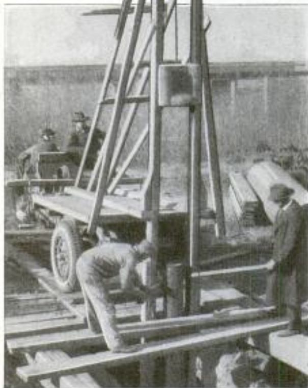
Effective Pile Driver Constructed in Three Hours' Time from Stock Lumber, and Fastened to the Rear of a Contractor's Truck
