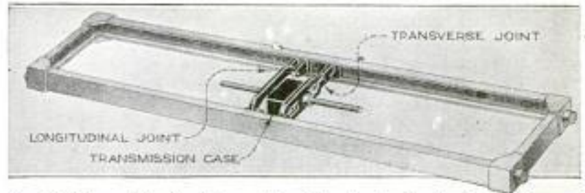
Flexible Support for the Transmission Case in the Center of the Frame of an Extra-Long Motor Truck: The Cross Members Carrying the Transmission Case are Hinged at Each End to Provide Thorough Flexibility
