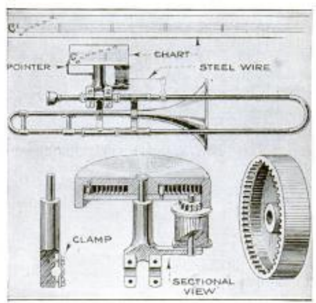
Complete Assembly of the Indicator is Shown and Noted on the View of the Trombone. Below, the Various Parts are Shown Enlarged and Partly in Section
