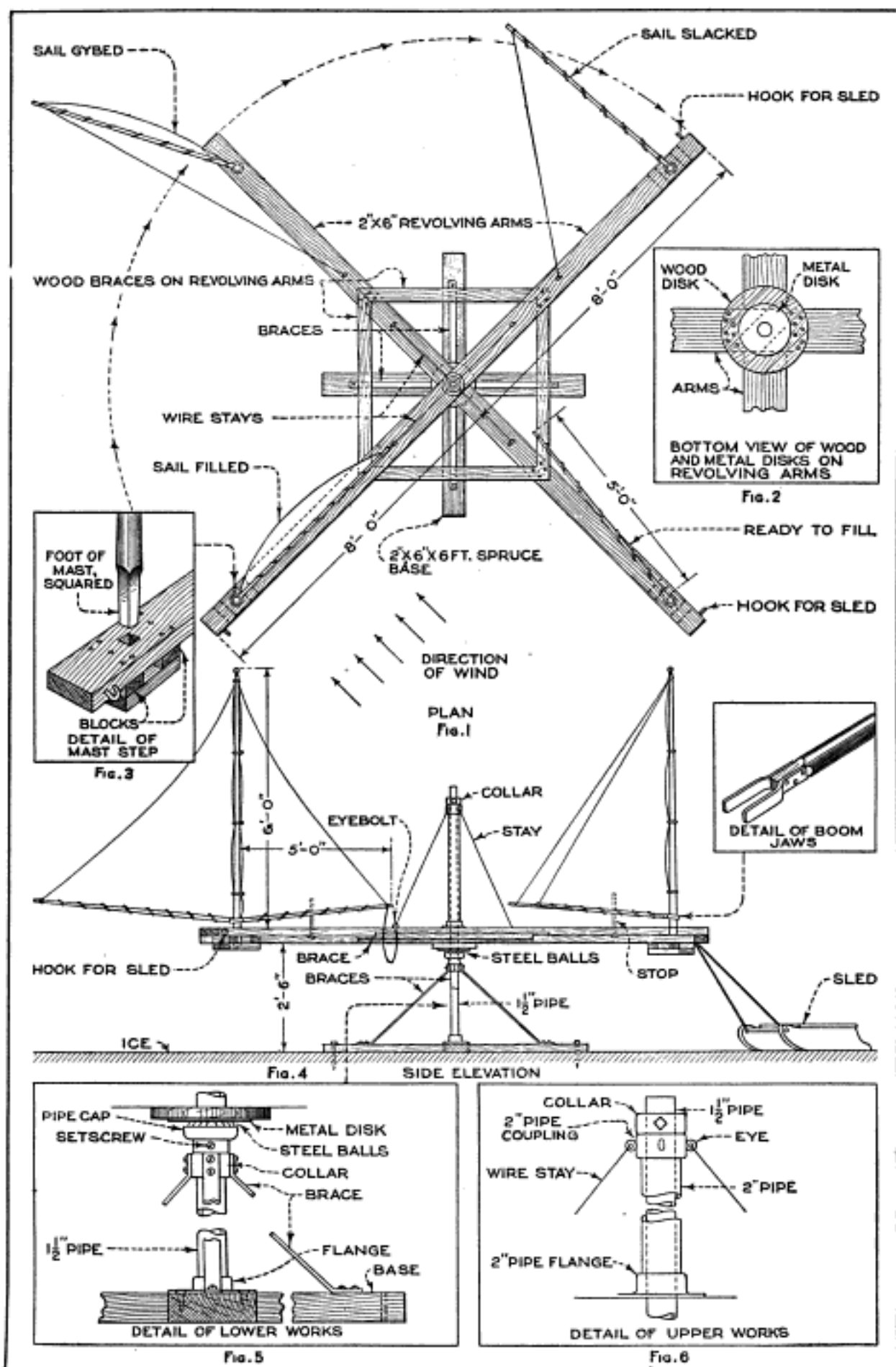
Figure 1: Plan Showing Base, Revolving Arms, and Braces; Also Positions of Sails in Relation to the Wind. Figure 2: Detail Showing Wood and Metal Disks on Revolving Arms. Figure 3: Squared Foot of Mast and Detail of Mast Step. Figure 4: Side Elevation, Showing Assembly of Merry-Go-Round. Figure 5: Detail of Lower Works. Figure 6: Detail of Upper Works
