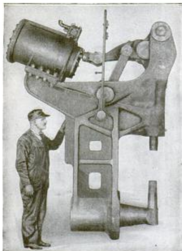
Portable Riveter, with a Capacity of 100 Tons, Designed for Driving Up the Last Heads in Boilers through the Manhole
