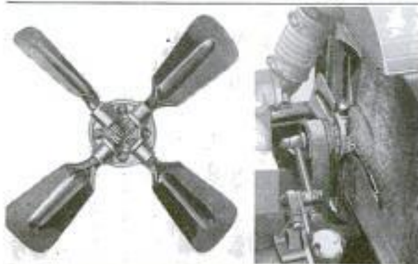
Left: Automobile Fan with Adjustable Blades for Reversing Flow of Air through Radiator. Right: Fan Installed in Car
