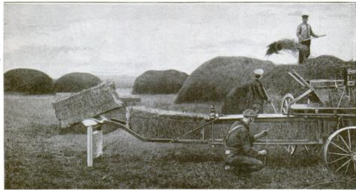
Hay-Baling Press at Work in the Field: As the Bales are Pushed from the Press Proper, They Pass over the Automatic Weighing Apparatus, Attached at the End of the Bale Conveyor, and are Weighed and Counted
