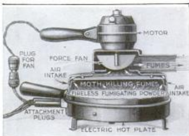
Fireless Electric Fumigator Reported to Be Effective in Destroying Insects That Infest Flour Mills
