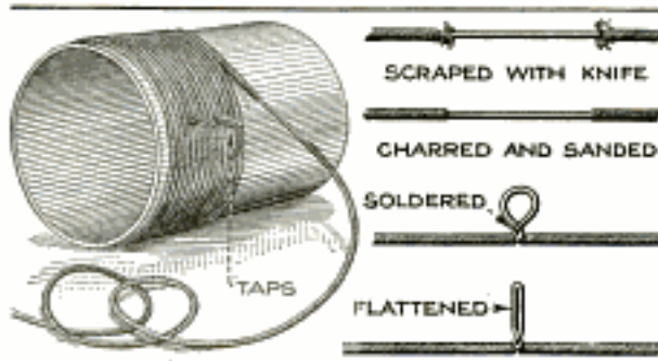
The Correct Method of Tapping Radio Coils by Charring the Insulation and Twisting the Bare Wire in a Loop While Winding the Coil
