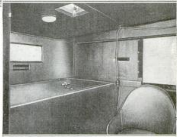
Interior of Rear Compartment of Armored Car, Showing Messenger's Seat and Safe in the Place of the Usual Rear Seat
