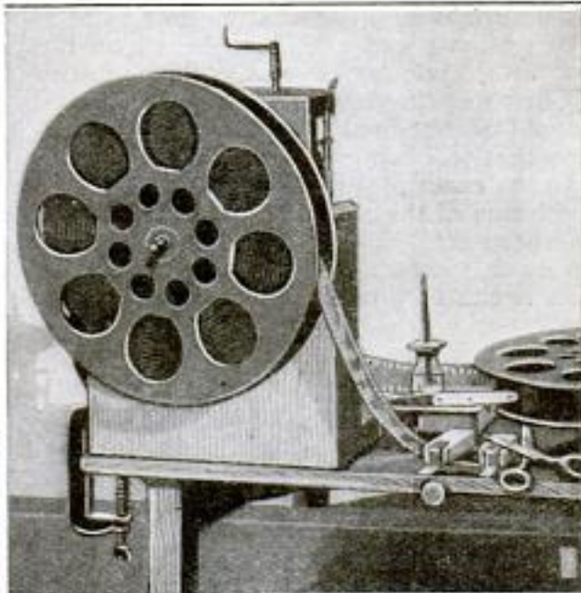
Left: Rear View of Film-Rewinding Machine, Showing How the Phonograph Motor is Attached. Right: Front View, Showing Reel in Place
