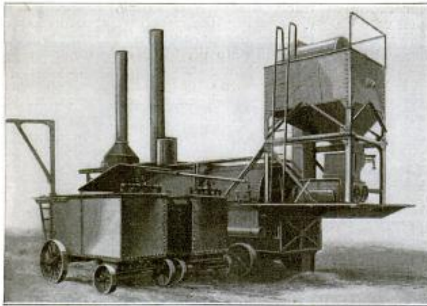
A New Portable Asphalt Plant in Which the Power Plant and Drier Form One Unit, and Two Kettles Are Separate: The Kettles are Heated by Means of Jointless Steam Coils
