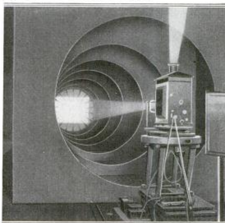
How the Projector is Set Facing the Tunnel: The Photometer and Curtains are Mounted on Rollers So That the Tunnel may be Adjusted to Various Lengths
