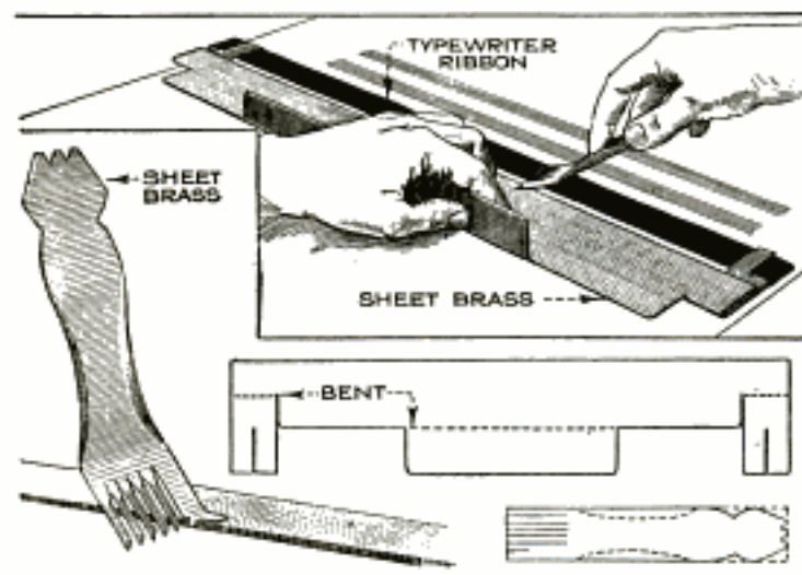
Above: Staff-Ruling Instrument in Use, Showing How the Special Ruler and Inker is Used. Below: Ruling Instrument Proper, and Patterns for Both Instruments
