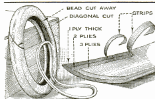
Homemade Reliners, Made from the Three Inner Plies of Old Fabric Tires, Greatly Increase the Mileage of a Set of Tires
