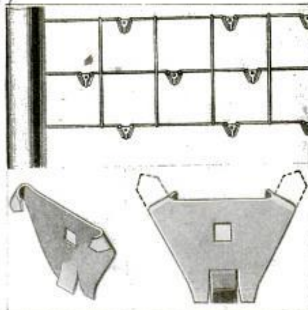
Triangular Clamp for Taking Up the Slack in Fence Wires, Operated by Inserting a Tool in the Square Hole in Center of the Plate, and Twisting the Wire
