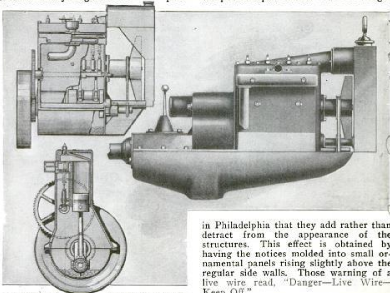
Above: View of Long-Stroke Auto Engine with Side Walls Partly Cut Away. Below: Cross-Sectional View. Right: Engine Fully Inclosed
