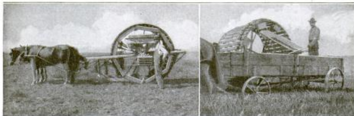
Left: Drum-Type Harvester Picking Up and Crating Potatoes: Two Horses Haul the Machine with Ease, and as There Are No Gears or Other Mechanisms, Upkeep Is Low. Right: Harvester Delivering Potatoes through a Canvas Chute to a Wagon Alongside
