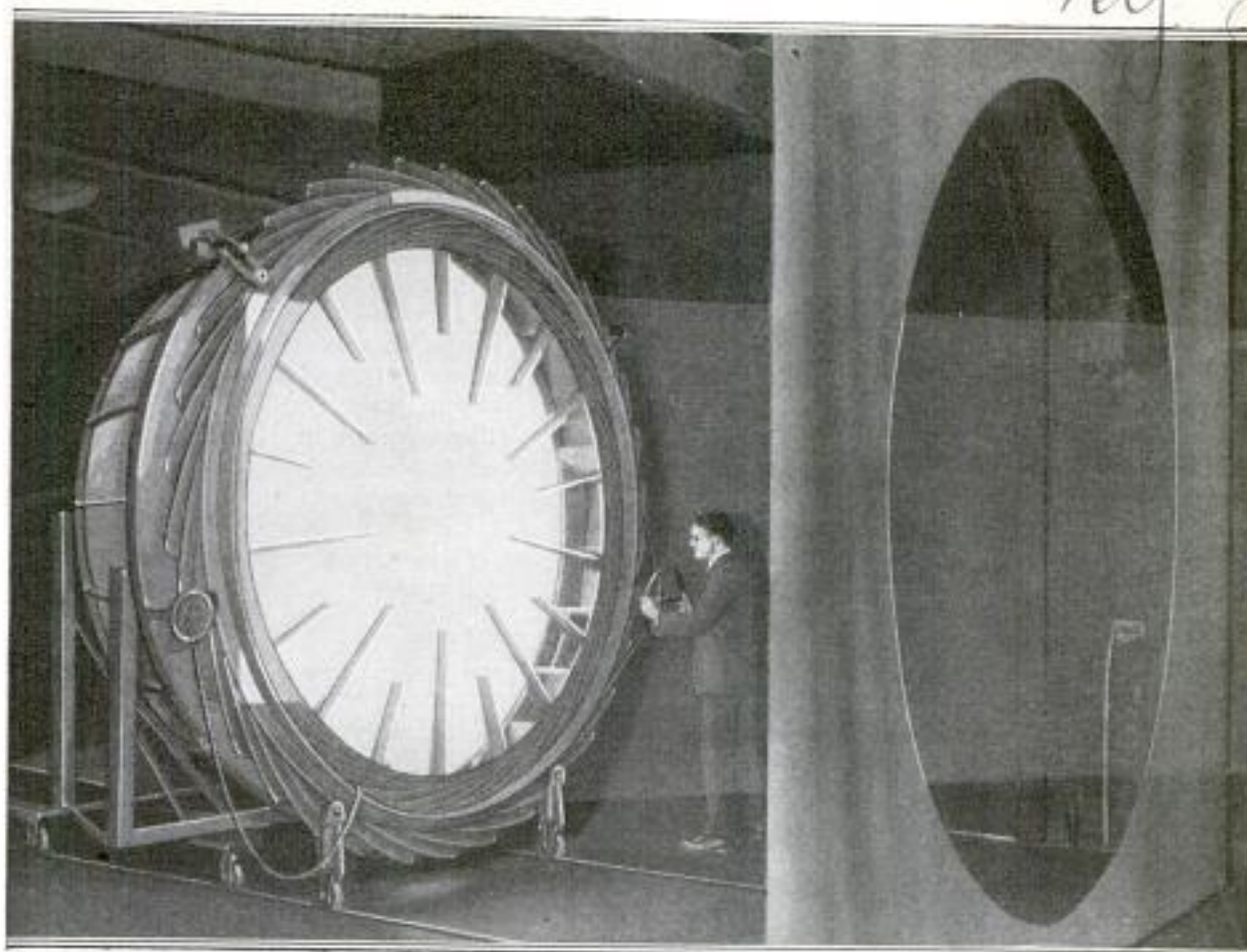
Close-Up of the Photometer, Which is Mounted at the End of the Tunnel to Measure the Light Received from a Motion-Picture Projector: The Radial Prongs, Extending Inward from the Shutter Ring, Are Black, and Serve to Correct Certain Optical Effects
