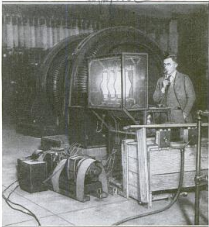
By Combining the "Superphone" with "Wired Wireless," the Operator is Talking from the Georgetown Power Station to the Bureau of Standards in Washington, Five Miles Away
