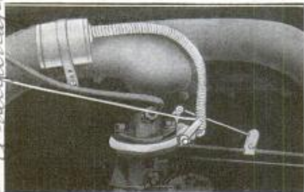
Air-Heating Device Installed on an Automobile Engine, Showing Its Controlling Attachment to the Carburetor-Throttle Rod, and the Auxiliary Control for Fine Adjustment
