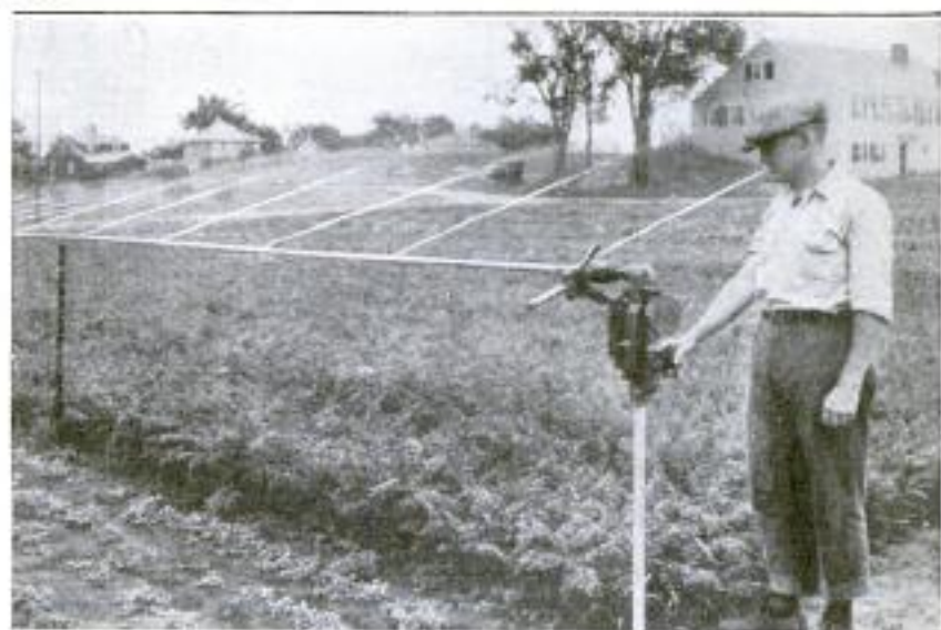
The Oscillating Device Shown at the Right Turns the Pipe from Left to Right So That the Stream Reaches Both Sides of the Garden. It can Also be Made to Spray One Side Continuously.
