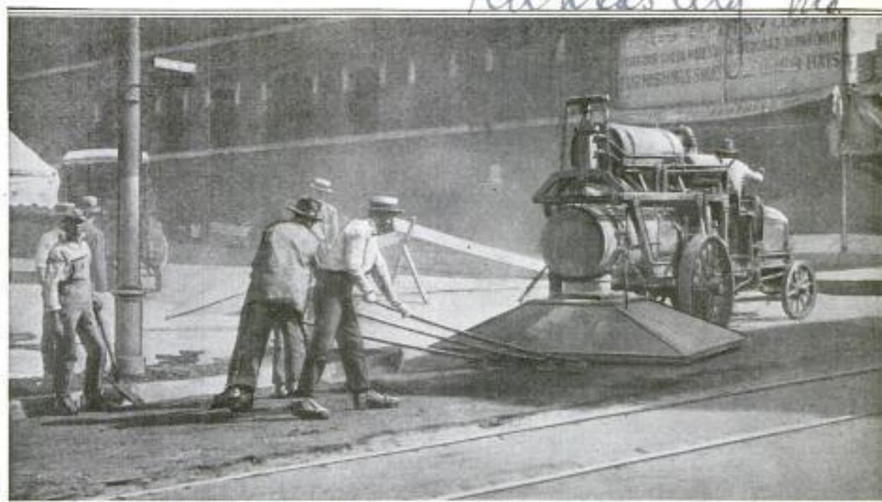
New Apparatus for Heating Asphalt Pavements Which are to be Resurfaced: Connected to the Steel-Plated Hood, Shown Here Resting on the Ground, Are Oil Burners, and Air-Blast Pipes Which Blow the Flame Downward
