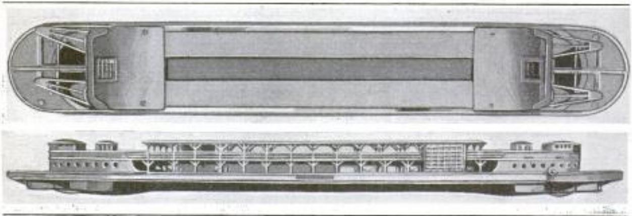
Top View of Hull and Side View of Completed Electrically Driven Barge for Erie Canal: It Has a Deck Space of Over 20,000 Square Feet, or About 15 Times That of the Average Canal Barge. Note the Peculiar Pontoon Rudders at Both Ends
