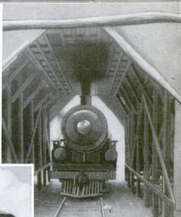
Upper Left: Locomotive Stack Discharging Smoke through Experimental Slots in Roof of Test House. Above: Locomotive in Test House Built to Determine Best Way of Eliminating Smoke Nuisance in New Union Station at Chicago
