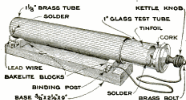
A Simple Type of Variable Condenser That Meets a Variety of Requirements in the Amateur's Radio Laboratory, is Easily and Inexpensively Built
