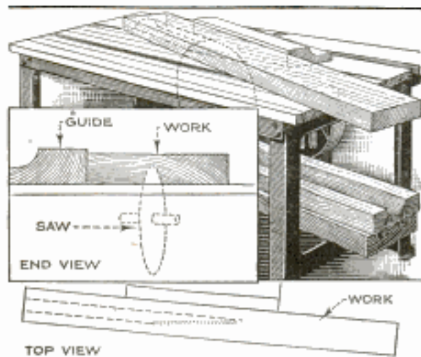
A Practical and Timesaving Method of Cutting Grooves of Varying Depth and Width in Wood, with a Power Saw
