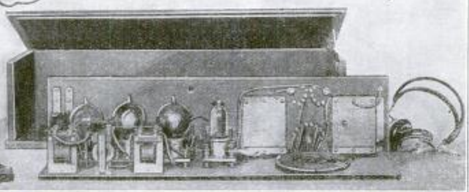
Receiver with Three-Step Amplifier: Above, Front View of Instrument, with Phones, and Detector and Amplifier Batteries; Center, Layout of Panel Front, and Rear View of Instrument, Showing Connections; Below, Rear View of Instrument, Cabinet, and Type of Loud Speaker Recommended
