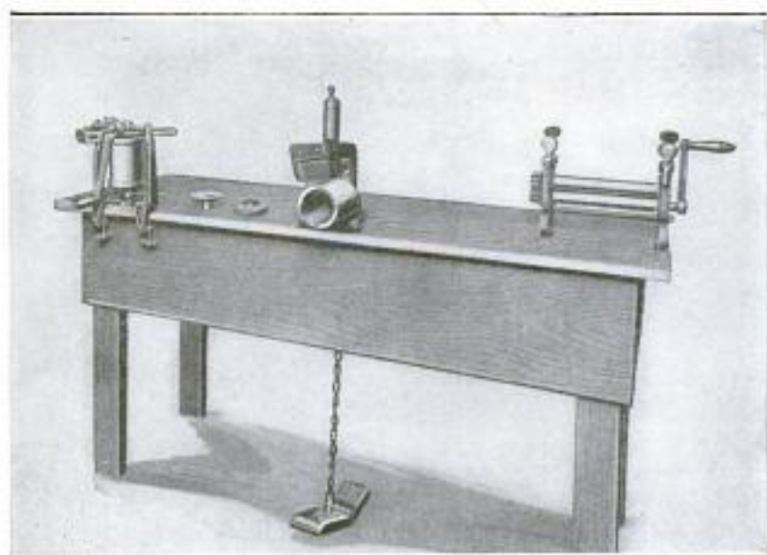
With This Simple Device, Tin Cans may be Made and Soldered, Saving the High Cost of Shipping. From Left to Right, the Machines Are the Crimper, That Puts on the Ends, the "Seamer," and the Shaper
