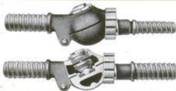
Top: Automatic Hose Coupling Which Takes the Place of a Globe Valve in an Air Line. Bottom: Sectional View of the Coupling
