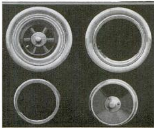
Illustrating the Assembly and Parts of a New Demountable Rim That can be Applied or Removed without Bolts or Lugs
