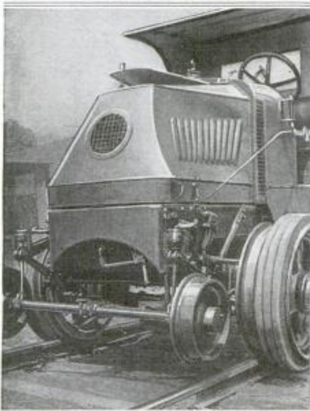
Front End of Motor Truck with Pilot About to be Lowered for Rail Travel: Four Coil Springs Hold the Pilot Wheels in Engagement with the Rails, After They have been Lowered
