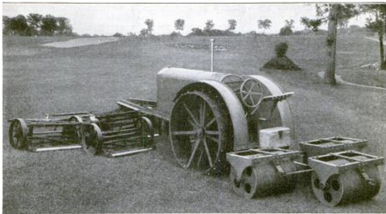
Combination of Tractor-Driven Roller and Mower That Cuts 80 Acres of Grass a Day on a Golf Course: The Five 30-Inch Mowers Cut a Swath 142 Inches Wide, and Are Flexible Enough to Conform to Irregularities in the Ground
