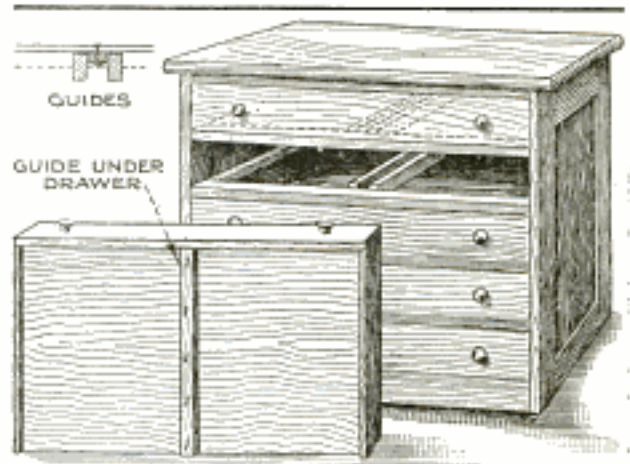
Binding and "Canting" of Drawers are Eliminated by Providing an Extra Slide in the Center
