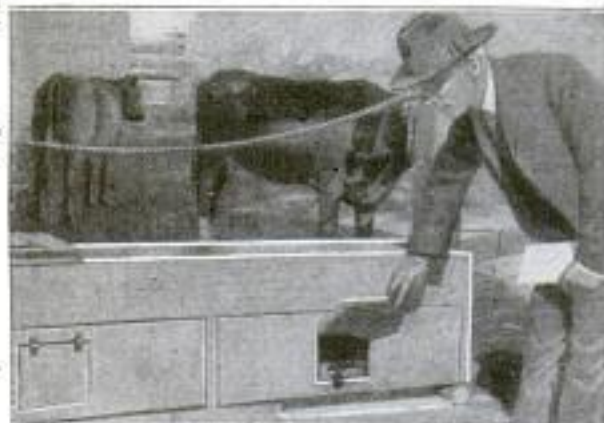
The Water in This Trough is Kept from Freezing by Two Lamps in a Lower Compartment, One Section of Which is Shown Open
