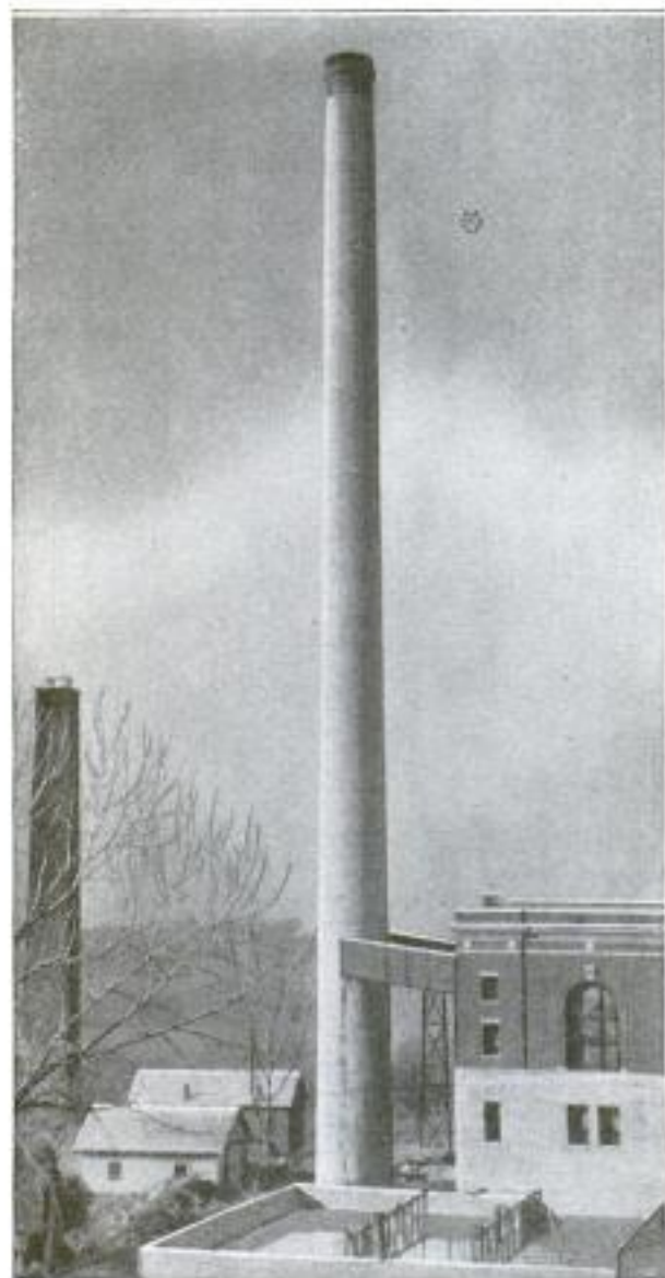
Reinforced-Concrete Stack, 257 Feet High, Recently Completed for the Power Plant of the University of Kansas
