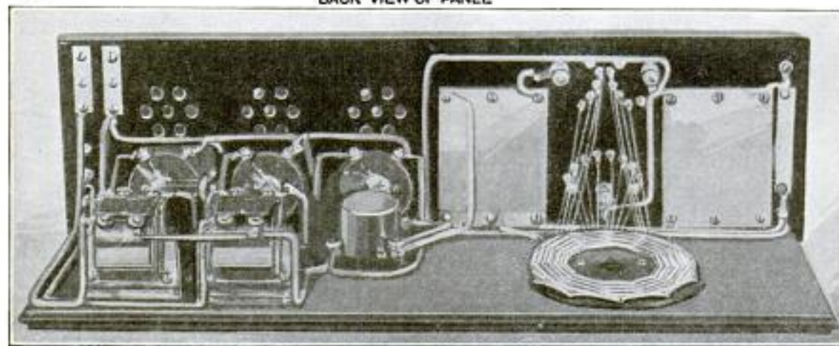
Receiver with Two-Step Amplifier: Above, Front View of Completed Instrument; Center, Wiring Diagram and Drawing of Back of Panel, Showing Arrangement of Parts; Below, Rear View of Completed Instrument, Removed from the Cabinet. The Tubes are Removed from Their Sockets
