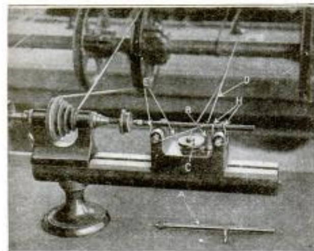
Lapping Diamond Wire-Drawing Dies in a Bench Lathe: The Toolholder is Reciprocated by Means of a Cam and Rubber Bands
