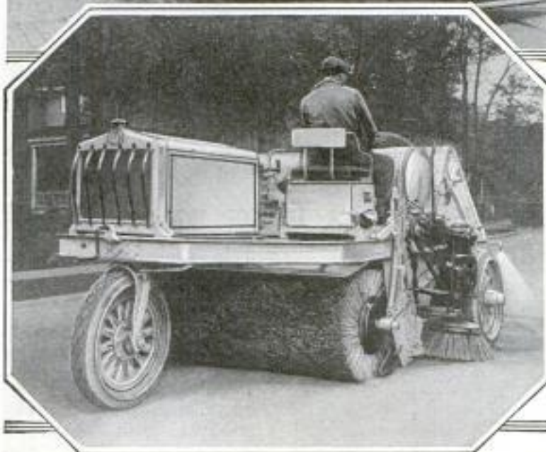
Combination Street Sweeper and Sprinkler Which Wets the Surface Ahead of the Revolving Brush and Prevents the Clouds of Dust That Usually Accompany Such Operations
