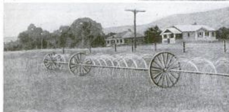
A Movable Irrigation Outfit Made from Perforated Pipe and Four Buggy Wheels: It is Shown Watering an Alfalfa Patch. Standpipes, 50 Feet Apart, Make It Possible to Use Only 25 Feet of Hose
