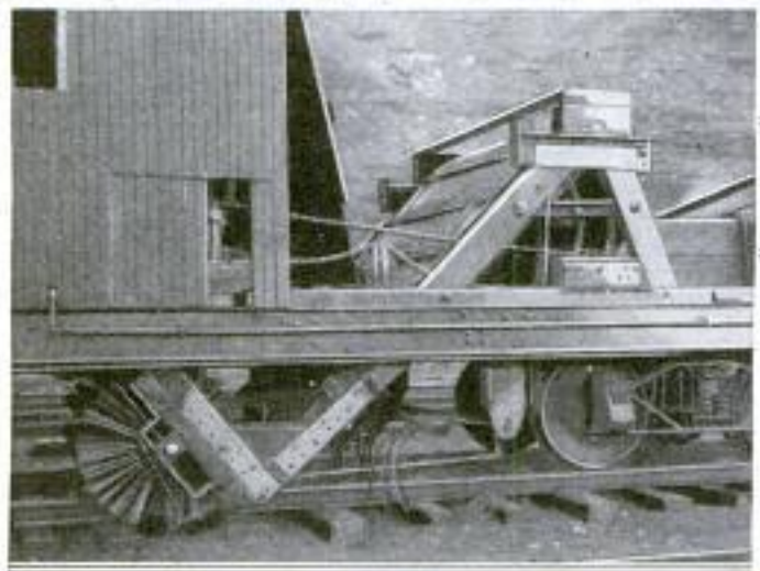
Close-Up of Steel Broom, Showing the Manner of Its Mounting and a Set of "Fingers" Ahead of It That Loosens Up the Dirt
