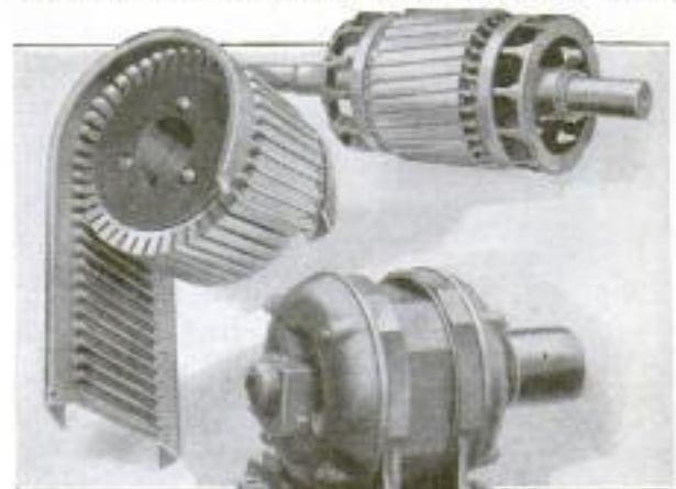
Rotor and One-Piece Winding for It: The Partly Wound Shows and Manner of Winding to Form Integral Joint with End Rings
