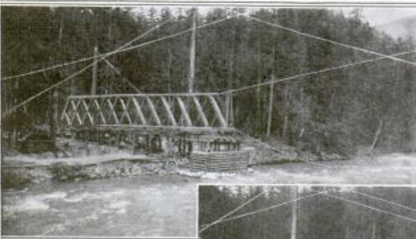
In the Photograph Above, the Completed Truss is Shown as It Appeared Just before being Pulled Out of, and over, the River
