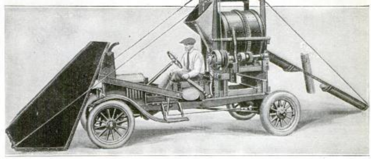
Complete Concrete-Mixing Outfit Installed upon the Chassis of a Motor Truck: The Mixer is Driven by the Engine of the Truck, and is Charged by Swinging Up the Hopper Seen Pivoted in Front of the Truck. The Concrete is Discharged by the Chutes in the Rear
