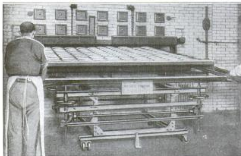
Showing How the Removable Tray, Accommodating 200 Loaves of Bread, is Rolled into the Oven from the Truck on Which It is Wheeled about the Shop Interior
