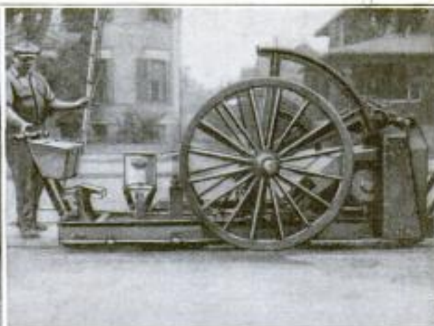
Left: Close-Up of Rail-Grinding Machine, Showing the Two Handwheels, by Means of Which the Pressure on the Stones is Regulated. Right: Side View of the Grinder at Work; Note the Large Wheels Used in Moving the Machine
