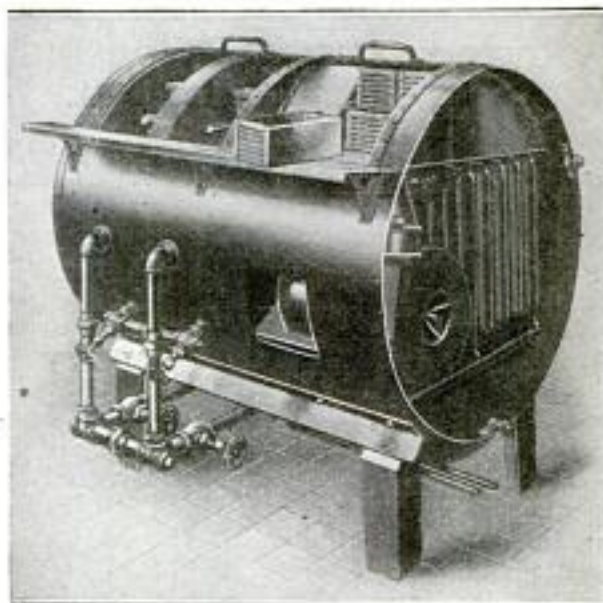
The Washer with One End of the Cylinder Exposed, Showing the Radiator and Fan under the Drying Chamber
