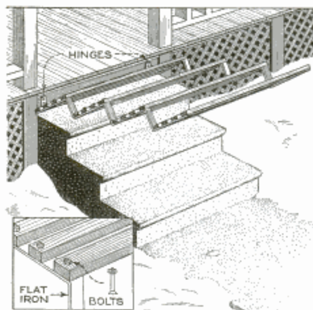
An Iron Frame, Provided with Wooden Treads, Eliminates the Danger Caused by Ice Accumulating on the Surface of Concrete Steps
