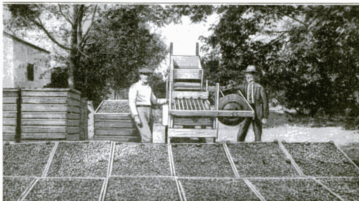
Using the Grading Machine Shown Above, Eight Sizes of Pecan Nuts can be Quickly Sorted. The Nuts Pass from the Hopper onto Rollers, with Various-Sized Openings between Them, Thence along Gutters Leading to Baskets on the Ground
