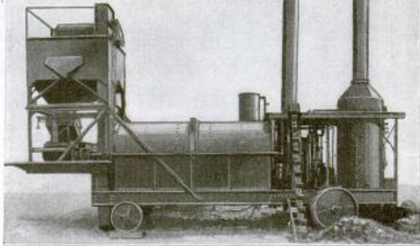
View of the Power Plant and Sand-Drier Unit: The Three-Compartment Bin Holds 10 Tons of Sand, and the Three-Drum Drier will Handle 120 Tons of Sand a Day
