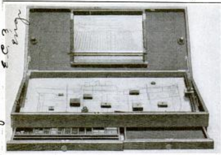
Arrangement of Charts and Weights by Means of Which the Stability of a Ship can be Readily Found for a Given Cargo or Ballast Loading, or a Combination of Both, and the Vessel Trimmed to Suit
