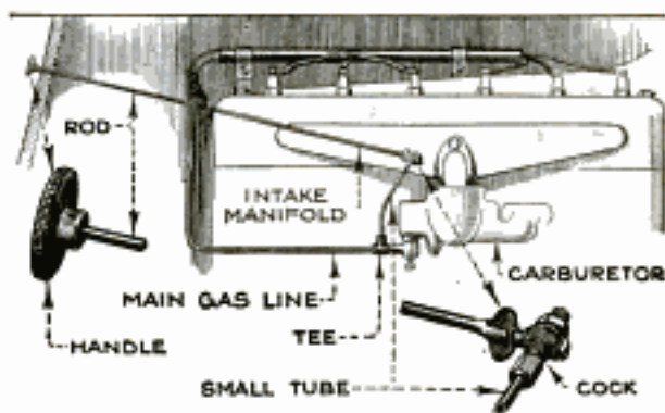
A Simple Primer for Automobiles That Have a Pressure Gasoline Feed: It is Operated by Turning a Small Knob on the Dash
