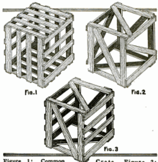
Figure 1: Common Crate. Figure 2: Bracing Giving Maximum Strength with Minimum Lumber. Figure 3: Type Recommended for Rigid Material
