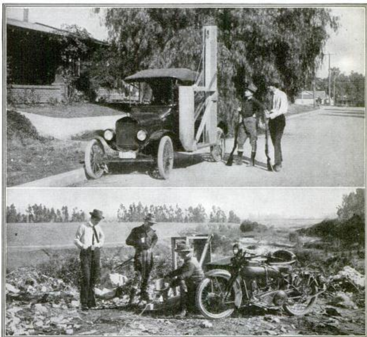
Above: The Enthusiastic Marksmen Strap the Catapult on the Running Board of a Small Car, to Convey It to the "Hunting Grounds." Below: Loading the Catapult; All That Is Necessary Is to Draw the Arm Down, Catch It to the Base by the Bolt, and Place the Cans on the End
