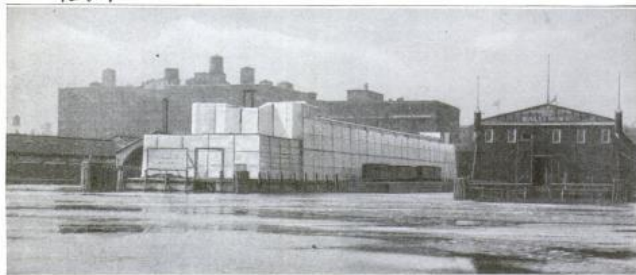
With the Huge Protecting Canvases Shown Above, Erected over the Steel Structure, and a Heating System Inside, the Men Building This Pier on the Delaware River Found They could Continue Working No Matter How Cold or Stormy It Was Outside
