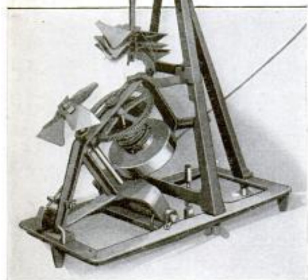
Automatic Trapshooting Machine That Fires and Reloads by Pulling a Cord: The Star-Shaped Markers Are Practically Indestructible and can be Used Again
