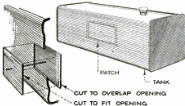
An Inconspicuous and Strong Repair for a Punctured Gasoline Tank Made by Sweating Two Plates Together
