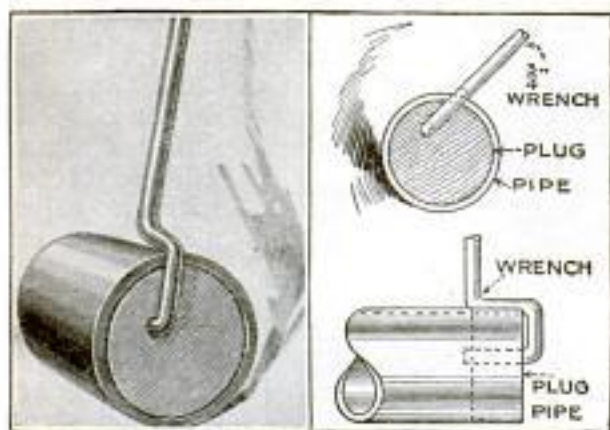
A Simple Wrench, Consisting of a Lever and a Wooden Disk, Makes a Good Substitute for a Large-Size Pipe Wrench
