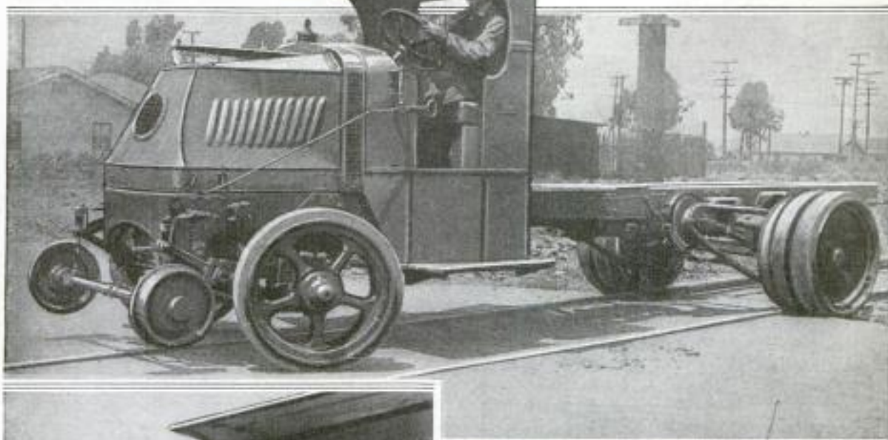
The New Double-Duty Motor Truck Running off the Track and onto a Smooth Road: The Lifting of the Pilot Wheels Unlocks the Steering Mechanism of the Motor Truck
