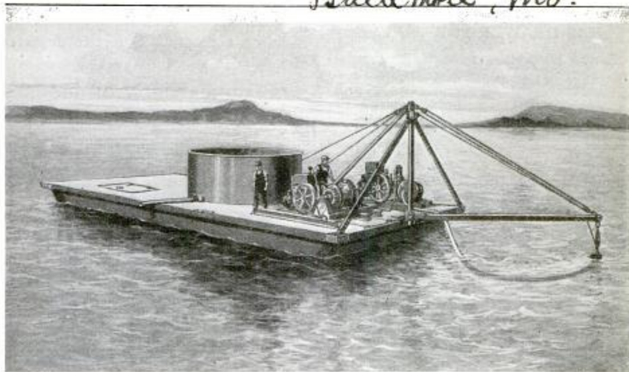
Apparatus for Skimming Waste Fuel Oil from the Surface of the Water in the Harbor of Baltimore, Maryland: On Board the Scow Is a Pump in Connection with the Hose, the Intake End of Which is Suspended from the End of the Boom. The Tank Is for Separating the Oil from the Water
