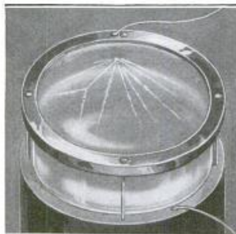
Appearance of Upper Glass Portion of Cylinder When Brilliantly Illuminated, at the Instant Atom Tracks are Formed: Note Collision between Two Atom Nuclei Shown by Forked Trail at the Left
