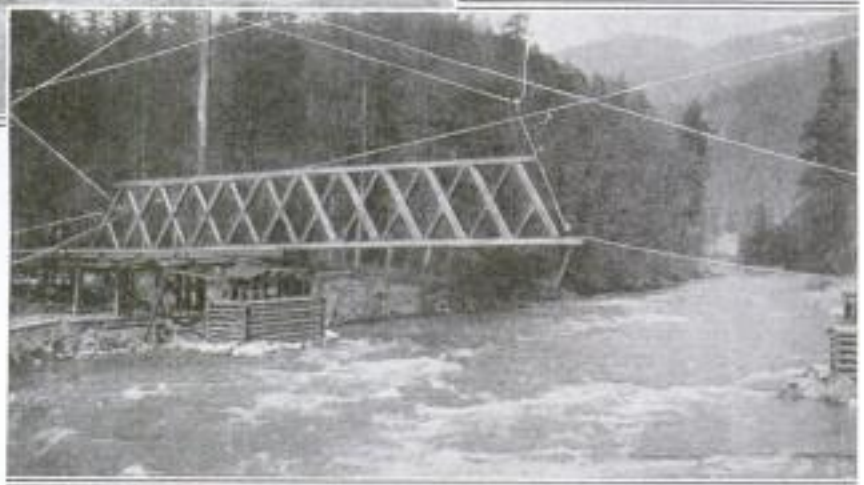
This Picture of the Truss was Taken as Its Right End Reached a Point About Midstream. A Few Moments Later It was Dropped in Place on the Piers, Which had Already been Constructed
