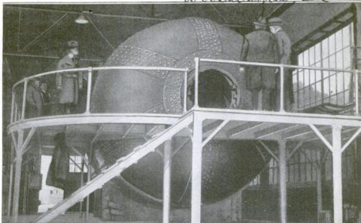
End of Compressed-Air Tank Inclosing Wind Tunnel Used in Testing Models of Airplanes: The Opening Shown is Closed by a Door Weighing Two Tons, Opening Inward. The Tank Operates under an Average Pressure of 300 Pounds per Square Inch
