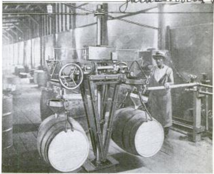
Revolving Scale for Filling Barrels with Oil and Other Liquids: When the Desired Amount has Run In, the Flow is Automatically Shut Off, and the Scale is Then Turned Halfway Around
