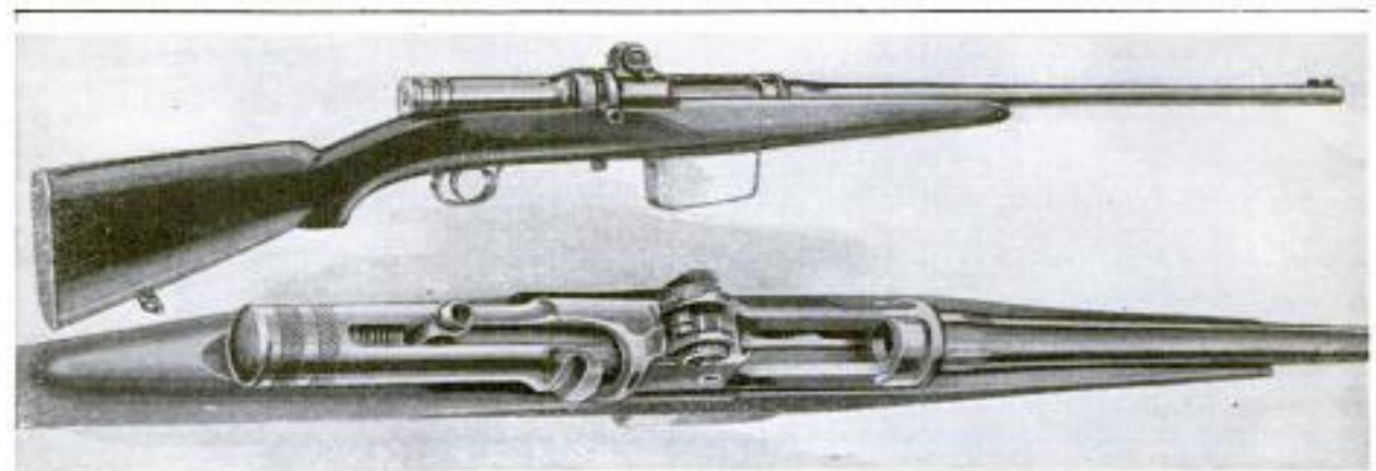
Top: Self-Loading Rifle Which has been Introduced for Use by the Infantry, Showing the Tubular Recoil-Spring Chamber and the Boxlike Magazine for the Cartridge Clips. Bottom: Looking Down upon the Rifle Mechanism at Close Range, Showing the Peculiar Bolt Action and the Recoil Spring
