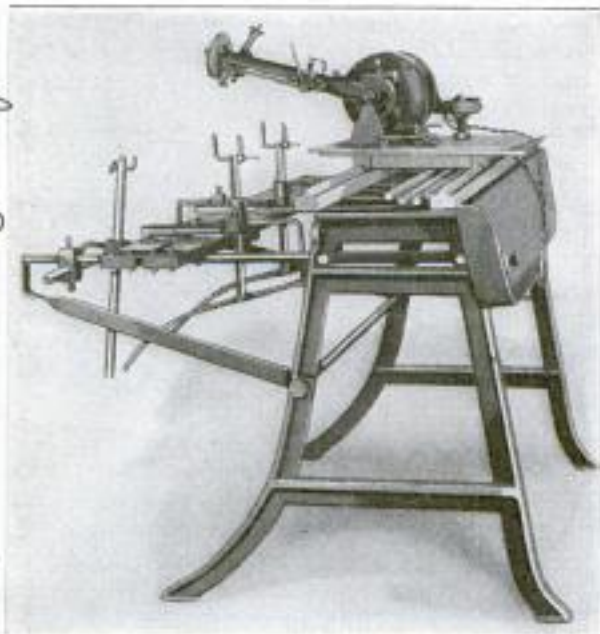
Machine for Grinding Any Size of Lawn-Mower Blade, Large Units of Which can be Set in the Machine and Ground without Removing the Reel
