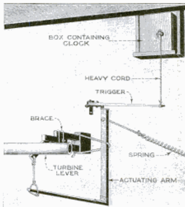
Crude but Thoroughly Practical Apparatus Which was Devised by a Miller to Extinguish the Lights in a Minnesota Village Automatically
