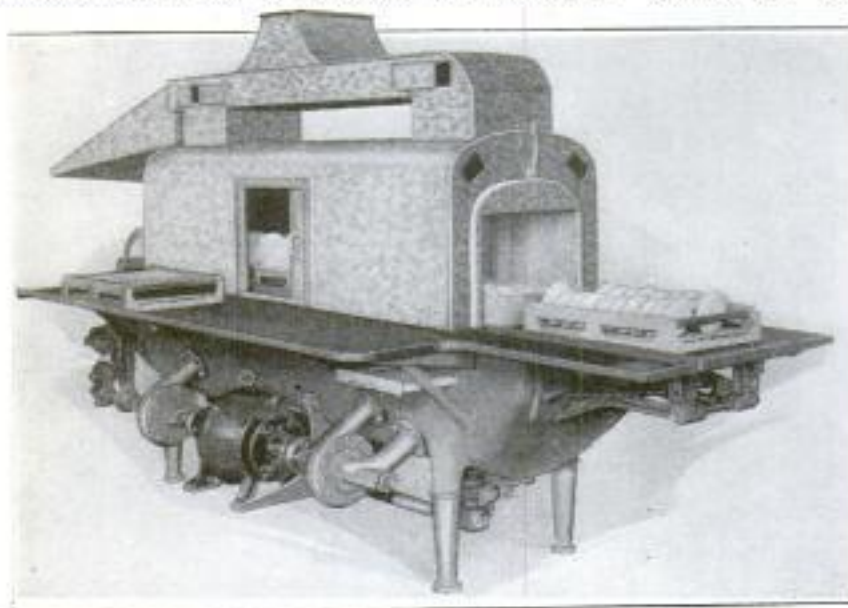
Automatic Dishwasher for Restaurant and Hotel Use, Which Has Duplicate Driving Motors and Pumping Units to Guard against Break-down, and Wooden Trays to Reduce Breakage
