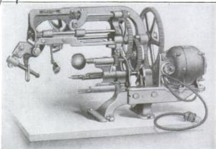
Motor-Driven Machine Which Automatically Cores and Pares 30 Apples a Minute: All the Operator Does Is to Place the Apples on the Holding Fork
