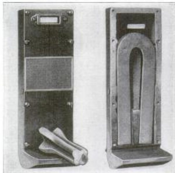
Left: Magnetic Indicator with Cover On, and a Drill Bit on the Shelf. Right: Cover Removed, Showing Horseshoe Magnet
