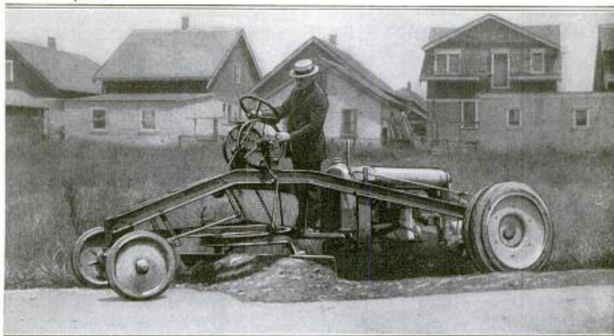
The New Road-Grading Outfit, Pictured Here, is Run Entirely by One Man, Who Stands on a Platform Built in Front of the Gasoline Engine. Within Easy Reach of the Operator Are Controls for Steering the Machine, and for Raising, Lowering, or Turning the Blade
