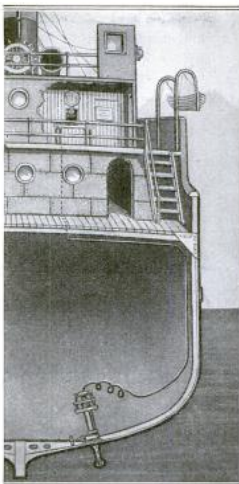
The Electric Log, Greatly Exaggerated in Size, as Installed in a Ship
