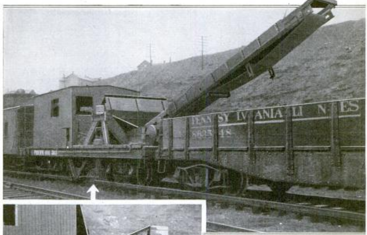
General View of the Track Sweeper Used by the Pennsylvania Railroad, Showing the Conveyor Belt and Receiving Car
