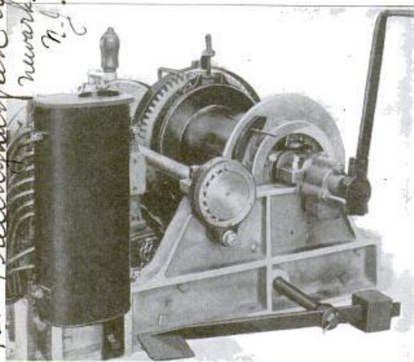
Hoist for Use with Standard Electric Motors without Solenoid Brakes, Which Has an Automatic Safety Brake and an Improved Screw That Reduces the Work of Operating the Friction Clutch
