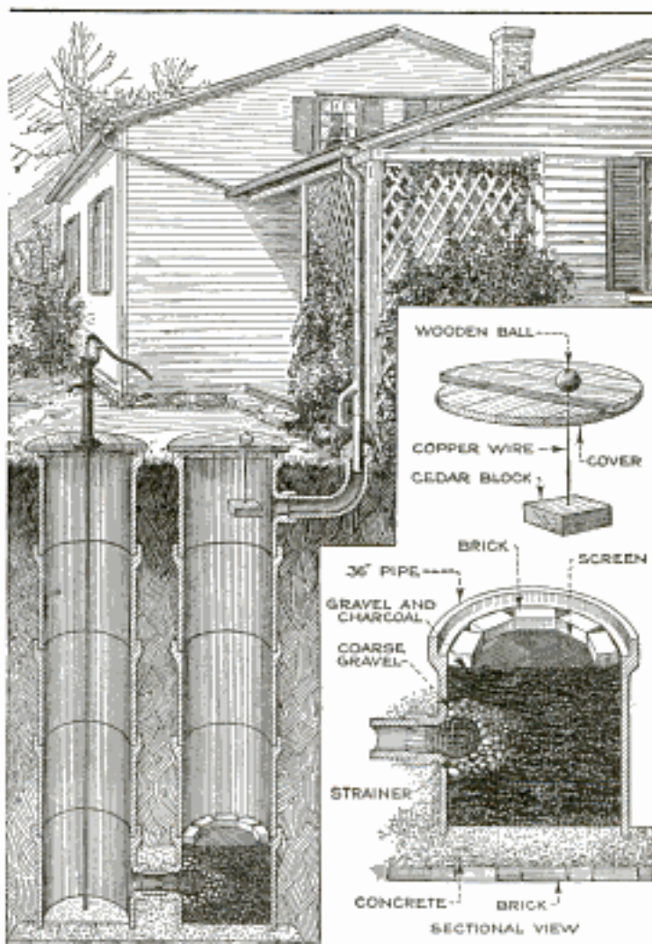
A Two-Section Farm Rain-Water Cistern Constructed of 36-Inch Vitrified Clay Pipe: It Is More Sanitary than Most Cisterns
