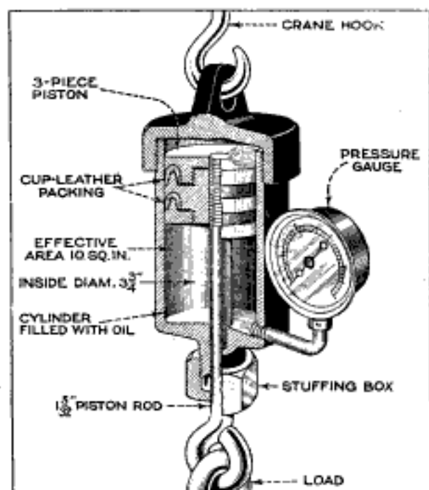
A Hydraulic Scale for Use on a Crane as a Safeguard against Overloading, Which can be Readily Detached
