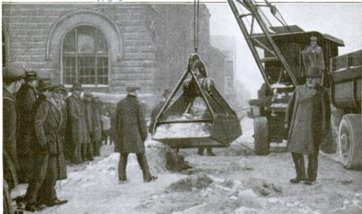
Cranes of This Kind with Extra-Wide Buckets have been Found Useful in Loading Street Piles of Snow onto Trucks in New York and Detroit. It is Estimated That Three of the Regular Five-Ton Trucks can be Loaded by This Method in 10 Minutes
