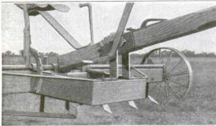
Weeder for Use on Dry Farm Lands: The Levers, Seen Handy to the Driver's Seat, Raise and Lower the Cutting Blades That are Suspended below the Frame of the Machine
