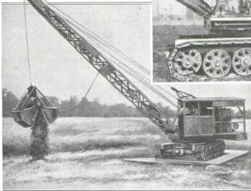
Above: New Crawler-Type Crane That Has a Capacity of 10 Tons at a 12-Foot Radius and 3 Tons at 30-Foot Radius. Left: Crane Mounted on Wooden Floats, Building a Swamp Road
