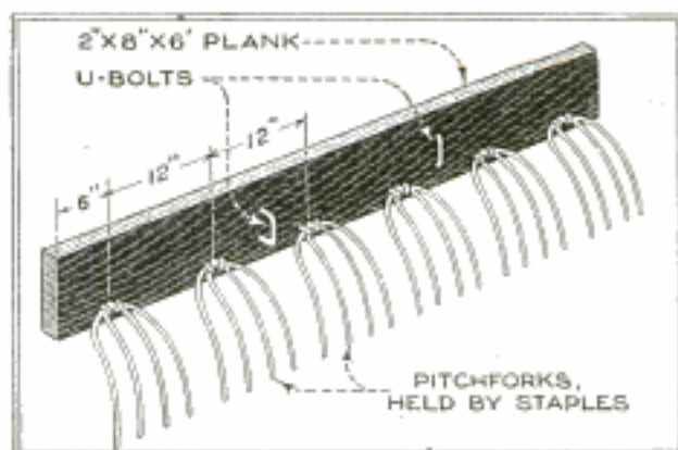
Details of the Soil Crusher: The Device can be Made in Half an Hour
