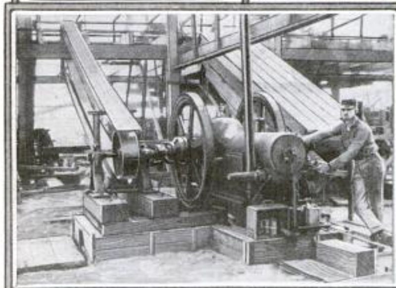
Right: A Safety Device in the Form of a Hinged Door That Serves as a Guard in Front of the Engine Flywheel. In Most Places in This Plant, Belting is Protected with a Housing of Boards, but in Some Instances It is Allowed to Run Exposed to All Sorts of Weather. The View Shows a 17-Horsepower Gas Engine, Which can be Used Alone to Run the Plant, or Run in Combination with the Other Engine
