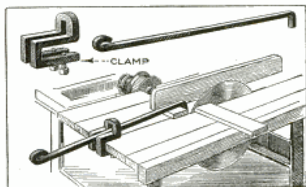
A Simple Safety Device for Protecting the Fingers of the Workman While Using a Circular Saw
