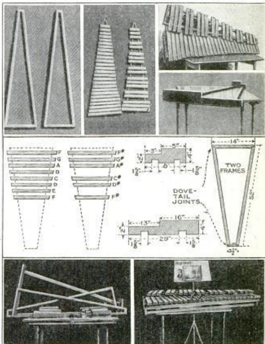
Upper Left: Triangular Bar Frames. Upper Center: The Finished Bars. Upper Right: Bars and Stand. Center: Details of Construction. Lower Left: Instrument Knocked Down. Lower Right: Xylophone Complete
