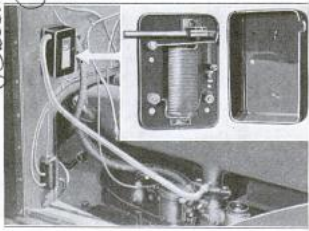
Air-Feed Regulator Shown Installed on the Dash of an Automobile: Enlarged Inset View Shows It Opened Up, Exposing Its Low-Resistance Coil
