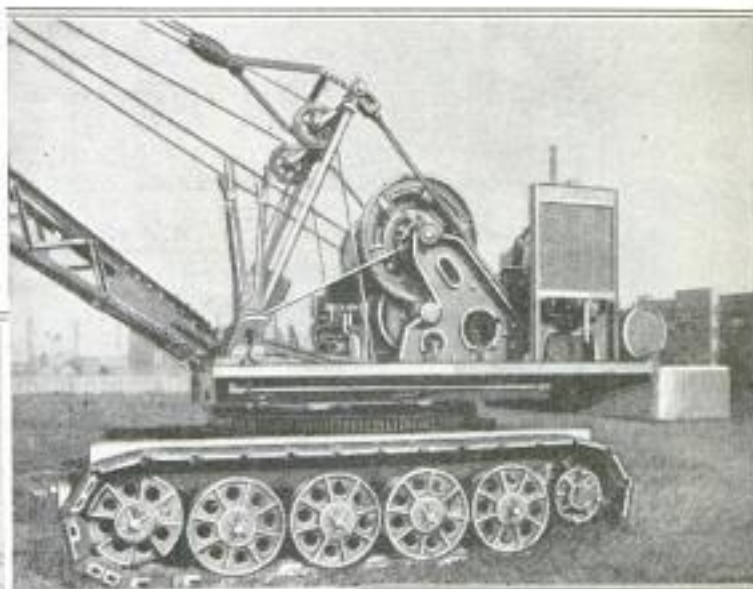
Above: New Crawler-Type Crane That Has a Capacity of 10 Tons at a 12-Foot Radius and 3 Tons at 30-Foot Radius. Left: Crane Mounted on Wooden Floats, Building a Swamp Road
