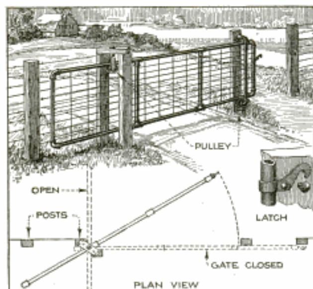
Sliding and Swinging Farmyard Gate That Serves Both Pedestrians and Cattle, or Vehicles
