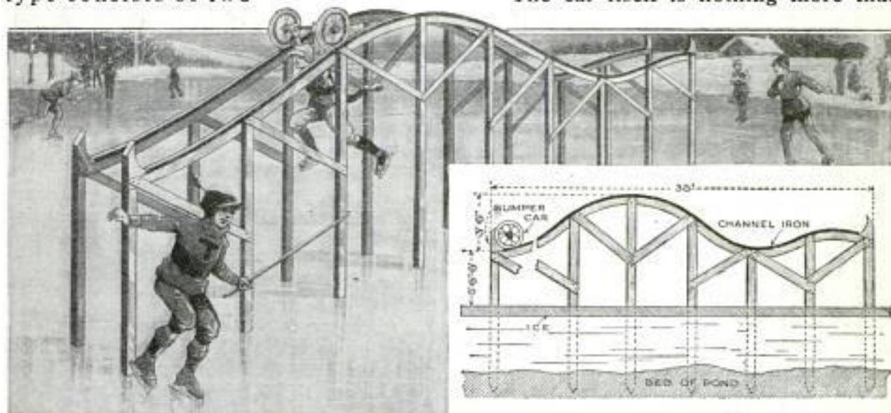
A Simple Coaster, Made of a Few Pieces of Lumber and Some Channel Iron, and Provided with a "Car" Made of a Tricycle or Buggy Axle, Furnishes Exhilarating Sport for the Skating Pond. The Drawing Serves Only as a Guide, the Dimensions Being Altered to Suit the Location or the Users' Convenience
