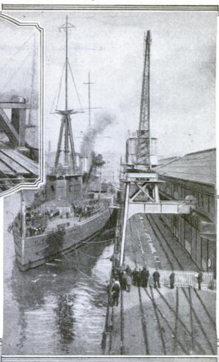
Above: Traveling Concrete Mixer at Work on One of the New Wharves in Connection with the Harbor Extensions at Auckland, New Zealand. It is Used for Making the Concrete Piles for the Wharf. Right: Part of One of the Reinforced-Concrete Wharves, Showing the Quay Side, with Its Railway Lines, and One of the Large Electric Traveling Cranes. Beside the Quay is Seen Part of One of the Two-Story Steel Cargo Sheds Which Are 320 Feet Long and 60 to 80 Feet Wide. Below: Concrete Pier Built to Act as a Tide Deflector in Connection with the New Harbor Extensions
