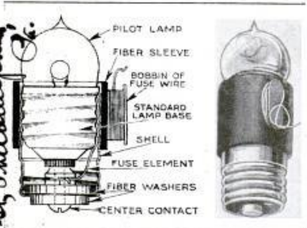
At the Left Is a Sectional View of the Plug-Type Renewable Fuse Which Contains an Indicating Lamp. Right: General View of Fuse
