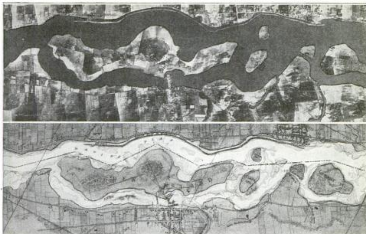
Top: Mosaic Map Made Up of 150 Photographs Taken from an Airplane. Below: A Hydrographic Chart or Standard Map, of the Same Area, Drawn to Approximately the Same Scale. Note the Accuracy of Detail in the Aerial Mosaic
