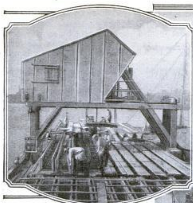
Above: Traveling Concrete Mixer at Work on One of the New Wharves in Connection with the Harbor Extensions at Auckland, New Zealand. It is Used for Making the Concrete Piles for the Wharf. Right: Part of One of the Reinforced-Concrete Wharves, Showing the Quay Side, with Its Railway Lines, and One of the Large Electric Traveling Cranes. Beside the Quay is Seen Part of One of the Two-Story Steel Cargo Sheds Which Are 320 Feet Long and 60 to 80 Feet Wide. Below: Concrete Pier Built to Act as a Tide Deflector in Connection with the New Harbor Extensions
