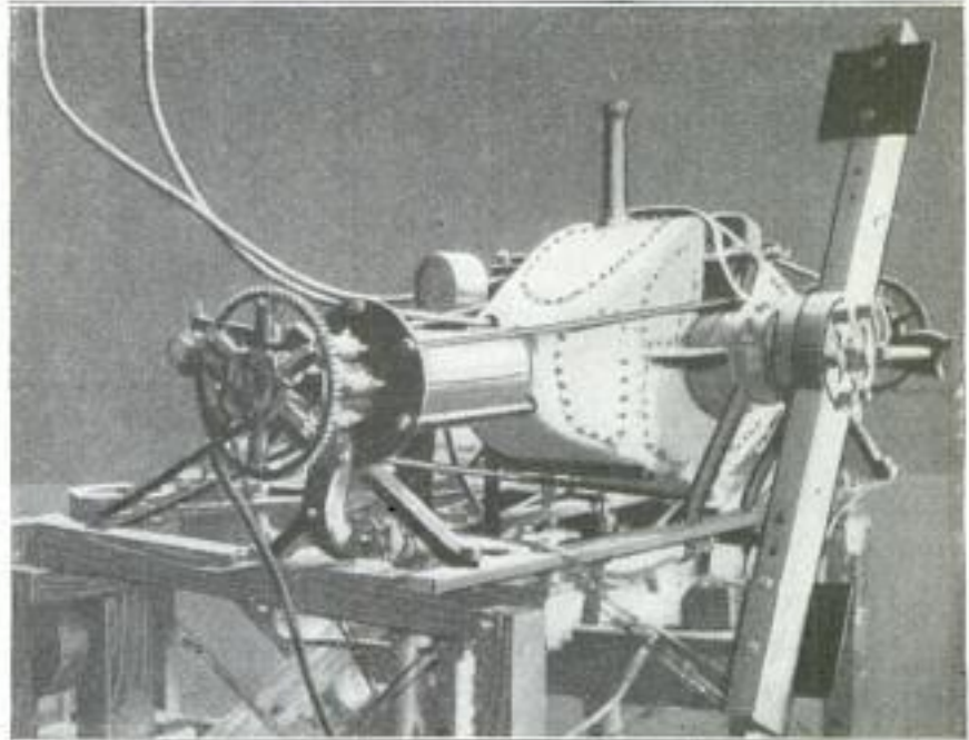
Novel French Airplane Engine, under Test, Which, after Combustion, Completes the Expansion of the Charge to Little More than Atmospheric Pressure: It Is Self-Cooled and Weighs About Two Pounds per Horsepower
