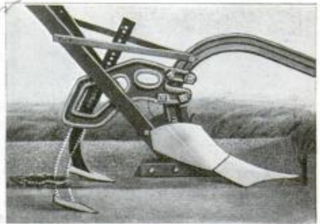
Subsoiling Attachment Connected to a Steel-Beam Plow: Dotted Lines Show How It can be Adjusted
