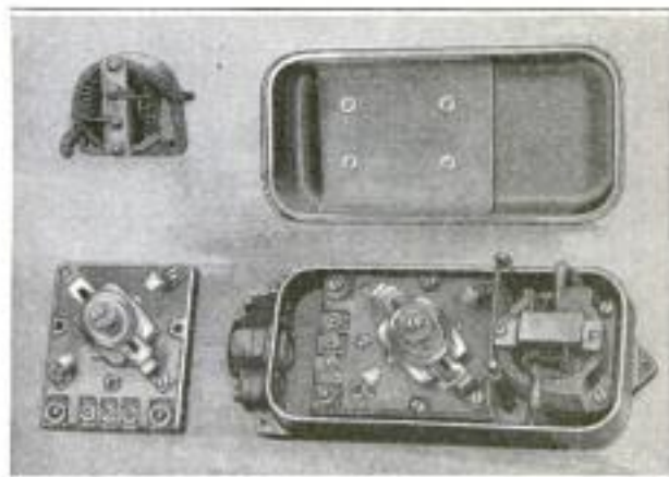
This Motor-Operated Snap Switch Is Adaptable Wherever Automatic Control of Electrical Devices is Desired, and Consumes Little Power
