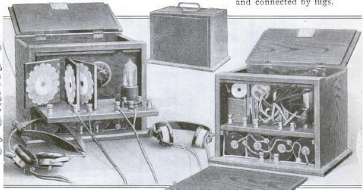
Left: Radio-Receiving Set Opened Up Ready for Use and Display. Upper Center: Reduced View of the Box Closed, Showing Carrying Handle. Right: Top and Side of the Box Opened, Illustrating the Compact Manner in Which the Outfit may be Packed for Carrying
