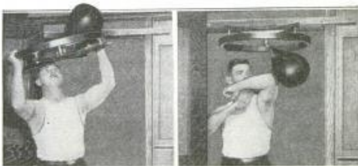
Left: Noiseless Punching-Bag Platform That Fits in Doorway without Marring Woodwork and is Quickly Put Up and Removed. Right: Punching-Bag Holder in Use
