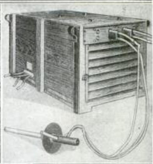
Welding and Cutting Transformer Shown in Connection with the Handle, Which can be Operated with One Hand
