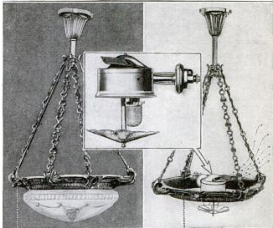
Left: Gas Fixture Completely Assembled. Right: Fixture with Bowl Removed, Showing the Heat-Deflecting Burner. Insert: Close-Up of Heat-Deflecting Burner, Mantle, and Saucerlike Mica Container
