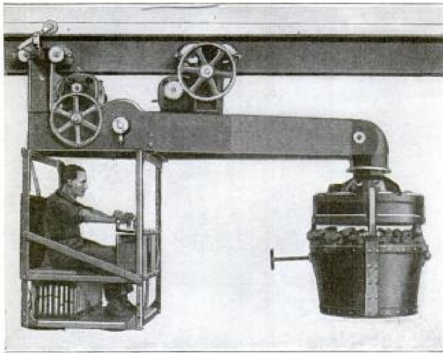
New Cupola-Charging Hoist with a Drop-Bottom Bucket Loaded with Coke: The Hoist is Operated Electrically, and the Charging Arm Also Carries a Magnet for Handling Pig Iron and Scrap
