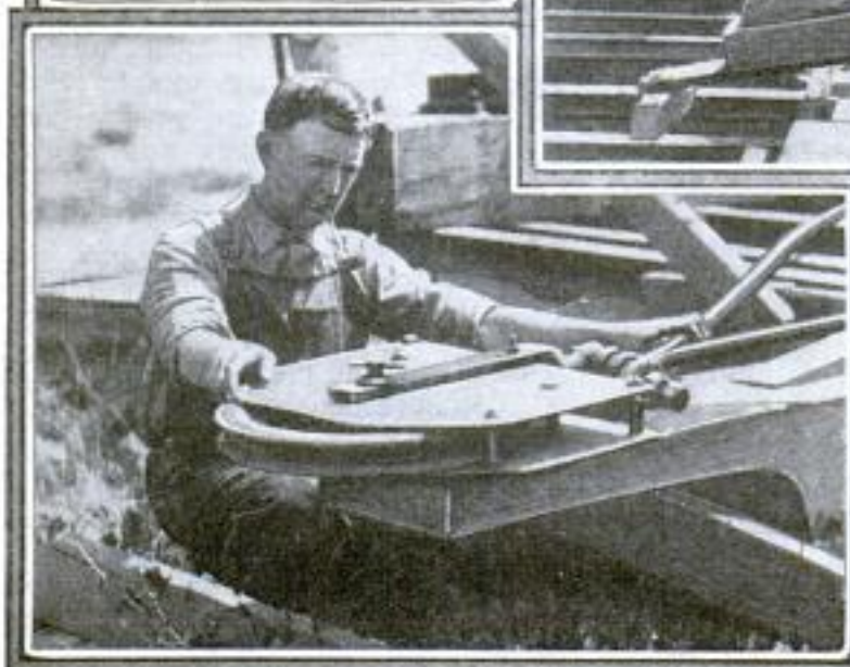
Above: The Bilge Blocks of the Cradles of the Marine Railway are Easily Slid into Position and Automatically Lock in Place under Water. Clamps Hold Them to the Cross Rails of the Cradle and They are Quickly Unlatched by a Jerk on a Cord. Left: Large Iron Sheave Made from Elevator Scraps and Used on the Head of One of the Smaller Cradles. It is Only One of the Many Evidences of Resourcefulness
