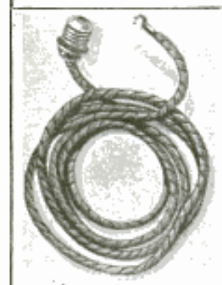
An Inexpensive but Satisfactory Attachment That Enables the Amateur to Use the Lighting Circuit as an Indoor Antenna
