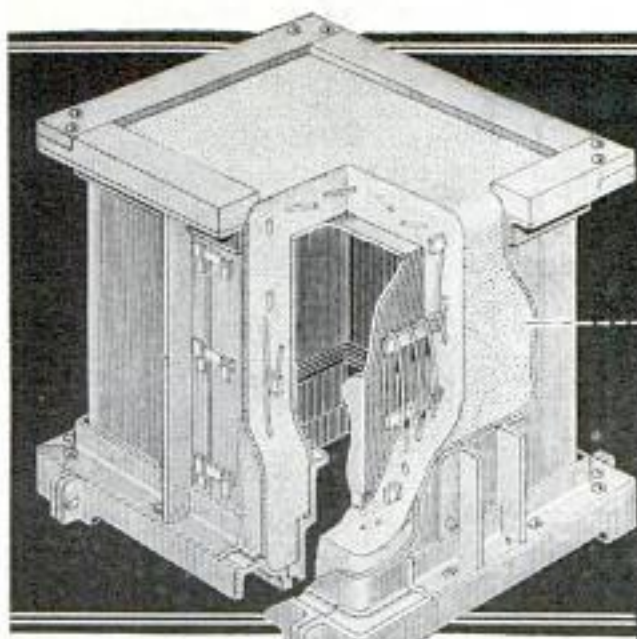
Partly Assembled Fireproof Portable Safe with Its Outside Layer of Concrete Stripped Off and One Corner in Section, to Show Details of Construction and the Reinforcement
