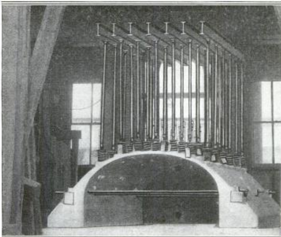
Method of Testing a Skew-Arch Bridge: Any Uniform Load is Applied by Means of the 42 Springs under the Pipes That Bear against the Overhead I-Beams. To the Right, One of These Springs is Shown Enlarged; the Tie-Rods between Abutments Are for Measuring the Thrust
