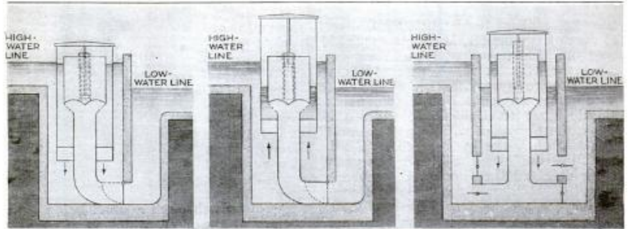
Left: New Low-Head Single-Acting Water Engine on the Down or Working Stroke. Center: Same Engine on the Upstroke. Right: Similar Engine of the Double-acting Type
