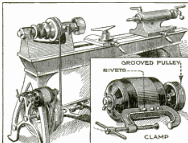
An Old Electric-Fan Motor, Attached to a C-Clamp, can be Used for Driving Any Light Machine
