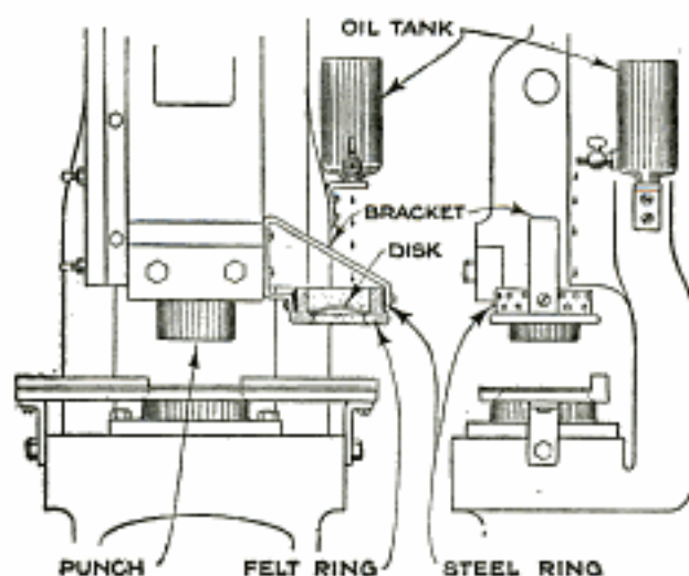
An Oiling Device for the Punching and Drawing Press, That Automatically Applies a Thin Film of Lubricant to the Face of the Stock at Each Downward Movement of the Ram
