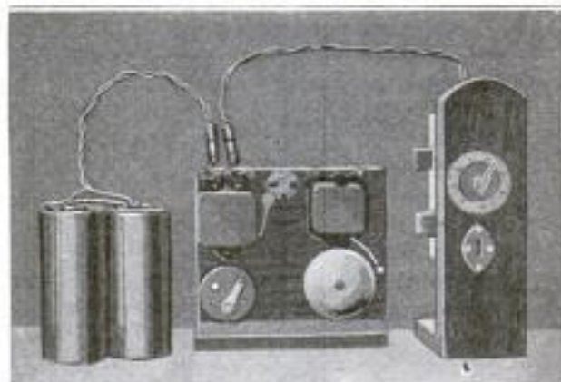
Combined Lock and Alarm, Showing the Batteries on the Left, the Alarms with Selective Switch in the Center, and Lock at the Right
