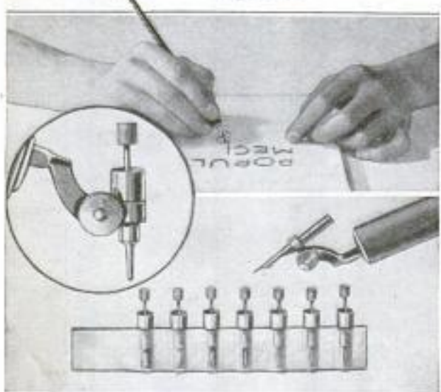
Seven Ruling Pen Points and, in Inset, One in Socket Ready for Use: To Right and Above, the Socket is Shown in Use with Ordinary Pen Point
