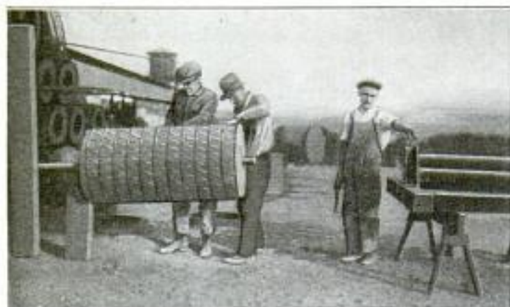
Fabricating the Reinforcing Mesh for a Section of Concrete Pipe Used on the Yuma Land Project: Raw Materials for Concrete Are Plentiful in This Region
