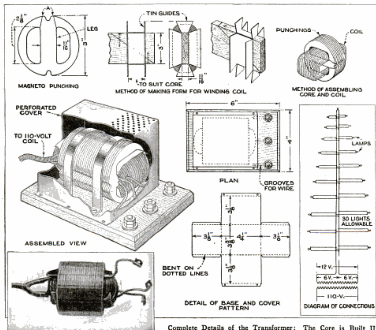
Complete Details of the Transformer: The Core is Built Up from the Discarded Magneto-Armature Punchings Shown at the Upper Left. The Insert at the Lower Left Shows the Completed Core and Coil, Ready for Mounting. A Wiring Diagram for the Lamp Cable is Given at the Right.
