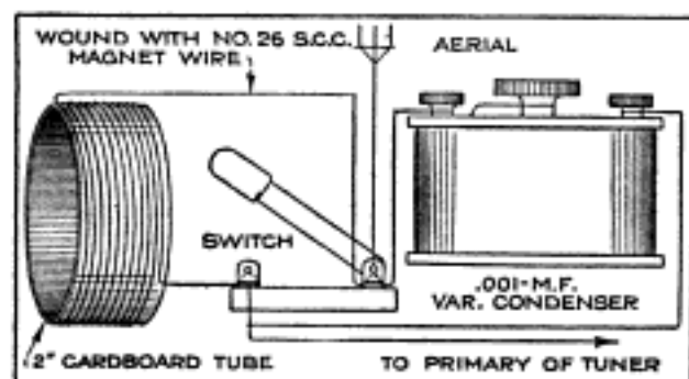
A Simple Radio-Wave Trap That will Eliminate Much Interference When Tuning the Radio-Receiving Set
