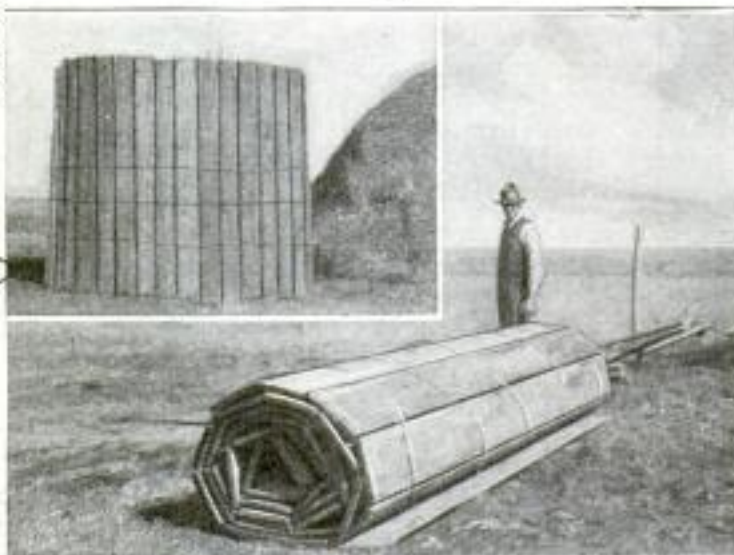
Demountable Grain Bin after being Emptied, Taken Down, and Rolled Up in Readiness to be Transported to the Storehouse: Insert Shows the Bin Set Up Ready for Use
