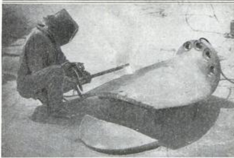
Tool in Use, Cutting Up a Propeller Blade: One Cut Is Completed and the Second Is under Way
