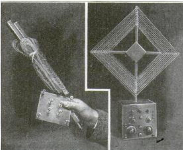
Left: Collapsed Loop Antenna of the "Reflex" Radio-Receiving Set, Together with the Metal Plate Which is Used to Hold the Loop Rigid When It is Opened. Right: Set Shown Erected in Readiness for the Reception of Broadcasting
