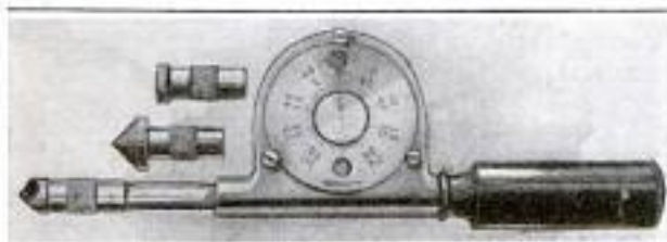
This New Speed Indicator of Simple Design Has, among Other Features, a Fiber Handle That Is an Insulation against Electricity
