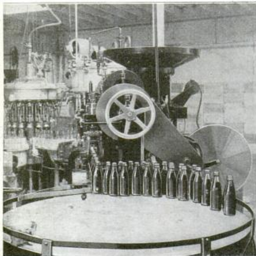
Automatic Bottle-Sealing Machine, Showing the Strip of Aluminum being Fed from the Coil at the Rear, While, at the Top of the Outfit, may be Seen the Large Hopper for the Cork or Paper Disks
