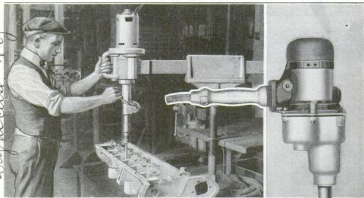
Left: Stationary Type of Screw and Nut-Setting Machine Which Handles Nuts and Screws from 1/2 to 1 Inch in Diameter, Right: Portable Screw and Nut-Setting Tool, Which will Drive and Set Nuts and Screws from 1/4 to 3/8 Inch in Diameter
