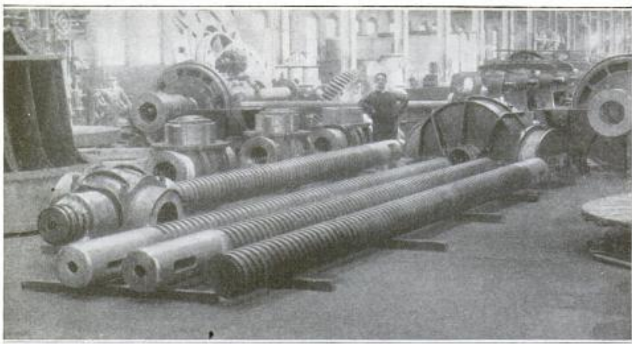
The Above are Reported to Be the Largest Luffing Screws Ever Made. Each Screw Is 15 Inches in Diameter, 28 Feet Long, and is Designed to Carry a Maximum Load of 1,000,000 Pounds; the Nut in Which It Turns, Weighs 5,000 Pounds
