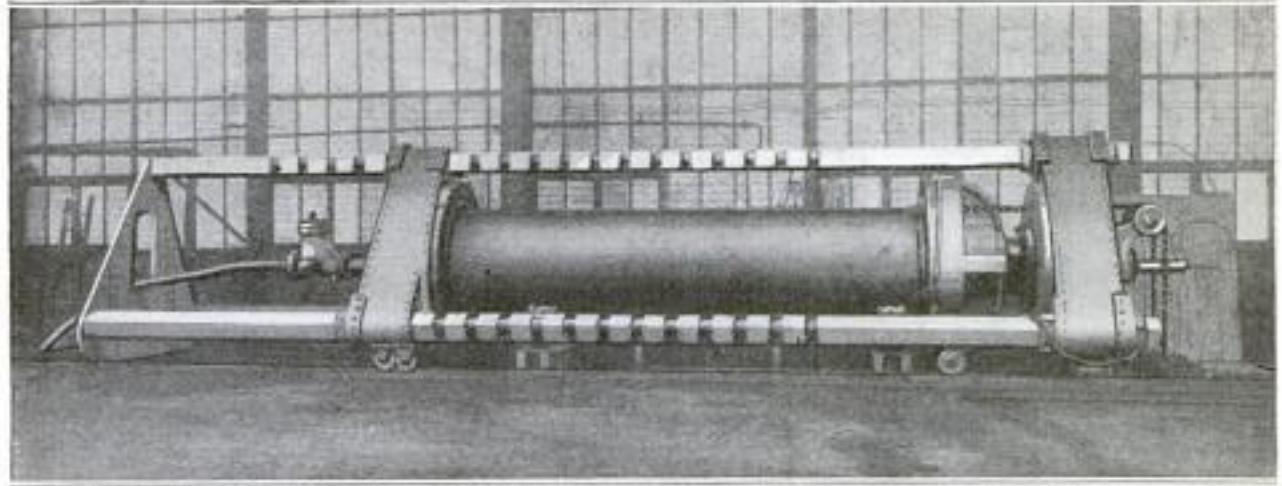
Hydraulic Testing Machine for Large Welded-Steel Pipes, Built in England, Where These Pipes Are in Extensive Use in Water Mains: The Pipe Shown under Test Is 16 Feet 6 Inches Long, 48 Inches in Diameter, 1/2 Inch Thick, and is being Tested at a Pressure of 260 Pounds per Square Inch
