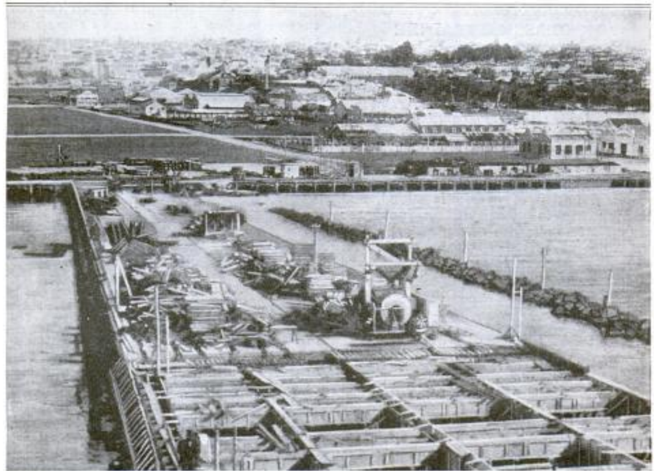
One of the New Reinforced-Concrete Wharves under Construction, That will Form Part of the Harbor Extensions at Auckland, New Zealand: These New Wharves Are 240 to 280 Feet Wide; along the Shore can be Seen Part of the Stone Wall Erected in Connection with the New Embankment
