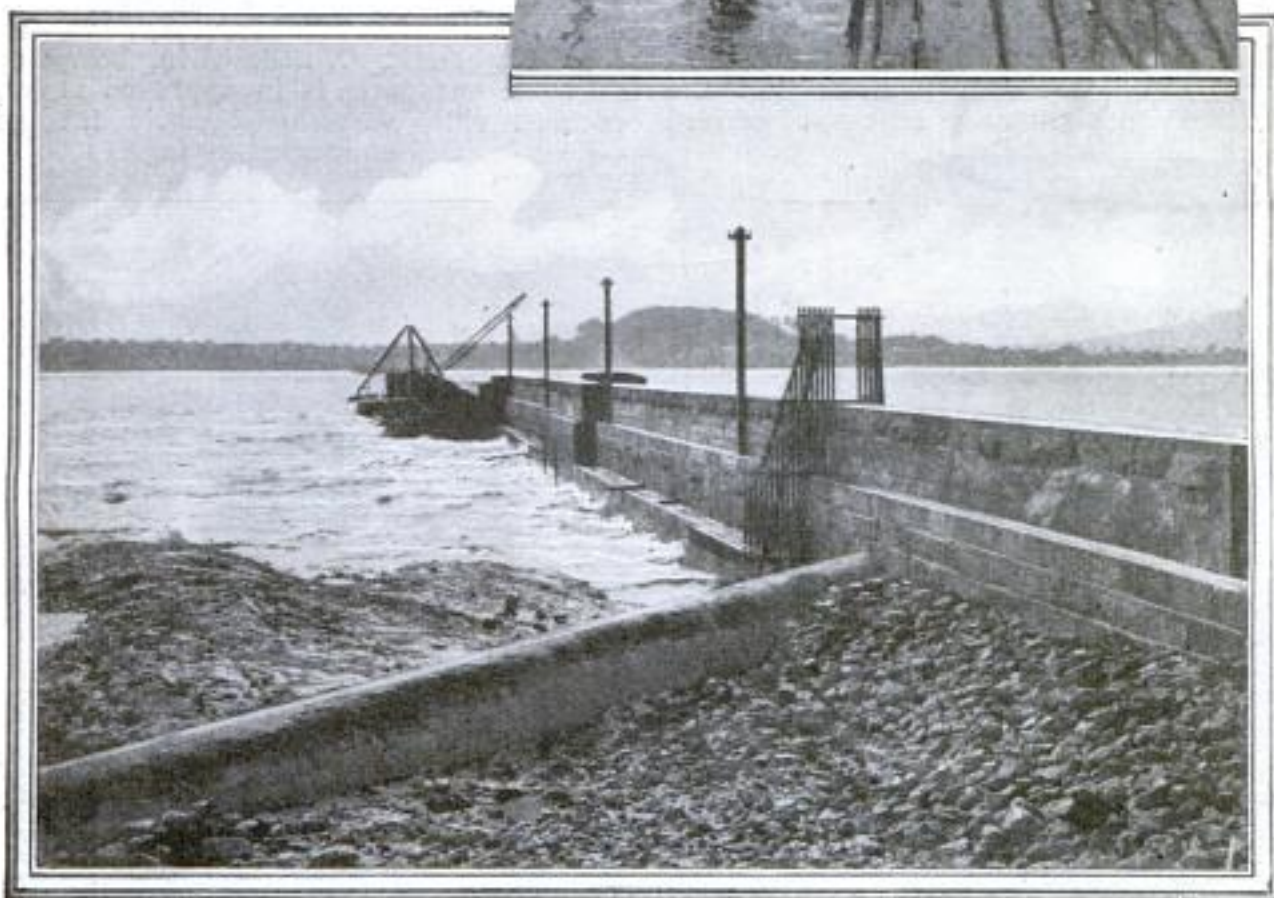
Above: Traveling Concrete Mixer at Work on One of the New Wharves in Connection with the Harbor Extensions at Auckland, New Zealand. It is Used for Making the Concrete Piles for the Wharf. Right: Part of One of the Reinforced-Concrete Wharves, Showing the Quay Side, with Its Railway Lines, and One of the Large Electric Traveling Cranes. Beside the Quay is Seen Part of One of the Two-Story Steel Cargo Sheds Which Are 320 Feet Long and 60 to 80 Feet Wide. Below: Concrete Pier Built to Act as a Tide Deflector in Connection with the New Harbor Extensions
