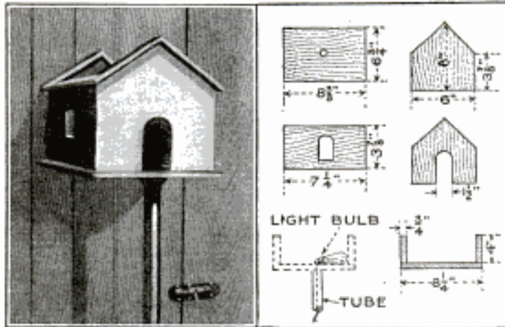
Two of These "Bird Houses" were Used as Indirect-Lighting Fixtures on a Porch, to Provide a Soft Light
