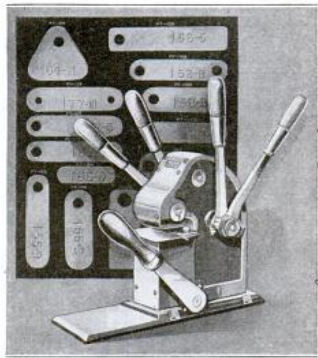
This Metal-Tag Marker Embosses the Entire Number at One Operation, Resulting in a Better Job, as Well as in Saving of Time and Labor
