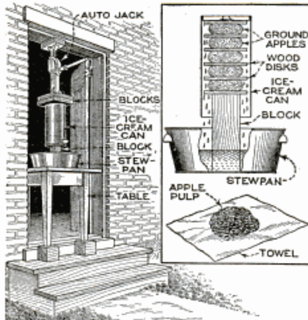
A Simple Cider Press That can be Improvised from Materials Found around the Average Household, or Easily Obtainable
