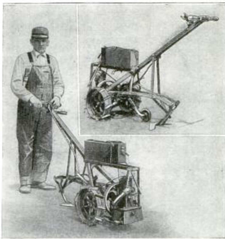
Front and Rear Views of Small Garden Tractor: This Is a Compact Little Machine That Is Capable of Hard Work
