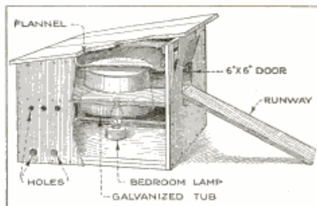
A Comfortable Brooder for Young Chicks: It can be Made in a Few Hours from Material at Hand on Any Farm
