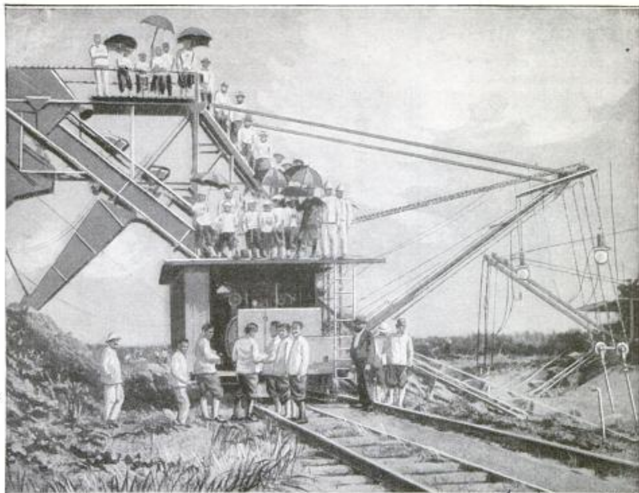
MODERN ROAD-BUILDING EQUIPMENT ADOPTED BY SIAM International
