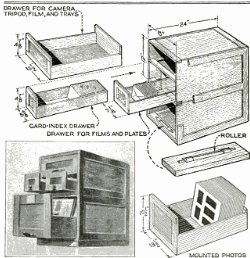
An Excellent Cabinet for Filing Prints, Negatives, and Other Photographic Matter: It Has a Subject Index, Referring to the Numbered Photographs and Negatives, and Space for the Camera, Tripod, and Developing Trays
