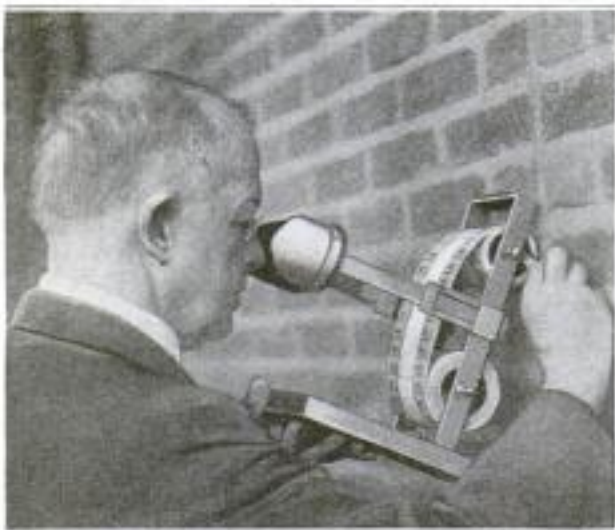
Simple Device That Aids Motion Study of Workers and Machines, Photographed by a Stereoscopic Moving-Picture Camera
