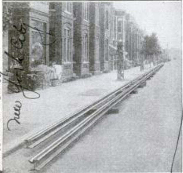
Rails, 420 Feet Long, Made by Welding Together Standard Lengths: They were Laid as Units
