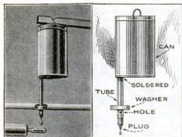
Simple Drip Can for Supplying Oil and Cutting Compounds to Taps in a Tapping Machine, Using Improved Supply-Regulating Valve
