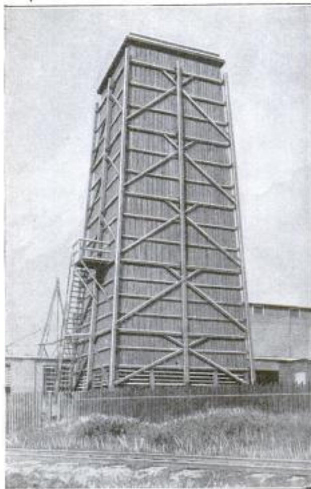
Ice-House Condenser Built of Creosoted Timber: It Is 32 Feet Square at the Open Lattices of the Base, 78 Feet High, and 27 Feet Square at the Top
