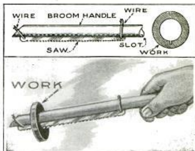
A Simple Tool for Sawing Internal Slots in Washers or Sleeves, Made from a Piece of Broomstick
