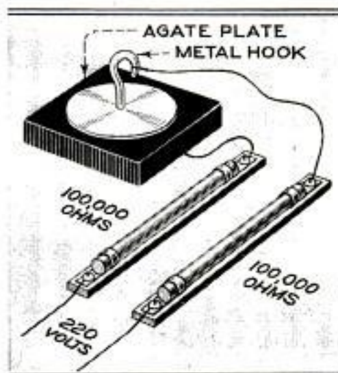
Crude Apparatus Which Constituted the Experimental Working Outfit: A Very Small Current Suffices to Produce the Nonmagnetic Attraction
