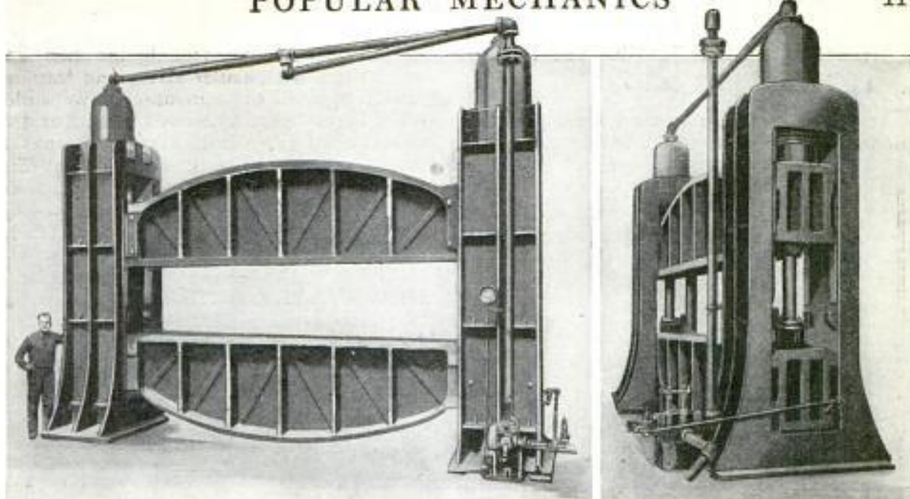
Left: Hydraulic Flanging Press from the Front, Its Immense Size Illustrated by Comparison with a Man's Height. The Controlling Hand Lever may be Seen under the Gauge. Right: End View of the Press, Showing the Huge Cylinders at the Top, with the Smaller Ones and the Poppet Valve Below
