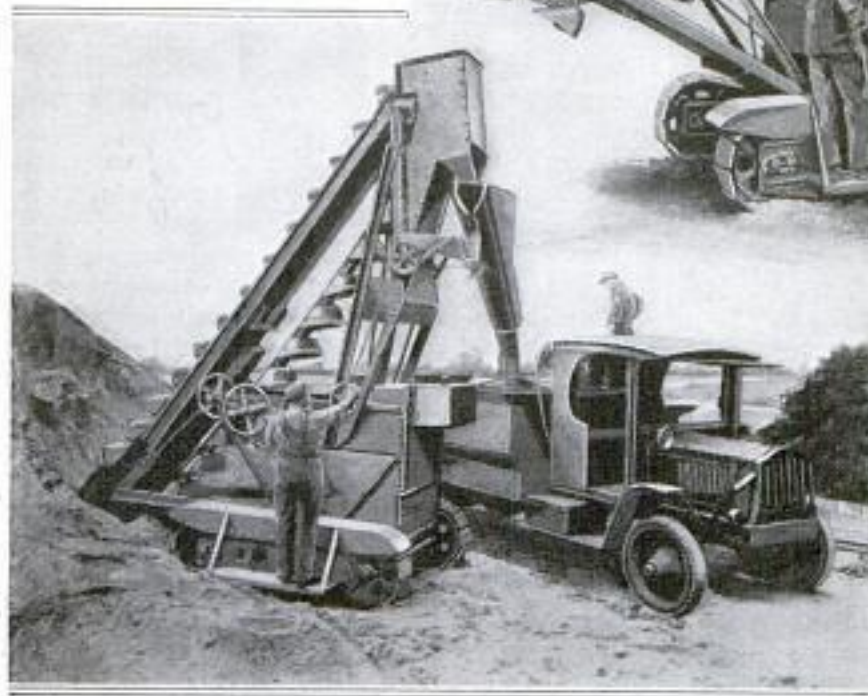
Portable Loader Shown Digging into a Pile of Material and Loading It from a Height of 9 Feet 6 Inches into a Motor Truck
