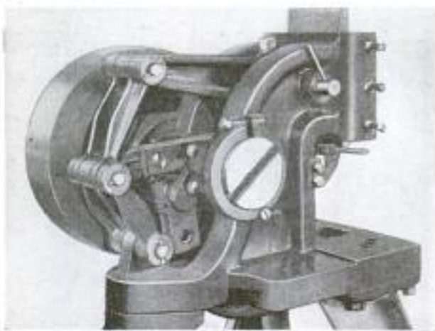
Combination Punch Press: By Changing the Position of the Bolt with the Slotted Head, the Press can be Operated Either by Foot or by Power
