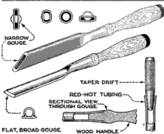
Steel Tubing, Used to Make Woodworkers' Gouges of Various Shapes and Sizes, and of Excellent Quality
