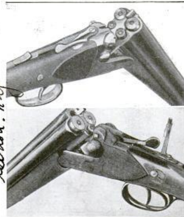
Above: Gun with Two Shotgun Barrels above Two Rifle Barrels. Below: Two 12-Gauge Barrels with a Rifle Barrel Above and Below
