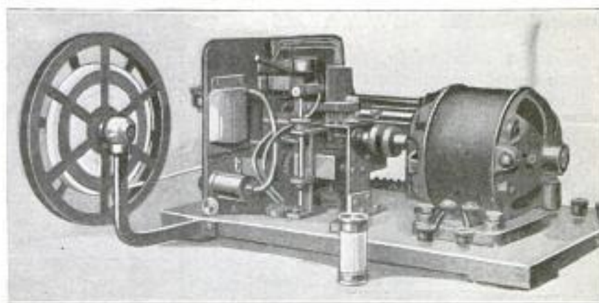
Rapid-Telegraphing Machine Which Prints from 400 to 2,000 Letters a Minute and Which is Based on the Phenomenon of Attraction between a Metal Disk and a Tinfoil-Covered Agate Plate
