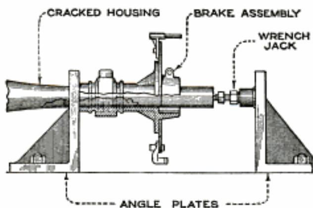
A Small Wrench Jack and Two Angle Plates Used to Force a Cracked Axle Housing from the Brake Assembly
