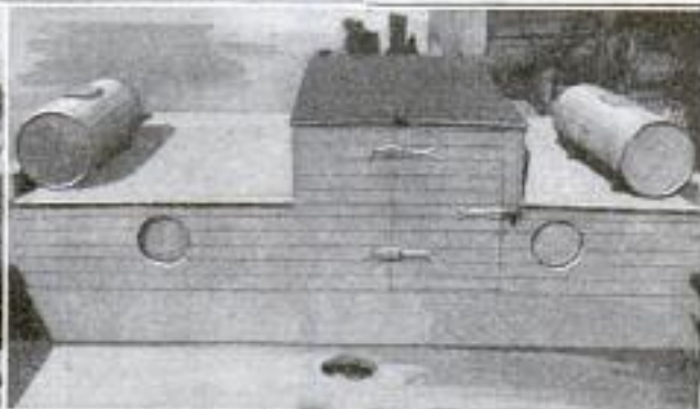
Above: Close-Up of the Deckhouse in the Center of Which the Two Engines are Located. Left: Hole in Deck through Which Grappling Chains are Operated
