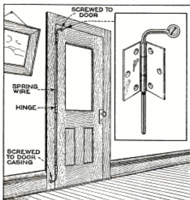
A Practical Spring That Is Neat in Appearance, and can Easily be Attached to Any Door
