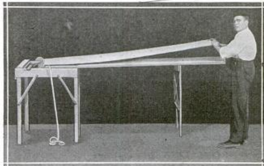
New Machine Which Trims the Selvage with a Revolving Cutter, Applies the Paste, and Wipes the Surplus from the Wallpaper as the Sheet is Pulled through the Rollers: It is Said to Have a Capacity of One Roll of Wallpaper in Three Minutes
