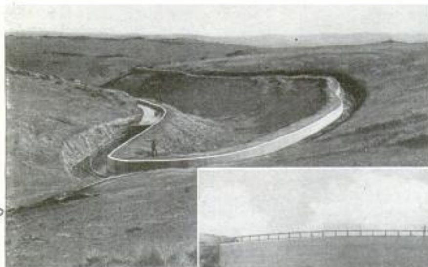
Bird's-Eye View of Concrete Irrigation Dam, Showing Its Outline, Curved with a Radius of 185 Feet, and 450 Feet Long, or Nearly a Complete Semicircle
