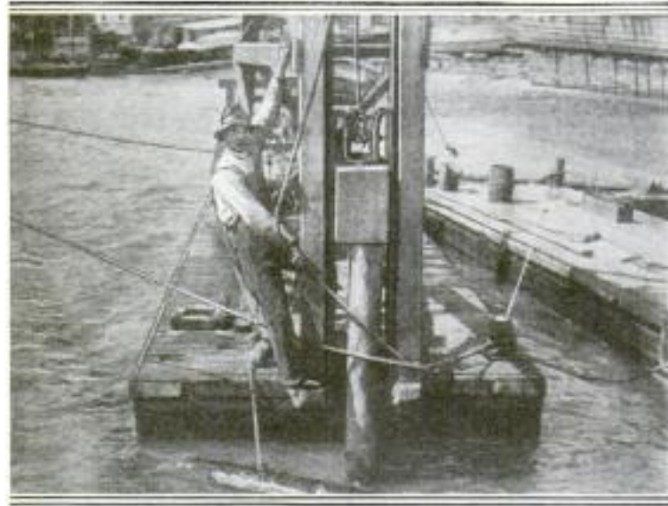
The Small Floating Pile Driver Operated by Percy Bagley: The Hammer Was Once the Counterweight of an Elevator. This 700-Pound Weight Now Easily Sinks a 10-Inch Pile
