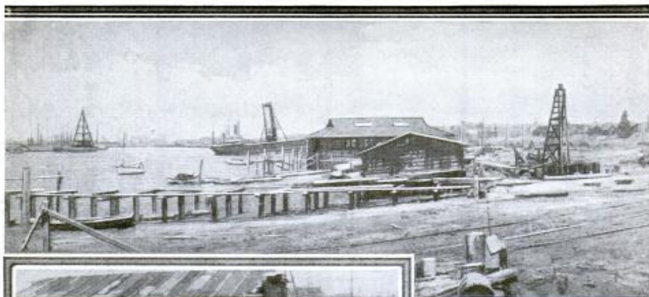
Above: A Partial View of the Bagley One-Man Shipyard from the Water's Edge, Showing the Pier, the Small Floating Pile Driver, and Several of the Portable Buildings of the Plant. In the Foreground a Portion of the Tracks of the Marine Railway can be Seen. The Shipyard Represents the Industry of a Father and Two Sons
