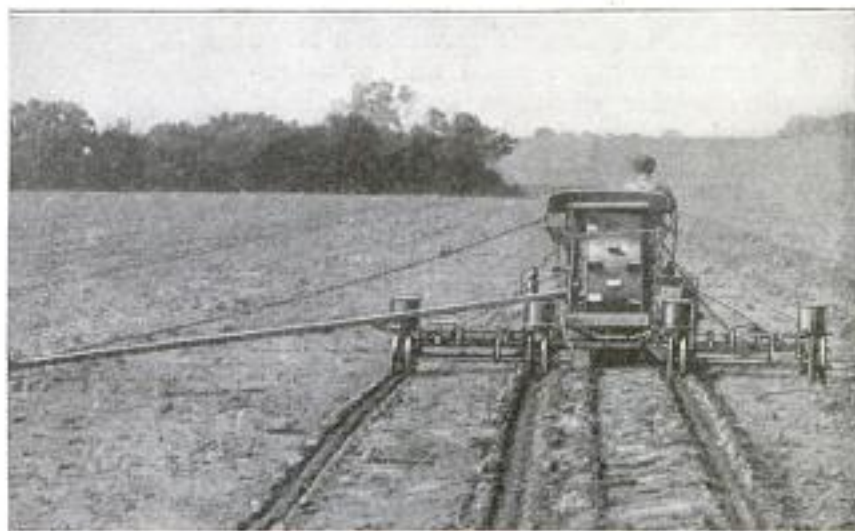
Corn Lister Which Plants Four Rows at One Time: The Speed of This Machine, When Crosschecking is Eliminated, may be Greatly Increased over That Obtained When Using an Ordinary Planter
