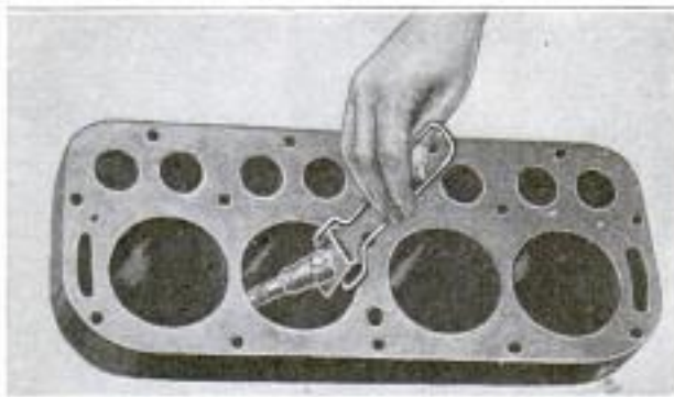
Self-Alining and Centering Inside Micrometer Gauge being Used to Measure the Bore of a Cylinder: The Small Setscrew Is for Locking It before Removal
