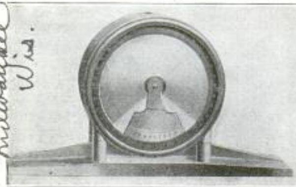
Inclinometer Which Gives Readings in Degrees and Minutes, Showing the Pendulum That Automatically Indicates the Angle of a Surface
