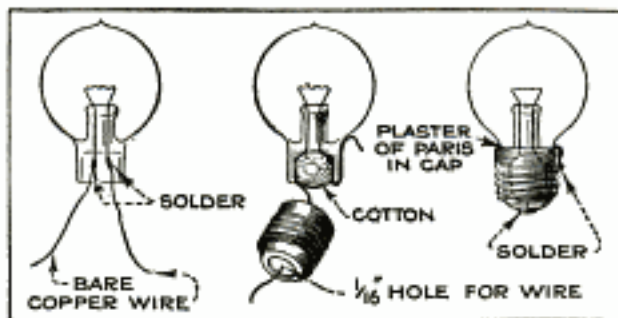
A Simple Method of Repairing Electric Lamps When the Brass Screw Caps Are Loose
