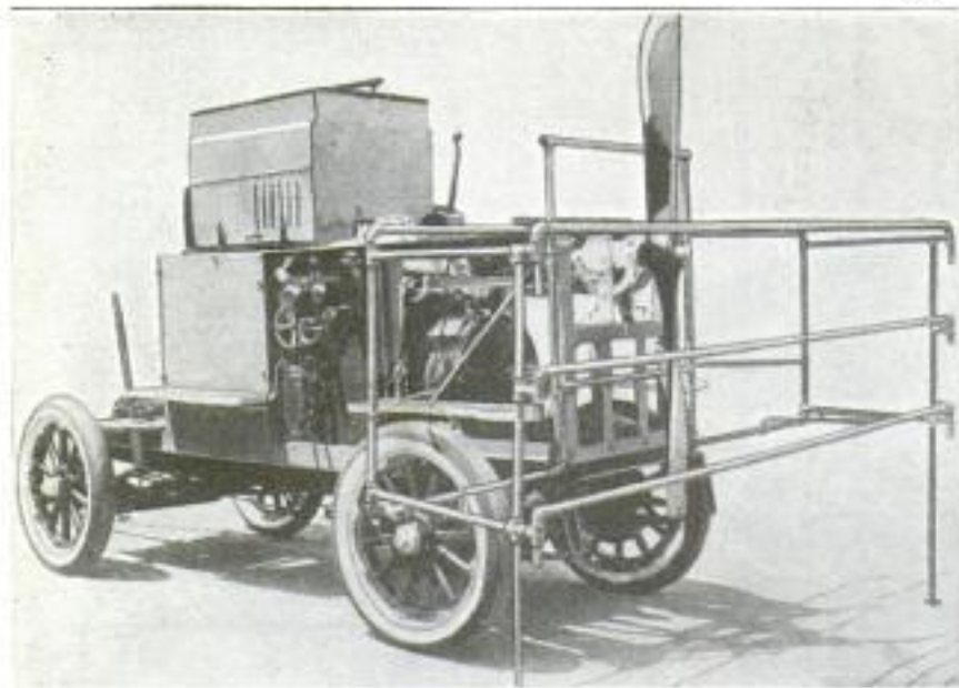
"Storm Machine," Showing the Box Containing the Arc Lights on Top, the Switchboard below This, While in Front are Seen the Generator and Propeller, with a Guard Rail around the Latter
