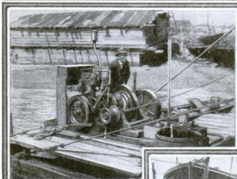
Above: A Partial View of the Bagley One-Man Shipyard from the Water's Edge, Showing the Pier, the Small Floating Pile Driver, and Several of the Portable Buildings of the Plant. In the Foreground a Portion of the Tracks of the Marine Railway can be Seen. The Shipyard Represents the Industry of a Father and Two Sons
