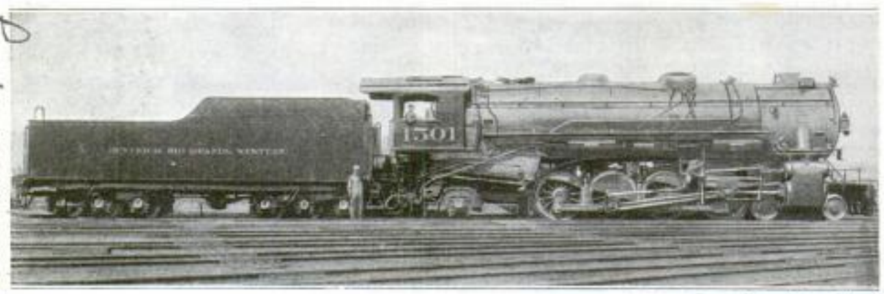
This is One of a Number of Similar Locomotives Which are the Largest and Most Powerful, of the Simple Engine Type, Ever Built for Passenger Service. It has a Drawbar Pull of 66,600 Pounds, and is Equipped with Automatic Stokers for Burning Soft Coal
