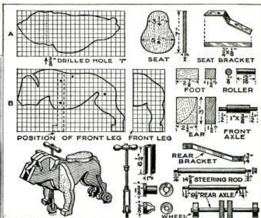
A Novel Push Car, Constructed and Painted to Resemble a Bulldog: It can be Made at Slight Expense, and will Provide an Endless Amount of Enjoyment for the Small Boy. The Body is Laid Out by Means of the Patterns Given
