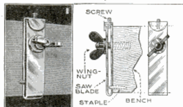
A Miniature Vise, Made from a Machine-Hacksaw Blade, for Holding Small Screws
