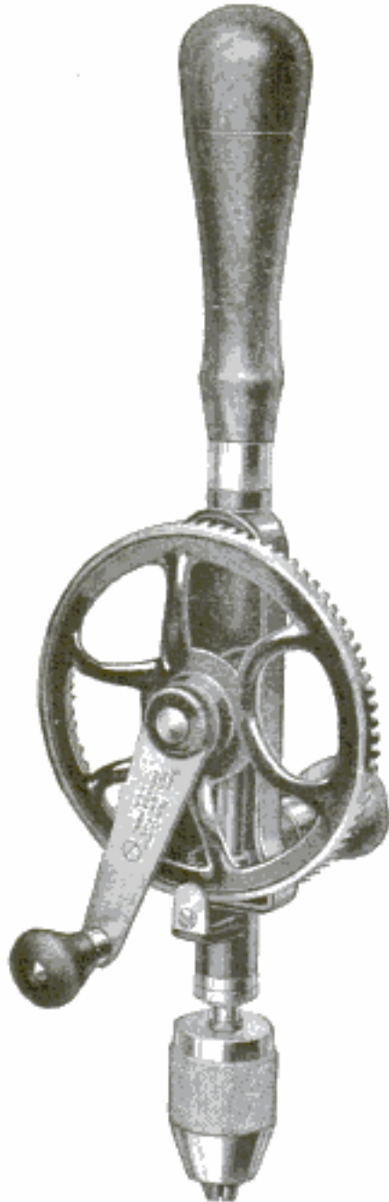
HAND DRILL No. 1515 Price $4.80 This is a single speed drill. It has a screw cap containing 8 tool steel drills, 1/16 to 1/64 inch.
