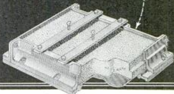
The Door of the Safe with Parts Cut Away to Show Its Construction: As Indicated by the Arrow, the Finished Door is Shown Immediately Above It, in the View of the Completed Safe
