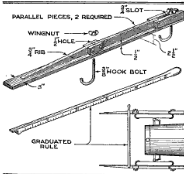
Truing Up the Front Wheels of an Automobile Is Not Usually a One-Man Job, but the Device Illustrated Above Makes It So
