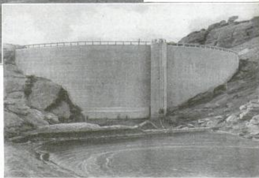
Front Elevation of Semicircular Concrete Dam, 90 Feet High above Ground and 23 Feet Deep below It: At the Ground Level It Is 25 Feet Thick
