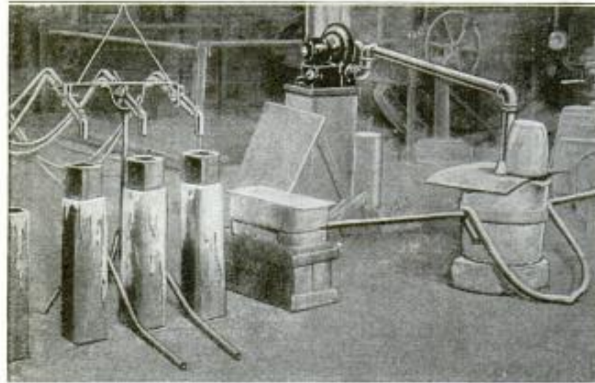
Left: Arrangement of Heaters for Ingot Molds to Reduce Amount of Scrap Cut Off. Right: Air-Gas Blower Used to Dry the Ingot Molds and Ladles
