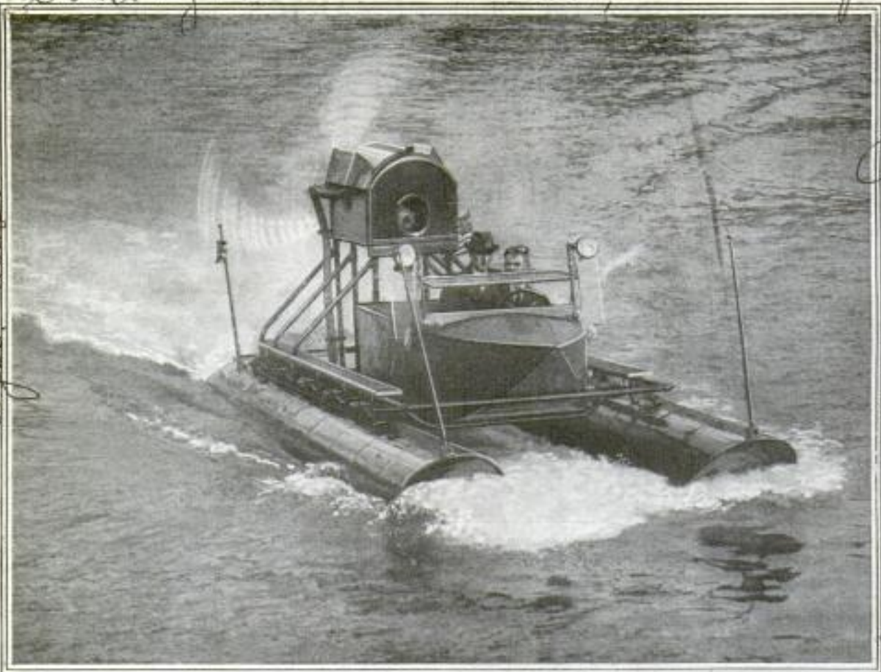
This Hydroglider, Built by an American Youth, Draws Only 1½ Inches of Water at a Speed of 45 Miles an Hour, and is Equipped with a Six-Passenger Automobile Body
