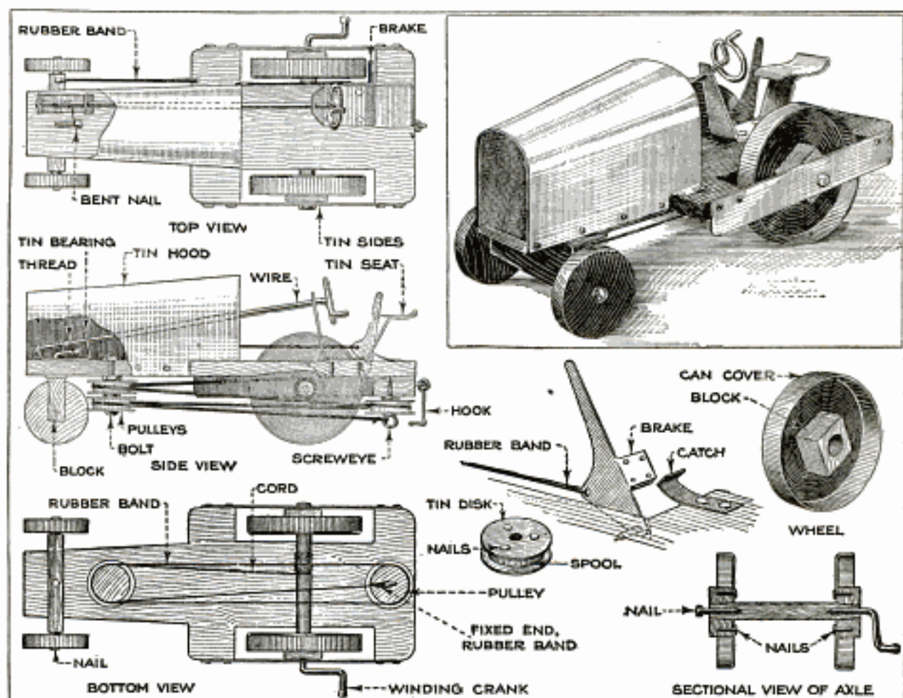
A Simple Rubber-Band Driven Toy Tractor That will Provide Much Amusement for the Little Folks: It can be Made Quite Realistic in Appearance, will Run 15 to 20 Feet on One Winding, and, If a Strong Band is Used, will Draw Small Trailers
