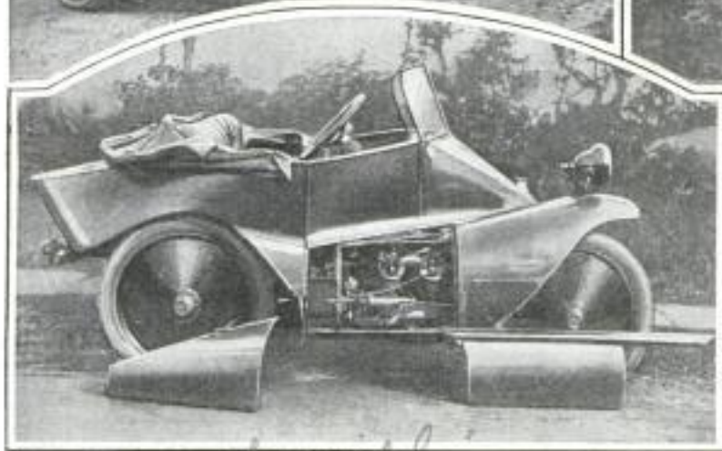
The illustration above and to the left gives a good idea of the mobility of the car. By noting the lines made in the roadway it is seen that the car is able to turn completely around with the third wheel remaining practically in a fixed position. Above: Rear view of the car, showing luggage compartment, collapsible top, and controlling mechanism. Below, left: Removable section taken out, showing the easily accessible motor, a 10-horsepower two-cylinder design
