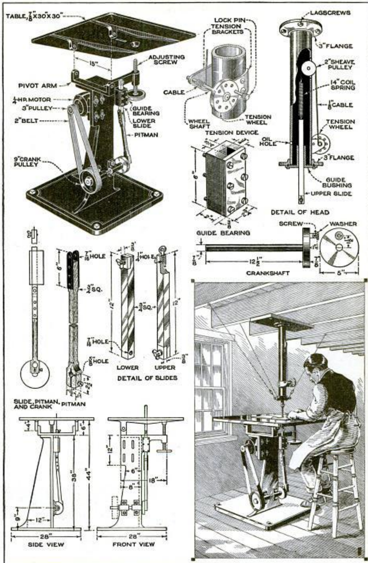
This Jig Saw will Prove to Be a Valuable Addition to the Equipment of Any Small Woodworking or Pattern Shop, as a Great Variety of Work can be Turned Out with It. It is So Designed That Many of the Objectionable Features of Older Models are Eliminated
