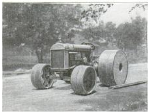
Small Gas Tractor That was Converted into a Road Roller by Substituting for Its Ordinary Traction Wheels Golf-Course Wheels Filled with Cement
