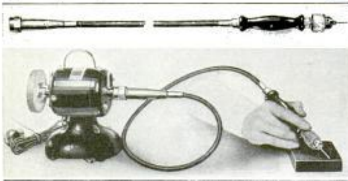
Jewelers' and Die Sinkers' Flexible-Shaft Outfit with Light Sheath and Cable: The Handle Chuck Has a Capacity up to One-Eighth Inch. A Heavy Sheath and Cable is Shown Above
