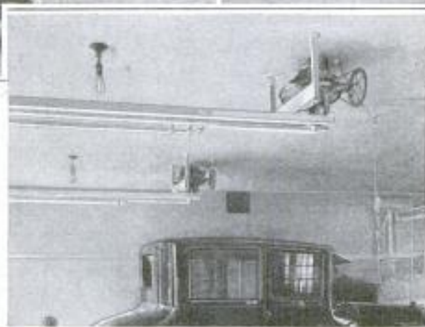
Interior of the Garage, Showing, Suspended from the Ceiling, Two Motors and Housings for the Gears That Operate a System of Levers for Opening the Doors: The Control Switches Are inside the Garage
