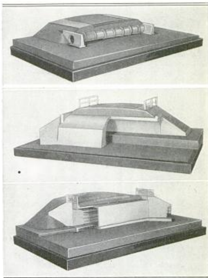
Models of Various Types of Road Construction for Engineering Schools: Top: Model Illustrating Concrete-Pipe Culvert Construction. Center: Model of Concrete-Arch Type of Culvert. Bottom: Model of Box Form of Culvert Construction
