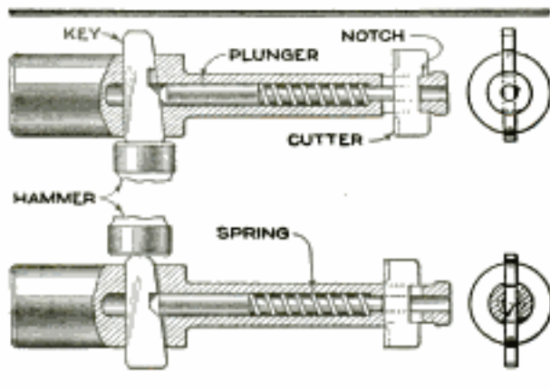
An Efficient Counterbore That Has No Loose Parts to Drop Out: This Tool is Designed for Spot-Facing, or Counterboring, the Underside of Drilled Holes relieved, making it easily removable.—Galen D. Watson, Bath, Me.
