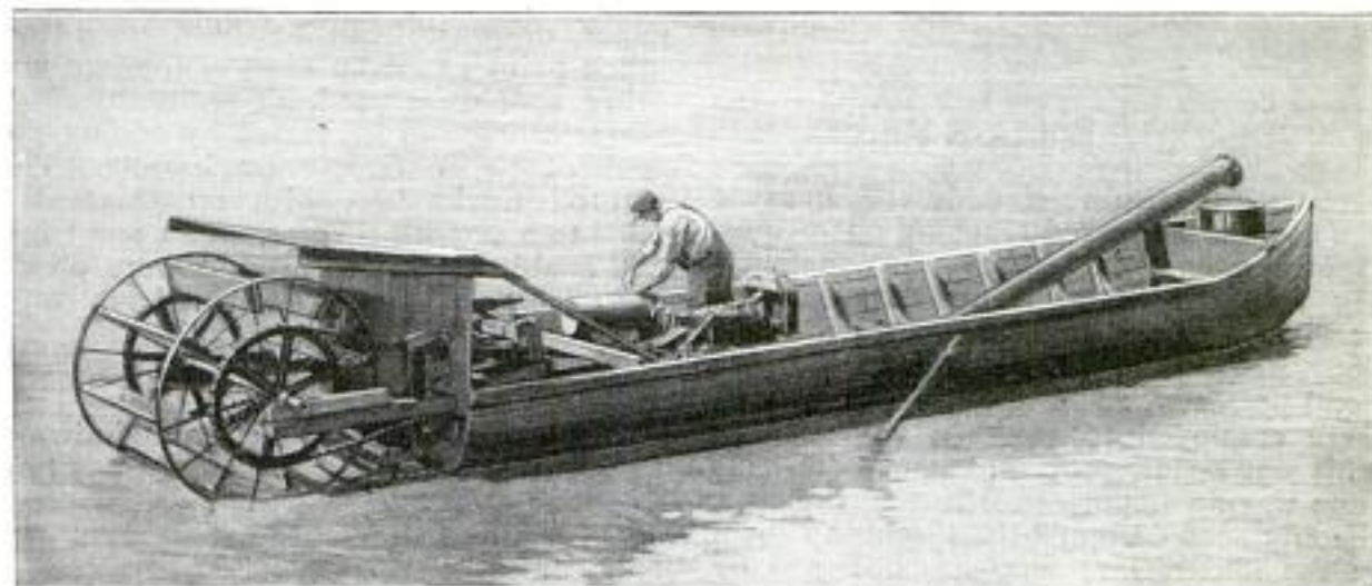
A Homemade Paddle Boat, Fitted with an Engine Taken from a Popular Car, Transports Men and Materials to the Piers of a New Bridge over the Missouri River. The Stern Wheel is Made by Bolting Boards to a Pair of Old Cultivator Wheels
