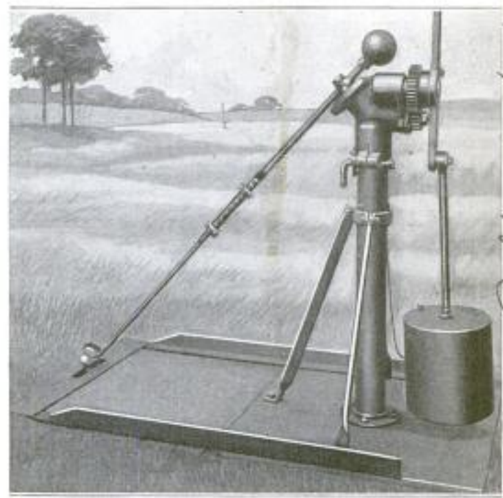
The Above Machine has been Designed to Test Golf Balls under Conditions to Which They are Subjected in Actual Play. The Length and Force of Stroke are Adjustable
