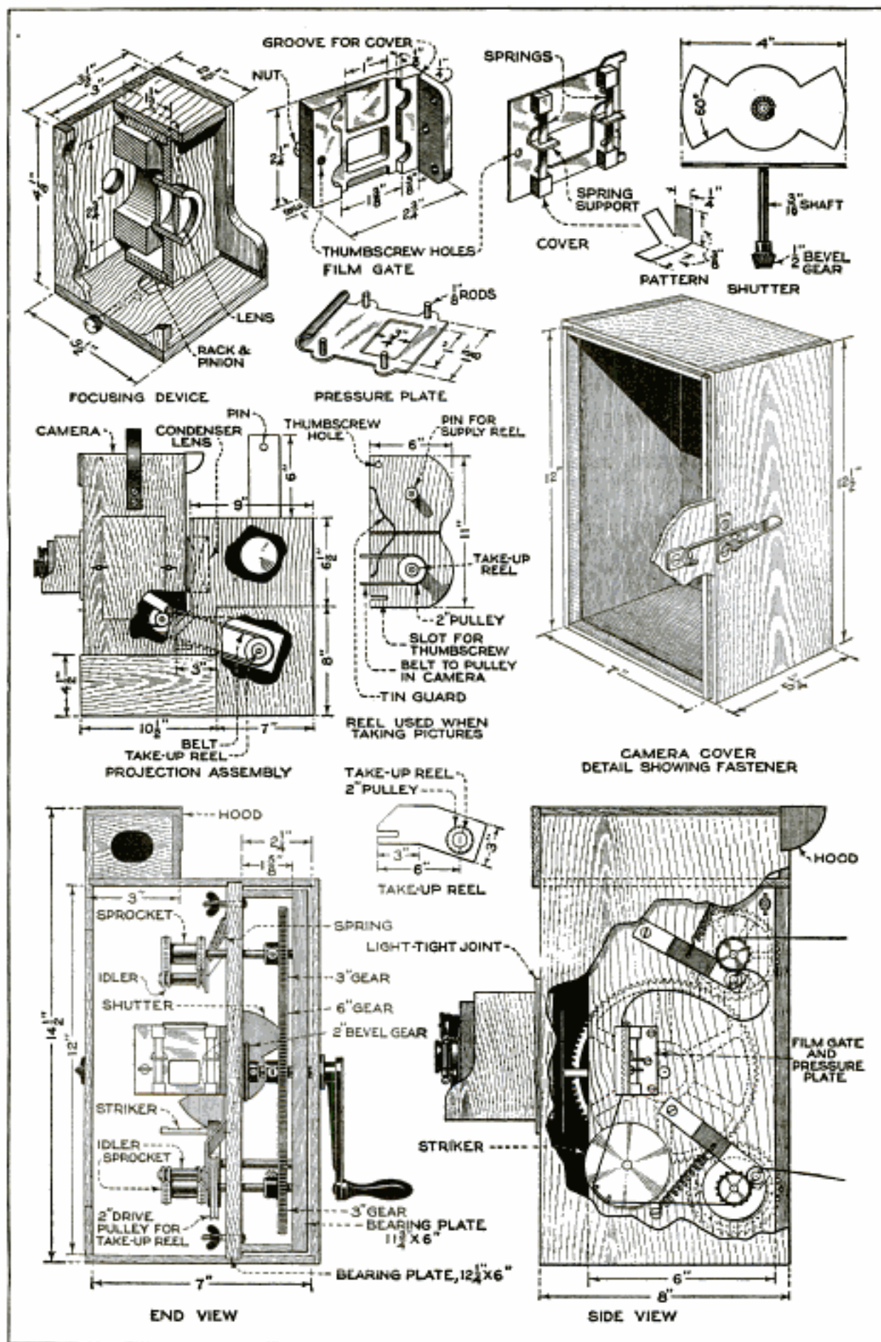
Complete Details of the Motion-Picture Camera and Projector: Upper Drawings Show the Construction of the Focusing Device, Film Gate, and Shutter; Center Drawings, Projection Apparatus, Picture-Reel Plate, and Camera Cover, and Lower Drawings, Side and End Views of the Camera Completely Assembled
