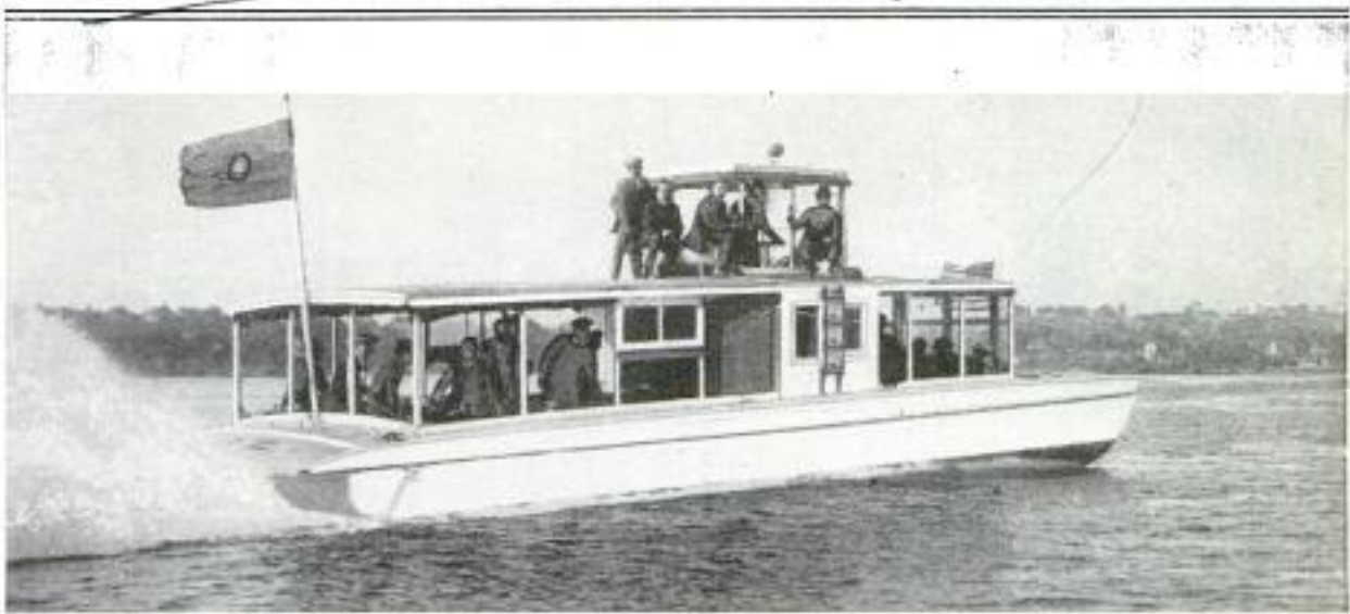
First of a Fleet of Seasleds That are being Built for Service on the Shallow Rivers of Colombia, South America: The Boat Has Accommodations for 20 Passengers and Their Baggage
