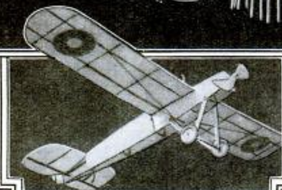
Toy Airplane, with a Wing Spread of 3\frac{1}{4} Feet, Shown Assembled in the Bottom View: Center View Shows Its Parts, and Upper View Shows the Plane Complete without Its Covering
