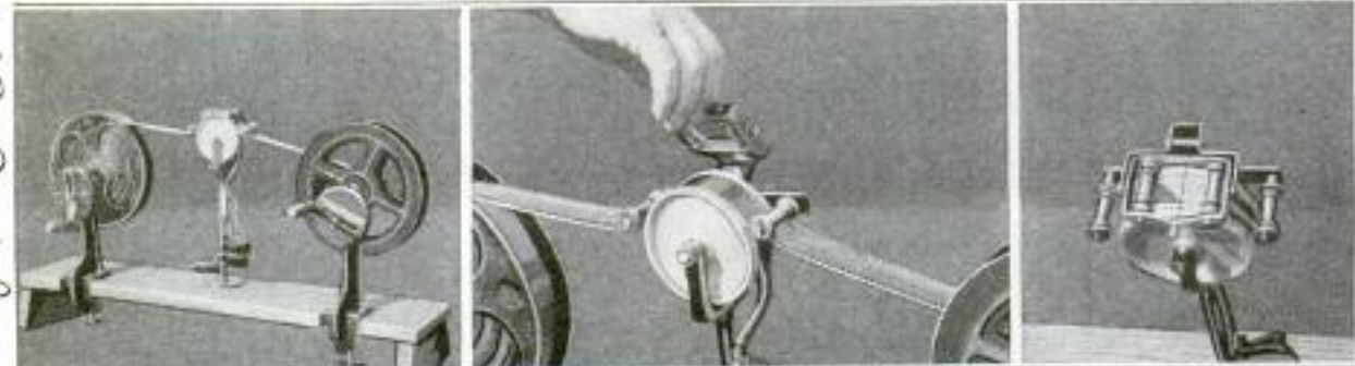
From Left to Right: The Misframe Detector Shown Mounted between the Two Film Reels; the Operator in the Act of Lowering the Clamp That Holds the Film in Place; Looking Down upon the Detector, Showing the Small Rollers That Guide the Film, and the Light from the Tiny Lamp Below
