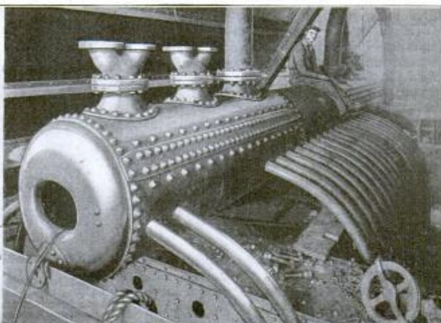
Left: Diagram Illustrating Toggle-Suspension Hangers, Which Permit a Total Play of 1\frac{1}{2} Inches to Take Care of Drum Expansion. Right: Immense Steam-Collecting Drum of Boiler, Rated at 2,650 Horsepower
