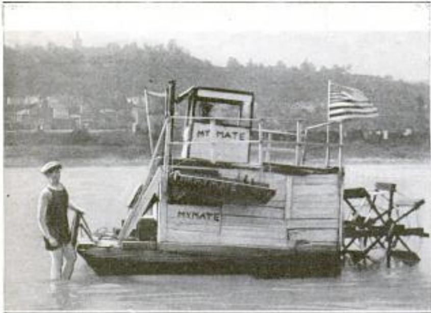
Man-Propelled Homemade Stern-Wheeler for Use around Bathing Beaches during the Summer: The Driver Sits at the Stern of the Boat and Rotates the Paddle Wheel with His Feet
