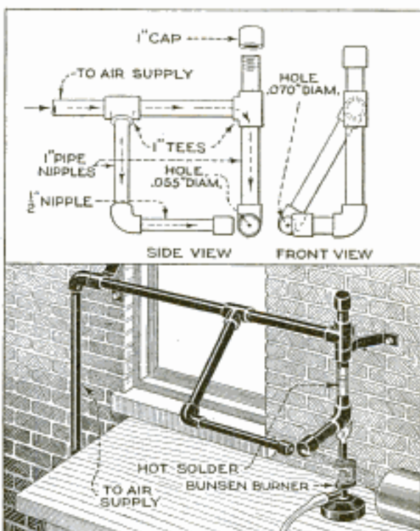
A Simple Device, Made of Pipe and Fittings and Using Air, to Pulverize Melted Solder, Which may be Used to Make Self-Fluxing Solder
