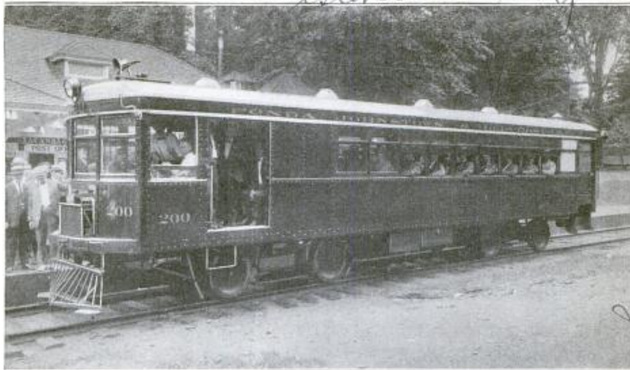
One of Two Gasoline Passenger Cars in Service on the Fonda, Johnstown & Groversville Railroad: The Car is Built of Steel and is Fitted with Air Brakes, Electric Lights, and All Standard Equipment. The Four Wheels of the Front Truck are Driven by a Powerful Engine of the Automobile Type
