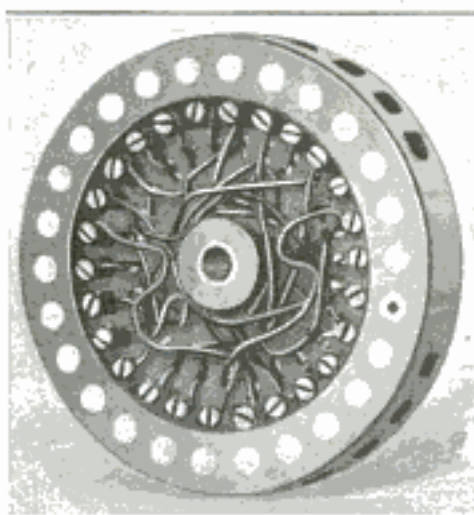
The Key, or "Master Wheel," of the New Coding Machine, and Its Intricate Electrical Wiring, in Which Lies the Secret of the Instrument
