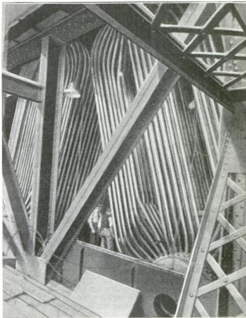
A Partial View of the Nest of Tubes Which Constitutes Most of the 26,470 Square Feet of Heating Surface of the World's Largest Boiler: If All the 3¼-Inch Tubing in This Boiler were Placed End to End, It would Form a Tube Nearly Six Miles Long
