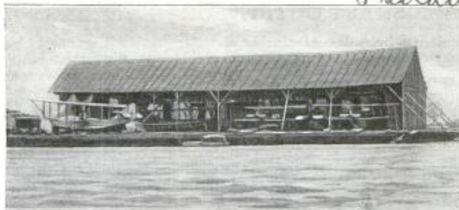
Hangar in Canton, China, Built Entirely of Bamboo, to House Four Large Seaplanes: The Poles are Notched Together, and the Framework Has a Grass Covering
