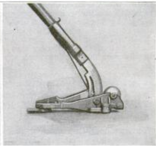
Left: With This Car Pusher One Man can Start and Keep in Motion Four Loaded Cars. It is Operated by Working the Lever Up and Down. Right: Close-Up of Car Pusher Which Automatically Grips the Rail and Has an Adjustable Fulcrum
