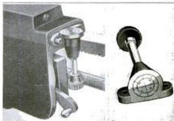
Left: Threading Dial Shown Attached to the Carriage of a Lathe. Right: Enlarged View of the Attachment, Showing the Dial That Guides the Operator
