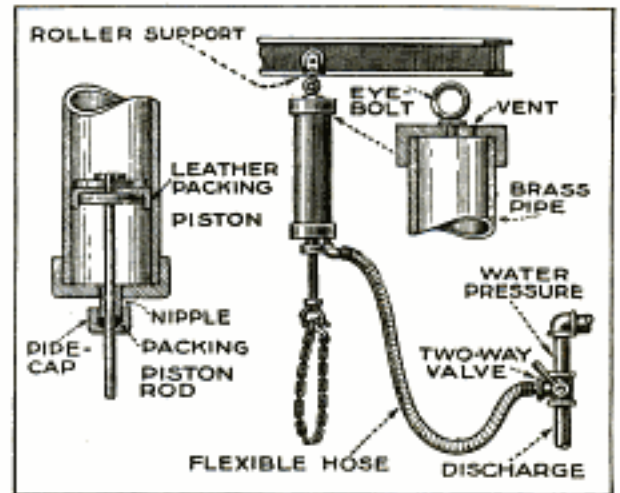
A Hydraulic Hoist for the Shop or Garage for Lifting Heavy Weights and Parts: The Whole Device can be Made from Standard Pipe and Fittings
