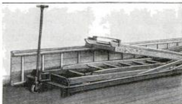
Above: Portable Scaffold Collapsed, Showing Steering Handle and Wheel. Right: Scaffold Shown Solidly Erected, Ready for Use
