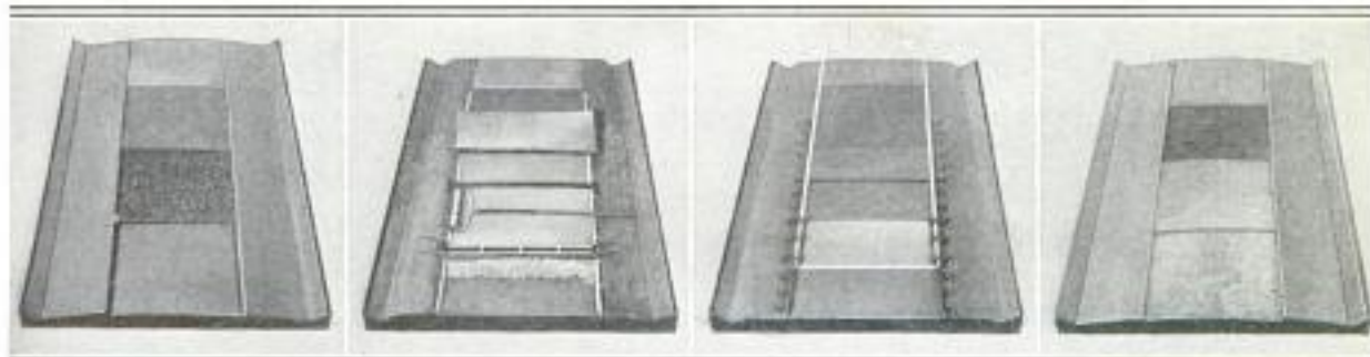
Models Showing the Elements of Four Different Types of Roadbed Construction, Made for the Instruction of Students in Highway Engineering: From Left to Right, Plain Gravel Road; Solid-Concrete Road; Paving Brick Laid on Concrete Base, and Macadam Base Surfaced with a Bituminous Material
