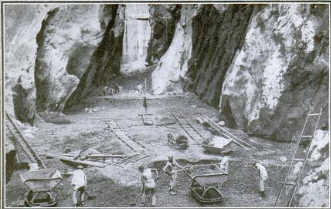
Clearing the Débris of Centuries from the Bed of the Fier River, So as to Provide a Firm Footing for the Dam at That Point: In Sinking the Caissons, Cement was Injected into the Gravel in Some Places
