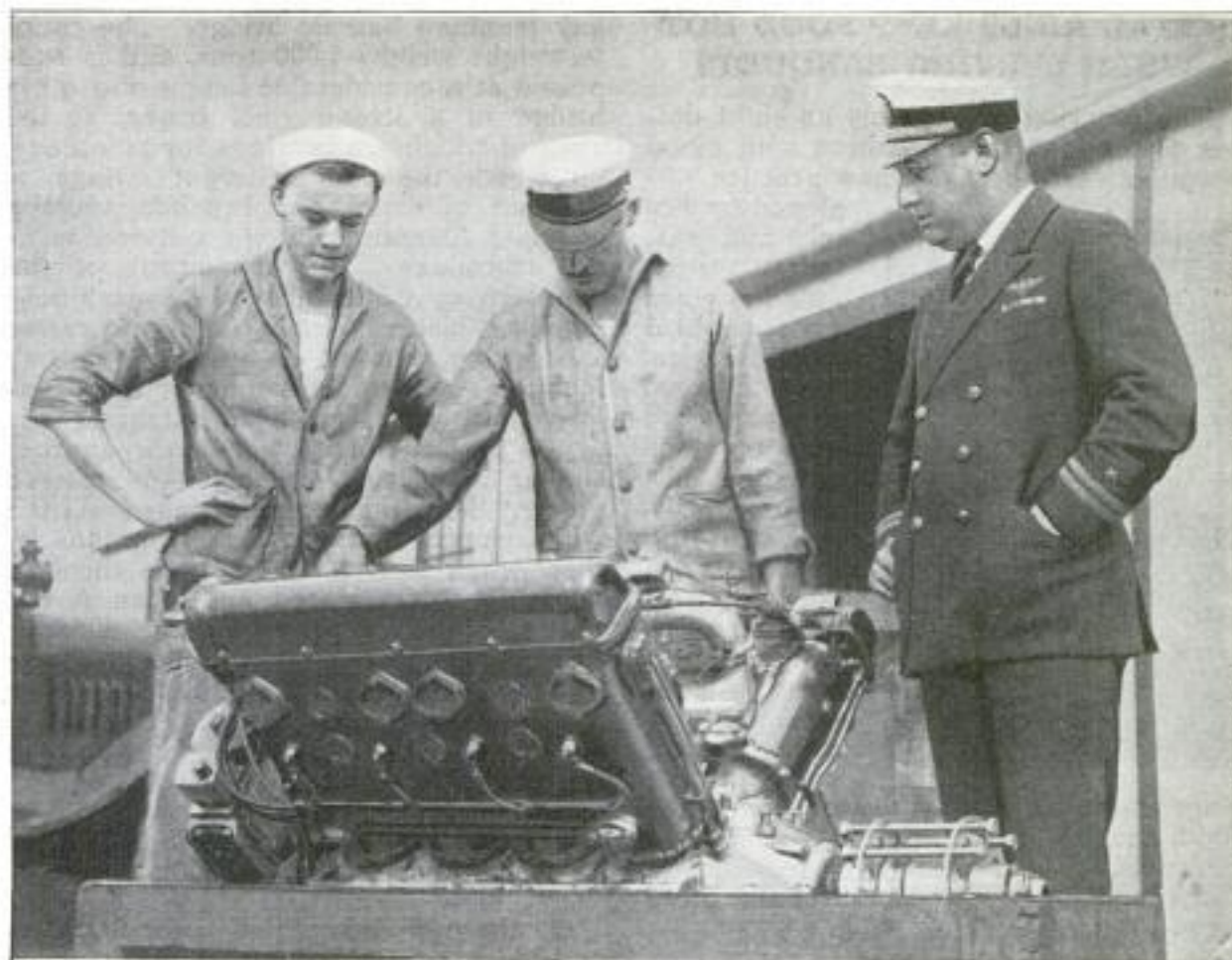
New Eight-Cylinder Air-Craft Engine Recently Tested by the Naval Bureau of Aeronautics: After a Total Run under Load Lasting 300 Hours, the Engine was Found to Be in Perfect Condition
