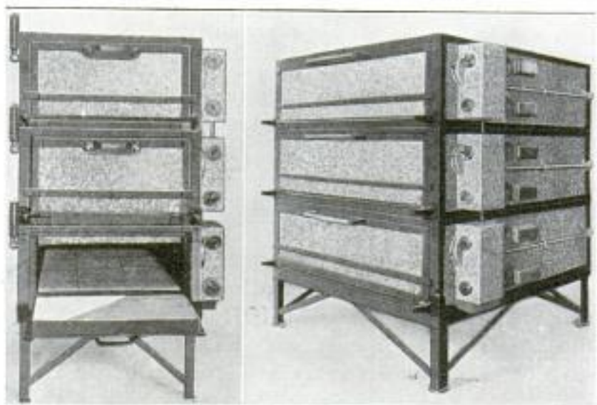
At the Left is Seen an Electrical Bake Oven Having Three 20-Loaf Sections, Mounted One above the Other, While at the Right is Shown an Oven Consisting of Three 60-Loaf Sections
