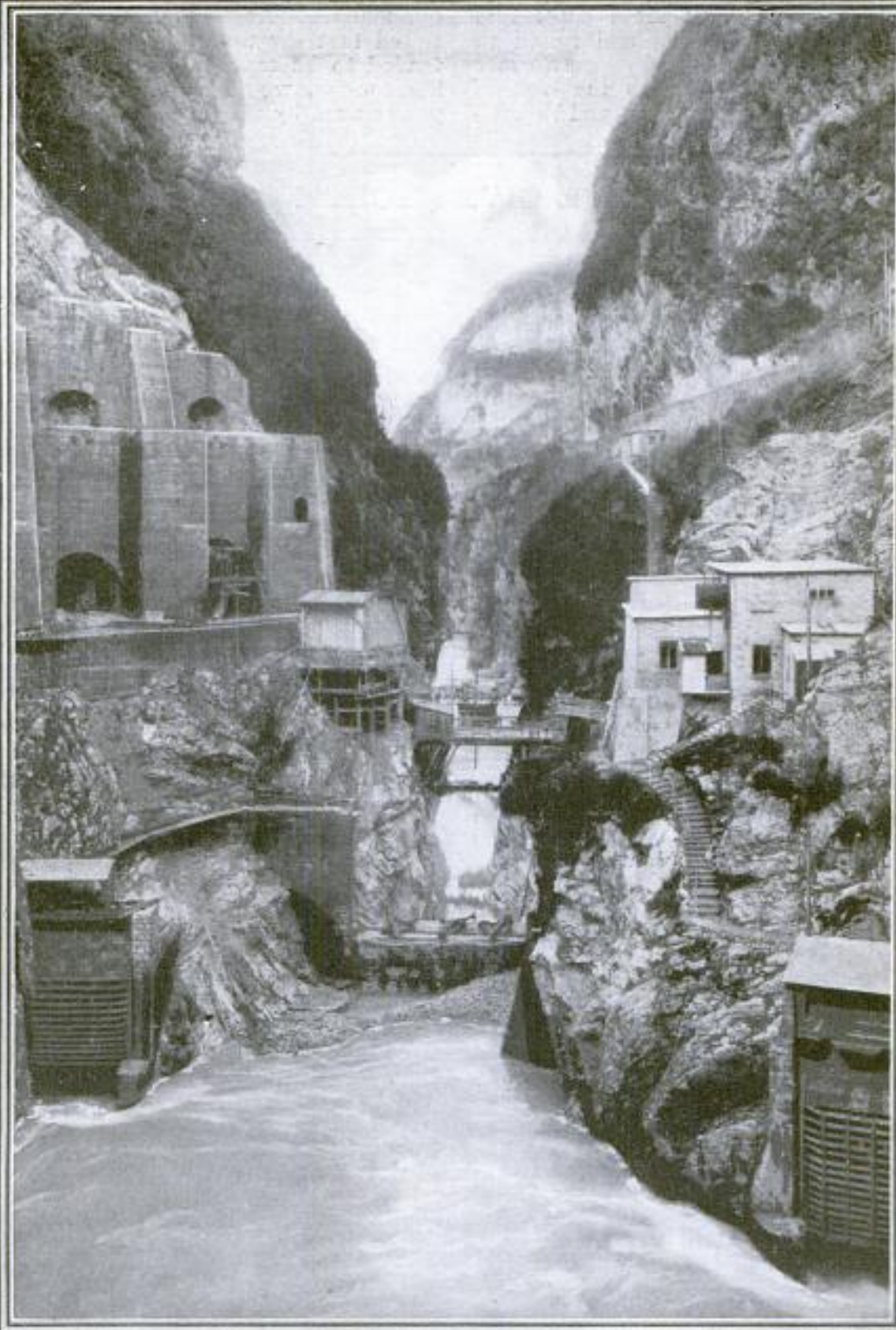
General View of Fier River Power Development during Construction at the Dam Site: Note, at Lower Edges of Picture, Outlets of Tunnels on Either Side of the River, Used to Divert the Flow during Construction
