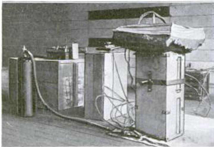
Apparatus for Temperature Tests on Seed Cones: It Includes an Electric Hot-Plate Heating Device in Which the Cones are Placed, a Potentiometer, a Rheostat, Switches, and a Gas-Supply Cylinder for Testing the Inflammability of Materials
