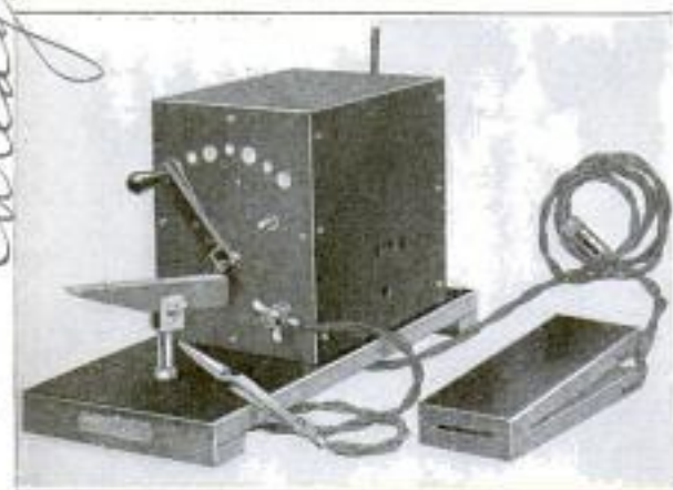
This Electric Soldering Machine Has Three Different Heats for the Repair of Jewelry, Which It Accomplishes Quickly and Neatly
