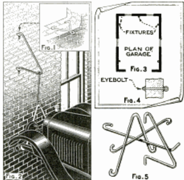
ILLUSTRATING USE OF FIXTURE AS CAR SUPPORT. FRONT AXLE REMOVED
