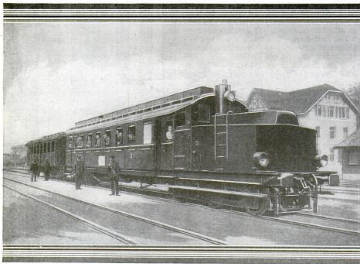
One of Switzerland's Powerful Locomotives, Which Has a Combination of Gasoline and Electric Propulsion and Which was Designed for Standard-Gauge Roads: Note How the Engine and the Coach are Combined
