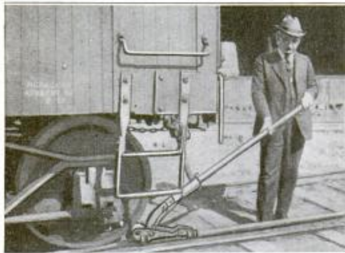
Left: With This Car Pusher One Man can Start and Keep in Motion Four Loaded Cars. It is Operated by Working the Lever Up and Down. Right: Close-Up of Car Pusher Which Automatically Grips the Rail and Has an Adjustable Fulcrum
