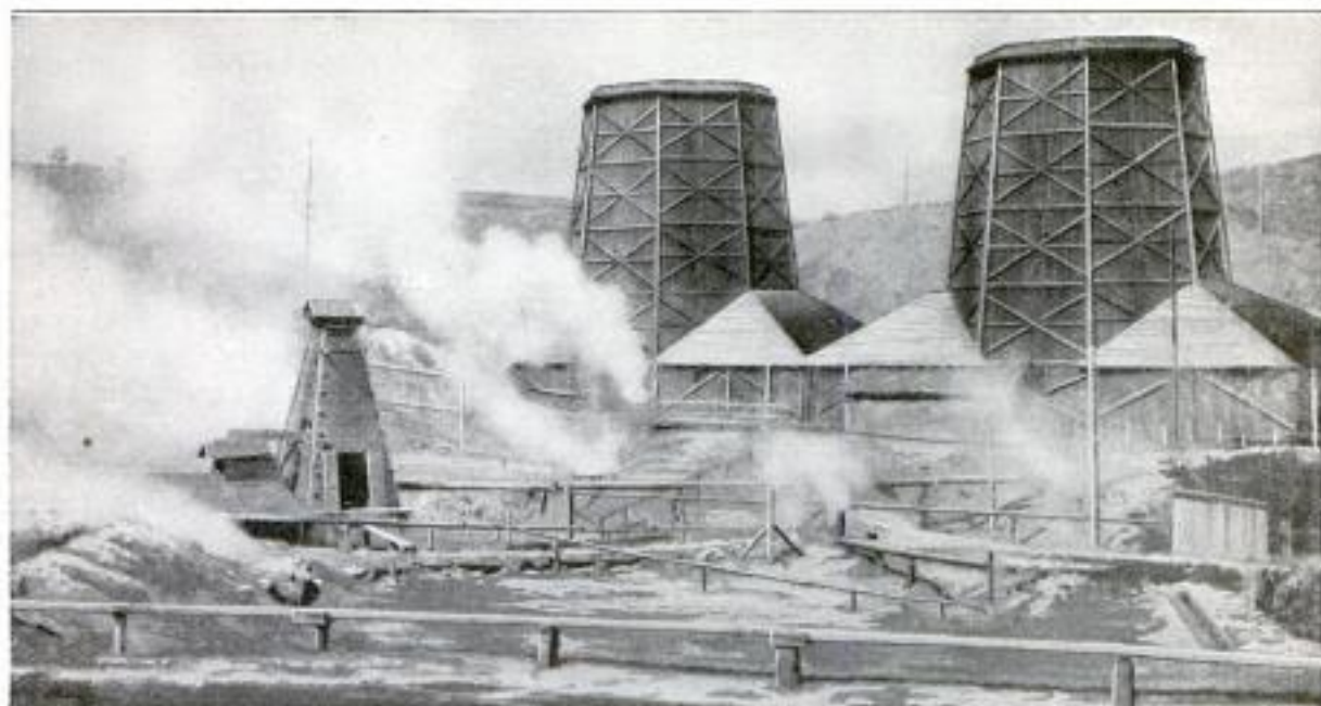
In the Queer, Tapering, Flat-Topped, Octagonal Buildings at the Hot Springs, the Mineral-Charged Steam Superheats Generated Steam That Drives the Turbines
