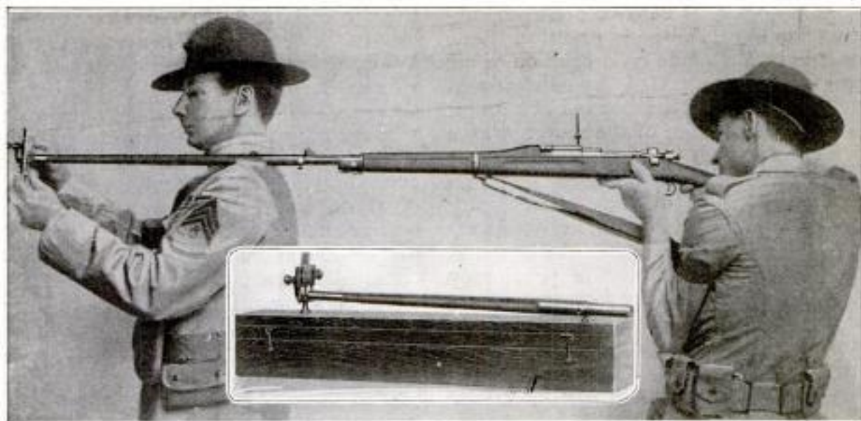
An Instructor is Here Shown Adjusting the Miniature Target on an Aiming Device According to the Pupil's Directions. On Word from the Pupil the Officer Registers the Aim with a Dotter. A Close View of the Attachment is Given in the Insert
