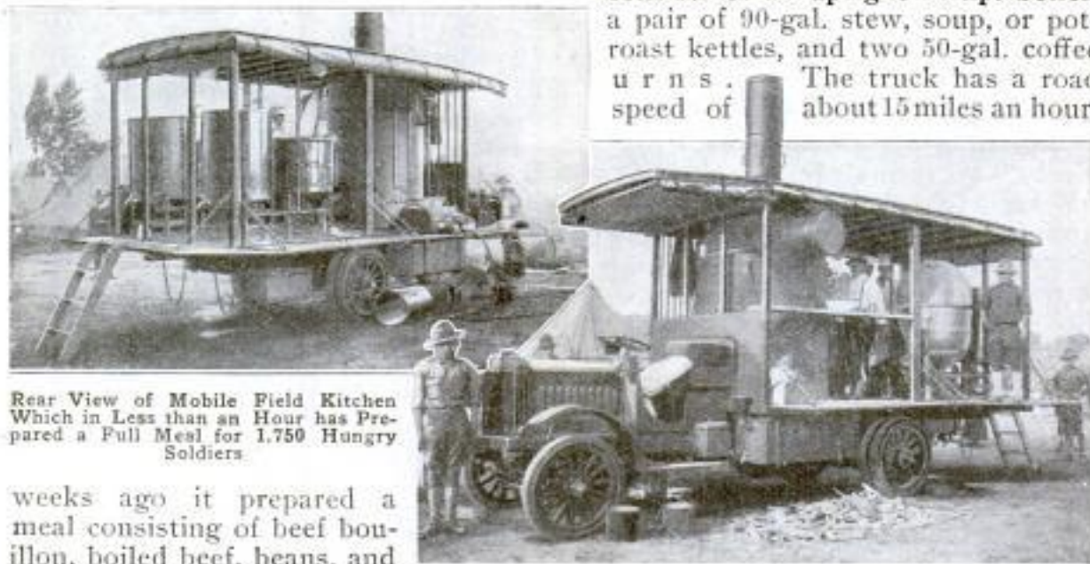
Two of the Units, It has been Demonstrated, are Adequate to Meet the Needs of an Entire Regiment of Men
