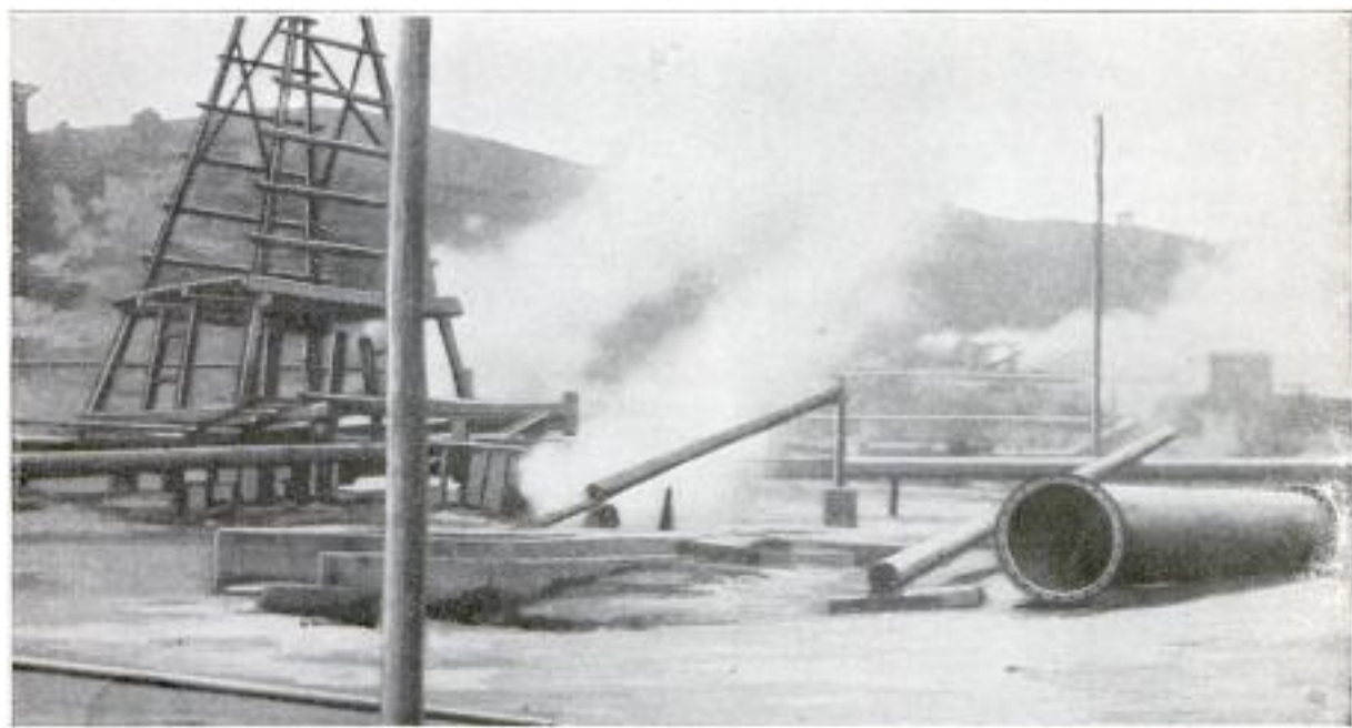
Close View of a Derrick That is Drilling through an Impervious Rock Stratum to the "Reservoir" of Natural Steam Some 500 Feet beneath the Surface of the Ground
