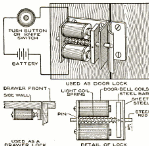
Details of the Electric Bolt Lock, and Methods of Installing It on a Drawer and a Door
