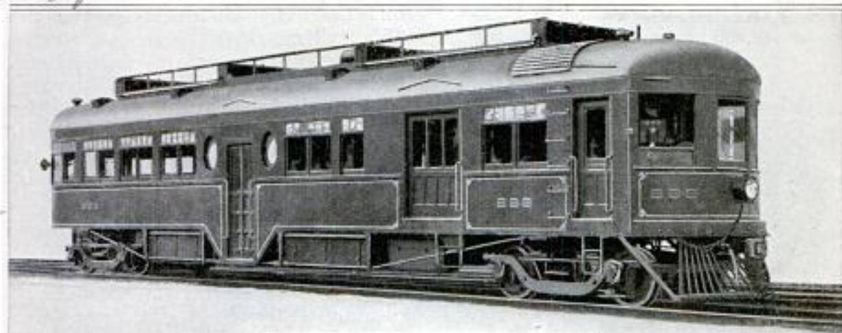
Showing the Exterior Appearance of the New Oil-Electric Motor Car Recently Built for the Nashville, Chattanooga & St. Louis Railway
