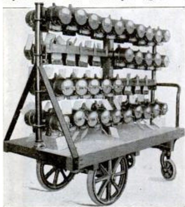
A Truck Designed by an Electric-Lighting Plant Superintendent Which Enables One Man to Move a Number of Meters Quickly and with Little Risk of Getting Them Out of Order
