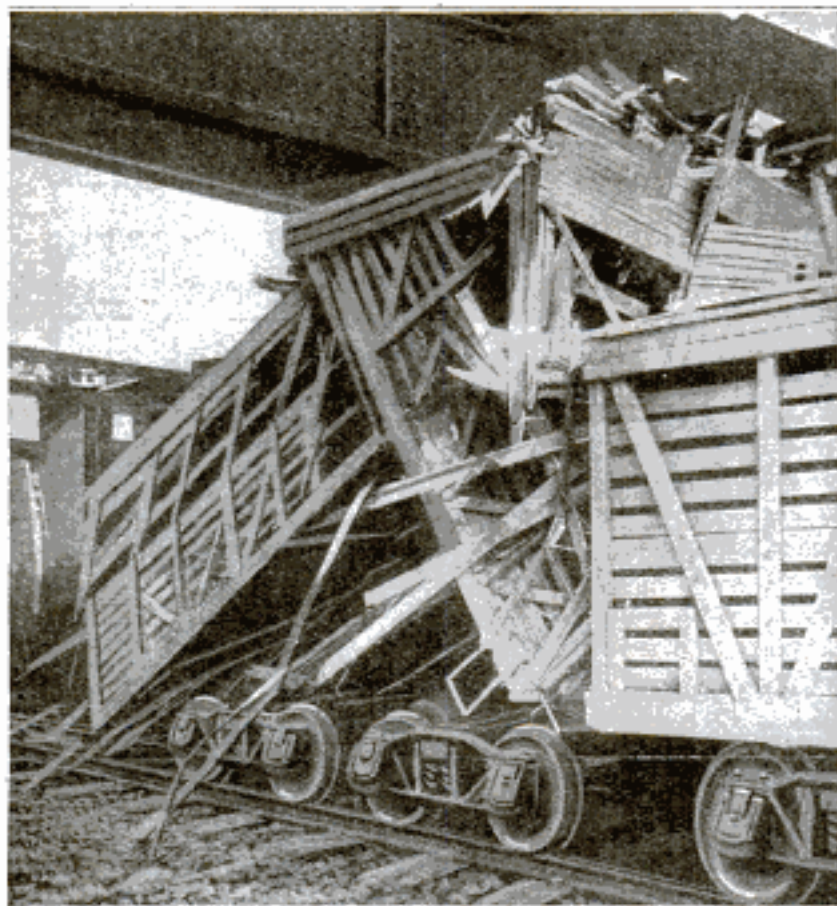
Stock Car Which Buckled beneath a Trestle When the Brakes were Suddenly Applied to the Train, Subjecting This Car to Too Great Pressure at Either End
