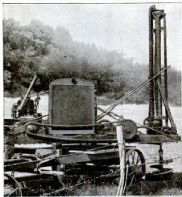
A Post-Hole Digger Driven by an Engine Taken from a Wrecked Automobile
