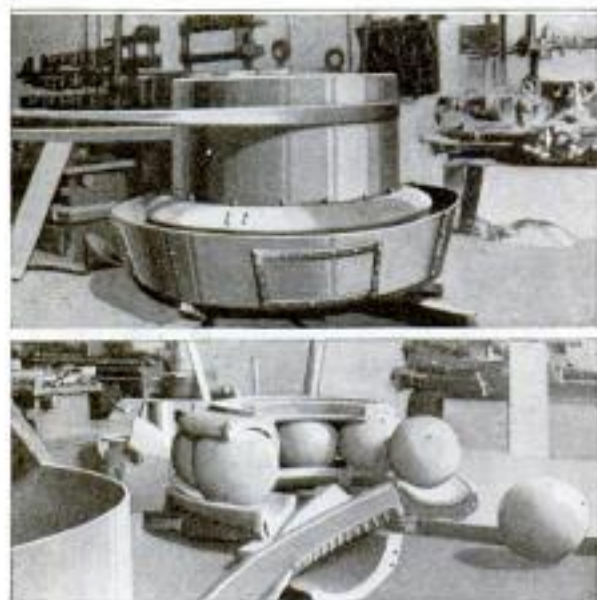
At the Top the Mill Is in Operation, While Below It is Disassembled to Show the Arrangement of Some of Its Parts and the Size of the Balls Used
