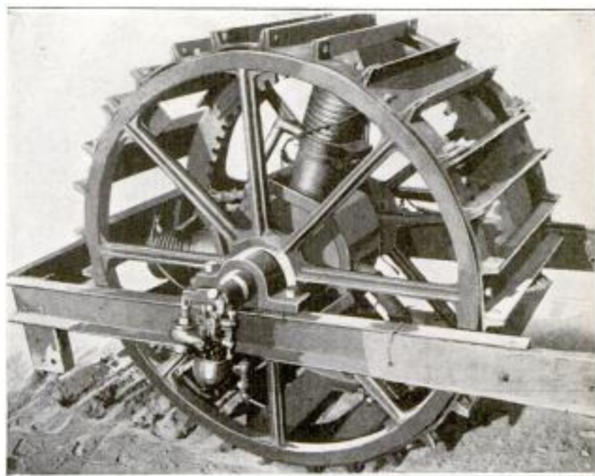
Novel 12-Horsepower Farm Tractor Driven by a Rotary Engine and Designed for Use on Small Farms
