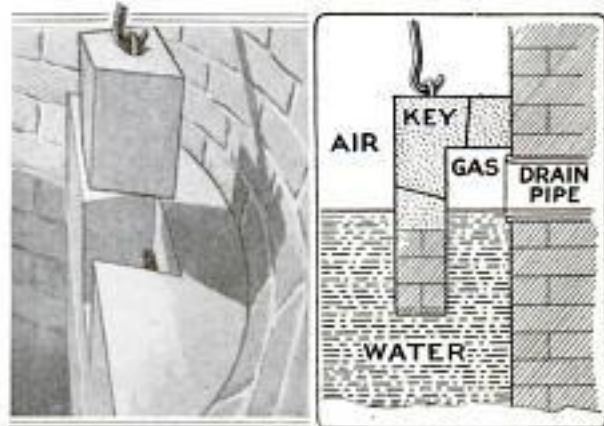
Catch Basin with Patented Trap, Showing the Cement Key That can be Removed to Give Access to the Outlet Pipe
