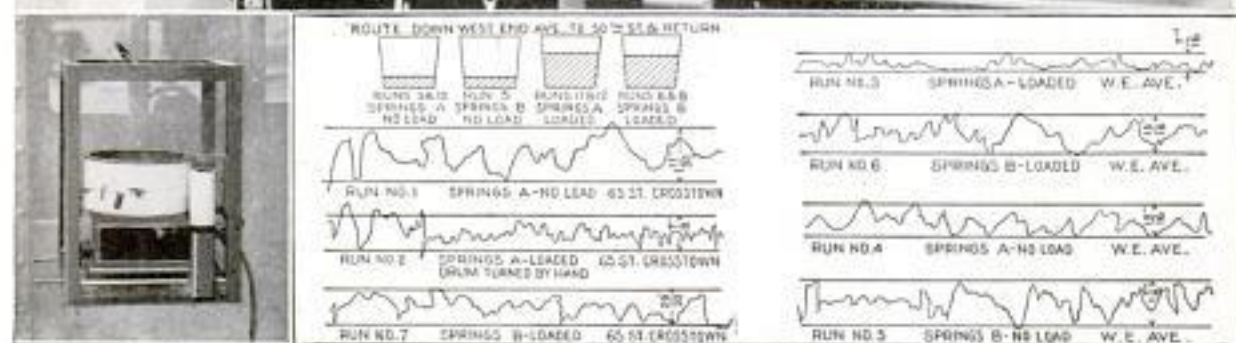
Left: Close View of the Seismographic Device, Showing Recording Pencil Held by Weighted Spring. Right: Records of Various Trips Made over the Same Route with Different Springs
