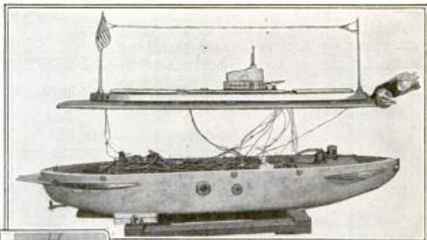
Showing the Mechanism Installed inside the Submersible, the Character of the Fins and the Elevator: The Hand Holds the Tiny Torpedo That is Fired
