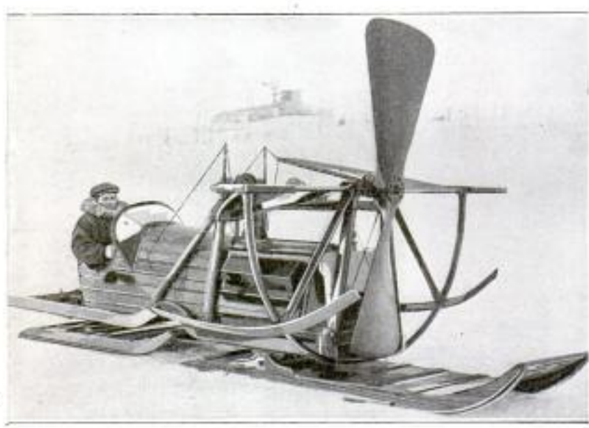
With Its 60 Horsepower, the Motor Gives the Squatty Snow Car Splendid Speed
