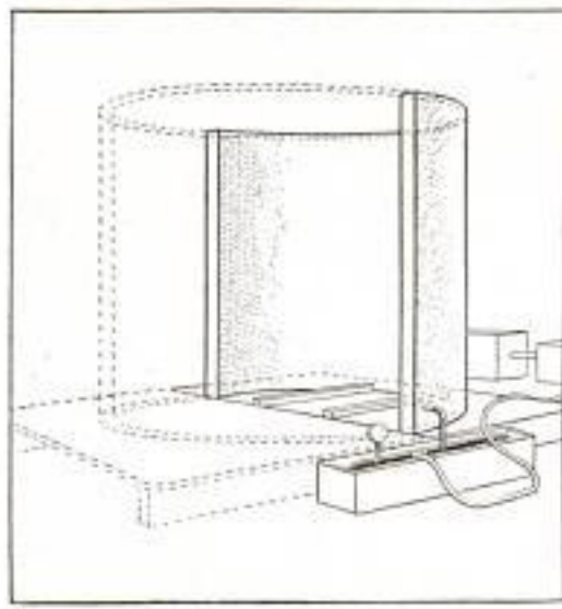
Apparatus for Freezing Whole Fruit Trees to Determine the Damage Which Various Temperatures Produce: The Two Halves of the Cylinder are Set Close about the Tree and Then Cold Air is Forced into the Inclosure
