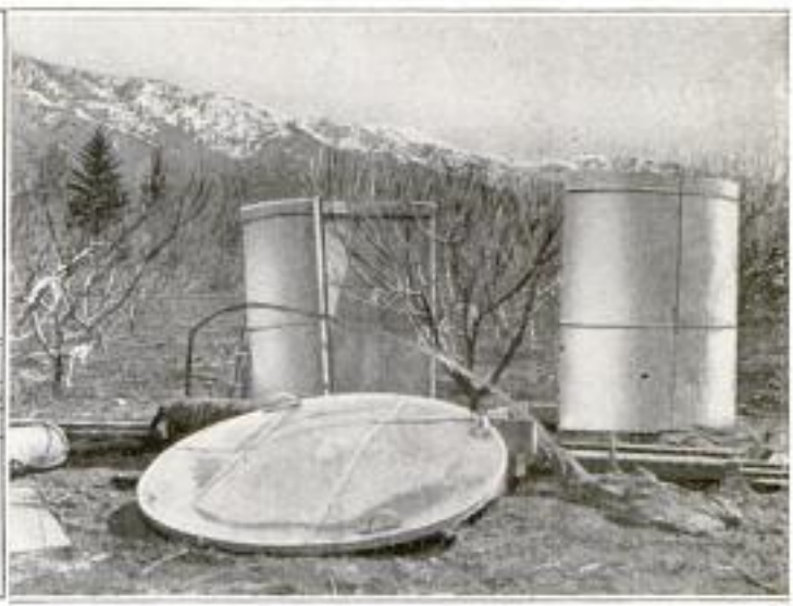
Apparatus for Freezing Whole Fruit Trees to Determine the Damage Which Various Temperatures Produce: The Two Halves of the Cylinder are Set Close about the Tree and Then Cold Air is Forced into the Inclosure
