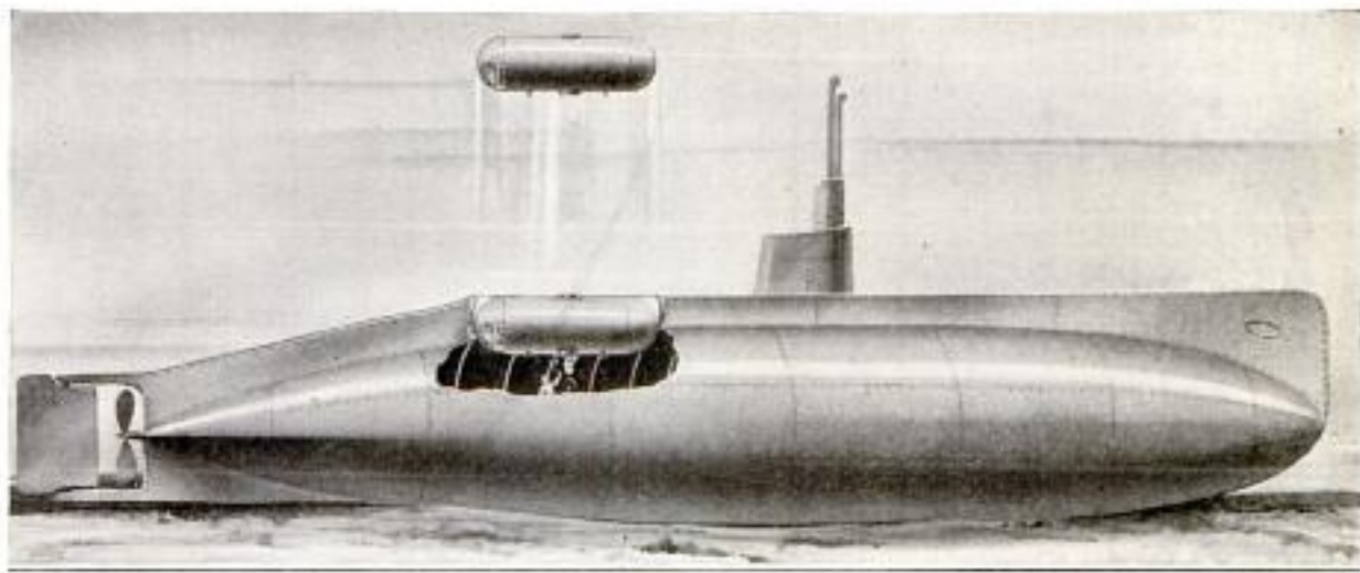
The Method of Carrying the Auxiliary Submersible and the Way It Leaves the Mother Craft are Shown in the Drawing Above. The Small Vessel is Self-Propelled and Accommodates 30 Persons
