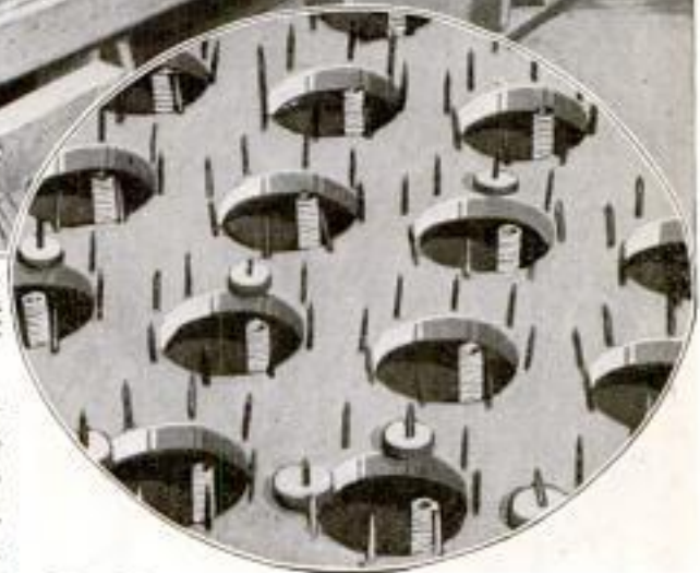
Close View of Top Surface of the Switchboard, Showing Some of the Disks in Place on the Upright Pins Encircling the Holes, Inside of Which the Coil-Spring Contacts will be Observed
