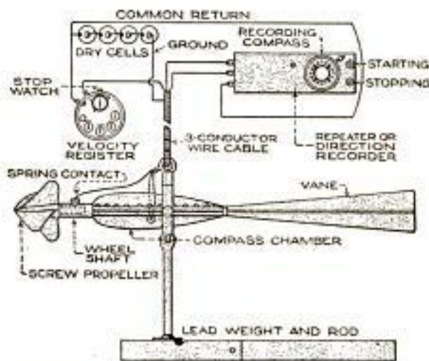
Diagram of New Current Meter Used from a Boat to Secure Data for Charts of Harbor and Coast Waters
