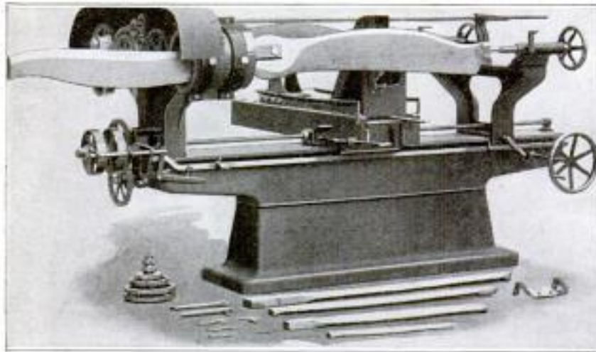
Lathe for Turning Aeroplane Propellers: It will Copy Any Model, Producing Both Right and Left-Hand Pieces, Either Larger or Smaller Than the Original
