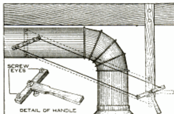
This Arrangement Made in Half an Hour Is a Great Convenience at the Furnace
