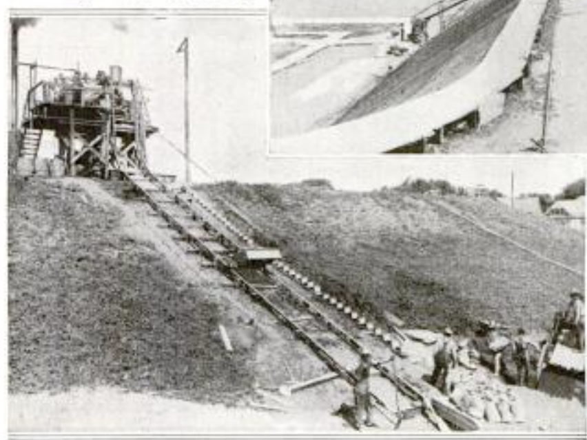
Making a Leaky Reservoir Water-Tight by Relineing with Concrete: The Inclined Track and Skip to Convey Materials to the Mixer Above are Shown at the Left, While the Method of Distributing the Concrete Inside the Basin is Seen Above
