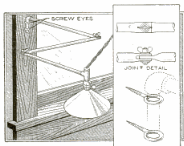
A Strong and Practical Bracket for a Bench Light was Made of \frac{1}{2} -In. Gas Pipe
