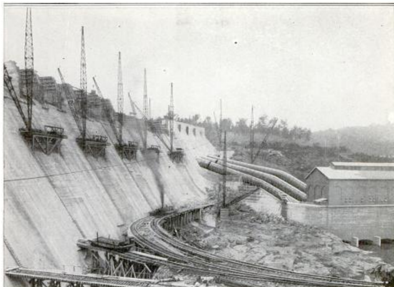
Construction was Greatly Expedited by the Use of 50 Derricks of 25-Tons' Lifting Capacity Each, Some Capable of Carrying 100,000 Pounds Each. The Power Plant will Generate an Average of 45,000 Kilowatts
