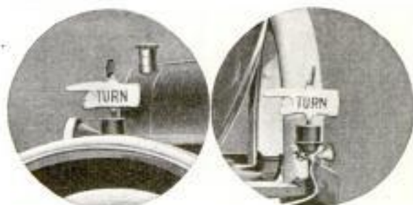
The Signals at the Front and Rear are Controlled by a Switch Mounted on the Steering Wheel. Current can be Taken from the Storage Battery or from Dry Cells
