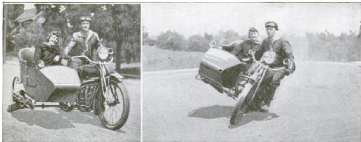
At the Left the Drag is Shown in Place and the Sidecar Supported at Its Normal Height. This Enabled a Quick Start. The Other Picture Explains How the 25-Mile Trip was Made with the Vehicle Balanced
