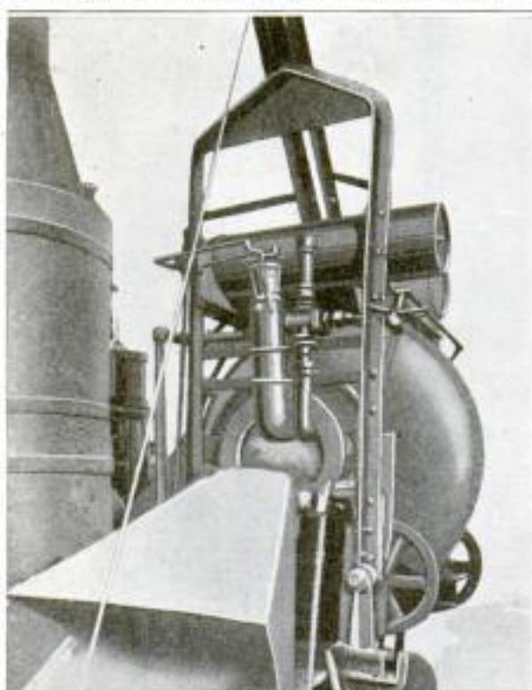
Oil Burner Which Forces a Flame into the Drum of the Cement Mixer, Thereby Preventing the Freezing of Materials in Winter
