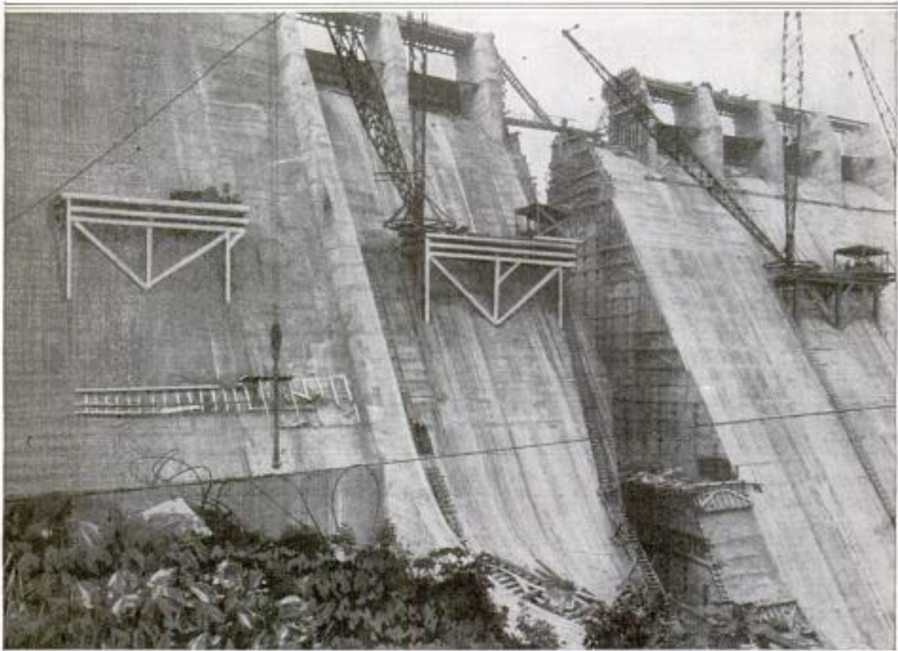
Close View of the Hydroelectric Power Dam on the Yadkin River near Whitney, North Carolina: Its of Which are Shown Here. Building Material was Brought within Reach of the Derricks on Flat Cars
