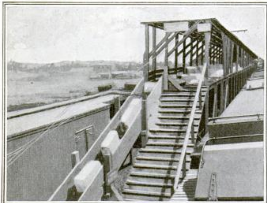
Some 150 Refrigerator Cars are Iced Daily during the Shipping Season at This Station. The Ice Is Unloaded on the Conveyor and Carried to the Platform above the Fruit Cars
