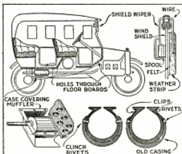
These Homemade Devices and Features Are Practical for Winter Touring or Driving. The Car is Warmed, the Tires Protected, and the Windshield Kept Clean.
