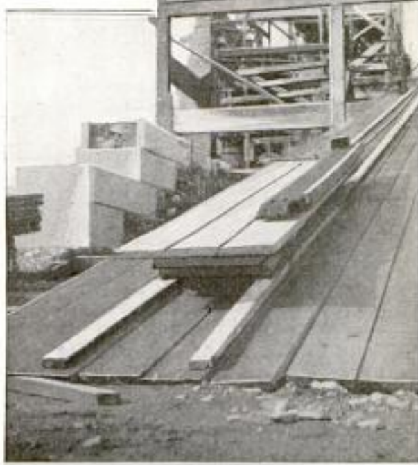
Simple Carrier Made by Mounting a Platform on Two Dollies: It was Operated by a Hoisting Engine and Elevated Three Wheelbarrow Loads of Mortar at a Time, as Well as Heavy Steel Girders
