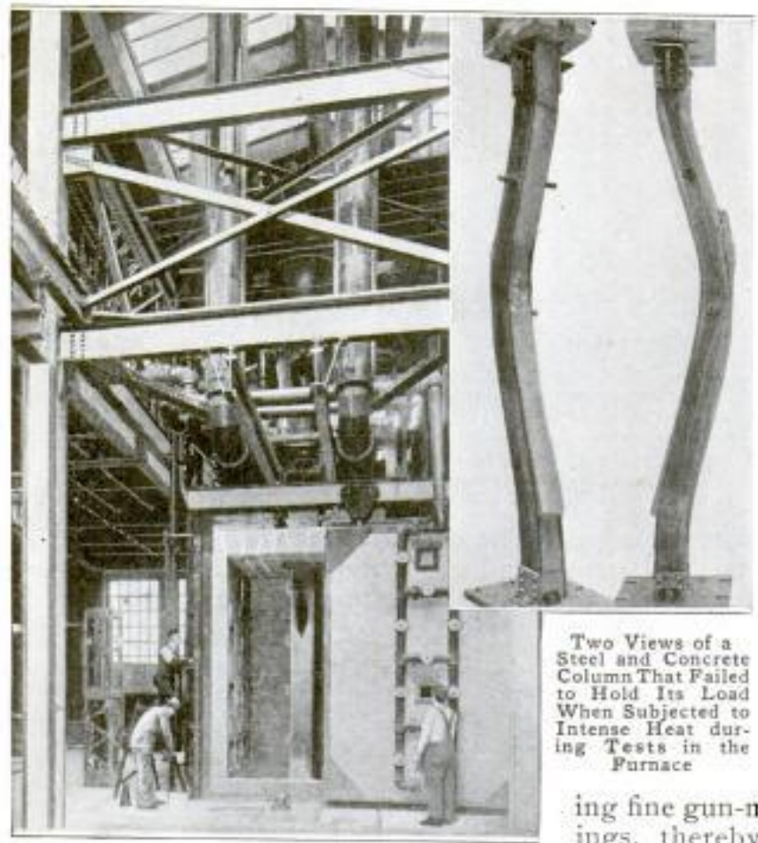
One of the Movable Furnace Walls Opened to Show a Large Building Column in Position for Test: The Ram is Supported by the Steelwork Above, While the Pipes are Flues for Discharging Fumes. Mica Windows are Provided for Observation
