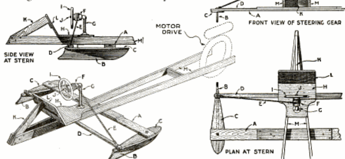
The Construction of This Motor-Driven Ice Sulky Is Interesting, the Power Plant being Located at the Forward End of the Frame, and the Weight of the Seat and Driver being so Distributed as to Give the Proper Balance and Traction
