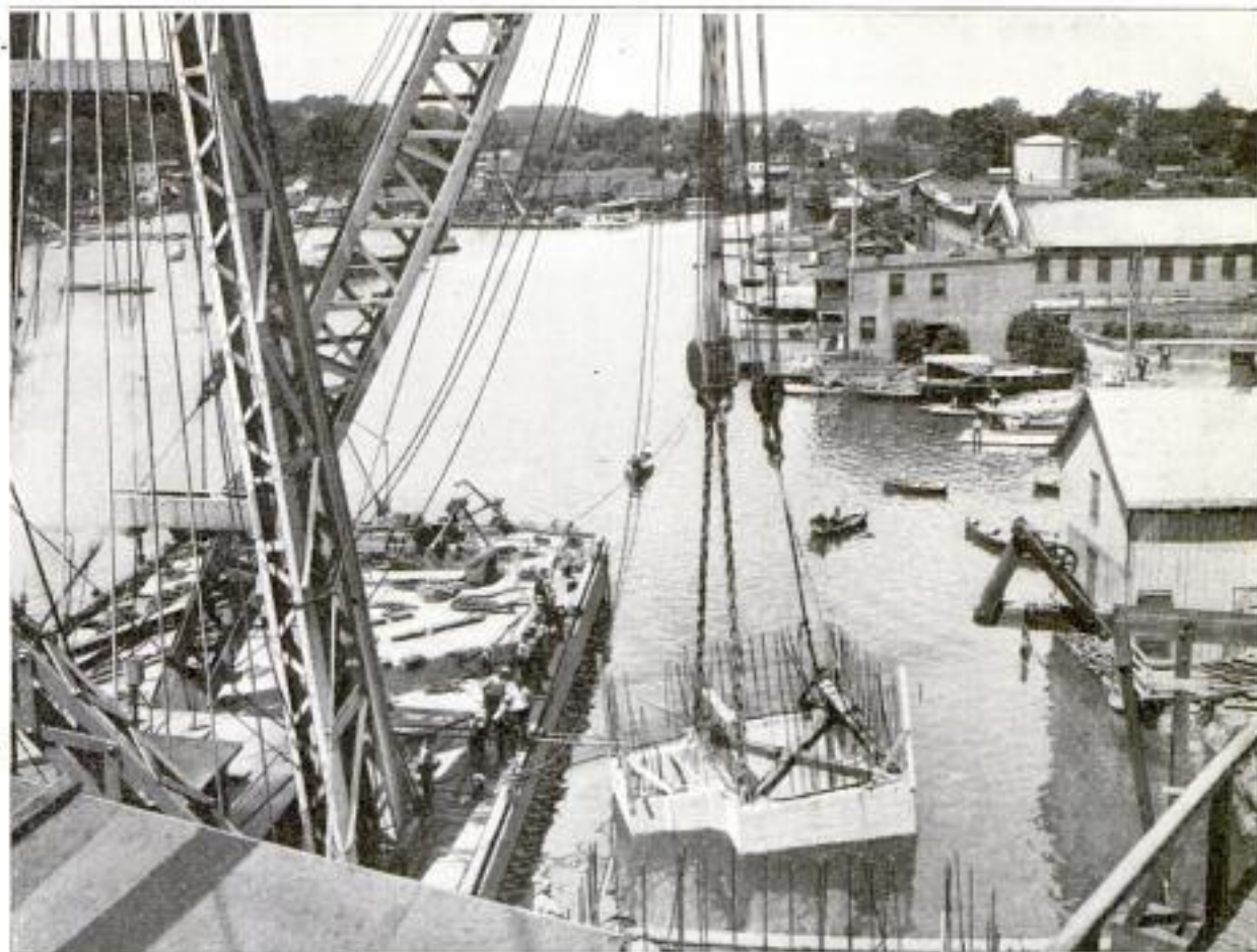
COPYRIGHT, BROWN & DAWSON Showing the Powerful Derrick at Work Lowering One of the Reinforced-Concrete Intake Cribs, Weighing 150 Tons, into Place in the Harbor
