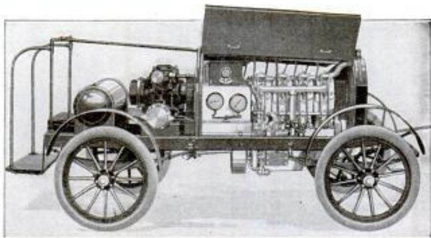
Novel Trailer "Fire Engine" of Low Cost That may be Operated at Moderate Expense by Small Municipalities and Suburban Communities
