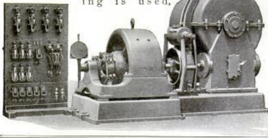
Worm-Gear Traction Elevator Engine Which Requires Low Starting Current and Is Easy to Operate: Panel Board, Which Is of Comparatively Simple Construction, is Shown at the Left of the Engine
