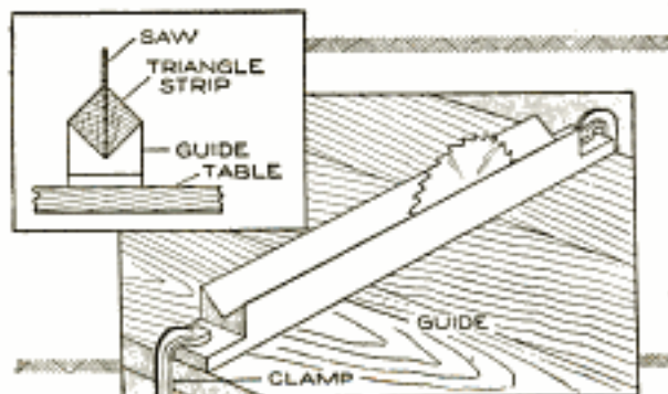
The Guide is Clamped on the Saw Table and the Squared Stock Ripped Diagonally
