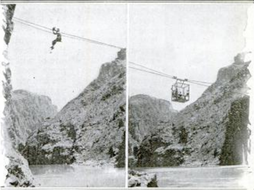
PHOTOS BY D. D. RUST Left: Crossing Hand over Hand with a Trapeze. When the Cage is Not Available One must Cross This Way or "Go Around," Which Means About a Week's Journey. Right: The Cage Propelled by Means of a Hand Windlass and a Light Cable; It Rides About 60 Feet above Mean Water Level
