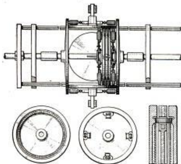
New Method of Applying Pressure in Friction Gear, by Means of Magnets: The Lower Sketches Show the Friction Wheels
