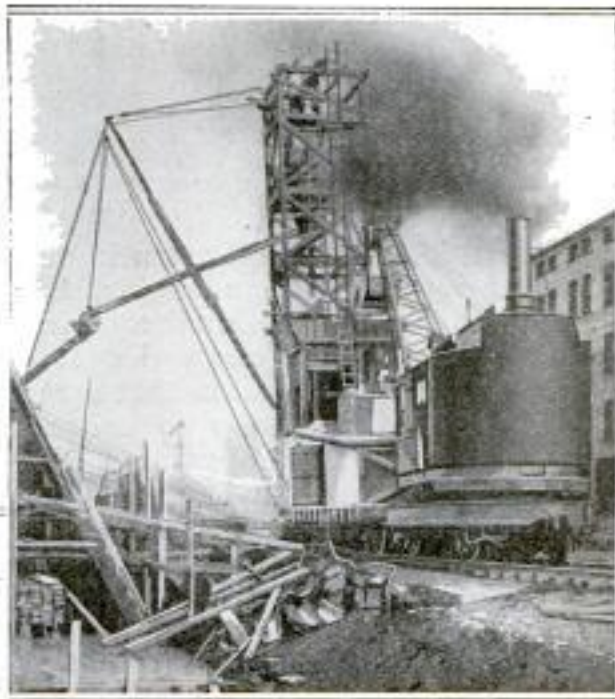
Above is a view of a portable concrete-mixing outfit, including a tower, mounted on a car. At the near end of the material-and-construction train in the left-hand picture, the mixer car is shown with tower removed.
