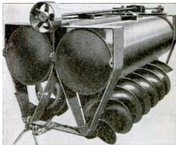
By Means of the Two Spiral Members, Which Are 10 Inches in Diameter, This Water Motor was Able to Develop More Than One-Fourth of One Horsepower in a Stream Having a Moderate Current
