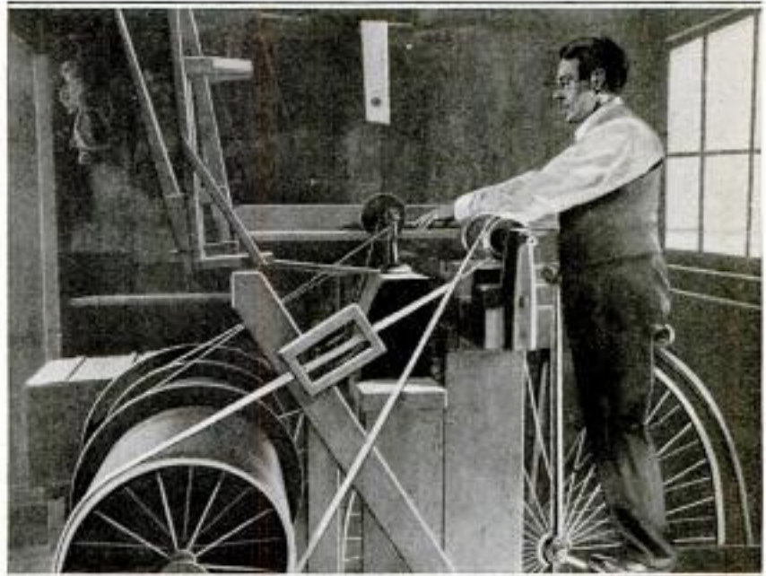
An Old-Fashioned High-Wheeler Bicycle was Rigged Up to Provide the Driving Gear for This Combination Machine; the Operator is Ripping Stock on the Circular-Saw Attachment
