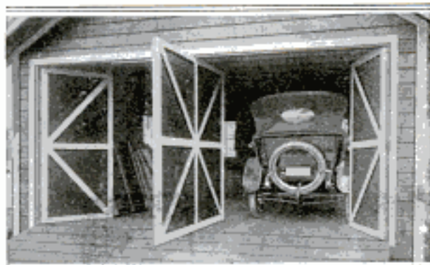
Handy Set of Doors for a Double Garage, Designed by the Owner and Built by His Son and a Boy Friend
