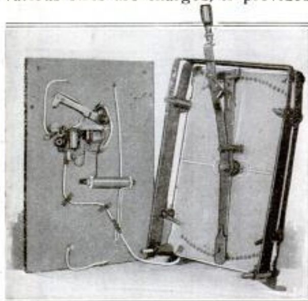
Foolproof Type of Universal Rheostat Taken Apart to Show the Lever Which Interlocks with Circuit Breaker so That When the Latter Is Open the Lever must First be Set at the Minimum Charging Rate to Close the Circuit
