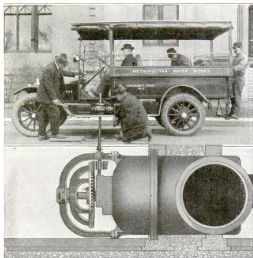
Showing the Device in Operation Opening a Water-Main Valve. It Saves Much of the Time and All the Labor Required by the Manual Method
