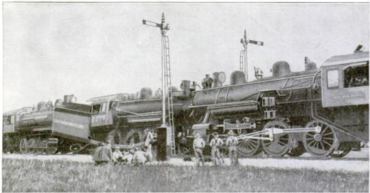
Collision Which Was Remarkable in That It Occurred Just at the End of a Signal Block: One Train Entered One Block Only Five Seconds Later Than the Other Entered the Adjoining Block. Both Trains were Drawn by Two Engines
