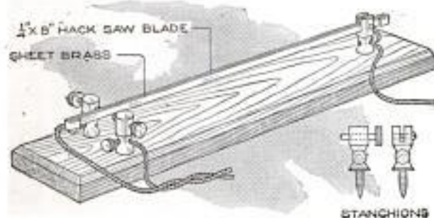
When the Incubator Becomes Too Hot or Too Cold, the Strip is Bent Toward One of the Binding Posts, and the Bell is Rung at a Distance
