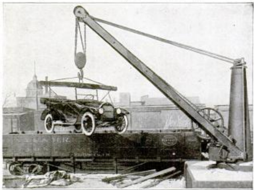
Simple Tackle for Lifting Automobiles from Gondola Cars: At the Points Where the Rope Touches the Car, Padding is Employed to Prevent Marring
