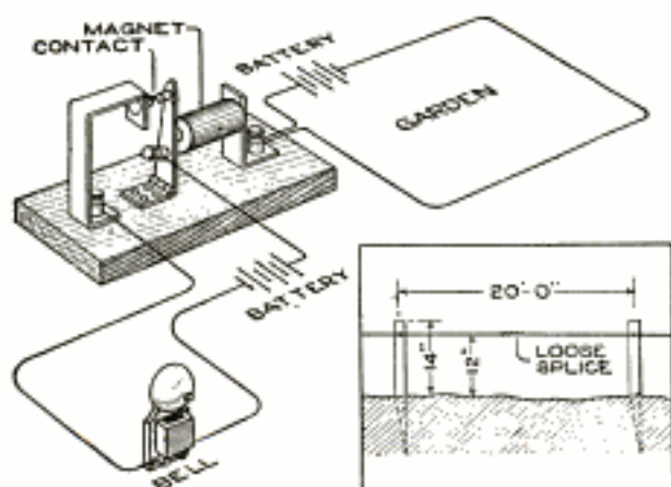
When Intruders in the Garden Break the Wire Circuit at Any of the Loose Joints, a Warning Bell Rings in the House
