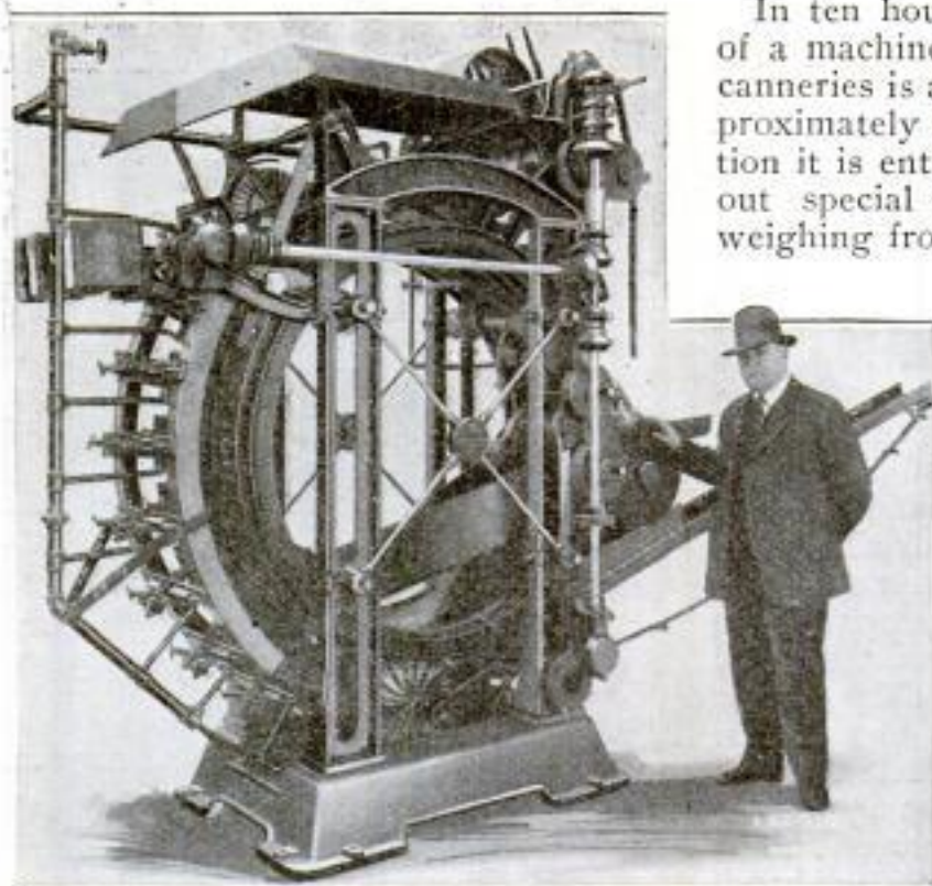
Doing the Work of About 60 Experts, This Machine Dresses and Cleans One Salmon Every Second
