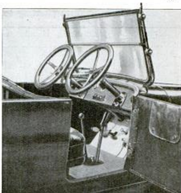
Car in Which Instruction is Given in Motor Driving: Danger of Accident is Practically Eliminated by the Use of Two Sets of Controlling Devices
