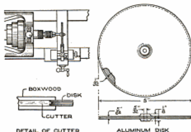
DETAIL OF CUTTER ALUMINUM DISK These Aluminum Disks were Grooved on Their Circumference by Rigging a Special Tool, as Shown
