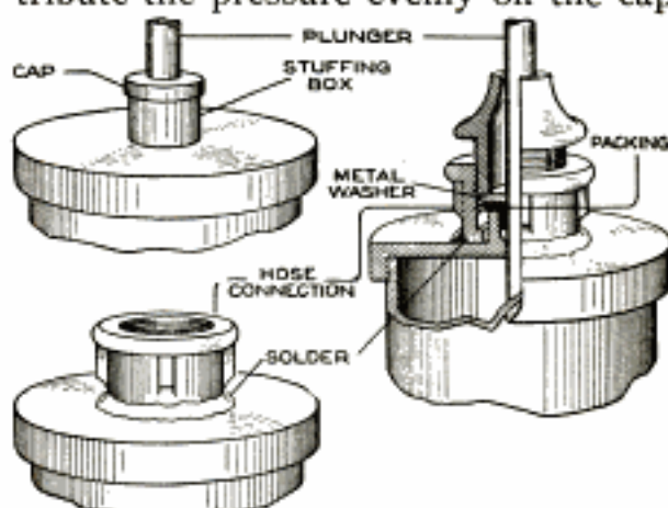
Hose Connections were Used to Repair the Stuffing Box, Making It Quite Serviceable
