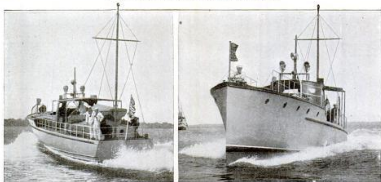
Dual-Service Boat, 66 Feet Long, Which the Government Recommends Yachtsmen to Copy in Building New Craft, so That in Case of Emergency Such Boats can be Requisitioned for Naval-Patrol Work
