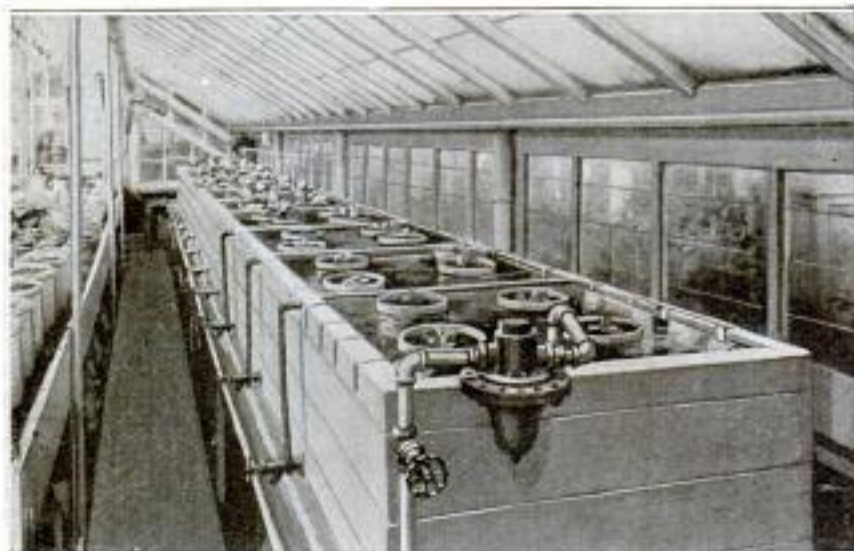
Special Apparatus for Testing Plant Diseases in Soil at Constant Temperatures in Use at the Wisconsin College of Agriculture: The Jars Seen in the Tank Compartments Contain Soil and Plants under Observation
