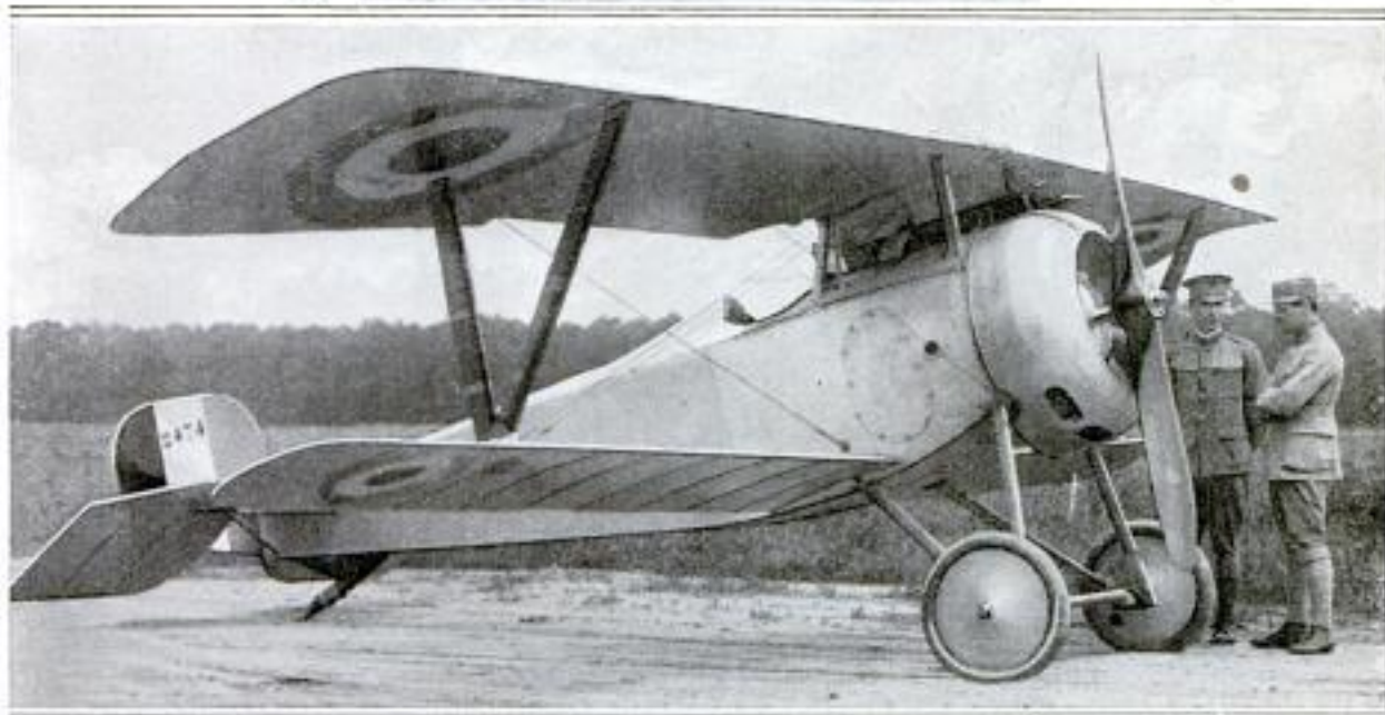
COPYRIGHT, INTERNATIONAL FILM SERVICE Close Views of a Nieuport Speed Scout during Its Inspection by an American Army Officer: At the Top is Shown the Nine-Cylinder Rotary Motor That Drives the Craft, While Below an Excellent Idea is Given of the Arrangement of the Struts and Bracing Wires
