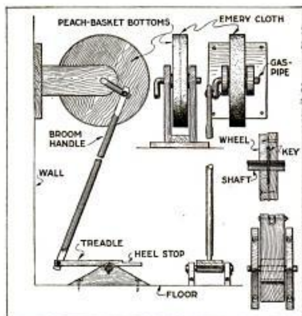
This Emery Grinder Proved so Handy in a Diesinker's Shop That One was Made for Home Use
