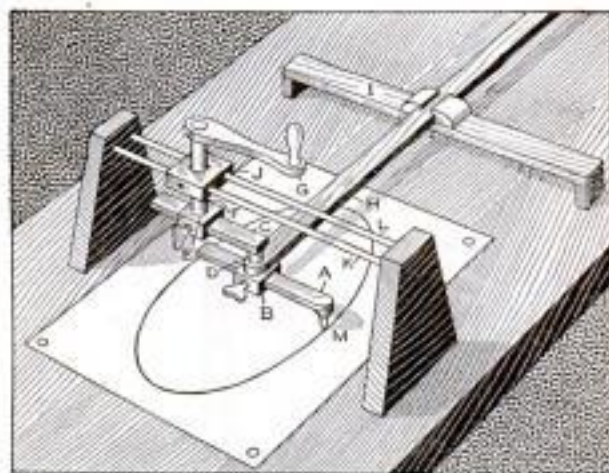
The Machine is Set According to the Desired Major and Minor Axes of the Ellipse, and the Figure Drawn Precisely
