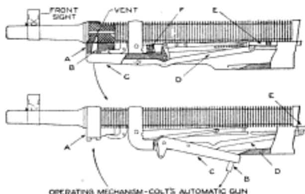
OPERATING MECHANISM—COLT'S AUTOMATIC GUN In the Upper Drawing the Gas Lever is Shown in the Closed Position, While in the Other Diagram It is Thrown to the Rear and the Retracting Springs Compressed. A, Gas Cylinder; B, Piston; C, Gas Lever; D, Gas-Lever Connection; E, Slide; F, Retracting Springs
