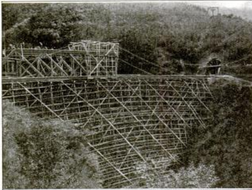
Japanese Railway Bridge being Built on a Falsework of Bamboo: The Useful "Grass" is Also Used for Scaffolding to Raise the Heavy Steel Beams to Place
