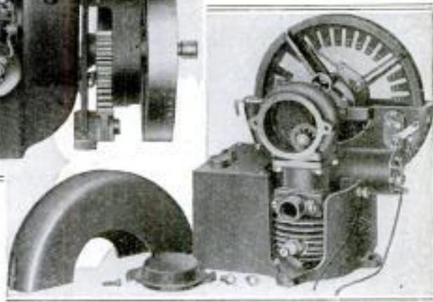
View of Portable Engine for Home Use Easily Operated by an Inexperienced Person. Lower View: Engine with Crank-Case and Flywheel Covers Removed, Showing Fan Flywheel and Cylinder
