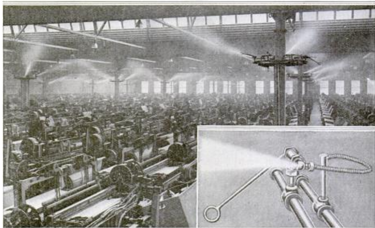
Humidifying the Air in a Textile Factory to Secure the Best Working Conditions for the Raw Material and Fabrics Made: The Insert Shows Details of Spraying Apparatus Seen on Each of the Pillars in the Larger Picture
