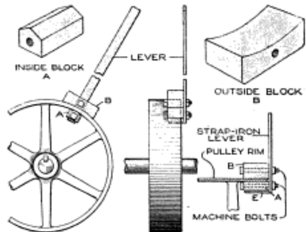
By the Use of This Lever Arrangement the Rims are Not Nicked in Resetting Pulleys
