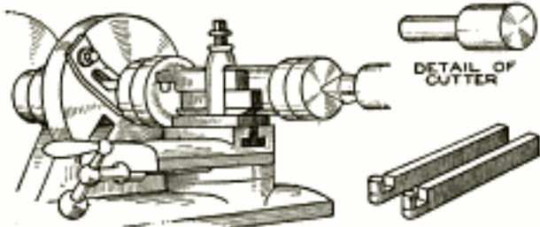
Smooth, Circular Curves were Cut in Turned Work on the Lathe by Means of Adaptable Cutters Made in Several Standard Sizes
