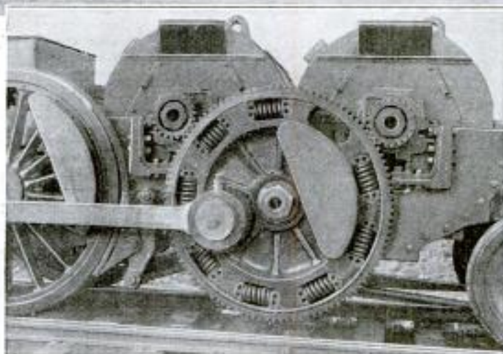
Big Electric Locomotive Constructed in Anticipation of the Electrification of a Railway Line in the Allegheny Mountains and a Close View of One of the Trucks, Showing the Character of the Spring-Gear Wheels through Which Dual Motors Transmit Their Power to the Drivers
