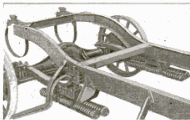
Indirect Suspension is Said to Oblviate the Rebound and Side Sway Produced by Ordinary Springs When Compressed by Road Bumps
