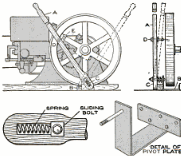
DETAIL OF HANDLE END An Engine, Too Heavy to be Started Handily Except by a Strong Person, was Rigged with a Starting Lever That a Woman can Use
