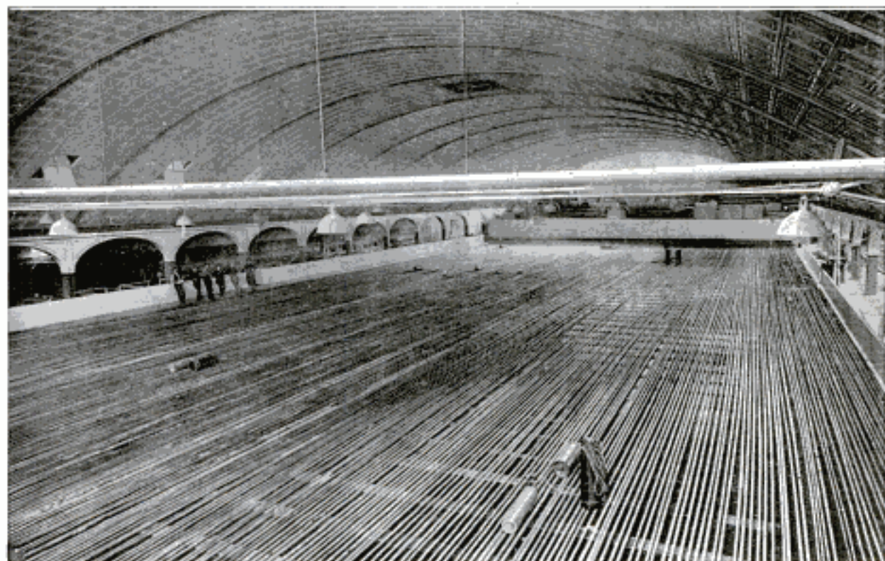
Ice Rink, Measuring 90 by 210 Feet, Showing the Floor Covered with 10 Miles of Refrigerating Pipe Which was Welded in Over 2,000 Places by the Oxyacetylene Process
