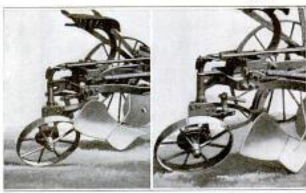
Two Views of an Automatic Brake on a Riding Plow: The One on the Left Shows the Plowshare Raised and the Brake Set; the Other Shows the Plow Lowered and the Brake Released
