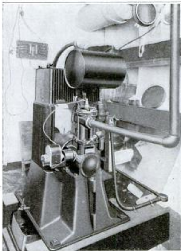
The Ship's Smooth-Running Light and Power Plant: Its Rated Capacity Is 500 Watts at 110 Volts. No Storage Batteries are Used
