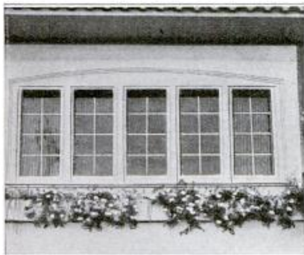
View of End of Apartment House, Showing Flower Boxes Built into the Wall at the Second-Story Level: They are Provided with Permanently Connected Spray Pipes and Drains
