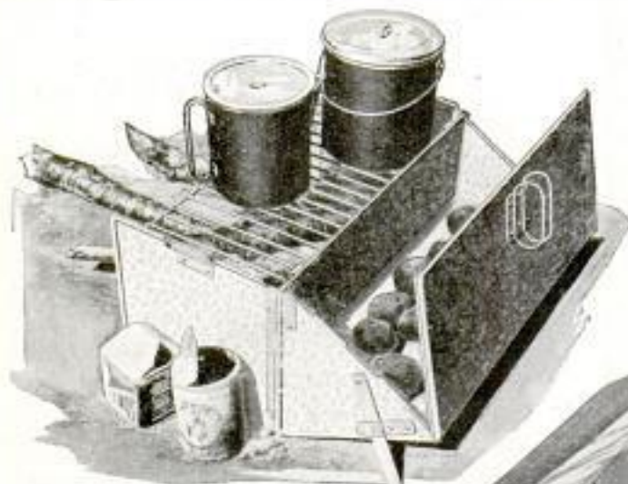
Collapsible Stove and Oven of Galvanized Iron: Wood of Any Length can be Burned by Inserting Sticks Endwise. Folded, It Makes a Flat Thin Package with Smoked Surfaces Within
