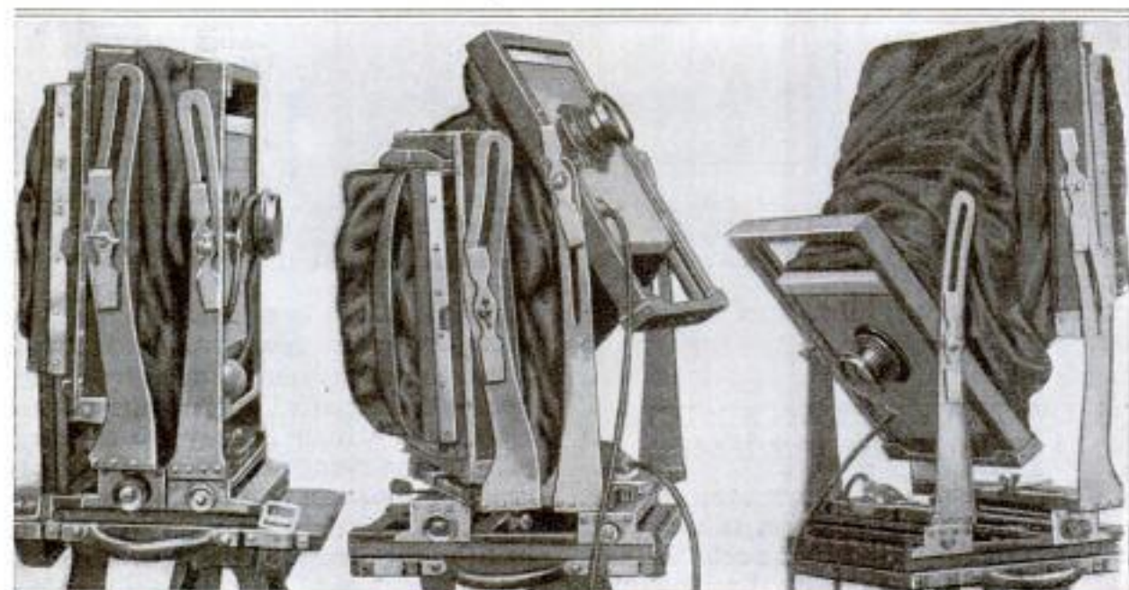
Above, the Camera is Focused in Three Different Ways to Show Its Extreme Flexibility. In the Middle Picture It will be Observed That the Plate is Turned at an Angle and the Lens Elevated and Inclined
