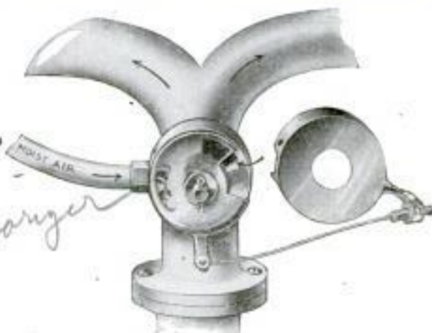
Showing Installation of Fuel-Saver, Which is Said to Cool an Engine and Eliminate Carbon
