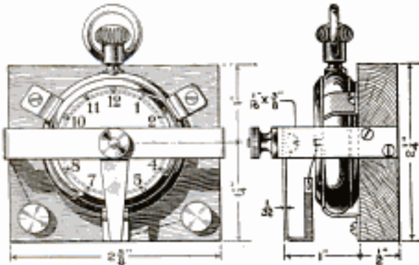
The Watch is Clamped on the Base and Electrical Connections Made as Indicated
