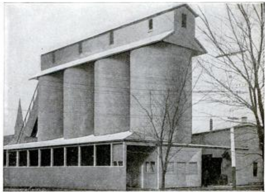
Coal Bins of an Unusual Type: These Cylinders Are 18 Feet in Diameter, 50 Feet High, and Each Has a Capacity of 1,400 Tons of Fuel
