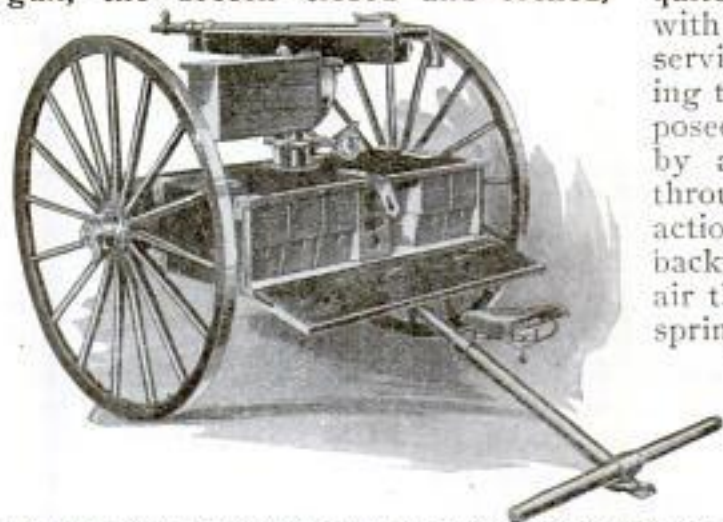
Here the Gun is Mounted on a Light Landing Carriage. The Ammunition Chest, Which is Shown Open, Contains Feed Boxes That Have a Capacity of 2,000 Rounds. The Seat is Attached to the Carriage Tongue
