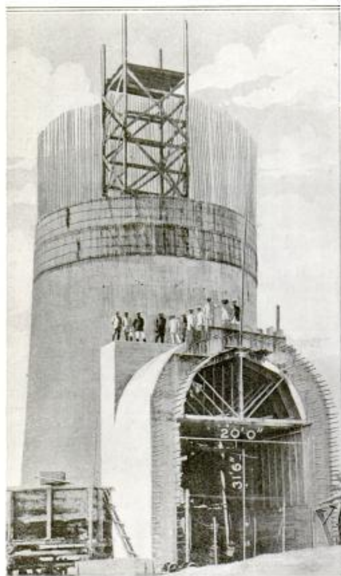
The Base of the World's Greatest Chimney. Showing the 31-Foot Arch to Which a Zigzag Flue was Later Built from the Smelter
