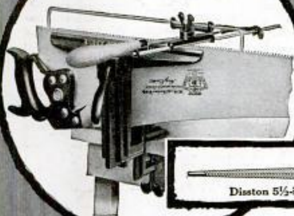
Disston D-3 Saw-Filing Guide
