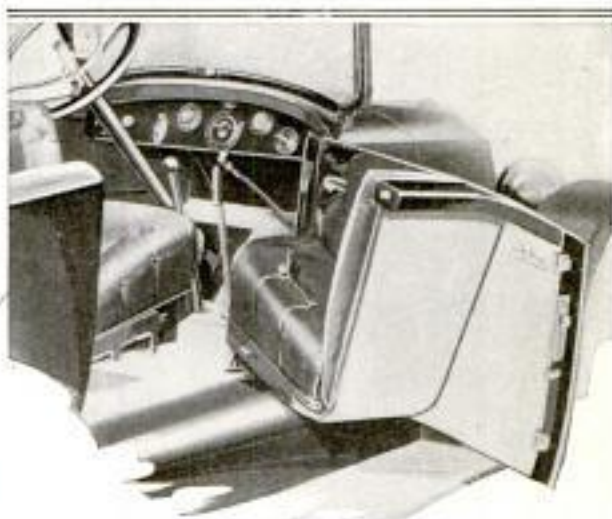
New Type of Roadster Door Which Gives Direct Access to Front and Rear Seats: With the Door Closed the Two Parts of the Front Seat Fit Tightly Together
