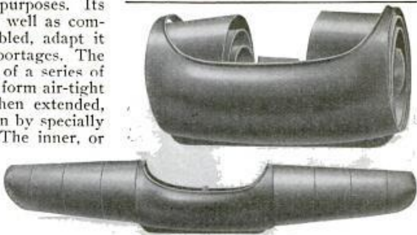
Locked in Place, the Separate Sections Form Air-Tight Compartments. When Telescoped, They Fit Compactly within the Central Hull Member
