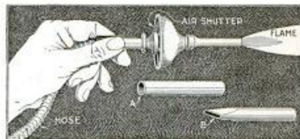
The Mantle Fixture was Quickly Converted into an Effective Bunsen Burner, with a Blowtorch Action, by Flattening the End of the Tube
