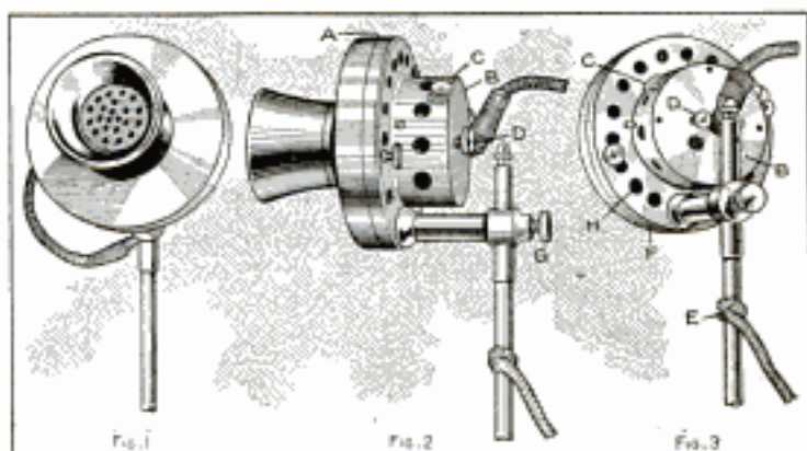
Assembly Views of the Transmitter, Showing the Mouthpiece, the Housing, and the Connections
