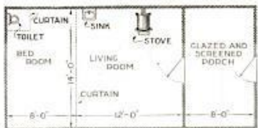
A Rough Floor Plan Showing How All the Cottages are Laid Out: They Are Both Convenient and Inexpensive
