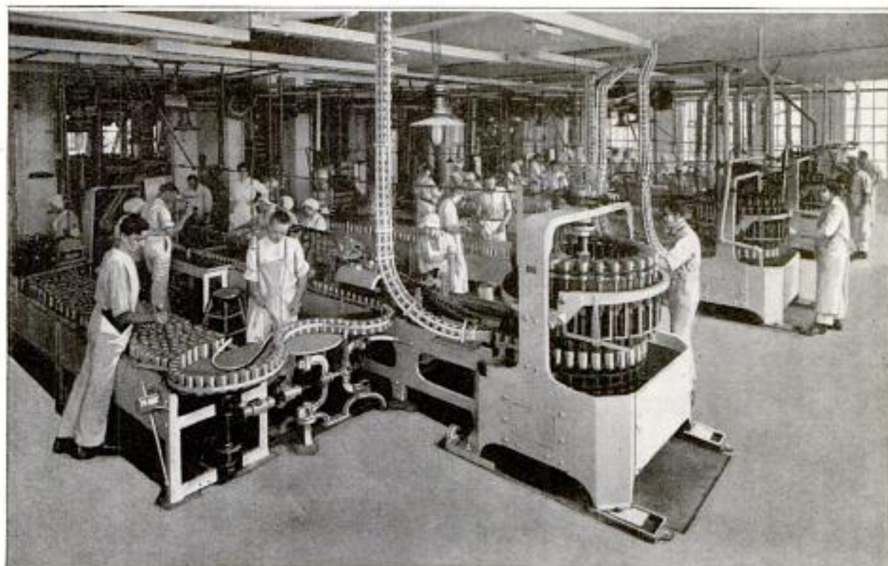
Each of the Machines in This Battery Fills 9,600 Cans an Hour When Operating without Interruption
