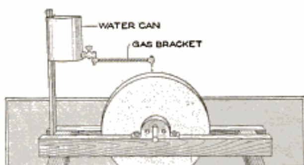
A Serviceable Adjustable Water Spout for a Grindstone was Made Out of an Old Gas Bracket
