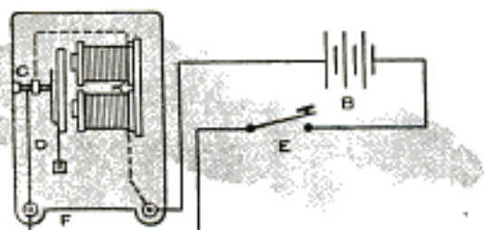
The Amateur can Practice the Morse Code Handily on This Sounder, Made from a Buzzer
