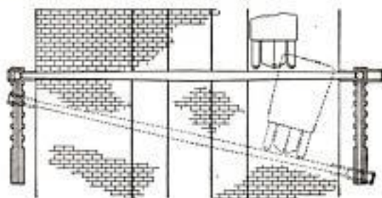
Plan and Side Elevation of Boom, Showing Its Action in Stopping a 4,000-Pound Auto Truck Running at 30 Miles an Hour
