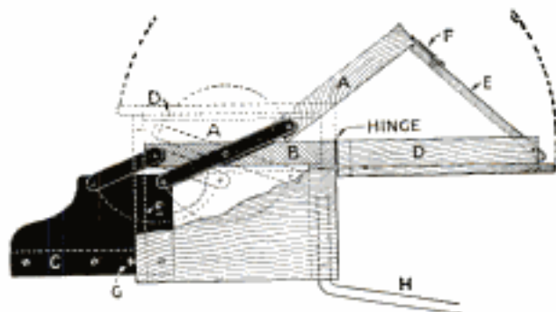
Diagram Showing the Method of Folding the Various Sections into the Cabinet
