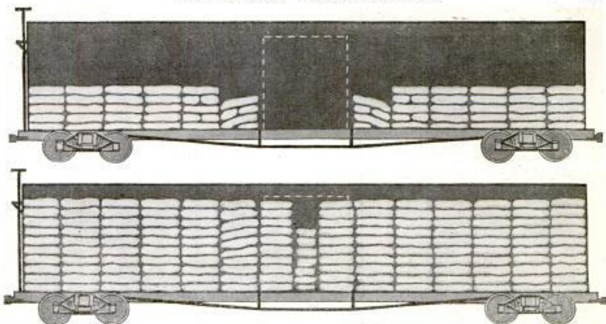
Four Hundred Bags of Sugar are Generally Considered a Carload. The Drawing at the Top Shows Such a Cargo, While That below It Illustrates How the Same Car can be Made to Carry 1,000 Sacks by Simply Utilizing the Available Space
