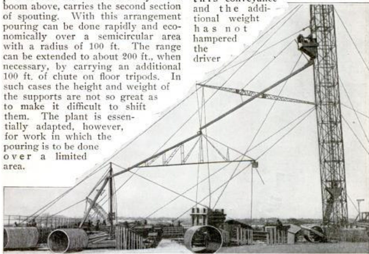
Showing the Easily Shifted Gravity Concrete-Chuting System as Used in Erecting a Warehouse for the Harbor Commission of Los Angeles
