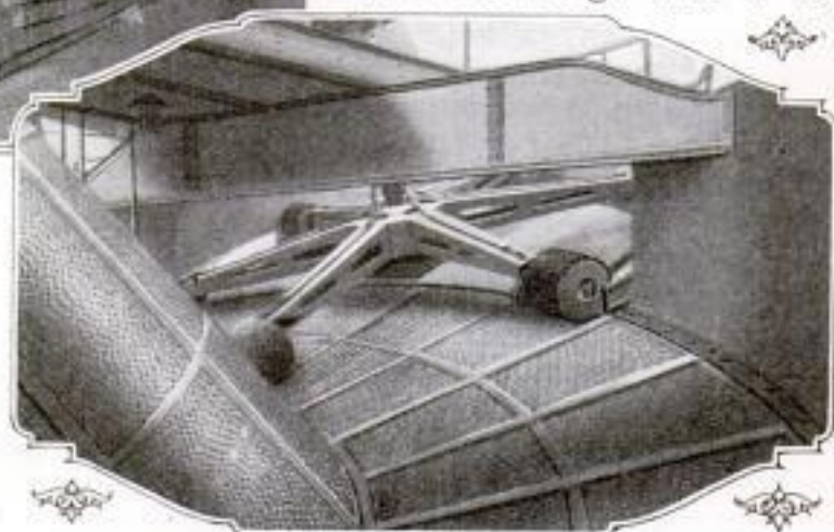
View of the Revolving Screen That Separates the Solid Matter from the Fluid Sewage, and the Rotating Brushes That Discharge It into Troughs
