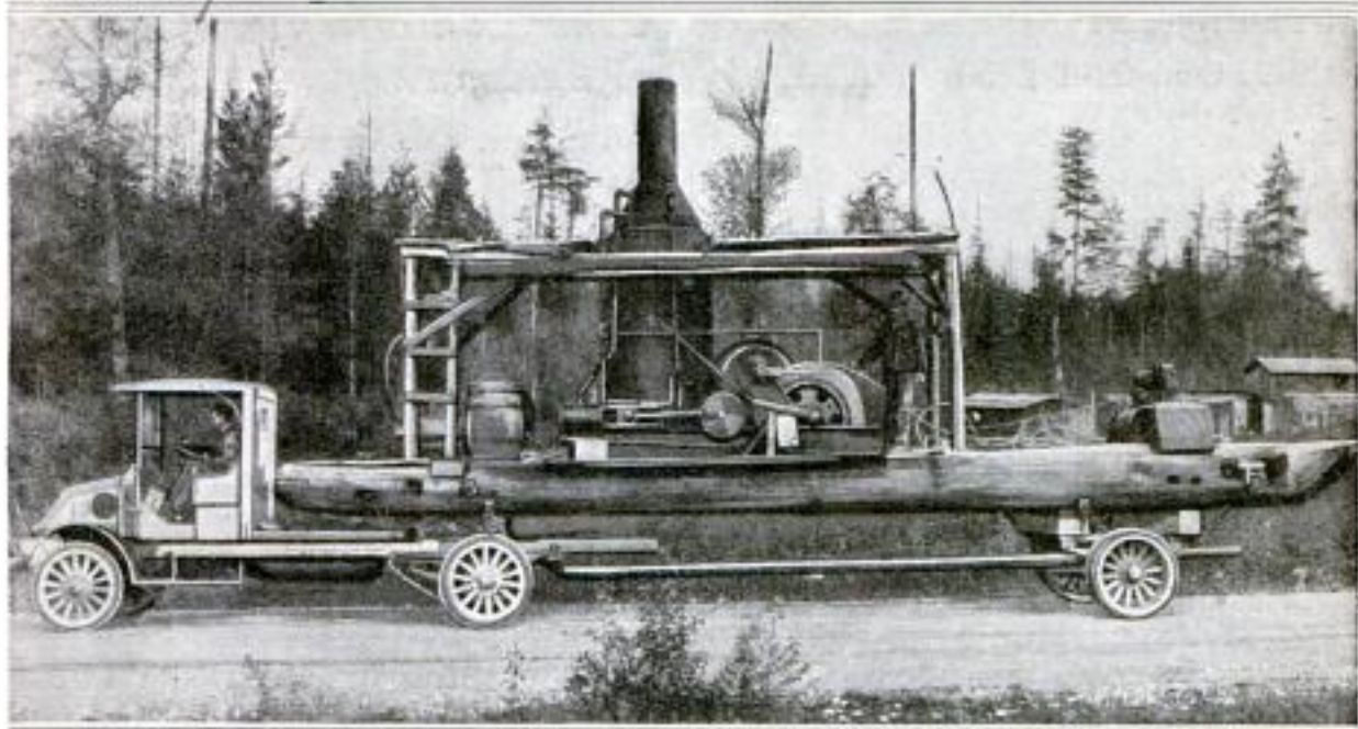
Carrying a 15-Ton Donkey Engine on a Motor Truck in the Washington Woods
