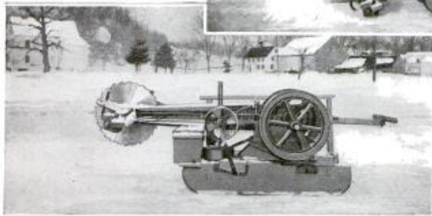
With This Circular Saw and Motor Mounted on a Sled a Maine Man and One Helper Cut from 10 to 15 Tons of Ice an Hour
