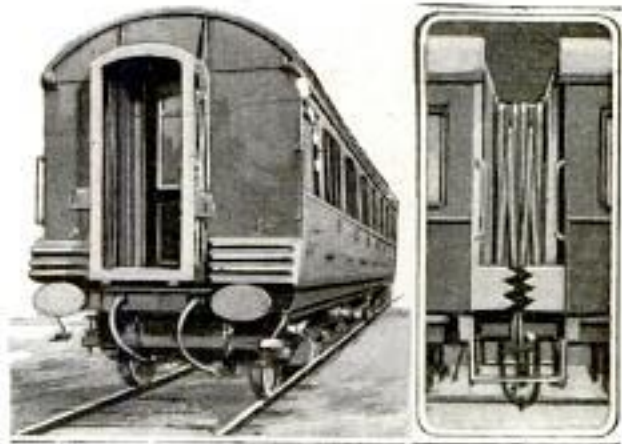
End and Side Views of Corrugated Fenders on English Train, Designed to Keep the Coaches in Alinement in Case of Collision, Thus Preventing Telescoping
