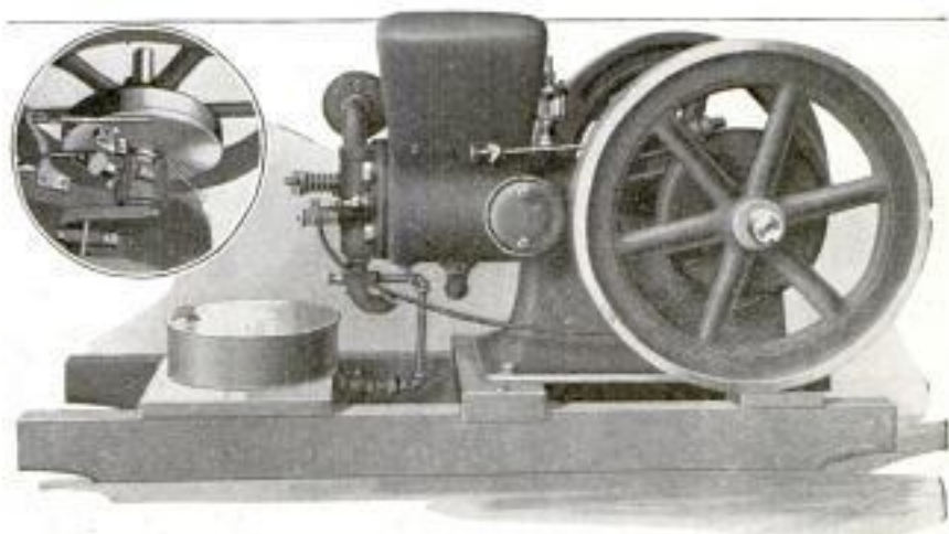
Gas Engine with New Circular Type of Magneto, Which may be Seen Mounted on the Crankshaft Inside of the Flywheel
