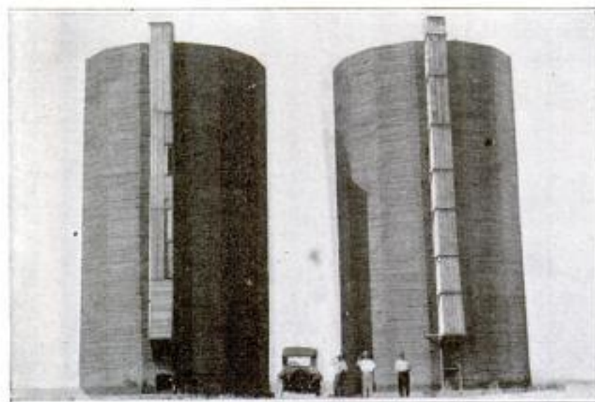
Two Big Silos on a Kansas Farm, Each Having 14 Sides, Made Entirely of Two-by-Fours Laid on Their Sides and Spiked Together. They Have a Combined Capacity of 1,020 Tons
