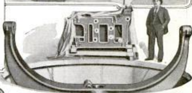
Elevator Installed beneath Telescope to Facilitate Removal of Reflector to Laboratory Below, Where the Periodical Resilvering of Its Surface will be Accomplished. Before Removal from the Instrument, the Mirror's Housing is Bolted to the Elevator's Uprturned Arms
