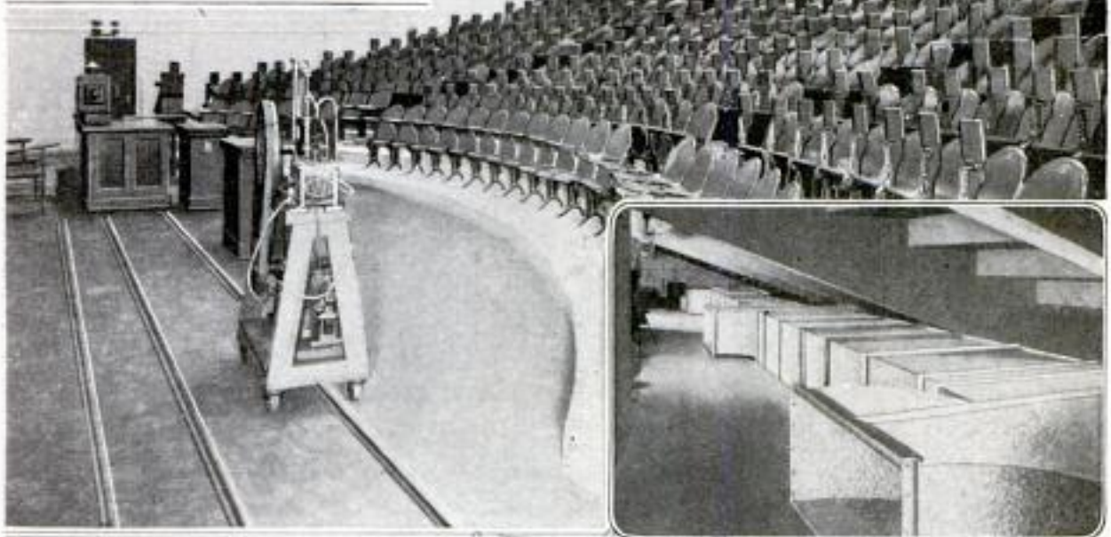
New Lecture Room, Massachusetts Institute of Technology: This Hall Seats 700 Students. At the Left Are Tracks for Bringing In Apparatus. The Insert Shows the Ventilating Chamber
