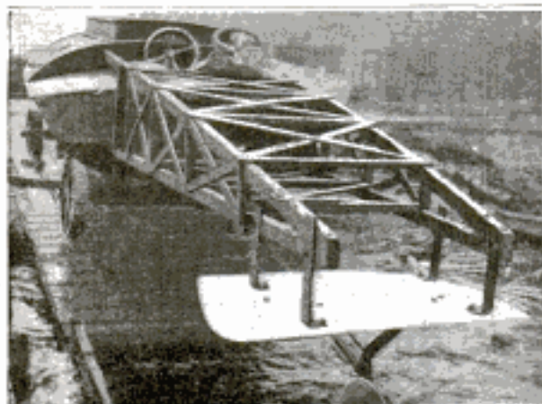
Rear View of Motorboat Extension, Showing the Metal Shield over the Propeller and the Construction of the False Stern
