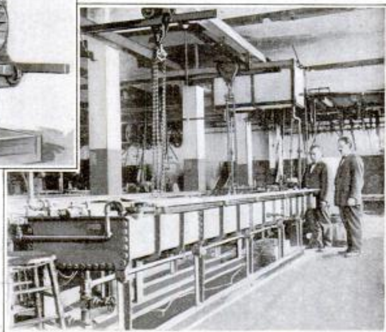
A Machine Which Cooks Sardines in Boiling Olive or Cottonseed Oil, Brought to the Required Temperature by Superheated Steam, and Discharges Them at the Rate of 65 Cans per Minute
