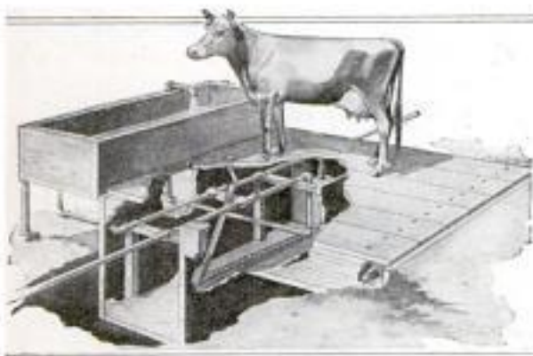
This Watering Trough is Filled Automatically When an Animal Steps on the Platform, and Emptied When It Steps Off. The Operating Valve Mechanism is under the Platform near the Trough
