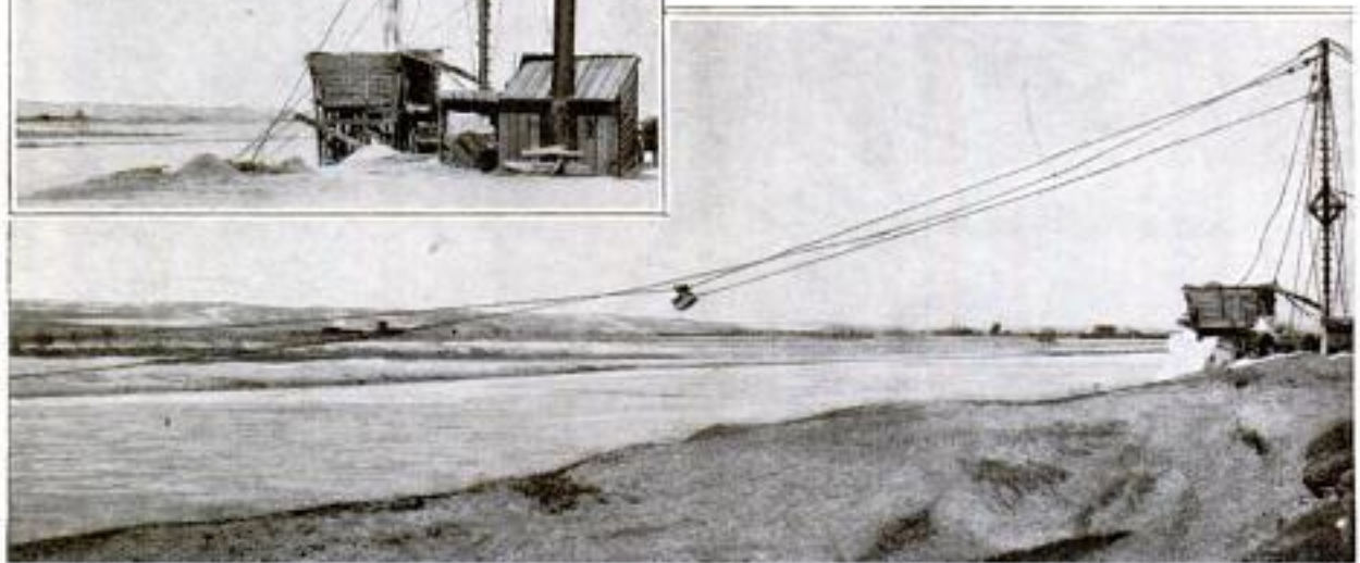
Aerial Tramway That Transports Gravel across the North River in Wyoming, Thereby Saving a Two-Mile Haul with Wagons. The Bucket, Shown Above Discharging Its Contents into the Hopper, Makes the Round Trip in About Two and One-Half Minutes
