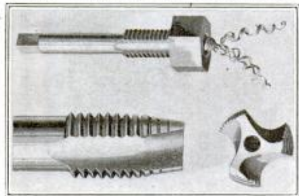
Views of New Tap Showing Flutes of Special Design Which Give the Tool Great Durability and Enable It to Operate with Less than Ordinary Pressure
