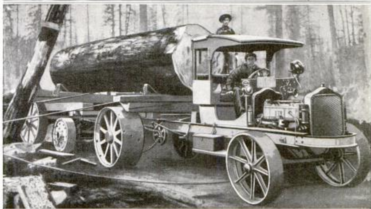
Wide-Tired Truck, with Trailer, Which Makes a Smooth, Hard Track as It Goes. The Outfit is Equipped with a Winch Which is Used in Loading the Logs and in Emergencies en Route
