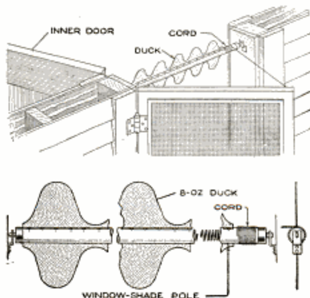
The Scalloped Roller is Revolved Rapidly When the Door is Opened, Frightening Flies
