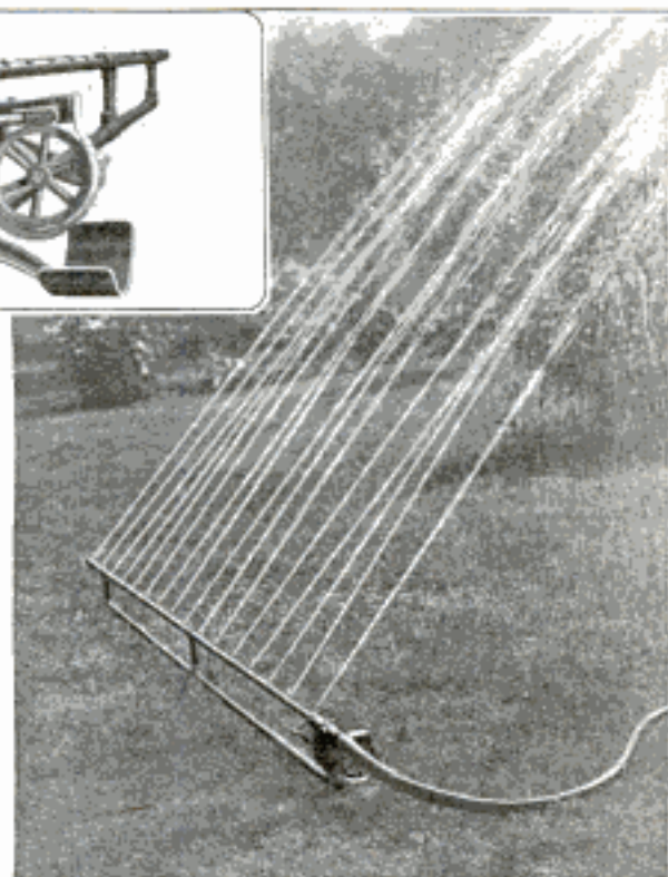
New Lawn Sprinkler in Operation: The Photograph at the Left Shows Details of Its Construction, Including the Turbine, Worm Shaft, and Wheel That Swings the Outlet Pipe in a Semicircle
