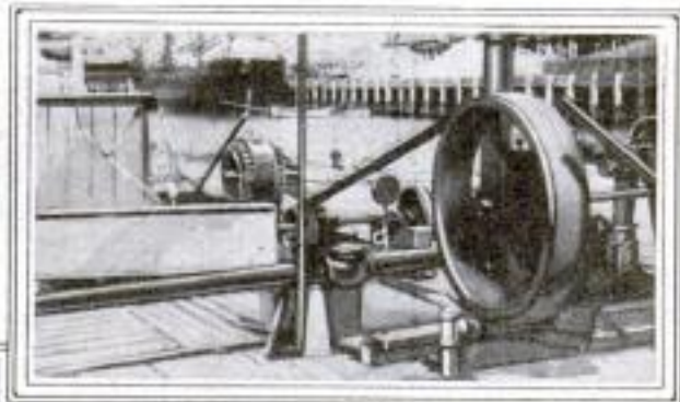
Above: View on the Deck of the Barge, Showing the 18-Horsepower Pumping Plant
