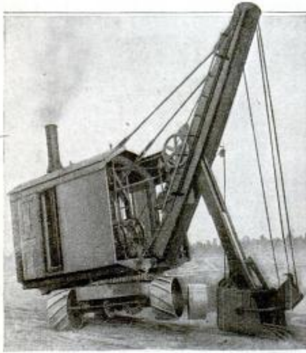
This Shows How a Steam Shovel was Raised from the Ground by Its Own Power, So That Planks could be Inserted under the Wheels. With the Bucket Lowered to the Ground, the Power was Turned On, Which Tilted the Whole Machine
