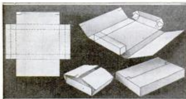
How the New One-Piece Folding Paper Box is Made: At the Left is a View of the Paper Blank, Then the Box is Seen in Process of Construction, and Finally the Box Completed and Locked
