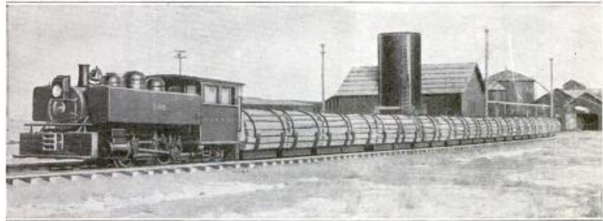
COURTESY OF ENGINEERING NEWS The Cars of This Novel Train are Loaded with Ties and are Designed Especially to be Backed into a Long Cylinder, in Which They and Their Load are Immersed in a Solution That Prolongs the Life of the Timbers
