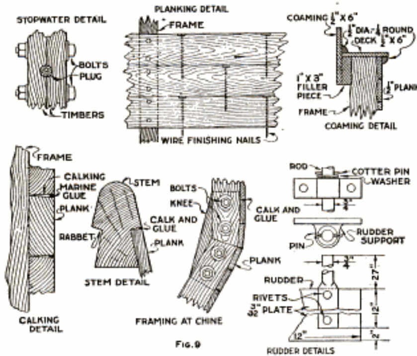
Fig. 9 Details for the Rudder, Coaming, Stopwater Plug, and Other Constructional Features
