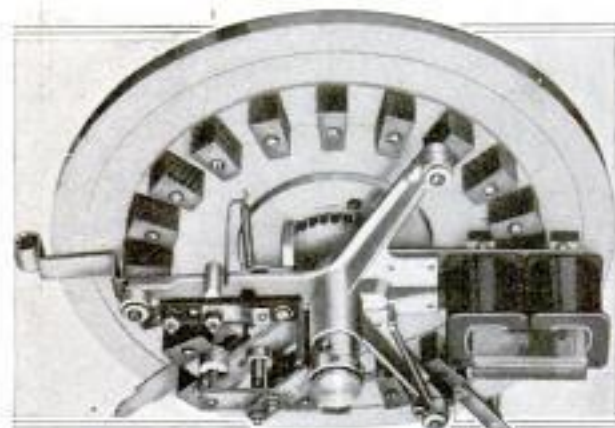
This Illustrates the Combined Turntable and Armature, an Arrangement That Permits Smooth Motion and Obviates Gearing
