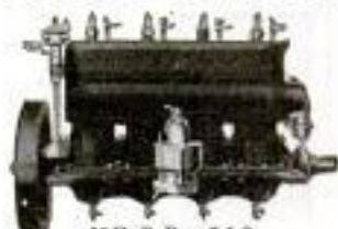
10 H. P. Bore 1-2 Inch Stroke 4-inch Net Price $240.00
