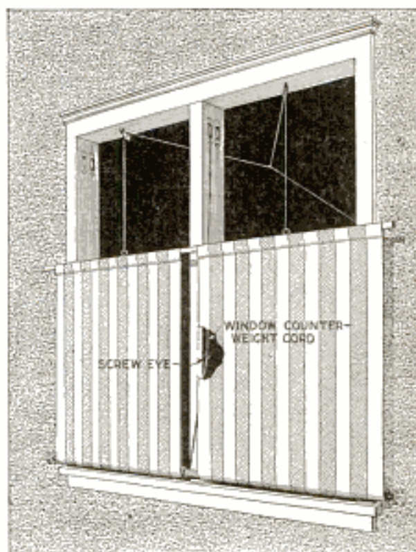
The Curtains are Held Taut and Rolled by the Center Cord Fixed to a Sash Weight
