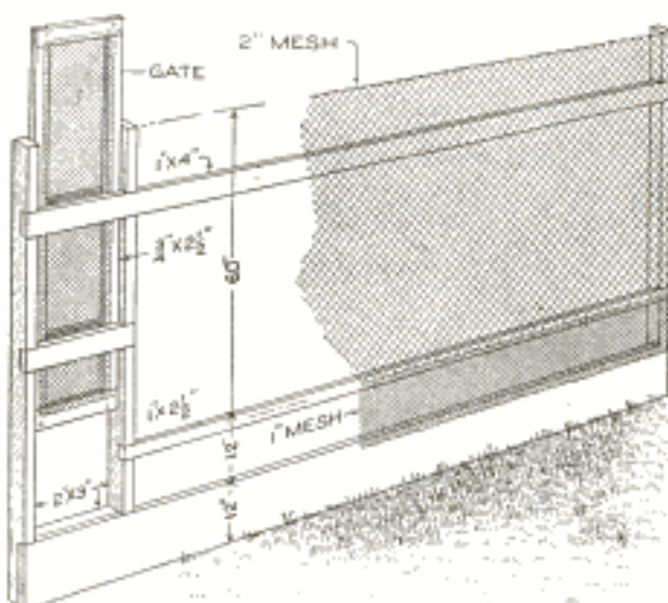
Poultry Fencing Made in Portable Sections Has Several Advantages over a Stationary Barrier
