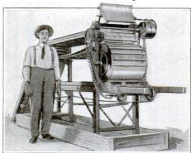
This Invention Dispenses with the Labor of a Large Number of Children Formerly Employed to Arrange Herring on Racks Preparatory to Sending the Fish to the Cooking Machines
