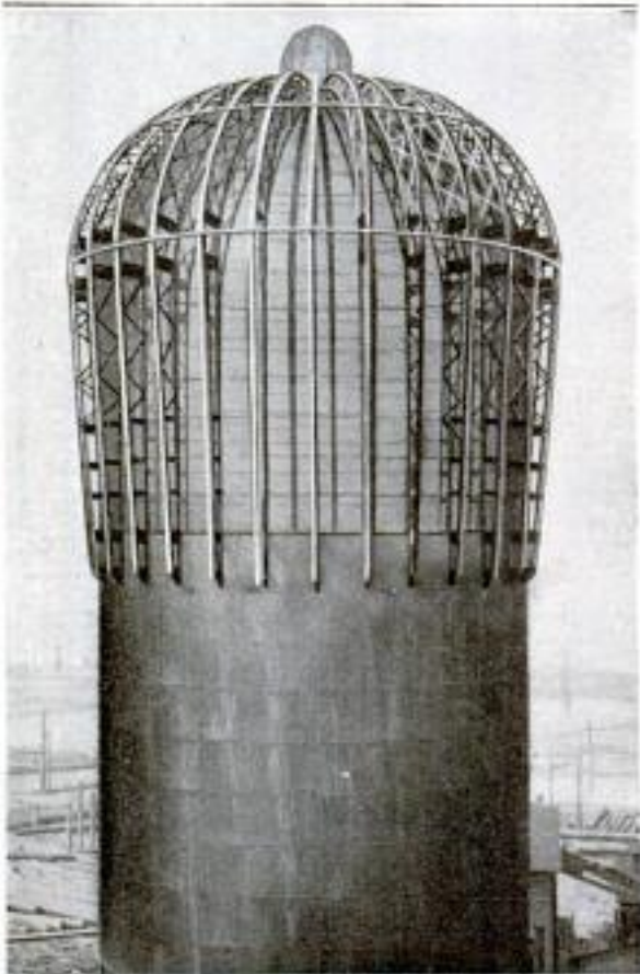
New Type of Refuse Burner for Sawmills, Having a Screen Top Held in Place by an Outside Framework Composed of Curved Trusses
