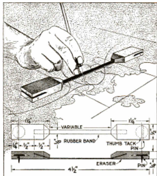
This Simple Device Is Useful in Enlarging or Reducing Drawings and Maps
