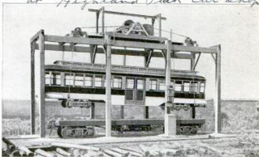
Hoisting Equipment Used to Lift Street Cars and Heavy Machinery on and off Freight Trains. It is Electrically Operated and with It Two Men can Do the Work of a Large Crew
