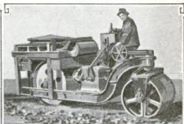
Roller Used on the Streets of St. Louis Which Derives Its Power from a Near-By Trolley Wire, View at Left Showing How the Cable is Attached to the Trolley Wire
