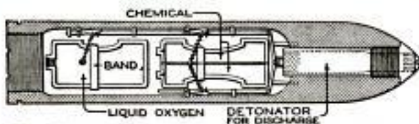
The Diagram Shows the Design of the Projectile and Indicates How Its Internal Mechanism is Operated
