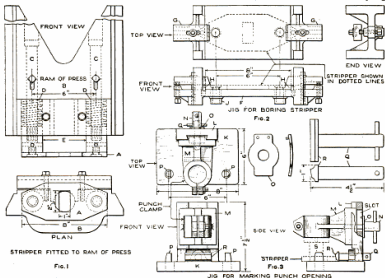
The Spring Stripper Makes for Safety, Economy in Production, and a High Grade of Work on Power Presses. Fig. 1 Shows the Stripper Fixed to the Ram of the Press. A Jig for Boring the Fastening Holes in the Stripper is Shown in Fig. 2, and a Jig for Marking the Clearance Hole for the Punch is Shown in Fig. 3, with Details of Parts
