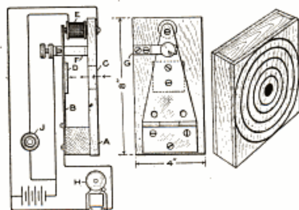
Fig. 1 The Bullet Forces the Hinge against the Thumb-screw, Causing the Bell to Ring
