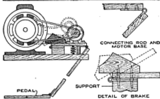
The Motor is Controlled by Pressure on the Pedal, the Brake at the Same Time Acting on the Flywheel
