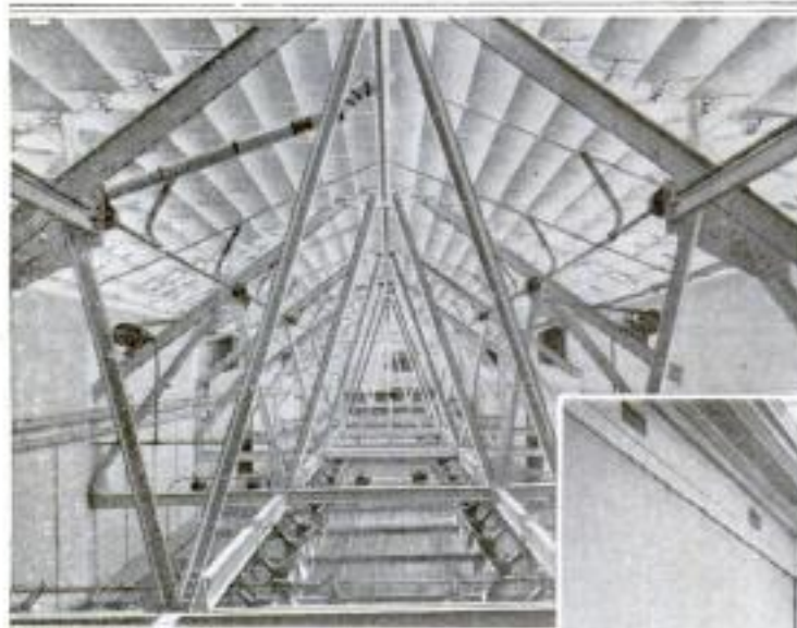
This Shows the Arrangement of the Hooded-Reflector "Daylight" Lamps between the Skylight and the Subskylight of the Cleveland Museum of Art
