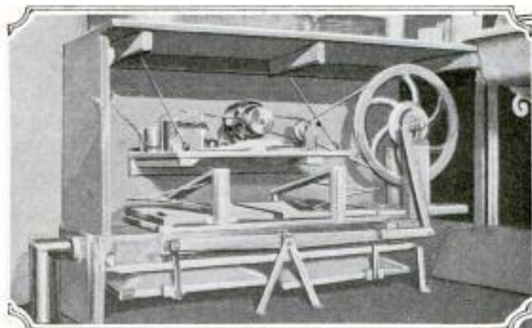
Motor and Homemade Bellows Installed in a Cabinet in the Kitchen, Which Supply the Organ with Air
