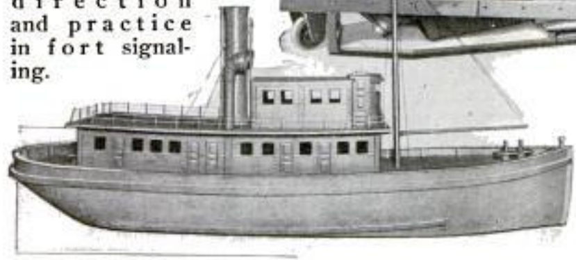
This Miniature Boat is Self-Propelled by Electricity and Moves about an Armory Floor to Furnish a Target for Coast-Artillery Practice in Vessel Tracking: The Concealed Operator and Mechanism are Seen Above
