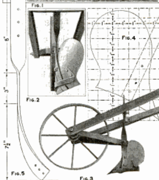
This Hand Garden Plow was Made of Old Material, a Shovel being Used for the Making of the Moldboard
