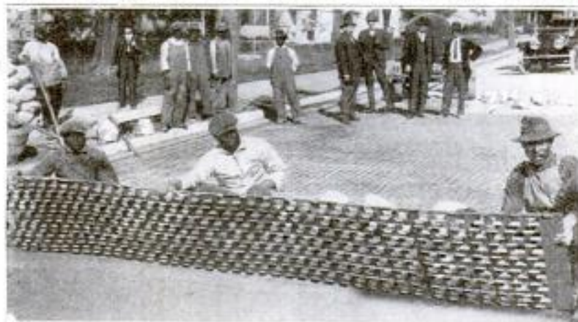
Laying a Steel Pavement on a Street in Charlotte, North Carolina: The Workmen in the Foreground Are About to Place the Pressed-Steel Sheet on Its Bed of Soft Concrete. A Completed Surface is Seen behind Them
