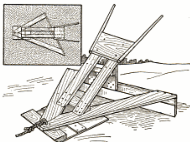
A Tennis Court was Smoothed and Leveled by the Use of This Scraper, Made Quickly of Rough Lumber
