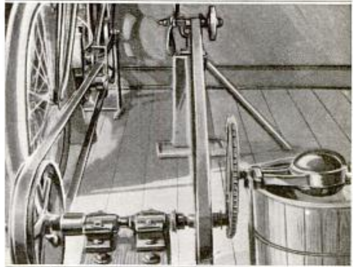
FIG. 1 Grinder, Fan, and Ice-Cream Freezer Driven by a Motorcycle Engine, the Speed Adjusted by Pulleys and Gears
