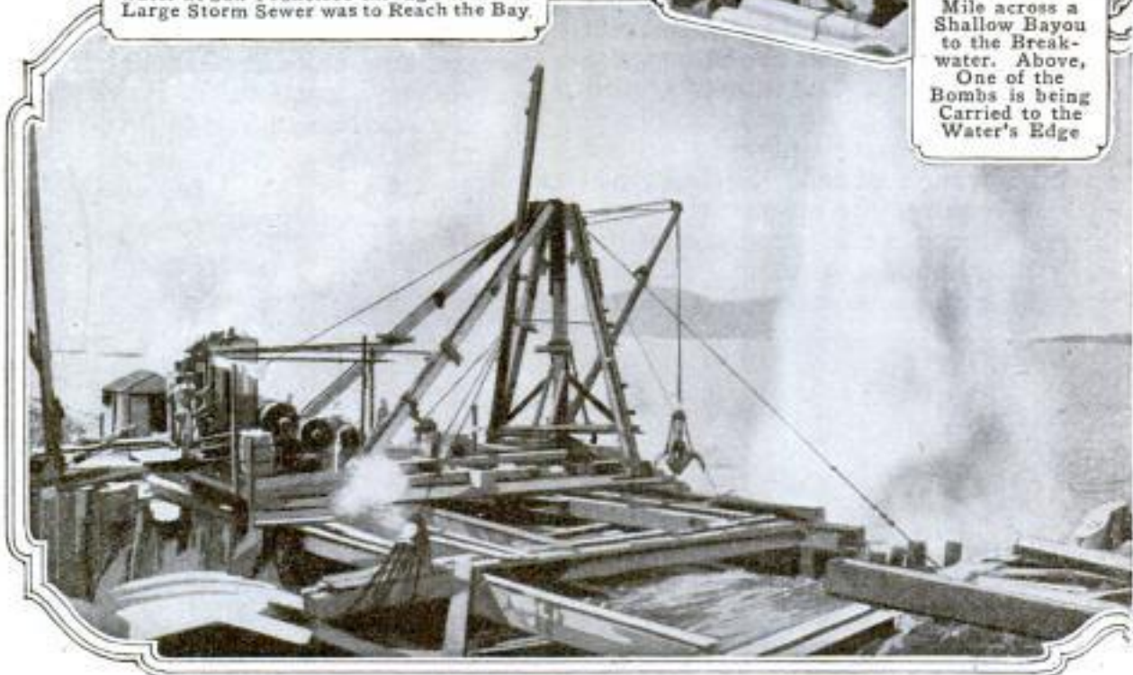
A Section of Sewer Pipe and Plenty of Dynamite Makes a Good Bomb. The Blasting was Done for the Purpose of Making an Opening in a Stone Breakwater at San Francisco through Which a Large Storm Sewer was to Reach the Bay.
