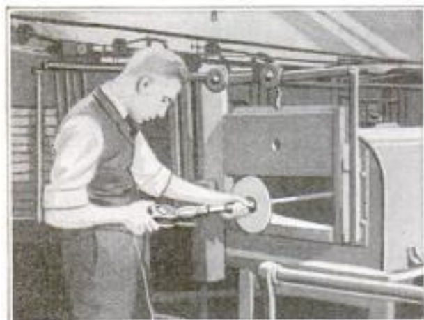
A Device Which Indicates When the Critical Point has been Reached in the Heat Treatment of Steel by Testing It for Its Magnetism
