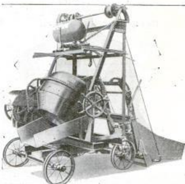
It Is Only a Matter of 10 Minutes' Work to Shift This Machine so That It Discharges from Either Side Instead of from the End. This Change is Made without Moving the Truck
