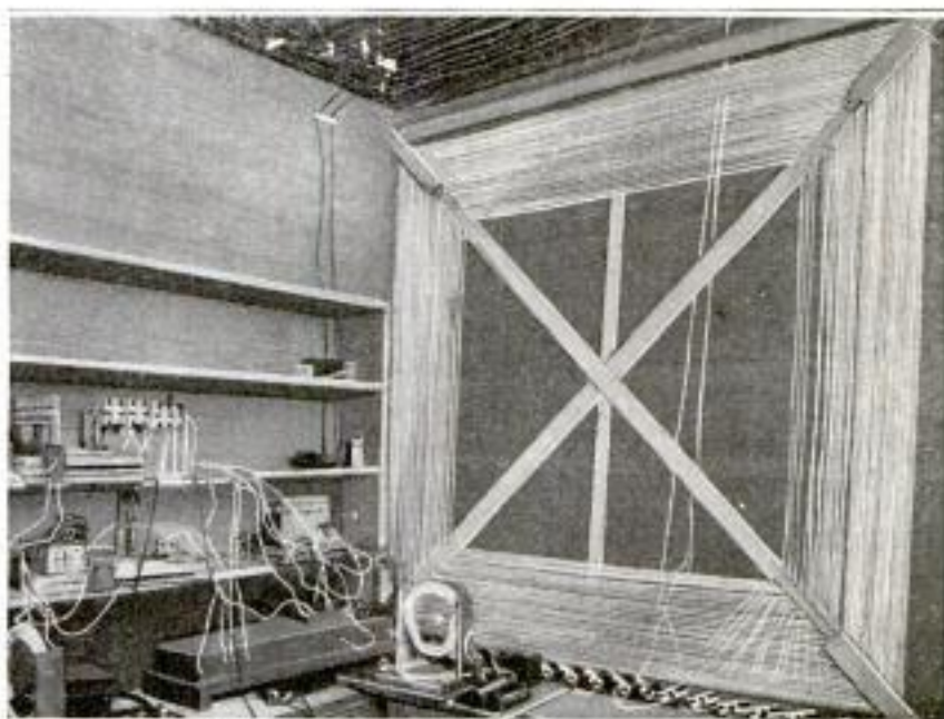
View in an Electrical Laboratory of Union College, Showing the Big Square Wireless Receiving Apparatus Which Operates Regardless of Weather Conditions and with Which can be Determined the Direction from Which a Message Comes
