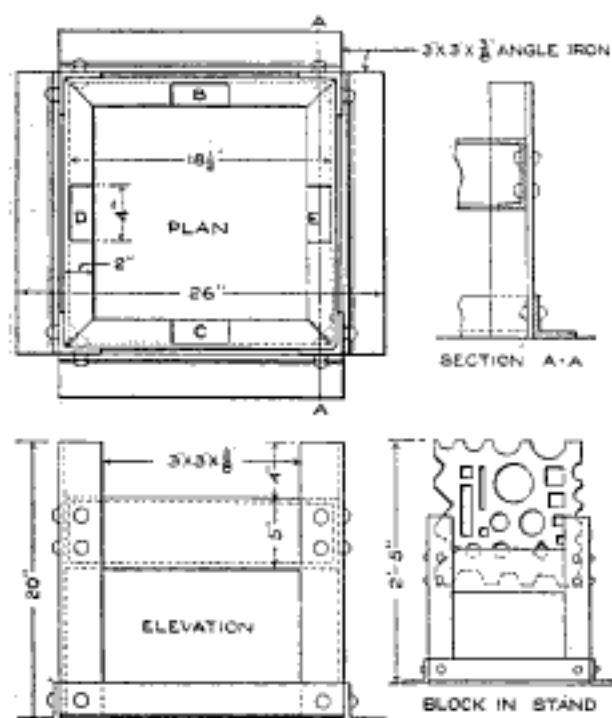
This Strong Frame Increased the Usefulness of the Swage Block
