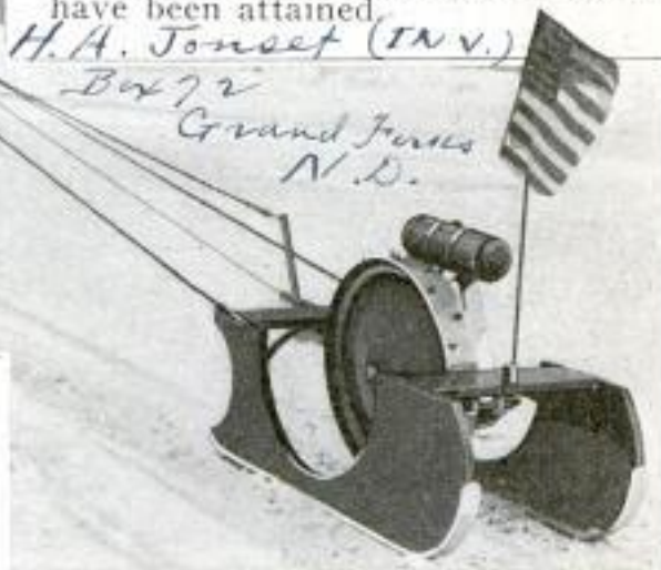
With This "Motor Horse" the Driver has Traveled as Fast as 40 Miles an Hour on Skis, as Seen in the Picture. The Motor is Concealed in the Studded Wheel and Controlled by Lines in the Driver's Hands, Attached to a Lever, as Shown. The Other Lines Serve for Towing
