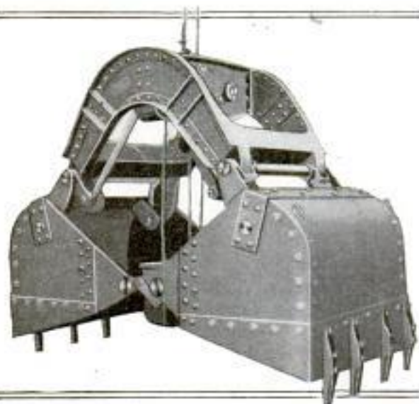
New Type of Clamshell Bucket Having a Steel Arched Yoke and Other Features Which Give It Compactness and Strength
