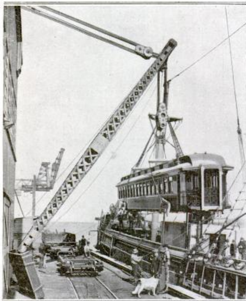
Passenger Cars for the Government's New Railway Lines in Alaska being Loaded onto Steamer at Seattle
