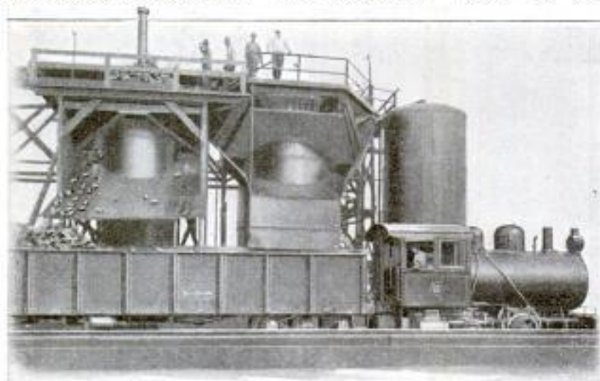
Instead of being Generated by It, Steam is Pumped into This Engine under High Pressure and in Sufficient Volume to Permit Operation for an Entire Day
