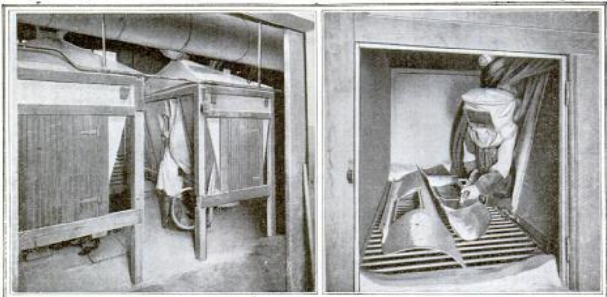
Improved Method of Sand-Blasting, Which Compels the Workman to Don the Safety Helmet to Get at the Work inside the Hopper: He Stands Outside, as Seen at the Left, with Head and Arms Protected Inside, as Shown at the Right
