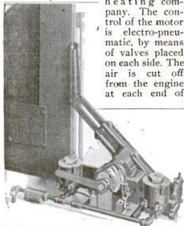
Pneumatic Motor Which Opens or Closes a Railway-Car Door and is Controlled by a Push Button
