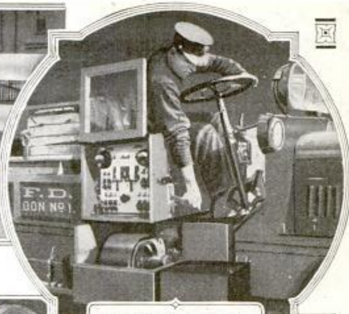
In This Photograph the Driver is Shown in the Act of Throwing the Generator into Gear to Furnish Current for the Searchlights on the Squad Wagon, Two of Which Are Portable. Above the Generator is the Switchboard by Which the Searchlights are Controlled
