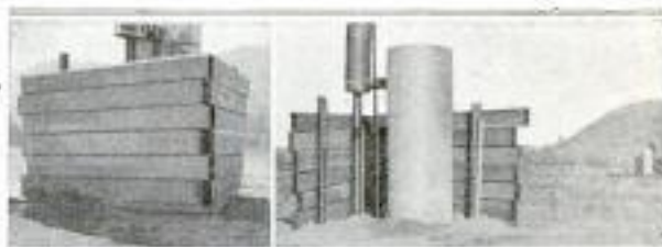
Timber Wedges Provided to Protect Wells in a Dry California River Bed against Flood Damage in Winter
