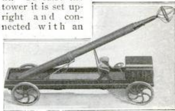
Portable Telescoping Tower for a Wireless Outfit: It can be Extended in Less than a Minute by Pumping Compressed Air into It
