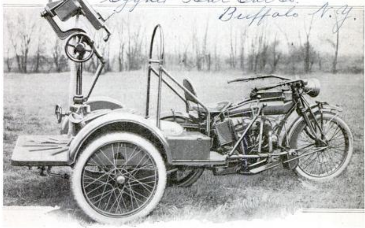
With This New Gun Carrier for Motorcycles the Machine Gun may be Used in Ground Battles, Elevated as in the Picture, or Depressed for Downward Shooting, and Swung around an Entire Circle if Necessary. The Outfit can be Operated by Two Men and Both Car and Gun are Quickly Detachable
