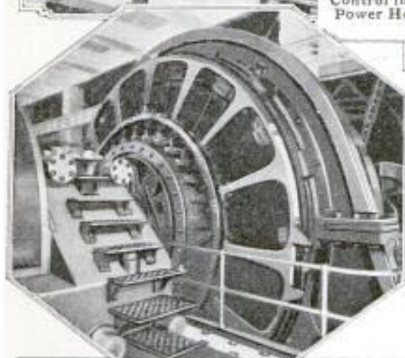
One of the Six Huge Electric Generators Installed in the New Power House of a Detroit Automobile Factory: They Are the Largest 250-Volt Machines of Their Kind Ever Built and Each of Them could Light More than 90,000 Tungsten Lamps
