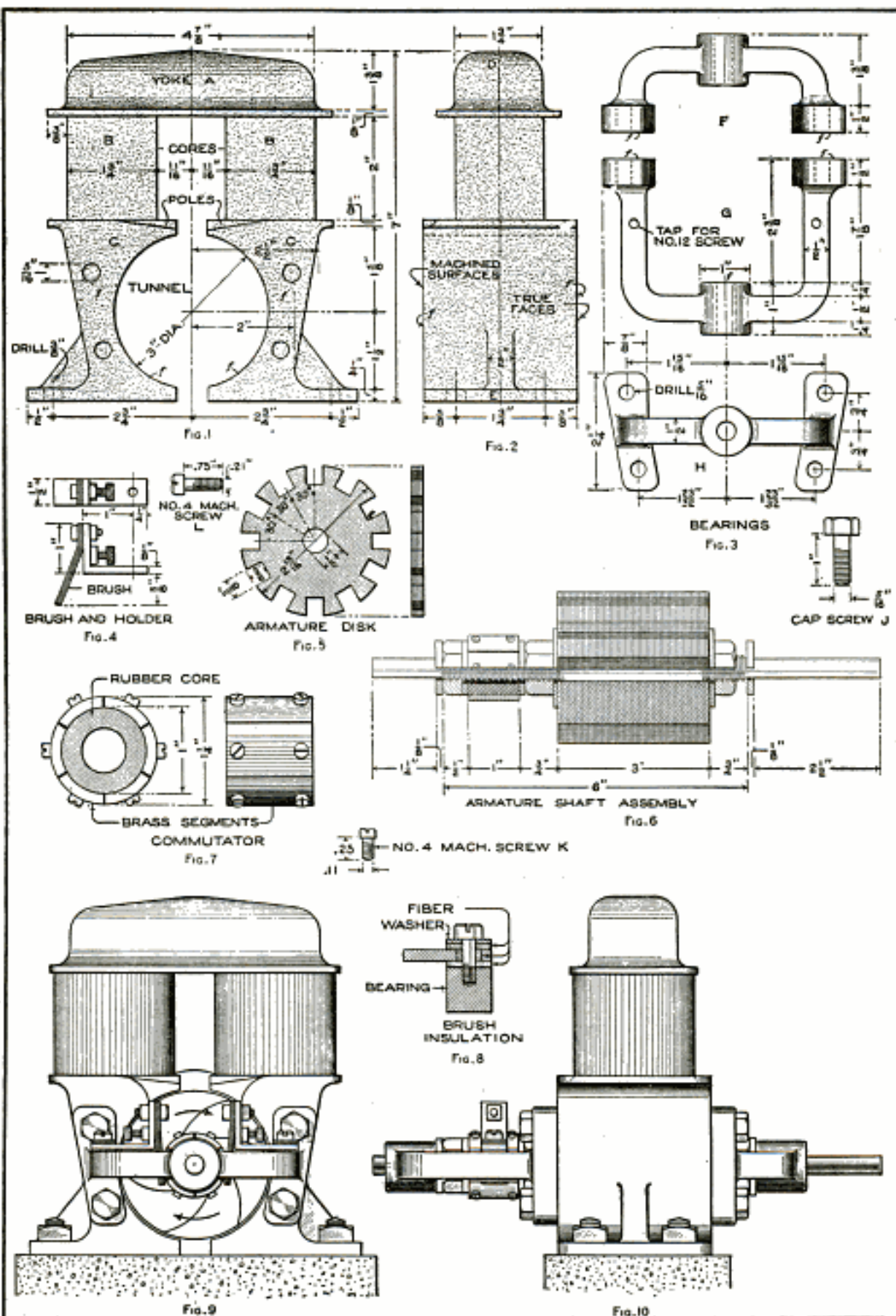
The Assembly Drawings, Figs. 9 and 10, Show the General Arrangement of the Parts, and the Working Drawings Present the Details of Construction. The Pattern for the Field Magnet, Shown in Fig. 1, is Built Up of Five Parts: The Yoke, Cores, and Poles. It is Cast in Gray Iron of Fine Texture, and the Bearings, Shown in Fig. 3, are Cast in Hard Bronze
