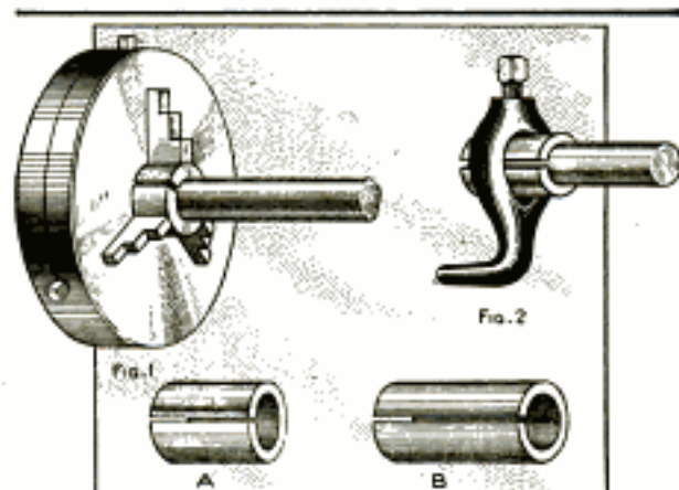
The Smoothly Turned Split Bushings Protect Highly Polished Spindles in the Chuck or Lathe Dog
