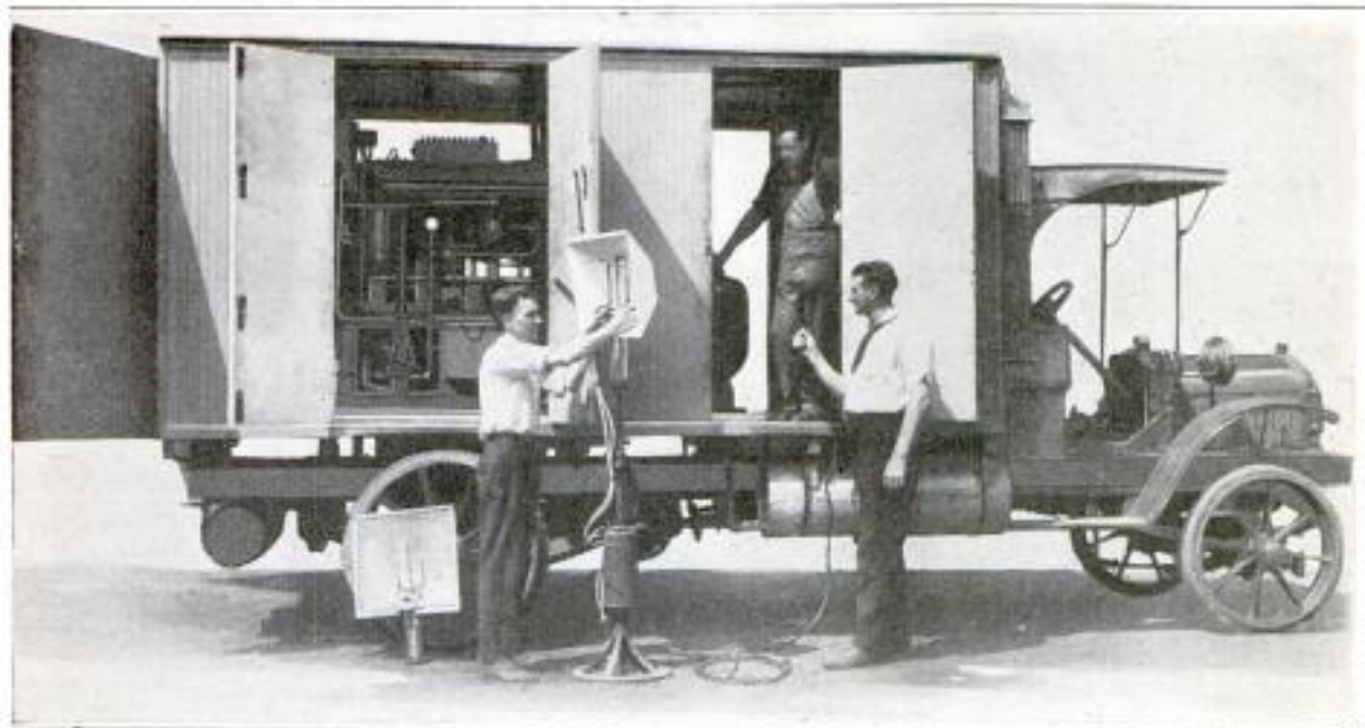
This Portable Lighting Plant Facilitates the Filming of Movie Dramas, Staged in Remote Sections Away from Electric-Transmission Lines
