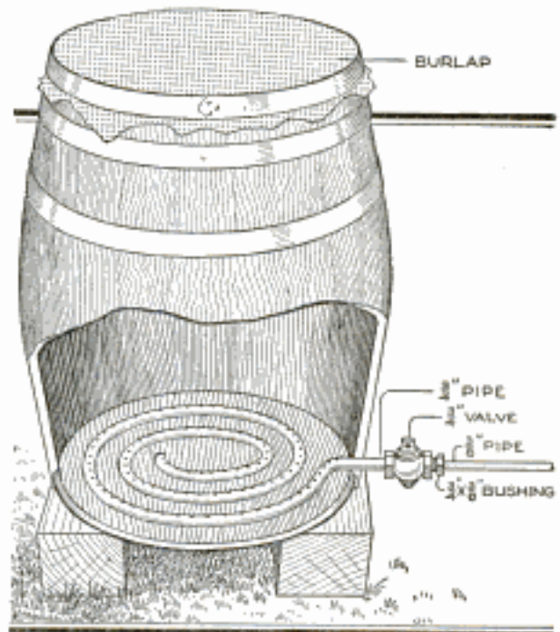
Sand to be Cleaned is Placed in the Barrel, the Air is Turned On, and the Dust Blown Out through the Burlap Covering
