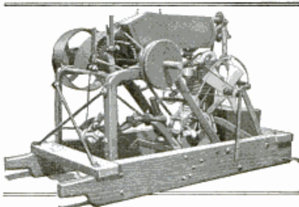
An Old Motorcycle Engine was Mounted on a Frame and Skids for Use as a Stationary Engine That could be Moved Readily
