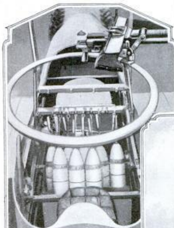
COPYRIGHT, UNDERWOOD & UNDERWOOD Cockpit of a French Military Aeroplane, Showing Store of Bombs Ready for Launching, and Novel Mounting of Machine Gun. The Latter is Held on a Revolving Ring so That It may be Fired in Any Direction
