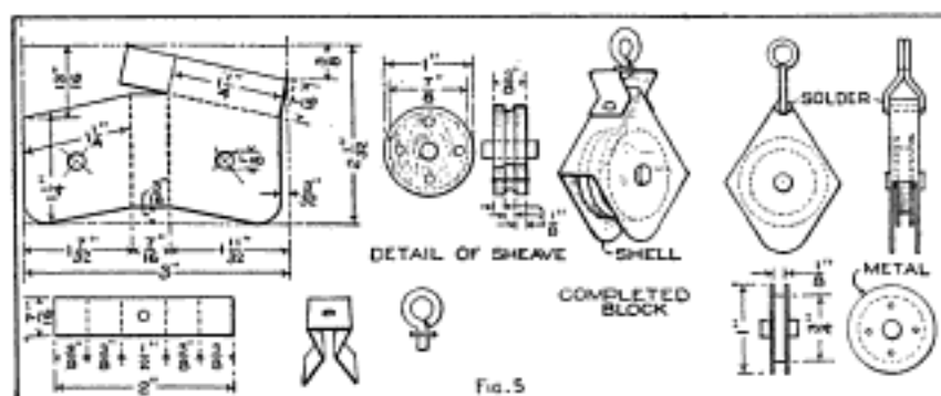
Two Simple Methods of Making the Blocks: The Sheaves are Made of Wood or Metal; the Shells are of Metal Fitted to the Sheaves
