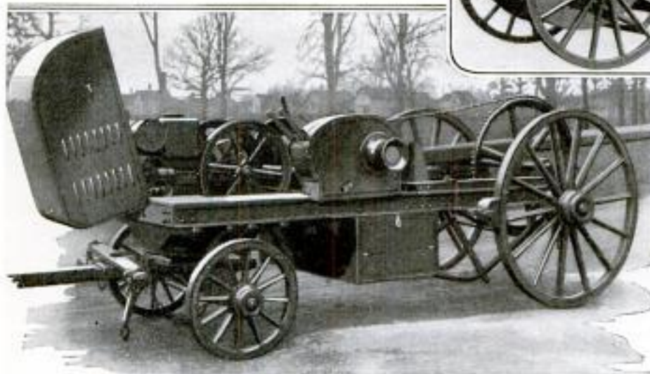
Two Views of the Telephone Construction and Cable-Handling Apparatus, the One Above Showing a Reel in Place for Unwinding, and That at the Left Indicating How the Derrick is Mounted. In Addition to Placing and Removing Poles, the Equipment is Arranged to Pull Lines through and Out of Underground Conduits and Do Other Work. It is Said to Cut Labor Cost Materially
