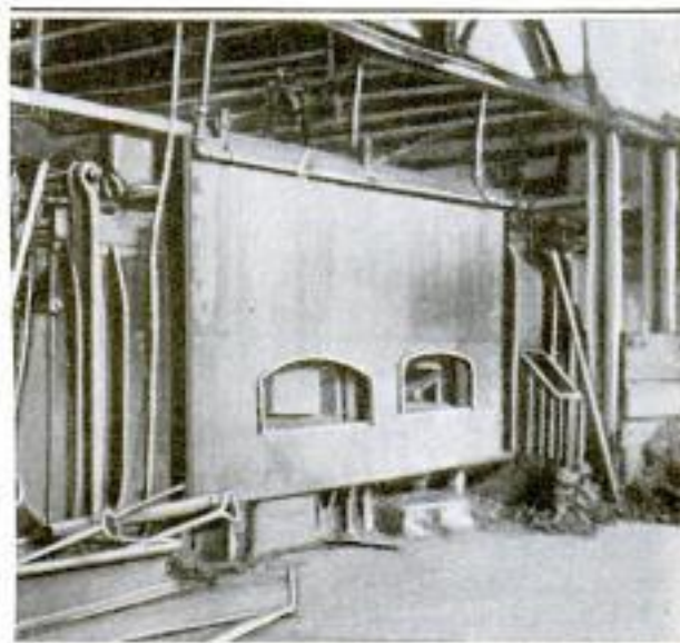
Sheet-Metal Shield Hung from a Track in Front of a Furnace: Down the Front of the Curtain Flows a Thin Sheet of Water to Protect the Workmen from the Intense Heat
