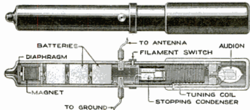
Having the Size and Appearance of a Large Fountain Pen, This Is in Reality a Miniature Radio Receiver
