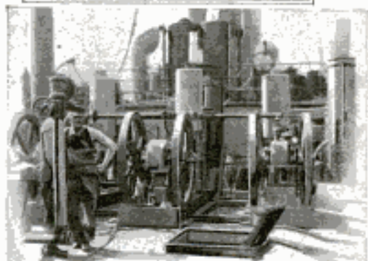
Trying to Raise the Wreck of the "Hector": At the Left, a Navy Tug Standing by the Wrecking Barges. At the Right, a Battery of Air Compressors Installed on the Wreck to Clear the Holds of Water
