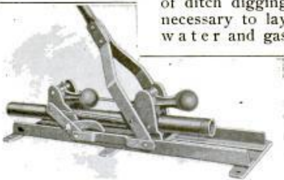
A Machine with Strong Leverage That Forces Pipe through the Ground, Thereby Lessening the Amount of Digging Necessary to Lay the Pipe
