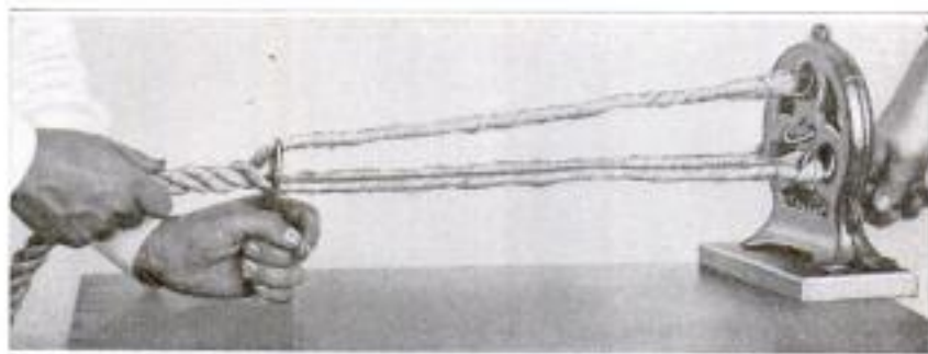
Making Rope from Binder Twine: A Simple Machine Which Twists the Strands About One Another. The Threader, at the Left, is Used to Keep the Strands Separate and to Make Them Twist Evenly
