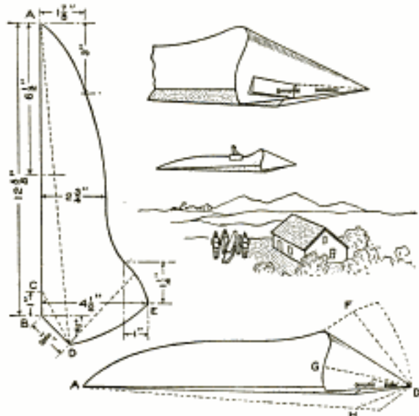
The Glider will Travel 30 Feet, Carrying a Message, if Carefully Made
