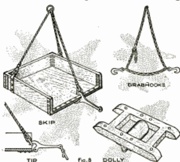
The Grab Hooks are Used with Chains in Handling Steel, Blocks of Stone, and Various Heavy Objects; the Trip Skip for Dirt and Bulk Material, and the Dolly in Bringing Certain Loads within Range of the Derrick
