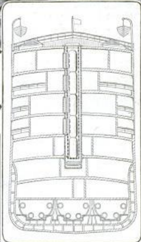
Cross Section of Ship Showing Central Shaft in Which the Separate Vaults are Carried. Doors in the Casings at Various Decks Give Access to Safes
