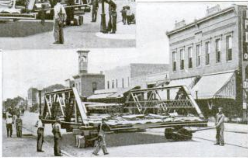
Above Is a Rear View and Below Is a Front View of a 60-Ton Highway Bridge on Its Journey of Two and One-Half Miles through Missouri Valley, Iowa
