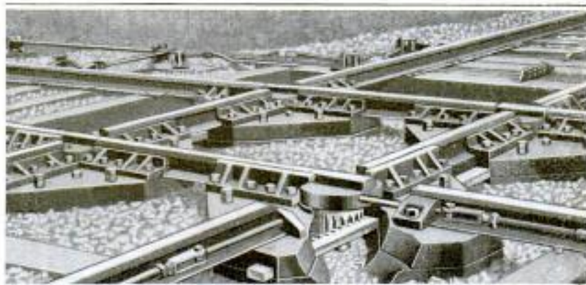
Railroad Crossing Having Four Short Rails at the Intersections, Which are Used to Make Either of the Two Tracks Continuous. The Cost of Operation and Maintenance Is Small
