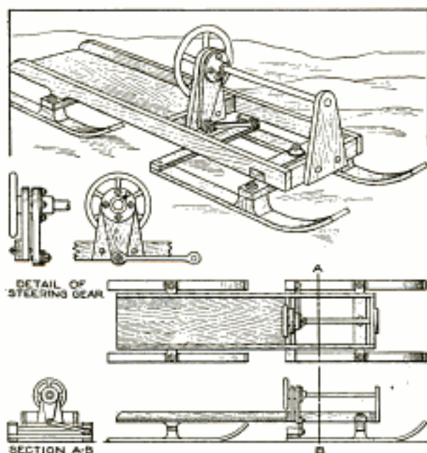
Turn the Wheel Slightly and the Runners are Turned Correspondingly by the Arm and Lever Fixed to the Rear Brace
