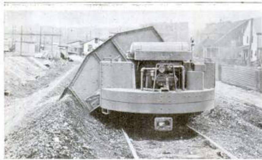
Dump Car Having an Electrically Operated Body Which Moves to One Side before Dumping, so as to Leave the Track Clear. The Capacity of This Dump Car is 18 Cubic Yards. Safety and Efficiency are Promoted by the Fact That the Tilting Body is Always under Full Control of the Motorman
