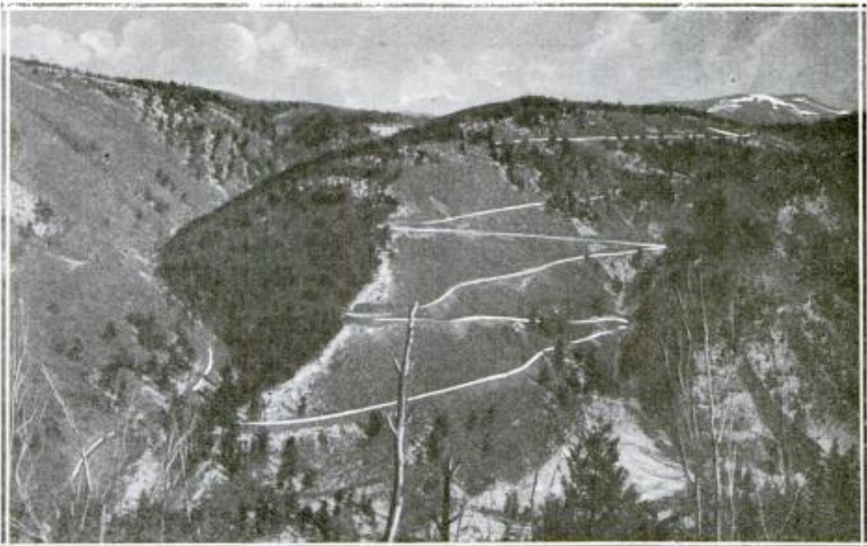
This New Government Road in Taos County, New Mexico, with a Maximum Grade of Seven and a Half Per Cent, Replaces an Old One Nearly Four Times as Steep
