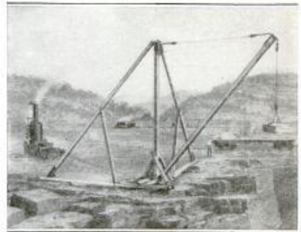
Fig. 1. Lifting Stone from a Quarry: The Boom is Slew'd by Means of the Bull Wheel and Rope Drive Connecting It to the Steam Hoist; Grabhooks Grip the Load
