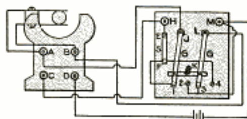
Toys and Other Small Electrical Constructions may be Reversed from a Distance by the Use of This Switch
