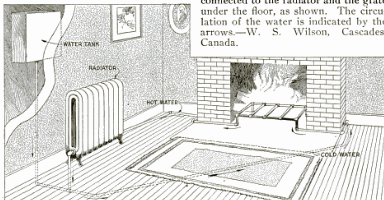
A Grate of Pipe was Built in the Fireplace and Made Part of a Hot-Water Heating System by Which Parts of the Room Remote from the Fire were Heated
