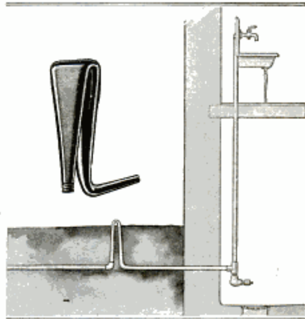
The Passage through the "Cut-Off" Is so Shallow That the Pipe does Not Burst When the Water Freezes within It
