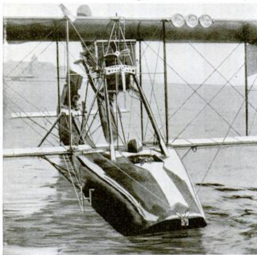
Curtiss Flying Boat Equipped with Special Lighting Outfit for Night Flying, Including a Bank of Three Searchlights on the Leading Edge of the Upper Plane, with an Air Turbine to Drive the Generator
