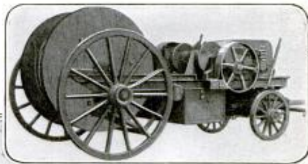
Two Views of the Telephone Construction and Cable-Handling Apparatus, the One Above Showing a Reel in Place for Unwinding, and That at the Left Indicating How the Derrick is Mounted. In Addition to Placing and Removing Poles, the Equipment is Arranged to Pull Lines through and Out of Underground Conduits and Do Other Work. It is Said to Cut Labor Cost Materially
