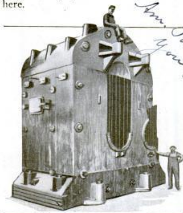
Portion of a Pattern for a Huge Pinion Housing Which It Took Four Men Nearly Four Months to Construct
