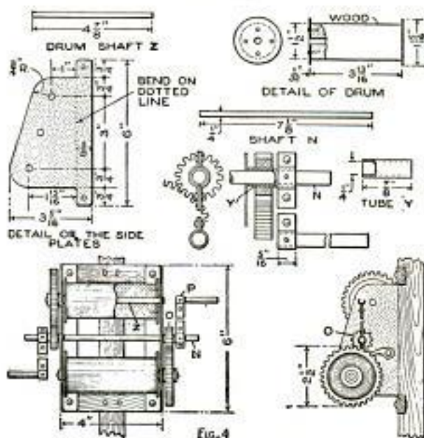
Details of the Hoisting-Drum Mechanism, or Crab: By Setting the Gears Properly Both Drums may be Operated Together
