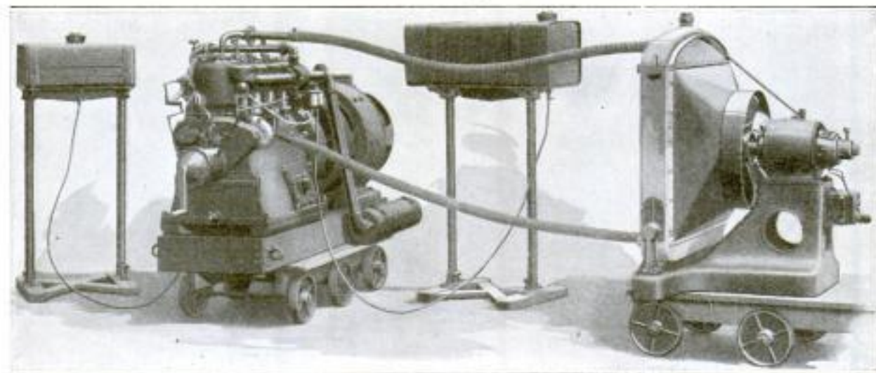
The Plant is Arranged so That It may be Quickly Assembled after being Transported to a New Position
