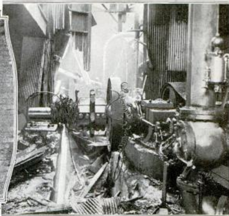
The View on the Left Shows a Big Hole Broken in a Brick Wall by a Section of the Shattered Flywheel. On the Right Is the Interior of the Engine Room after the Accident. The Shaft Which Drove the 30-Ton Wheel is Shown Wound with Wire
