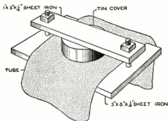
This Homemade Vulcanizer Utilizes the Heat from a Slowly Burning Disk of Cardboard
