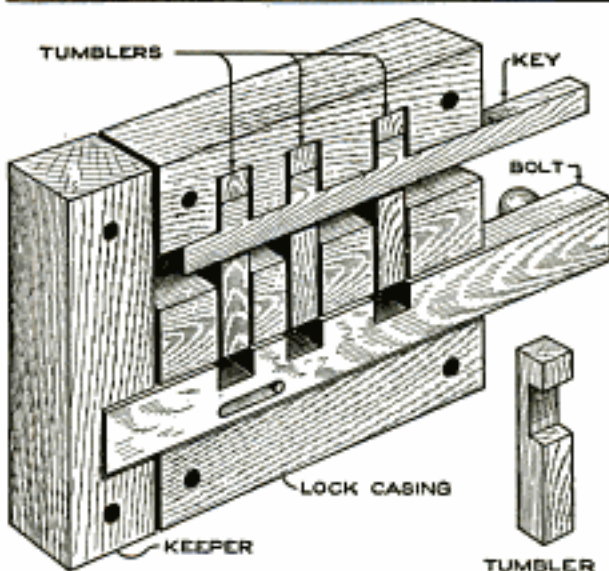
This Lock is Made Entirely of Wood and cannot be Picked Easily
