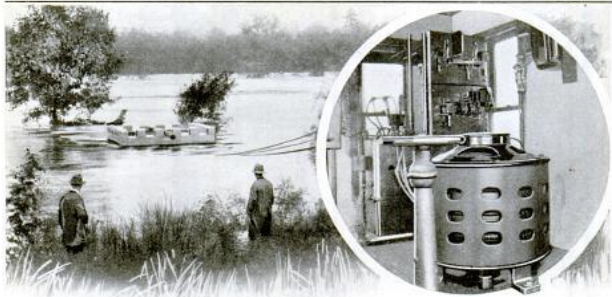
View of the Flood at Its Height, Showing the Water Almost as High as the Roof of the Concrete Power Station. When the River Receded the Motors were Coated with Mud. Insert Shows Part of Electrical Equipment Which was Put in Operation without being Allowed to Dry Out, after having been Submerged for 36 Hours
