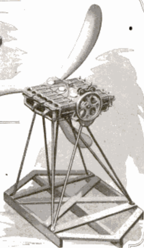
Upper Photograph Shows Cylinder Arrangement, Which Gives Minimum Over-All Length, and Indicates Way Crank and Propeller Shafts are Geared. Manifolds may be Seen at Side in Other View
