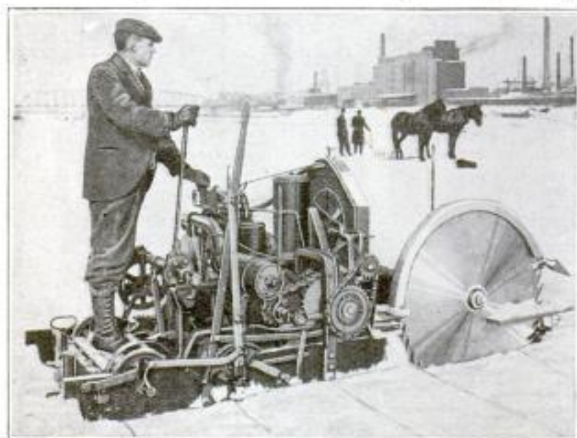
This Machine is Run by a 35-Horsepower Gasoline Engine, Is Self-Propelled, and will Cut 30,000 Cakes of Ice per Day
