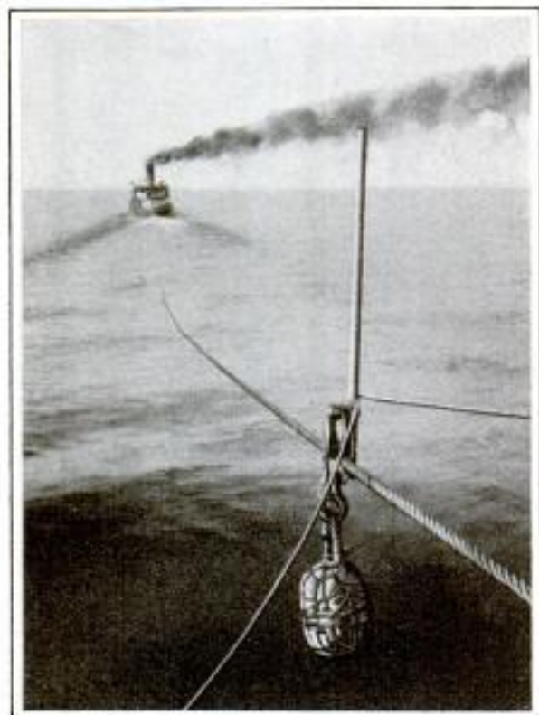
This Shows One of the Sticks in Place on a Towing Cable ahead of a Barge. Just the Top of the Fog Stick Is Visible to a Man at the Wheel
