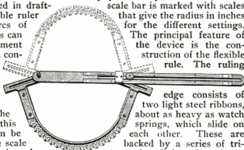
This Rule can be Set for Any Circular Arc from 3½ to 100-Inch Radius. Full Lines Show Rule Set for Concave Curve; Dotted Lines, Convex
