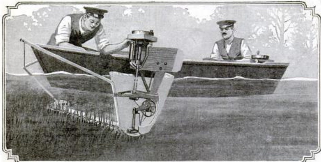
Sickle Set Up beneath Rowboat Mows Under-Water Weeds of Shallow Lakes. A Gasoline Engine Drives the Sickle and a Second Engine Propels the Boat into the Weed Beds
