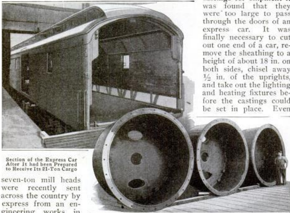
The Three Mill Heads Ready for Shipment to Arizona
