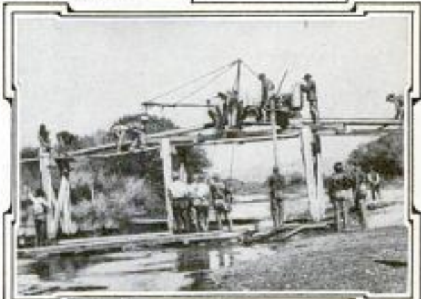
A Pipe-Screwing Machine, Made from an Automobile Engine, Capable of Putting Together 6,000 Feet of Pipe Daily
