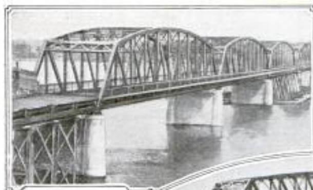
Bridge Spans Which have been Floated into Position: The Supporting Barges are Still under the Third Span
