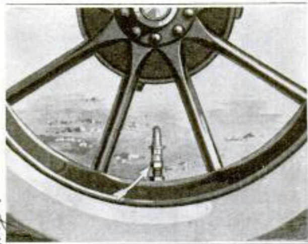
This Tire Valve Automatically Relieves Pressure in a Tire When on Account of Weather or High Speed the Pressure Becomes Too Great
