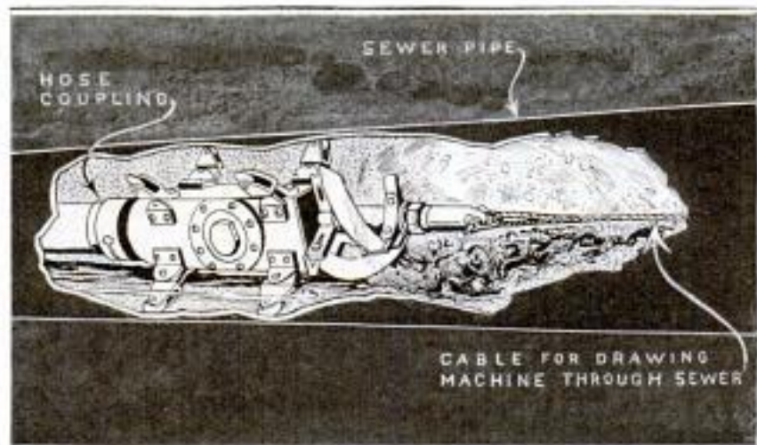
Sewer-Cleaning Machine Uses Water from Fire Hose to Operate the Hydraulic Motor Which Propels the Cutter Blades
