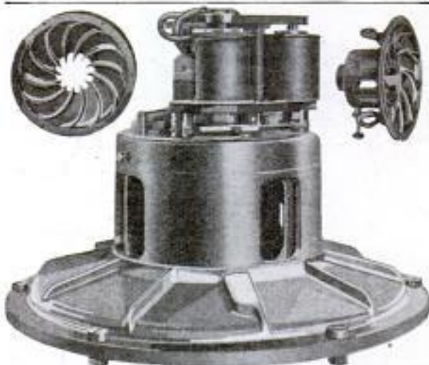
Air Siren Used as Battleship Signal over Short Distances
