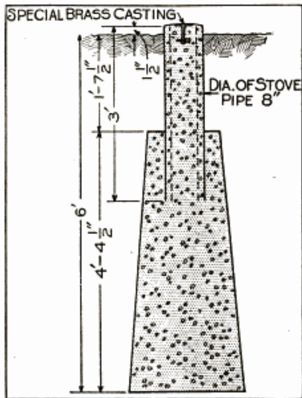
Concrete Bench Mark Adopted as Standard in Milwaukee: A Section of Stovepipe is Used for Molding the Upper Cylindrical Part
