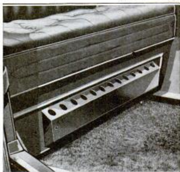
The Heater Makes Use of the Hot Gases Given Off by the Motor and may be Regulated without Leaving the Car
