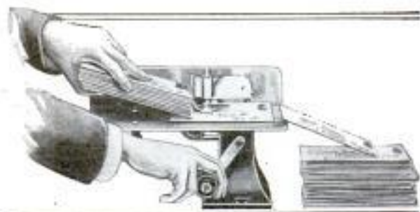
With This Hand-Operated Machine 85 to 150 Letters can be Opened per Minute
