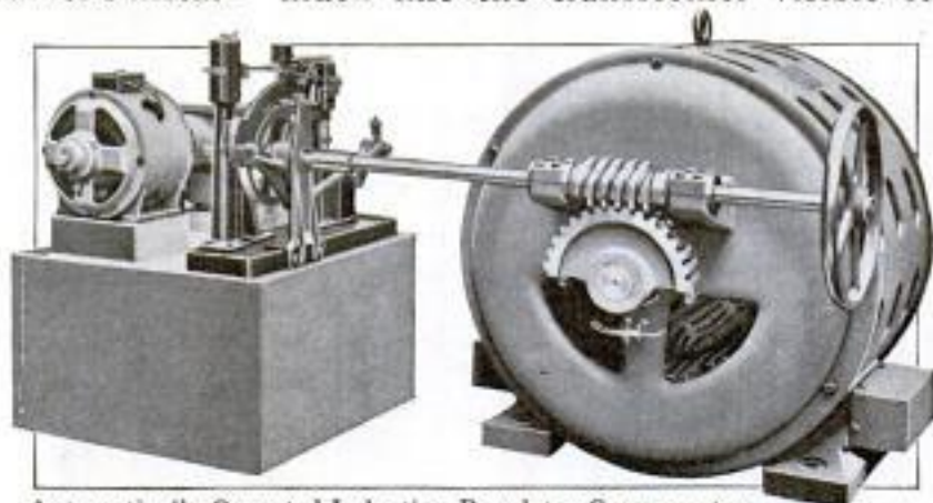
Automatically Operated Induction Regulator Compensates for Voltage Variations in Transmission Lines
