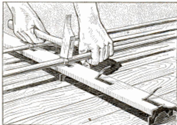
Spacing Bar Holds Concrete Reinforcements Firmly in Position
