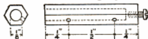
Fig. 7 Detail of the Brush Holders, One Inch Long, with Holes as Shown
