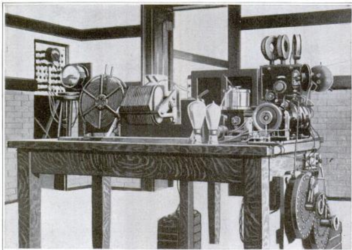
This Apparatus Indicates the Direction from Which Wireless Signals are Emanating
