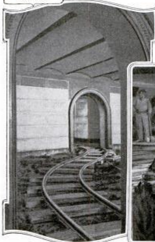
Left: Dump-Car Track Extending through Basement of Building. Above: Hoisting Dirt to Wagons Waiting at Street Level. Right: Putting the Underpinnings in Place beneath Pavement
