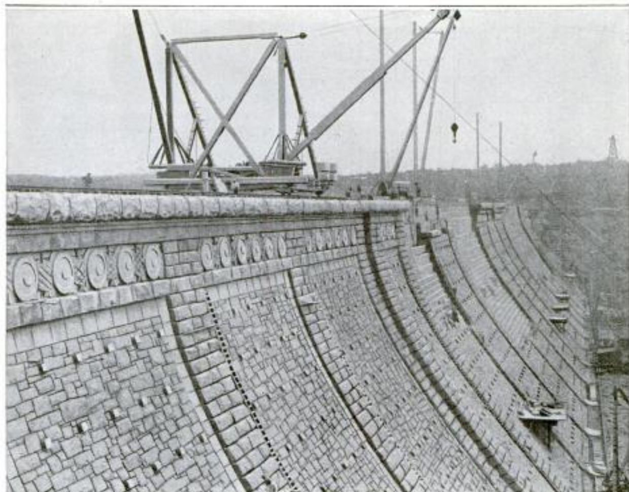
The Downstream Face of the Kensico Dam, Showing the Paneled Granite Facing Partly Finished. The Stones of the Torus Are Four Feet Thick and Weigh from Nine to 14 Tons Each
