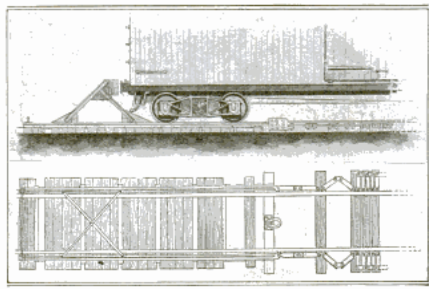
The Buffer and the Ties on Which It is Mounted Slide under the Impact of a Car, Bringing the Car to a Stop Gradually
