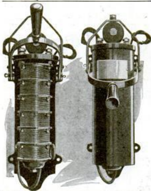
In Addition to being of Compact Size, the Starter Is without Sliding Contacts or Springs
