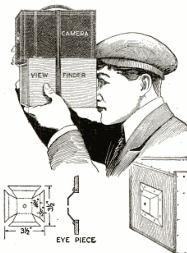
Sight through the Eyepiece for a Direct View of the Object Photographed, Thus Insuring More Nearly the Accuracy of the Result
