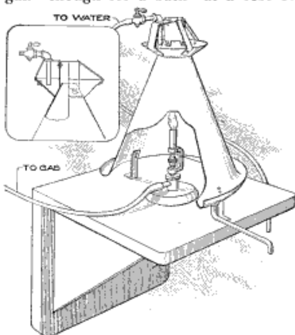
The Water, Running over the Outside Surface of the Funnel, is Heated Quickly
