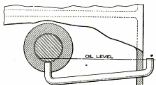
The Oil will Seek Its Level and Lubricate the Bearing
