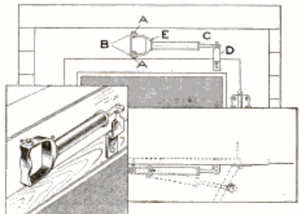
Air-Cushion Check Made of a Bicycle Foot Pump for a Screen Door
