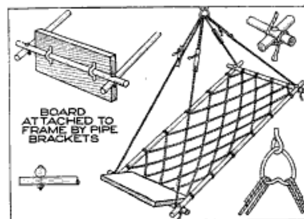
Reclining-Chair Hammock That can be Used Upright or at an Angle by Adjusting the Ropes
