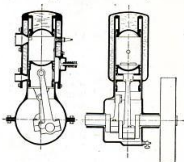
New Two-Cycle Gas Engine in Which the Gas is Entirely Controlled by a Sliding Sleeve
