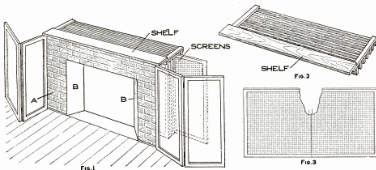
FIG. 1 Frames Made of Light Material and Covered with Black Mosquito Netting Serve as Screens Which are Operated in Runs Located behind the Fireplace That is Made Up in a Like Manner and Penciled to Represent Brick
