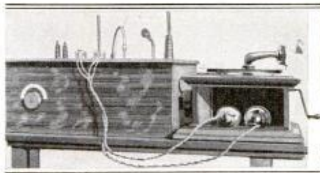
Wireless-Telephone Apparatus at the Sending Station Showing Transmitters Placed in the Horn of a Phonograph, Music from Which was Transmitted to Several Receiving Stations
