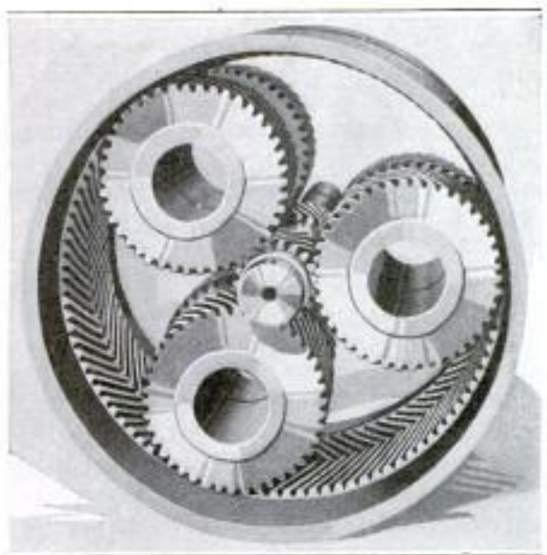
Internal Helical Gear Forms Compact Speed Reducer
