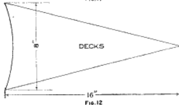
The Shape of the Deck or Breast Hooks and the Beams That Support Them
