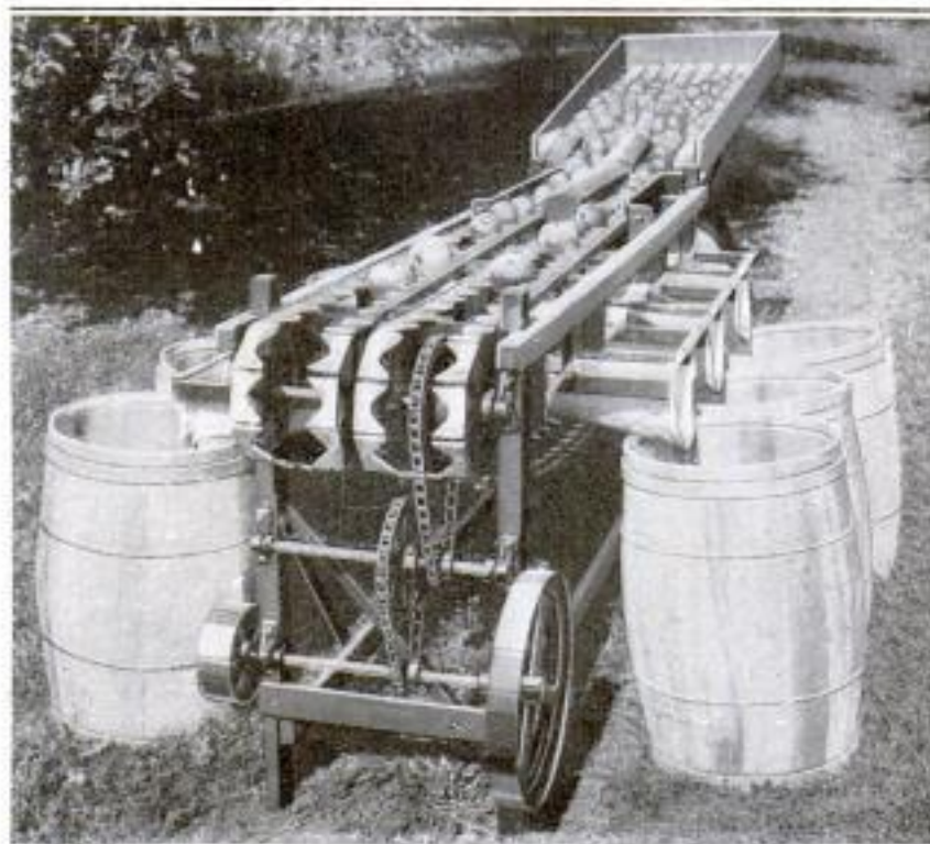
This Machine Sorts Apples at the Rate of 50 Barrels per Hour
