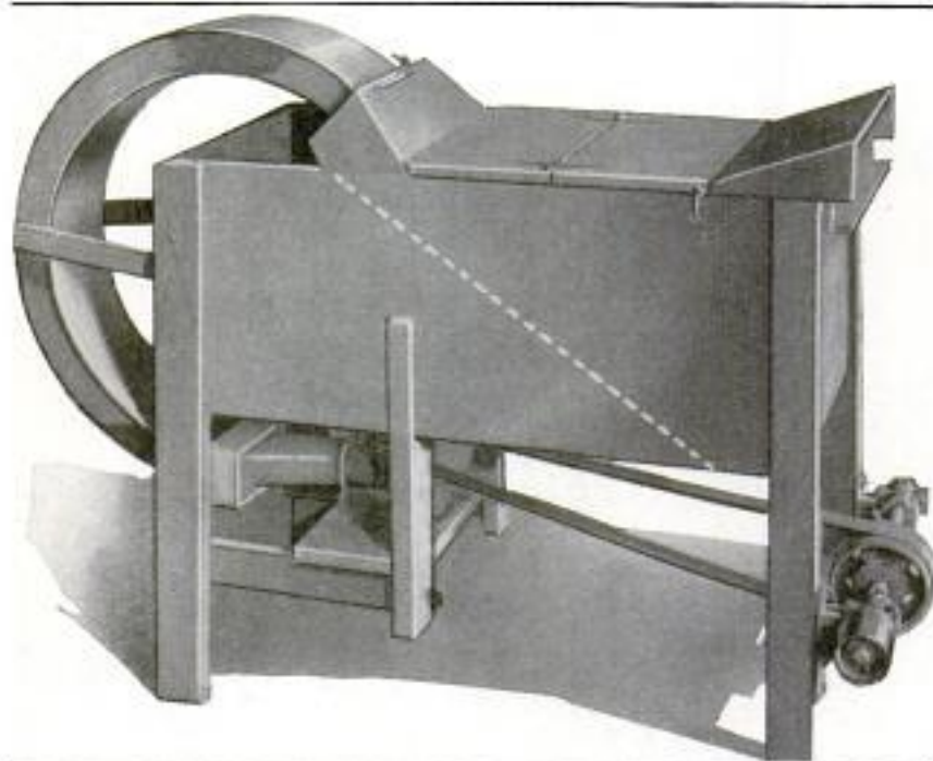
This Machine Scratches Hard-Coated Seeds by Hurling Them Against Sandpaper. With Their Covering Broken Such Seeds Germinate More Quickly
