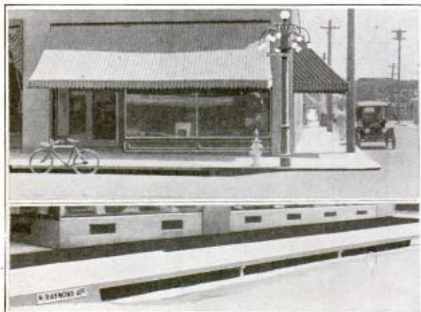
Storm Sewers of Adequate Capacity and Large Intakes Keep Streets from being Flooded during Heavy Rains
