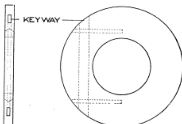
A Two-Piece Hub Liner for Insertion without Removing Locomotive Wheels from Their Frame
