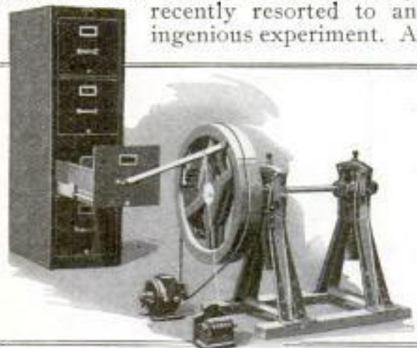
Machine Tests Filing Cabinet by Running Drawer In and Out 361,321 Times
