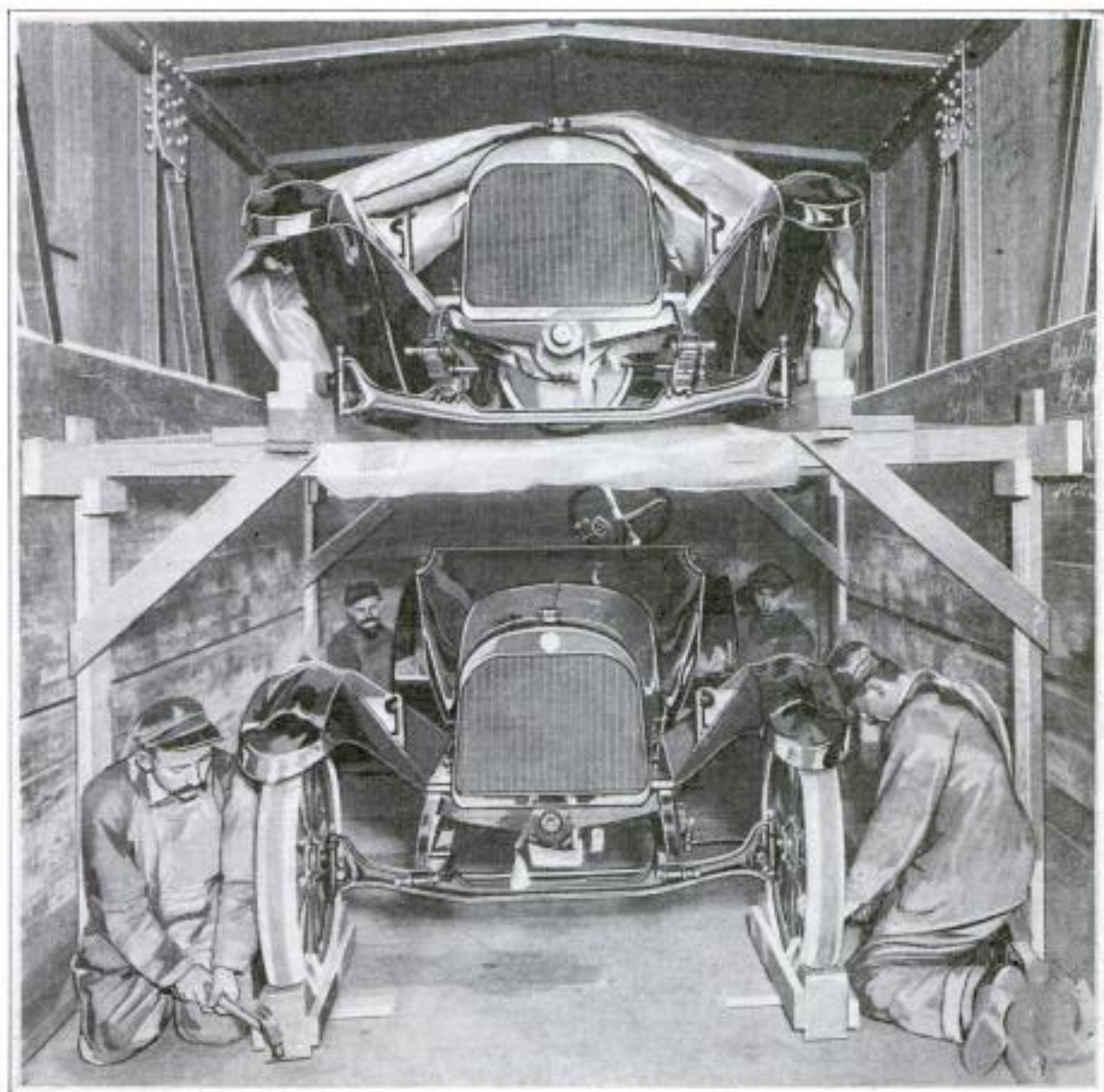
Five Machines of the Size of These can be Loaded into One Car and Shipped without Difficulty: Two are Placed at Either End, as Shown, and One in the Middle of the Car
