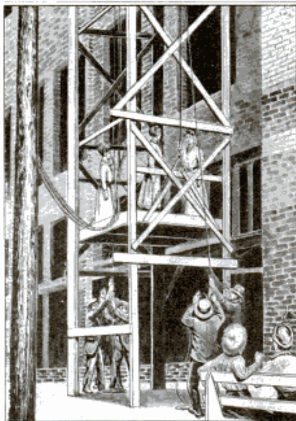
By Lifting Simultaneously a Telephone Switchboard and Two Operators in This Temporary Elevator a Telephone Company Was Able to Give Its Subscribers Uninterrupted Service While Transferring Its Apparatus to the Second Story of Its New Building
