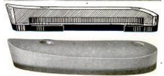
Large Air Chamber in This Recoil Pad Makes It an Effective Shock Absorber
