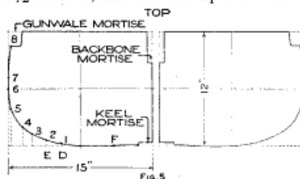
This Mold is Placed Amidships, in the Center of the Canoe, and Only One is Required
