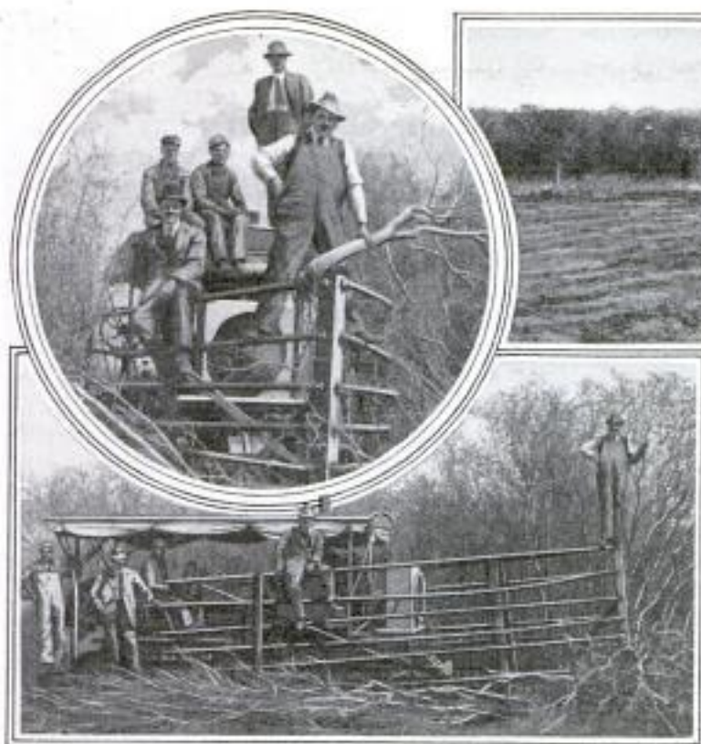
Above, and in the Insert, the Brush Cutter is Shown in a Dense Thicket Leveling the Undergrowth and Piling It on One Side of the 16-Foot Path It Cuts
