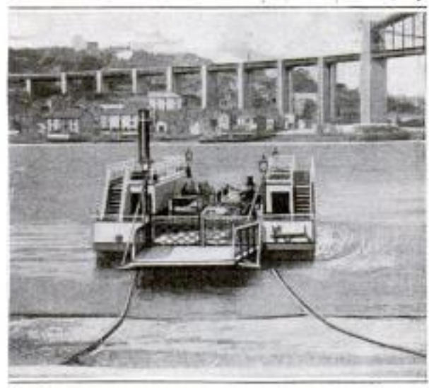
Ferry across River Tamar in England Uses Chains Attached to Shore As Guide in Coping with the Strong Current
