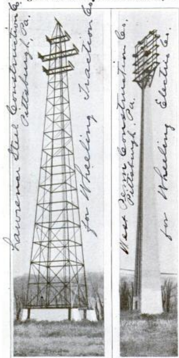
Large Towers Which Carry High-Tension Transmission Lines across Ohio River
