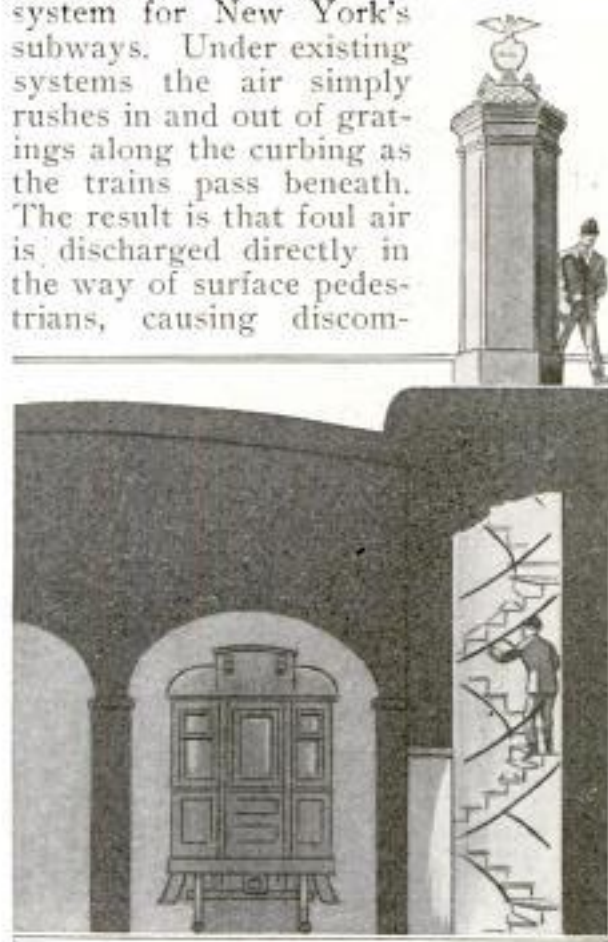
By Constructing Kiosks as Shown Here, It Is Proposed to Furnish Ventilators for New York's Subways That may Also be Used as Exits
