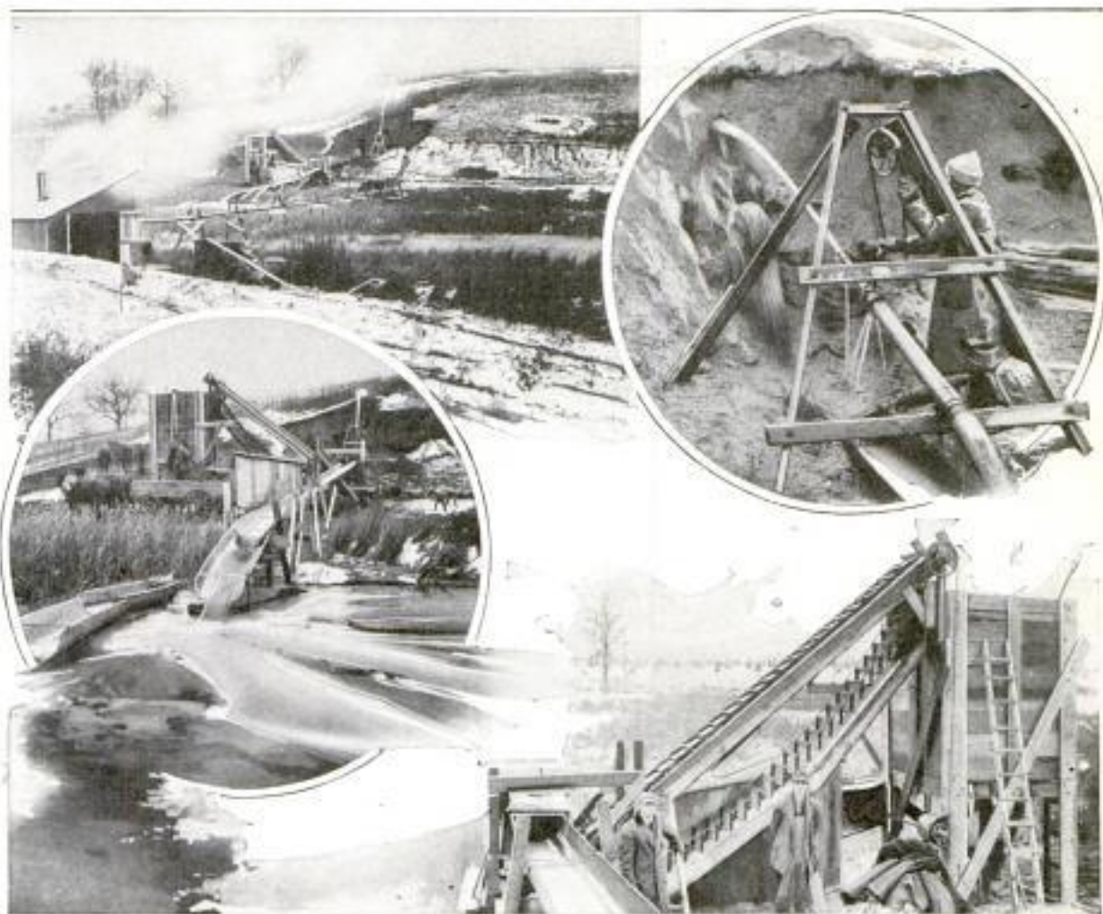
The Photographs Above Illustrate the Hydraulic Process of Mining Gravel for Use in Road Building: At Top, on the Left, Is a View of a Plant Operating near Battle Creek, Michigan. The Insert at the Right of This Shows How the Water Cuts into the Embankment and Carries the Gravel and Sand into Sluice Boxes. The Former is Caught in the Screened Pockets of a Conveyor, Washed, and Elevated into a Hopper, as Indicated Below at the Right. In the Other Insert the Sand and Dirt are being Sluiced into a Hollow
