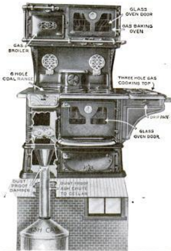
When the Grate is Shaken the Ashes are Discharged into the Chute and Deposited in a Can Provided in the Cellar
