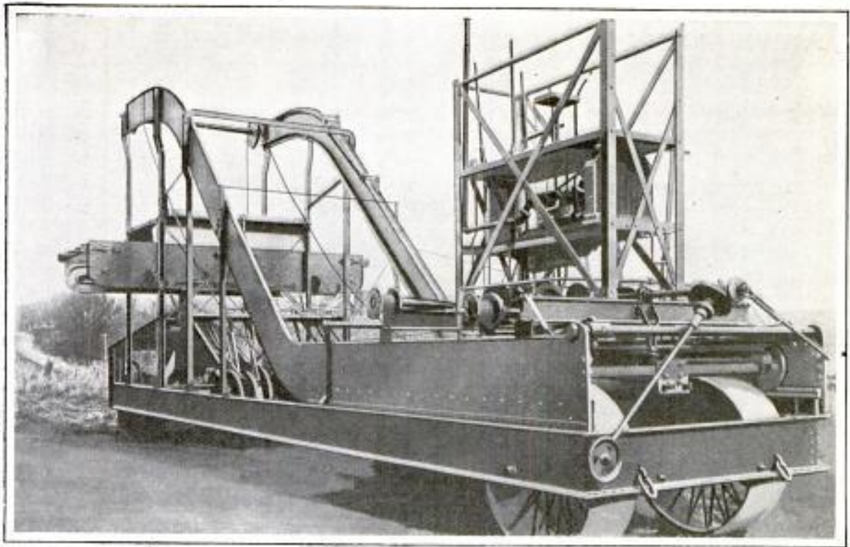
Machine Plows Up Dirt and Loads It into Wagons for Constructing Railroad Embankments and Such; It Is Capable of Delivering 80 or More Two-Yard Loads per Hour
