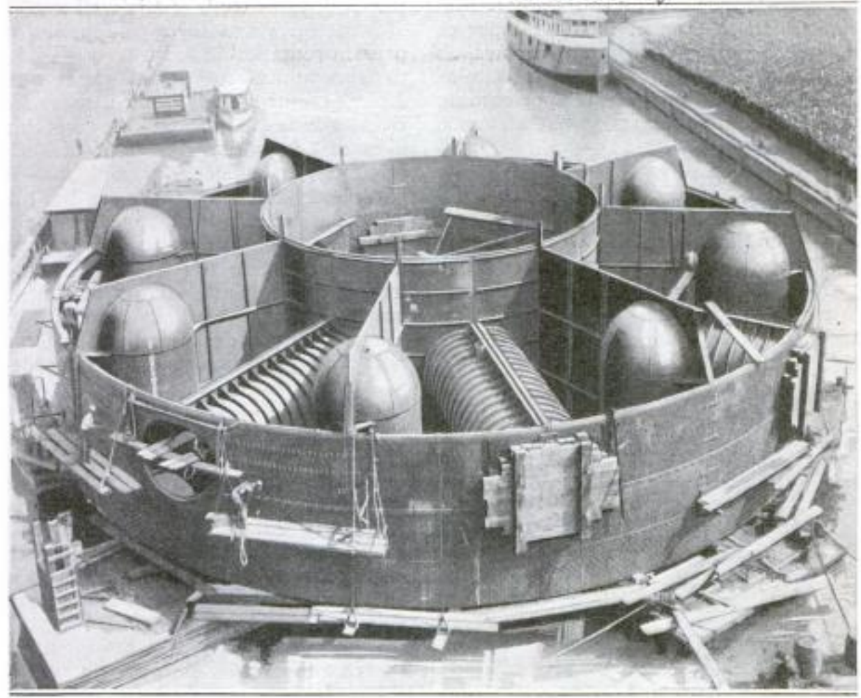
Sealing the Ports in the Substructure in Order to Provide a Sufficient Air Column to Keep the Shell Afloat during the Remainder of Its Construction
