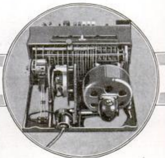
Addition, Subtraction, Multiplication, and Division are All Performed on This Small, Electrically Driven Desk Machine
