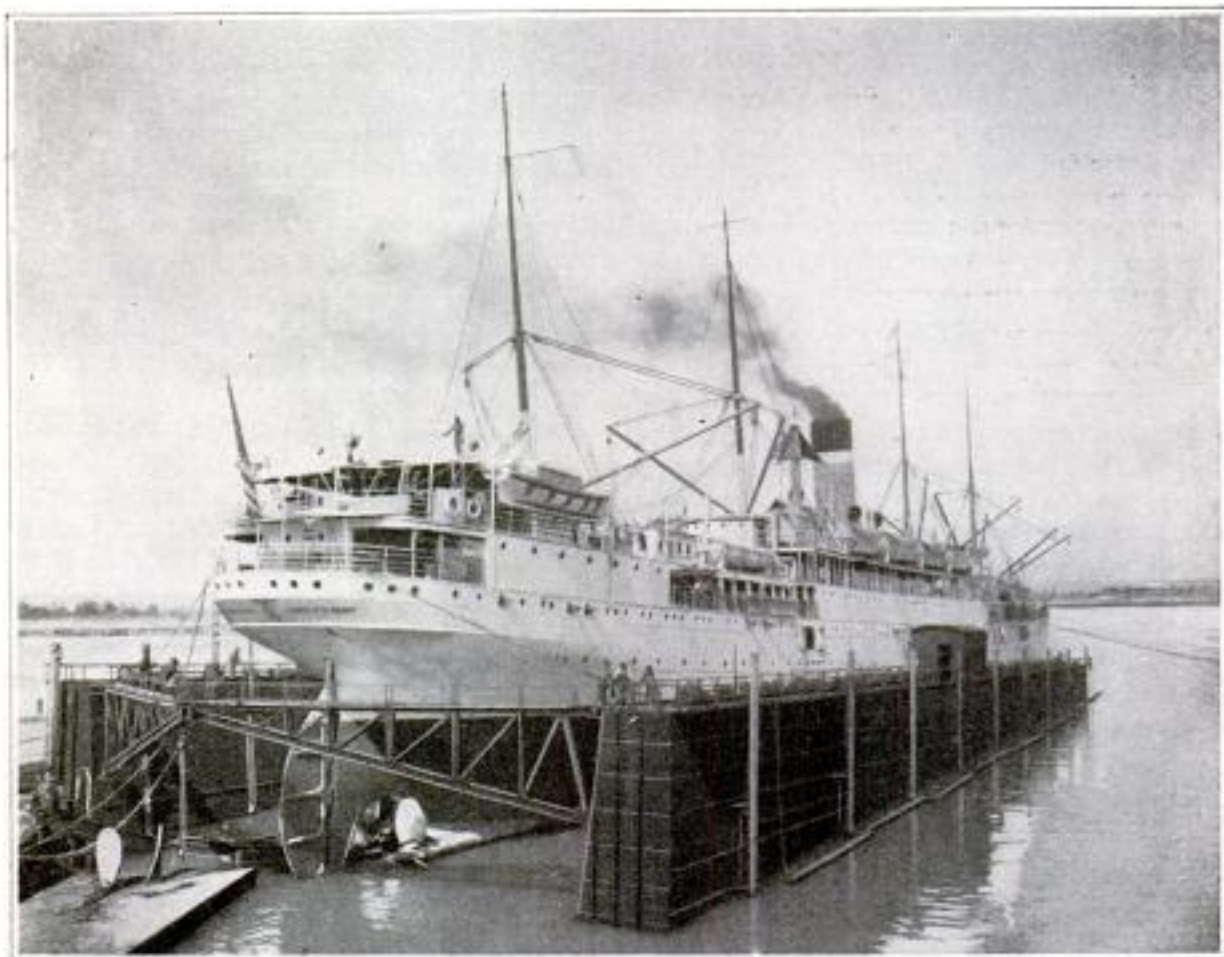
The Transport "Thomas," an 11,000-Ton Ship, is Here Shown being Repaired in a Floating Dry Dock Which Has a Capacity of Only 4,500 Tons. The Boat is 118 Feet Longer than the Dry Dock.
