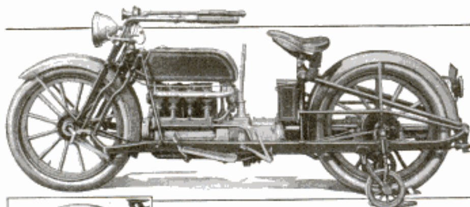
New Motorcycle with Motor-Car Frame, Wooden Wheels, Shaft Propulsion and Selective Transmission
