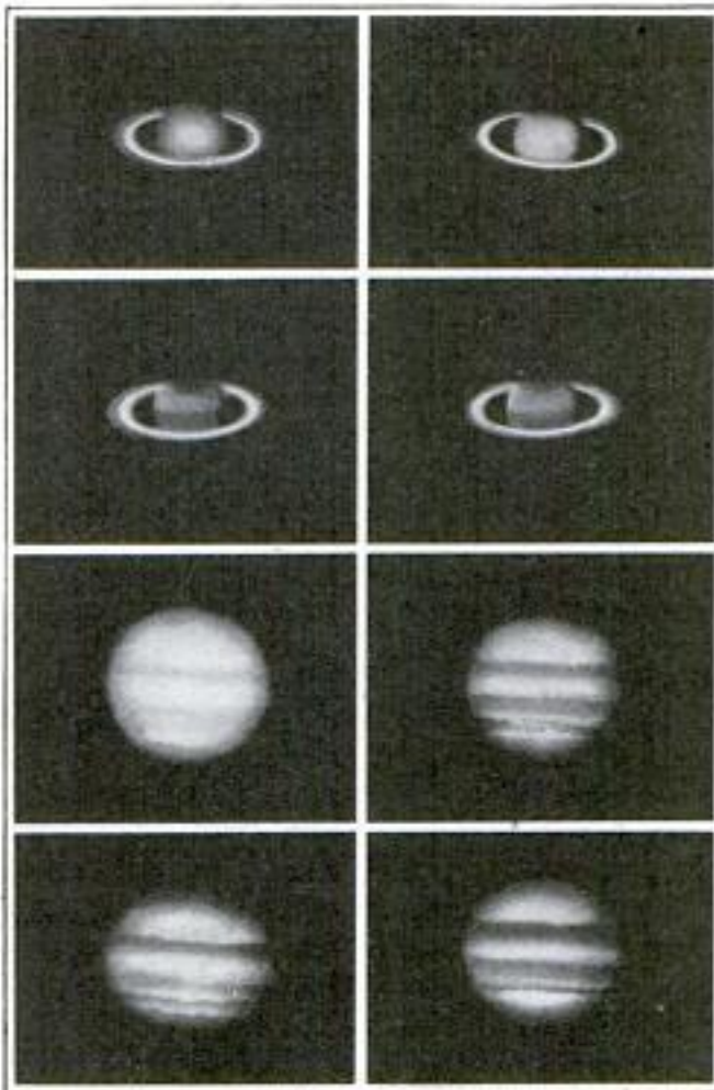
The Four Top Views Are of the Planet Saturn. Reading from Left to Right, They were Taken by Means of Infrared, Yellow, Violet, and Ultraviolet Rays. The Four Lower Pictures Show Similar Views of Jupiter, Arranged in Like Order
