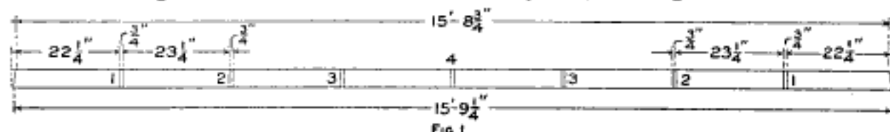
FIG. 1 The First Step in the Construction of a Canoe Is to Get Out the Backbone and the Molds, or Forms, Which Give the Correct Dimensions and Shape of the Craft
