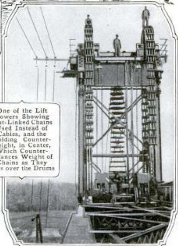
A Bridge so Built That Any One of Its Spans may be Transformed into a Lift Span by Moving the Lift Towers
