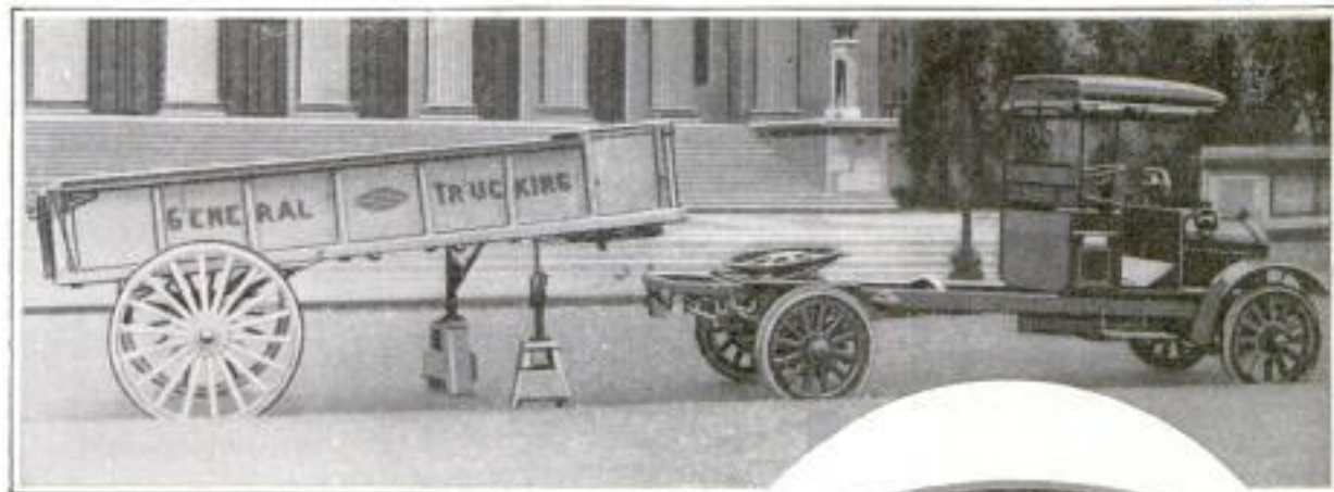
By Means of This "Fifth Wheel," Which Has Several Distinctive Features, a Two-Wheel Trailer can be Easily Attached to or Detached from a Motor Truck
