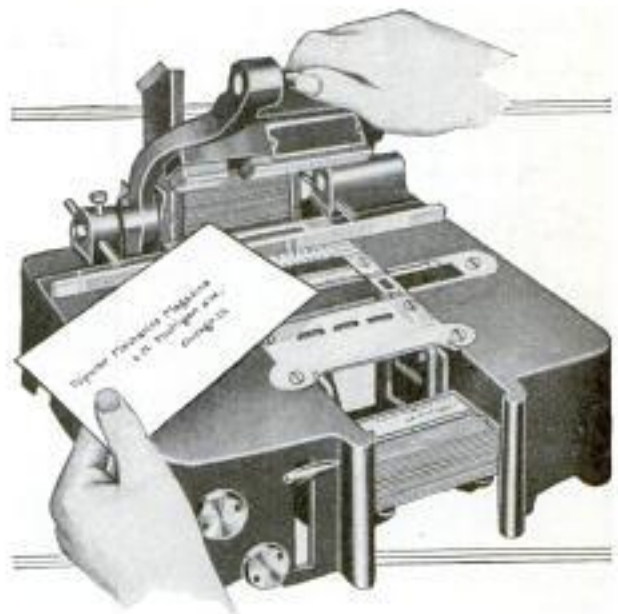
Mailing Machine Prints Whole Address in One Blow
