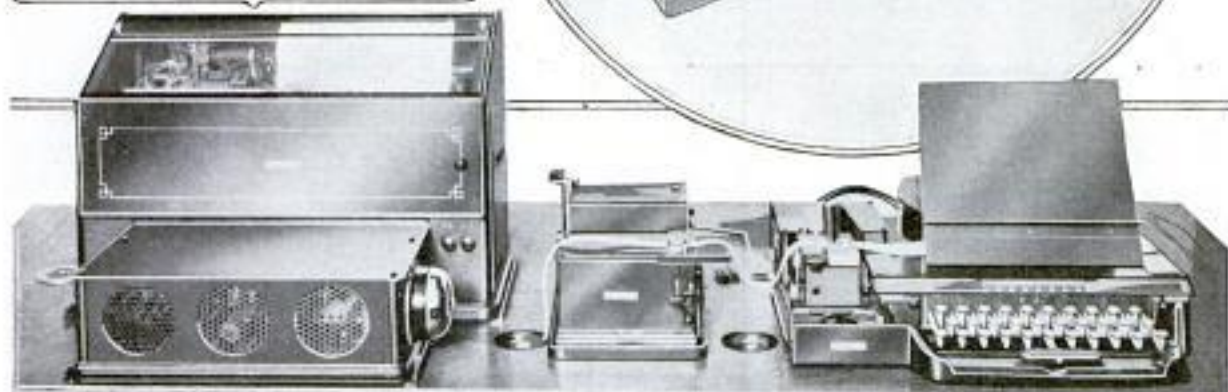
The Above Instrument, a Distributor, Makes the Multiplex Operation Possible. It Is by Using an Apparatus of This Kind at Each End of a Line that the Signals Rendered by Different Transmitters are Directed to the Proper Receivers. At the Right Is a Perforator
