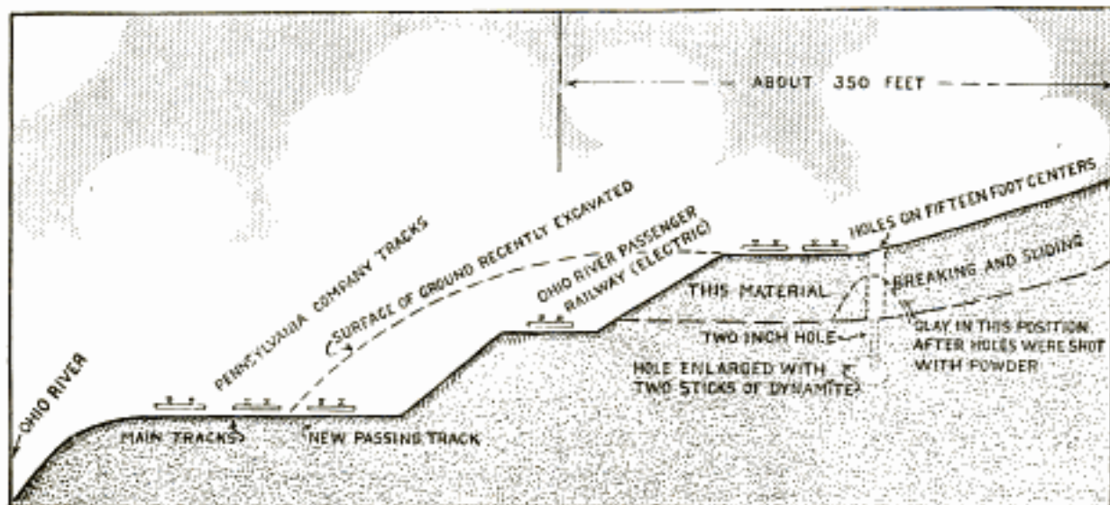
How the Humps were Formed by Explosives in the Underlying Clay Stratum to Stop a Landslide
