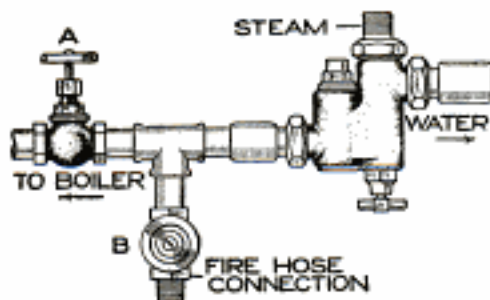
The Injector on the Engine Produces the Pressure for the Fire Hose
