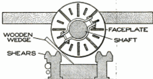
The Wedge, Driven in Snugly between the Shears and Faceplate Edge, Stops the Chatter
