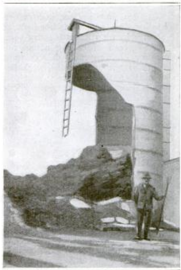
Too Sparing a Use of Cement in Mixing the Concrete Was the Cause of This Silo Breaking Apart While Filled
