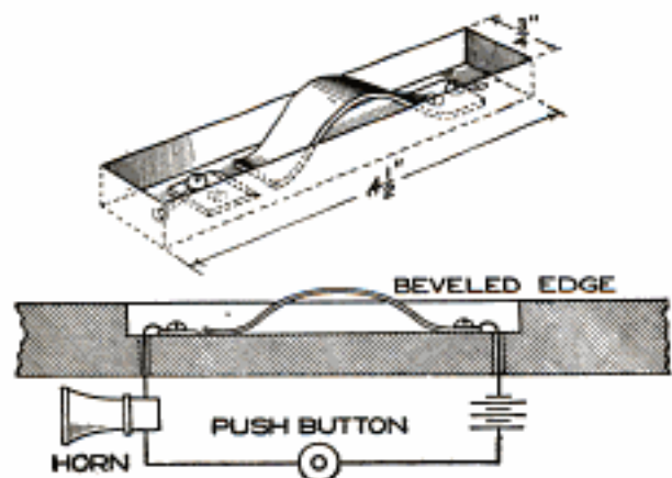
The Concealed Switch in the Circuit is Operated by the Cushion on the Driver's Seat
