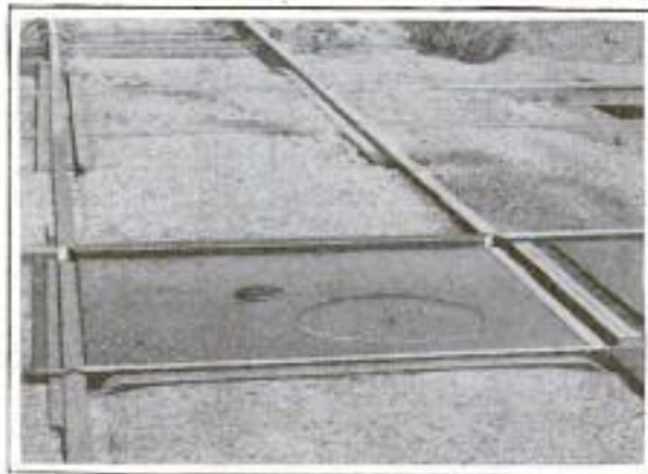
When One Pair of Rails in This Railway Crossing is Raised the Other Pair is in Lowered Position and Out of the Way of the Wheel Flanges
