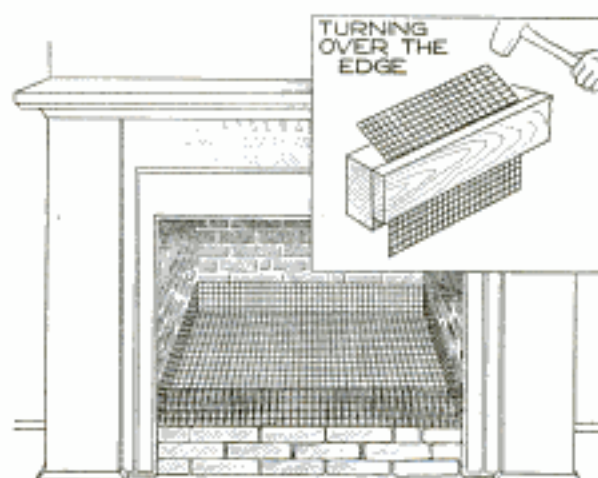
Grate Made of Coarse-Mesh Screen, to be Used for Coal in a Wood-Burning Fireplace
