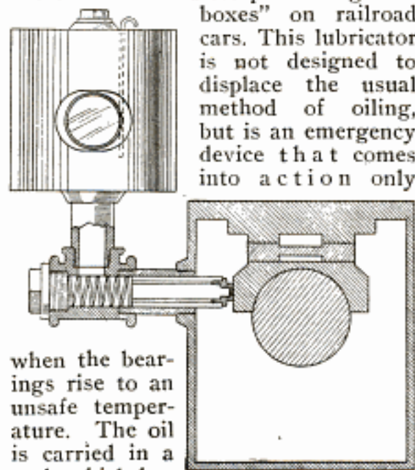
This Railway-Car Lubricator Fills the Journal Automatically with Oil When the Bearing Begins to Run Hot
