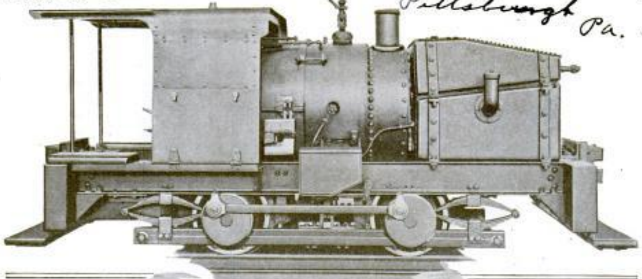
In This Oil-Burning Locomotive, Which is Designed Particularly for Construction Work, a Full Head of Steam can be Raised in 15 Minutes
