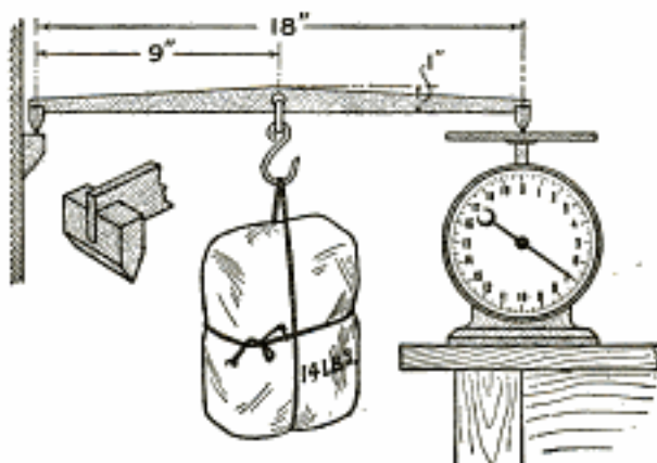
The Beam Provides a Means of Weighing Large Objects on a Small Spring Scale
