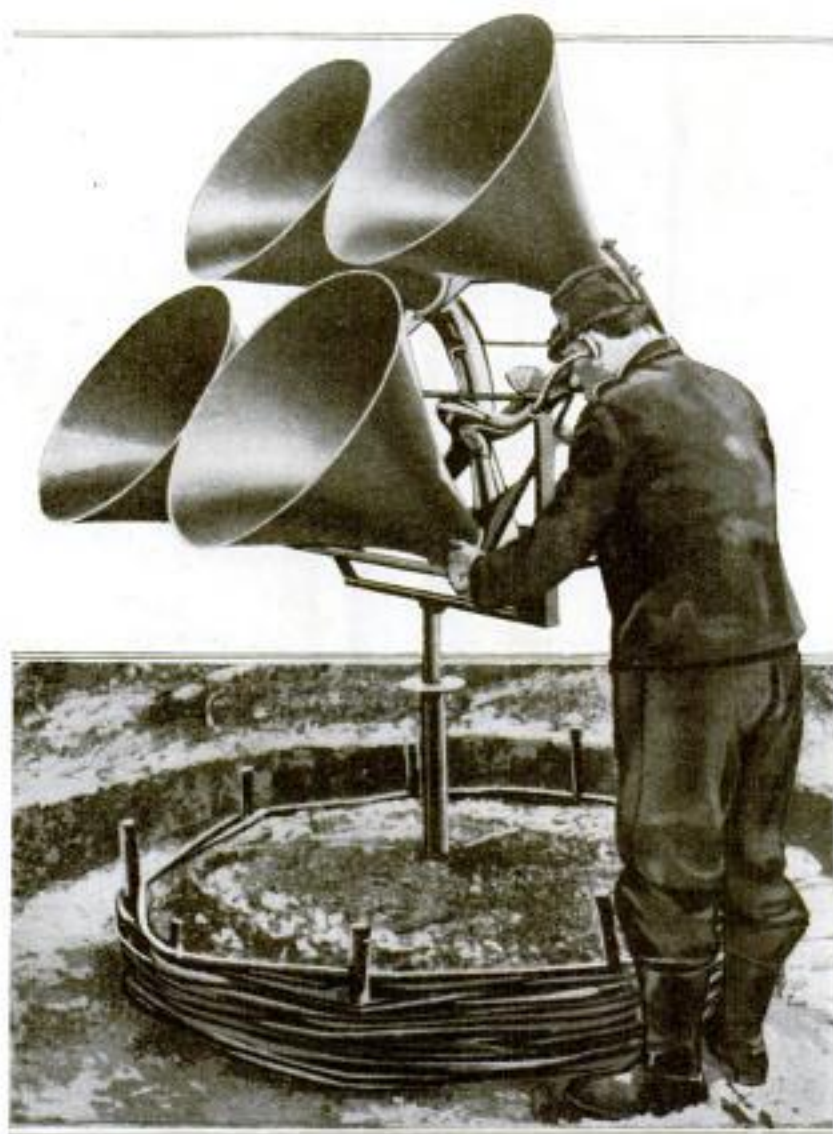
This Detector, Which Consists of Four Megaphones Connected with a Microphone and Equipped with Receivers, is Used Both Day and Night: With It the Purr of an Aerial Engine may be Heard While the Machine Itself Is Invisible
