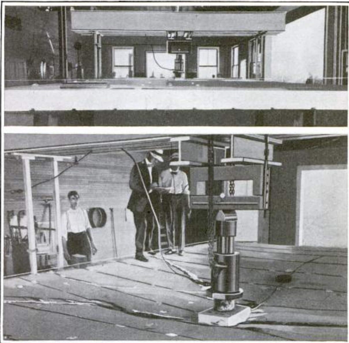
View of the Bridge before the Test, and Later While being Put under Pressure by the Hydraulic Jack
