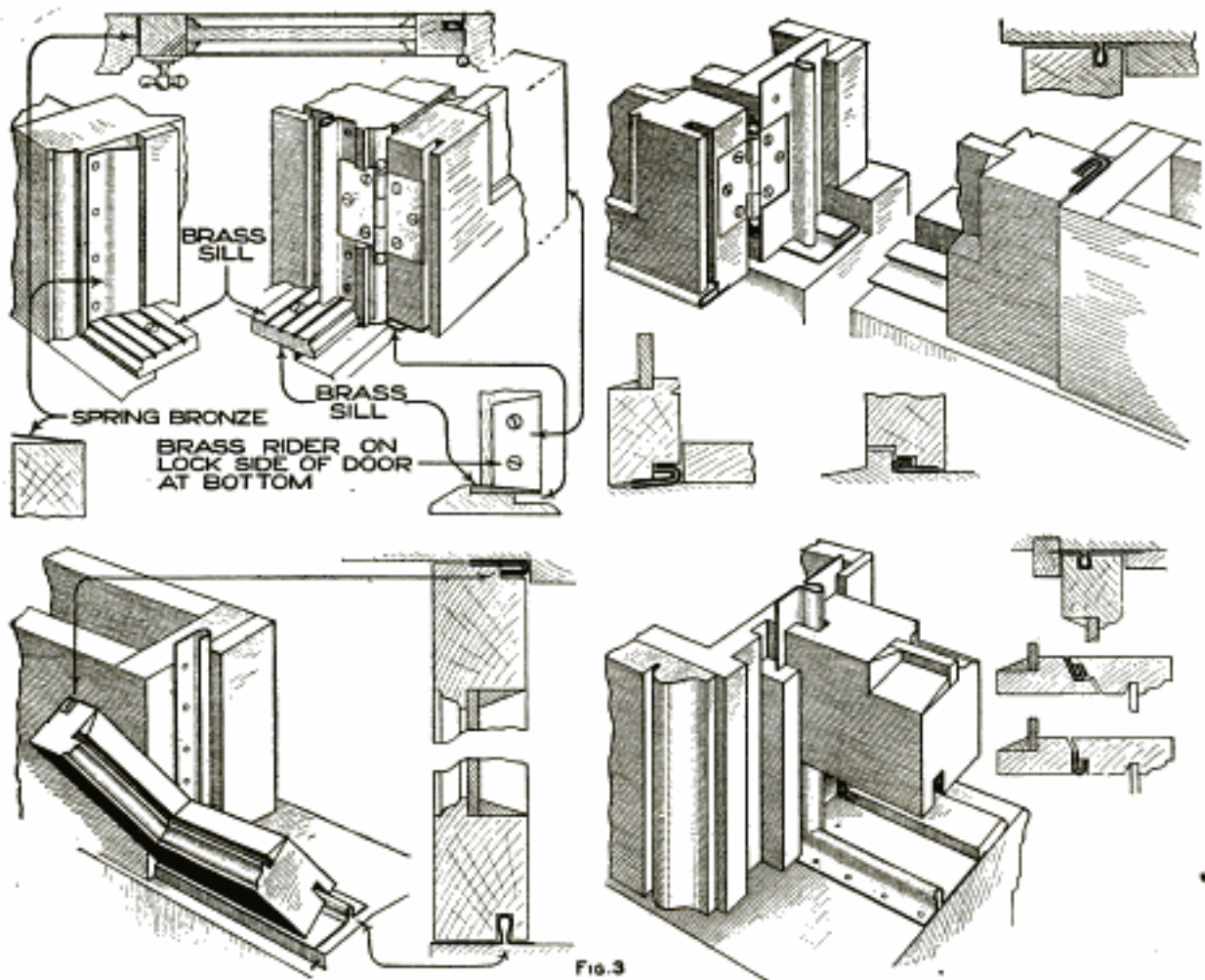
Metal Weather Strips are Put in Place and Forgotten, Are Practically Invisible, and Need No Painting or Repairing, as They are Made of Bronze, Which Never Corrodes
