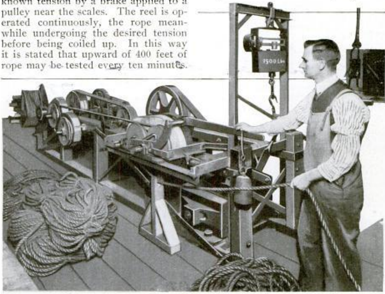
The Straight Length of Rope between the Pulleys in the Foreground and Those in the Back Is under a Tension Applied with a Brake and Measured with the Scales
