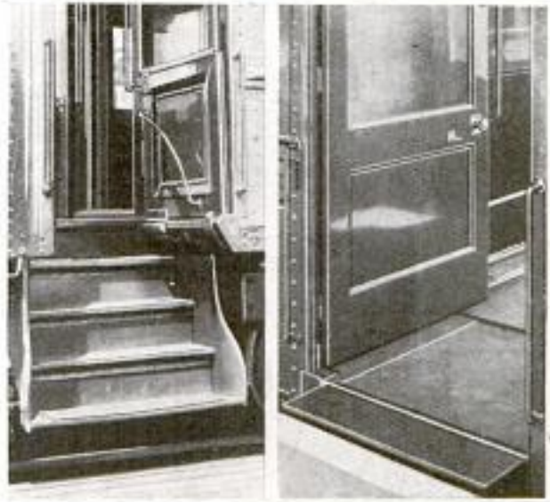
When Extended by Opening the Vestibule Door, the Auxiliary Leaf Bridges the Gap between the Car and a Station Platform. A Means is Also Provided for Opening the Door without Actuating This Mechanism, So That the Steps may be Used
