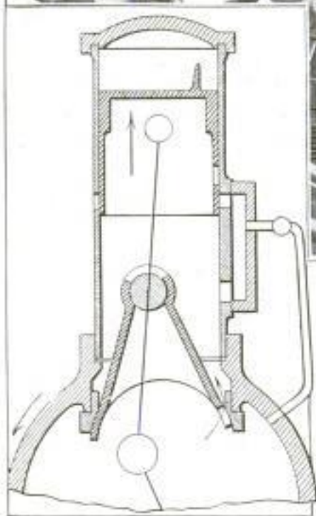
In This Two-Cycle Gas Engine the Gas is Compressed in the Inner End of the Cylinder Instead of in the Crank Case. The Rocking Valve for Admitting the Gas to the Cylinder is Shown in the Diagram at Left
