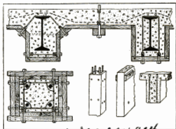
The Rod Not Only Serves as Reinforcing After the Concreting is Completed but Provides Sockets with Which Attachments are Easily Made
