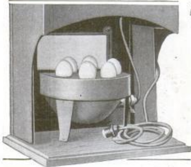
With This Tester a Case of Eggs may be Inspected and the Unfit Ones Separated from the Others Rapidly
