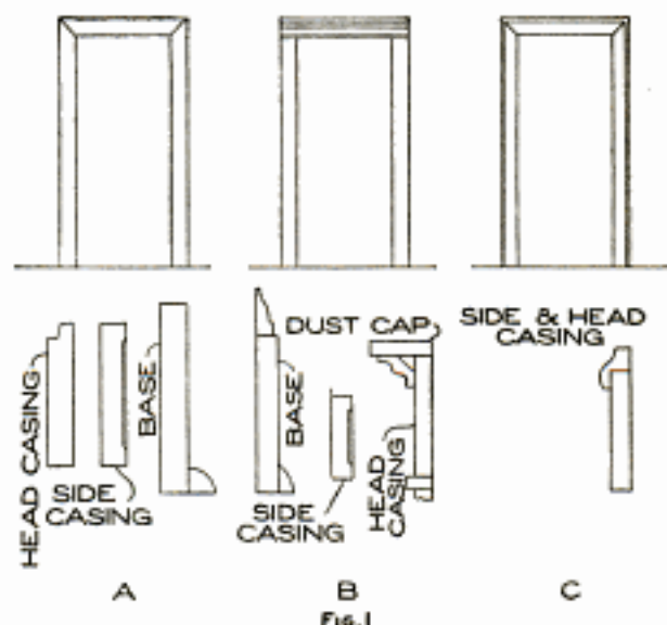
Fig. 1 Three Styles of Finish Most Commonly Used: The Mitered, the Cabinet-Head, and the Back-Band
