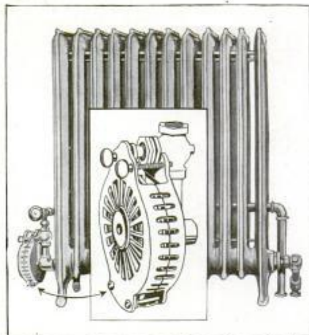
By Installing a Controller on Each Radiator, Various Rooms may be Kept at Different Temperatures
