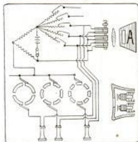
Cross Section of Instrument
