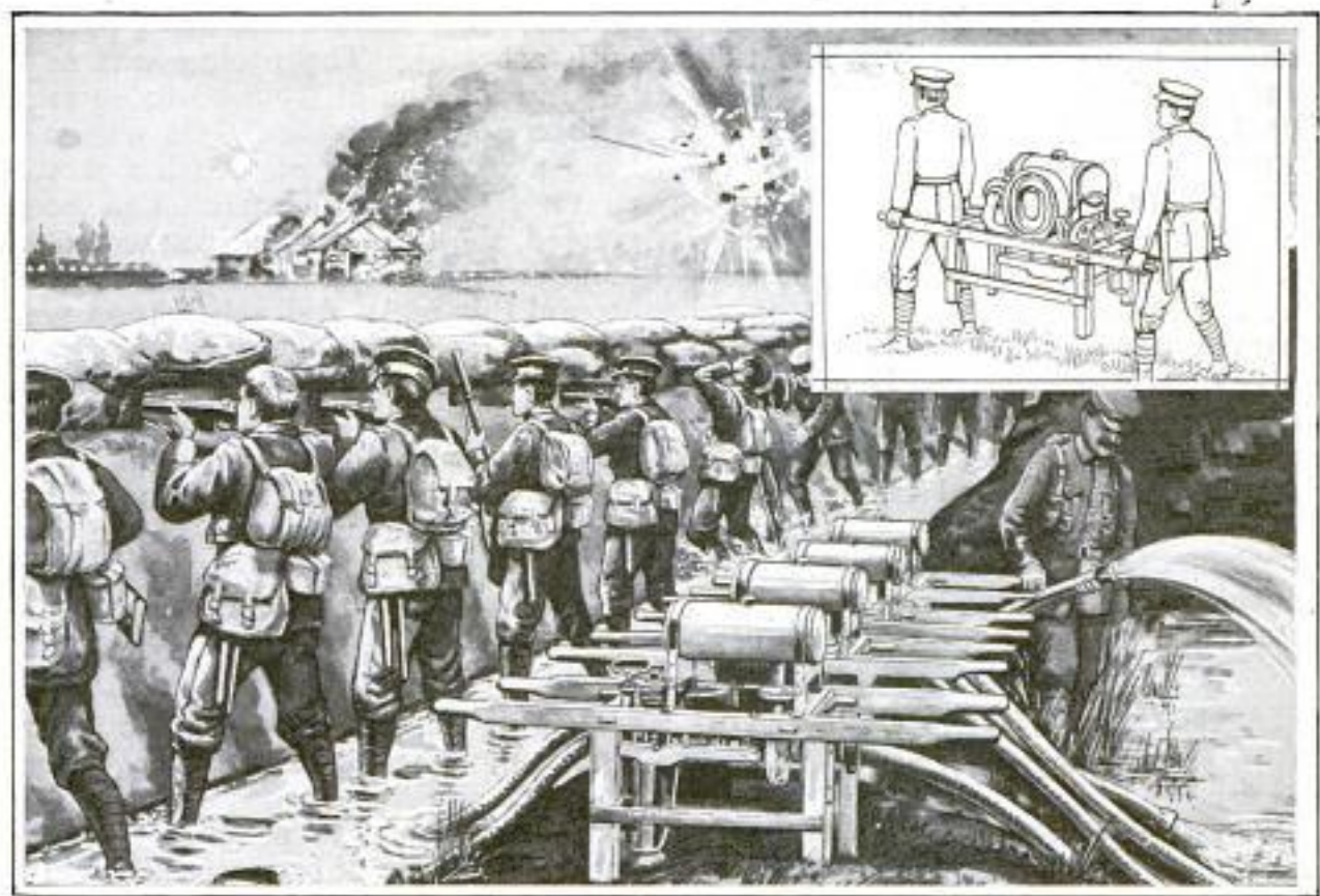
A Battery of Four Gasoline Pumps in Action Draining a British Trench in Belgium. The Picture at Top Shows How the Pumps are Transported from Trench to Trench
