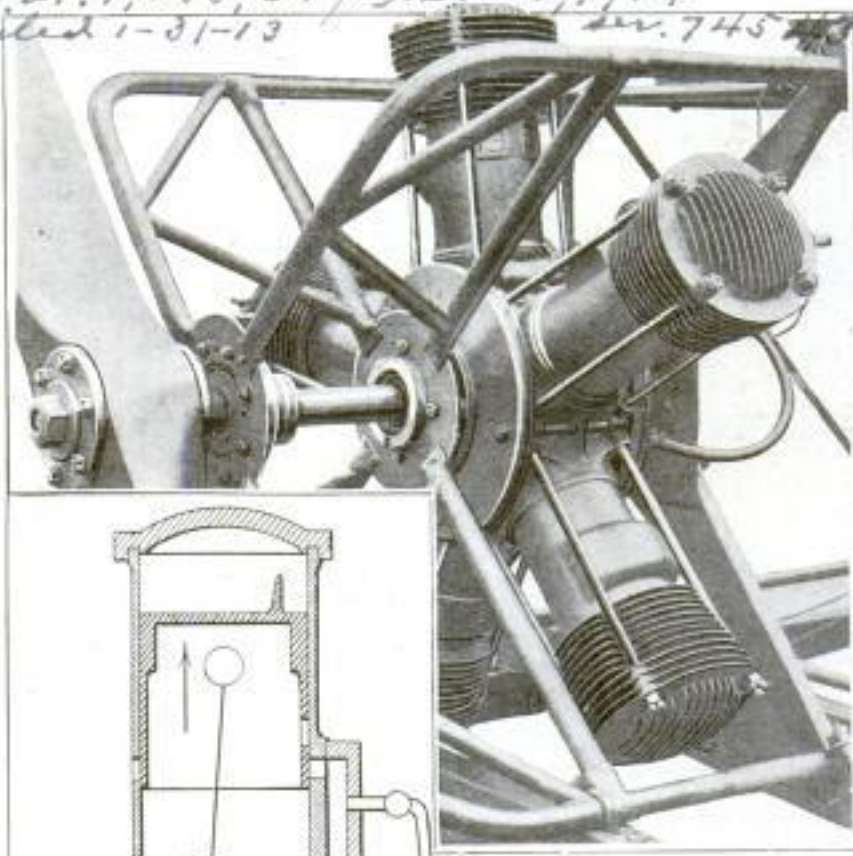
In This Two-Cycle Gas Engine the Gas is Compressed in the Inner End of the Cylinder Instead of in the Crank Case. The Rocking Valve for Admitting the Gas to the Cylinder is Shown in the Diagram at Left
