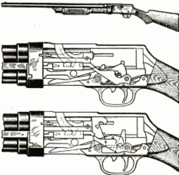
A Repeating Shotgun and the Position of Its Different Parts When Cocked and after Firing
