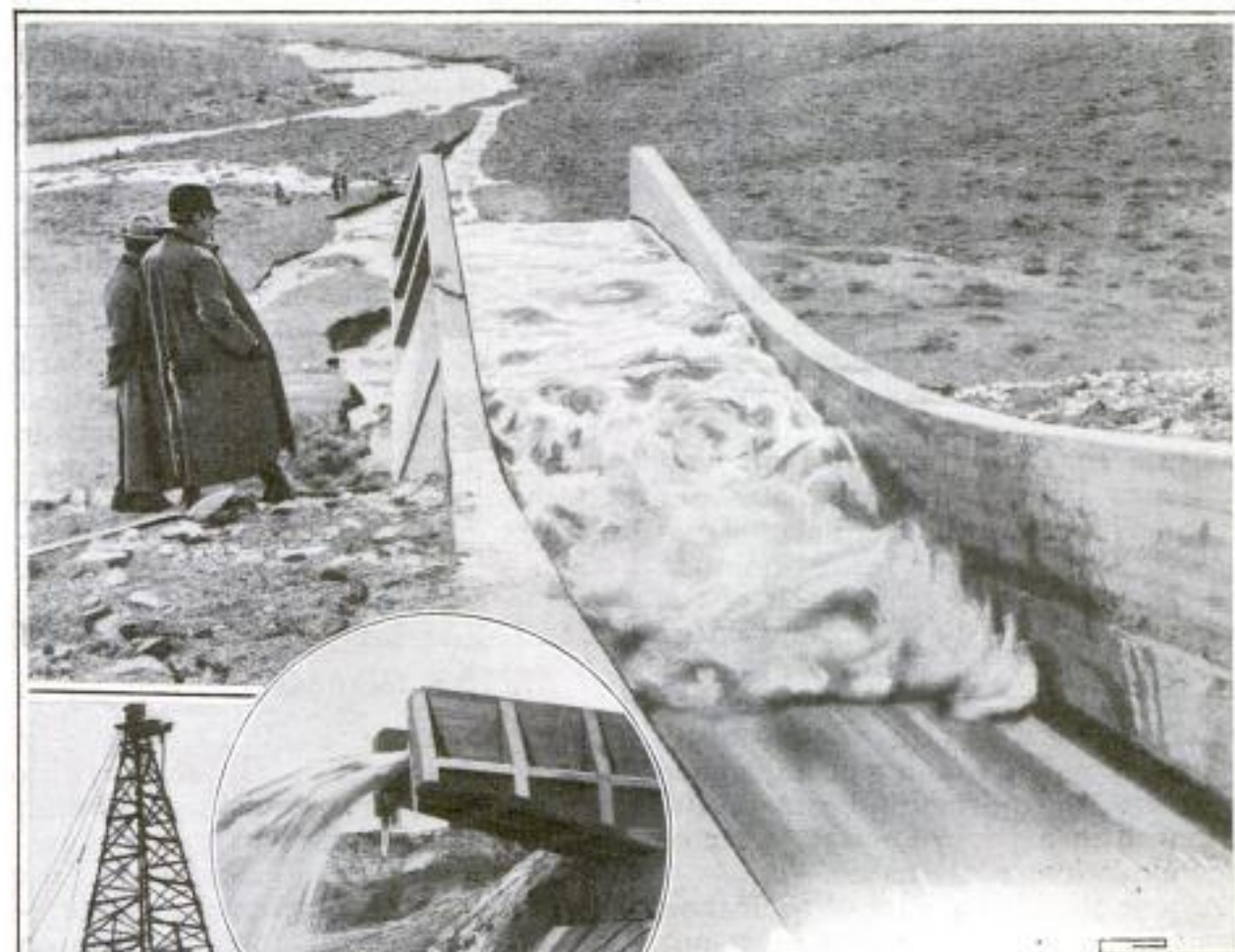
The Back-Water Wave That Forms at the Nozzle When a Small Volume of Water is being Discharged
