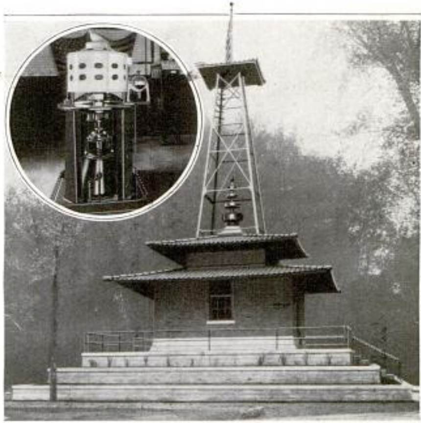
The Terraces Raise the Building above the High-Water Mark. Insert Shows the Type of Pump Employed in This Novel Station
