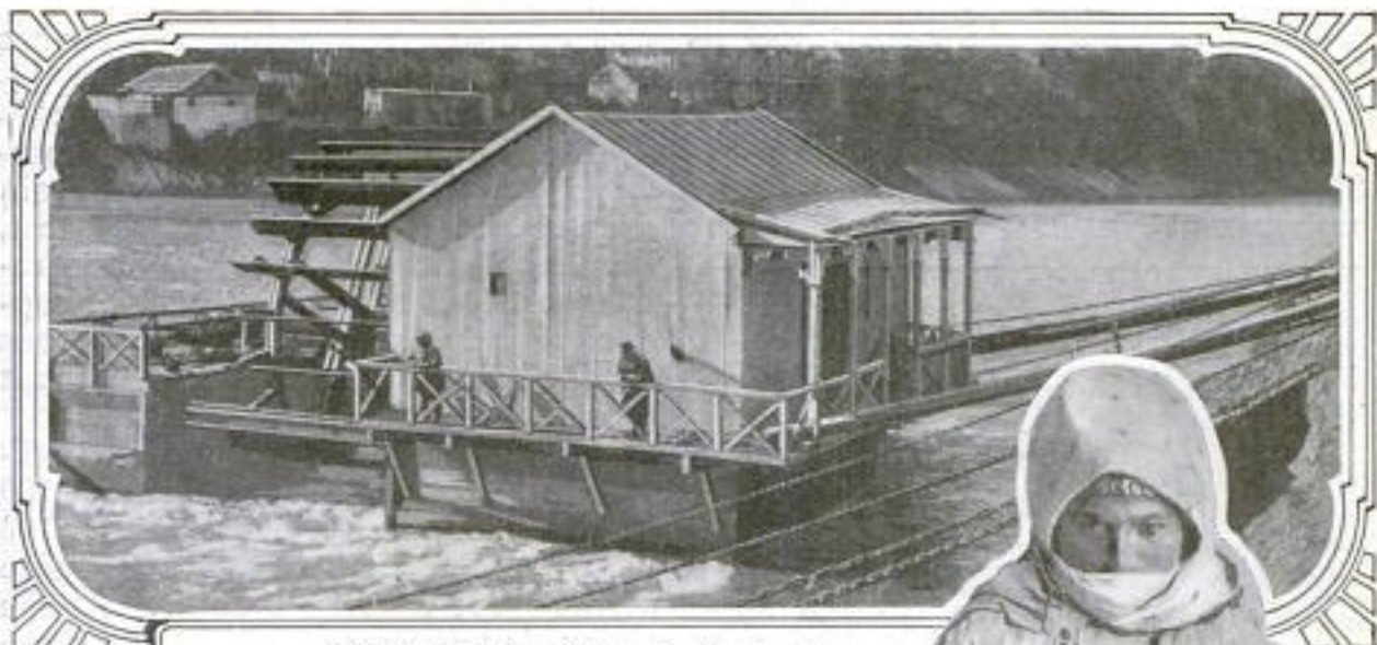
Mill on the River Kur in the Southeastern Part of Trans-Caucasia: This Structure is Built on pontoons and Worked Up and Down the Stream, Grinding First at One Place and Then Another
