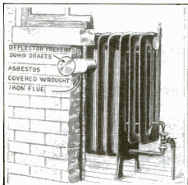
Steam Radiator in Which the Heat is Supplied by Gas: Each Radiator Forms a Unit and No Piping is Required
