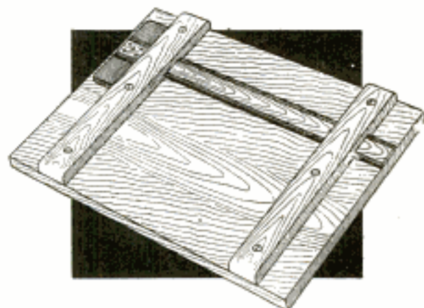
Notches Cut in the Battens of a Drawing Board to Admit the Blade of the T-Square
