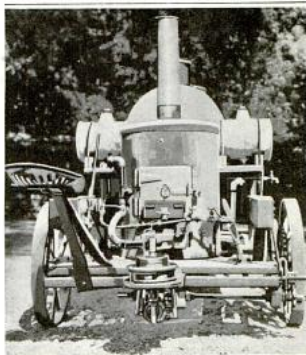
Machine Used in California for Sprinkling Country Roads with Oil
