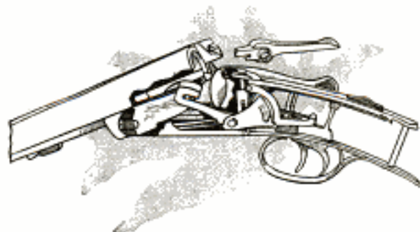
The Side-Plate Lock Is a Development of the Old Hammer Lock with the Striker Inside
