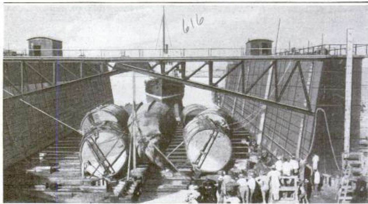
The Submarine "F-4" as It Appeared after being Raised and Placed in Dry Dock: The Steel Cylinders alongside the Vessel Are the Ones Used for Making the Final Lift to the Surface
