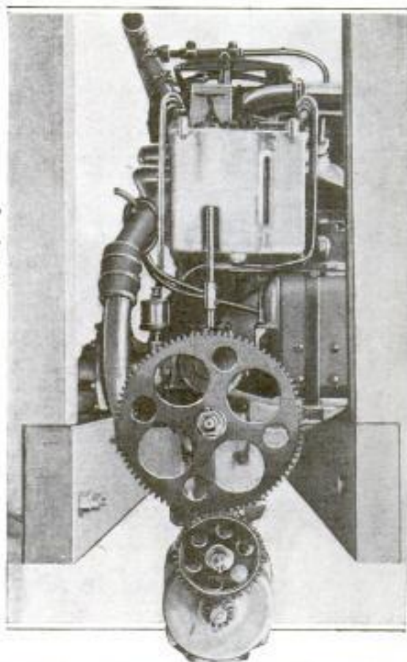
A 90-Horsepower Aerial Motor Fitted with One of the New Electric Starters, Which is Built as an Integral Part of the Crank Case
