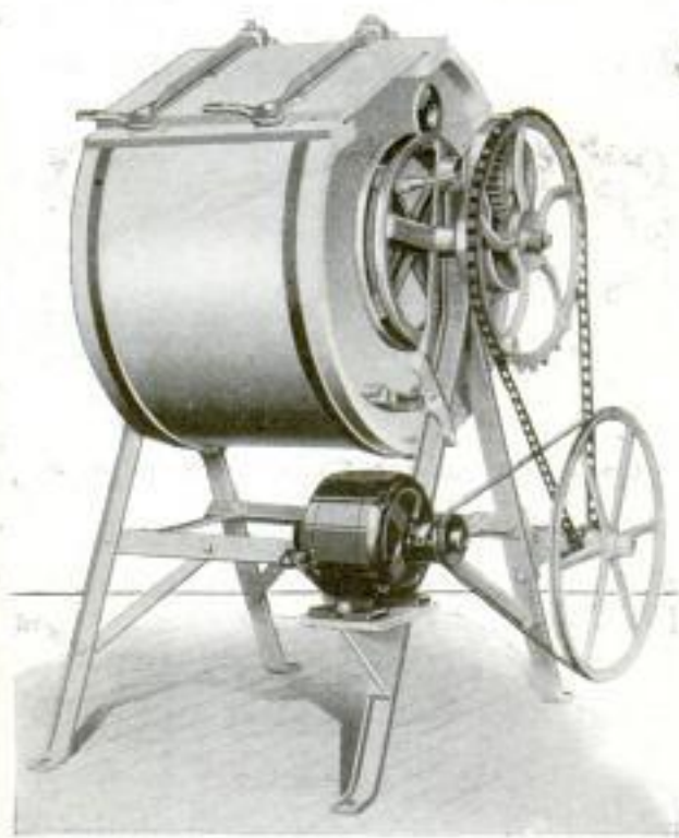
The Machine may be Operated Either by a Gasoline Engine or an Electric Motor
