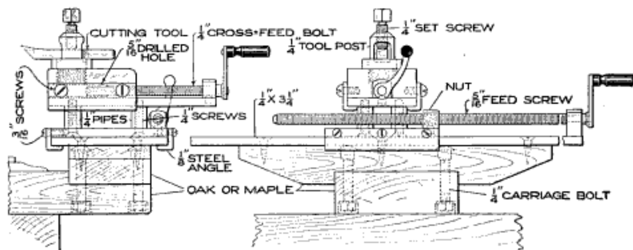
A Compound Rest Adds Greatly to the Equipment of a Wood Lathe, Which Makes It Possible to Turn Accurate Tapers as Well as to Turn Small Diameters in Metals
