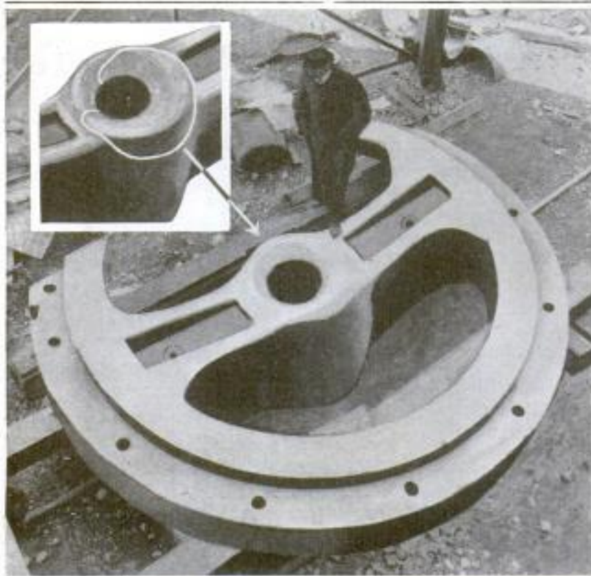
In Repairing the Hub of This 30-Ton Spider, More than 900 Pounds of Metal was Welded into Place with the Oxyacetylene Flame
