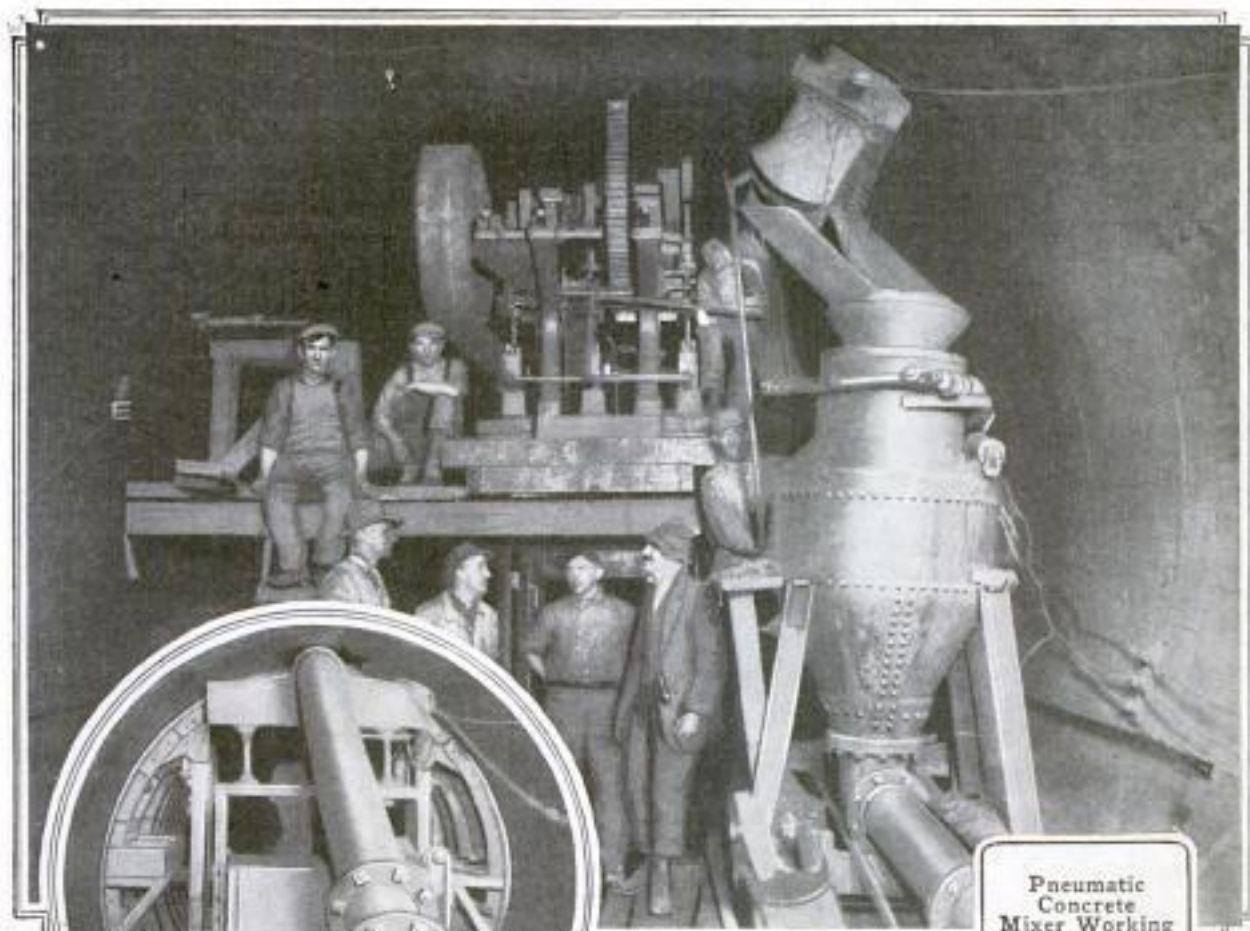
Blowing Con- crete through a Pipe over the Top of Forms in an Eight-Foot Tun- nel for St. Louis Water Works
