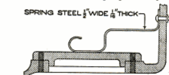
A Stout Spring Makes a Better Holding Device for a Gear-Box Cover than Bolts
