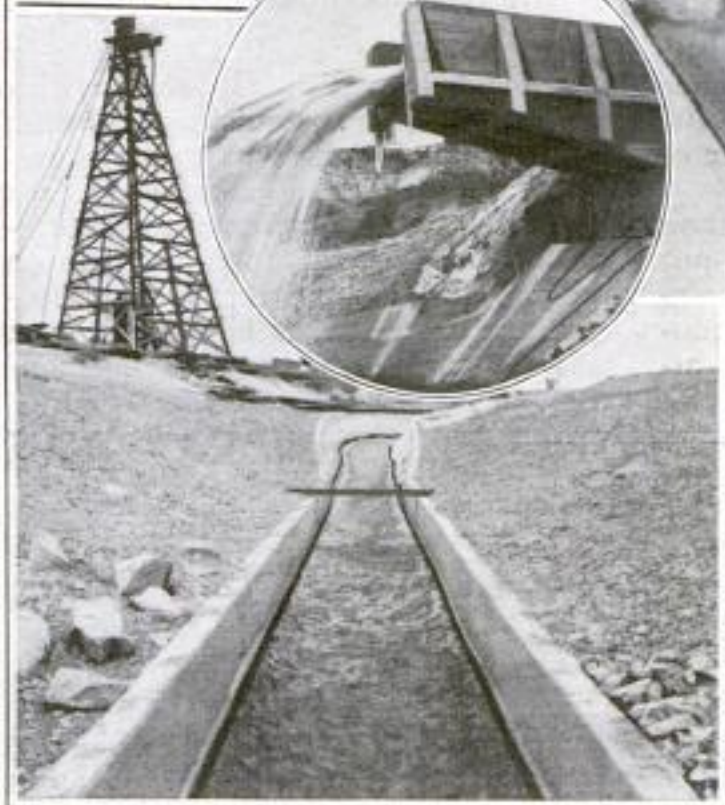
An Intermediate Section of the Chute, Showing How the Rounded Section is Changed to a Rectangular Section. Insert Shows How the Water is Thrown Upward and Outward by the Concrete Nozzle
