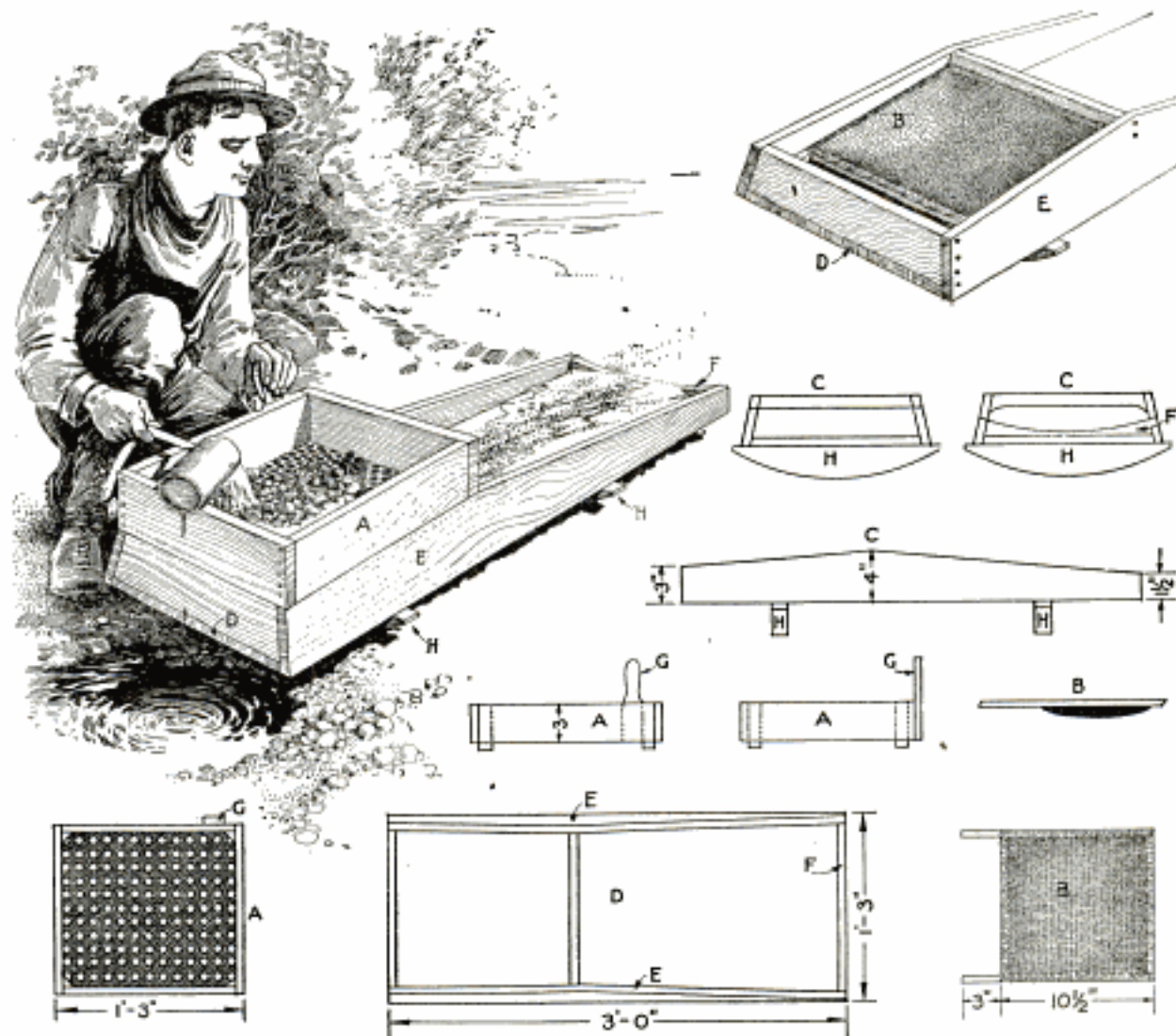
The Cradle or Rocker is Used Instead of the Sluice Box for Recovering Gold in River Beds. It Consists Mainly of Three Parts: the Hopper, Cradle, and Apron, or Inclined Riffle
