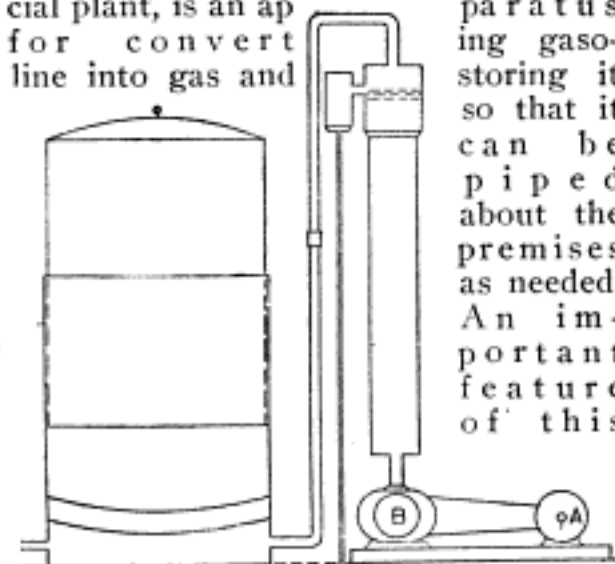
Apparatus for Converting Gasoline into Gas; Air is Forced into the Upright Cylinder by the Blower B, Which is Driven by the Motor A; the Air and Gasoline, After being Mixed in the Enlarged Upper End of the Cylinder, Pass through the Pipe into the Storage Tank at the Left
