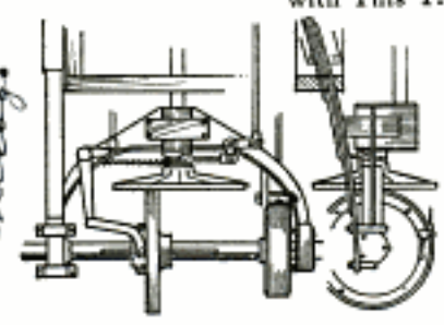
This Rear-Axle Transmission Set Is One of the Simplest Forms of Friction Drive That has been Applied to Cyclecars
