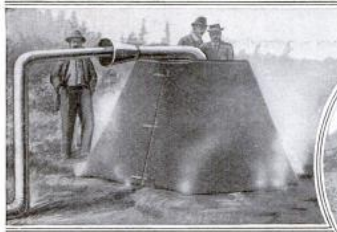
New Type of Stump Burner Which Leaves Only Ashes Behind
