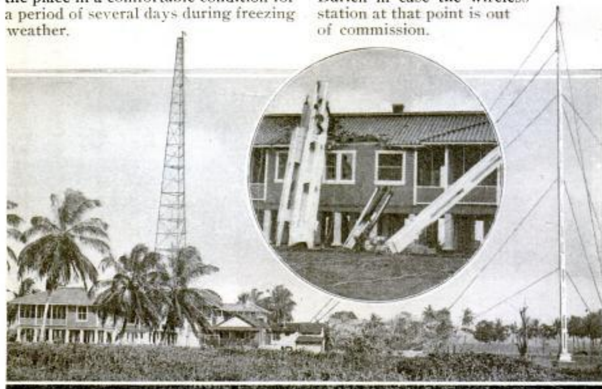
New Steel Tower for Wireless Station at Colon and Wreckage of Wooden Mast That Collapsed While being Taken Down
