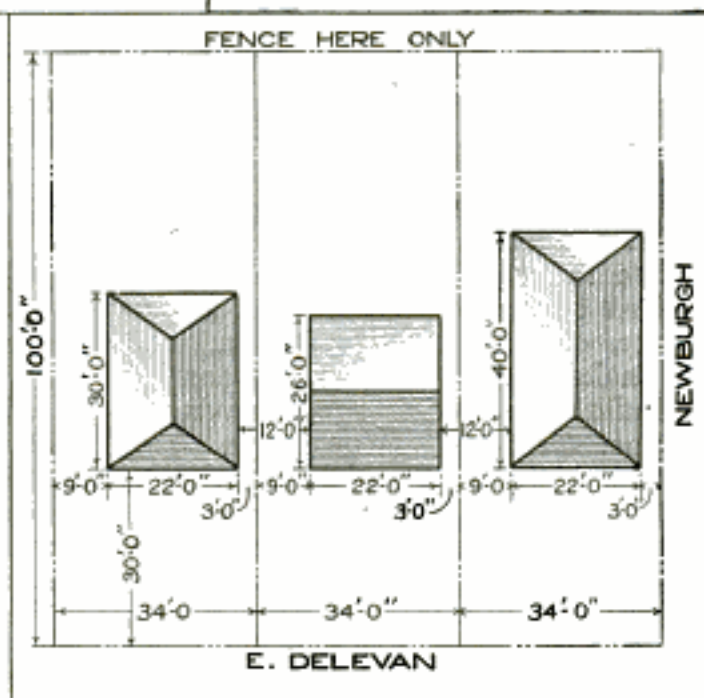
A Ground Plan of a Bungalow, a Semi-Bungalow, and a Two-Family Flat, Erected on Adjoining Lots, Each Having a 34-Foot Front, and All the Lots being Terraced
