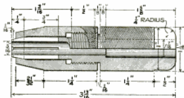
The Knurled Part on the Chuck and Handle are the Same Length to Provide an Equal Grip
