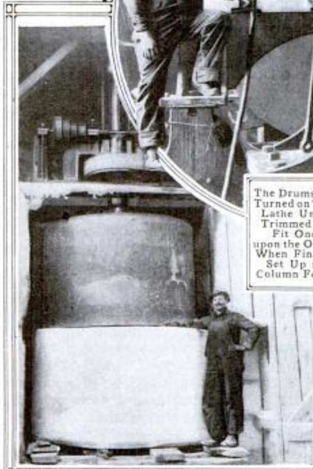
After being Sized, the Marble is Cut by a "Barrel" into Large Cylinders Which are Later Fluted and Polished
