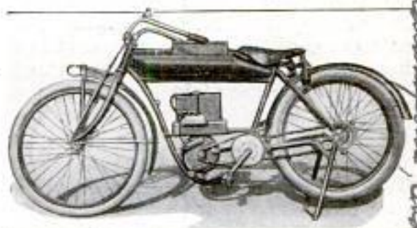
This Motorcycle is Driven by an Electric Motor, Power being Supplied by a Compact Storage Battery
