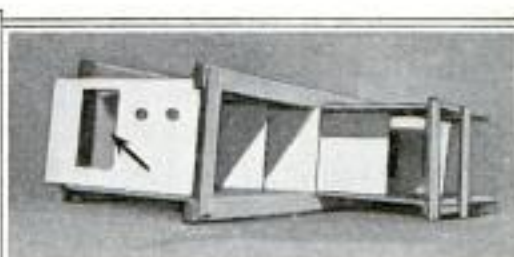
Model of Section of "Empress of Ireland"; Arrow Indicates Cut in Side of Ship
