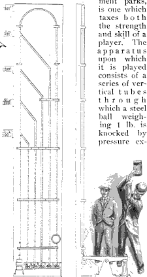
The Harder the Blow the Higher the Steel Ball will Go
