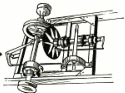
A True Rolling Surface on Fourth Speed and an Automatic Spring Tension at All Speeds are Given with This Transmission Unit
