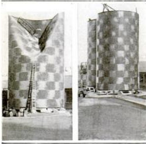
Condition of a Steel Silo After being Hit by a Storm, and How It Looked After It had been Straightened Out with Steel Cable and Pulleys
