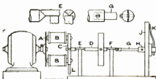
A Torque is Used as Basis for Calculations in Finding the Horsepower of a Small Motor
