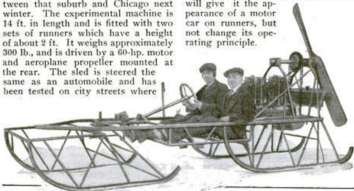
Experimental Aero-Sleigh Which has been Used on City Streets and Driven at a Speed of 35 Miles an Hour
