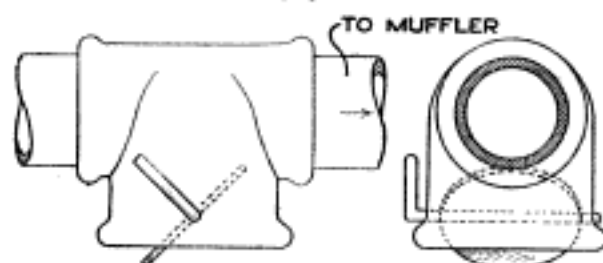
Cut-Out Made of a Tee Fitting Having a Large Side Outlet for the Disk Valve
