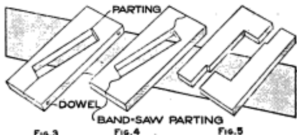
Small and Thin Cores are Made in Boxes Formed of Two Pieces of Wood
