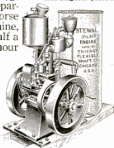
Stewart 3 1/2 horse power engine with high tension magneto $125.00.
