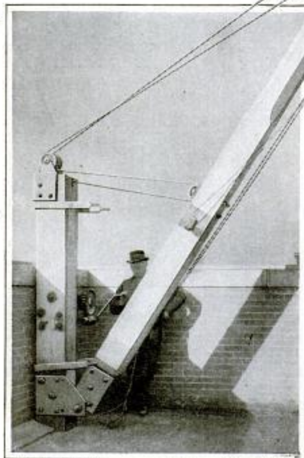
When It Is Necessary to Paint or Repair This Flagpole It may be Lowered onto the Roof of the Building
