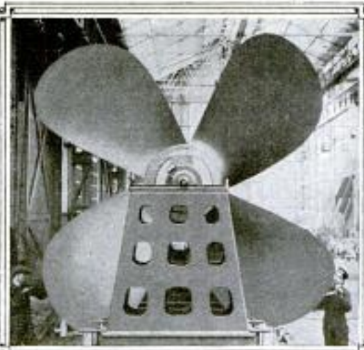
The Center Propeller, Driven by the Parsona Turbine, Is One Solid Piece of Manganese Bronze Weighing 22 Tons
