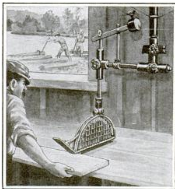
This Saw Guard is Lifted Automatically as the Wood Goes Through, but Falls Instantly into Place as Soon as the Wood Has Passed the Saw
