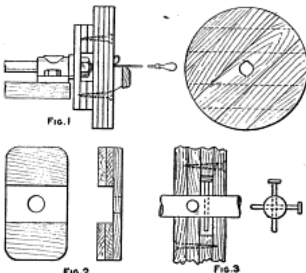
FIG. 2 Operations Necessary in Building Up a Pulley from Pieces of Board, and Method of Keying It
