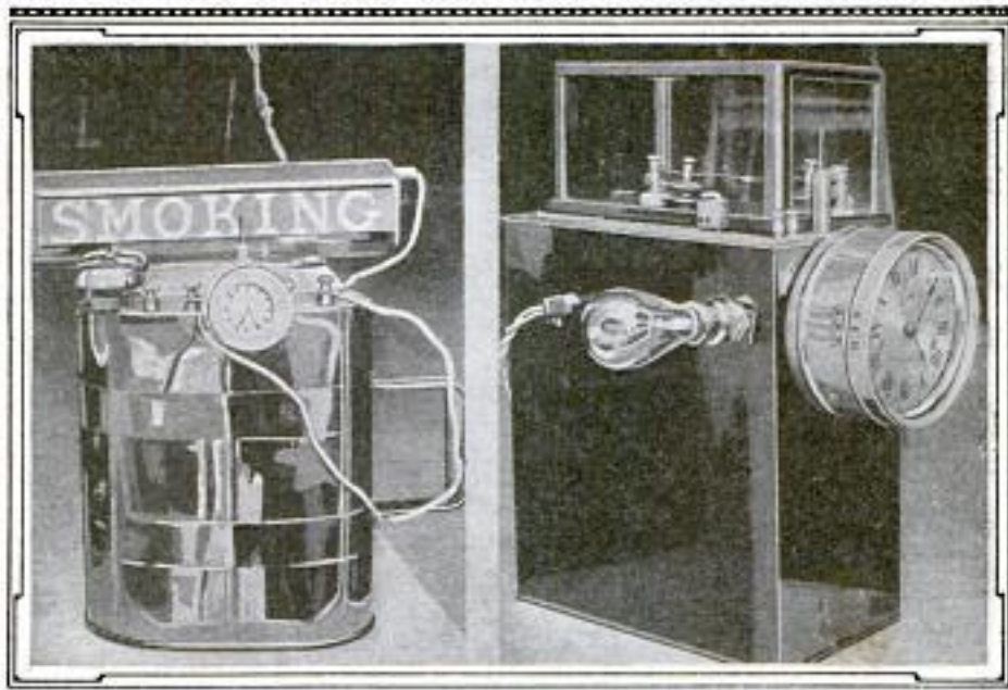
This Sign, "Smoking," is Illuminated When the Smoke from the Factory Stack Exceeds a Reasonable Minimum. Upper Right: Alarm Clock That Rings When the Chimney Smokes, and Records the Time
