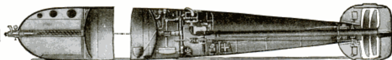
The Nose of This 18-Inch Torpedo Carries about 250 Pounds of Wet Guncotton, Enough to Blow a Hole in Any Ship. Next to This is the Compressed-Air Tank, While Back of the Tank Is the Intricate and Delicate Mechanism That Drives the Propellers and Controls the Rudders
