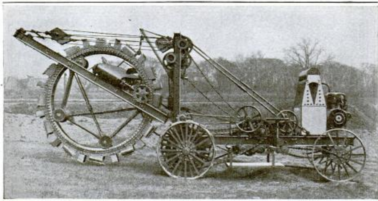
A Trench-Digging Machine That is Propelled and Operated by Gasoline Power
