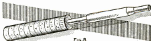
FIG. 8 The Corks Glued in Place on the Butt and the Wood Sleeve, or Reel-Seat Core, Ready to Slide Down and Glue in Position
