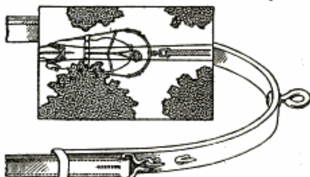
The Rounding Ends of the Singletree do Not Present Any Projection That will Bark a Tree
