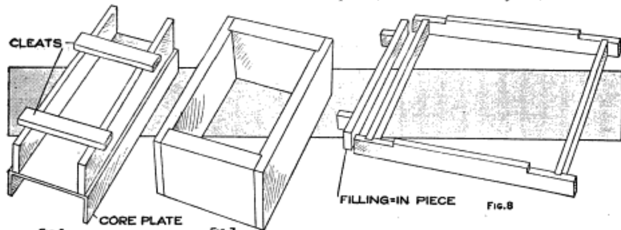
Where It Is Necessary to Make a Long Core for a Column, or a Similar Piece, It is Shaped on a Channel Iron with Straightedges, and Cores for Large Work are Made Up of Separate Pieces into Box Form
