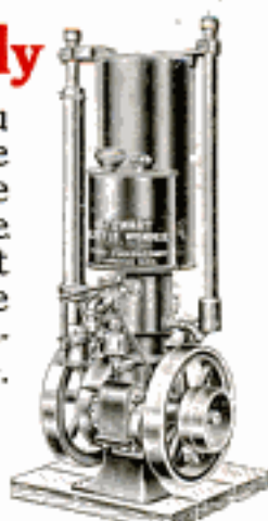
Stewart Little Wonder 2 horse power water cooled, with battery $50.00; with high tension magneto $60.00.
