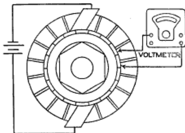
Fig. 3—Connecting a Voltmeter and Current to a Commutator to Test Out for a Short-Circuited Coil rocker arm, and thus short-circuit the machine.
