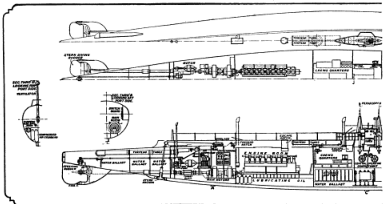
These Diagrams Show How a Typical Modern Submersible is Built; the Vessel is Equipped with Torpedo with Two Periscopes, One Facing Straight Ahead and the
