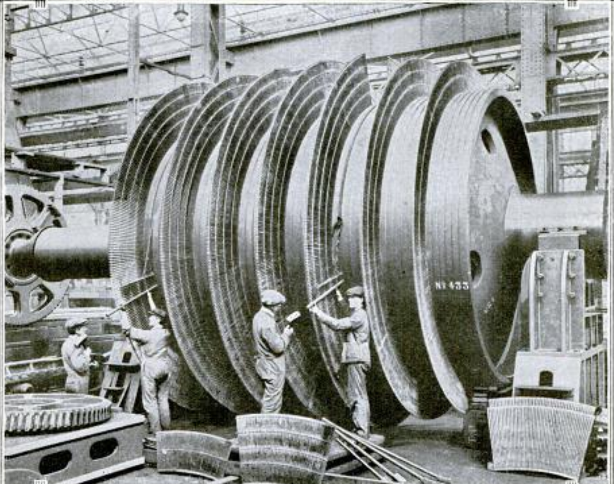
Putting the Blades in the Parsona Turbine: The Blades in This Turbine, 58,946 in Number, would Reach 12\frac{1}{2} Miles If Placed End to End
