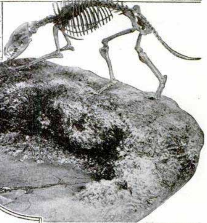
Skeletons of Extinct Animals Found in California Asphalt Pool, Where They had been Trapped Ages Ago
