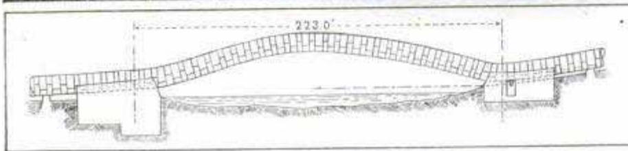
Penstock Arching over the River L'Arc
