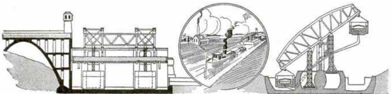
New Canal Lock of Great Lifting Power, Showing Towers and Wells, and How Trough is Raised to High Level
