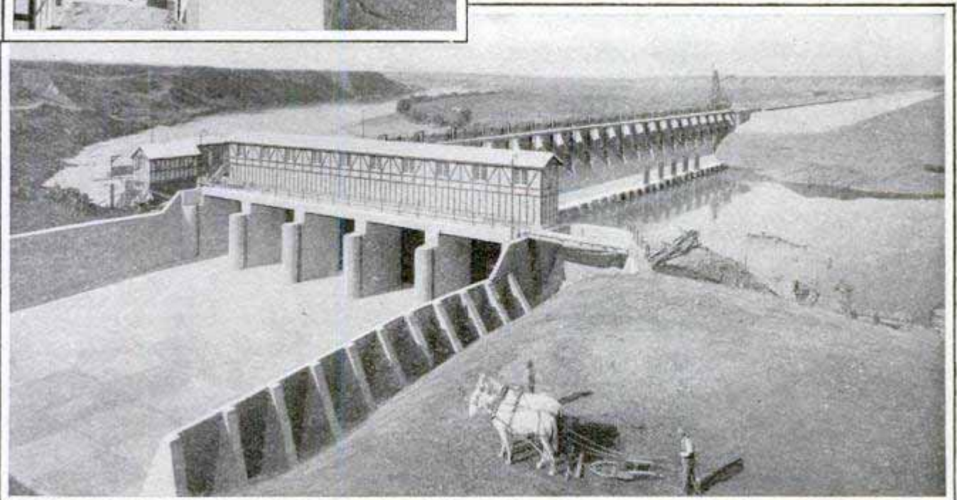
Bassano Dam and Beginning of Main Canal, Upper View Showing Spillway and Protecting Dike
