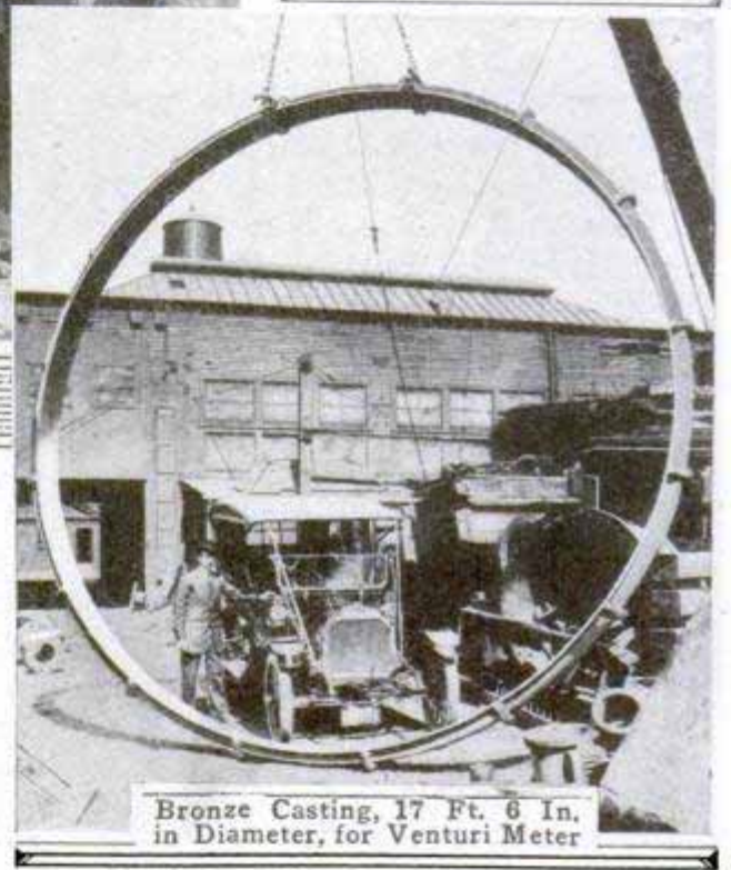
Building One of the Great Venturi Meters Which will Record the Flow of Water
