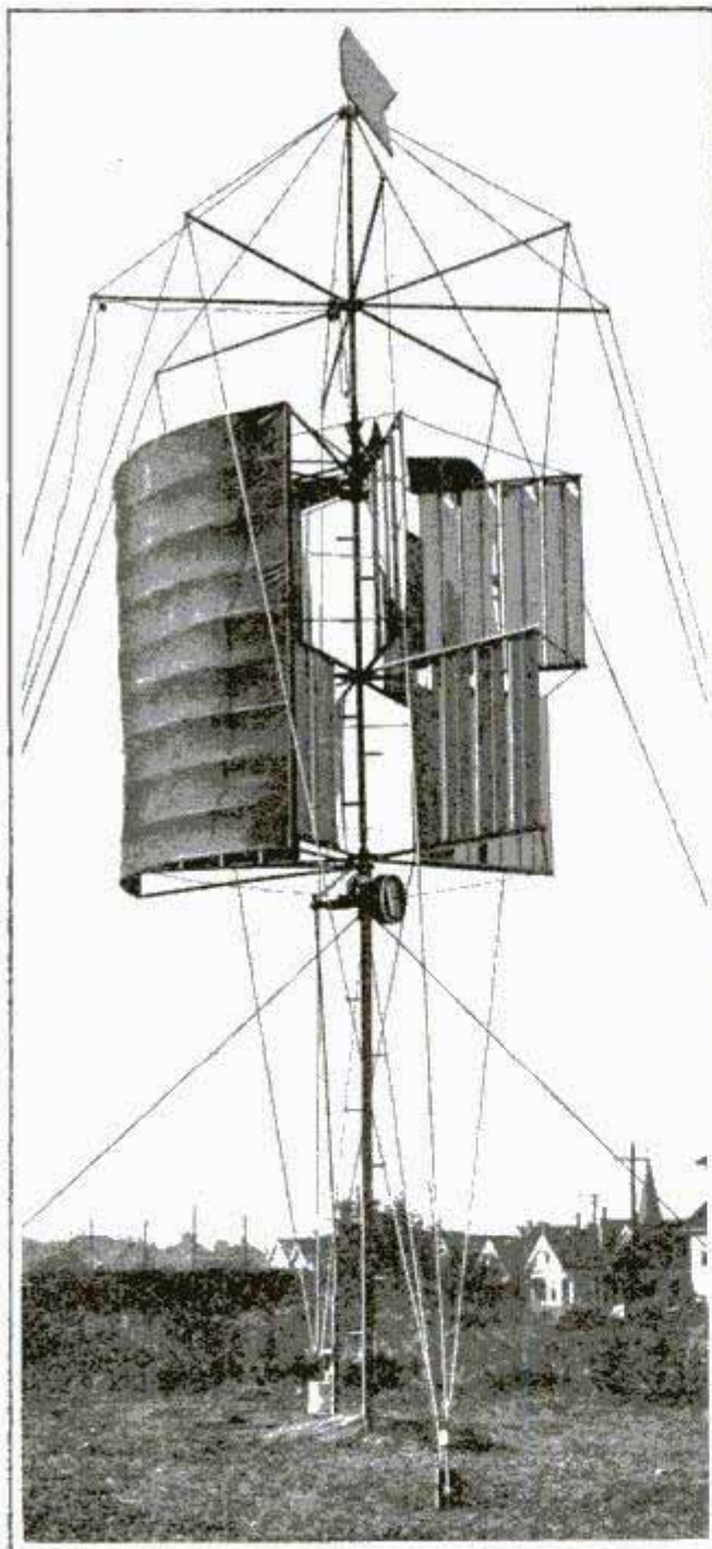
New Idea in Windmill Construction
