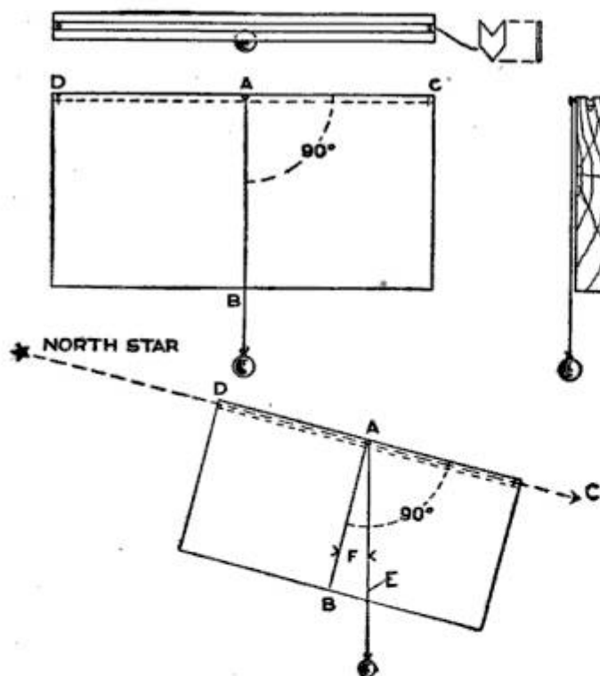
The Main Part of the Instrument Consists of a Board with a Plumb Attached
