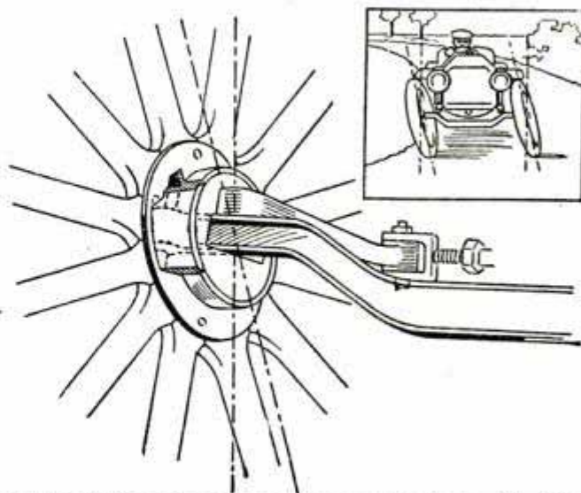
Caster Effect Secured by Connecting Axle with Hub at Point Ahead of Wheel Center. Position of Wheels as Car Makes Turn Shown at Top
