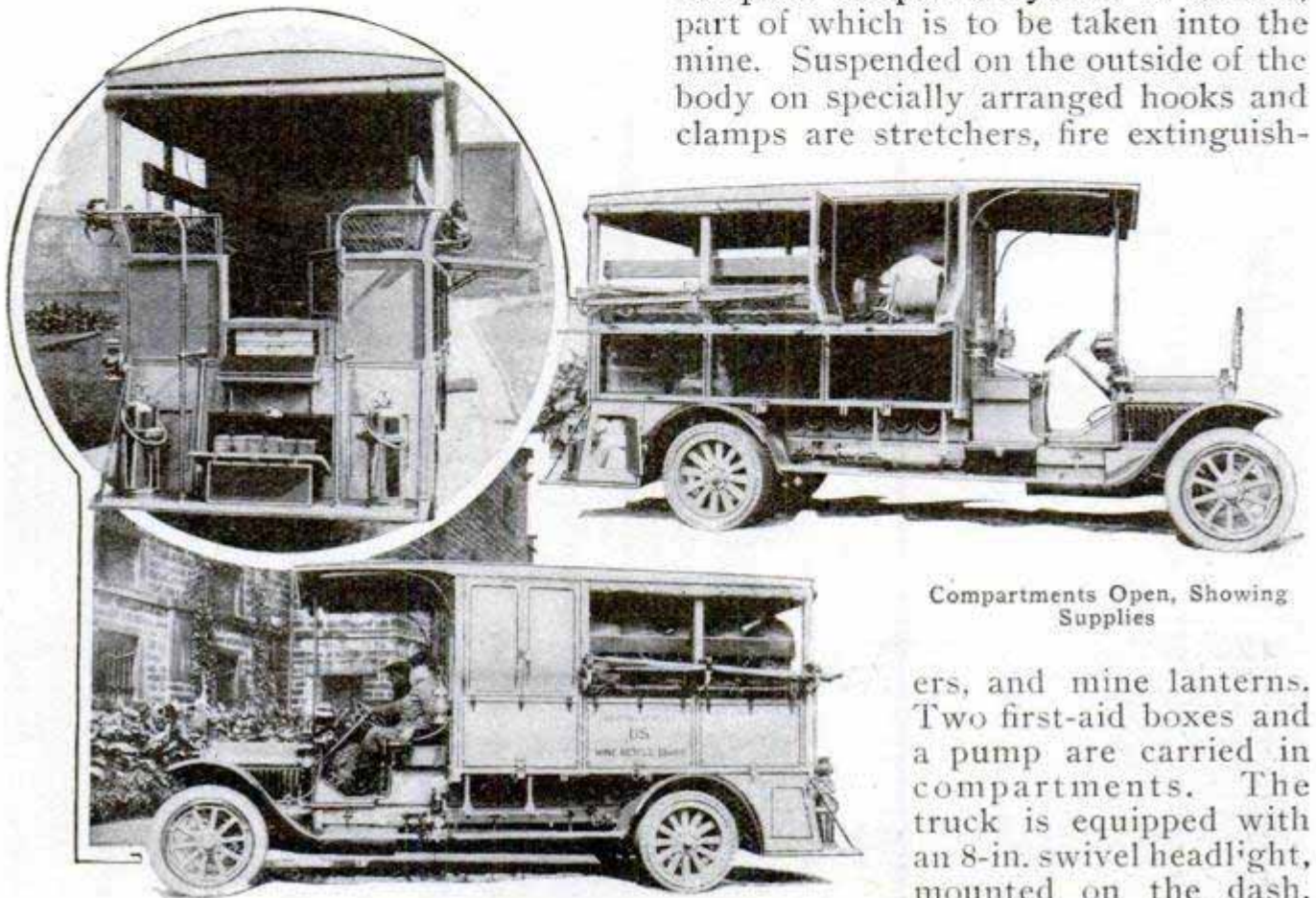
New Type Rescue Truck, Ready for Work. Above, Rear View of Truck, Showing Seating Capacity and Fire Extinguishers
