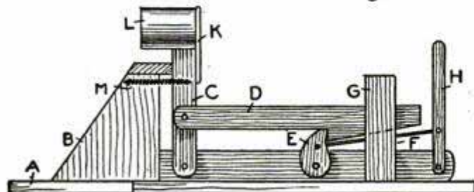
The Dimensioned Parts and the Detail of the Completed Snowball Thrower
