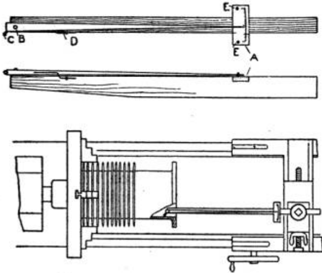
This Homemade Tool will Indicate Any Slight Setting Out of True
