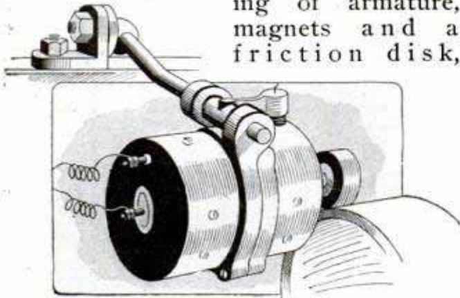
Copyrighted by The Car Small Dynamo for Headlights Which Takes Its Power from the Flywheel
