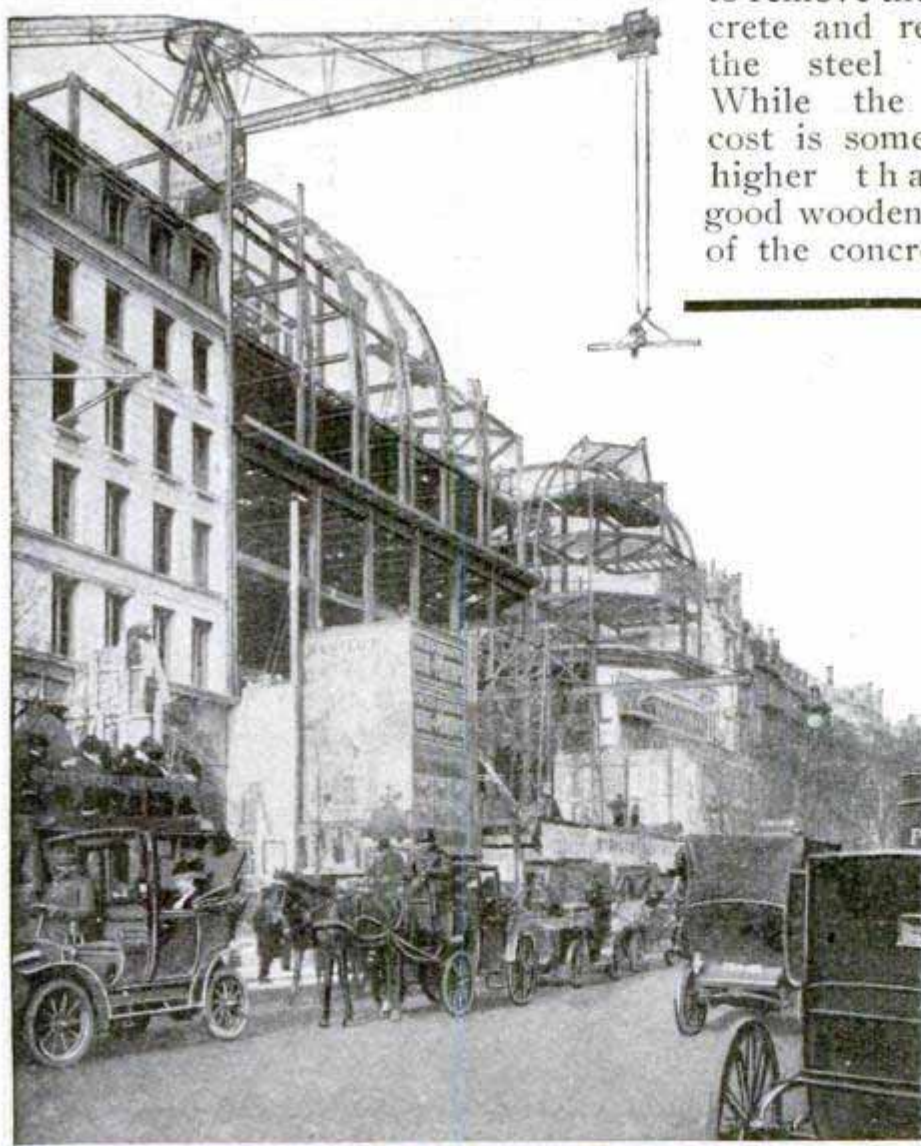
Ingenious Derrick with Movable Crane and Hoist. Right, Trussed Beams Supporting Central Tower
