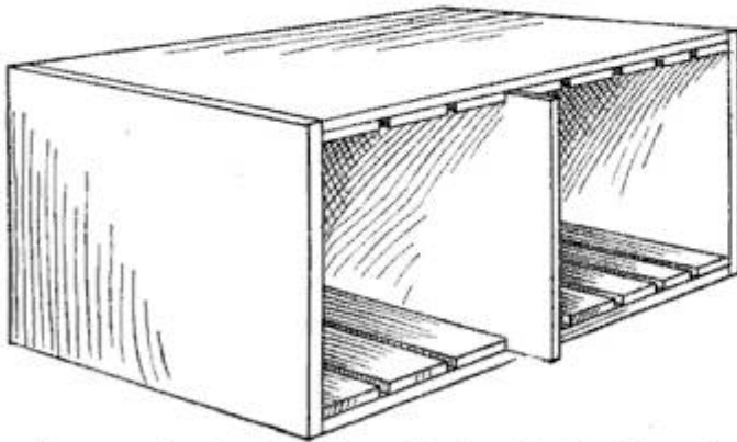
Grooves for the Partitions Made with the Use of Small, Thin Strips of Wood
