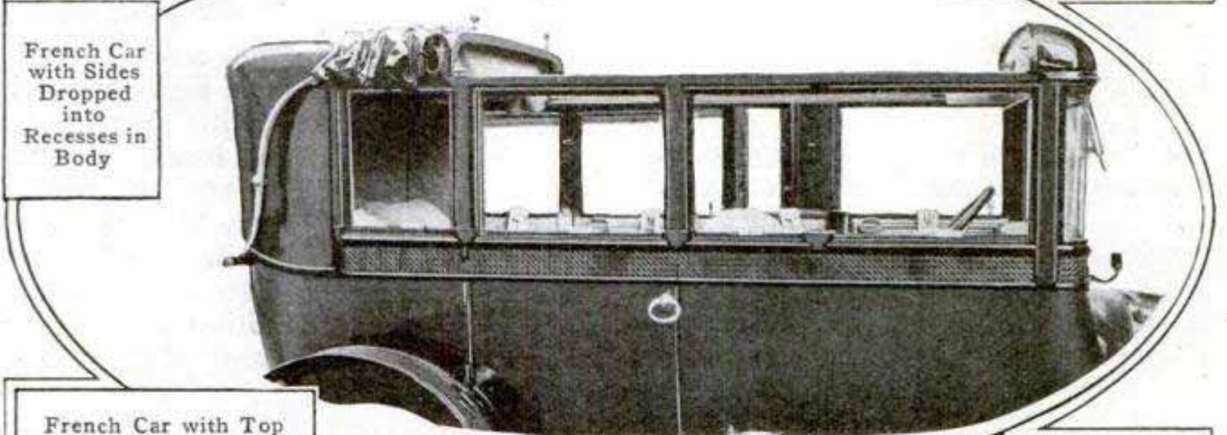
Longitudinal Bars Supporting Top Fold into Windshield
