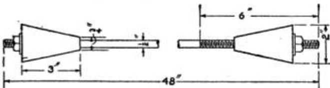
Tapered Cast-Iron Plugs and a Rod Used to Stop Up a Leaky Boiler Tube
