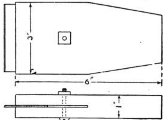
A Handle Attached to a Plain Scraper Blade Makes the Work Much Easier
