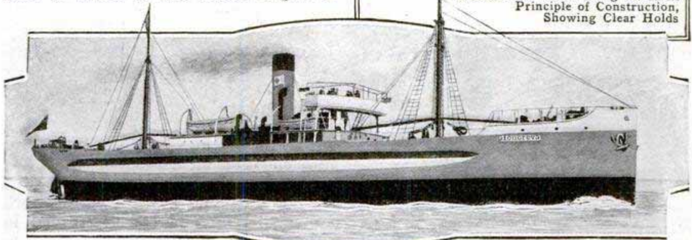
One of the Arch-System Vessels Afloat
