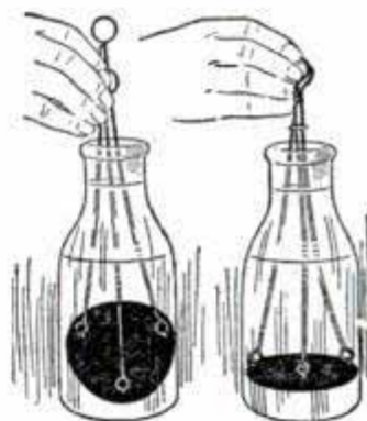
Flexible Rubber Disk Provides an Easy Means of Lifting Cream from Milk
