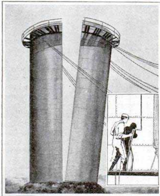
Pulling Down Standpipe Which had been Cut in Two by Oxyacetylene Torch Insert—Cutting Standpipe with Torch
