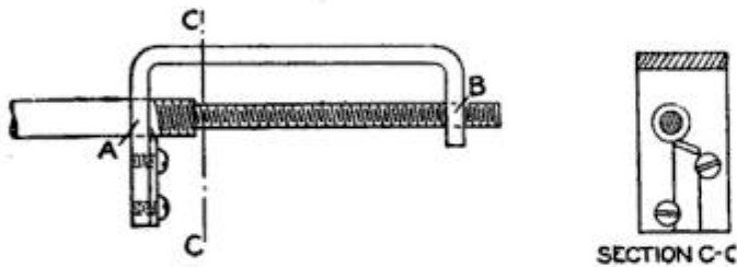
The Standard-Size Threads Make a Feed for the Tool Which Cuts the Threads on the Large Part
