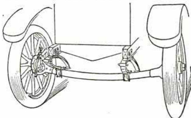
Inclined Front Axle with Support of Car Body Placed Ahead of Wheel Centers
