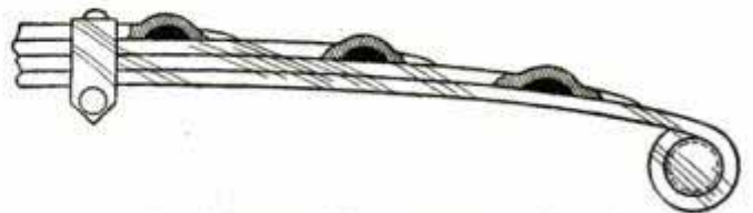
Leaf Spring Which Greases Itself
