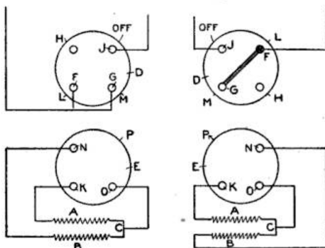
FIG. 1 FIG. 2 Connections of the Heating Elements to Produce Three Changes of Heat in the Pad
