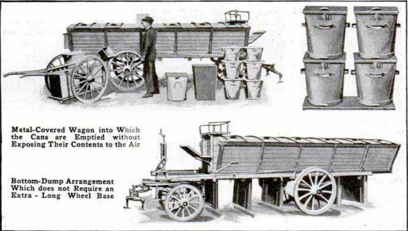
Special Equipment Used in New System of Sanitary Garbage Collection: The Cans Have Square Tops and Tightly Fitting Sliding Covers
