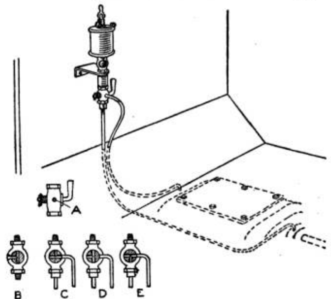
An Oiling System to Take the Place of Wick-Oiling the Bearings on an Automobile
