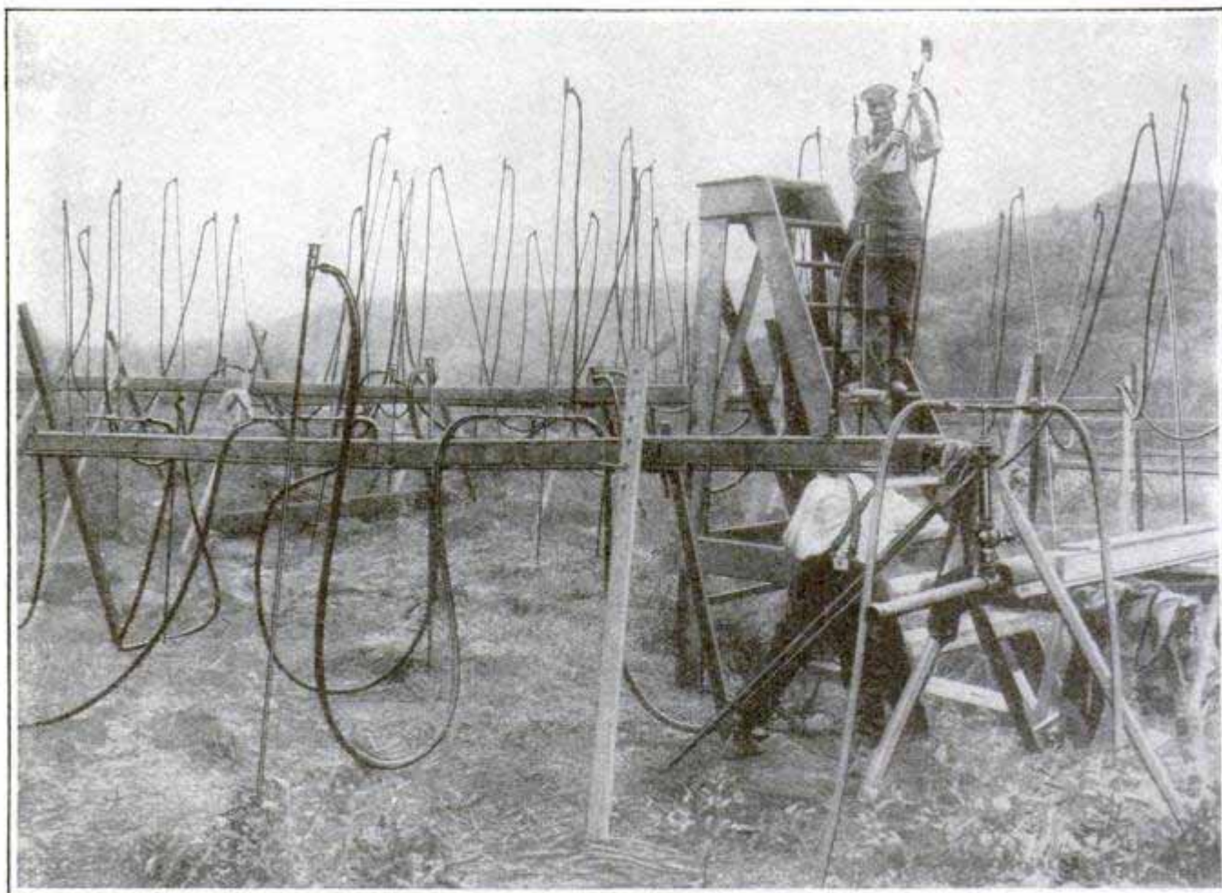
Courtesy The Valve World The Long Alaskan Winter Freezes the Soil to Great Depth, Rendering Mining Difficult. Patches of Ground are Thawed Out with Live Steam
