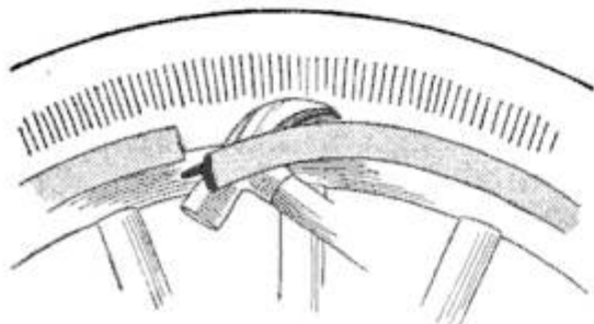
The Claw on a Carpenter's Hammer Inserted under a Rim will Quickly Remove It
