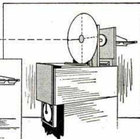
A French Invention Which Registers Hits in Target Practice
