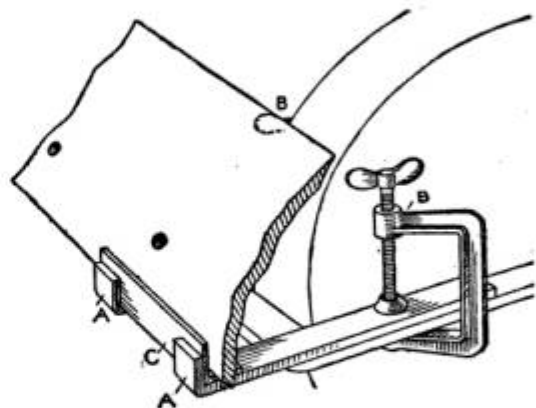
Holder for Grinding Machine-Cutter Knives on an Ordinary Stone or Emery Wheel
