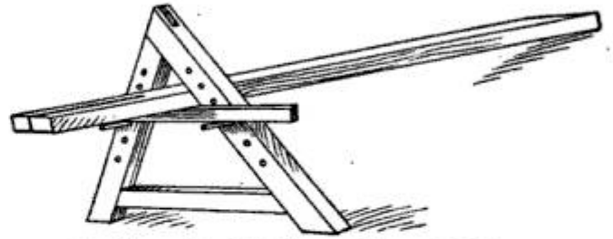
A Horse for Holding a Heavy Timber While Ripping It with a Handsaw
