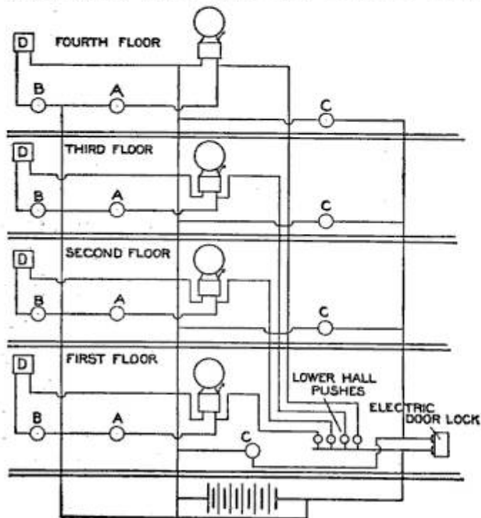
Complete Electrical Circuit for the Front and Back-Door Bells and the Electric Lock
