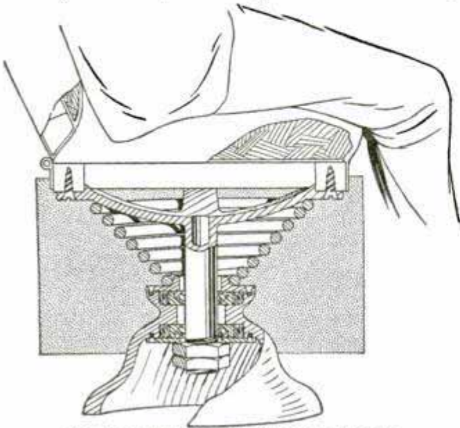
Car-Seat Support Designed to Absorb Vibration of Train.
