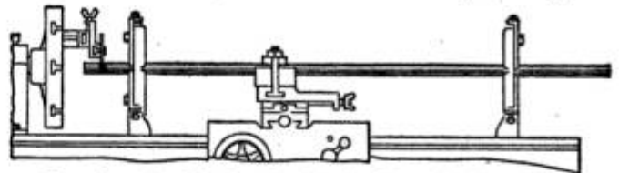
Turning the Ends of a Shaft That is Too Long for the Bed of a Lathe
