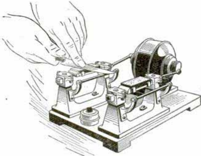
Electrical Vibrating Grinder
