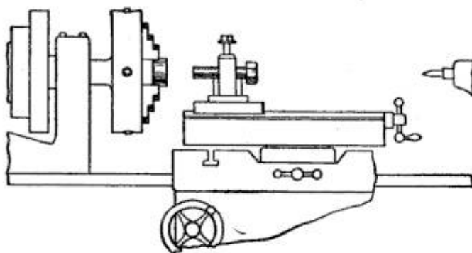
The Studs were Clamped in the Tool Post and Threaded in a Die Held in the Chuck
