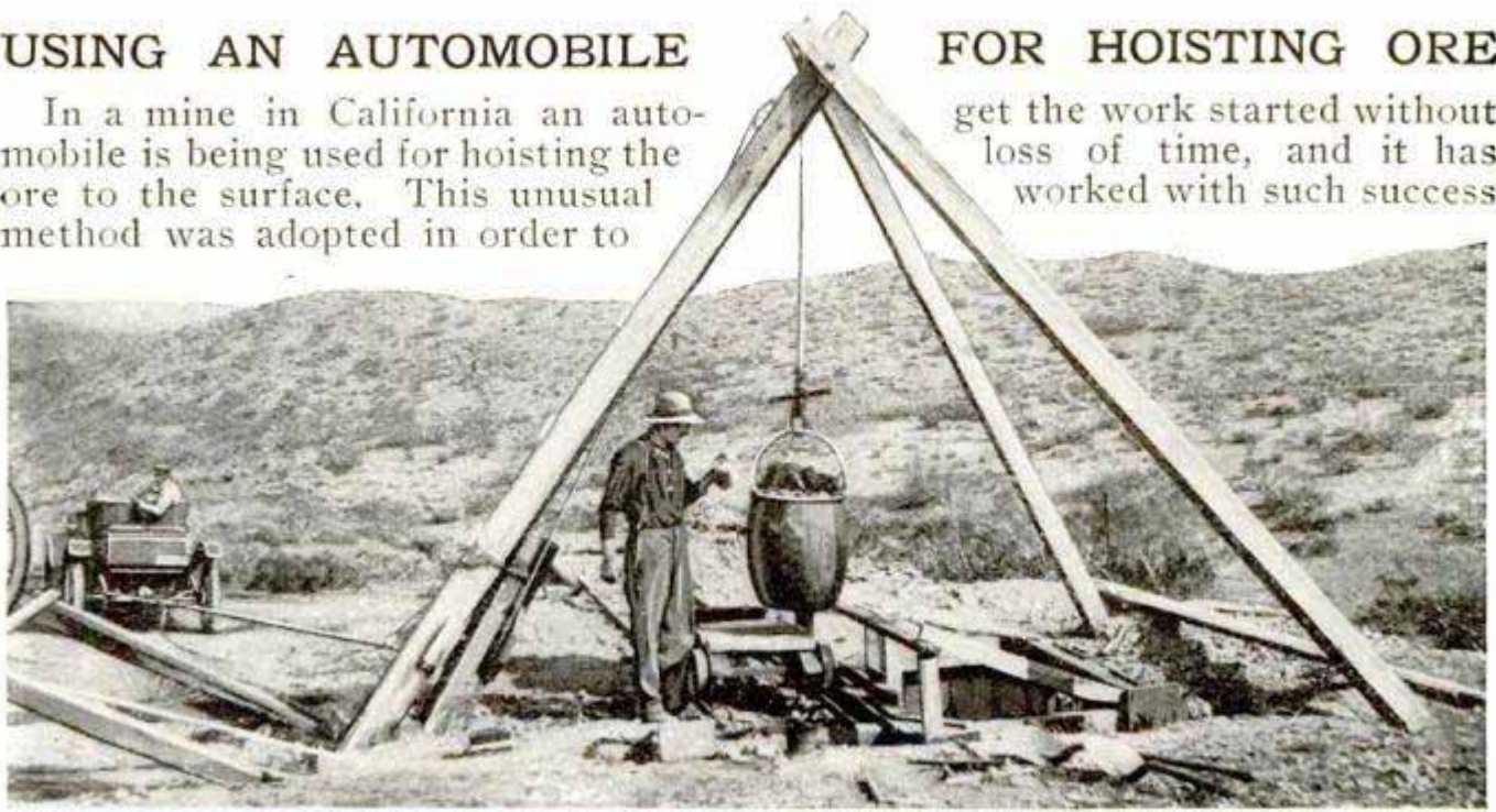
Automobile Supplies Power for Hoisting Ore
