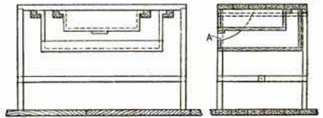
To Place One Drawer within Another under a Bench Top is Handy and Saves Space
