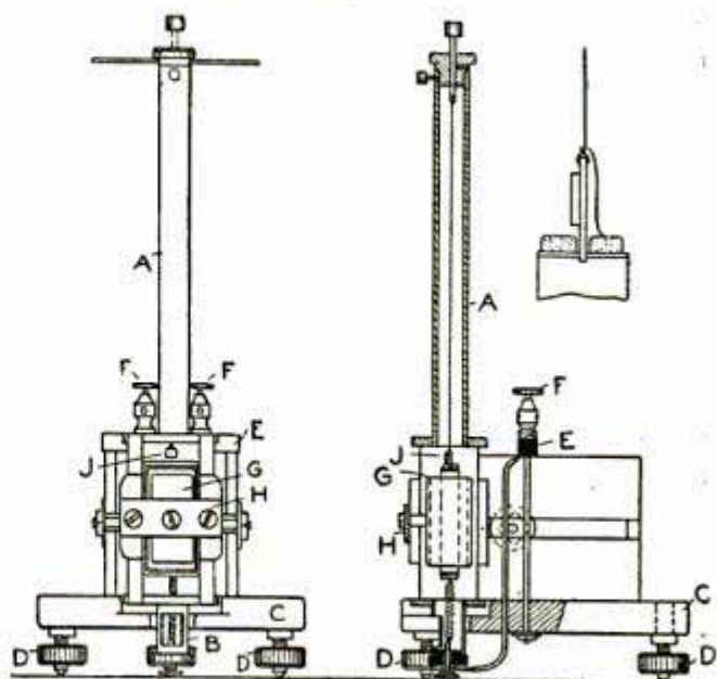
Galvanometer Constructed of Parts Taken from a Two-Bar Telephone Magneto Ringer
