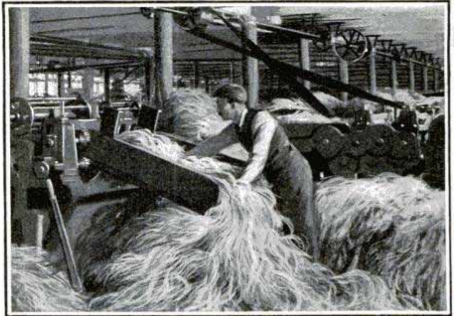
Making "Sliver" or "Roping," the First Mechanical Process in the Manufacture of Rope
