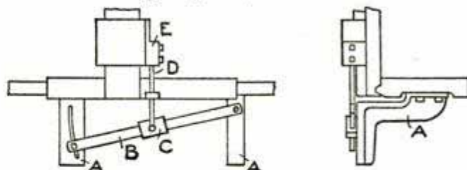
The Slide on the Bar Controls the Cross Feed So That a Taper Cut is Taken
