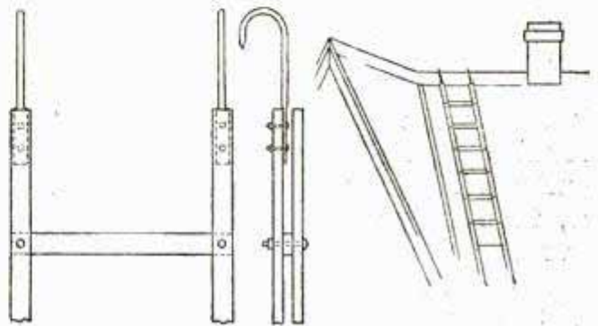
An Adjustable and Folding Ladder to Fit Any Slope or Angle of a Roof
