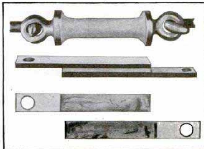
Steel Disks Vulcanized to Round Piece of Rubber— Rubber Vulcanized between Steel—Steel Pieces Torn Apart, Rubber Adhering to the Steel
