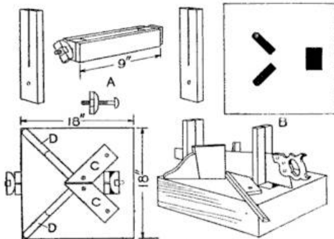
Homemade Miter Box for Sawing Frame Molding and to Hold the Parts for Fastening Together
