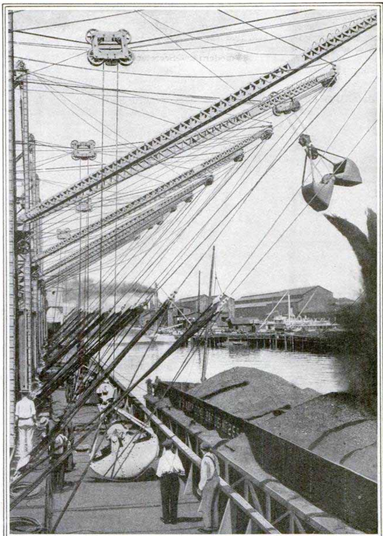
A View along the Deck of the "Proteus," Showing Operation of the Equipment for Coaling War Vessels
