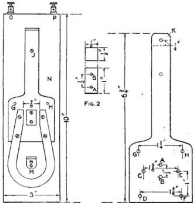
FIG. 1 FIG. 2 FIG. 3 The Permanent Magnet and Its Brass Support, and Their Position on the Base
