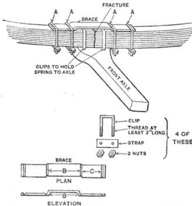
The Brace Clamped to the Broken Parts will Hold the Spring Temporarily Until It can be Repaired
