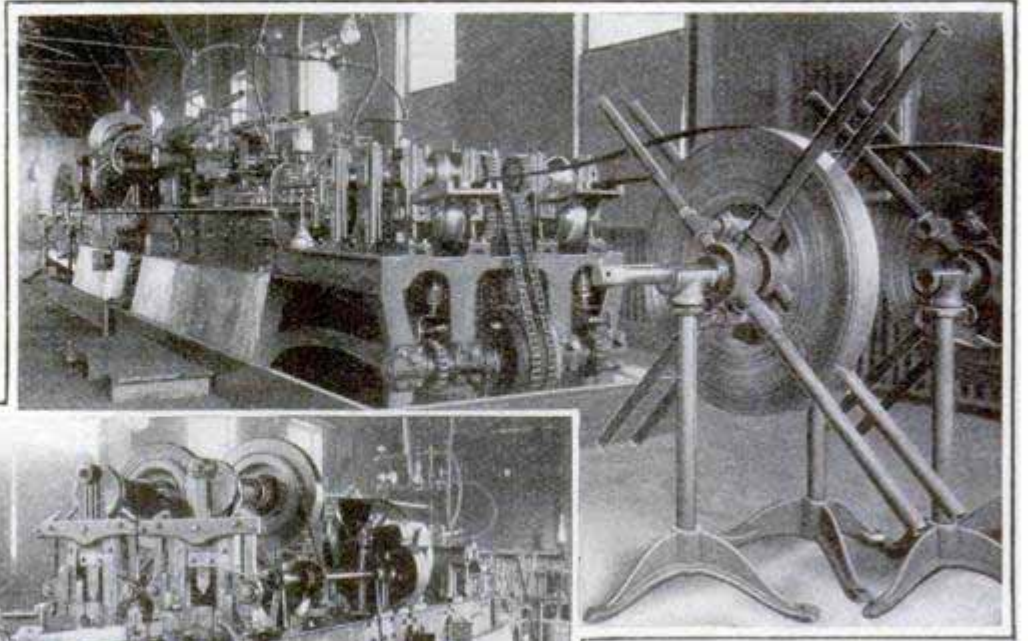
How the Sheet Metal is Fed into the Tube Machine
