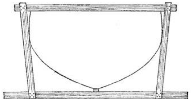
Holder to Keep a Boat on an Even Keel When the Tide Goes Out
