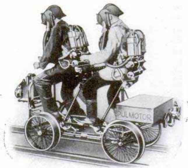
First-Aid Car for Saving Life in Mine Disaster
