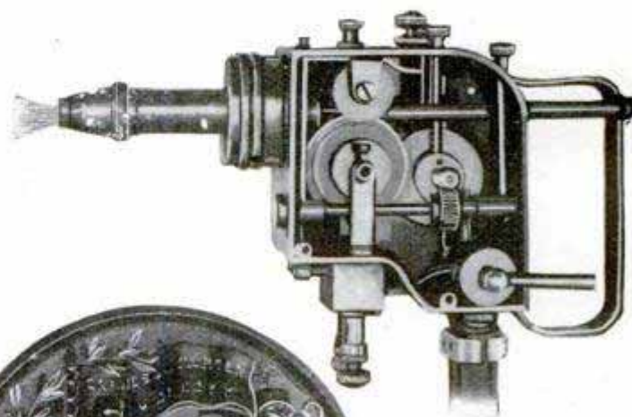
The Nozzle Consists of an Oxyhydrogen Flame Which Melts and Sprays Small Particles from the End of a Wire
