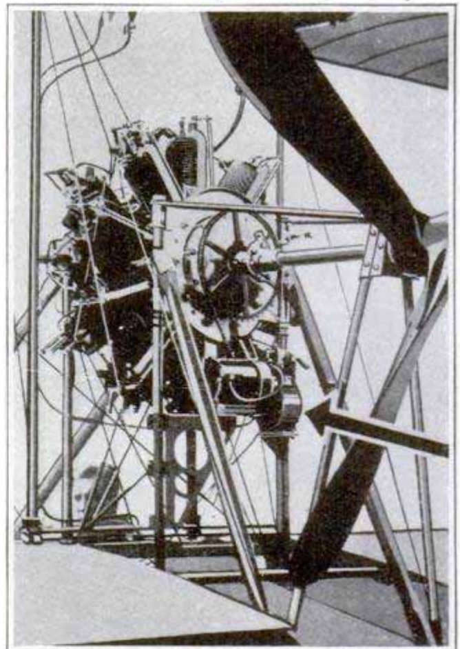
Arrow Shows Electric Starter Installed on Flying Boat
