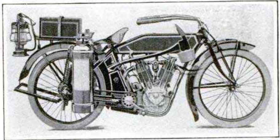
An American Motorcycle Equipped for Fire Service
