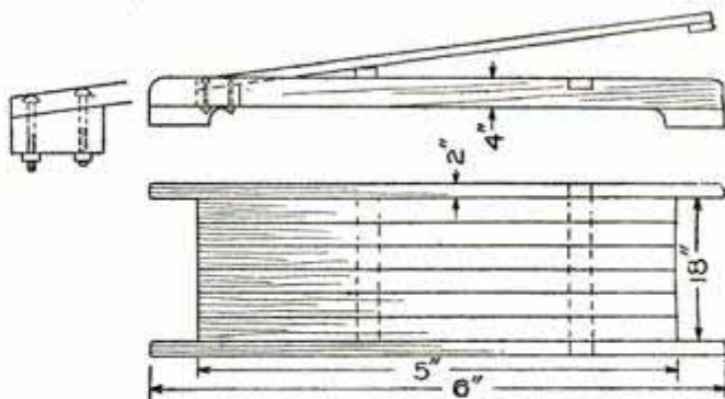
A Springboard for Use in Connection with a Vaulting Pole or for Turning Acts
