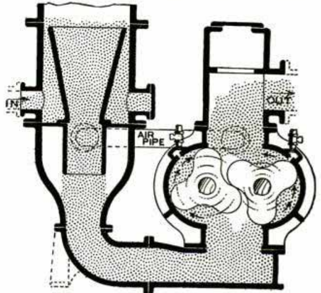
This Vacuum Pump Has No Valves, the Impellers Working Together Like the Parts of a Gear
