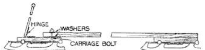
Homemade Pushmobile, Constructed the Same as the Wheeled Kind, with Runners for Snow and Ice
