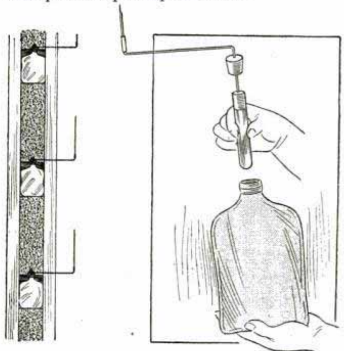
Arrangement of Hot-Water Bottles in Concrete Test Column
