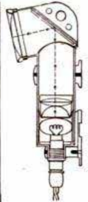
New Type of Automobile Headlight Which Throws Light Beams Forward and Downward Only
