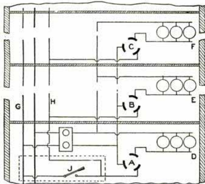
A Separate Light Circuit for Applying Current to All Lights of a Building from a Secluded Switch
