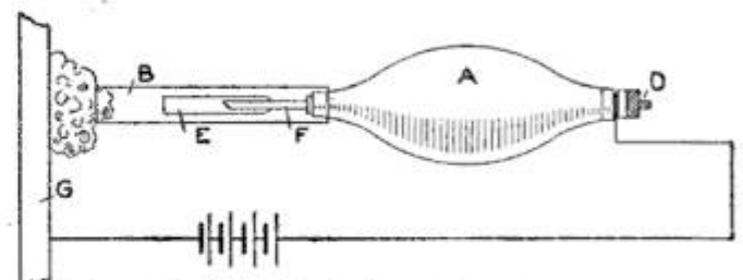
A Hand Tool for Applying a Plate Electrically to the Surface of Metal
