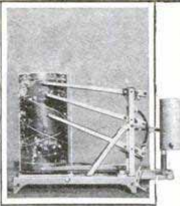
Meteorograph for Recording Temperature, Humidity, and Pressure
