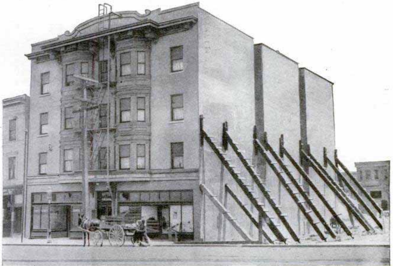
San Francisco Building That was Moved and Then Set Back on New Foundation
