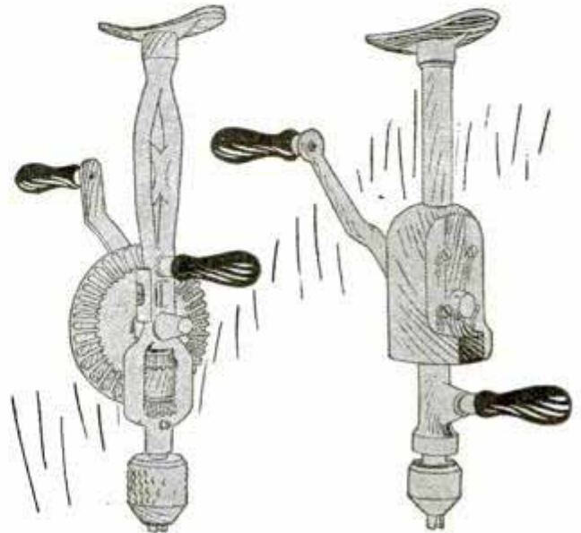
American Breast Drill with Exposed Gears
