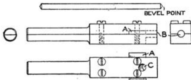
An Inexpensive Tool Used in a Drill Press the Same as a Drill for Pointing Rod Ends
