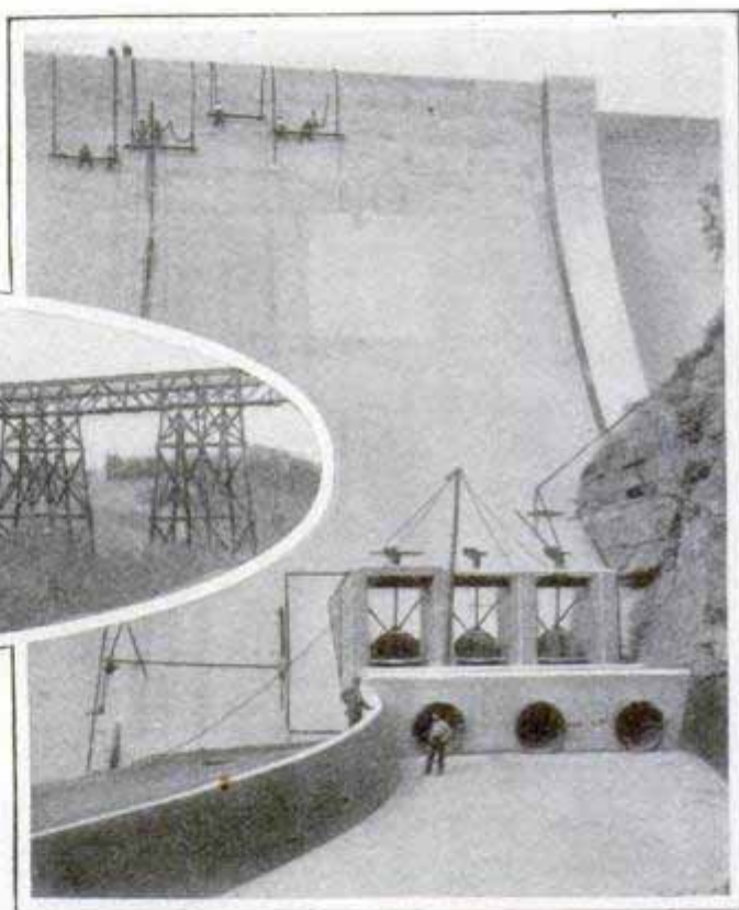
Main Outlet Gates of Medina Dam
