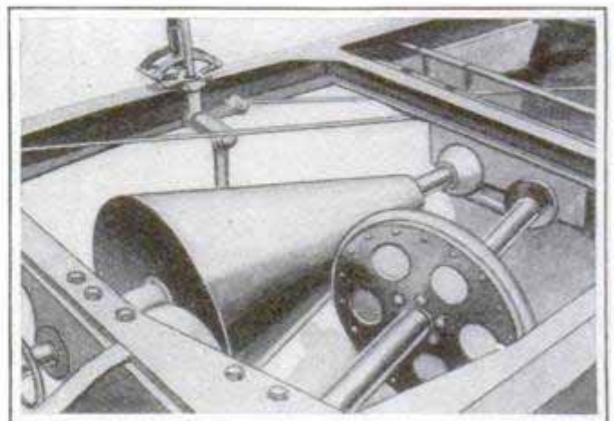
Variations in Speed Secured by Sliding Wheel to Engage Larger or Smaller Sections of Cone
