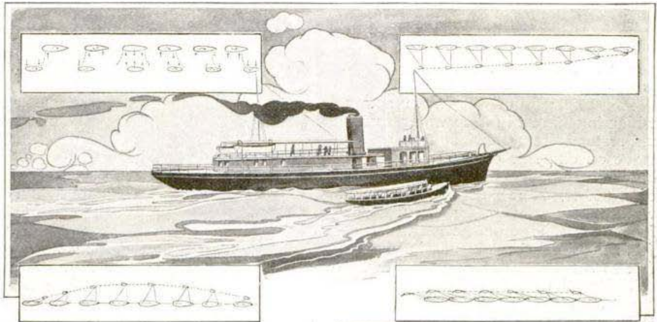
The Suction between Passing Ships Which Causes Them to Collide: Forces Exerted on a Launch Passing a Yacht Traveling in the Same Direction
