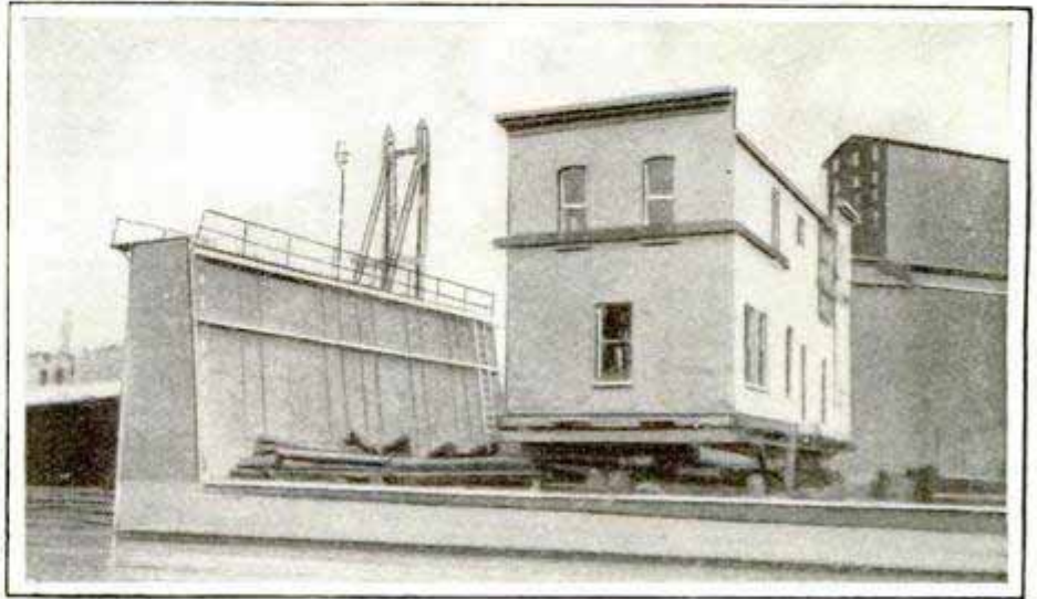
Brick Building Loaded on Floating Dry Dock and Moved to New Site
