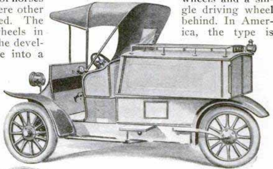
English Three-Wheeled Light Truck, Driven by the Rear Wheel
