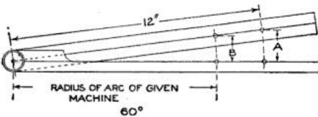
Gauge for Setting Boring Mills or Other Machines to Do Accurate Taper Work
