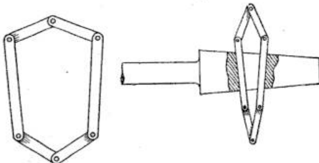
Template Made of Discarded Hacksaw Blades for Obtaining the Shape of a Taper Hole
