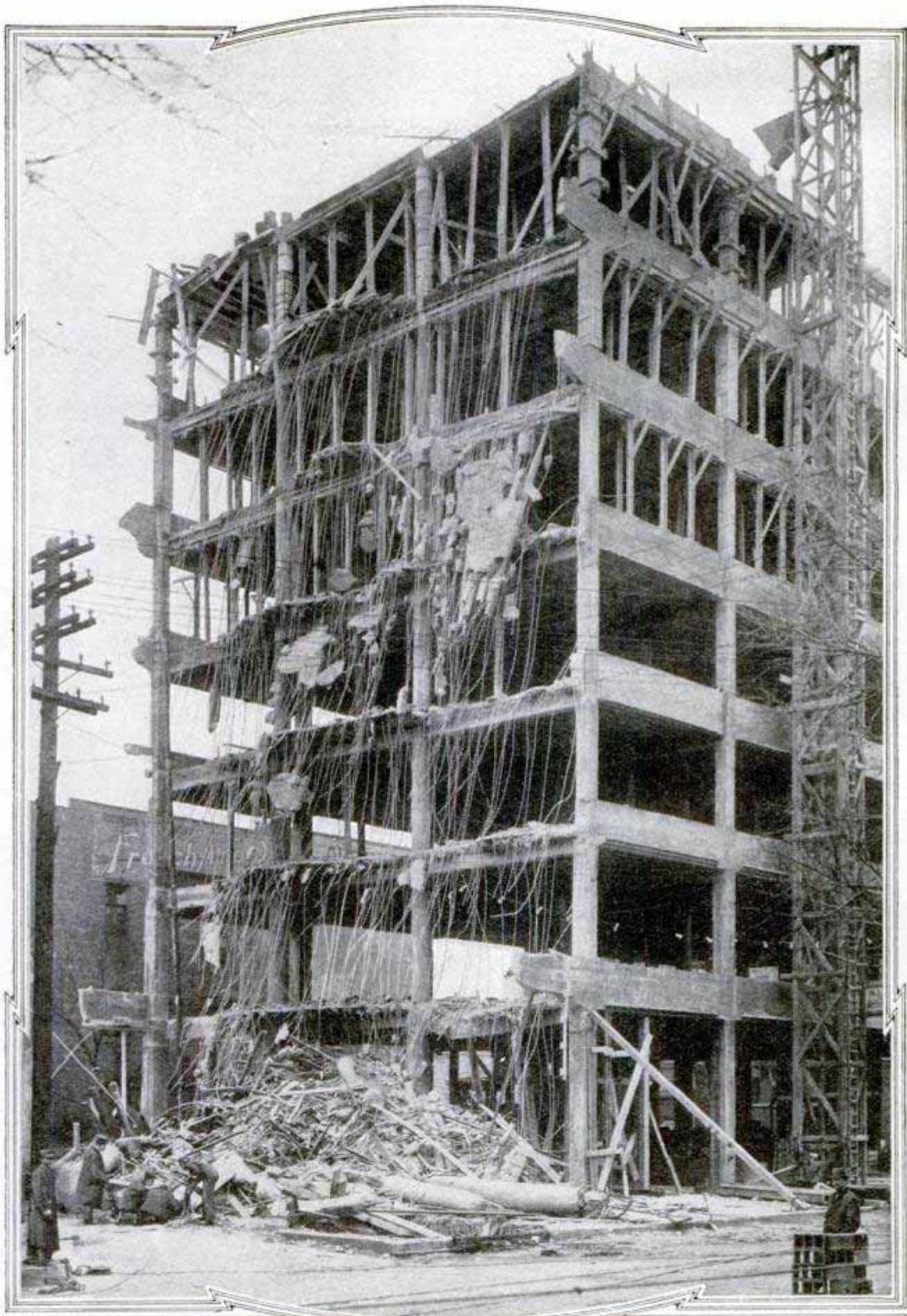
While the Roof of This Building was being Poured, the Supports Gave Way and the Entire Section Fell
