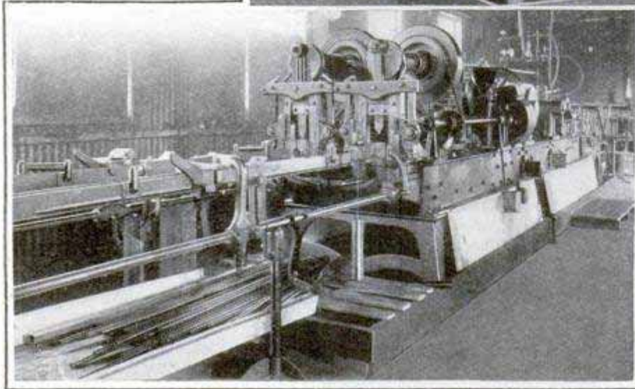
The Other End of the Machine, Where the Finished Tubes are Deposited
