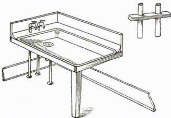
Concrete Filling and Support for a Kitchen Sink That is Sanitary and Bug-Proof
