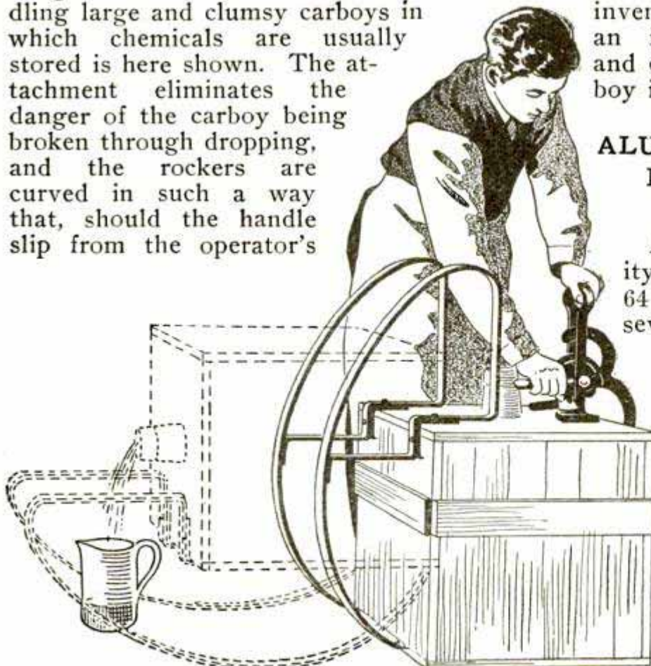
Device for Handling Heavy Carboys with Ease
