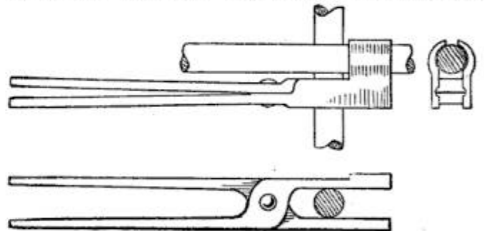
The Jaws' Shape is Such That Either Flat or Round Stock may be Held in Them
