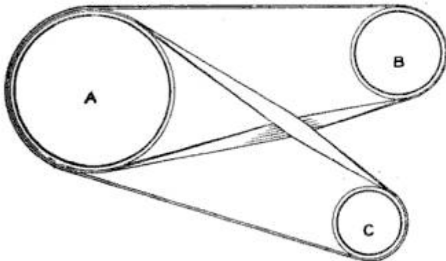
One Belt on One Driver Runs Two Small Pulleys without an Idler between Them
