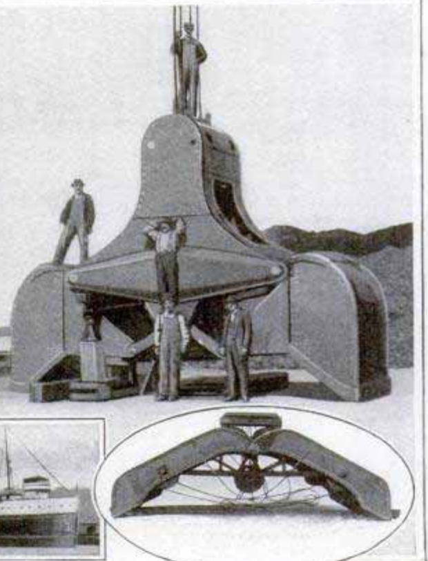
Bucket That Picks Up 12 Tons of Coal at One Time The "Trimmer" Bucket Used for Cleaning the Hold after Bulk of Coal has been Taken Out
