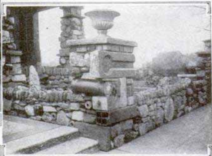
Effect Obtained by the Use of Old Drain Pipes, Paving Blocks, Cobblestones and a Cement Coping
