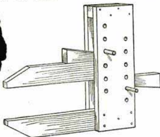
The Clamp is Actuated by Wedges and Pins for the Adjustment to the Width
