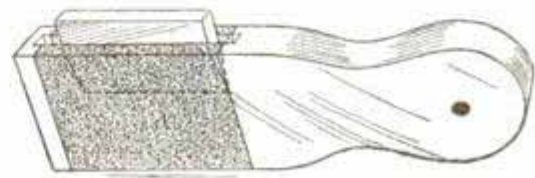
A Wedge Attachment for a Pencil-Sharpener Stick for Changing the Sheets of Abrasive
