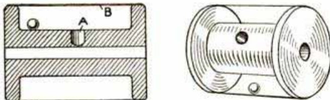
The Steel Ball is Not So Easily Run Into the Hole as It Appears
