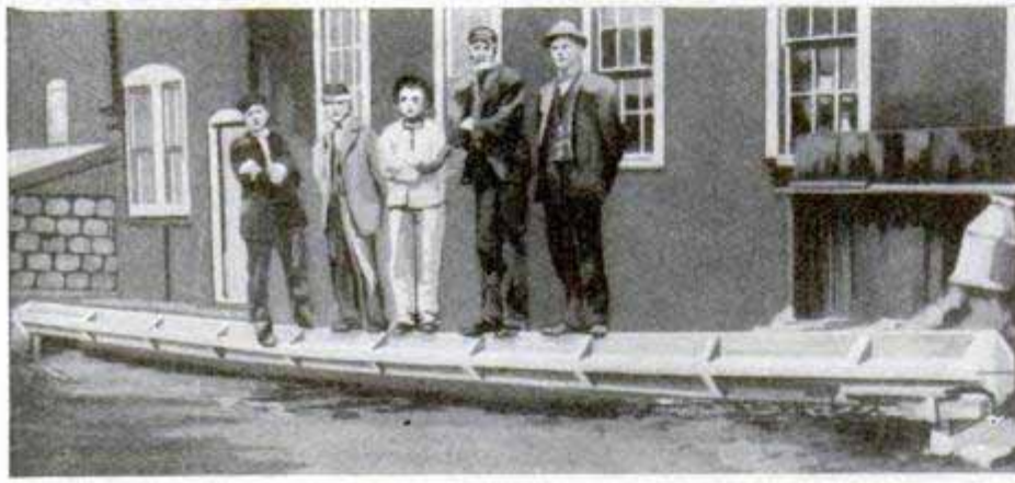
30-Ft. Concrete Trolley Pole of New Design, Supporting a Load of 800 Lb., and Cross Section Showing Reinforcing
