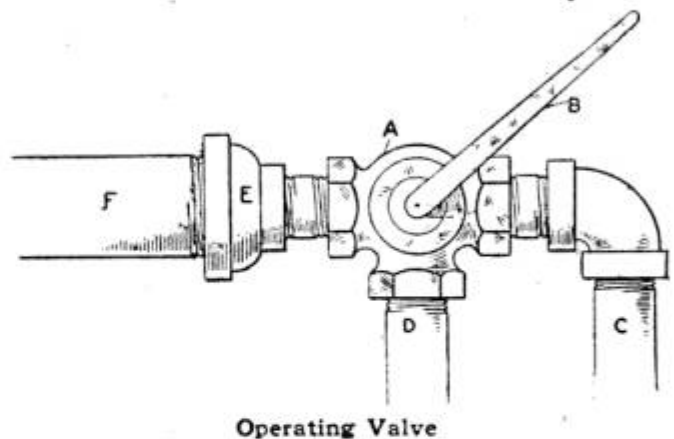
Operating Valve
