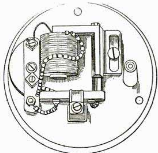
A Device for Limiting the Amount of Current Used
