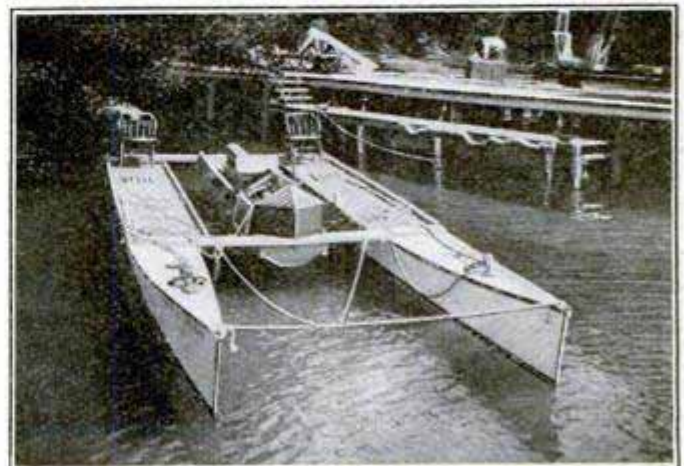
A Motor Catamaran which Acts as a Tender and Launcher for an Aeroplane
