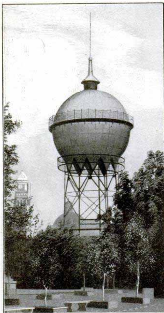
A Spherical Water Tank in Mexico
