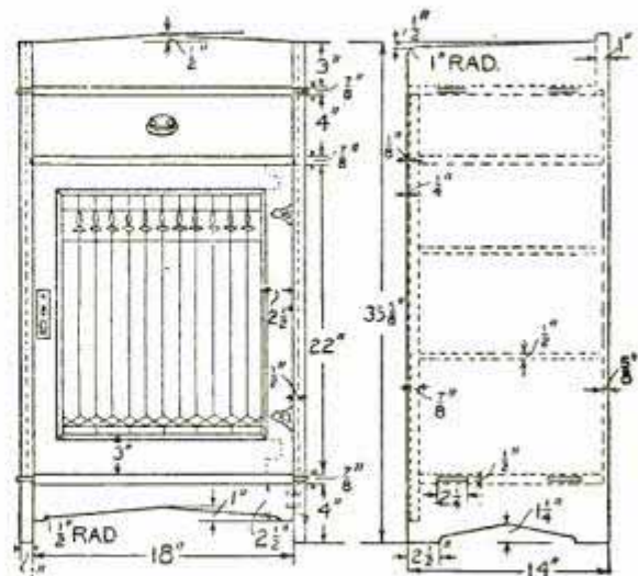
Fig. 112 — Cabinet Details
