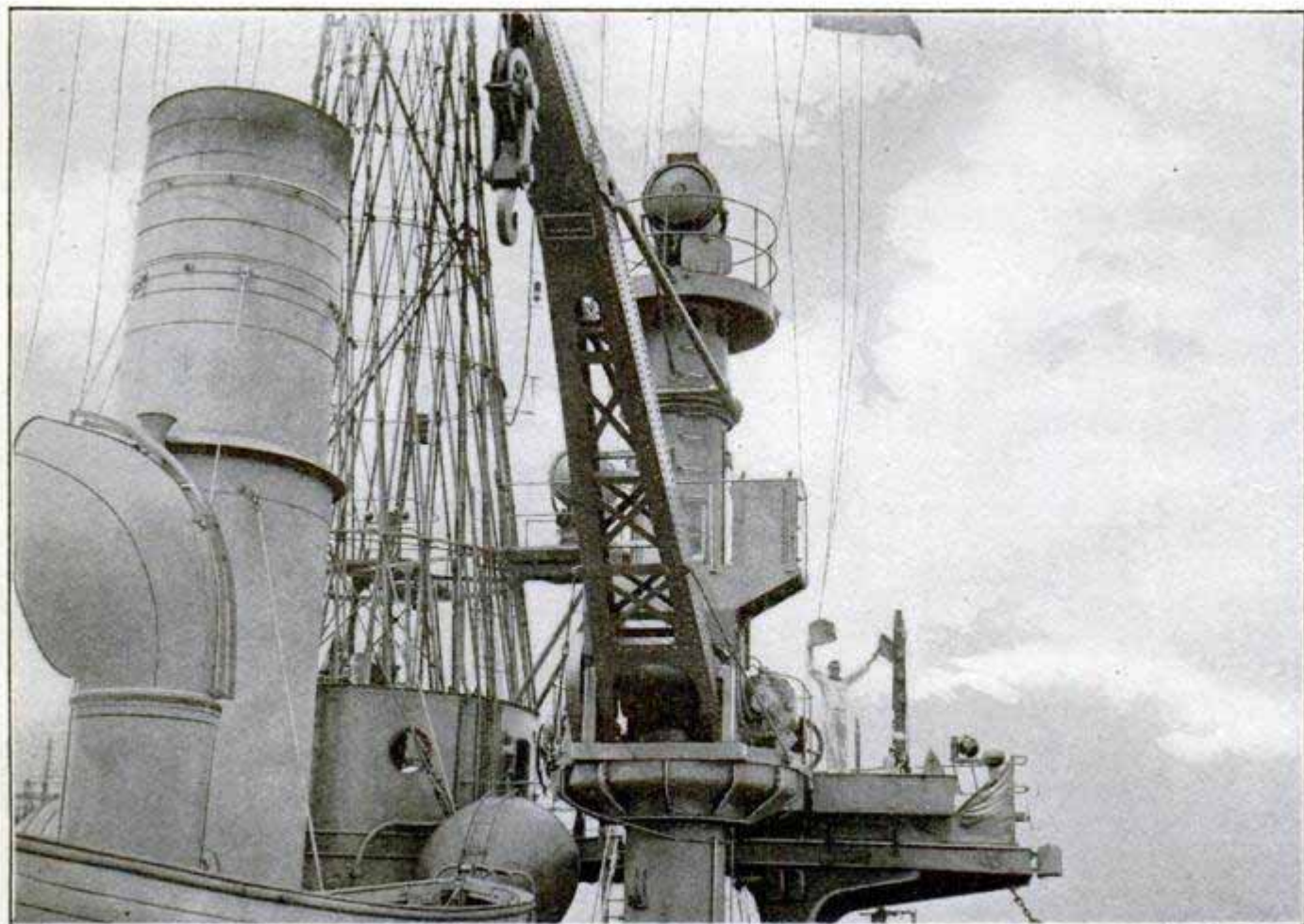
The New Tower on Latest Battleship Which Serves for Crane and for Searchlight
