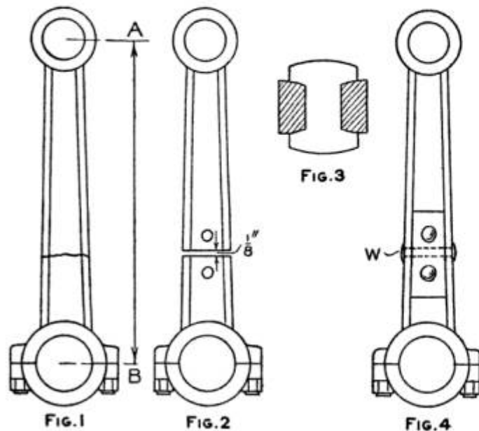
Connecting Broken Parts with Steel Plates
