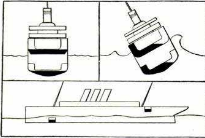
Water in Tanks When Ship is Steady Position of Water When Ship Rolls Location of the Fore and Aft Tanks
