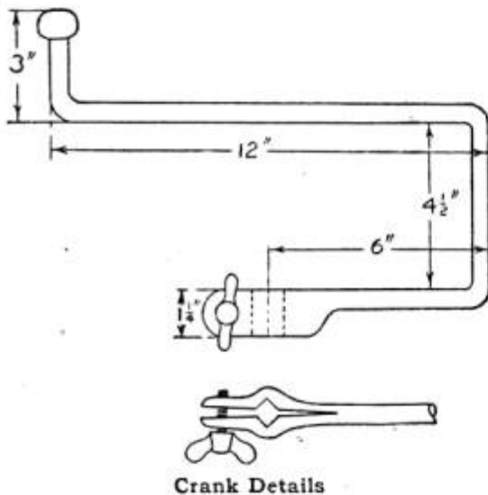
Crank Details
