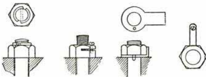
Locking Nuts
