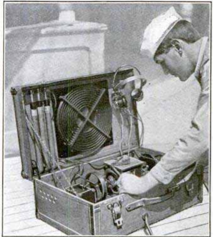
Portable Wireless Set Used in Navy
