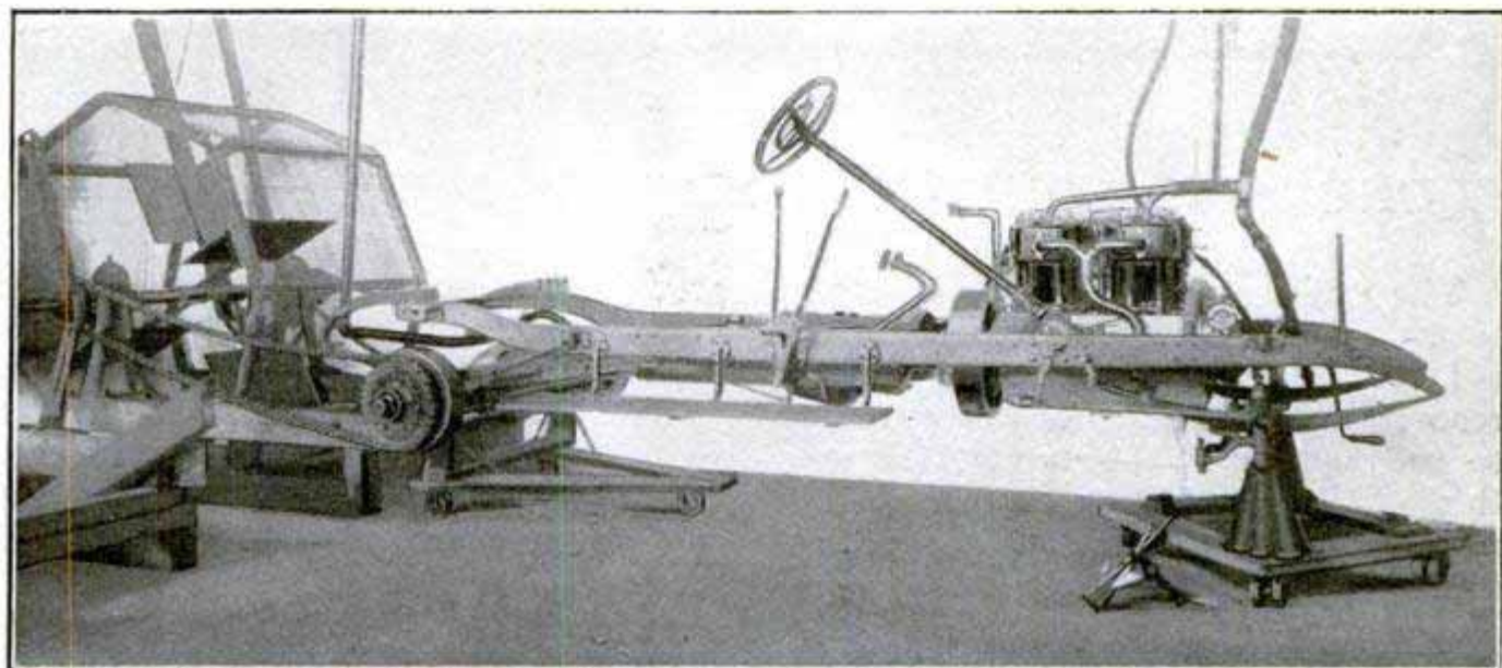
The Resistance of Revolving Fan Takes Place of Road Resistance in Testing Engine
