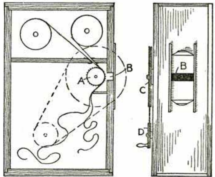
Fig. 7—Printing Machine
