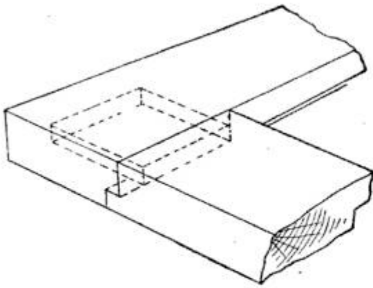
Fig. 116—Shouldered Tenon Joint for Glass Panel
