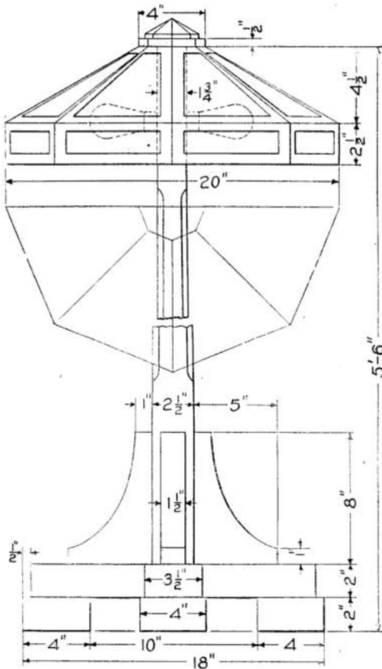
The Standard and Base Details of the Arts-Crafts Piano Lamp, Showing the Finished Shade in Place
