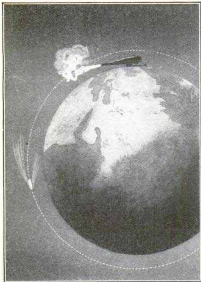
Flammarion Says a Muzzle Velocity of 26,000 Ft. per Second Would be Sufficient to Enable a Projectile to Overcome the Earth's Gravity Enough to Become a Satellite
