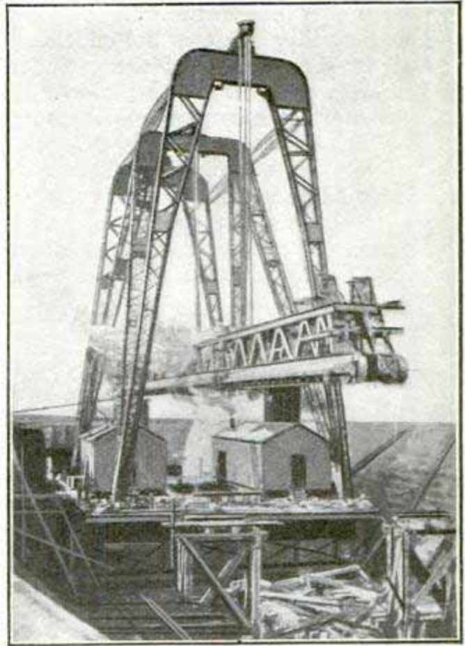
The "Hercules" Raising Her Own 216-Ton Truss into Place
