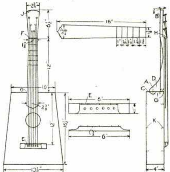
Details of Guitar
