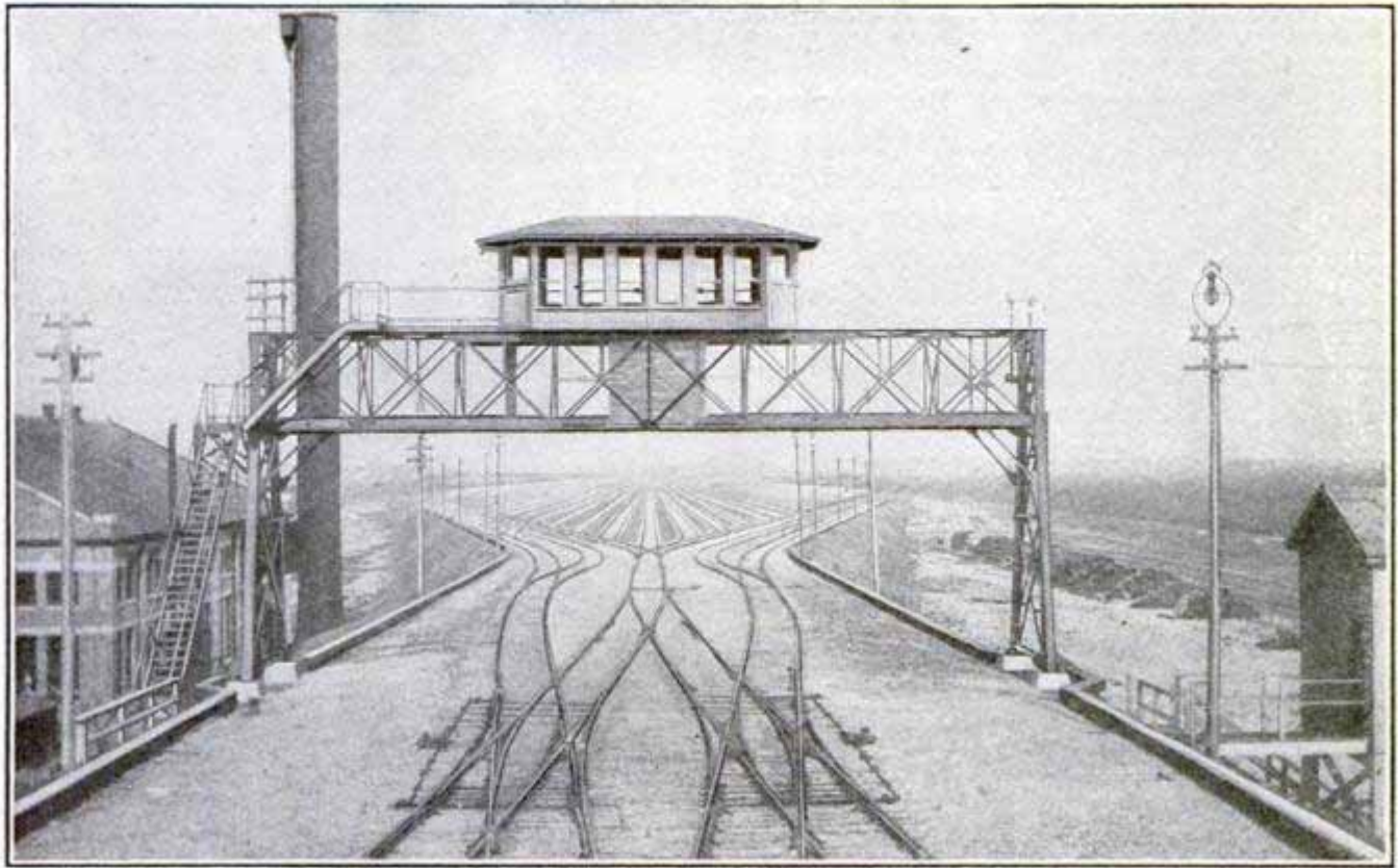
Chicago's Great Freight-Distributing Yard. The "Hump" is Shown in the Middle Foreground, and the Man in the Switch Tower Electrically Controls the Switching of the Cars to Their Proper Tracks
