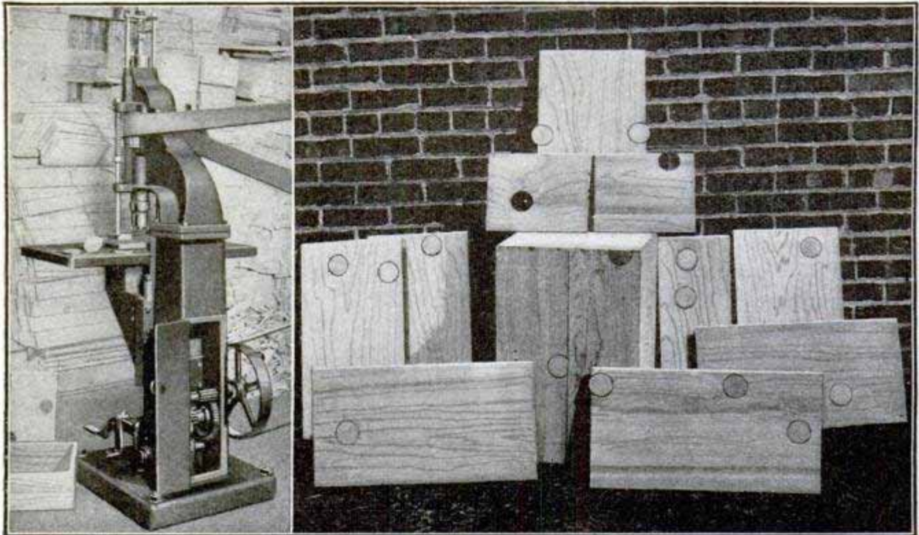
Removal of Knots Gives Packing-Case Boards Greater Strength
