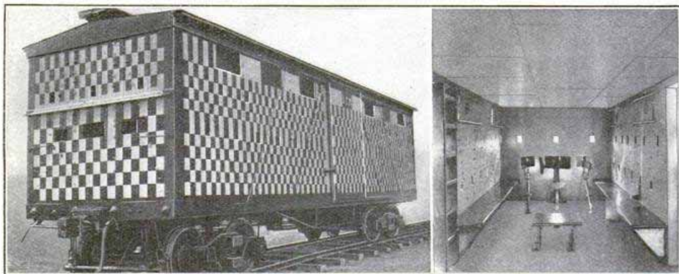
Exterior and Interior Views of Railroad Car Transformed into Moving Fort by Mexicans. Checkerboard Appearance Makes it Difficult for Enemy to Locate Portholes
