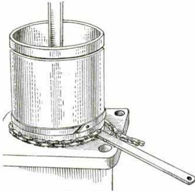
Holding a Ring in Place
