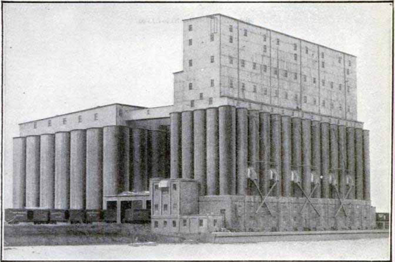
Fort William Reinforced Concrete Grain Elevator. Working House on Right, Storage Bins in Rear
