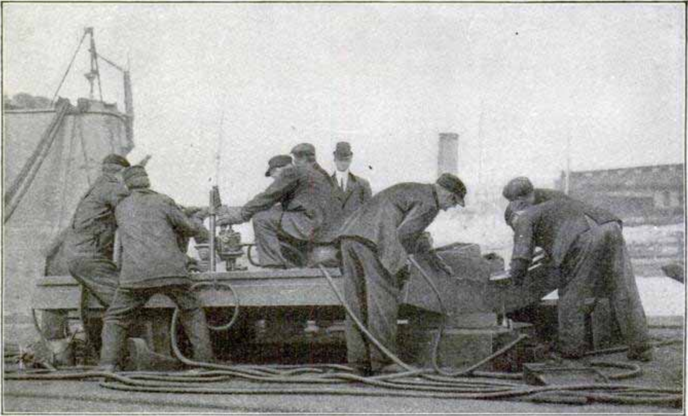
ARMOR PLATE FOR TURRETS
