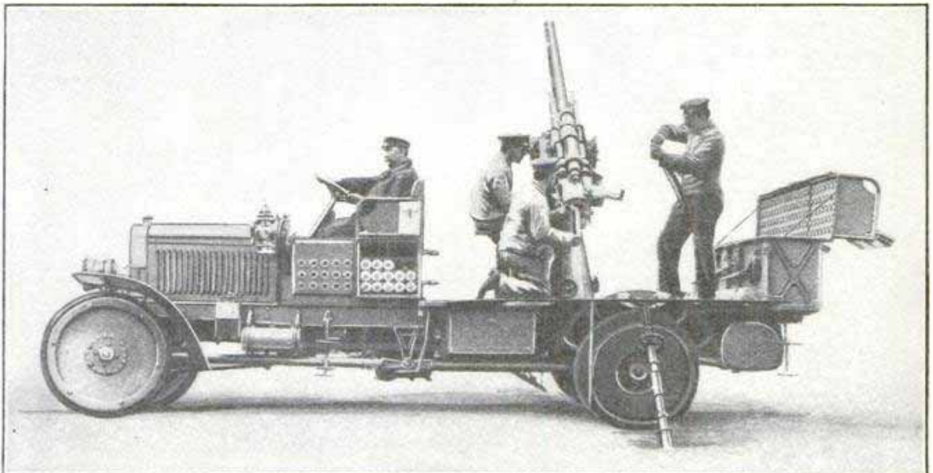
New Gun Designed for the German Army as Protection Against Air Craft
