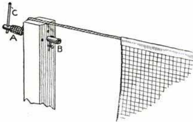
Tightener on Post
