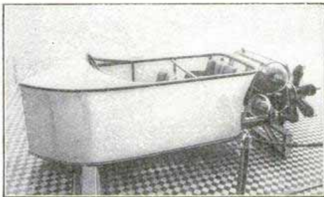
A Three-Seated Biplane Body
