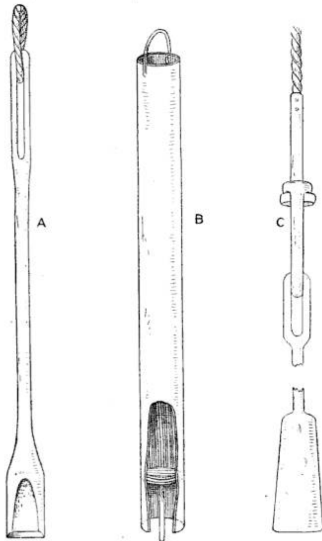
Fig. 1—Drilling Tools
