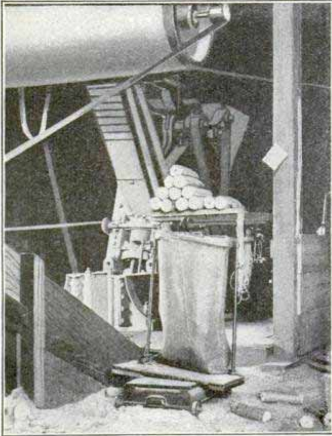
Electrically Driven Machine that Compresses Five Tons of Sawdust Briquettes per Day
