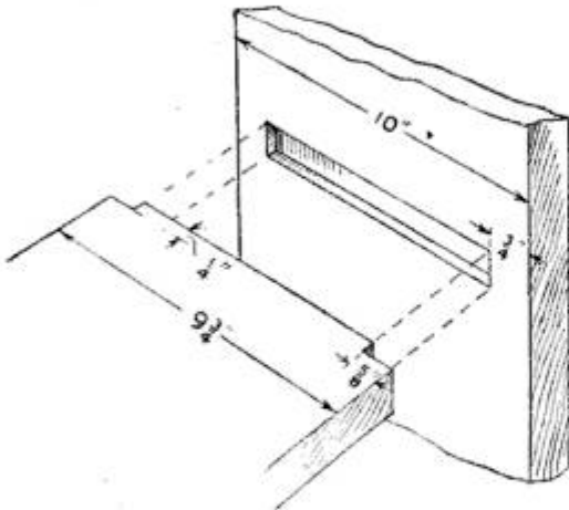
Fig. 95—Shelf Joints
