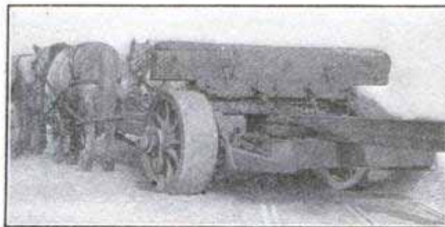
Front of 100-Ton Truck with 14-In. Wheels
