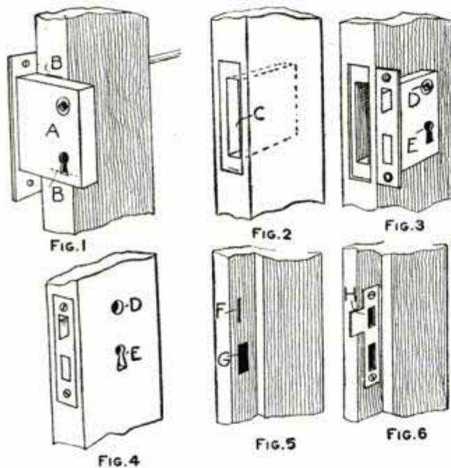
FIG. 4 Different Stages in Lock Fitting
