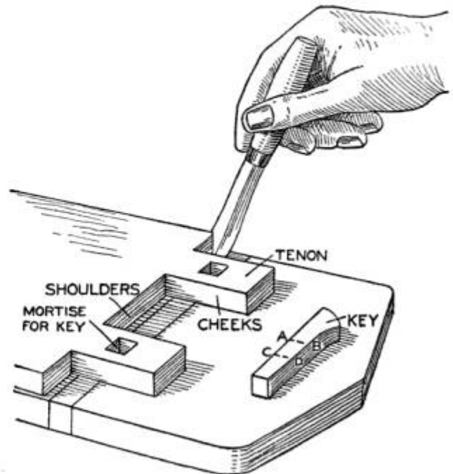
Fig. 98—Marking Mortises
