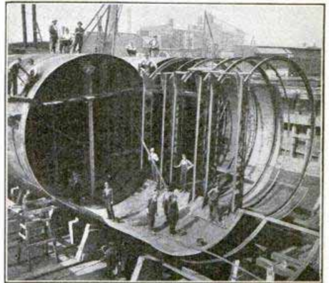
Erecting the Steelwork for the La Salle Street Tunnel, Chicago
