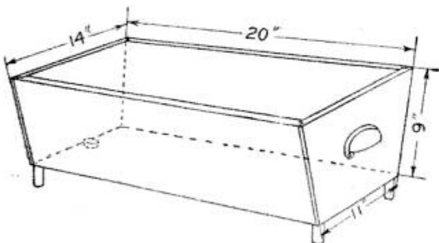
Sink Washtub
