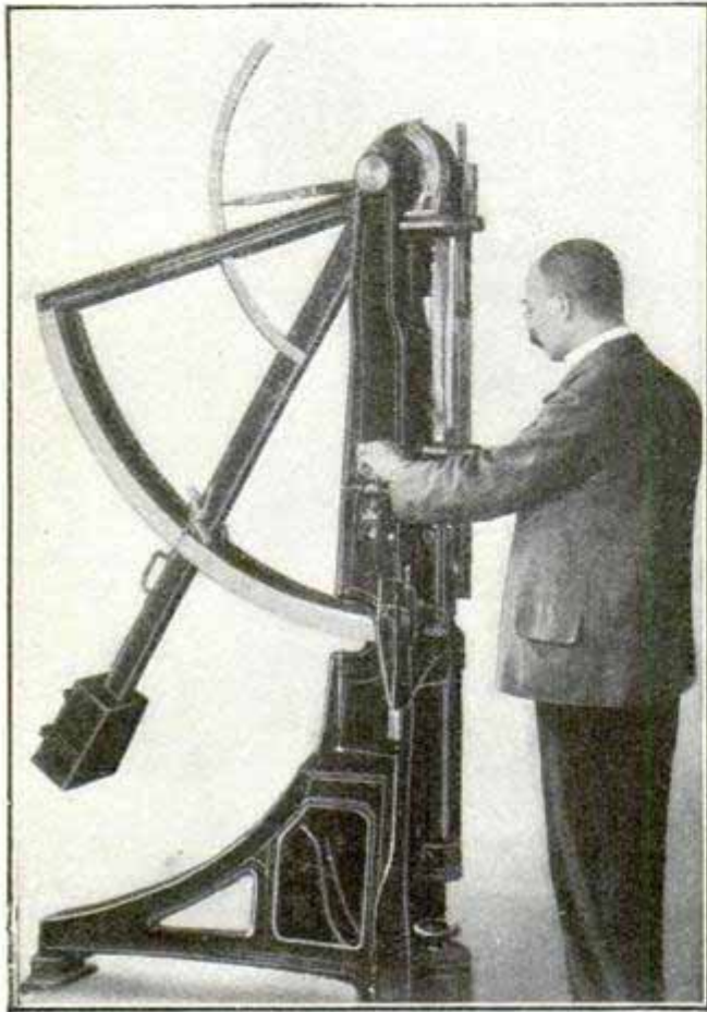
Testing a Strip of Sail Cloth in a Machine Built Especially for the Purpose
