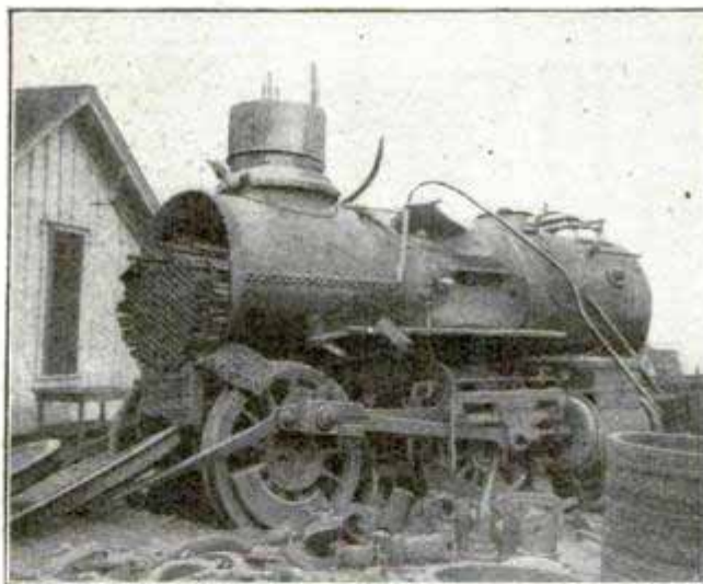
Near View of the Locomotive Which Exploded and Was Blown 75 Ft. The Drivers Were Stripped from the Axles But Held by the Side Rods
