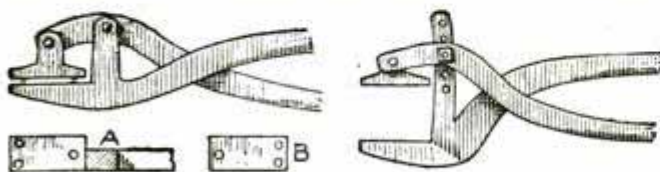
Three-Point Contact on Jaws
