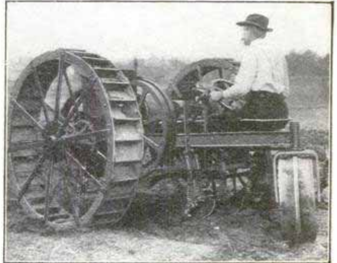
Gasoline Traction Cultivator Making a Turn
