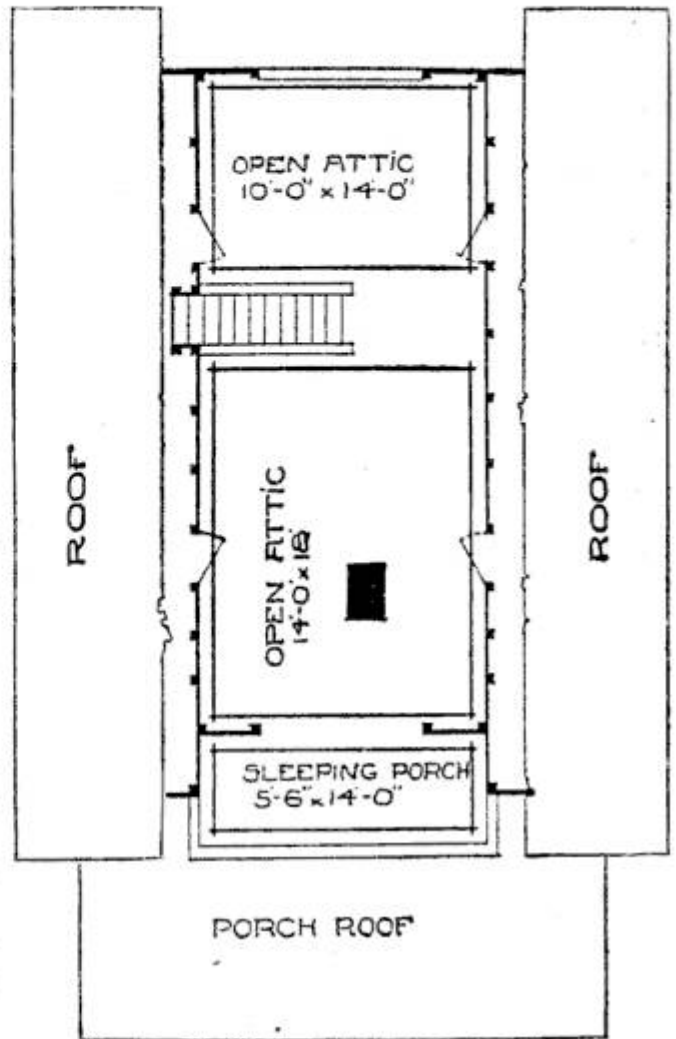
Second-Floor Plan
