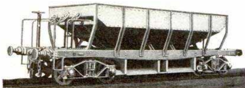
Self-Discharging Ballast Car Especially Designed for Railroad System in the Argentine Republic
