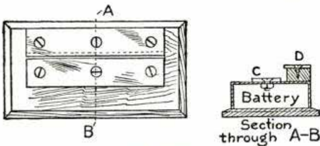
Lamp Tester
