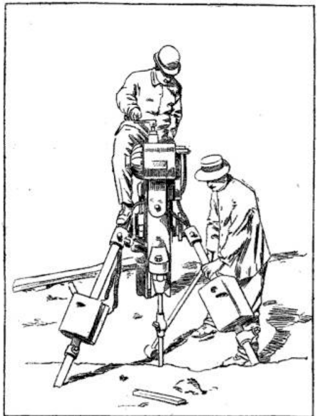
A Compressed-Air Cushion Transmits Energy from Motor to Plunger in this Rock Drill
