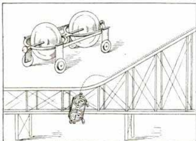
Model with Two Gyroscopes, Which When Revolved in Same Direction, and Run Down Incline, Acted as Aeroplanes Do Under Same Conditions. The Model Turns to the Left and Leaves the Track
