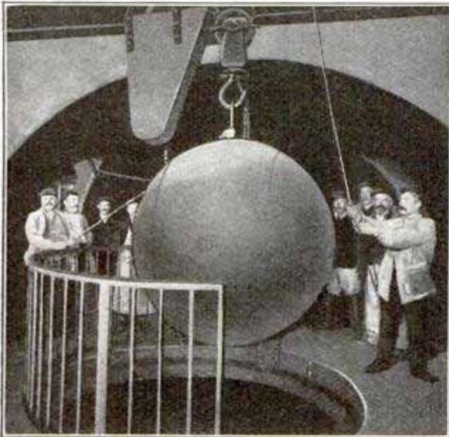
Lowering the Huge Wooden Ball into One of the Sewers of Paris
