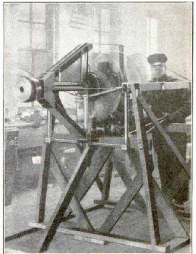
Motor in Operation, Revolving Propeller at the Rate of 1200 R.P.M.
