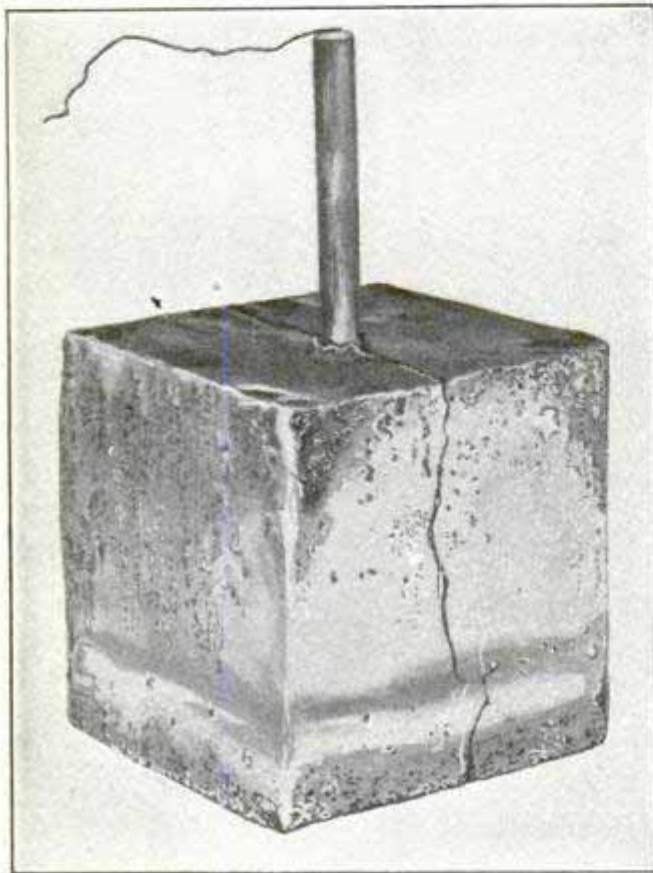
Test Block with Iron Rod Imbedded, Showing Size of Crack after Two Weeks' Exposure to Electric Current
