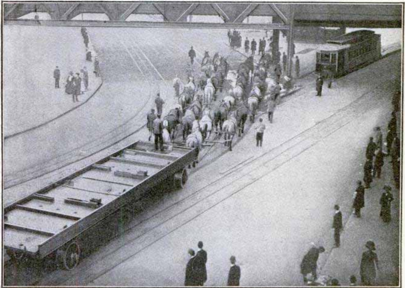
62-Ton Girder Passing Under Brooklyn Bridge Structure
