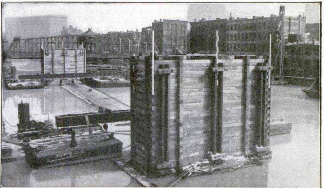
The Tunnel Lying Afloat and Nearly Submerged in the Chicago River, at Right Angles to Its Site. The Upstanding End Portions Are Caissons for Use in Joining Tunnel to Its Approaches
