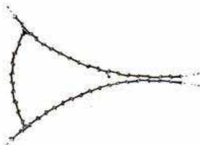
How Separate Steel Piles Are Connected to Form Strengthening Arcs
