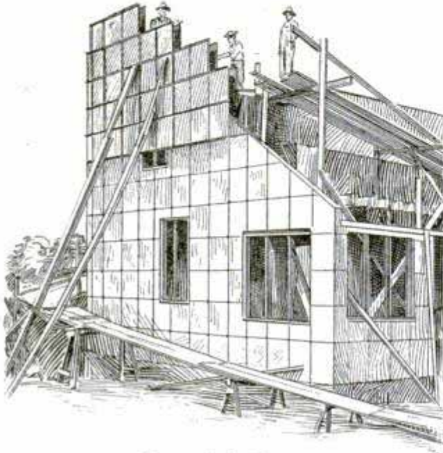
Forms in Position
