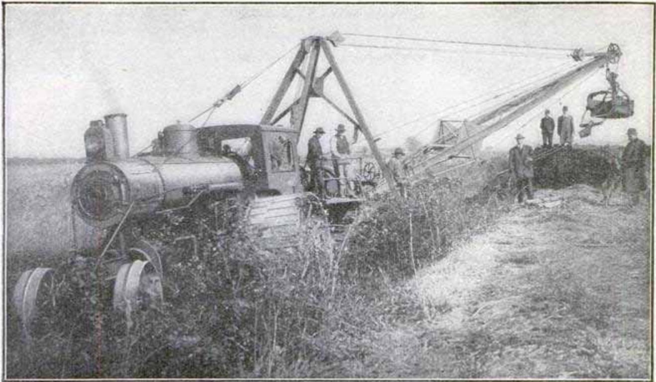
A Steam Shovel and Traction Engine Arrangement That Will Go Almost Any Place
