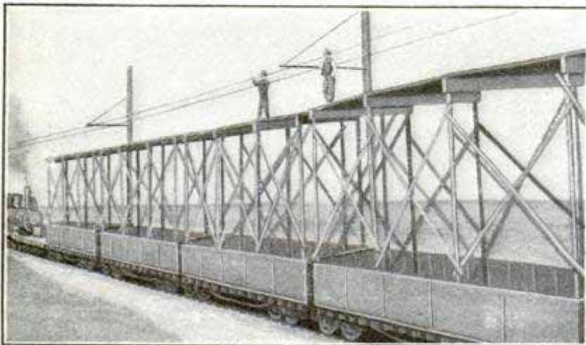
Construction Train for Overhead Construction on Electric Railroad
