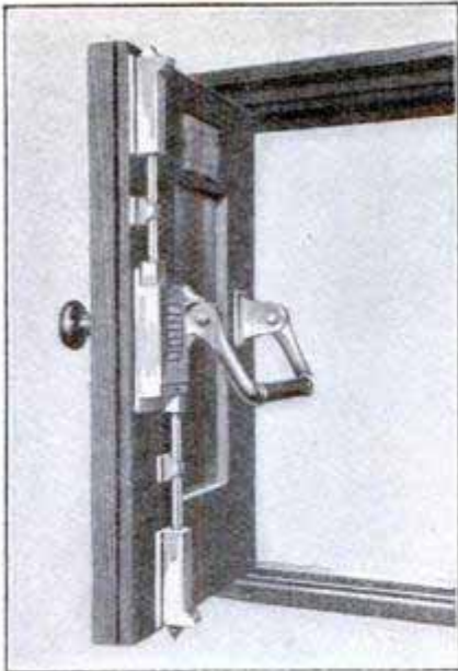
Model of unlocking device for emergency exit doors of theaters and other public places where fire may make rapid exit necessary. On pressing the bar, the door is instantly unlocked.
