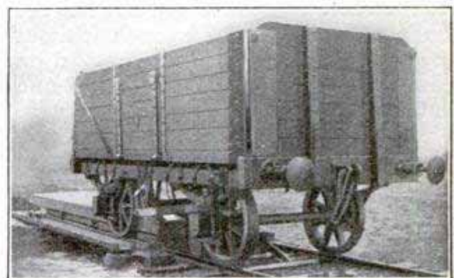
Running English Broad-Gauge Freight Car onto Narrow-Gauge Transporter
