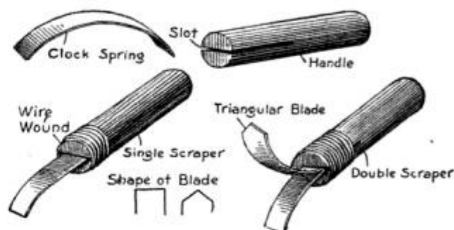
Parts of the Scrapers
