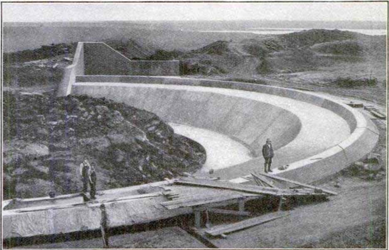
Spillway at Head of Waste Channel, North End of Belle Fourche Dam
