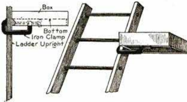
Sign Painters' Ladder Bracket
