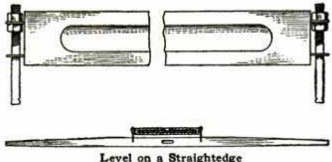
Level on a Straightedge
