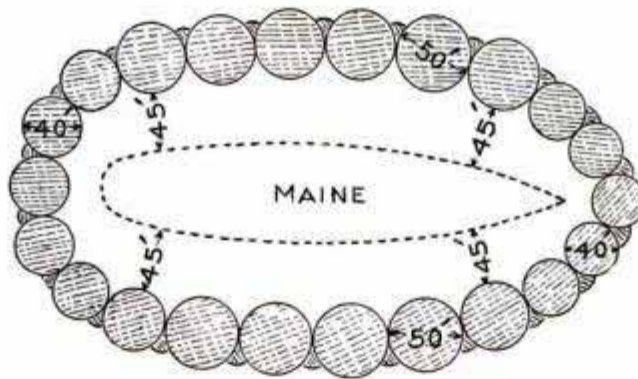
Plan of Cofferdam Being Built Around the Sunken Ship
