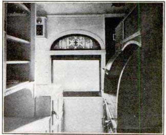
Kitchen Built in Private Trolley Car Showing Range, Refrigerator and Shelves for Dishes
