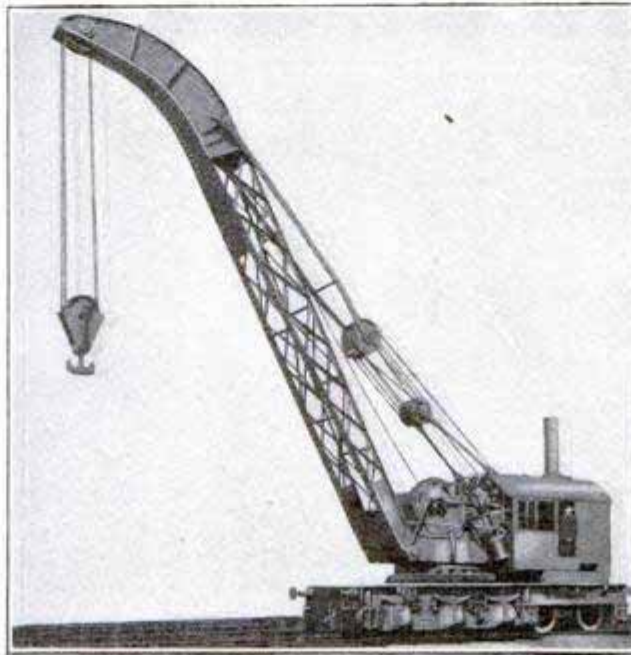
Crane in Operating Position
