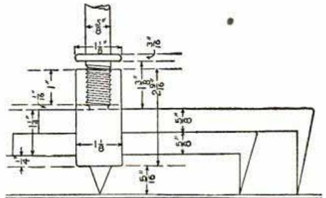
Details of Gasket Cutter
