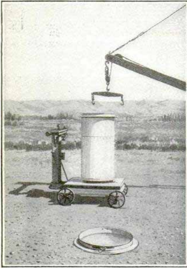
Tank Used in Determining Effect of Mulch in Preventing Evaporation
