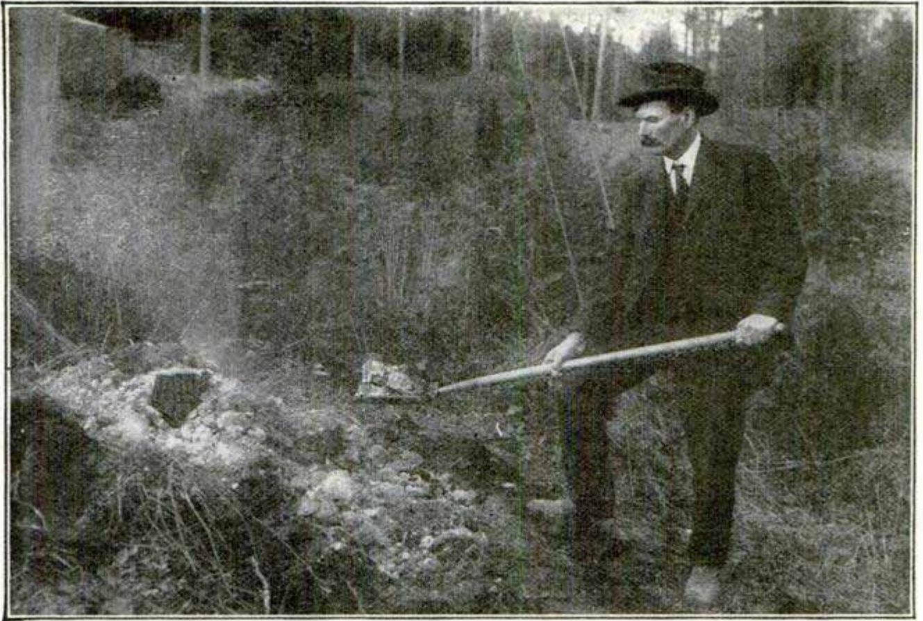
Showing How Soil is Burned to Charcoal by Char-Pit Process
