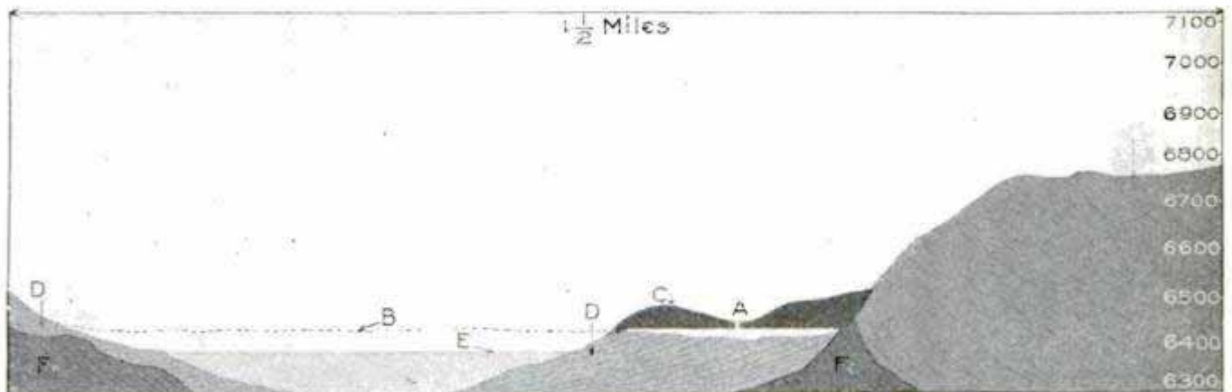
Diagram Showing Occurrence and Origin of Salt at Crow Creek, Near Montpelier, Idaho, at Different Heights above Sea Level, as Shown on Right
