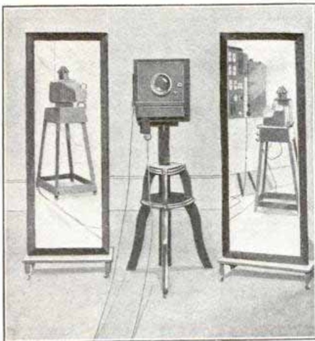
Photosculpture Apparatus—Camera in Center with Projection-Lantern Reflected in the Mirrors
