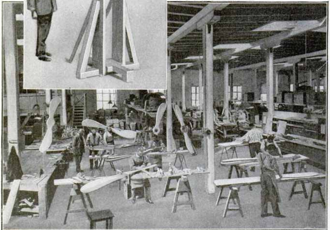
Testing the Balance of a Finished Propeller
