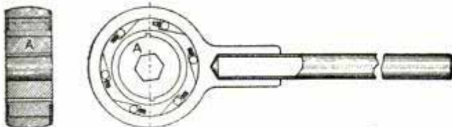
Roller Pawl Ratchet Wrench
