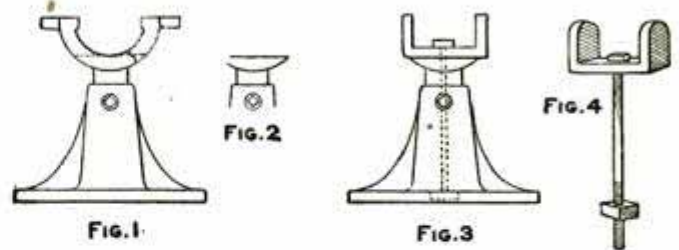
Wrought Iron Ears on Hanger
