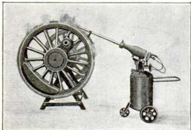
Crude-Oil Tire Heater in Operation
