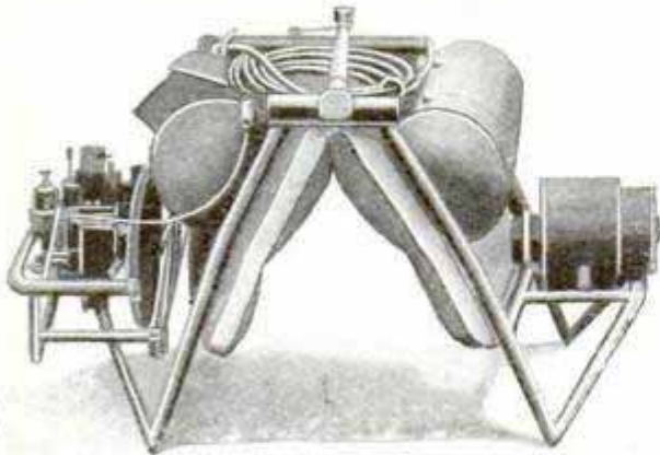
Portable Wireless Field Set as It Is Placed on the Pack Saddle
