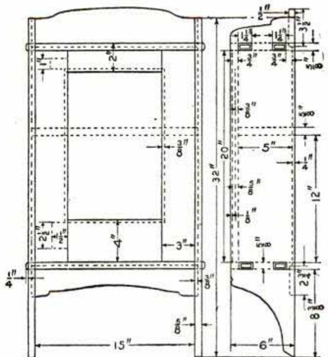
Wall Case Details
