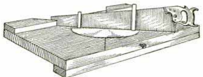
Saw in Guides
