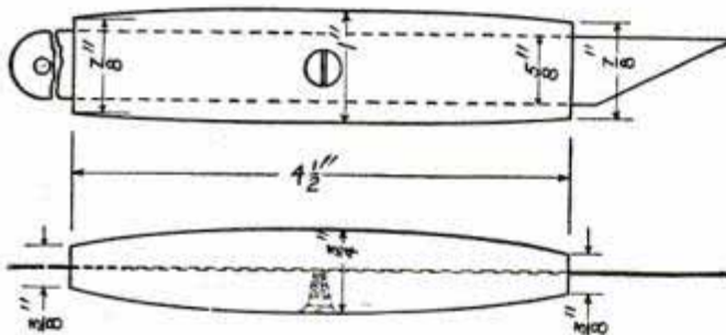
Details of Handle
