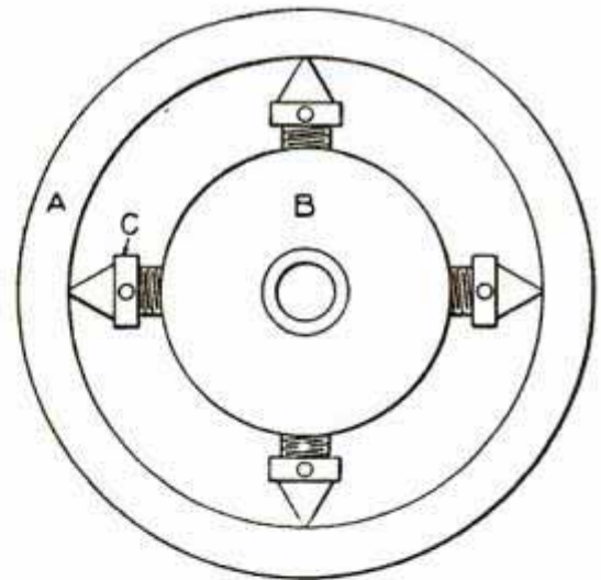
Hub with Center in Casting
