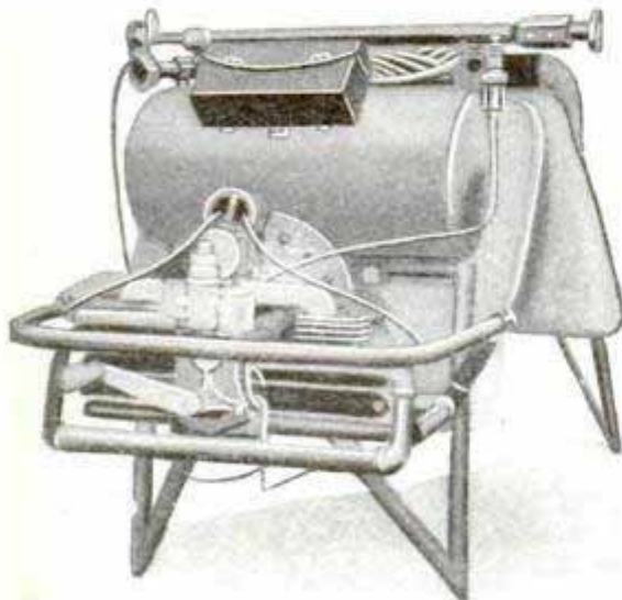
Another View of Portable Wireless Field Set, Showing Arrangement of Engine
