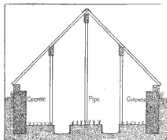
End View of Greenhouse
