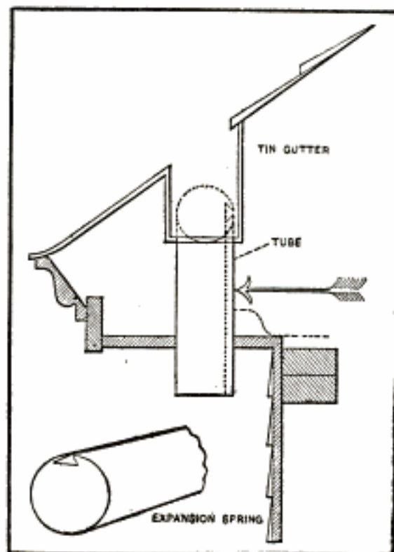
Expansion Leader Tube
