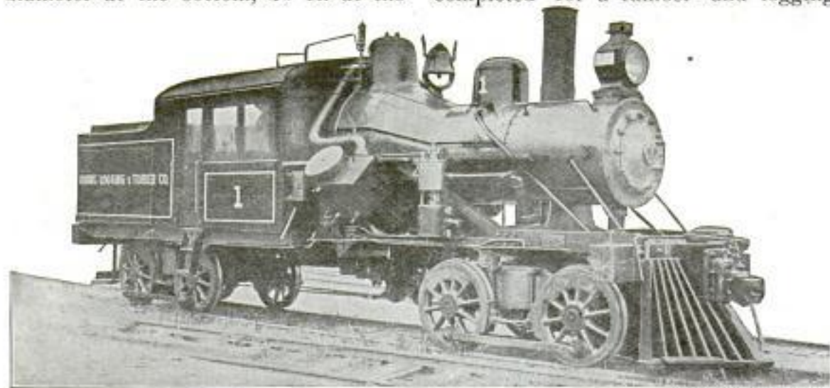
Logging Locomotive That Burns Oil
