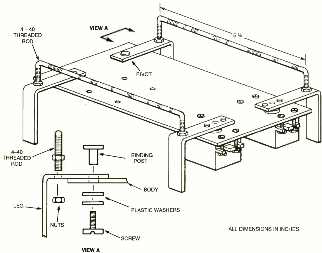
Fig. 7. The linkage system consists of two threaded rods that connect the front and rear legs, which permits synchronous movement.
