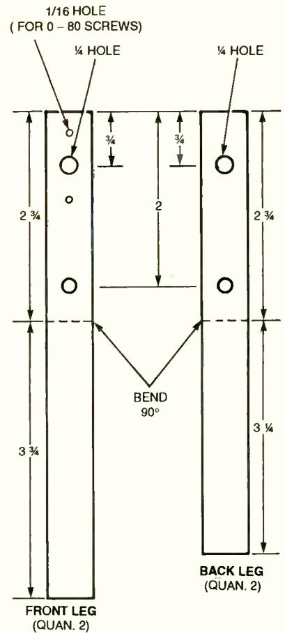
Fig. 4. Here are the guides for constructing the front and rear legs of the robot.
