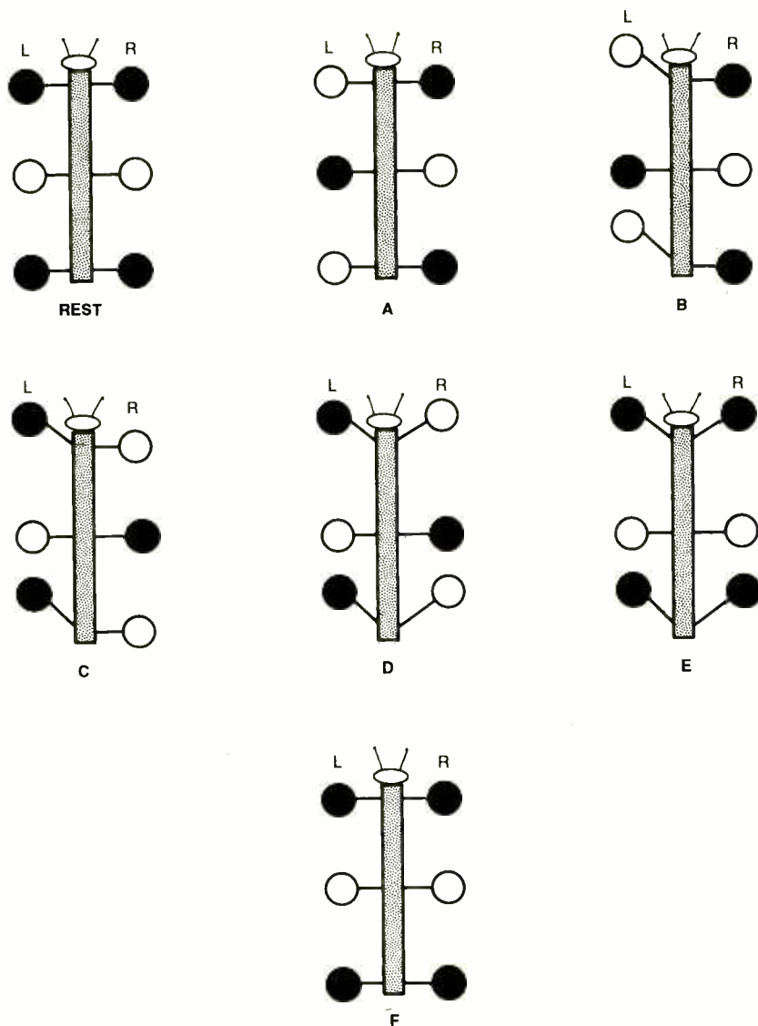
Fig. 2. Here is the walking pattern of a hexapod powered by three servos. Notice that, at rest, the center legs do not support any weight.
