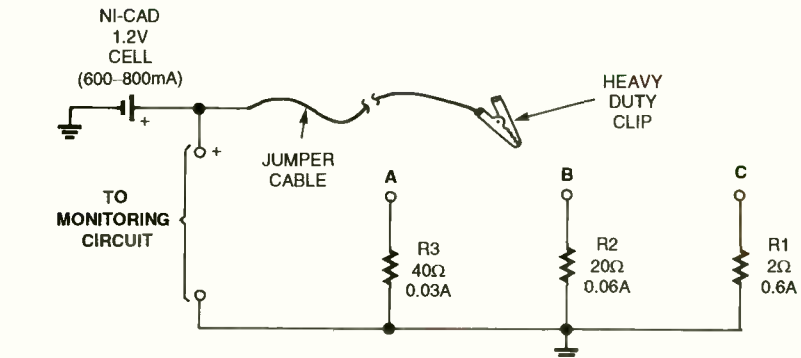
Fig. 1. This is a simple circuit for monitoring and testing the capacity of NiCad AA cells. The only components needed are inexpensive resistors.
