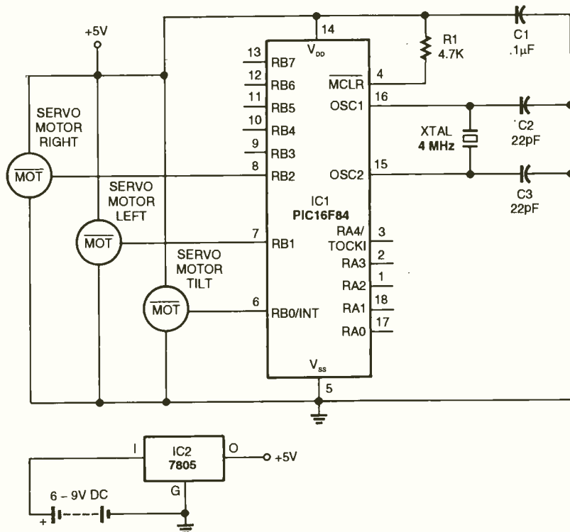
Fig. 8. At the heart of this hexapod lies a PIC16F84 with an external 4-MHz crystal linked to the oscillator pin-outs, 16 and 15.
