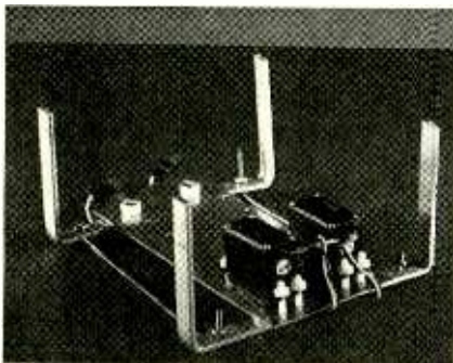
No, it's not dead...it's resting. Here you can see the underbelly of the hexapod with two servos in place.
