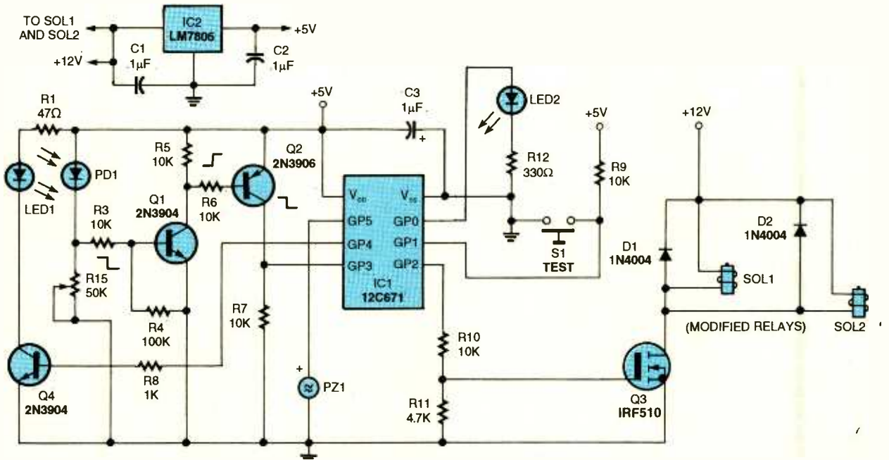
Fig. 4. The schematic above shows the circuit for the Electronic Mouse Trap. The circuit is controlled by a PIC12C671 microcontroller. Note the locations of LED1 and PD1. When an object blocks LED1's light from hitting PD1, the solenoids activate and release the doors.
