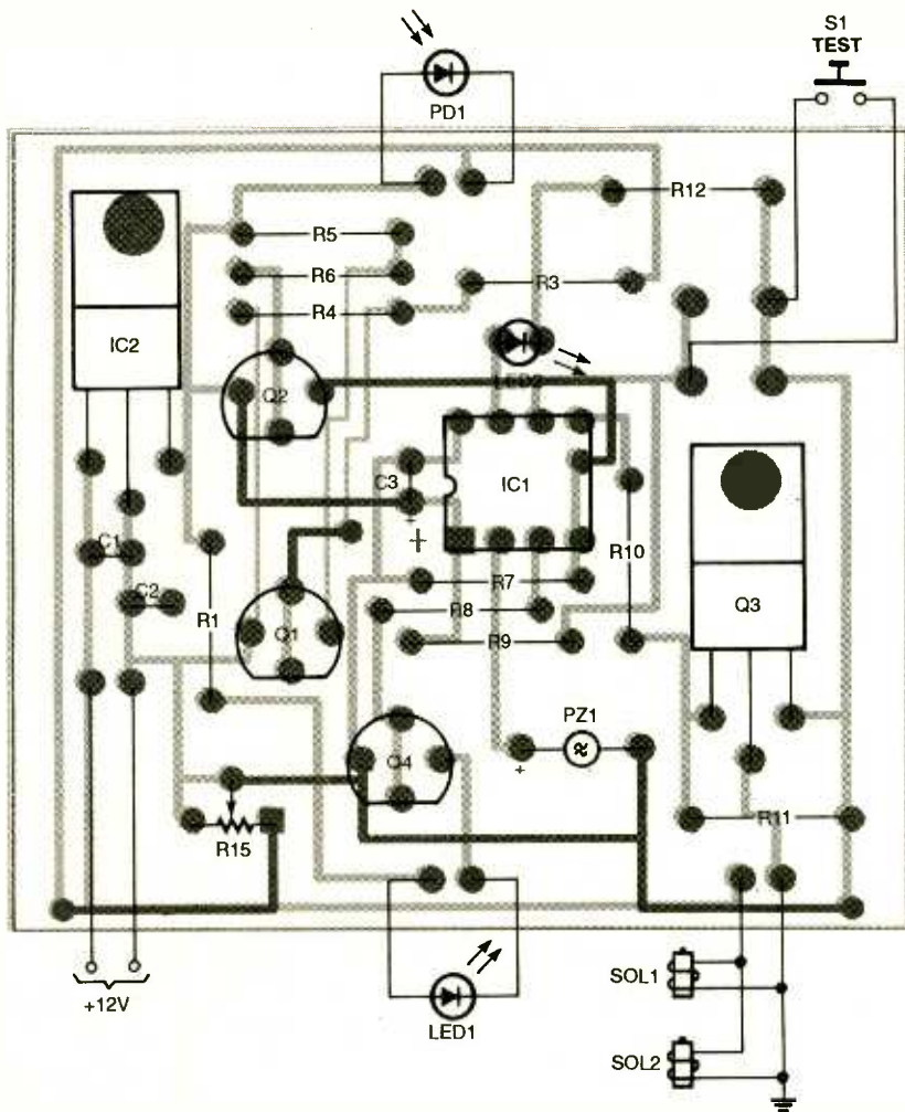
Fig. 6. Use the parts placement diagram above as a reference for constructing the Electronic Mouse Trap. Make sure to observe capacitor polarity.
