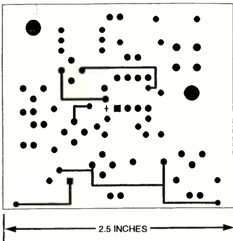
Fig. 7. This foil pattern represents the component-side copper trace.
