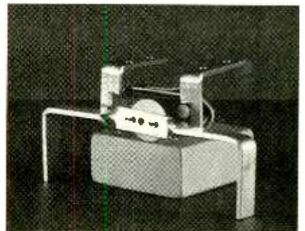
The center servo is shown here ready to be attached to the body. The center legs and the two L-brackets have been attached to the servo.
