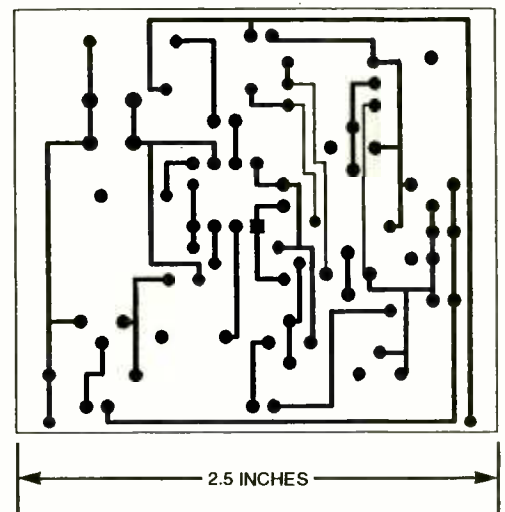
Fig. 8. Here is the solder-side foil pattern for the main PCB module.
