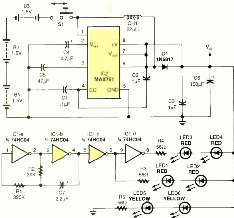
Fig. 1. Once again we bring you the schematic for the Pumpkin Safety Light. Note the changes to IC1-d and the connection of CH1.
