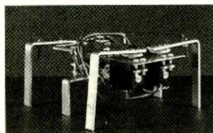
The hexapod is ready for action. Two threaded rods provide linkage for the synchronous movement of the rear and front legs.
