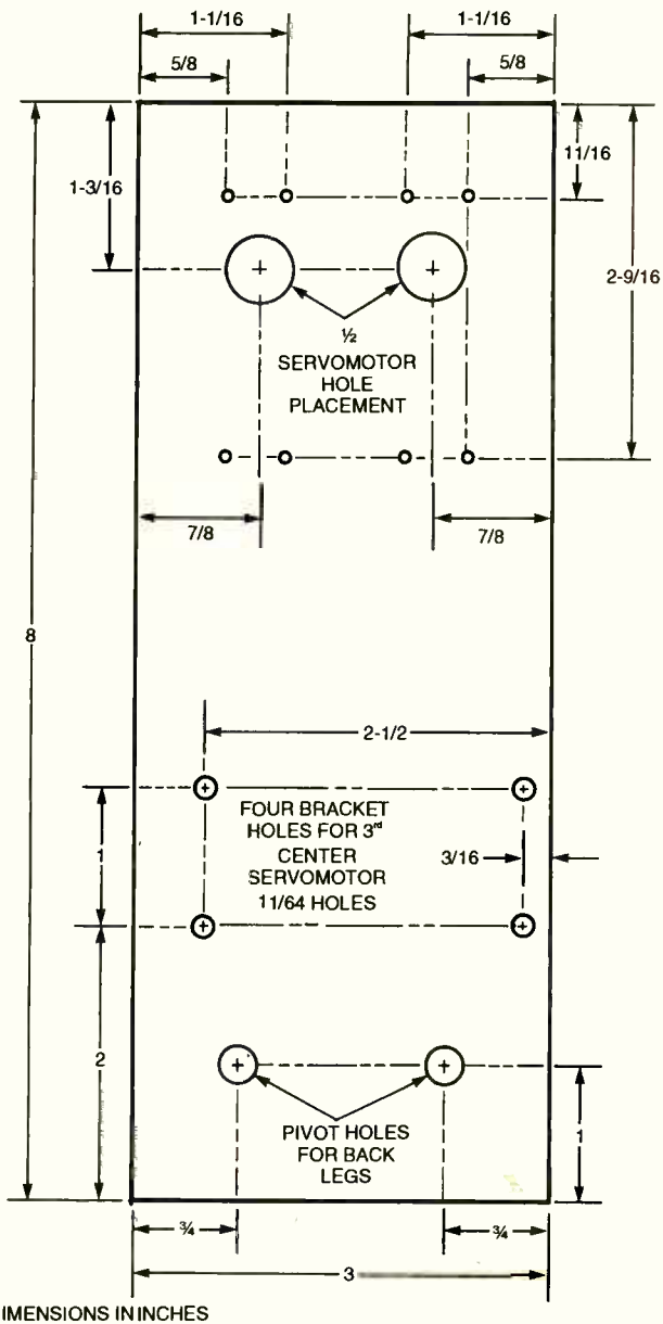
Fig. 3. The above figure can be used as a template for constructing the hexapod's body.
