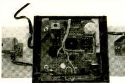
Here is a close-up view of the circuit used in the author's prototype. The voltage regulator is seen in the upper left corner, while the piezo tweeter is nearly dead center, and to its right is the PIC microcontroller that is mounted in a socket. Notice that the two servos can be seen to either side of the control box.
