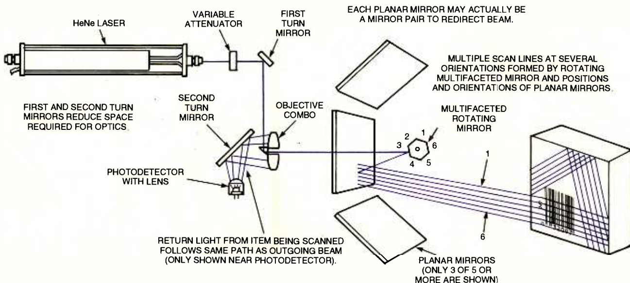
Fig. 1. Here is a diagram that shows the optical path of a typical barcode-scanner. The HeNe lasers used can often be found via wholesale and liquidation companies.
