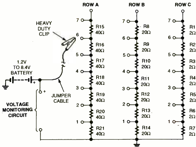
Fig. 2. The schematic above shows a battery tester capable of testing up to seven stacked NiCads. The load is adjustable for 30 mA, 60 mA, and 600 mA.
