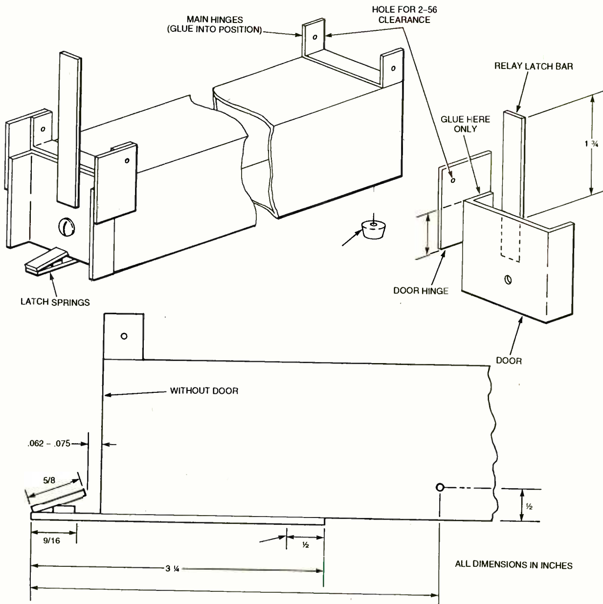
Fig 2. This figure shows how all the pieces fit together, as well as the various points where glue is needed. Be sure to follow all directions and heed all warnings related to the glue.
