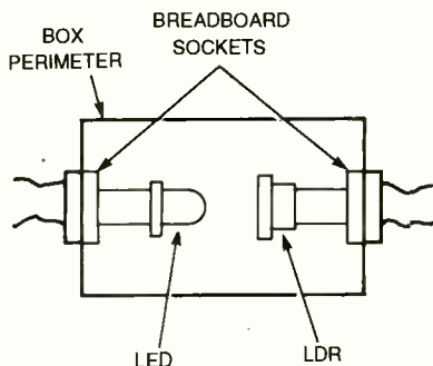
Fig. 2. This drawing shows how the solderless breadboard connectors are located on opposing sides of a light-tight box.
