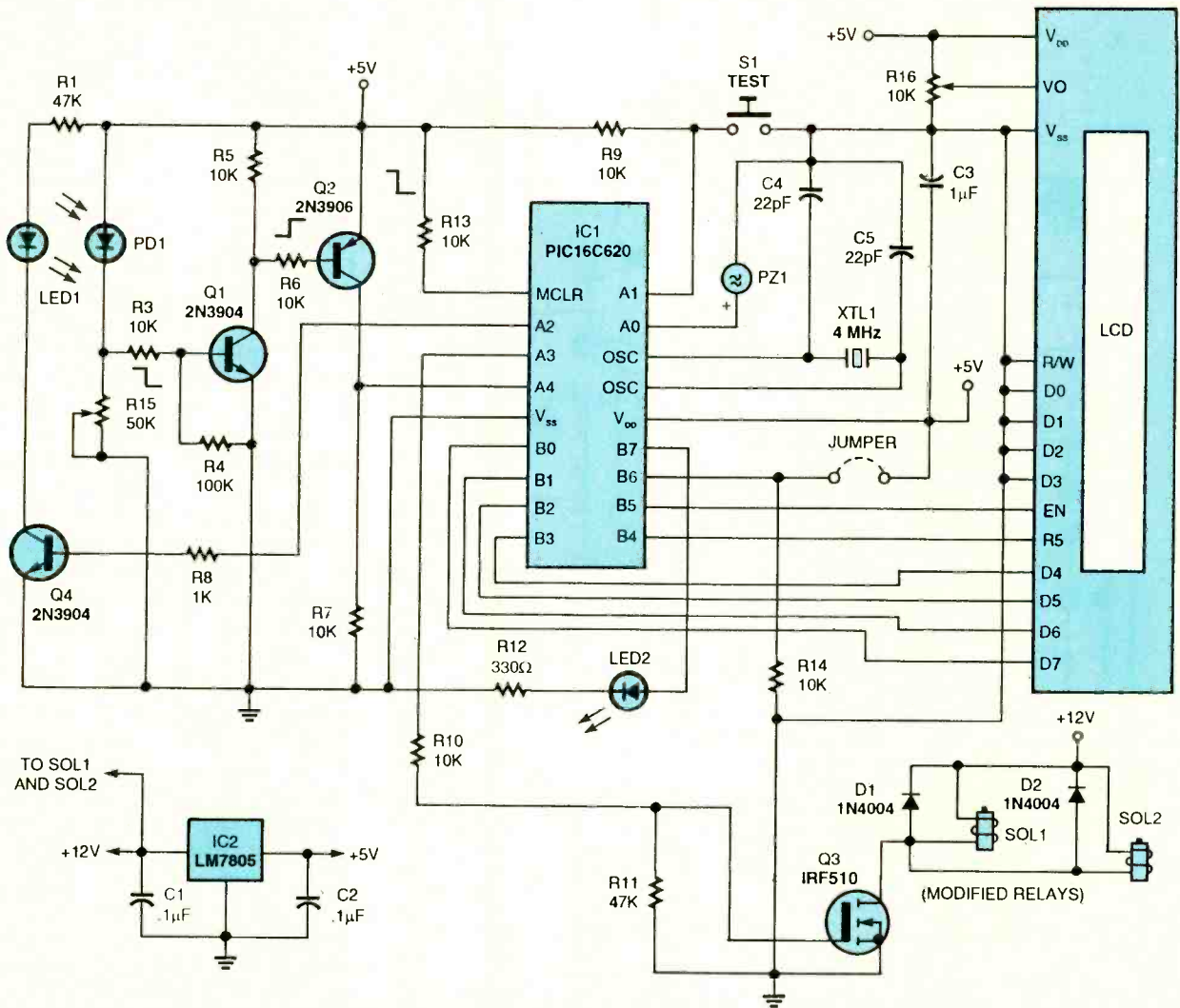
Fig. 5. This is the schematic for the upgraded Electronic Mouse Trap (MTRAP18). The modified version employs a PIC16C620 with a crystal oscillator. Another addition is an LCD display that gives a visual indicator of the trap's performance.
