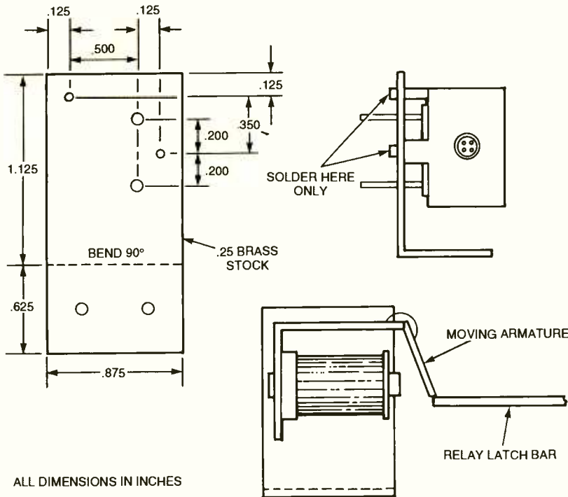
Fig. 3. Solenoids provide the control for the spring-loaded doors. This figure shows how to properly mount the two solenoids required.
