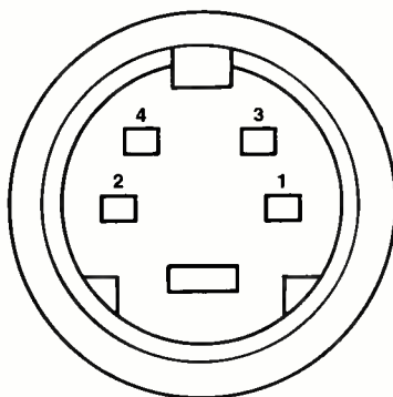
Fig. 1. The S-Video plug as viewed from the "solder tab" end, illustrating the pin locations as described in the text, is a 4-pin "mini-DIN" type of connector.
