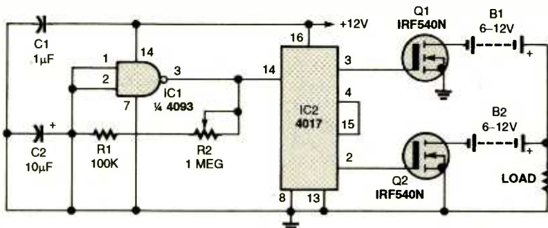
Fig. 3. Two batteries can be life tested at the same time with the circuit shown above. A NAND Schmitt trigger is at the heart of a square-wave circuit that controls the tester.
