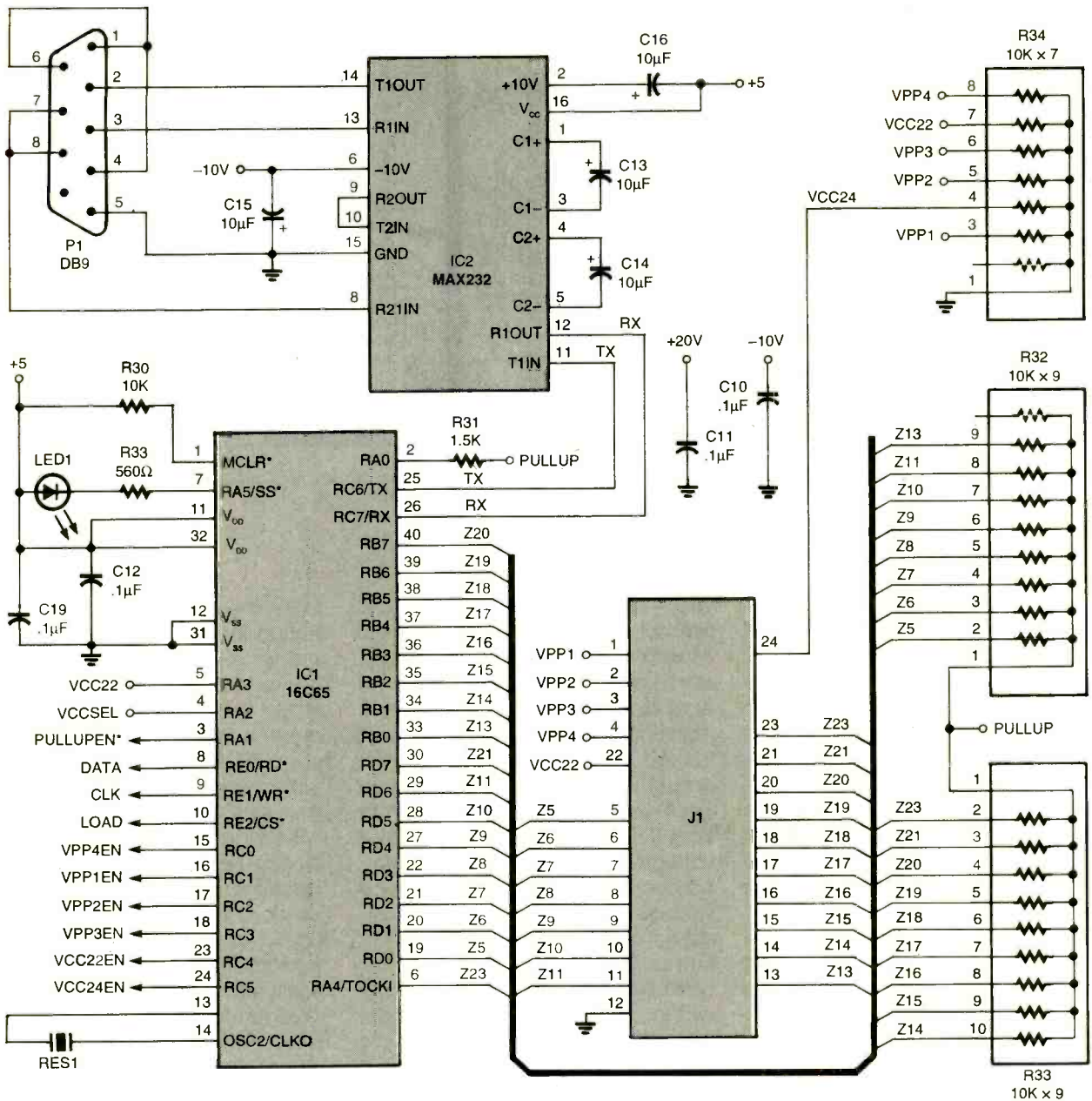
Fig. 2. The on-board PIC microcontroller takes commands from a host PC and manipulates the signals going to a ZIF socket holding the PLD being programmed.
