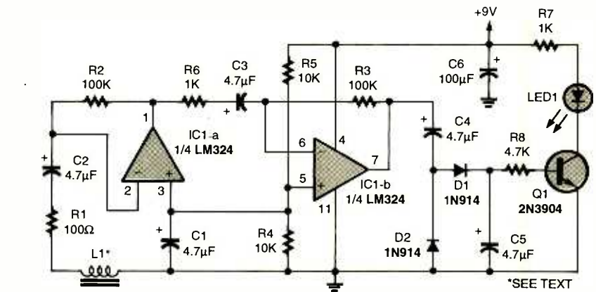
Fig. 7. Any large piece of iron passing near L1 will distort the Earth's magnetic field, creating a weak signal that's amplified by IC1.
