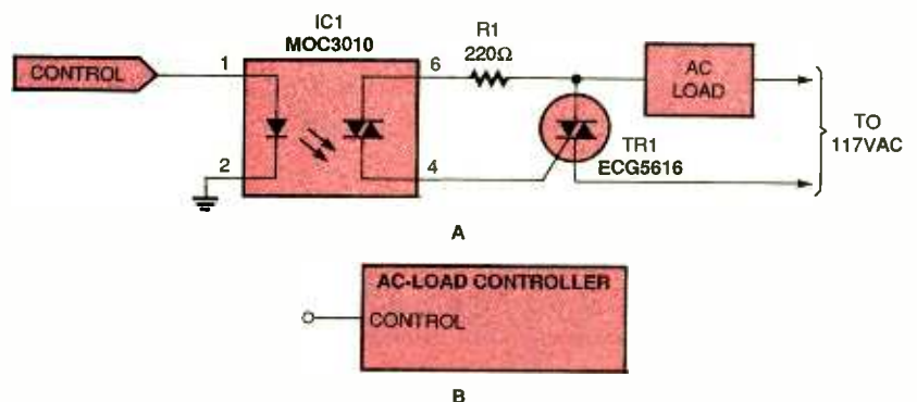
Fig. 2. This opto-coupler-based circuit (A) can be turned into a single AC-load controller block (B).
