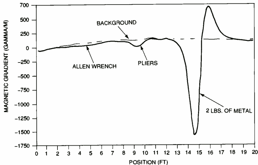
Fig. 2. Extremely sensitive magnetometers can distinguish between various size and mass. Here's a charted magnetic gradient from a sensor that was exposed to a small, stainless-steel allen hex wrench; a heavy pair of carbon-steel pliers; and two pounds of carbon steel used to simulate the size and mass of a large handgun. They were all hidden on a person.
