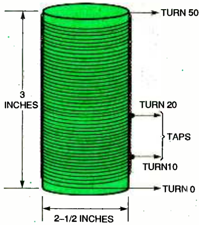
Fig. 3. This 50-turn coil, which is used in the receivers in this month's column, has taps at the 10th and 20th turns.
