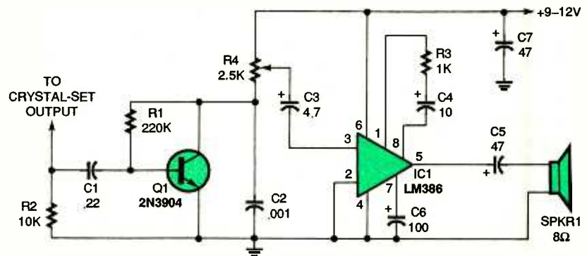
Fig. 2. If you'd like to hear your crystal set at a comfortable room-filling volume, hook it up to this amplifier.
