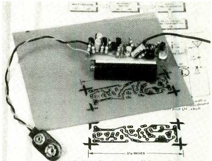
Fig. 5 The Tracking Transmitter was assembled on a small printed circuit board measuring only 2 1/2 inches long by 1 1/2 inches wide. Because of its size, the active components (all resistors and 11) must be mounted vertically.
