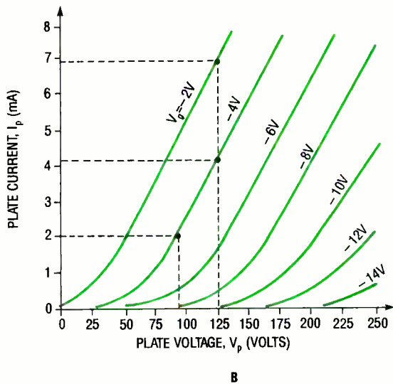
Fig. 6. The simple circuit in A can be used to characterize a triode by measuring its output voltage, and output current while adjusting its input voltage and load. the results are shown in B and C.
