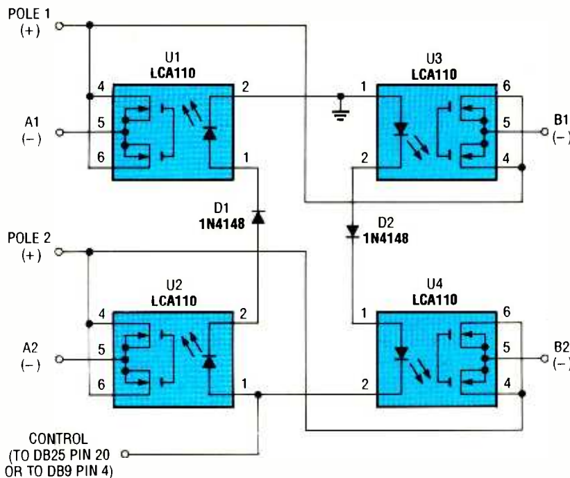
Fig. 3. The version of the A/B switch shown back in Fig. 2 is fine for AC signals, but it can be enhanced for DC operation by rewiring the optocoupler outputs as shown here.
