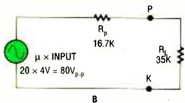
Fig. 8. Redrawing the triode amplifier so it appears as in A makes it easier to view as a signal generator with output impedance, as shown in B.
