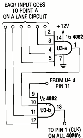
Fig. 5. Two gates are combined to form a larger AND gate, which is used to generate a clock pulse for each car as it crosses the finish line.
