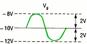
Fig. 9. With correct biasing, the quiescent output voltage should be right in the middle of the minimum and maximum output voltages (A). Incorrect biasing (B) leads to unsymmetrical waveforms and distortion.
