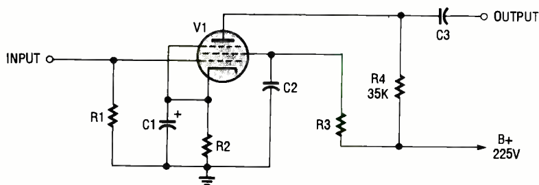
Fig. 16. In the pentode, a third grid, known as the suppressor, is fitted between the screen and plate. The suppressor prevents secondary electrons from the plate from reaching the screen.
