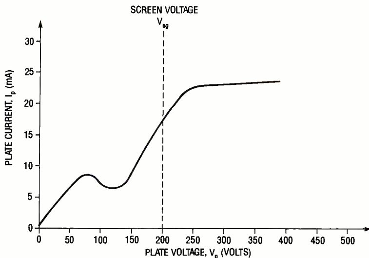
Fig. 15. Secondary emission produces a dip in the characteristic curve of a tetrode because of the presence of the screen grid. Obviously, that is therefore not a problem with a triode
