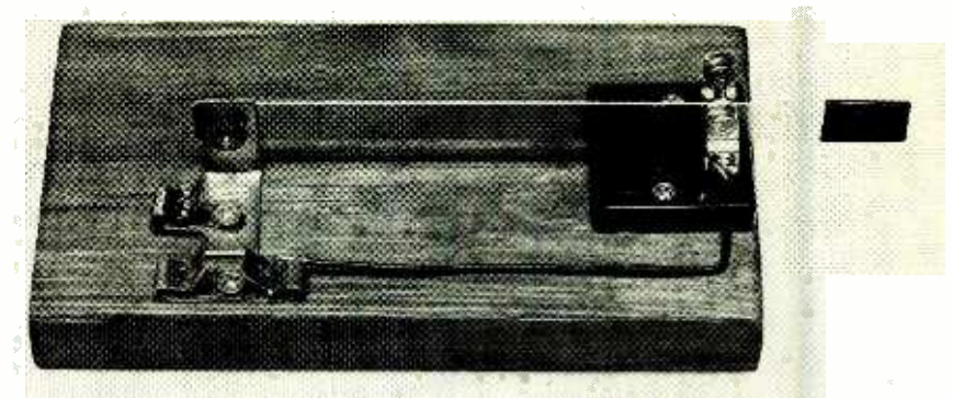
The Sideswiper is no longer made, but it is was the first of the high speed code keys. It's as easy to build as it is to use, and you can get all the parts at a hardware store!
