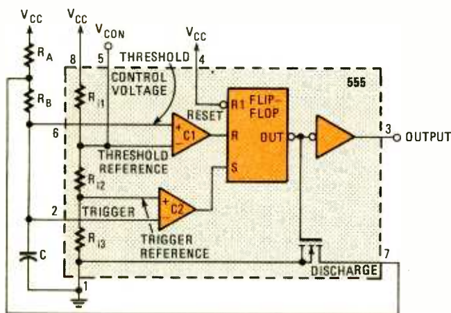
Fig. 1. Shown here are the basic building blocks of the 555 timer IC accompanied by a few external timing components.
