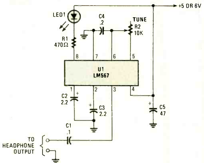
Fig. 8. By connecting this circuit to the headphone jack of a general-coverage communications receiver, hearing-impaired hams can continue to enjoy their hobby.
