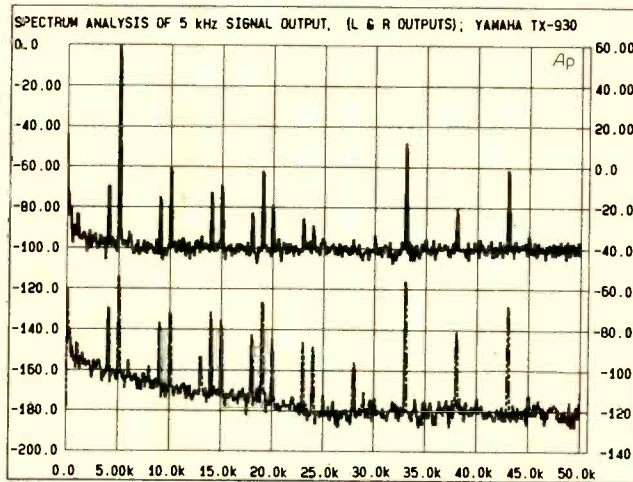
Spectrum analysis of left (solid line) and right (dashed line) outputs when a 5-kHz signal is input only to the left channel. Use the right-hand scale to read the crosstalk and distortion levels.
