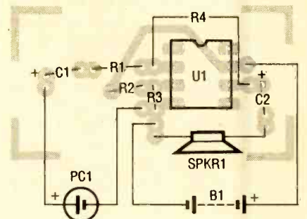
Fig. 6. Be careful when assembling the receiver circuit: some solar cells are extremely fragile, and are easily damaged by heat and other stress.
