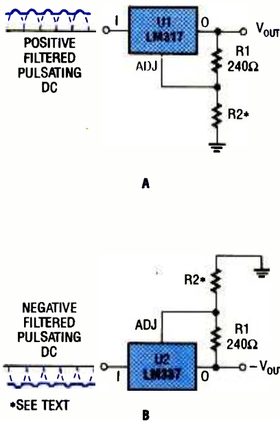
Fig. 1. Adjustable regulators are easy to use. Whether you need a positive (A) or a negative (B) output voltage, you just have to add two resistors and a filtered source of pulsating DC.
