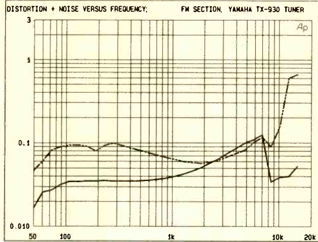
The THD figures were quite low when the receiver was in the wide-IF mode. The solid line is mono; the dashed line is stereo.
