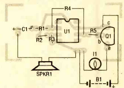
Fig. 5. Assemble the transmitter's printed-circuit board using this parts placement diagram as a guide.
