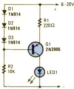
Fig. 3. With only a slight change in output brilliance, this pilot circuit can be used as an indicator for DC sources that vary in voltage from 6 to 20-volts.
