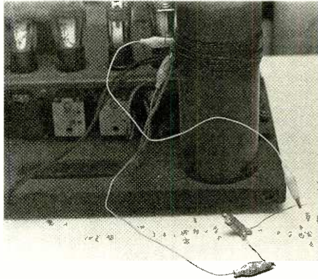
The test lamp, in holder, is clipped to the terminals of the pickup loop for volume-control tube filament voltage.
