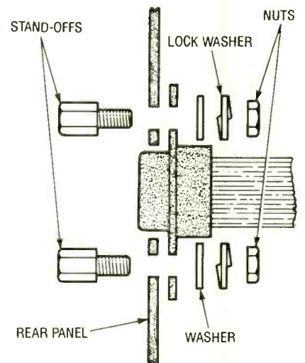
Fig. 5. Use these mounting details for the Video and SCSI connectors. It's a good idea to mount them onto the back panel before installing the motherboard.
