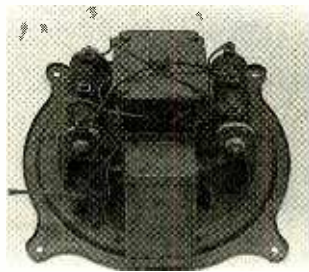
The model 106 speaker was removed from its cabinet to check its cone. Note the two cylindrical copper-oxide rectifier stacks.
