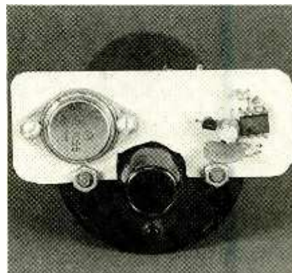
Here is the Laser Power Supply board mounted to the auto ignition coil. Note that the board is held in place by screws on the coil's positive and negative power-input terminals. Those screws also make electrical connection from the board to the coil.
