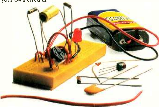
With your first module you'll use this solderless breadboarding system. As you add additional boards to create your Explorer Design Lab you retain the ability to connect and build increasingly complex circuits easily and quickly.
