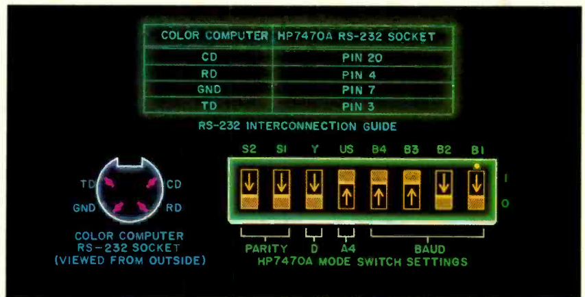
Fig. 6. How to connect a plotter to the Color Computer.
