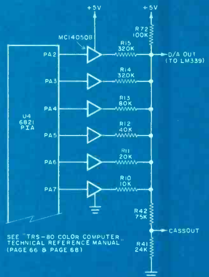
Fig. 2. D/A converter circuit.
