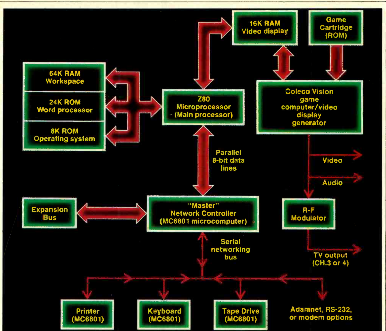
Block diagram of Adam's "central nervous system."
