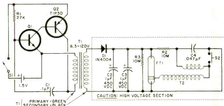
Fig. 9. Single-flash xenon strobe circuit.
