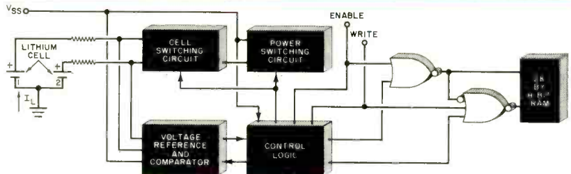
Fig. 5. Block diagram (above) of Mostek's lithium-cell RAM.
