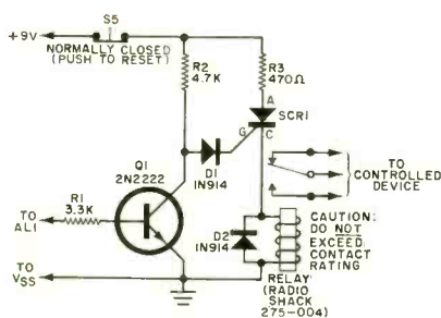
Fig. 8. Output interface for clock module.
