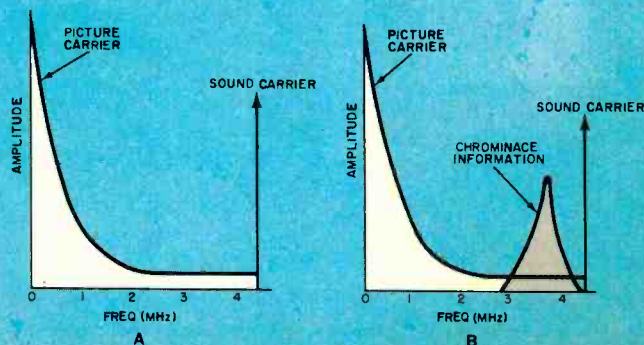
Fig. 3. Envelopes of (A) monochrome signal and (B) with chrominance added. Energy is actually bunched at intervals of horizontal scanning rate of 15,750 Hz to give an interleaving effect and avoid interference.
