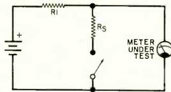
Fig. 1. Circuit for determining meter resistance using two precision resistors.
